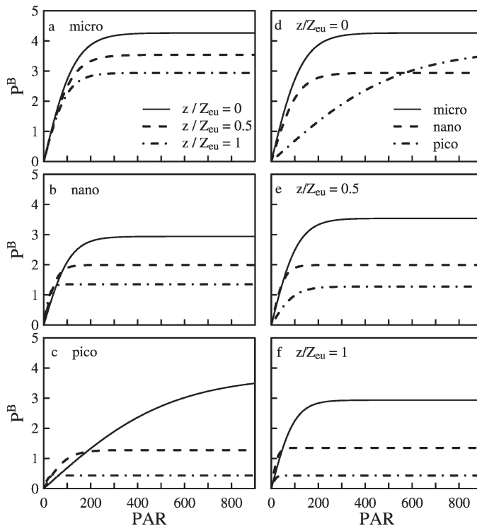
Fig. 5. P^B [mg C (mg Chl a ) ^{-1} h ^{-1} ] versus PAR ( \mu mol quanta m ^{-2} s ^{-1} ) curves reconstructed for the three phytoplankton pigment-based size classes for three different depths. (a–c) for each phytoplankton class at z/Z_{eu} = 0 (solid lines), z/Z_{eu} = 0.5 (dashed lines), and z/Z_{eu} = 1 (dotted lines). (d–f) At each depth, for micro- (solid lines), nano- (dashed lines), and picophytoplankton (dotted lines). The curves are reconstructed using the parameters listed in Table 4.
