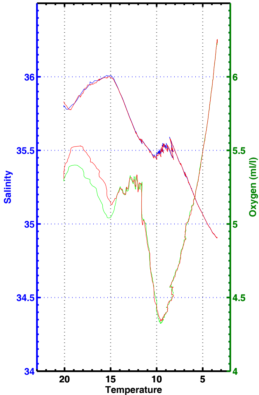
T-S , T-02 , station 3062
