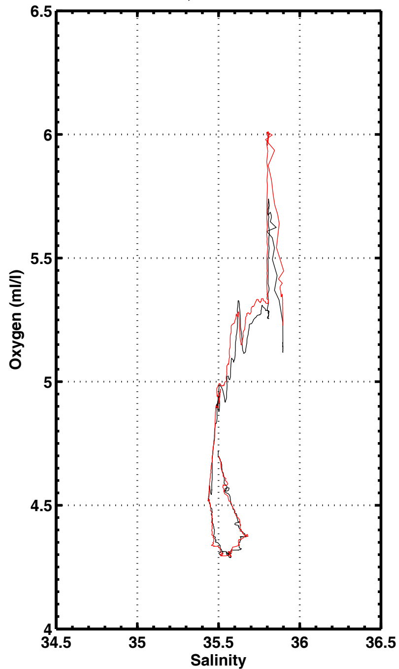
S-O2 , station 3244
