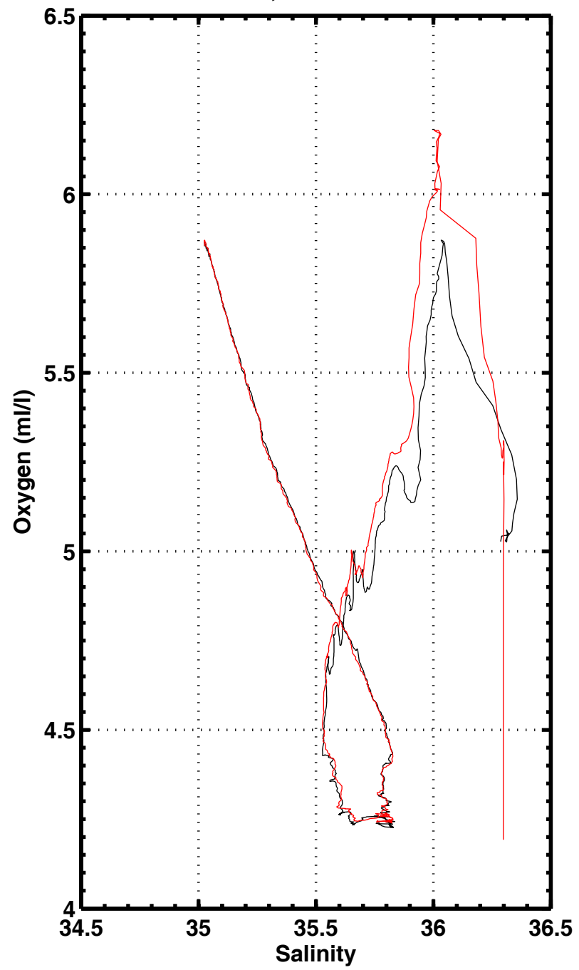
S-O2 , station 3082
