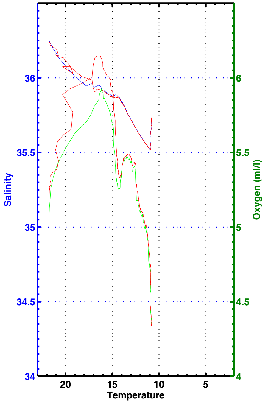
T-S , T-02 , station 3095
