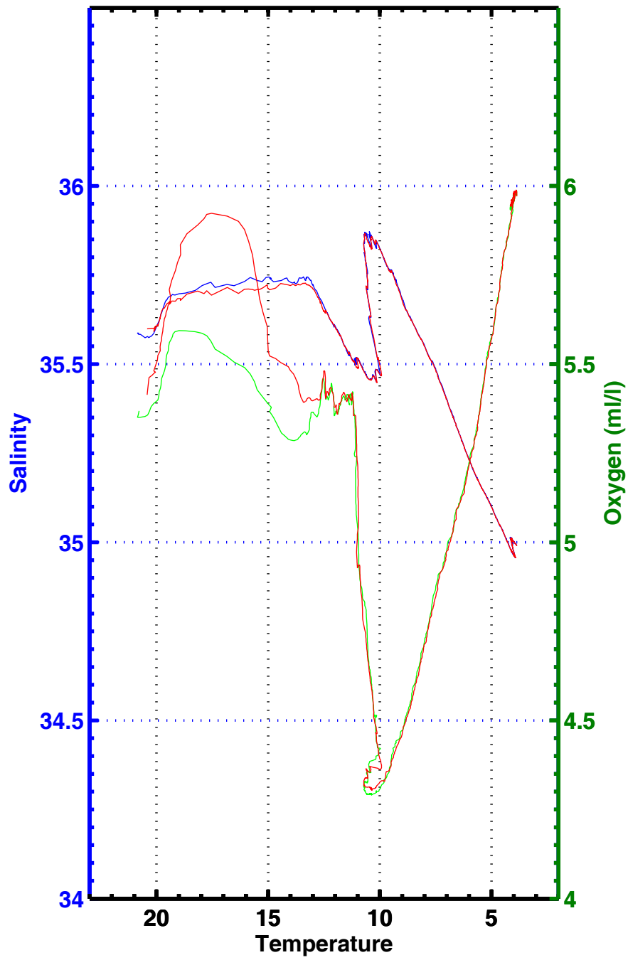
T-S , T-02 , station 3028
