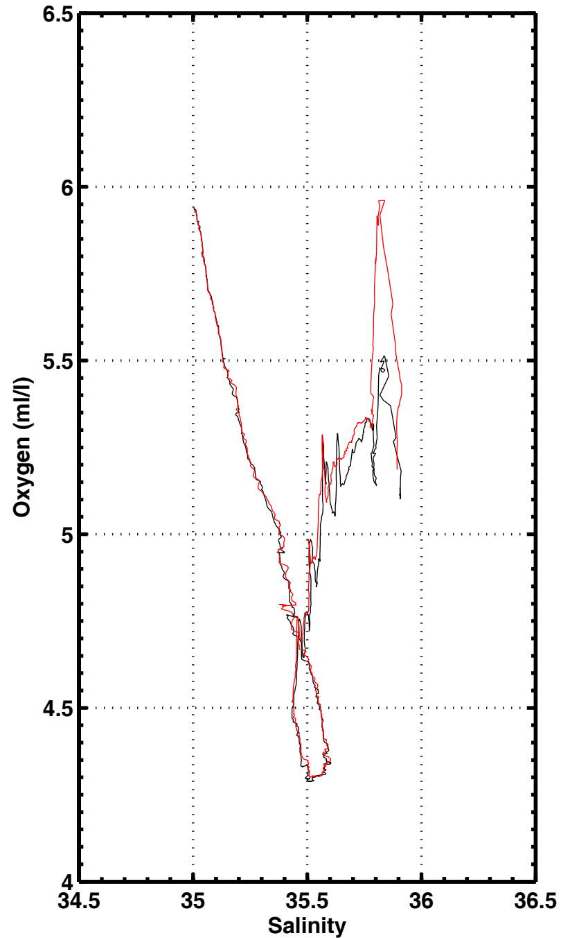
S-O2 , station 3239
