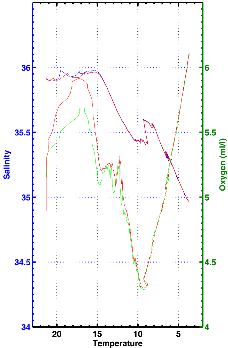
T-S , T-02 , station 3052
