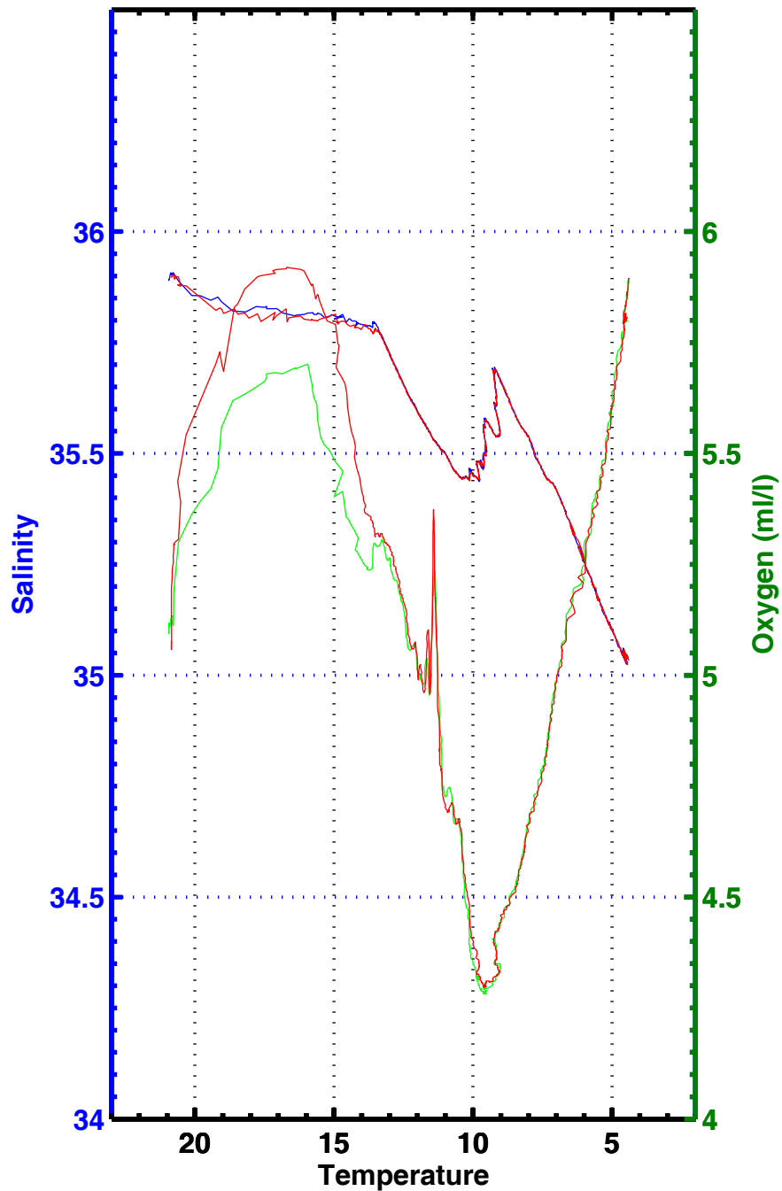
T-S , T-02 , station 3251
