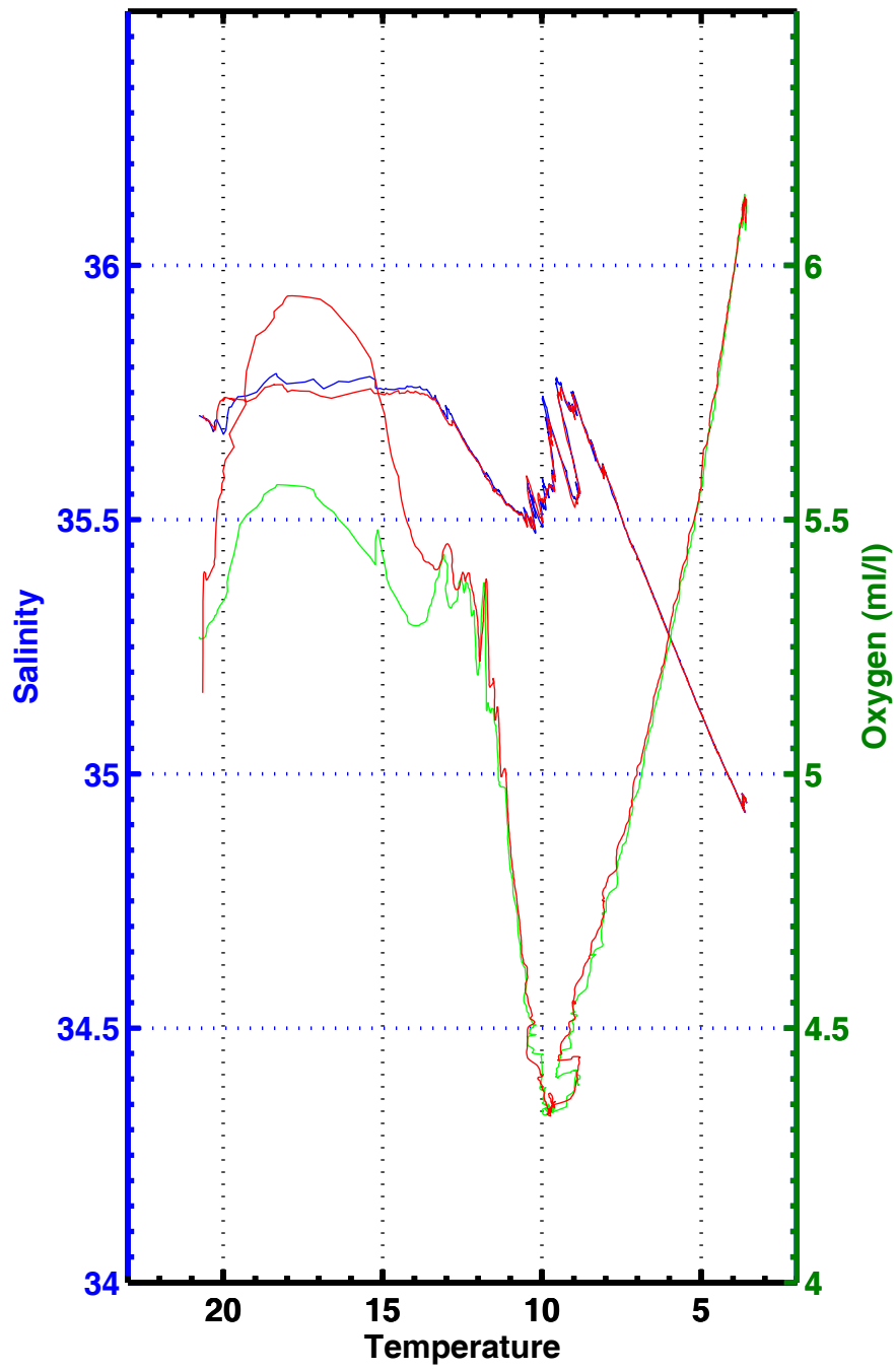
T-S , T-02 , station 3029
