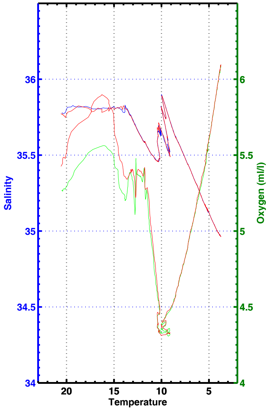
T-S , T-02 , station 3022
