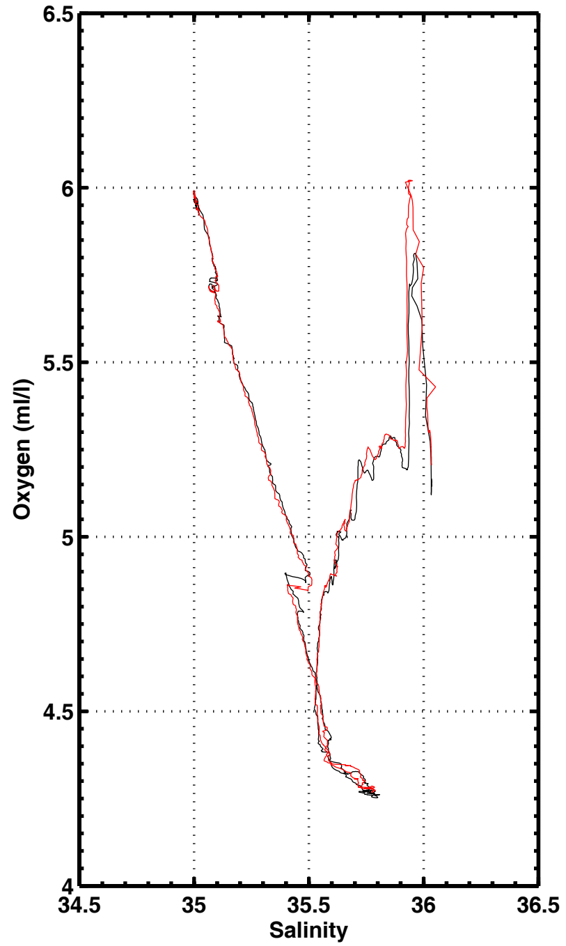
S-O2 , station 3047
