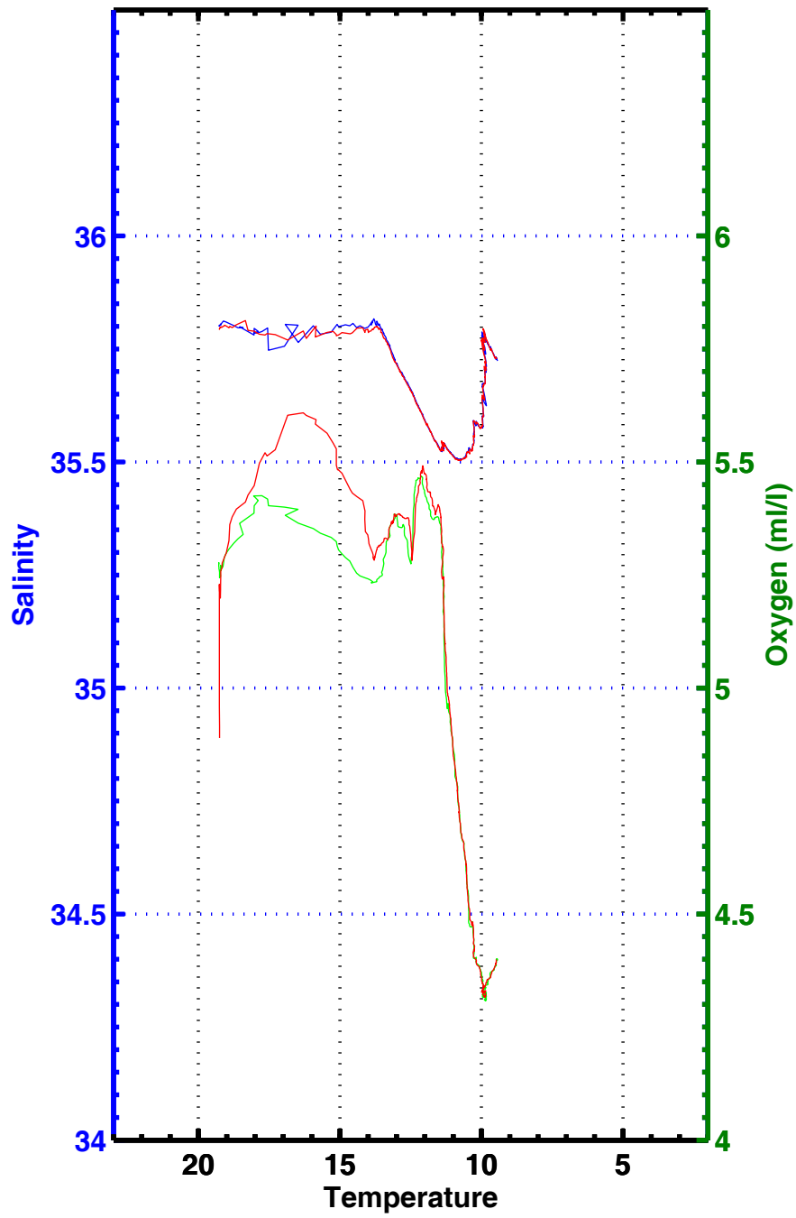
T-S , T-02 , station 3326
