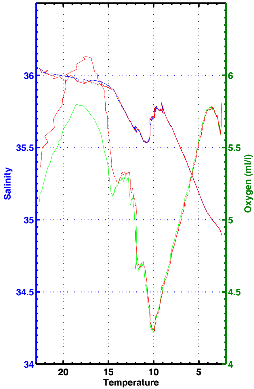
T-S , T-02 , station 3036
