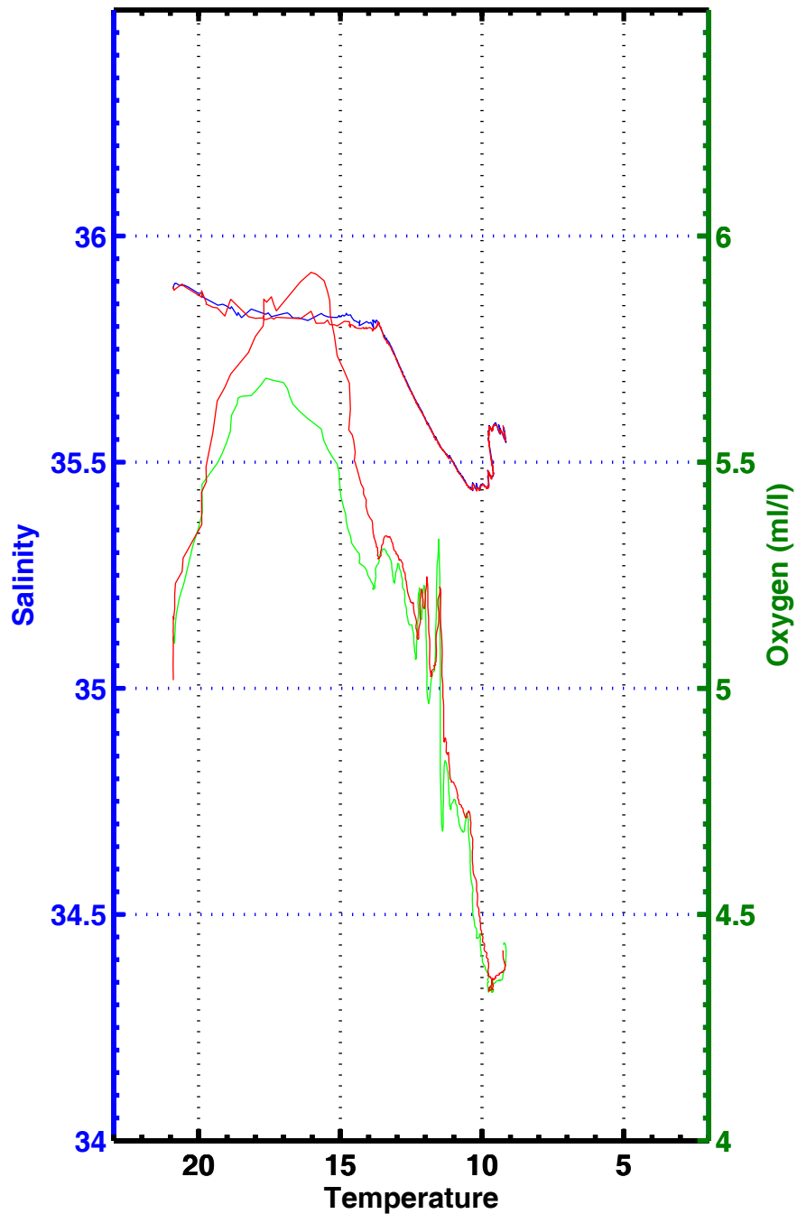
T-S , T-02 , station 3248
