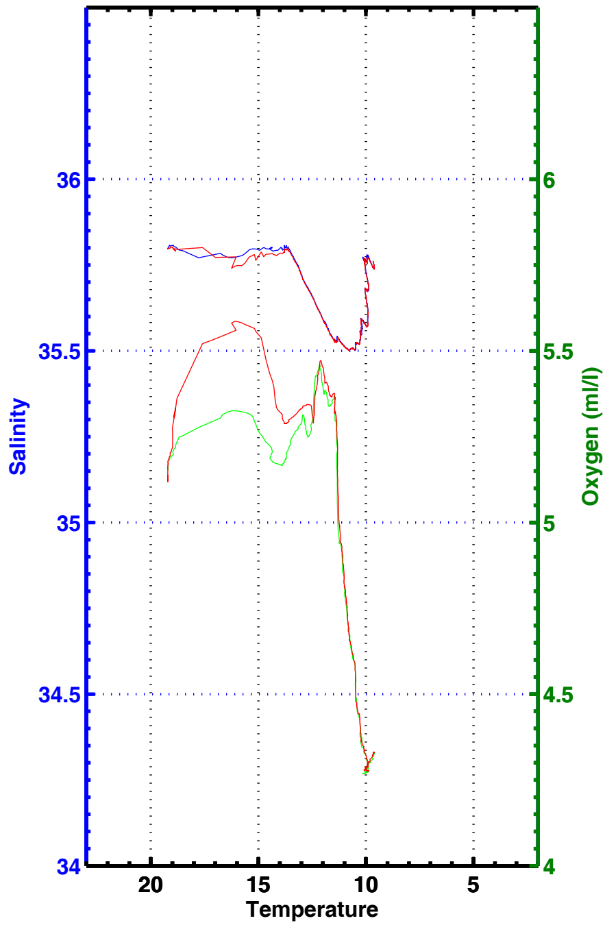
T-S , T-02 , station 3328
