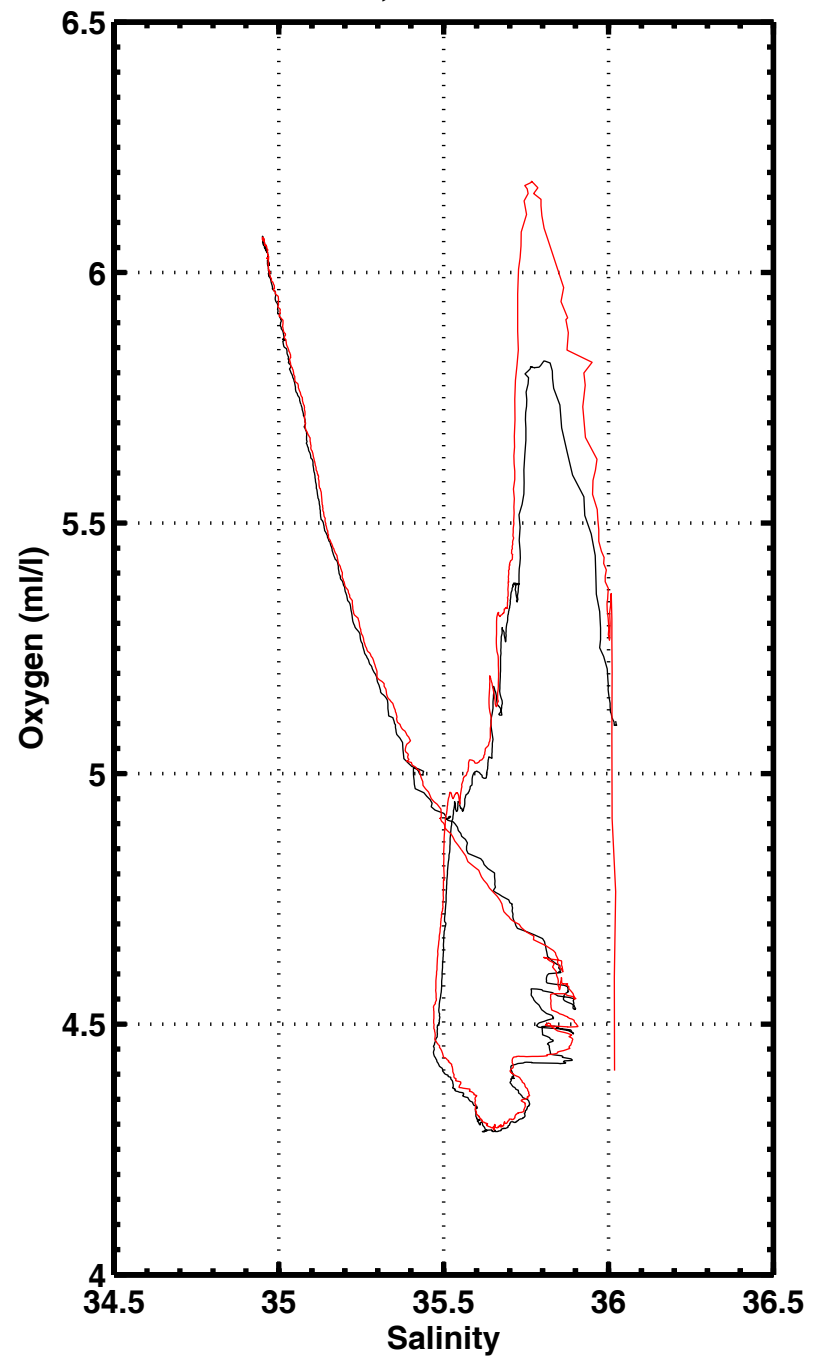
S-02 , station 3016
