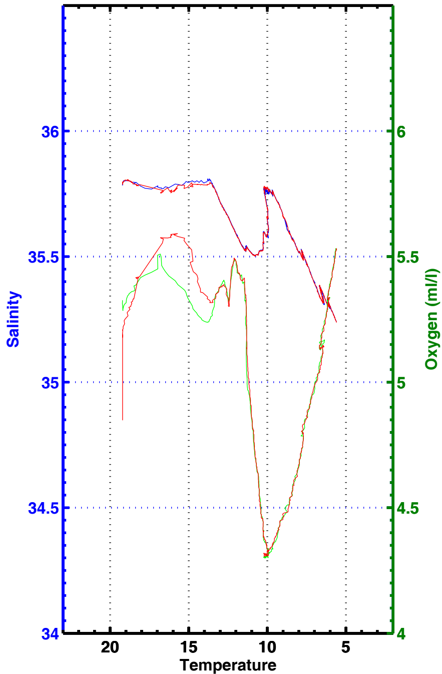
T-S , T-02 , station 3327
