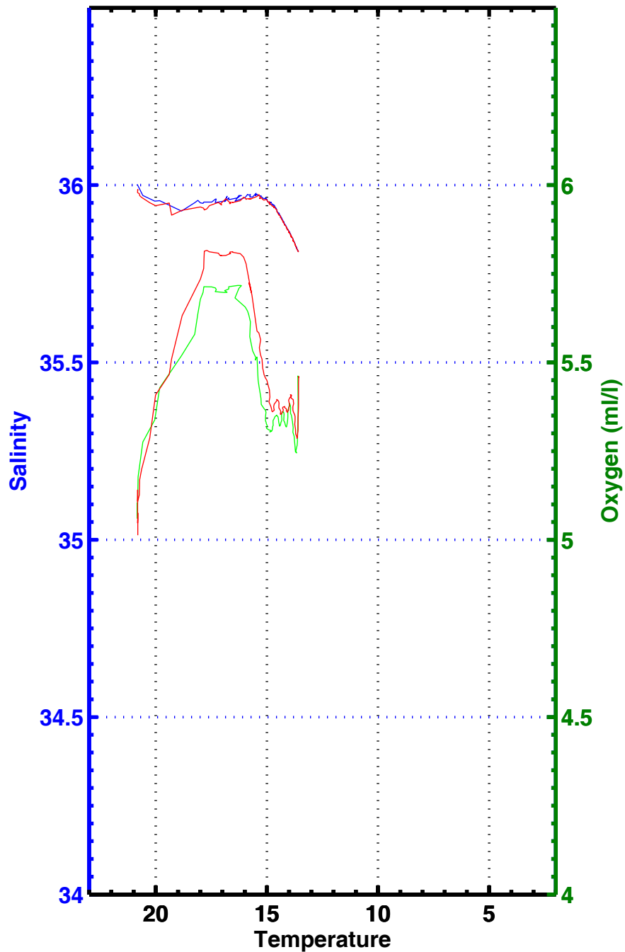
T-S , T-02 , station 3165
