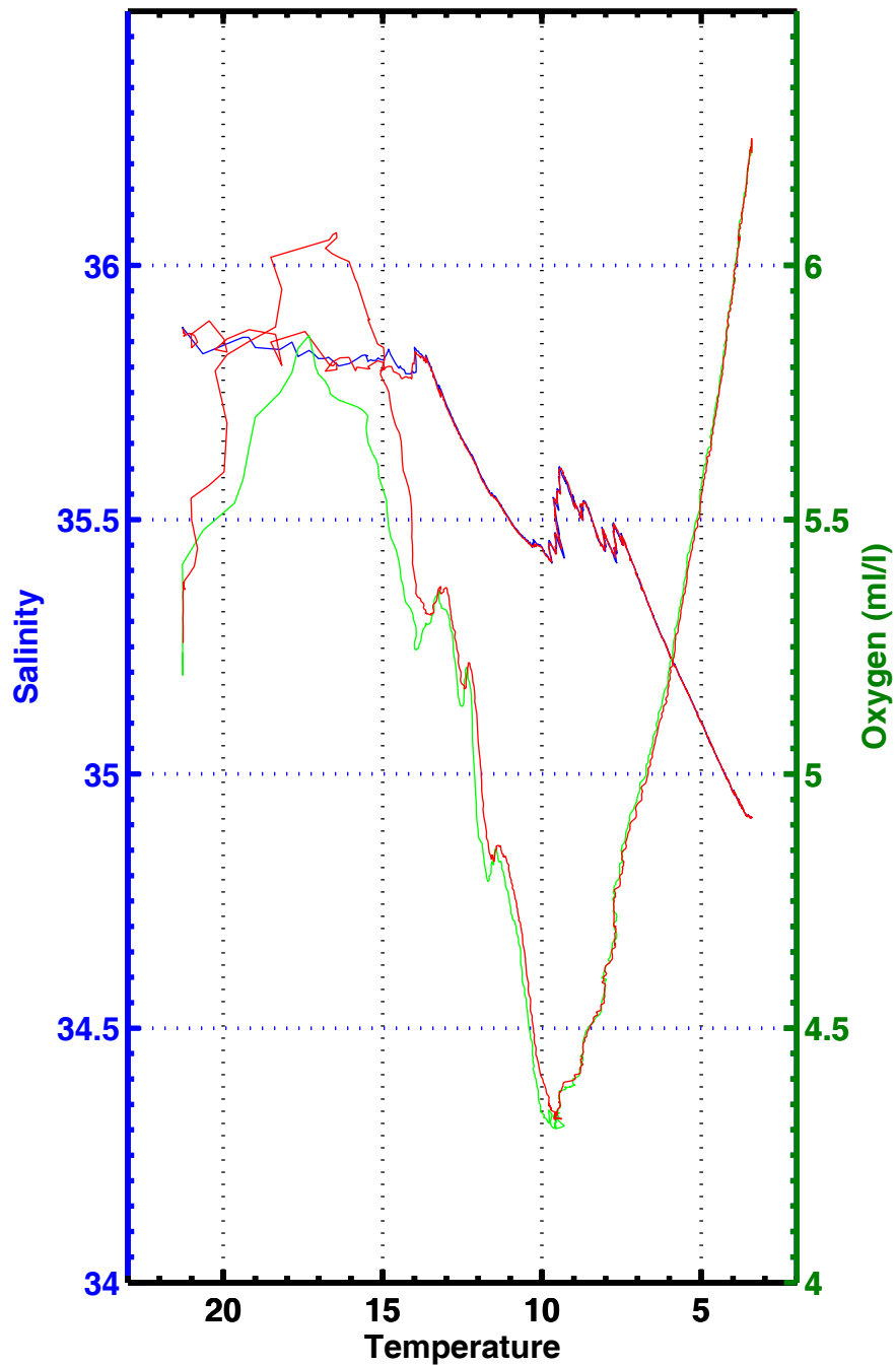
T-S , T-02 , station 3072
