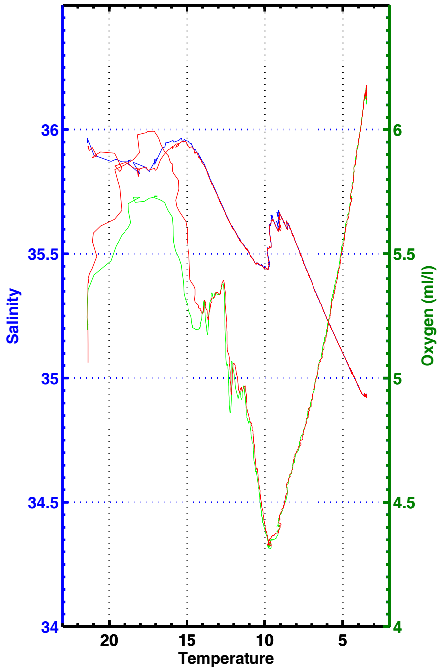
T-S , T-02 , station 3075
