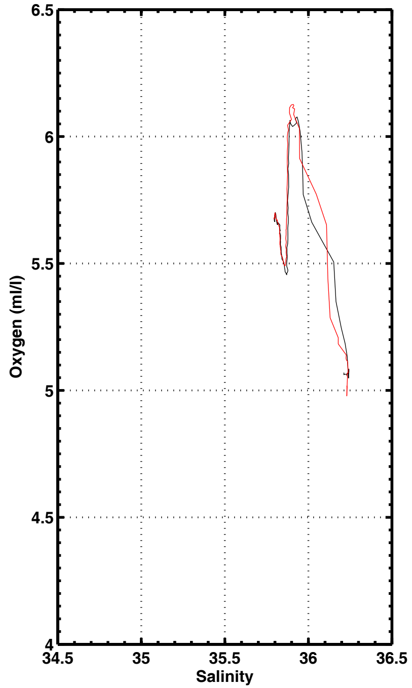
S-02 , station 3096
