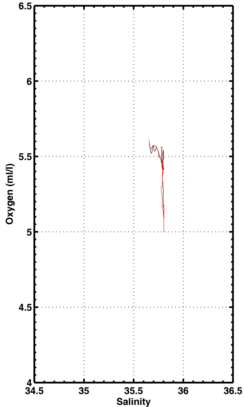
S-02 , station 3330
