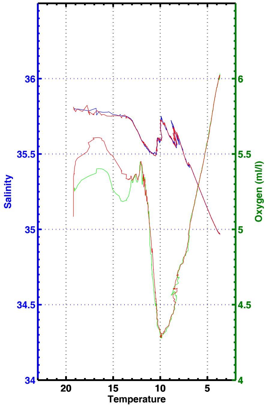
T-S , T-02 , station 3336
