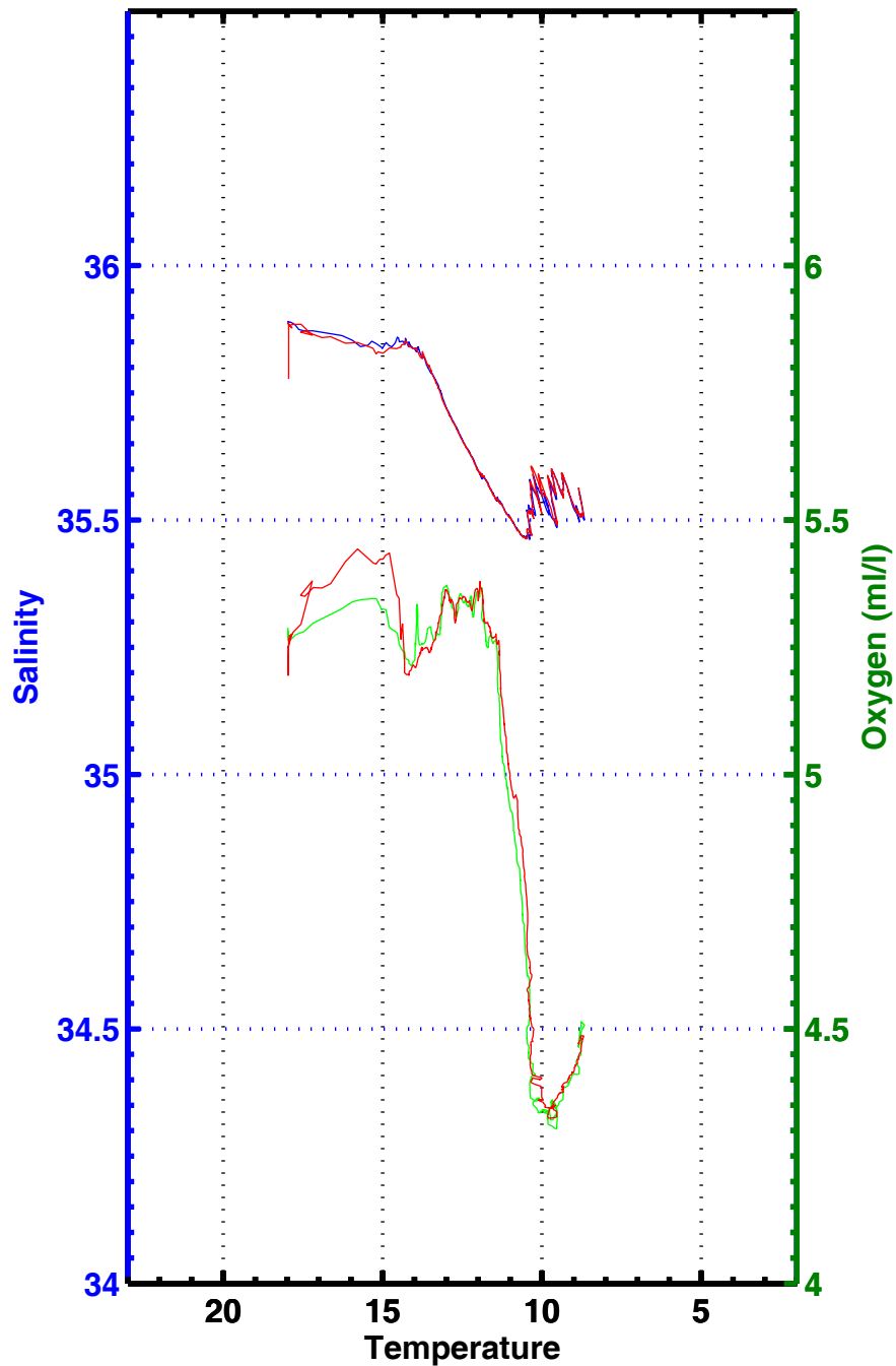
T-S , T-02 , station 3338
