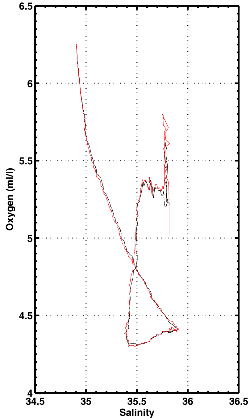
S-O2 , station 3051
