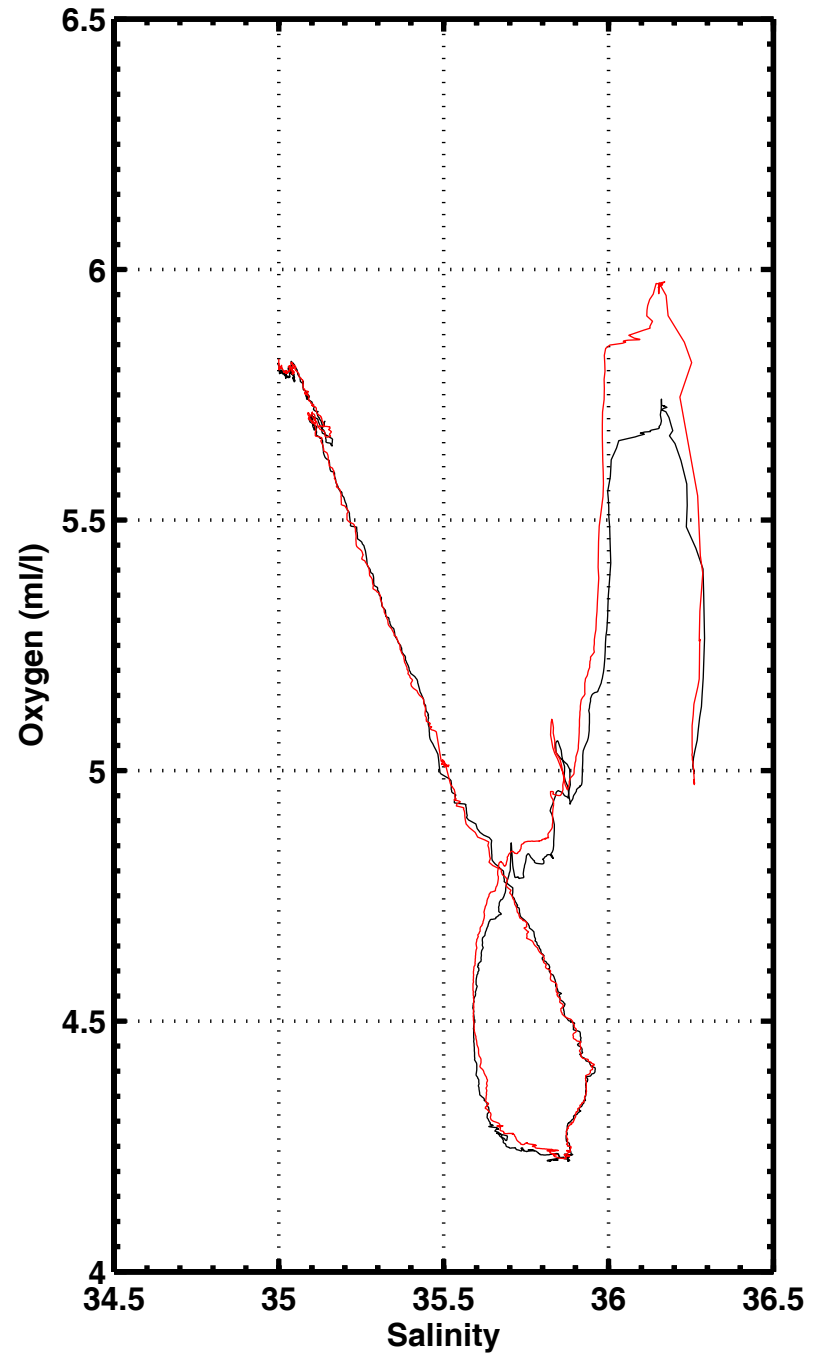
S-O2 , station 3013
