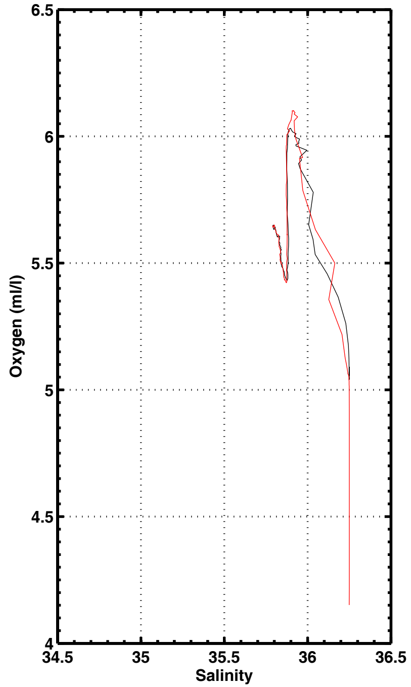
S-02 , station 3093
