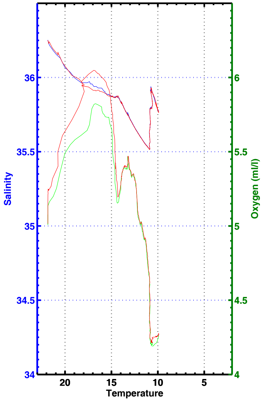
T-S , T-02 , station 3088
