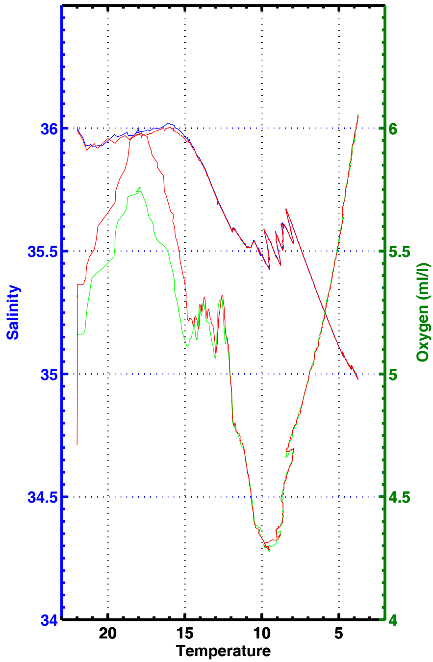
T-S , T-02 , station 3077
