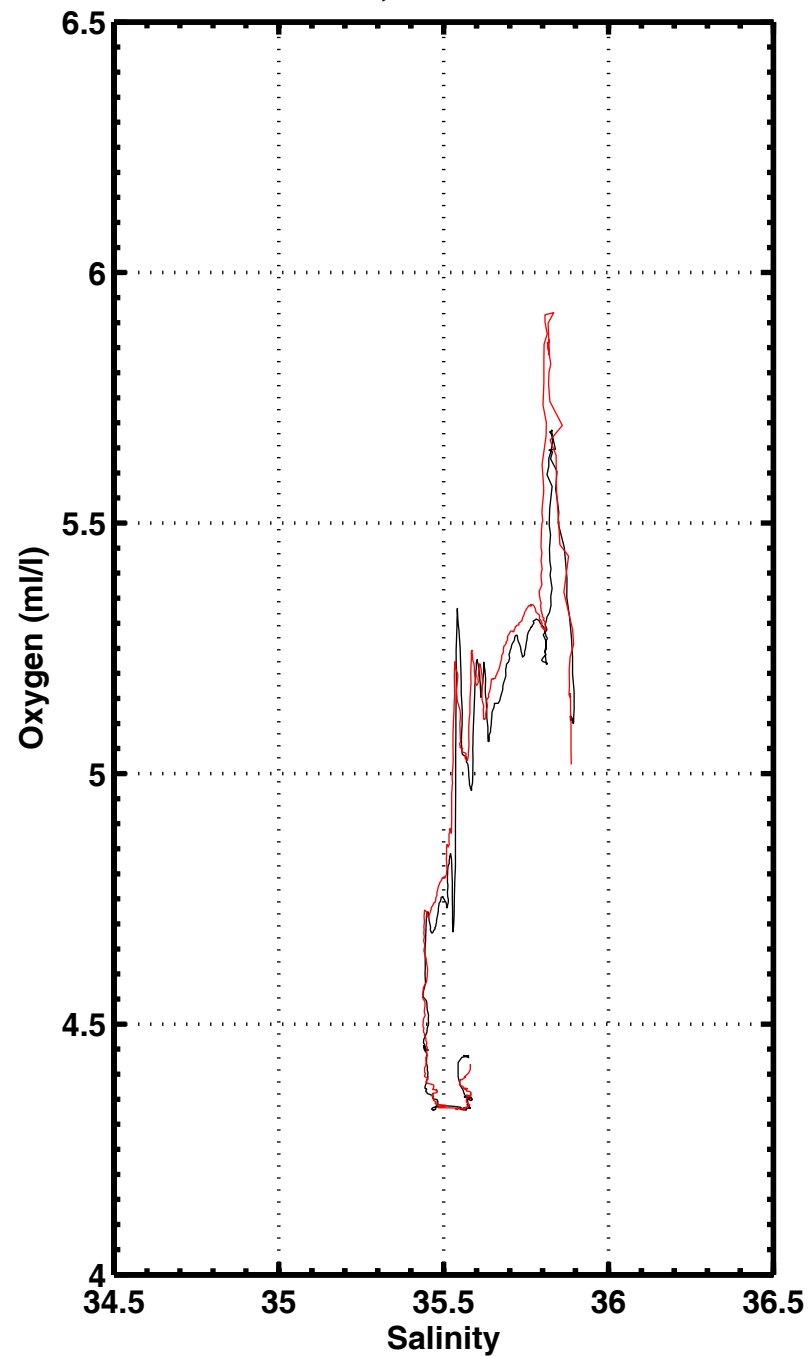
S-O2 , station 3248
