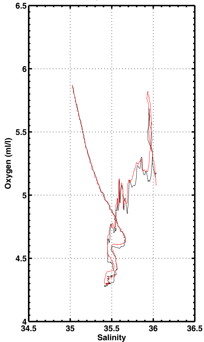
S-O2 , station 3167
