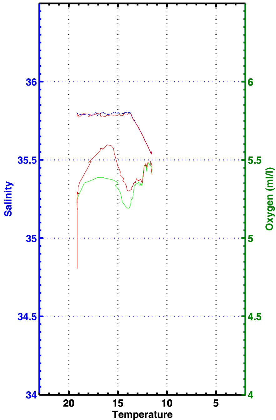
T-S , T-02 , station 3329
