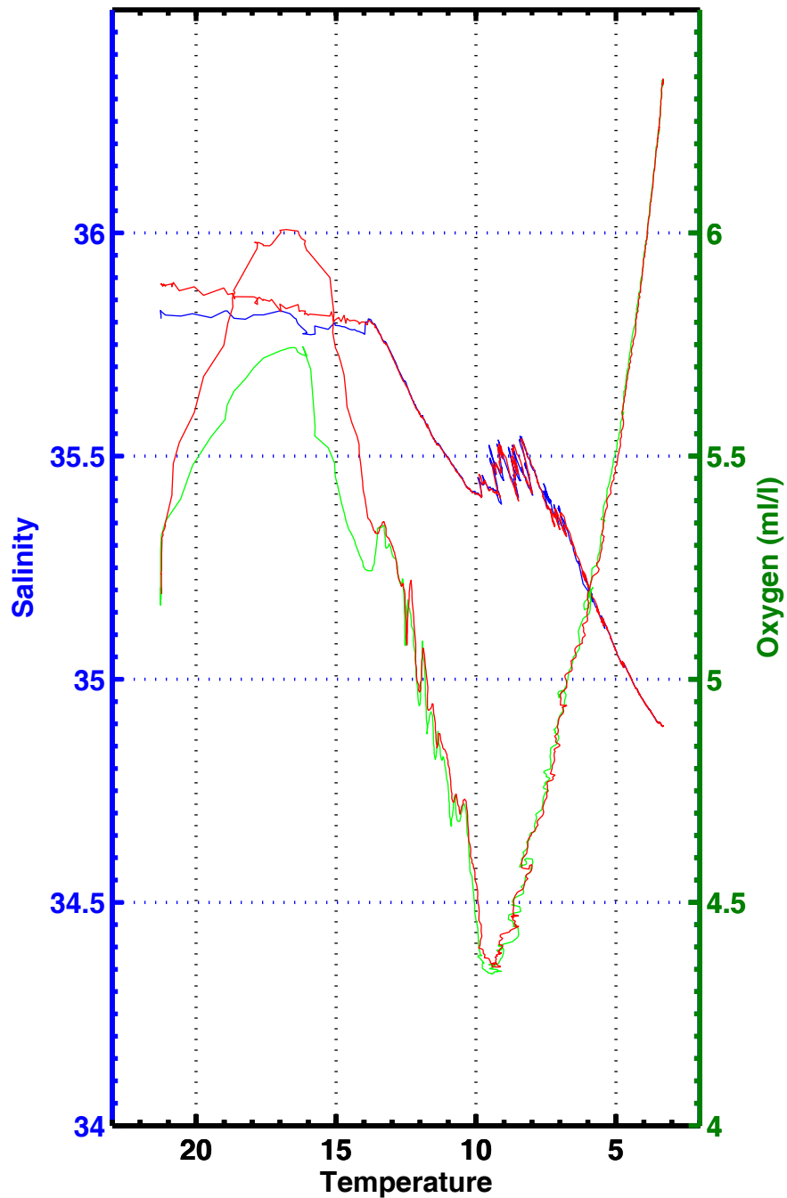
T-S , T-02 , station 3071
