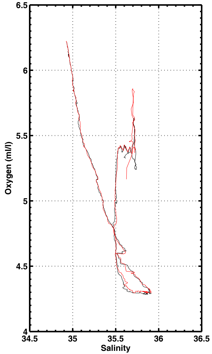
S-02 , station 3021
