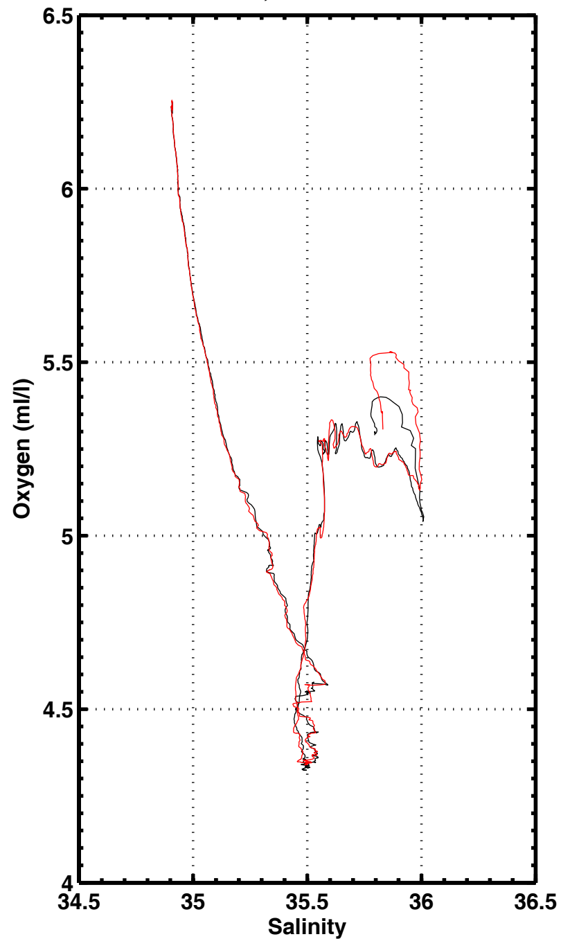
S-O2 , station 3062
