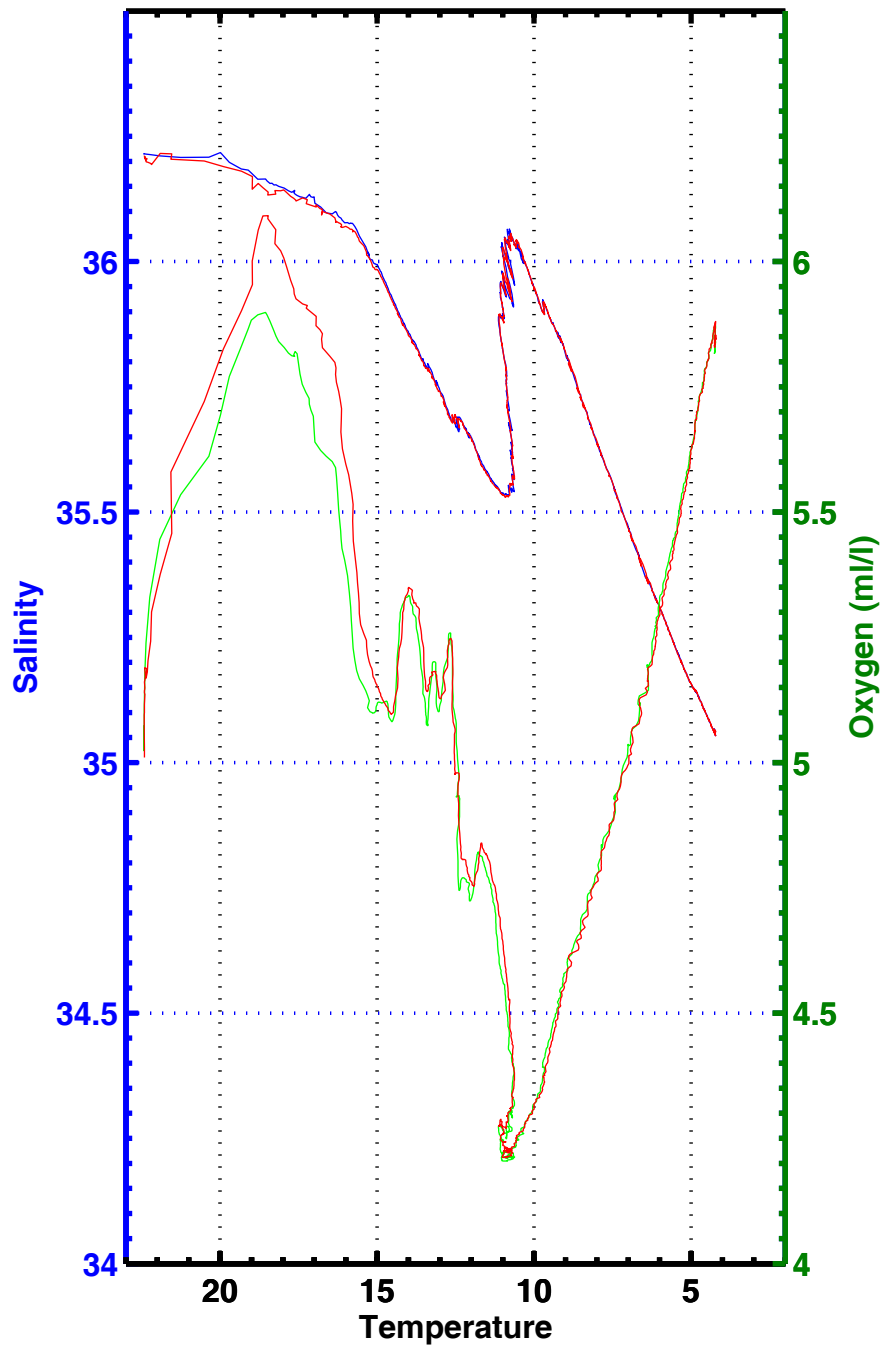
T-S , T-02 , station 3044
