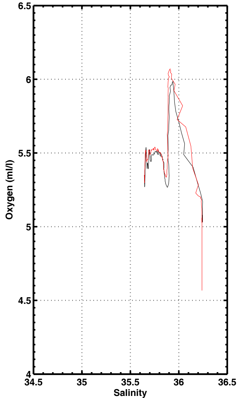
S-02 , station 3092
