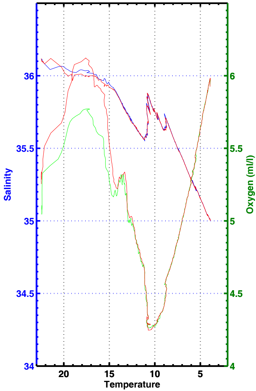
T-S , T-02 , station 3040
