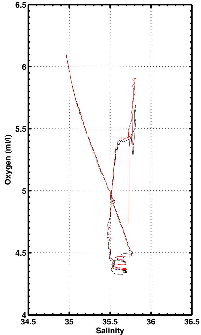
S-O2 , station 3065
