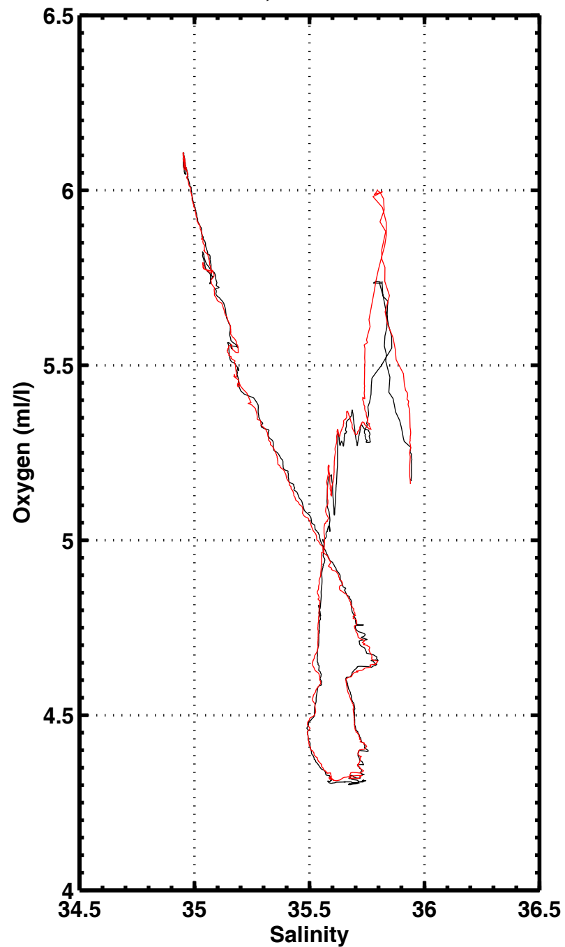
S-O2 , station 3017
