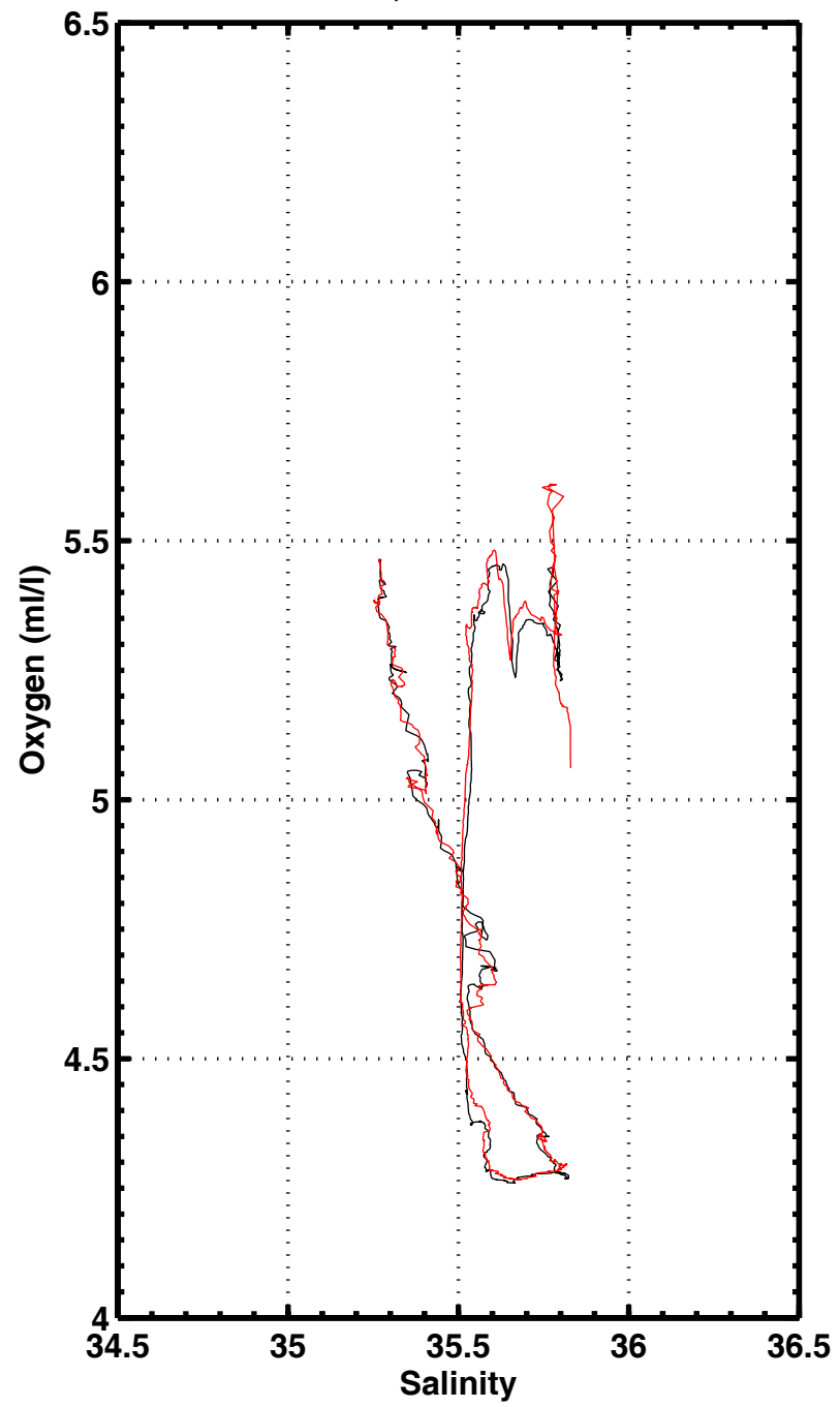
S-O2 , station 3334
