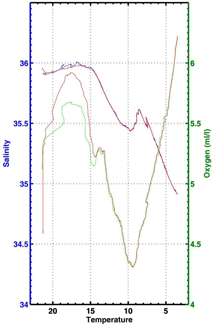
T-S , T-02 , station 3048
