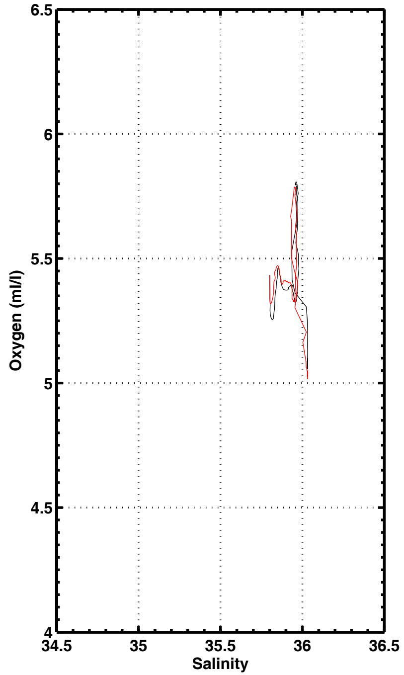
S-02 , station 3163
