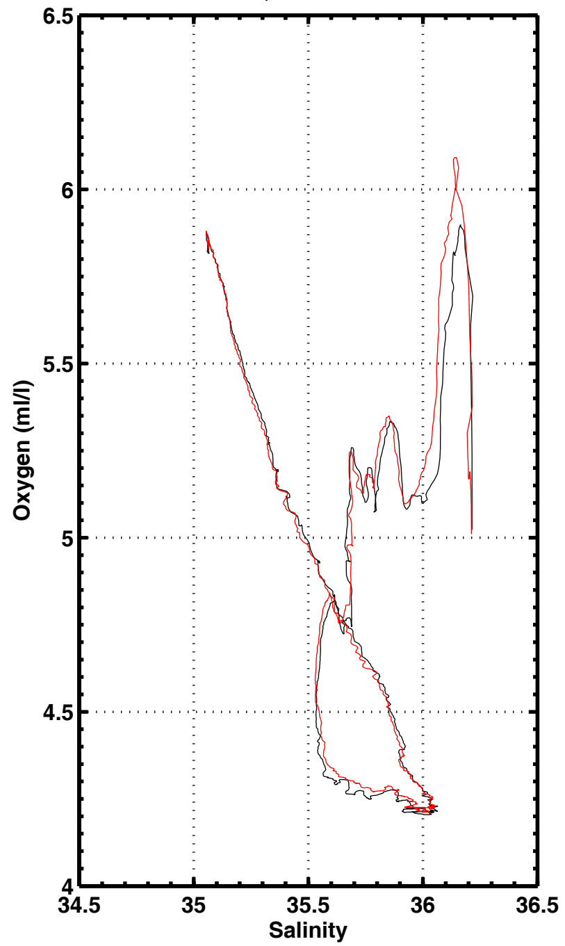
S-O2 , station 3044
