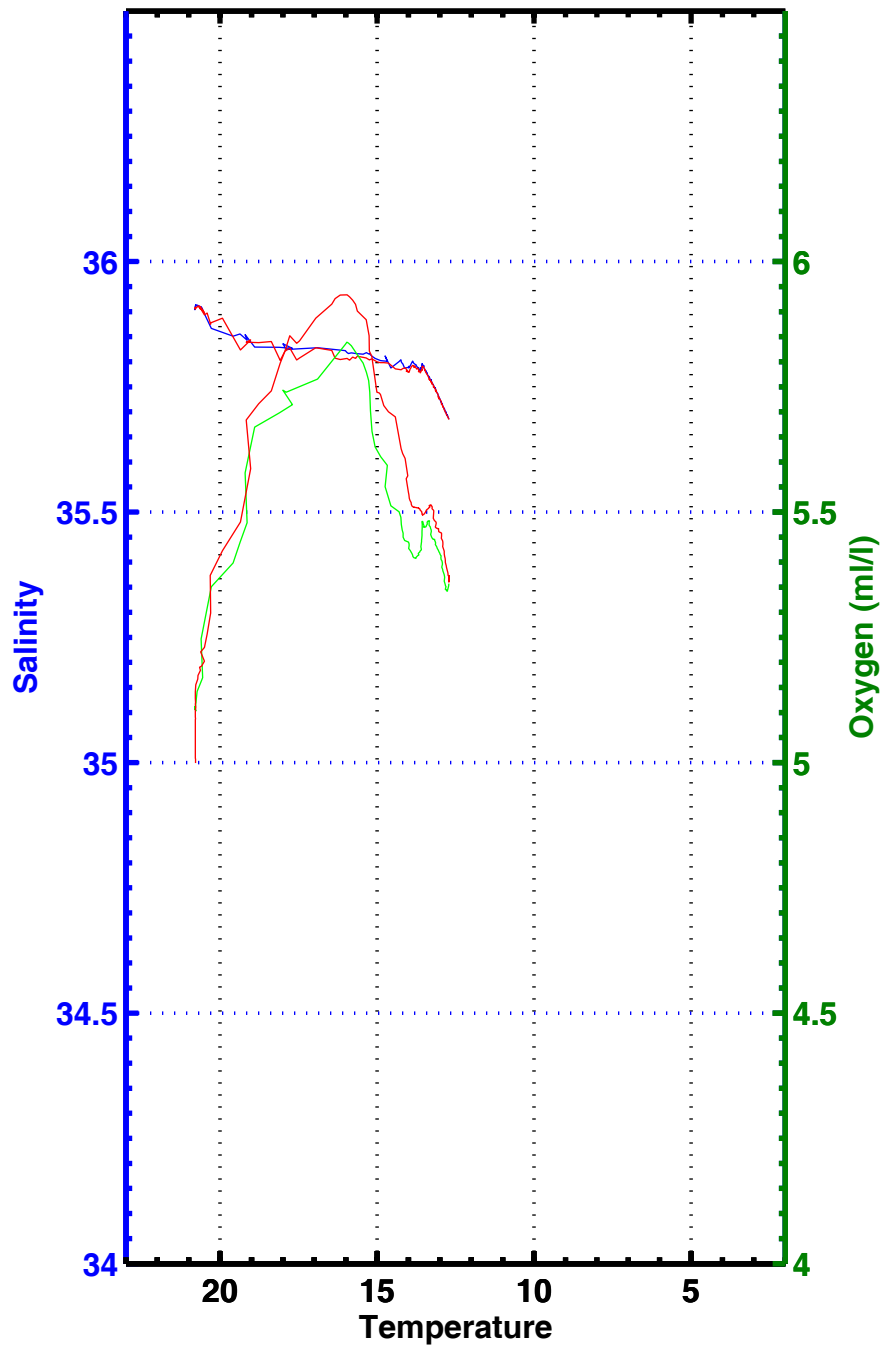
T-S , T-02 , station 3240
