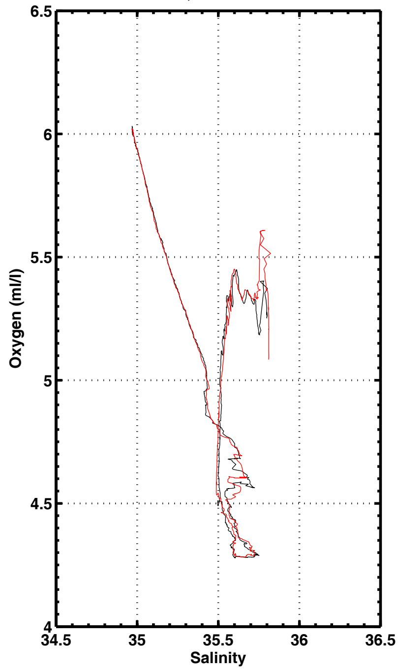
S-O2 , station 3336
