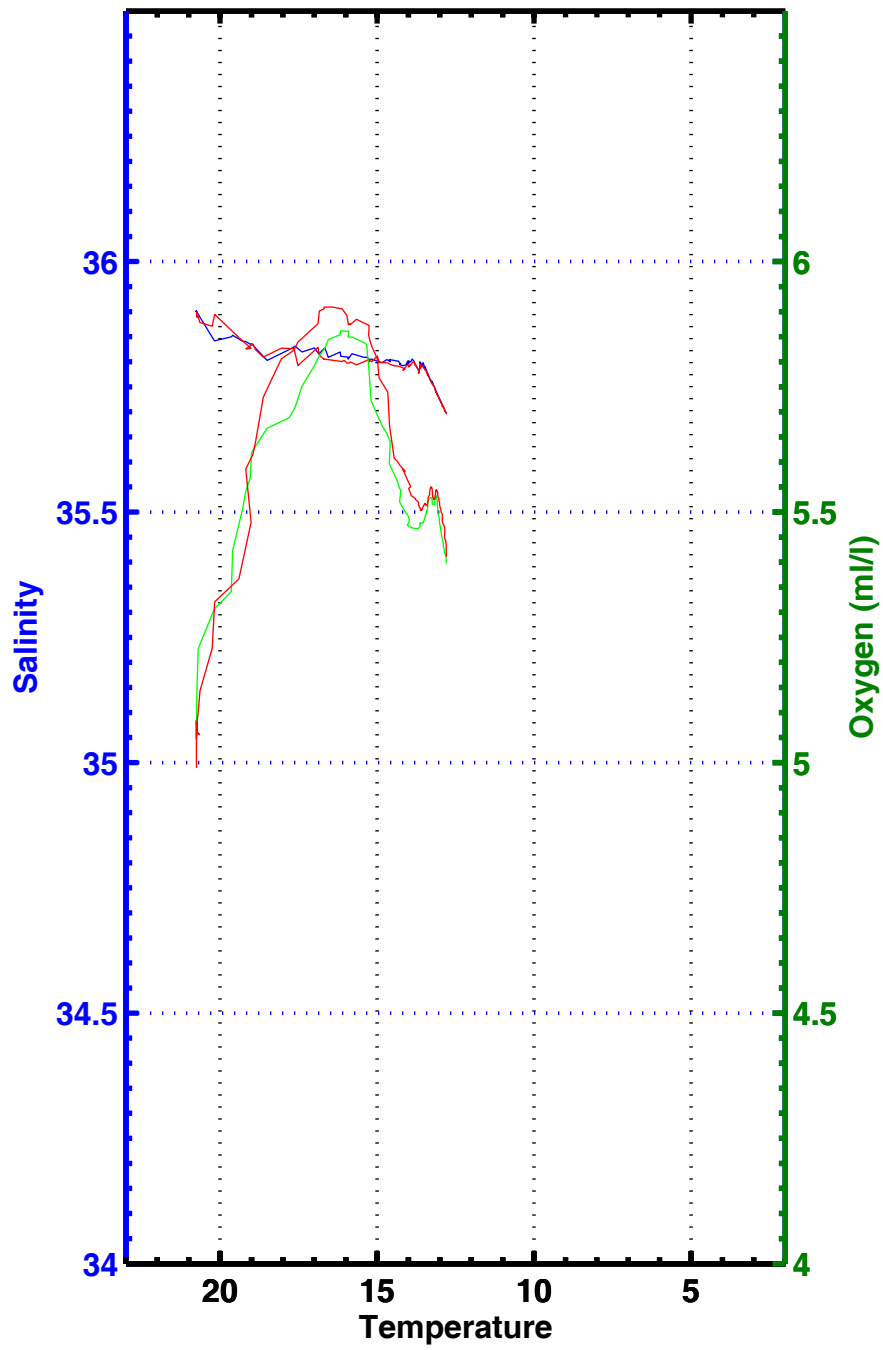
T-S , T-02 , station 3249
