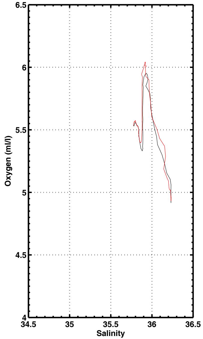
S-02 , station 3086
