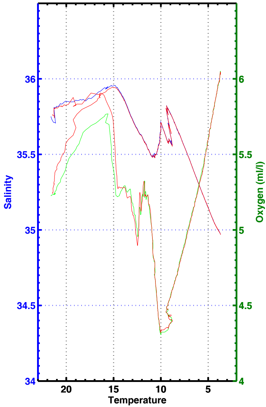
T-S , T-02 , station 3020
