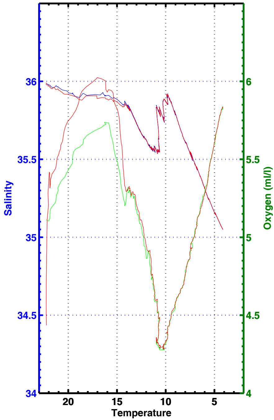
T-S , T-02 , station 3018
