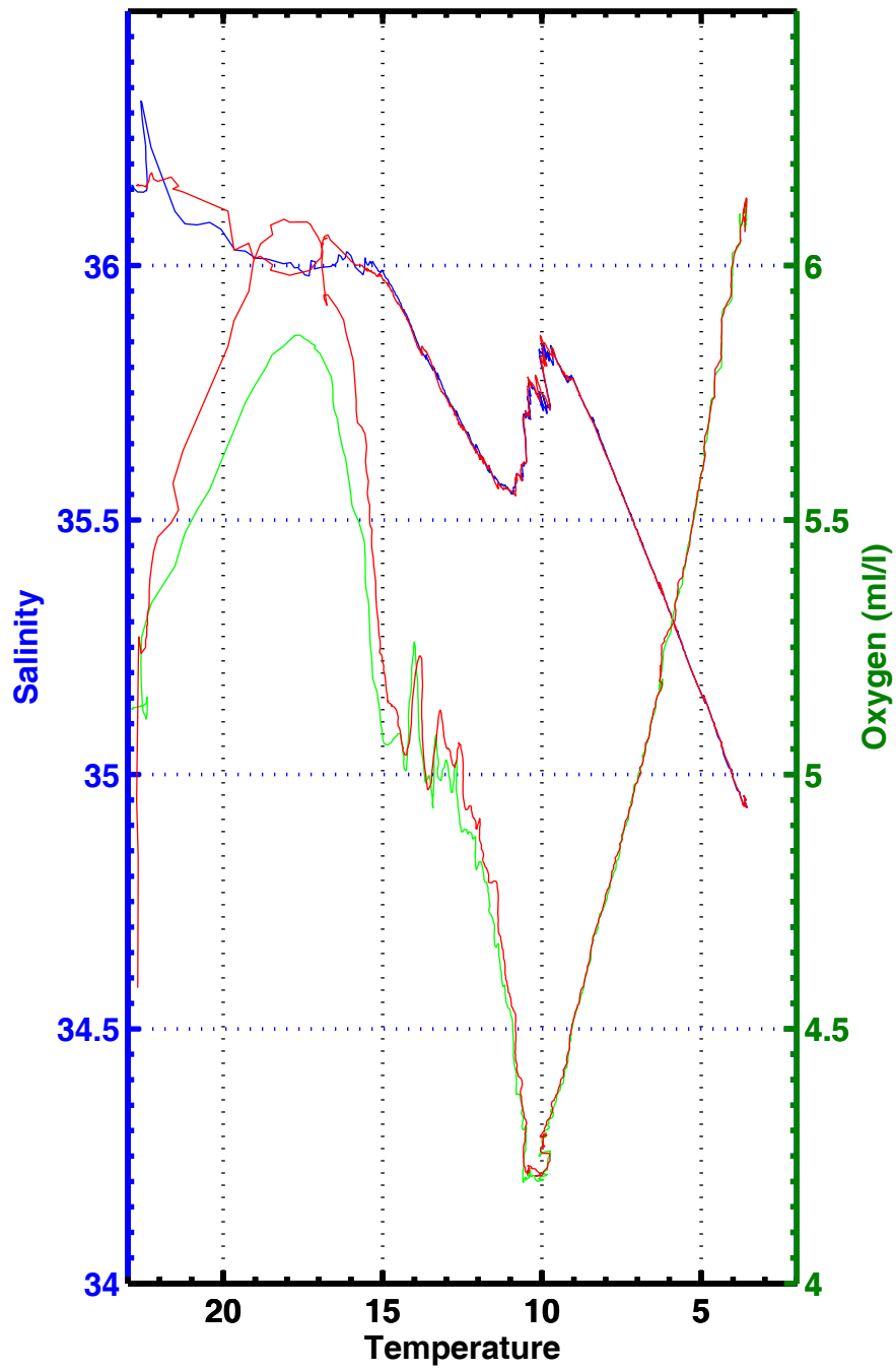
T-S , T-02 , station 3079
