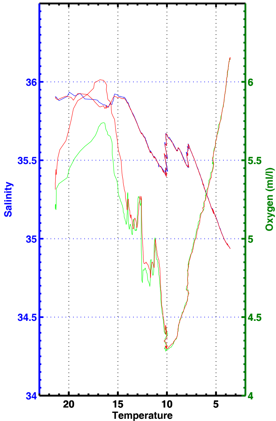
T-S , T-02 , station 3058
