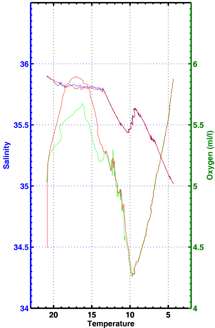
T-S , T-02 , station 3243
