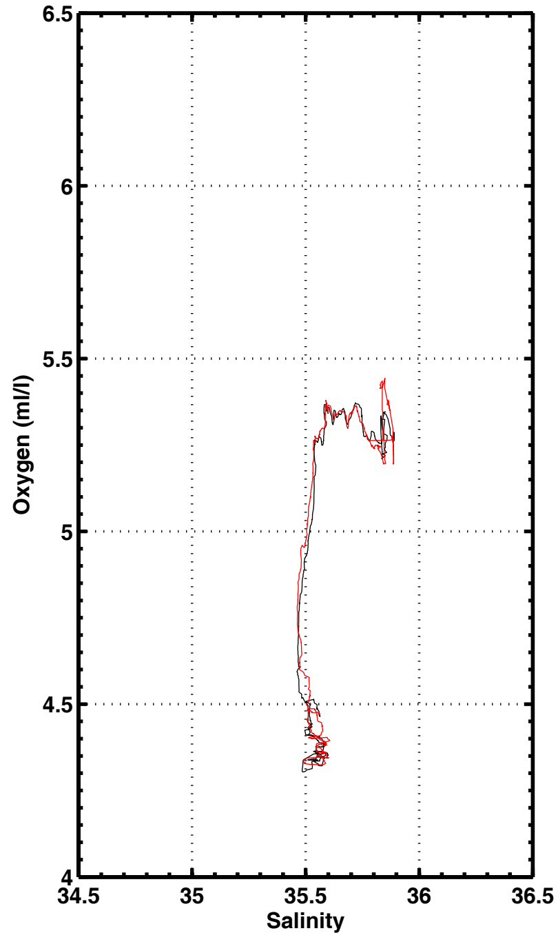
S-02 , station 3338
