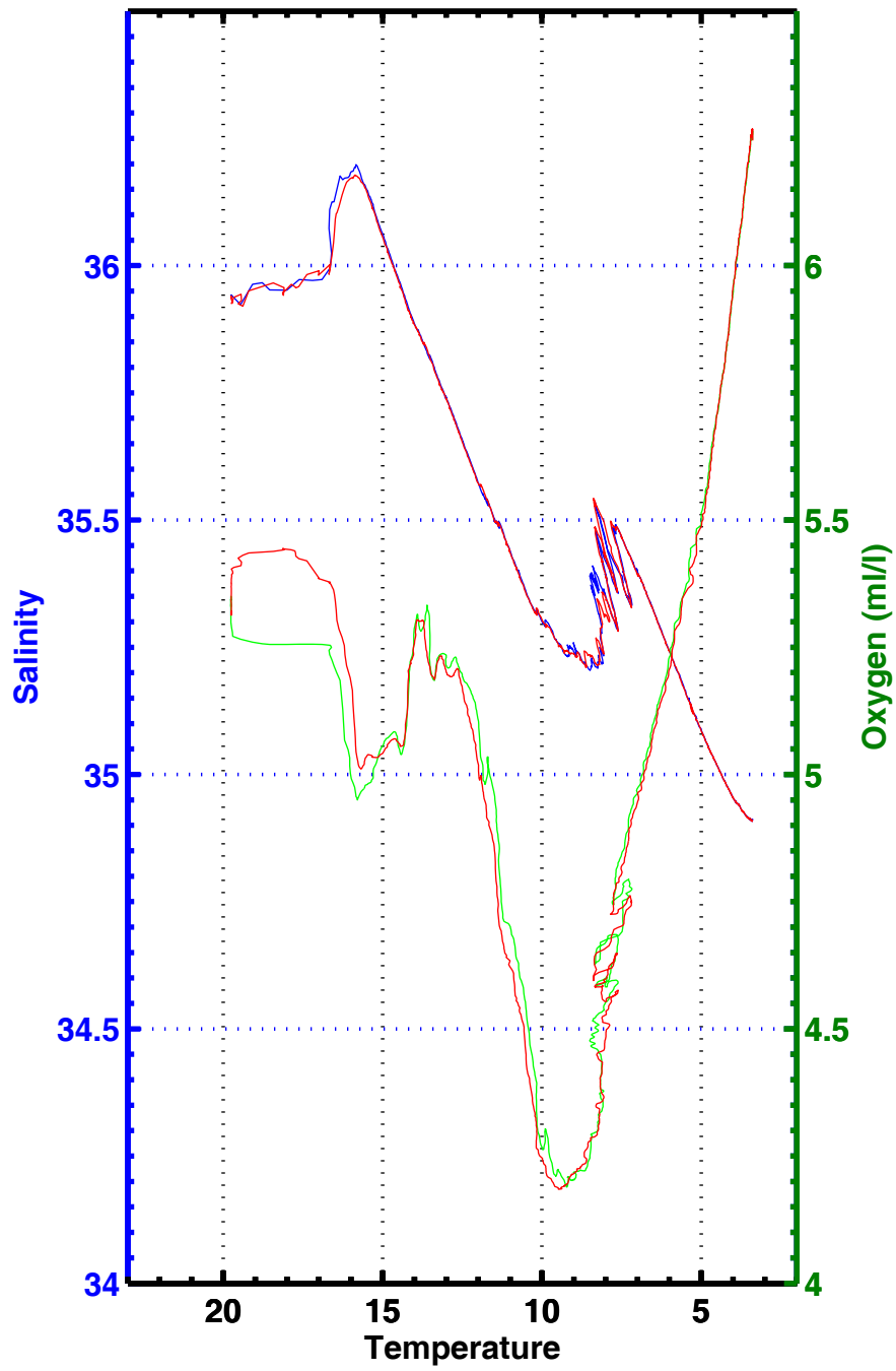
T-S , T-02 , station 3067
