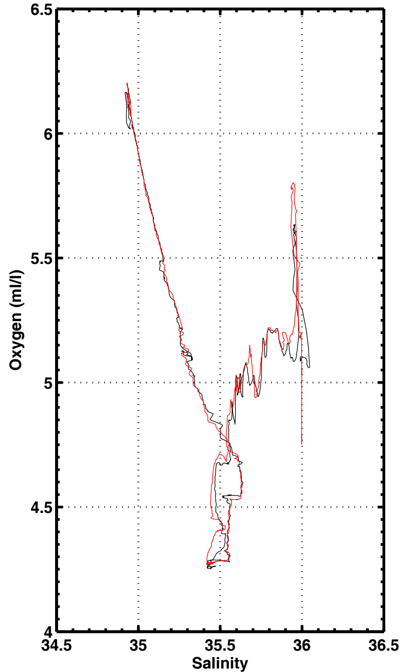
S-O2 , station 3168
