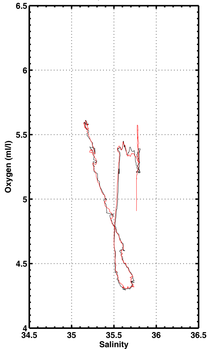
S-O2 , station 3323
