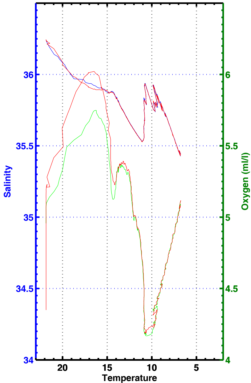
T-S , T-02 , station 3085
