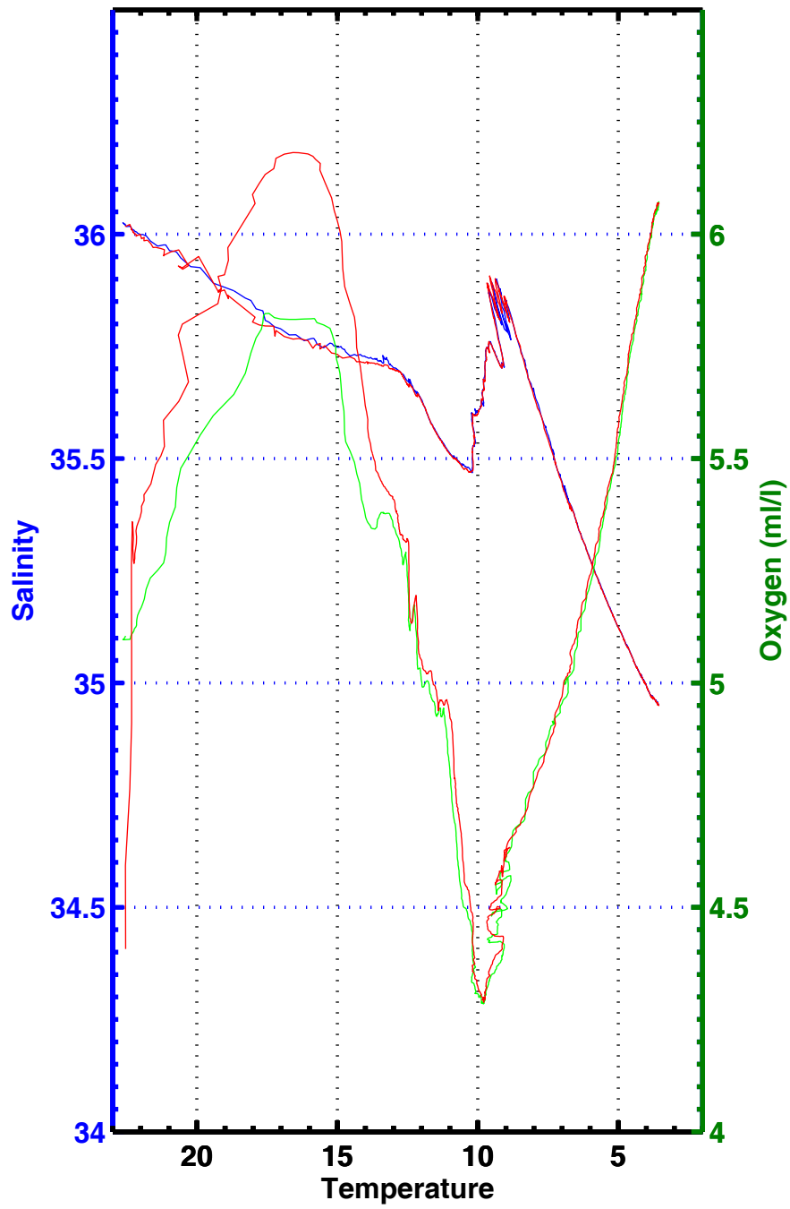
T-S , T-02 , station 3016
