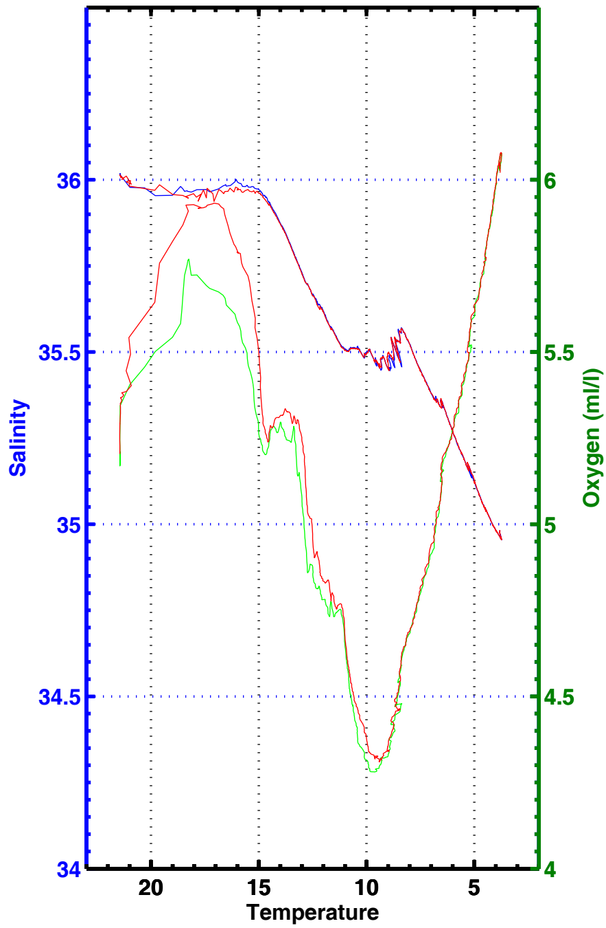
T-S , T-02 , station 3054
