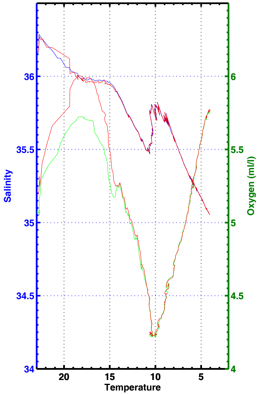
T-S , T-02 , station 3083
