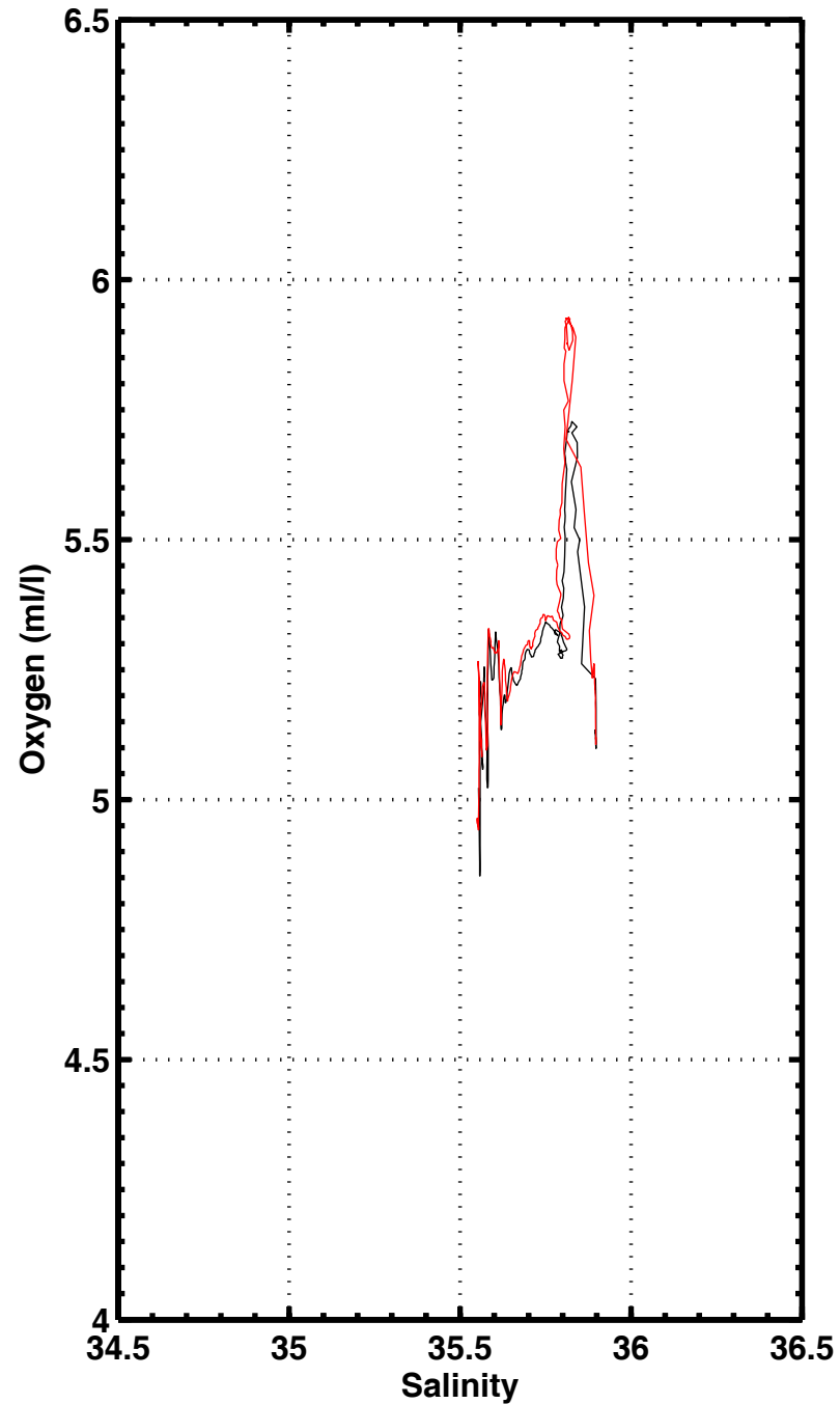
S-02 , station 3245
