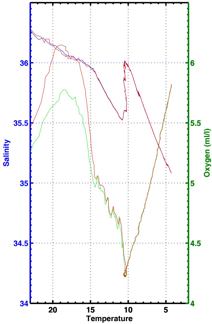
T-S , T-02 , station 3038
