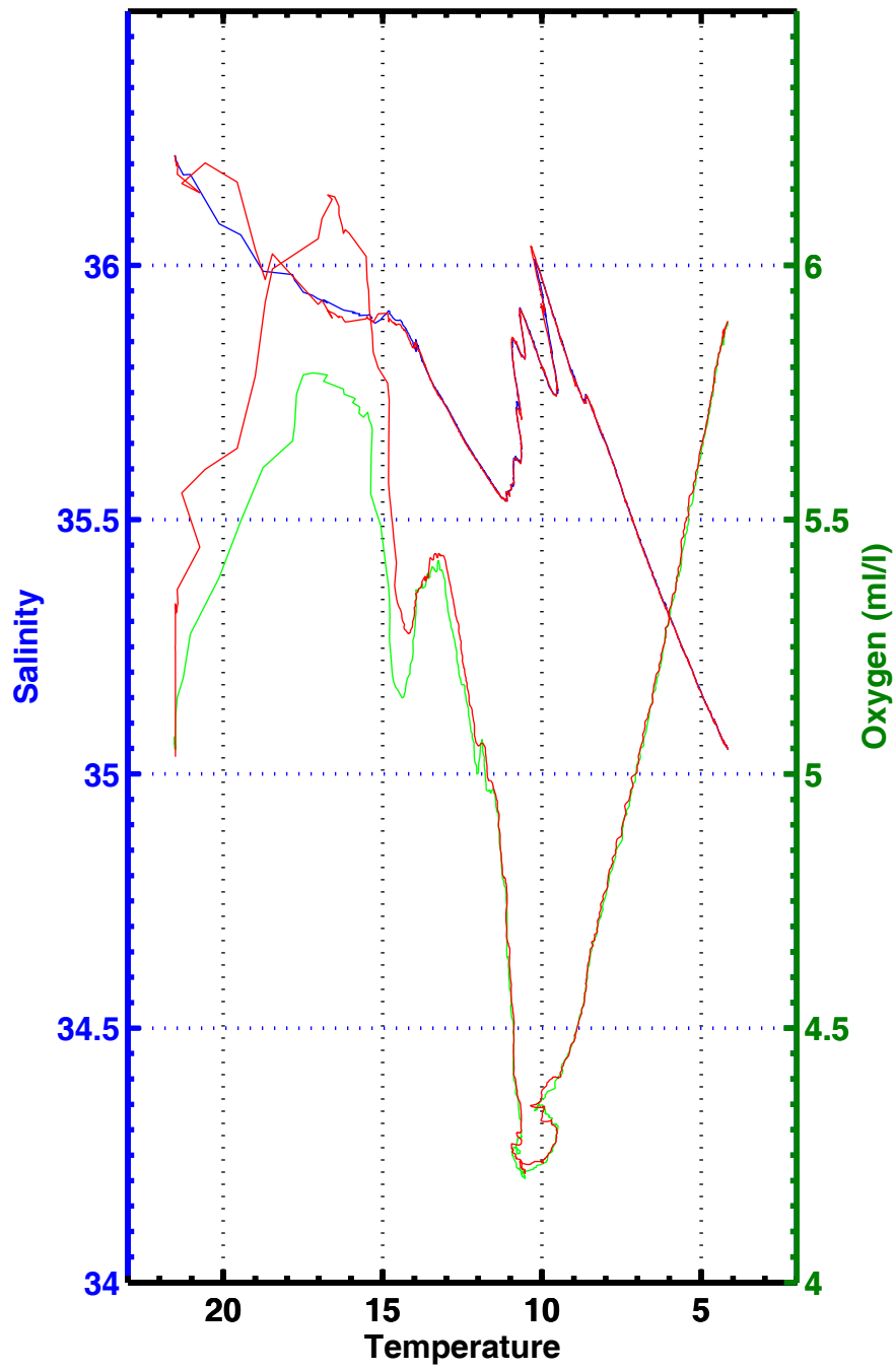
T-S , T-02 , station 3099
