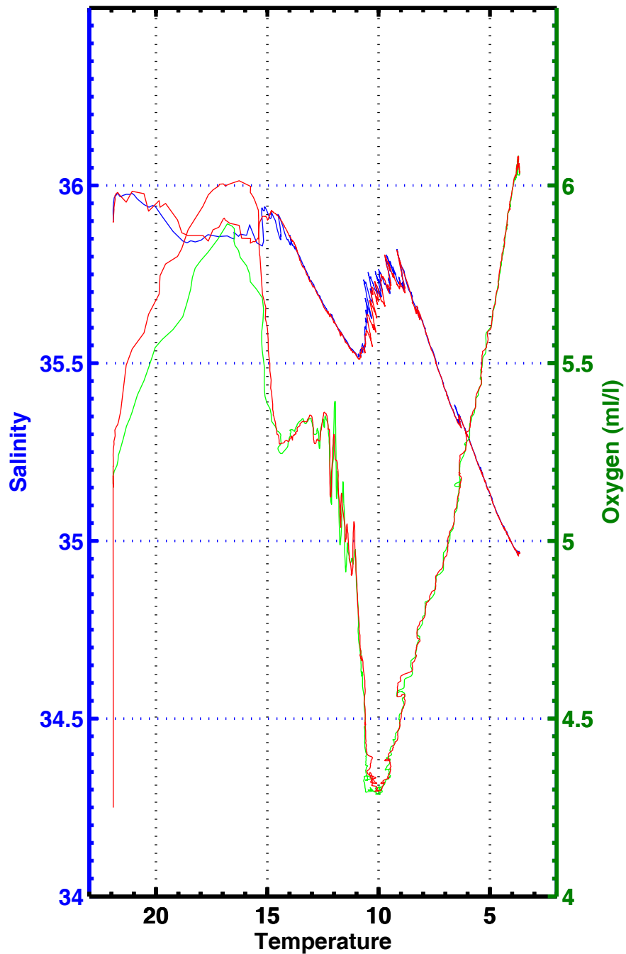
T-S , T-02 , station 3032
