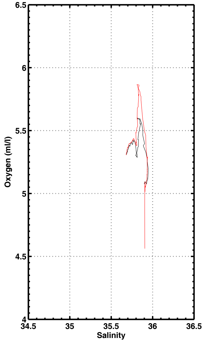
S-02 , station 3238
