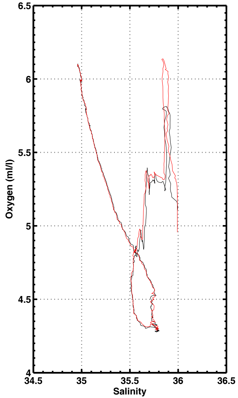
S-O2 , station 3033
