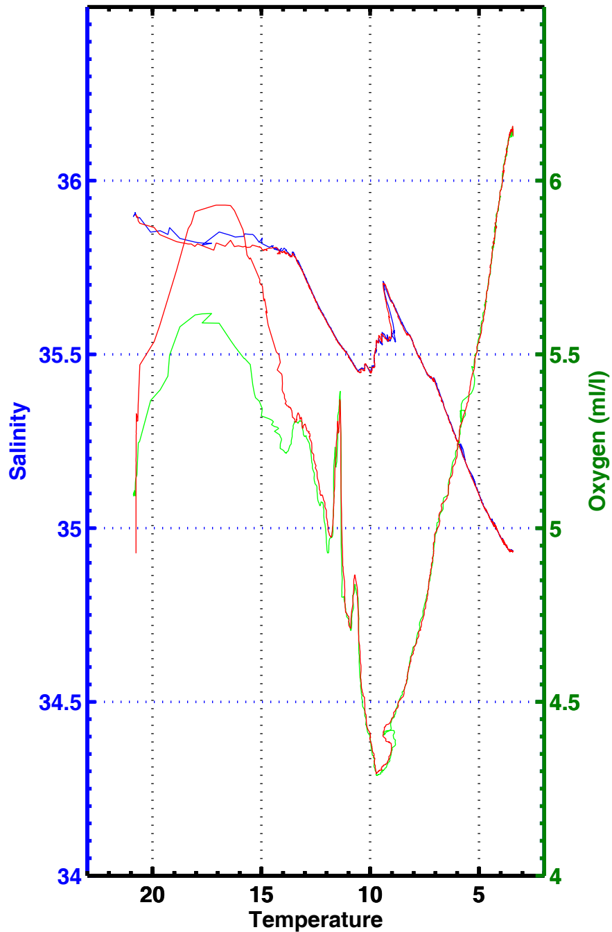
T-S , T-02 , station 3252
