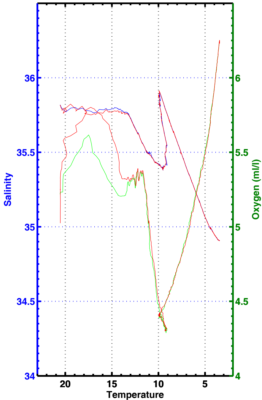
T-S , T-02 , station 3051
