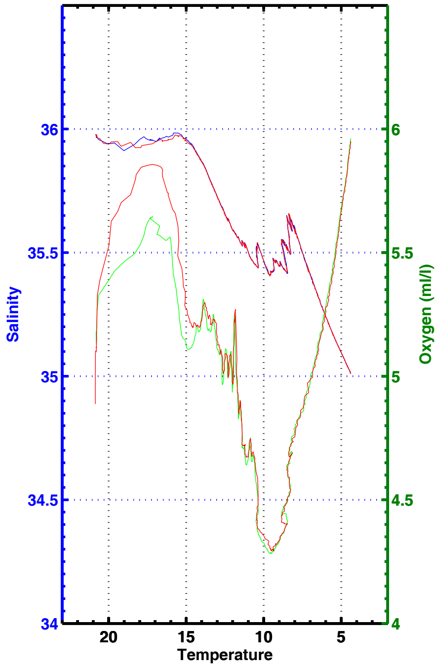
T-S , T-02 , station 3166
