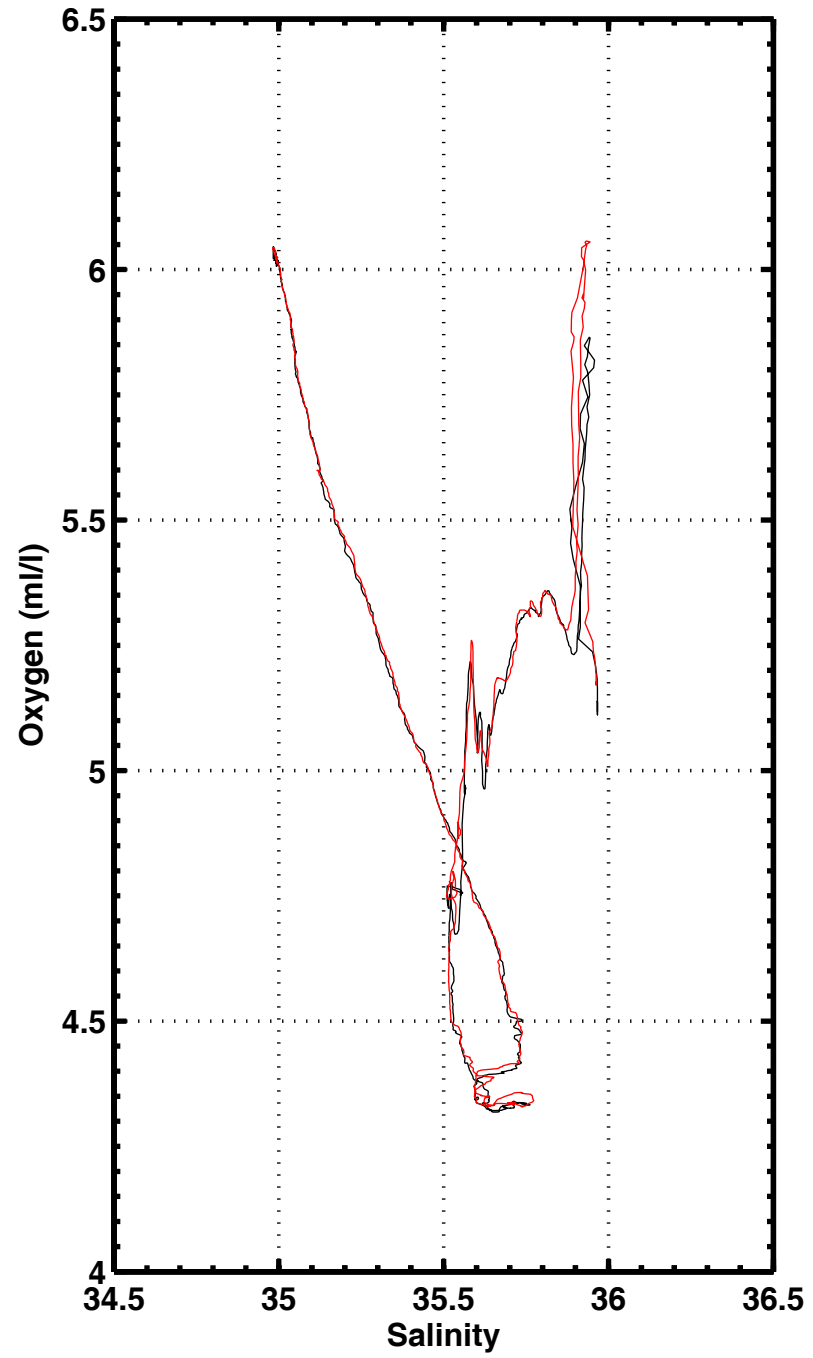
S-O2 , station 3034
