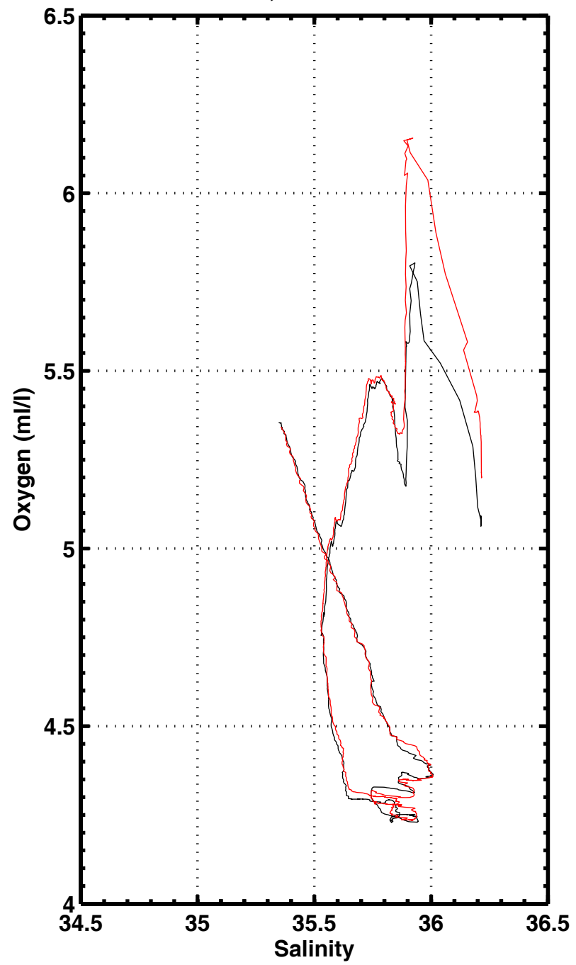
S-O2 , station 3098
