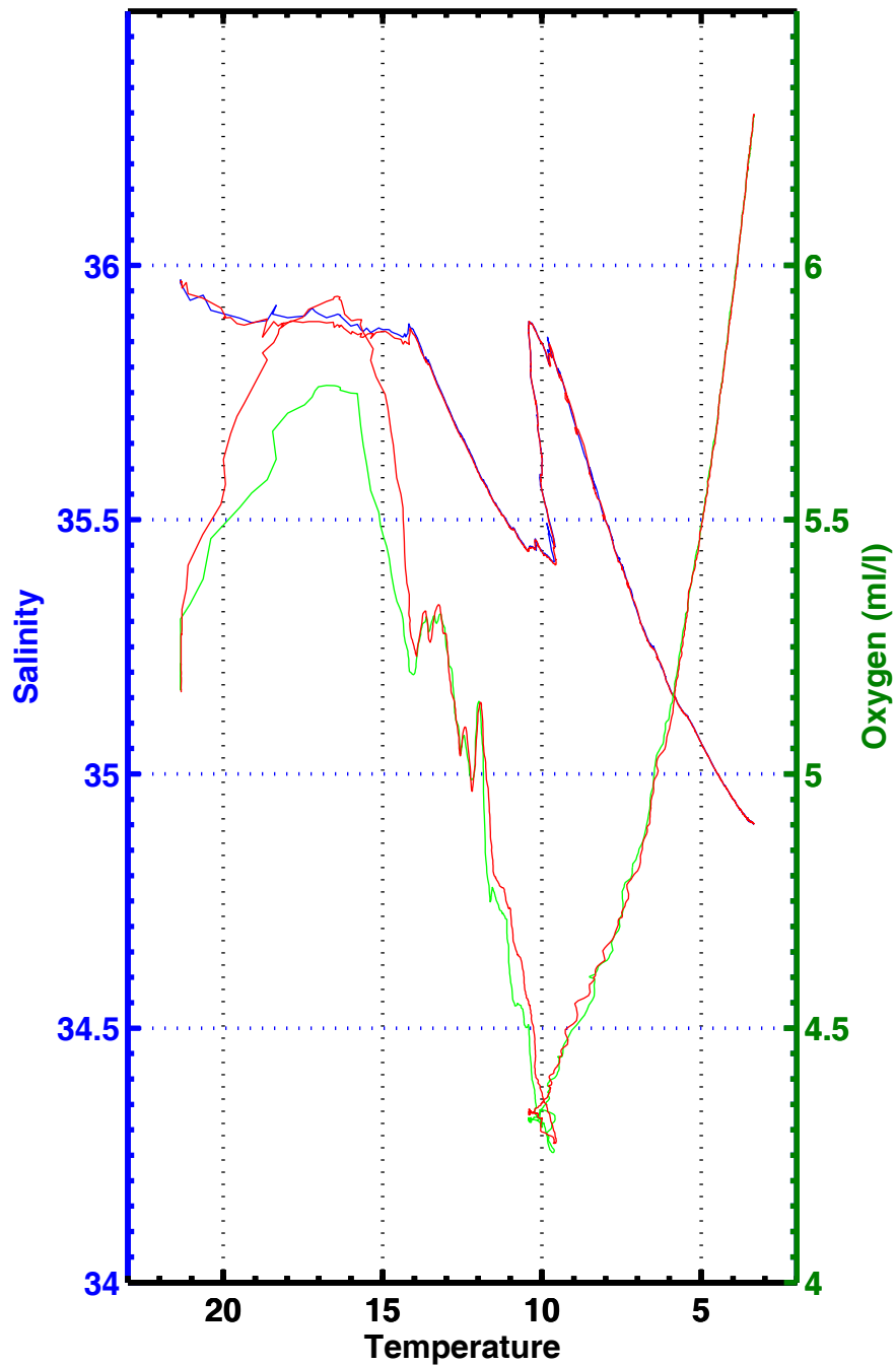
T-S , T-02 , station 3061
