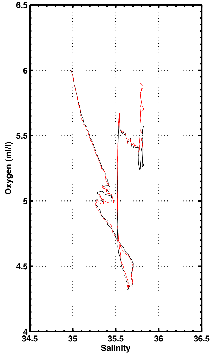
S-O2 , station 3026
