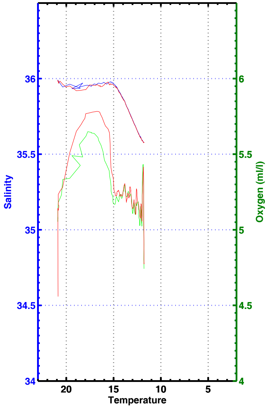
T-S , T-02 , station 3161
