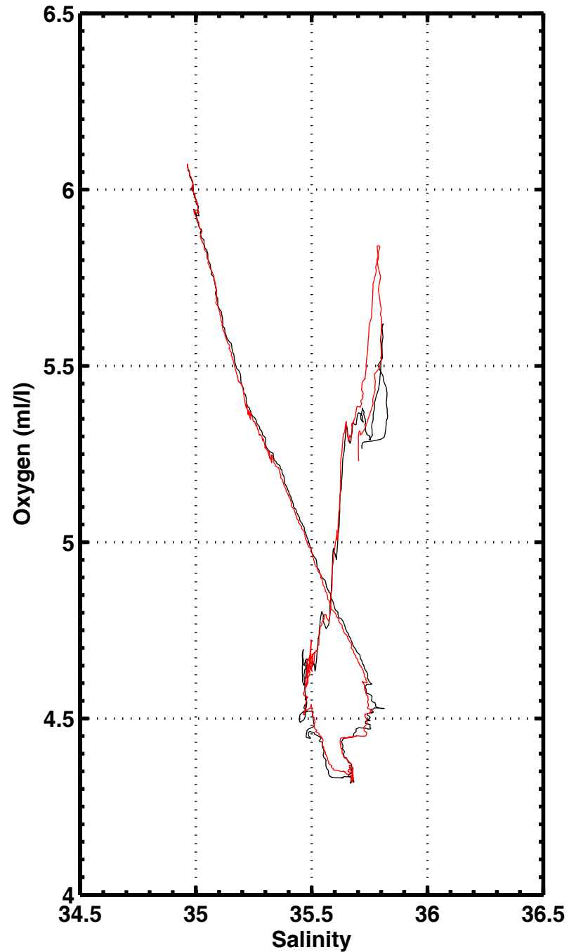
S-O2 , station 3005
