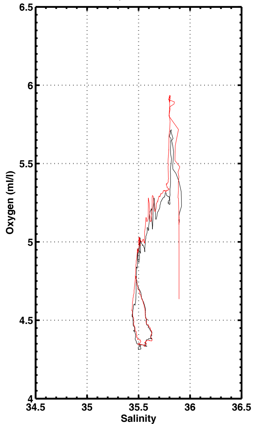
S-O2 , station 3242
