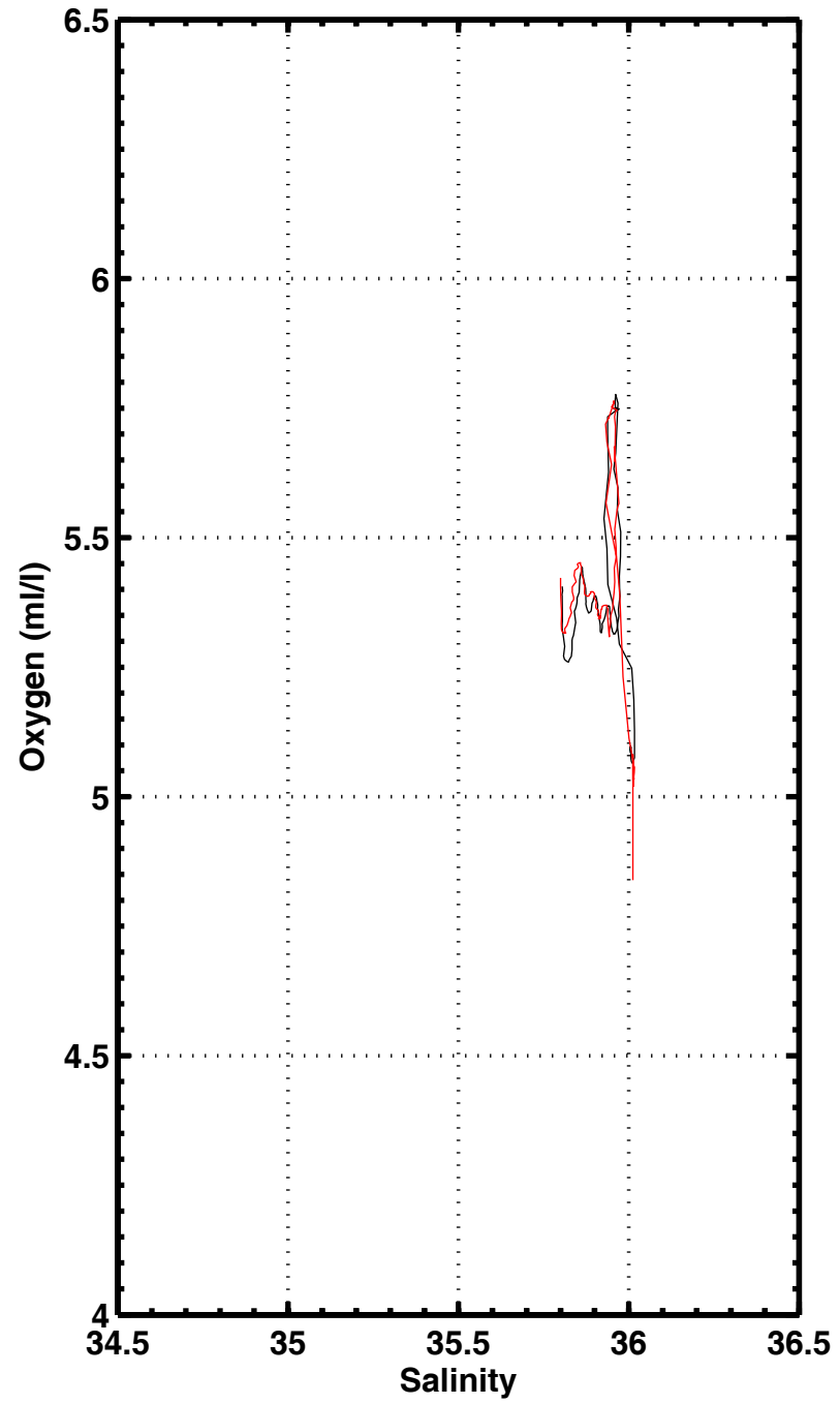
S-02 , station 3162
