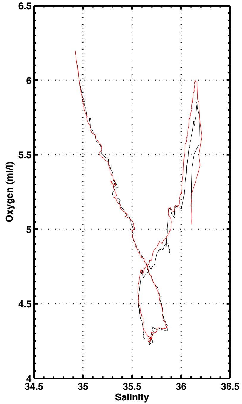
S-O2 , station 3043
