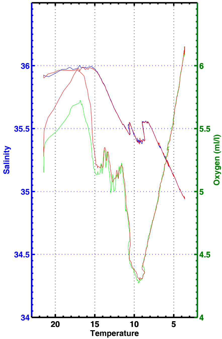
T-S , T-02 , station 3053
