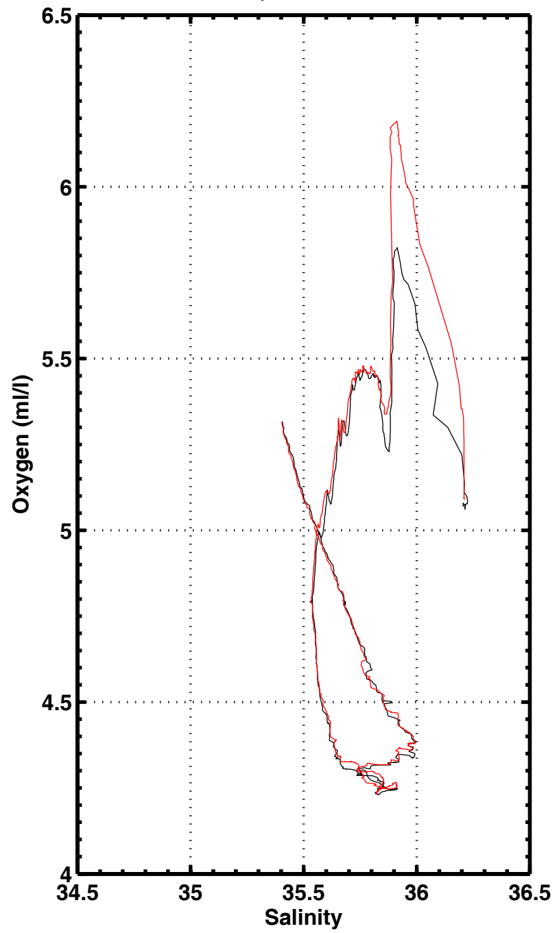
S-O2 , station 3097
