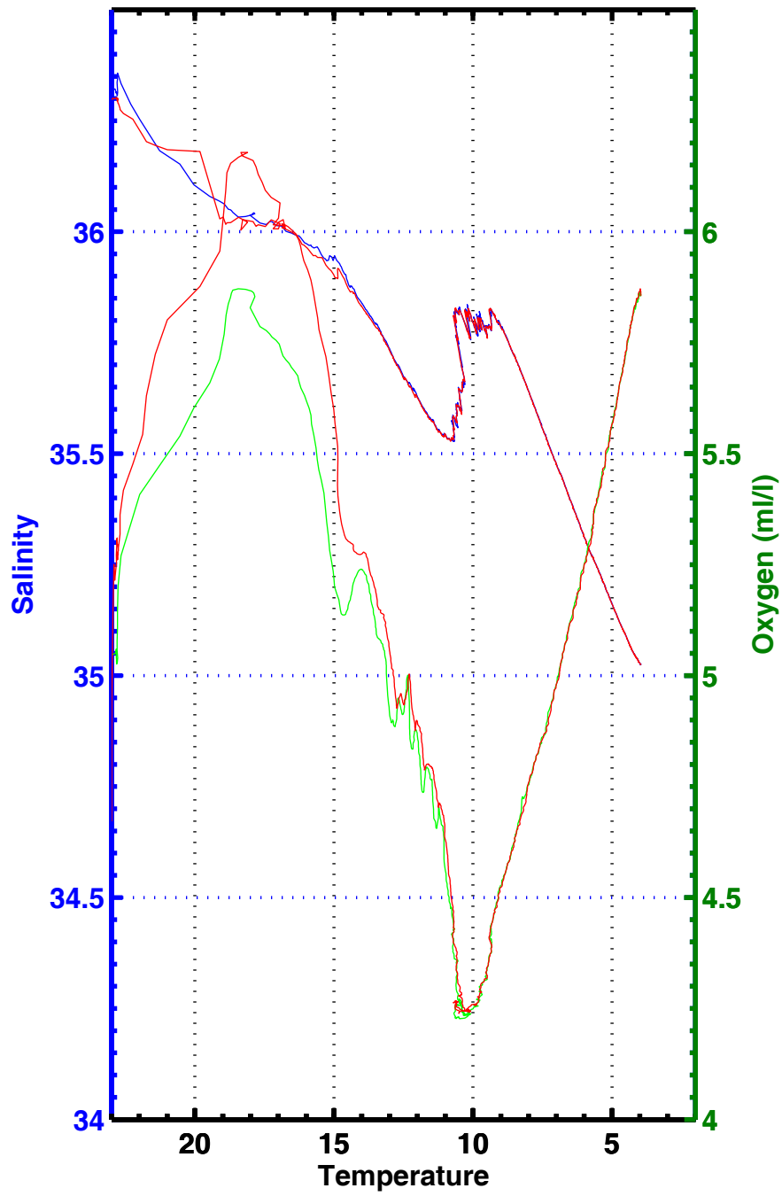
T-S , T-02 , station 3082
