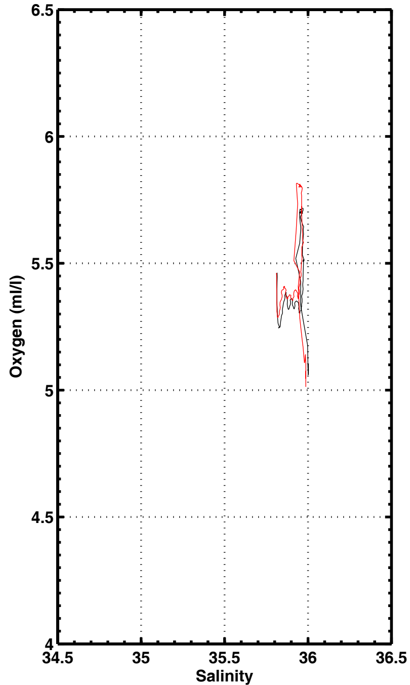
S-02 , station 3165
