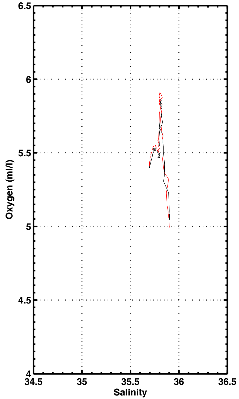
S-02 , station 3249
