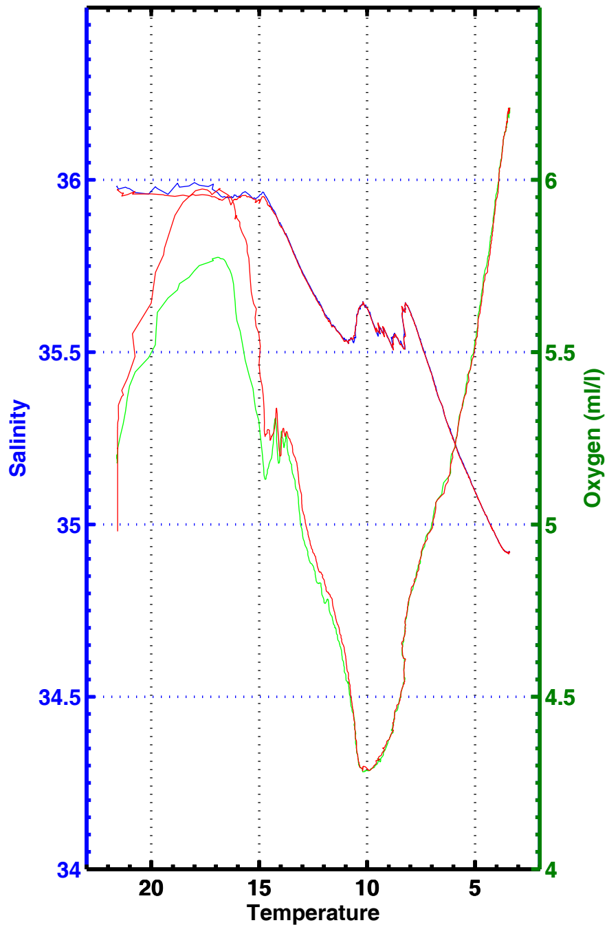
T-S , T-02 , station 3059
