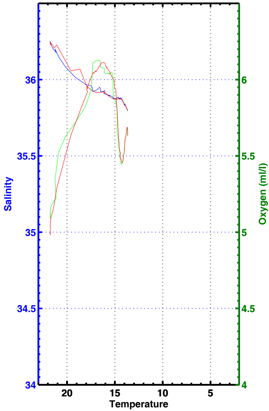
T-S , T-02 , station 3094
