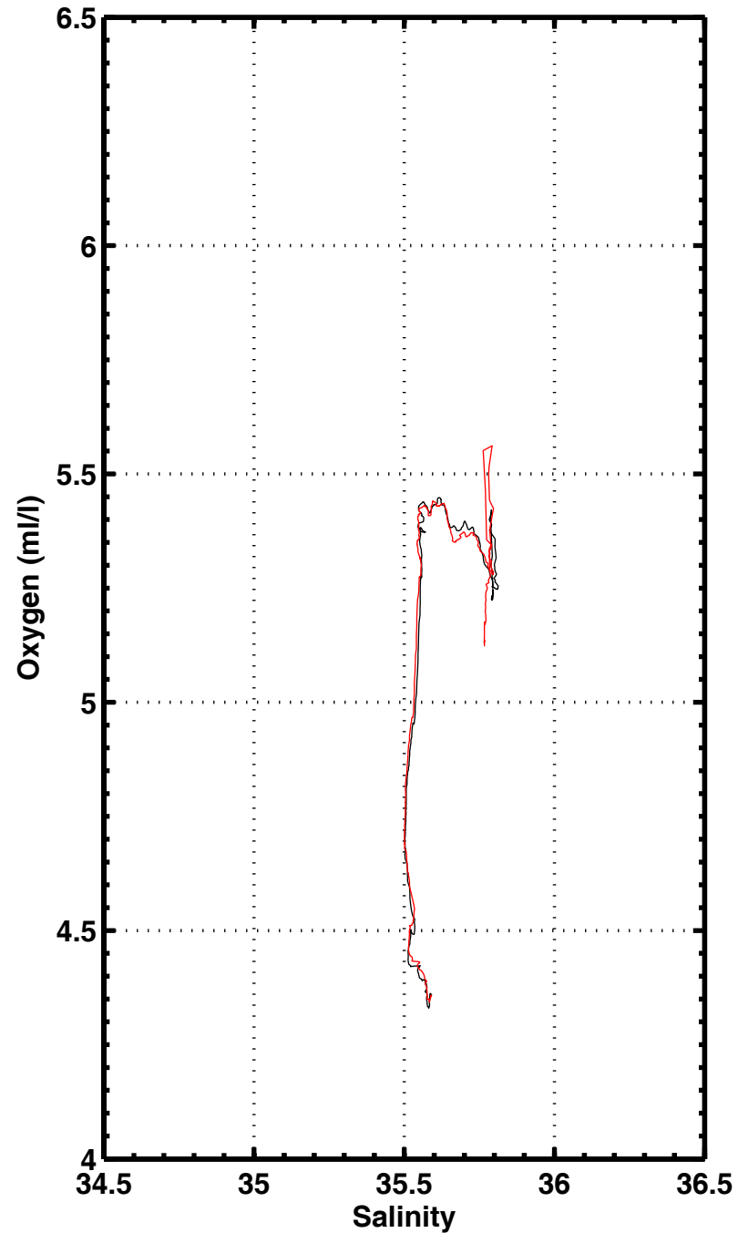
S-02 , station 3332
