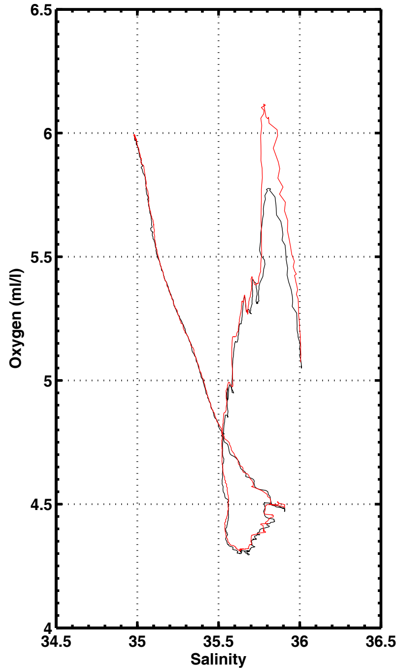
S-O2 , station 3009
