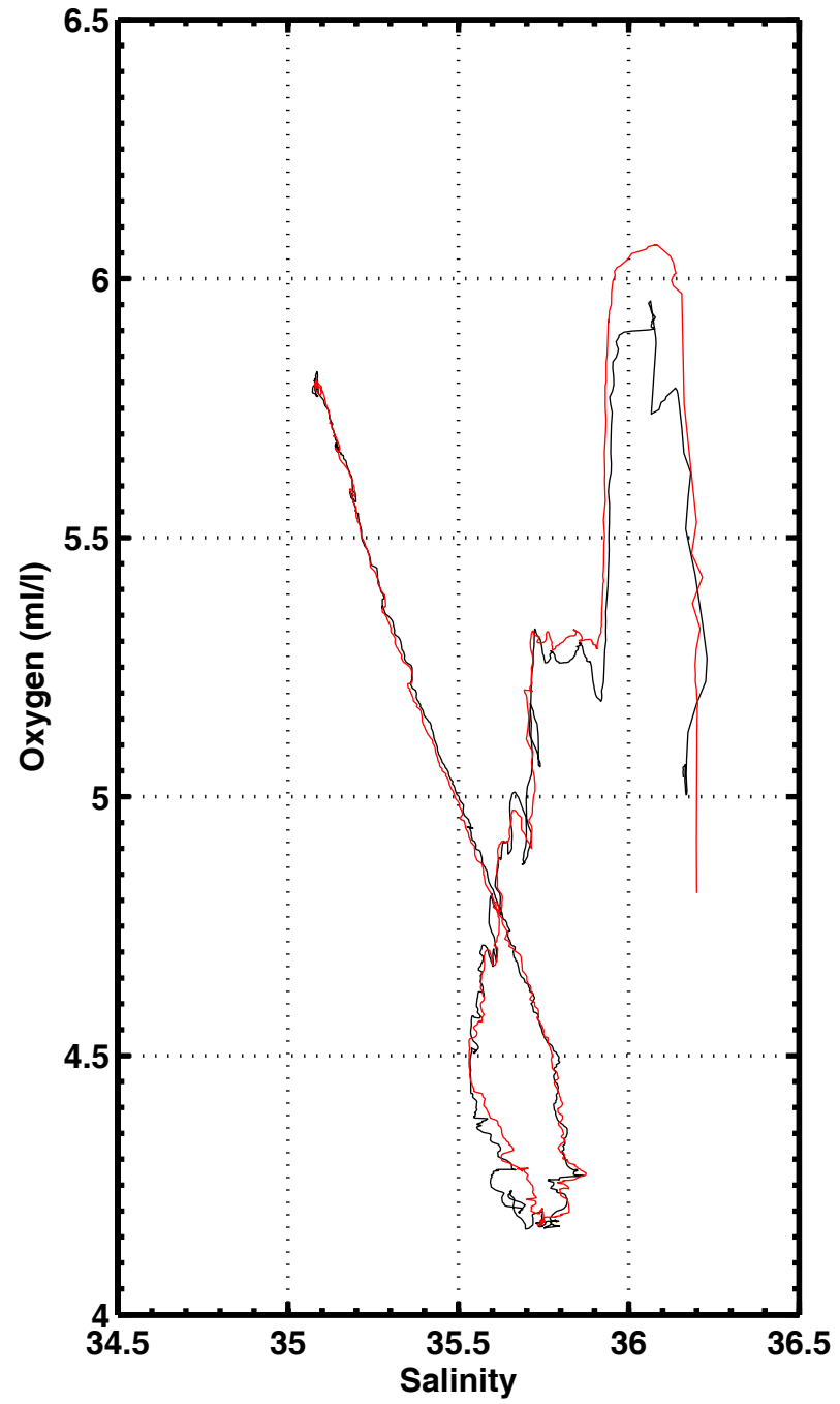
S-O2 , station 3039
