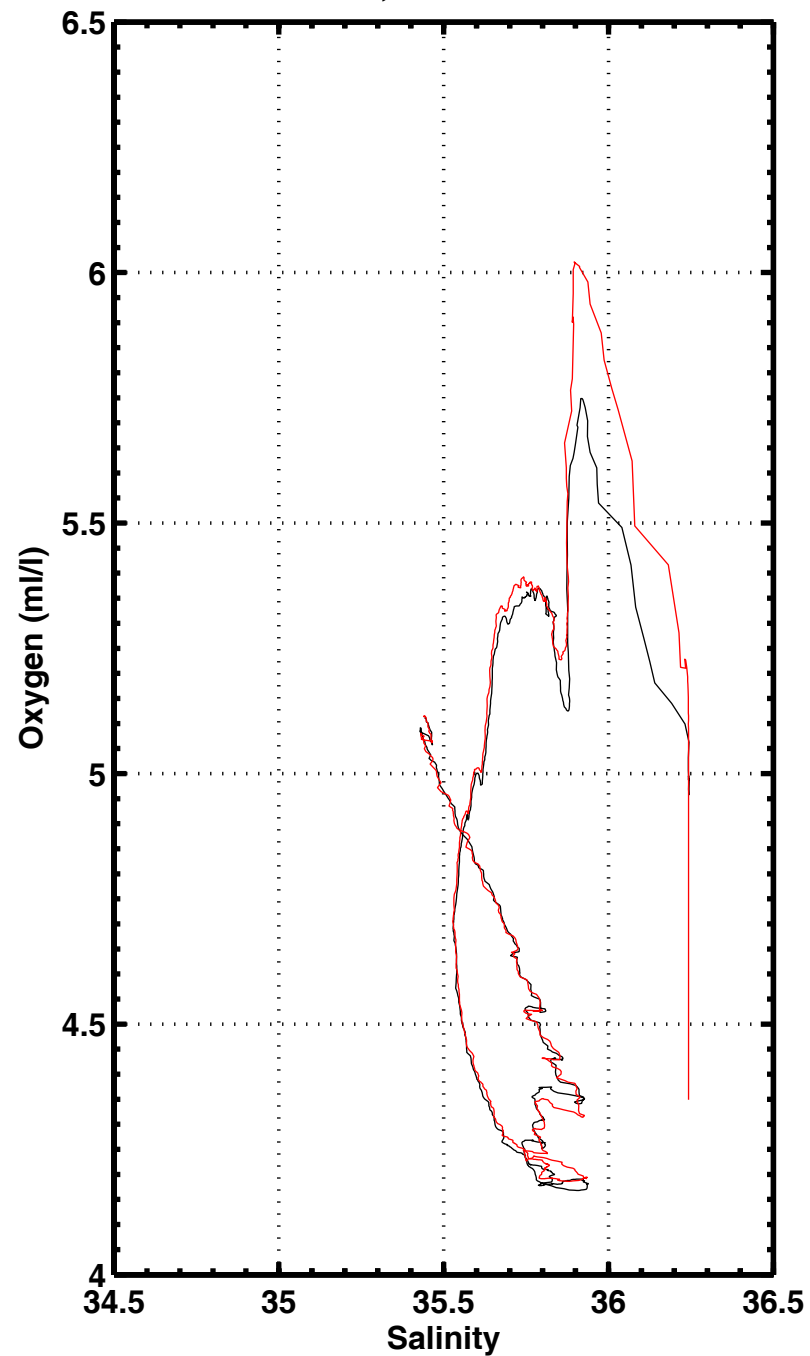
S-O2 , station 3085
