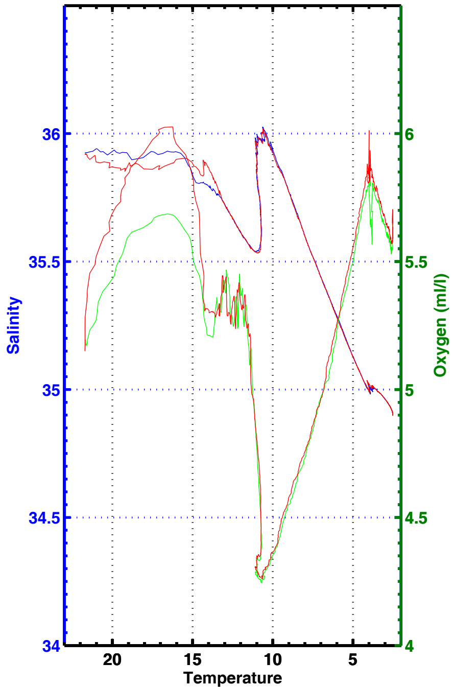
T-S , T-02 , station 3006
