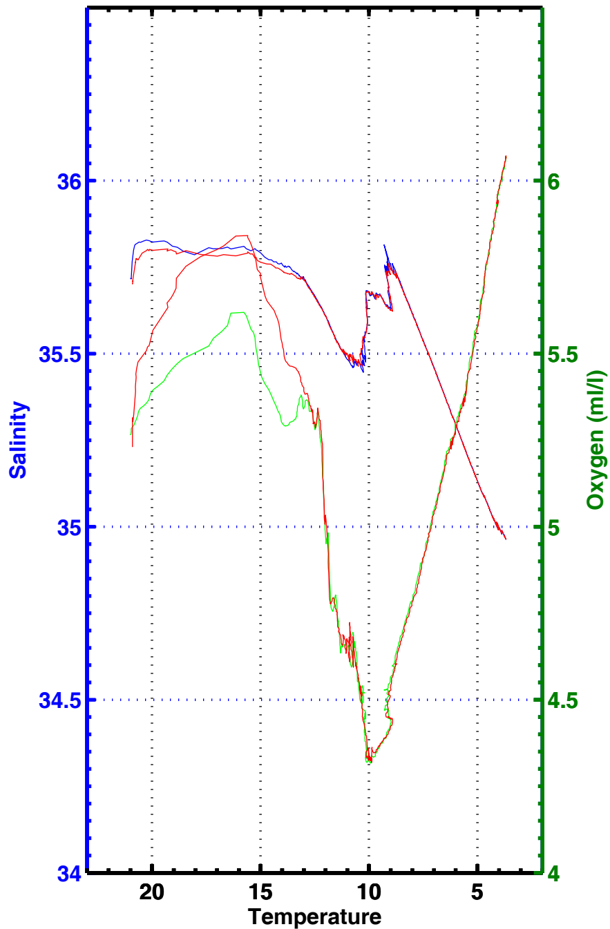
T-S , T-02 , station 3005
