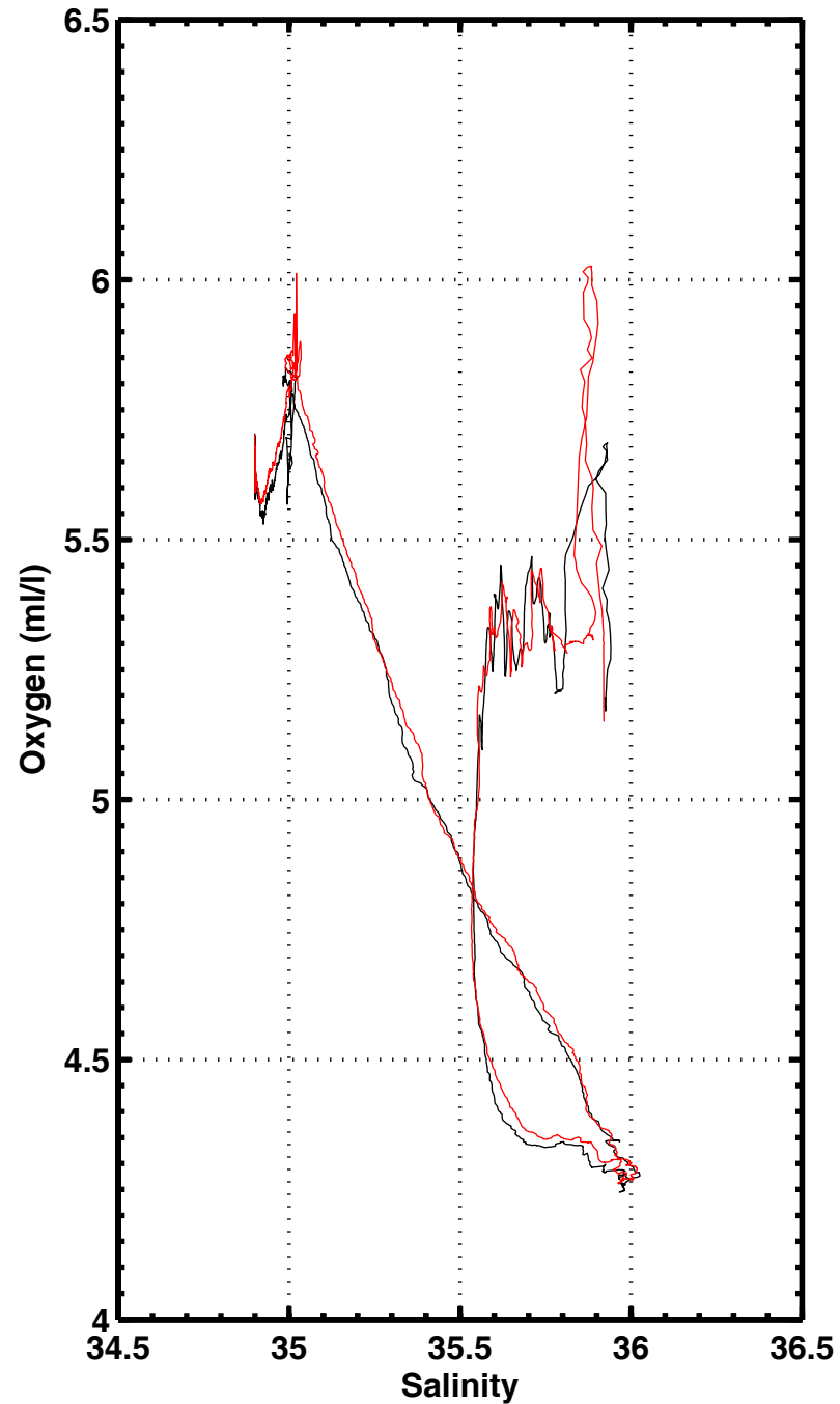
S-O2 , station 3006
