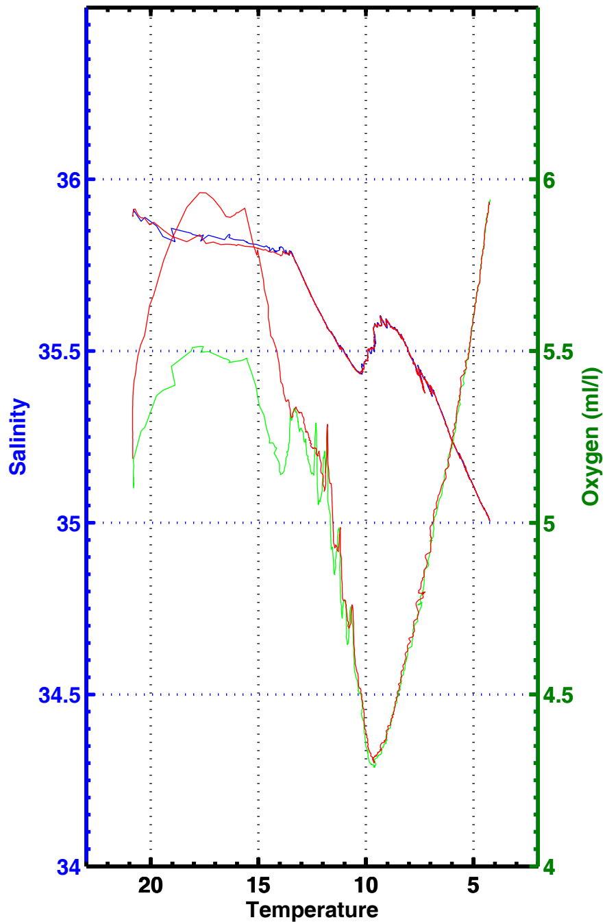
T-S , T-02 , station 3239
