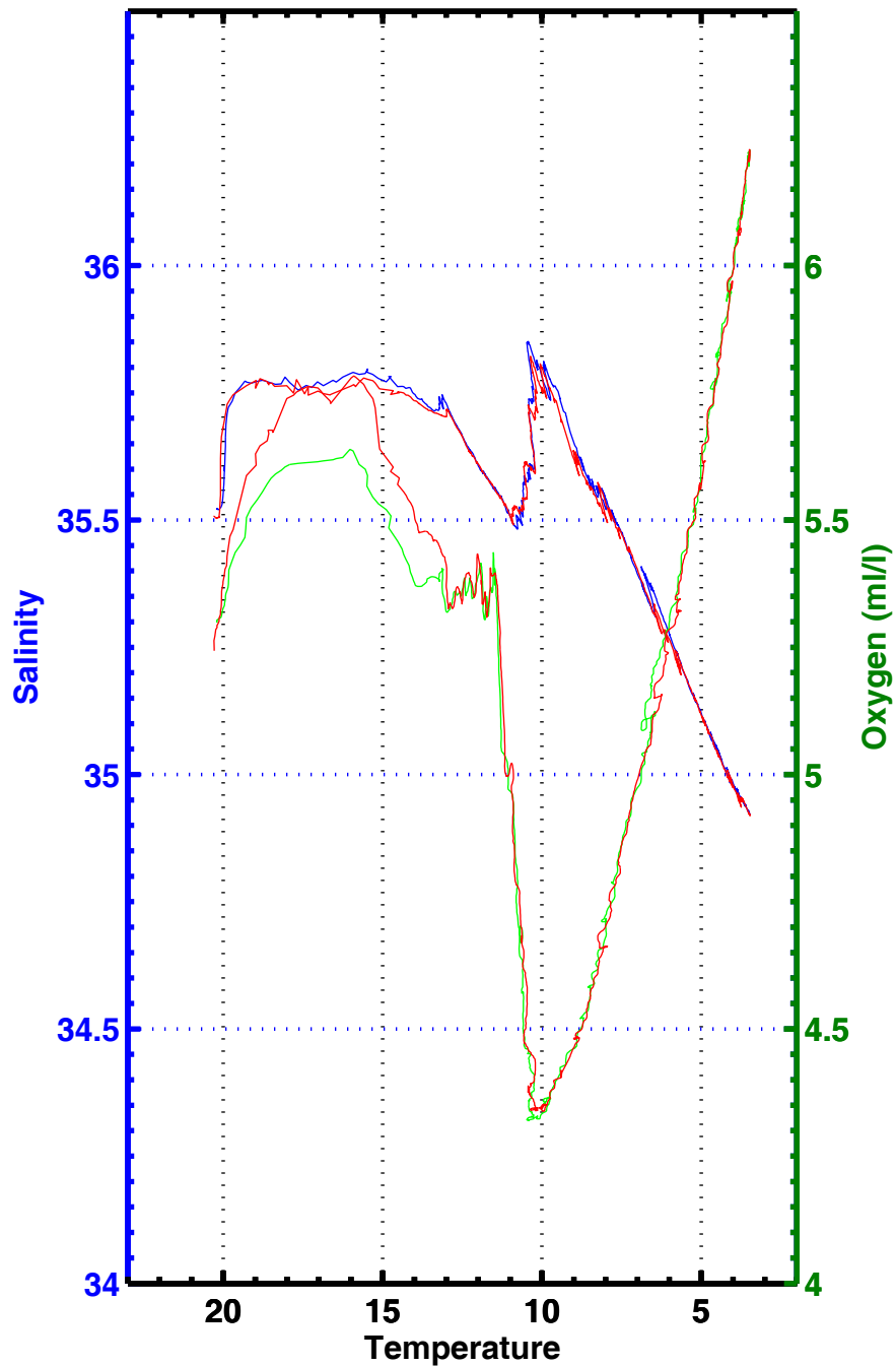
T-S , T-02 , station 3003
