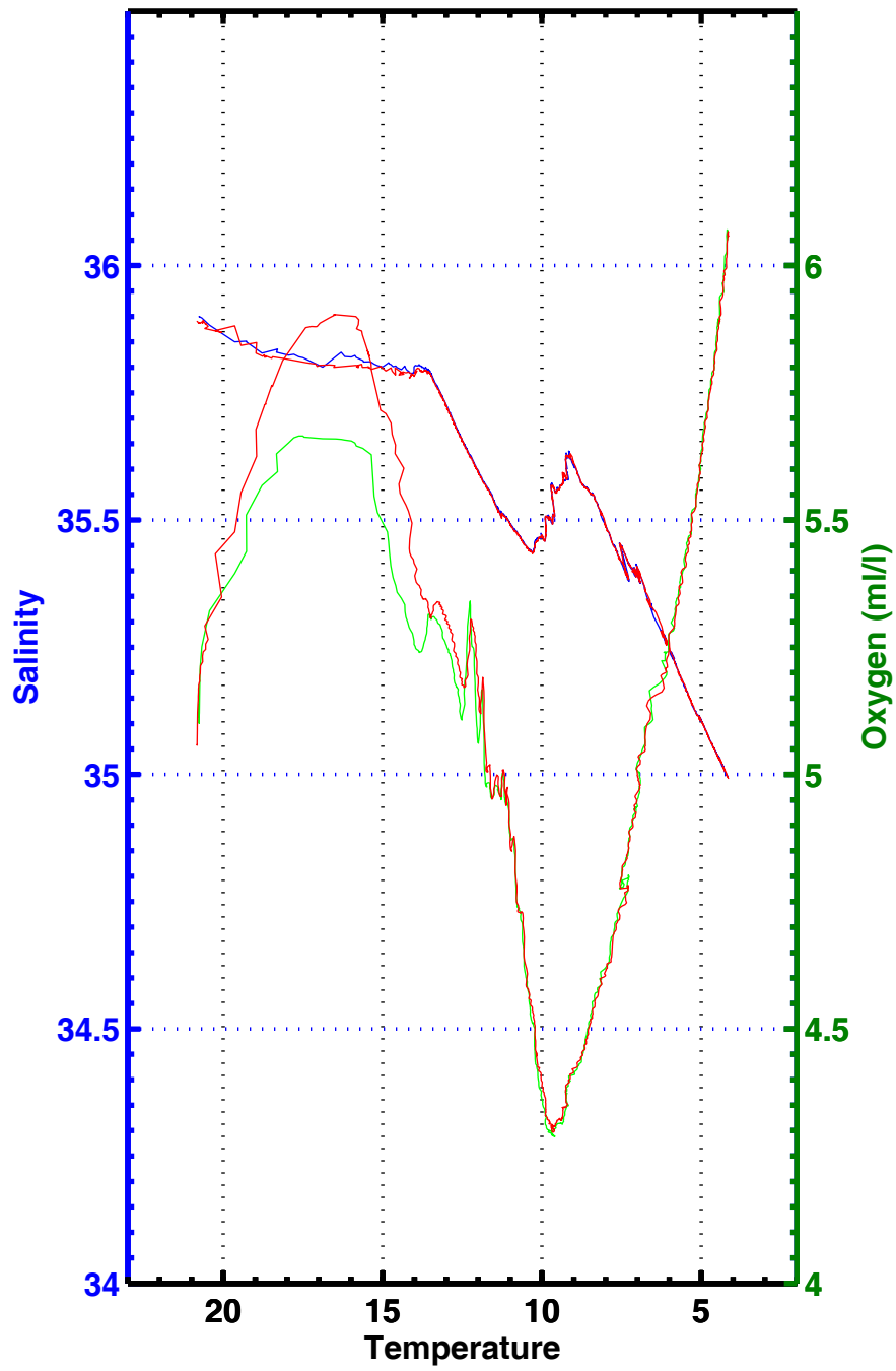
T-S , T-02 , station 3241
