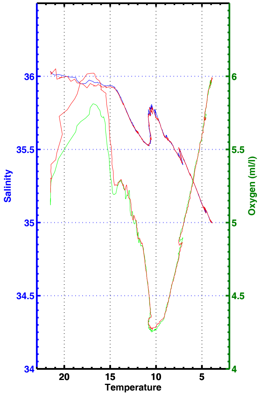
T-S , T-02 , station 3047
