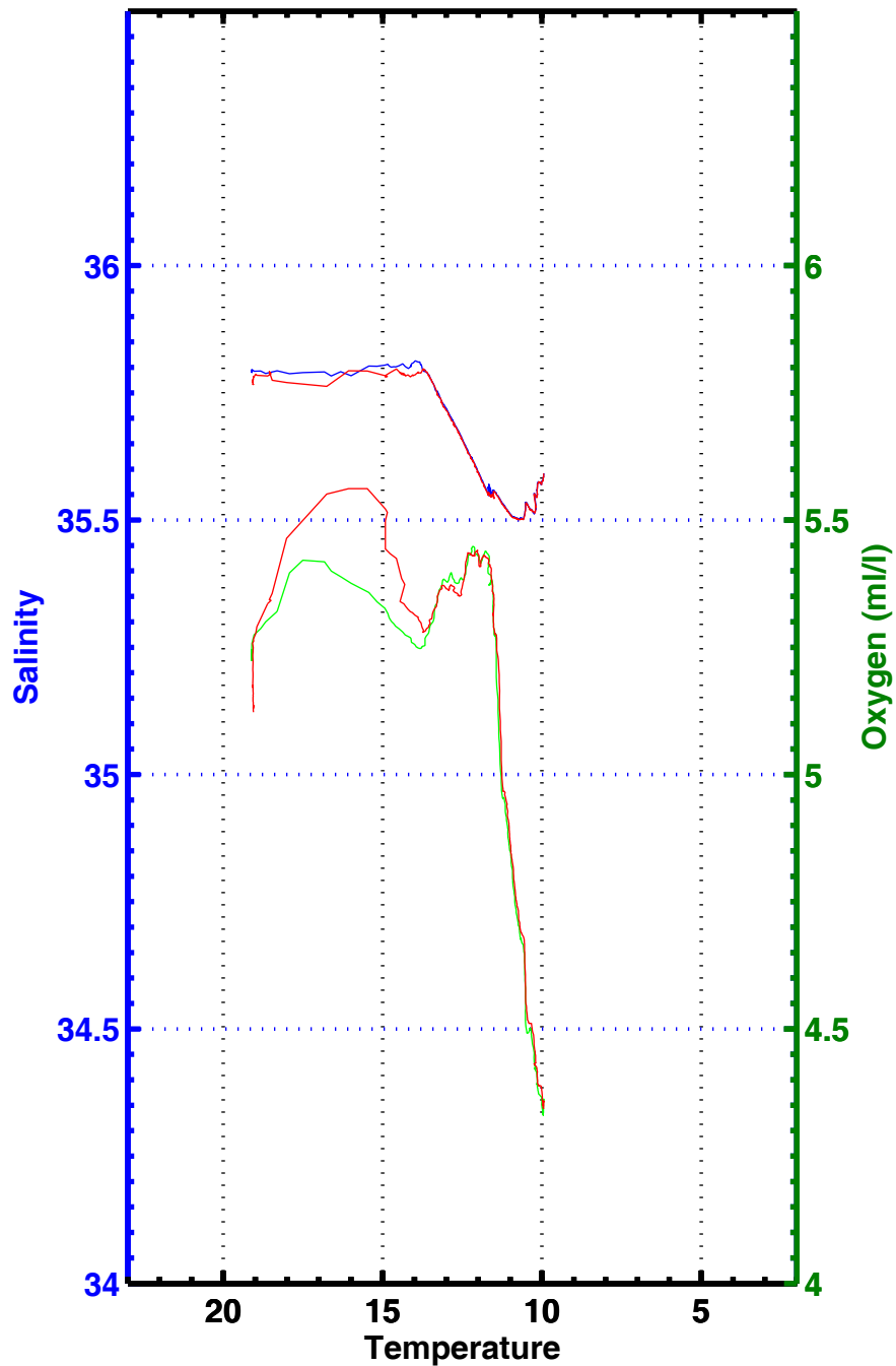
T-S , T-02 , station 3332
