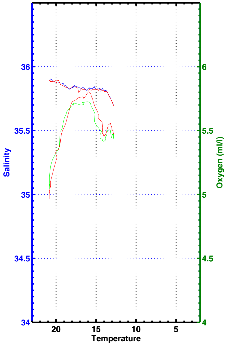
T-S , T-02 , station 3247
