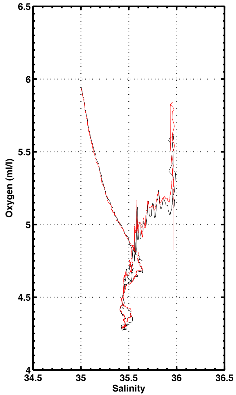
S-O2 , station 3159
