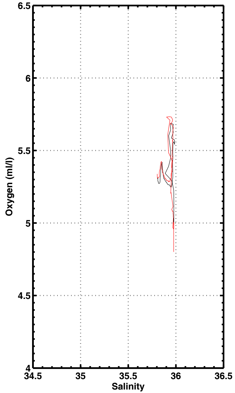
S-02 , station 3156
