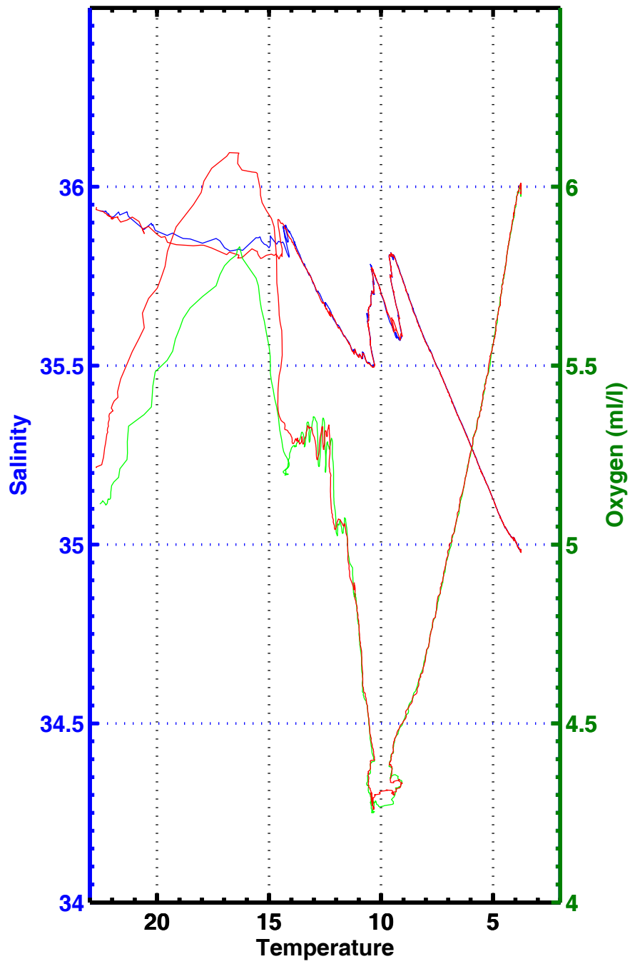
T-S , T-02 , station 3015
