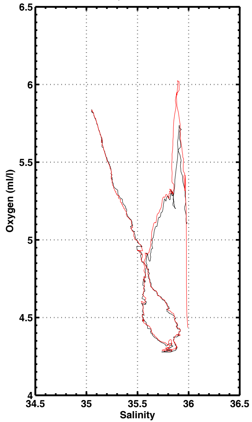
S-O2 , station 3018
