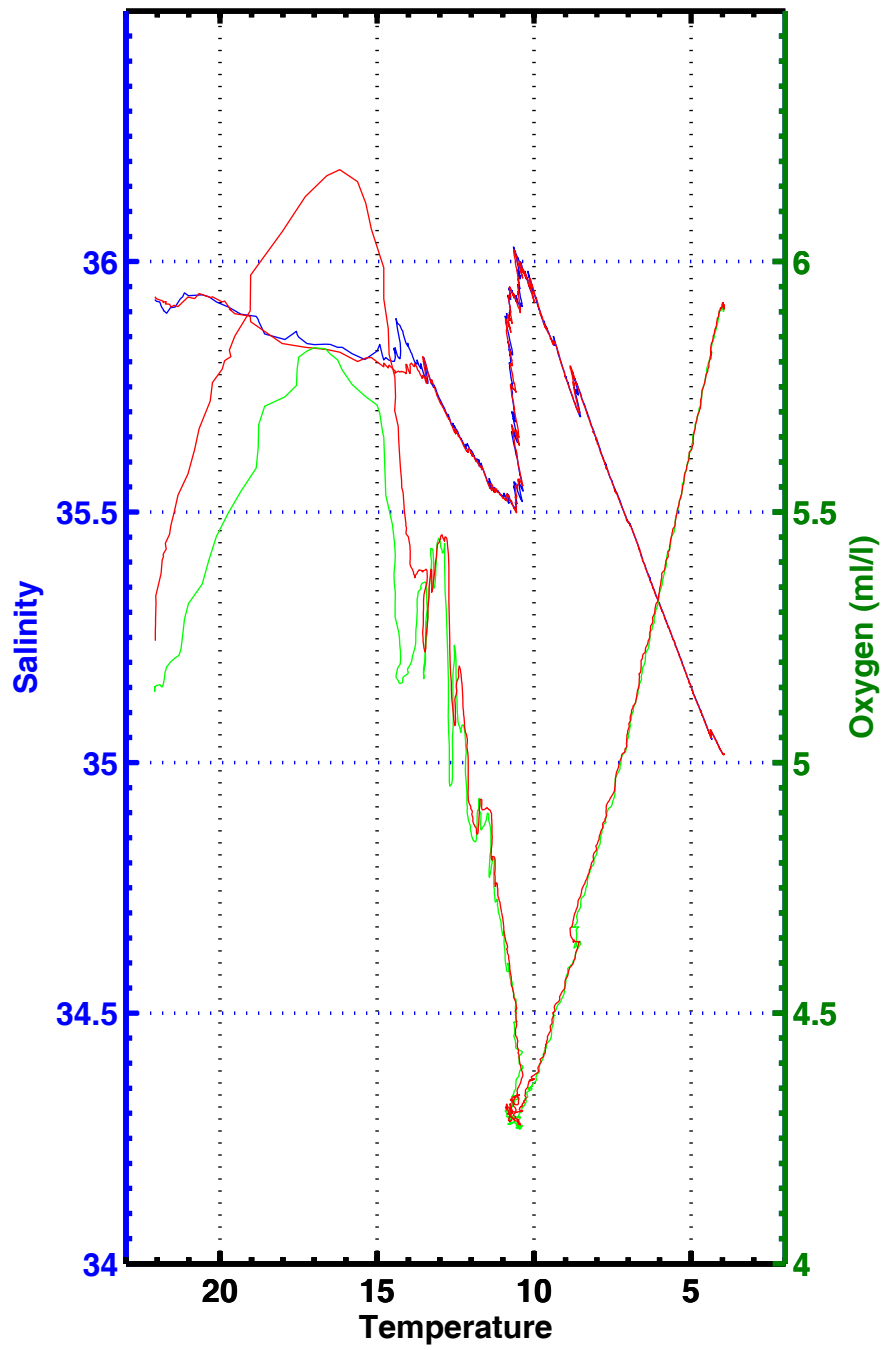
T-S , T-02 , station 3007
