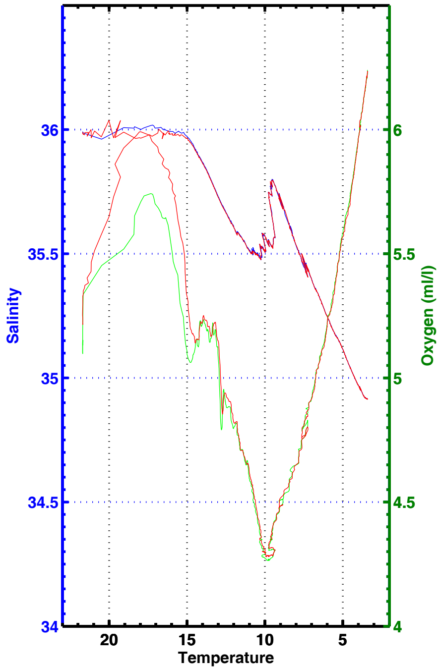
T-S , T-02 , station 3057
