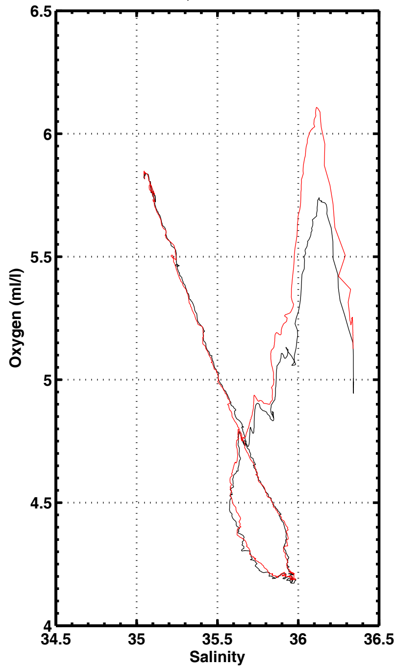
S-O2 , station 3014
