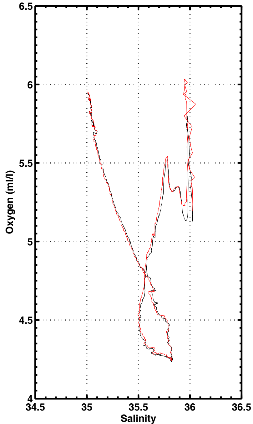
S-O2 , station 3046
