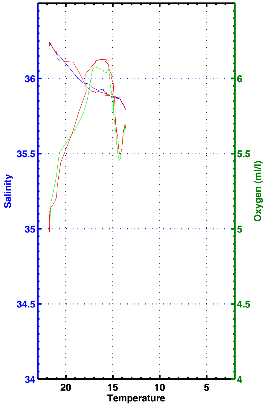
T-S , T-02 , station 3096
