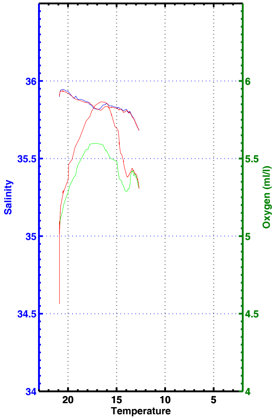
T-S , T-02 , station 3238
