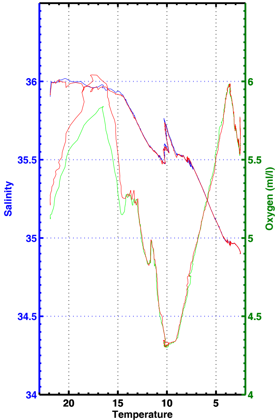
T-S , T-02 , station 3031
