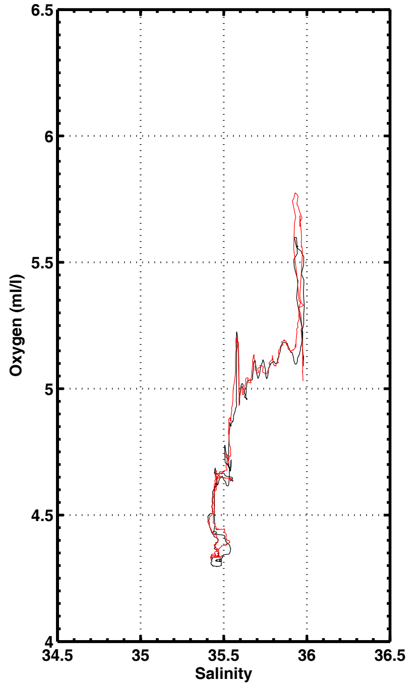
S-02 , station 3158
