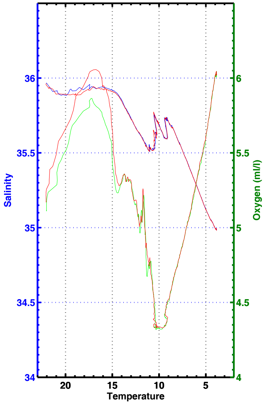
T-S , T-02 , station 3034
