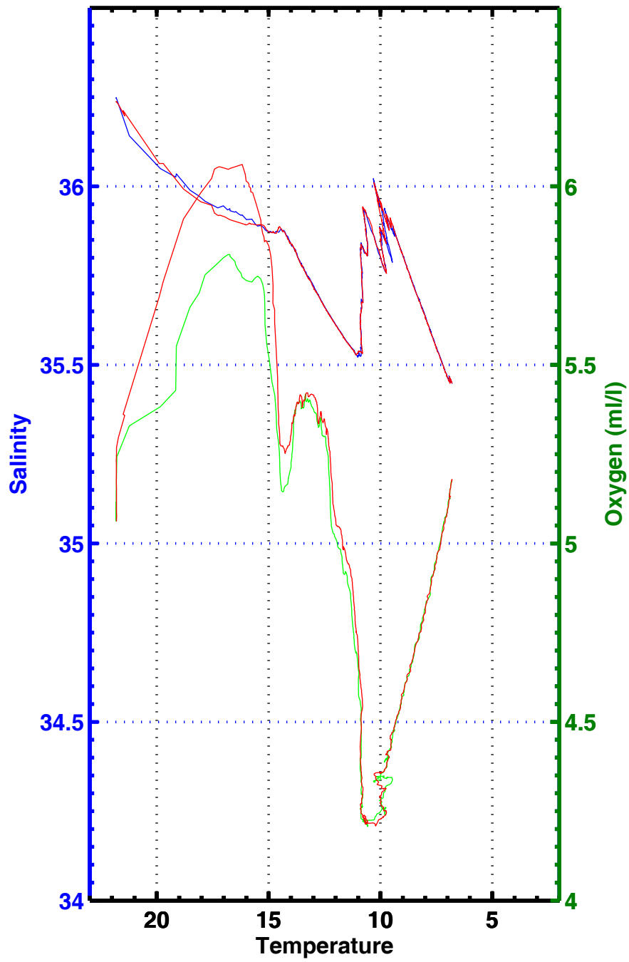
T-S , T-02 , station 3089
