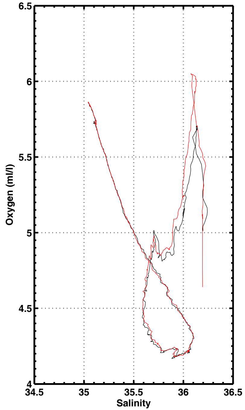
S-O2 , station 3011
