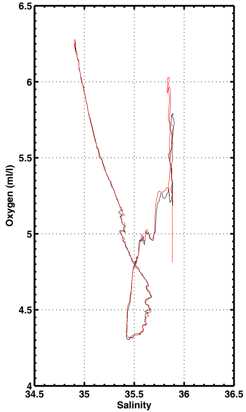
S-O2 , station 3060
