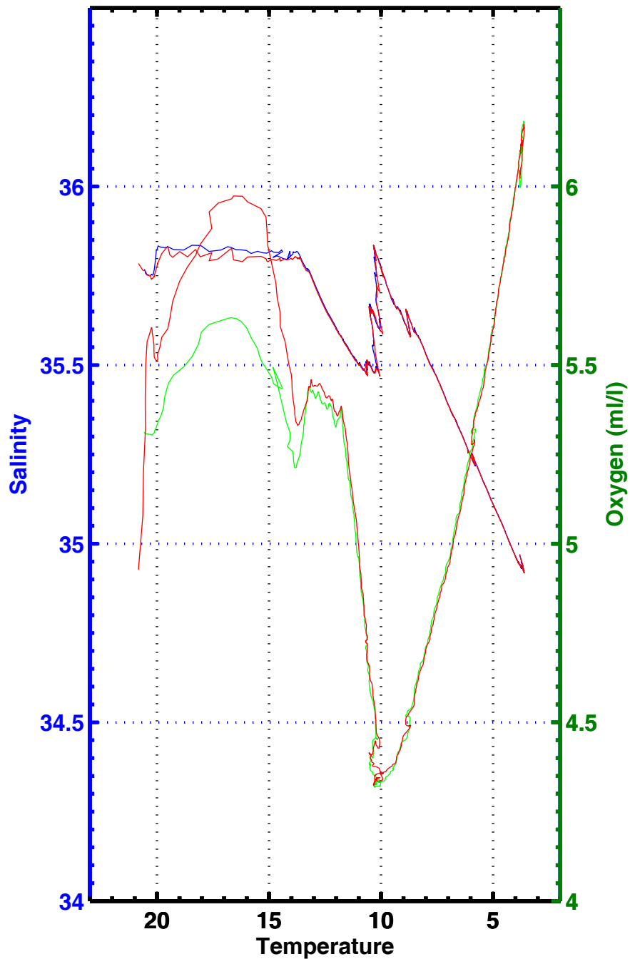
T-S , T-02 , station 3027
