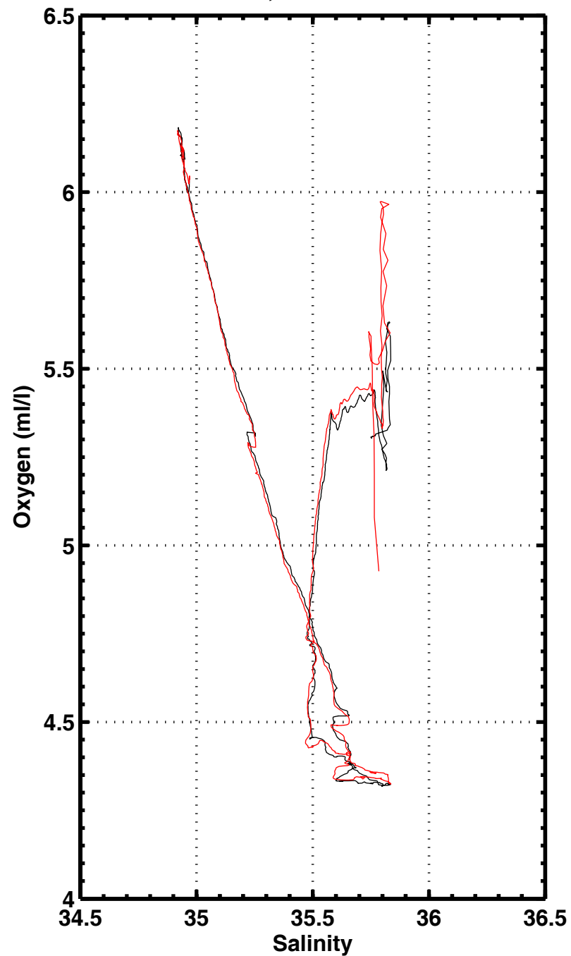
S-O2 , station 3027
