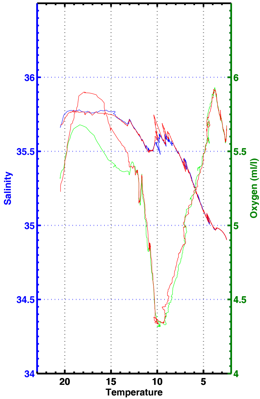
T-S , T-02 , station 3004
