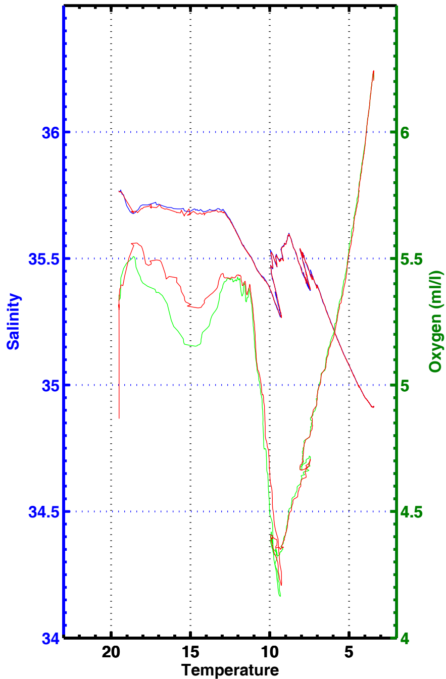
T-S , T-02 , station 3066
