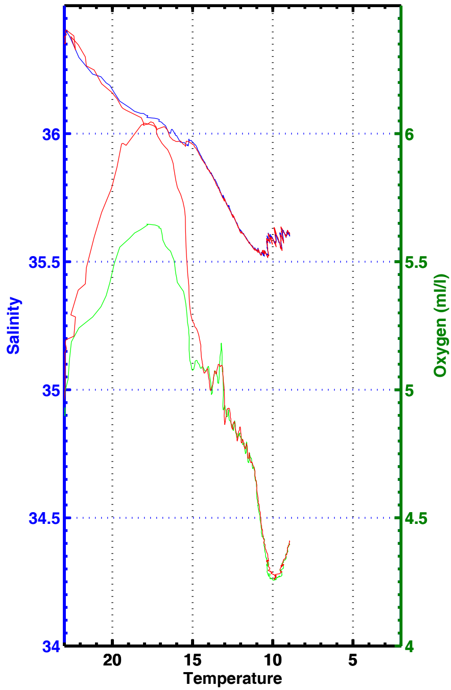
T-S , T-02 , station 3084
