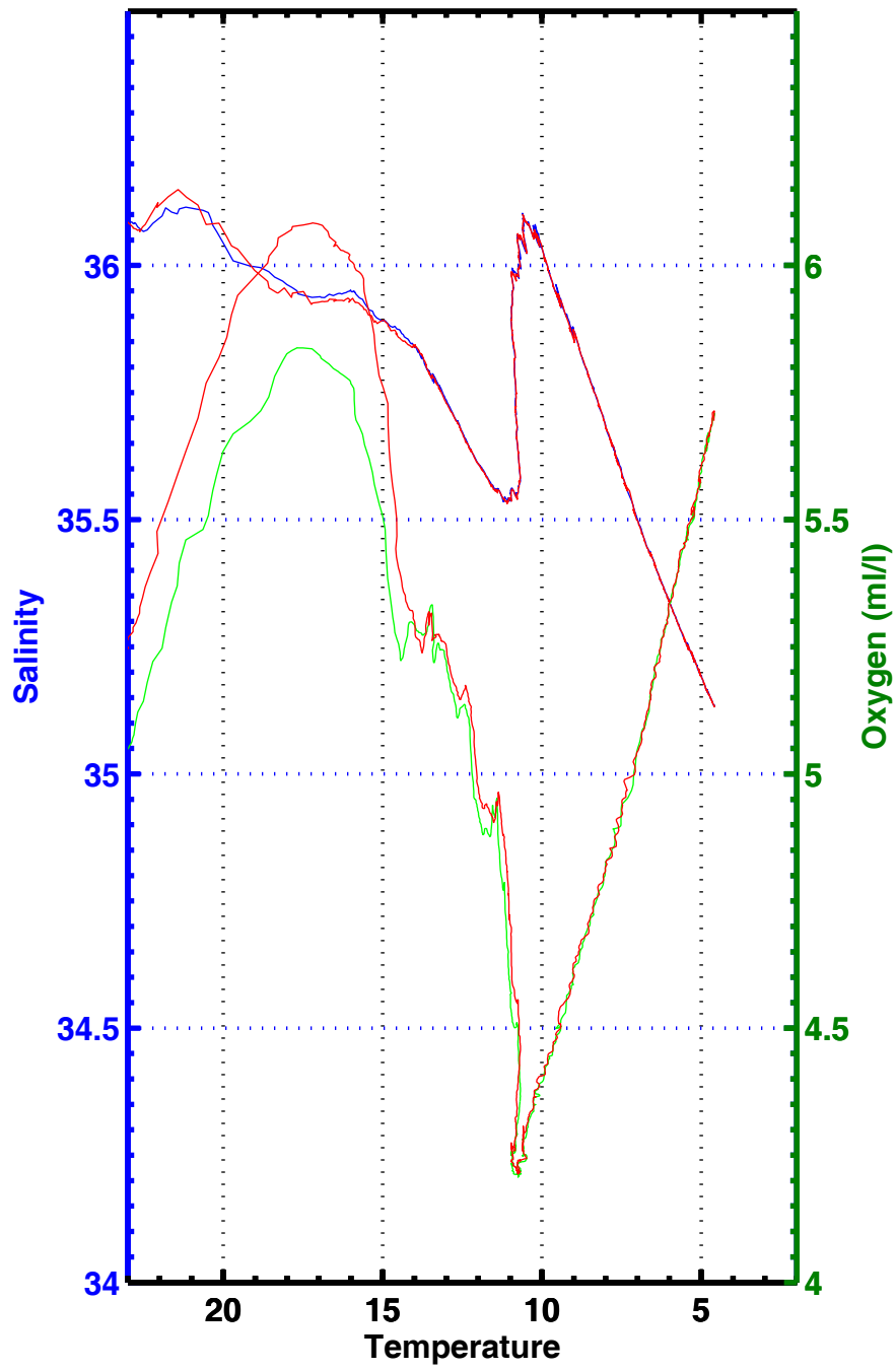
T-S , T-02 , station 3012
