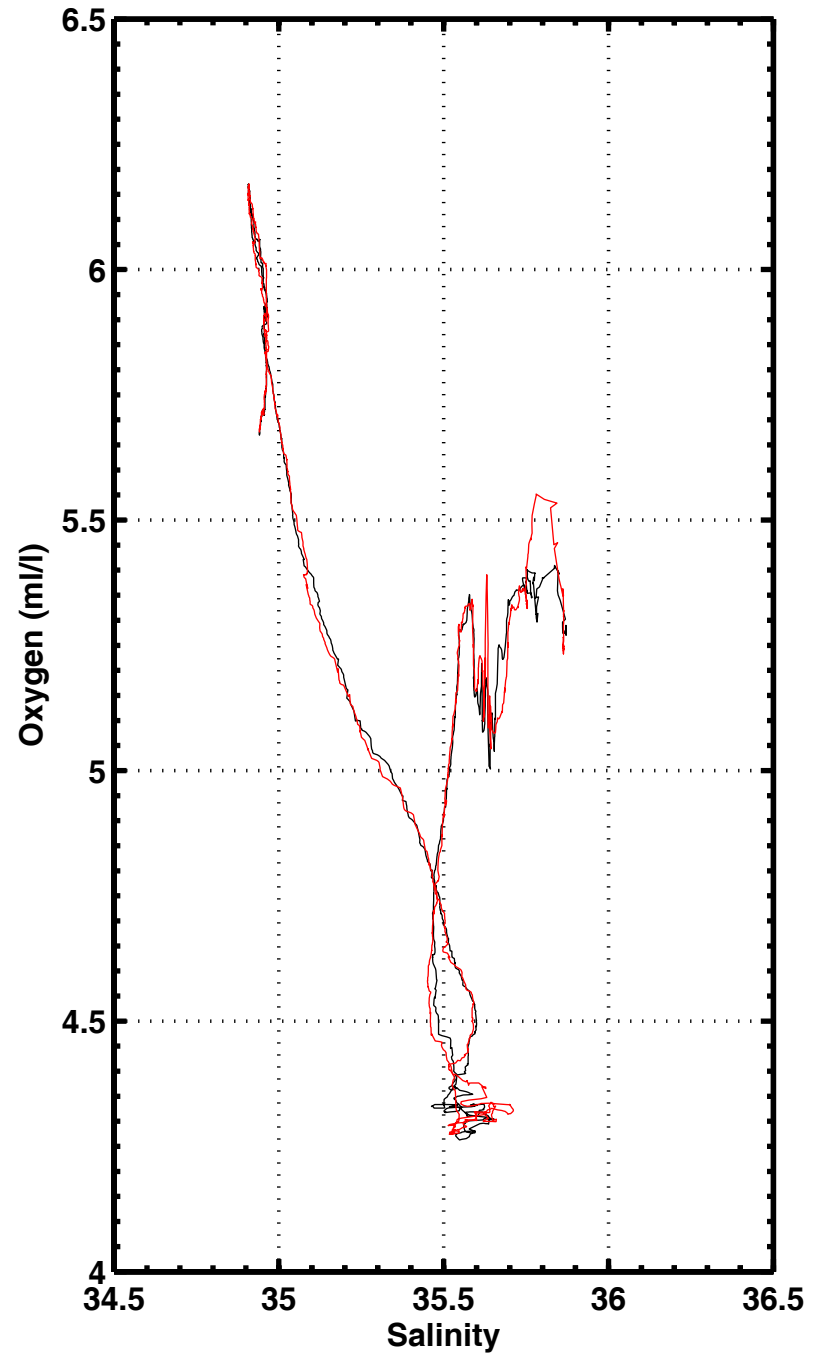
S-O2 , station 3339
