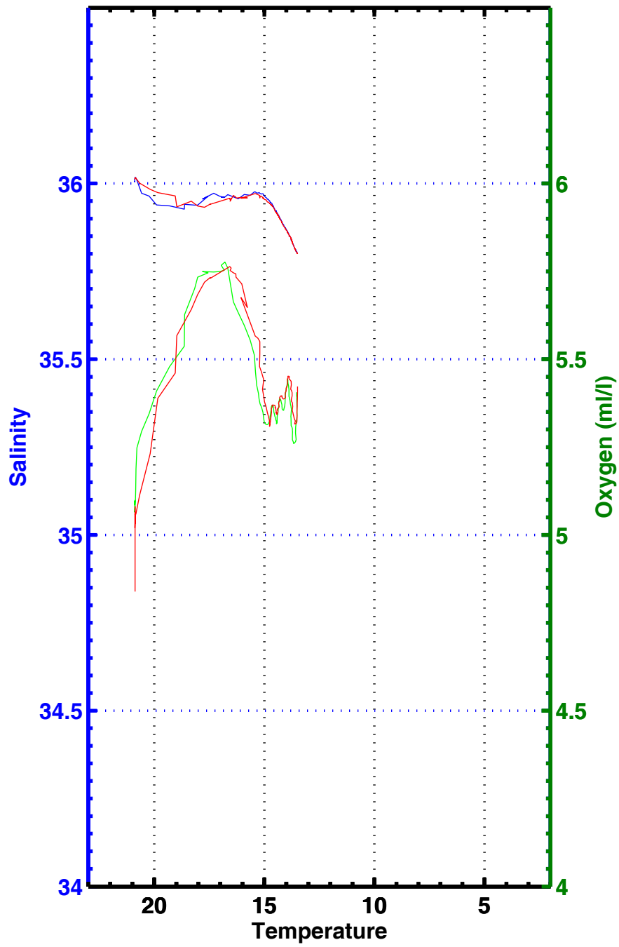
T-S , T-02 , station 3162
