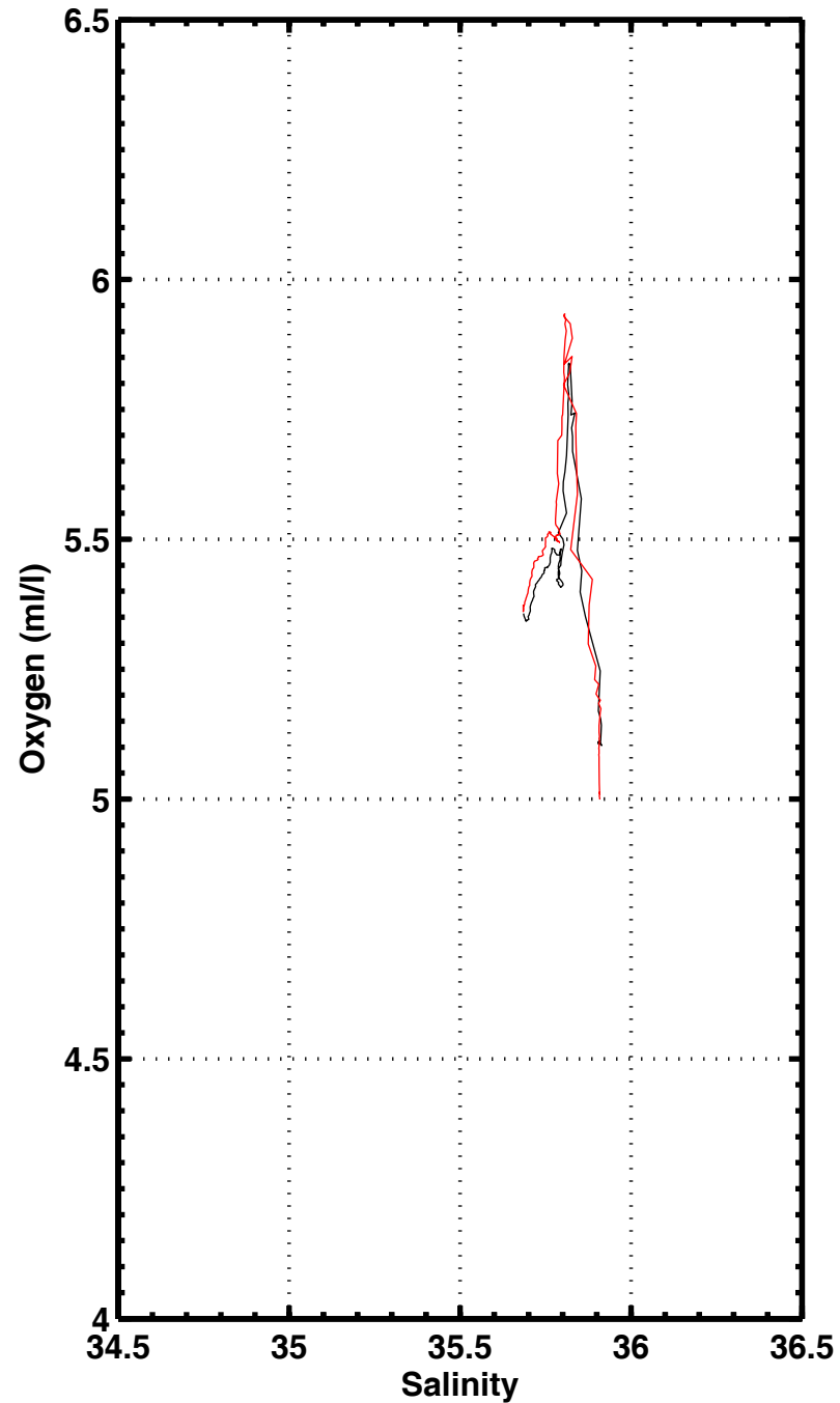
S-02 , station 3240
