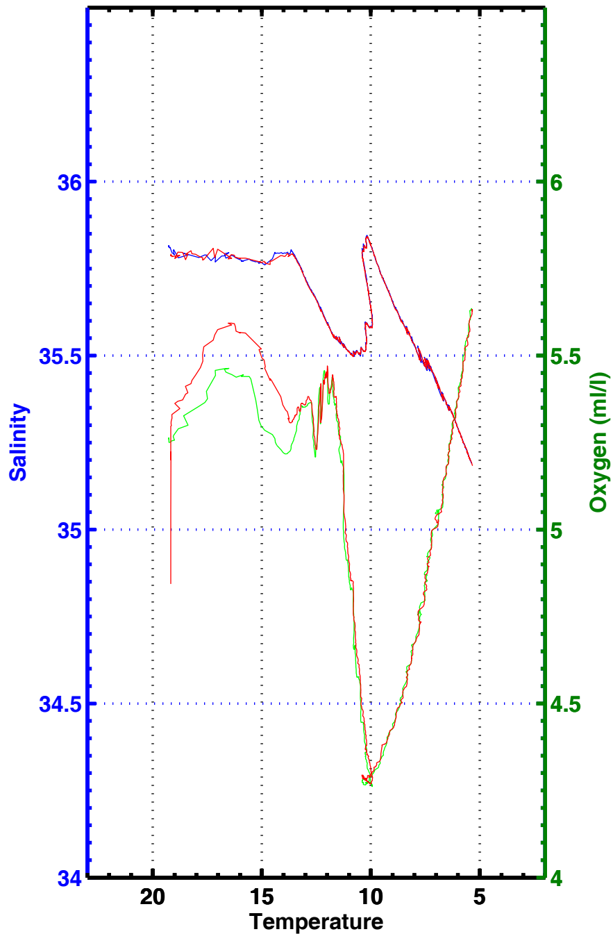
T-S , T-02 , station 3335
