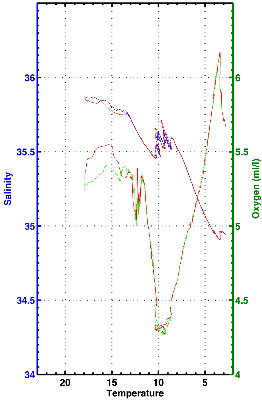
T-S , T-02 , station 3339
