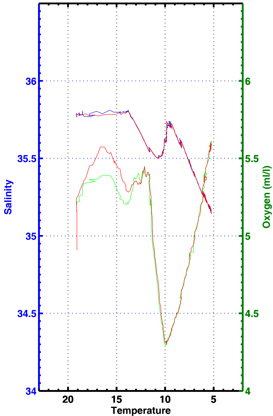
T-S , T-02 , station 3323
