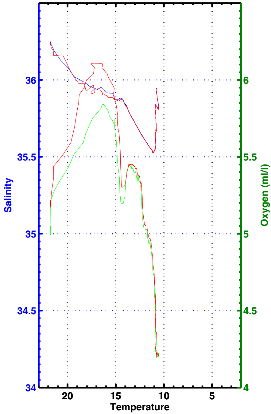
T-S , T-02 , station 3091
