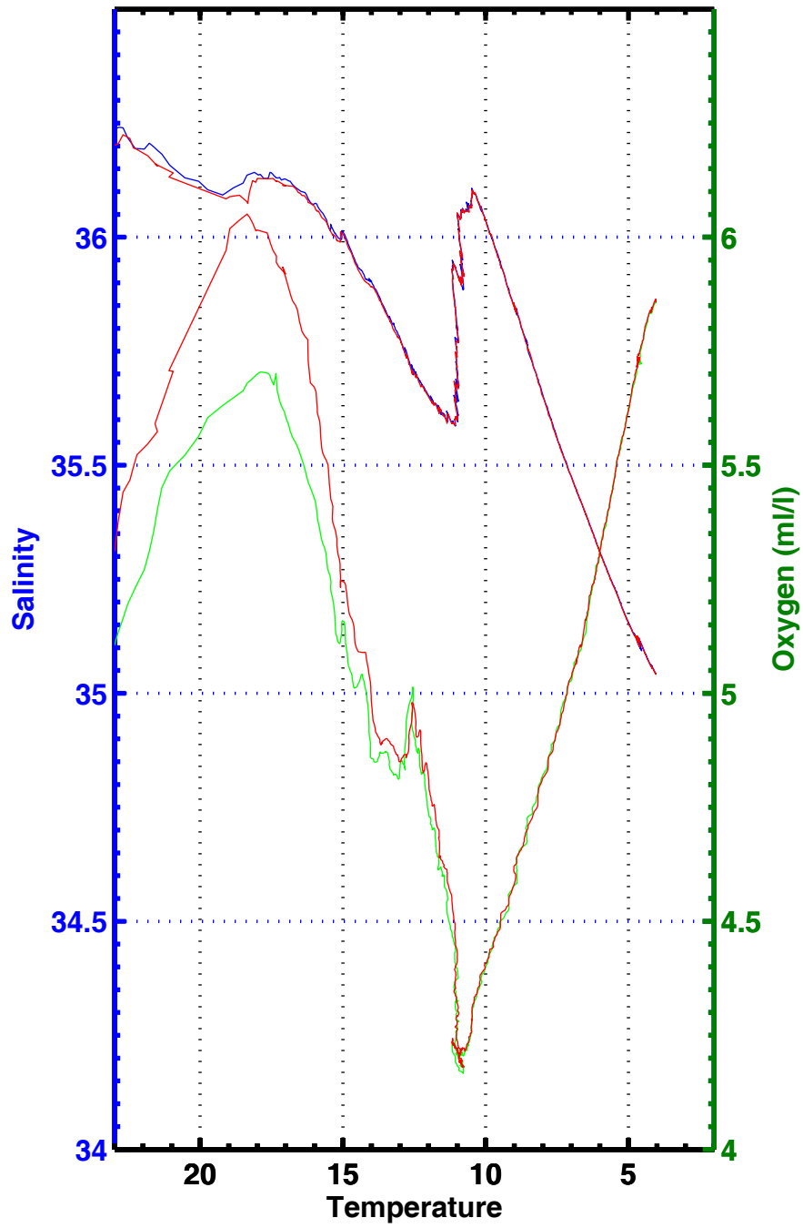
T-S , T-02 , station 3011
