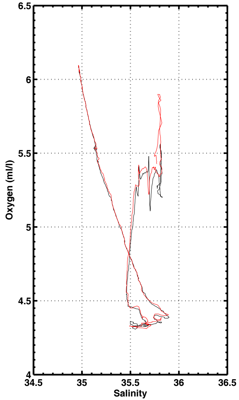
S-O2 , station 3022
