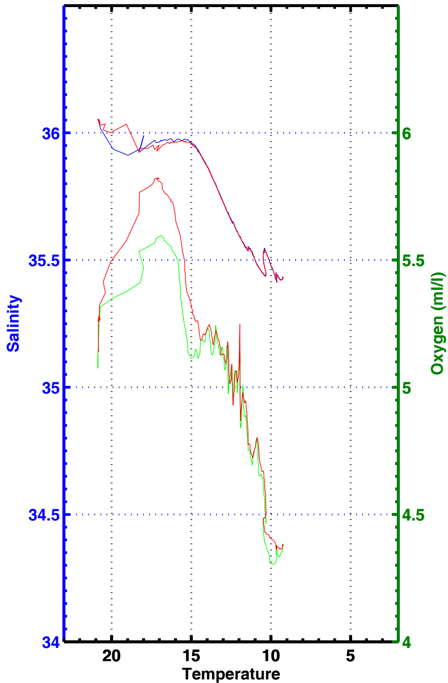
T-S , T-02 , station 3164
