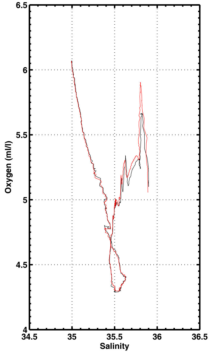
S-O2 , station 3241
