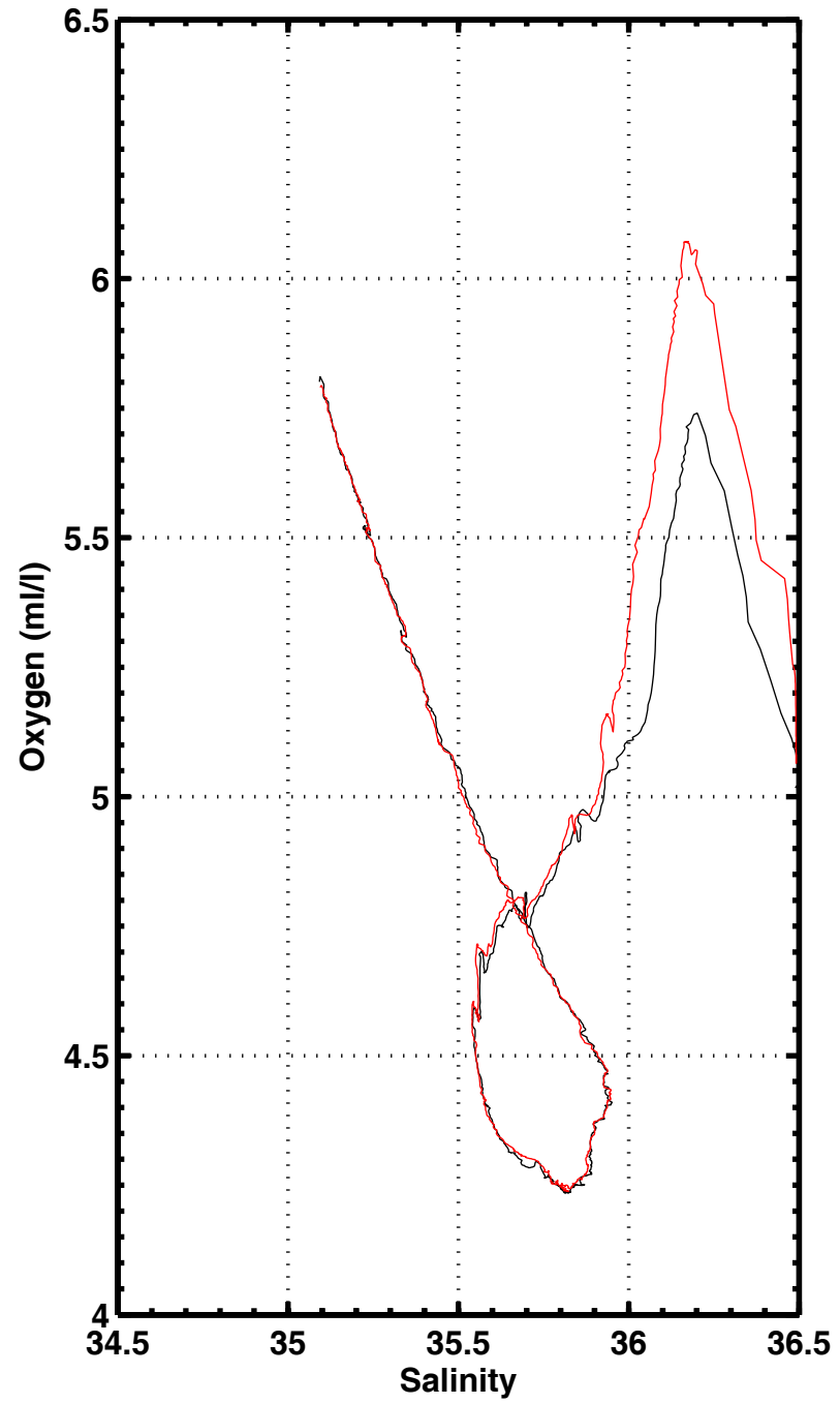
S-O2 , station 3037
