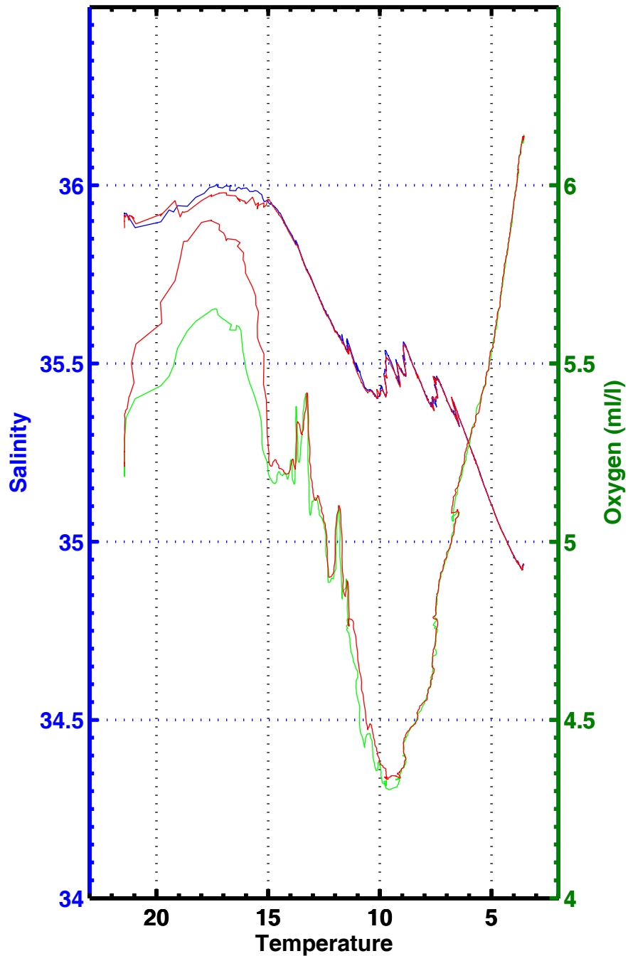
T-S , T-02 , station 3076
