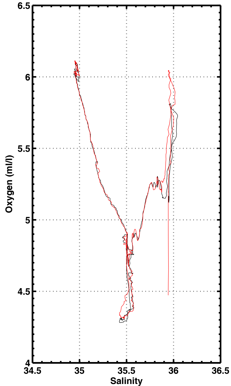
S-02 , station 3019
