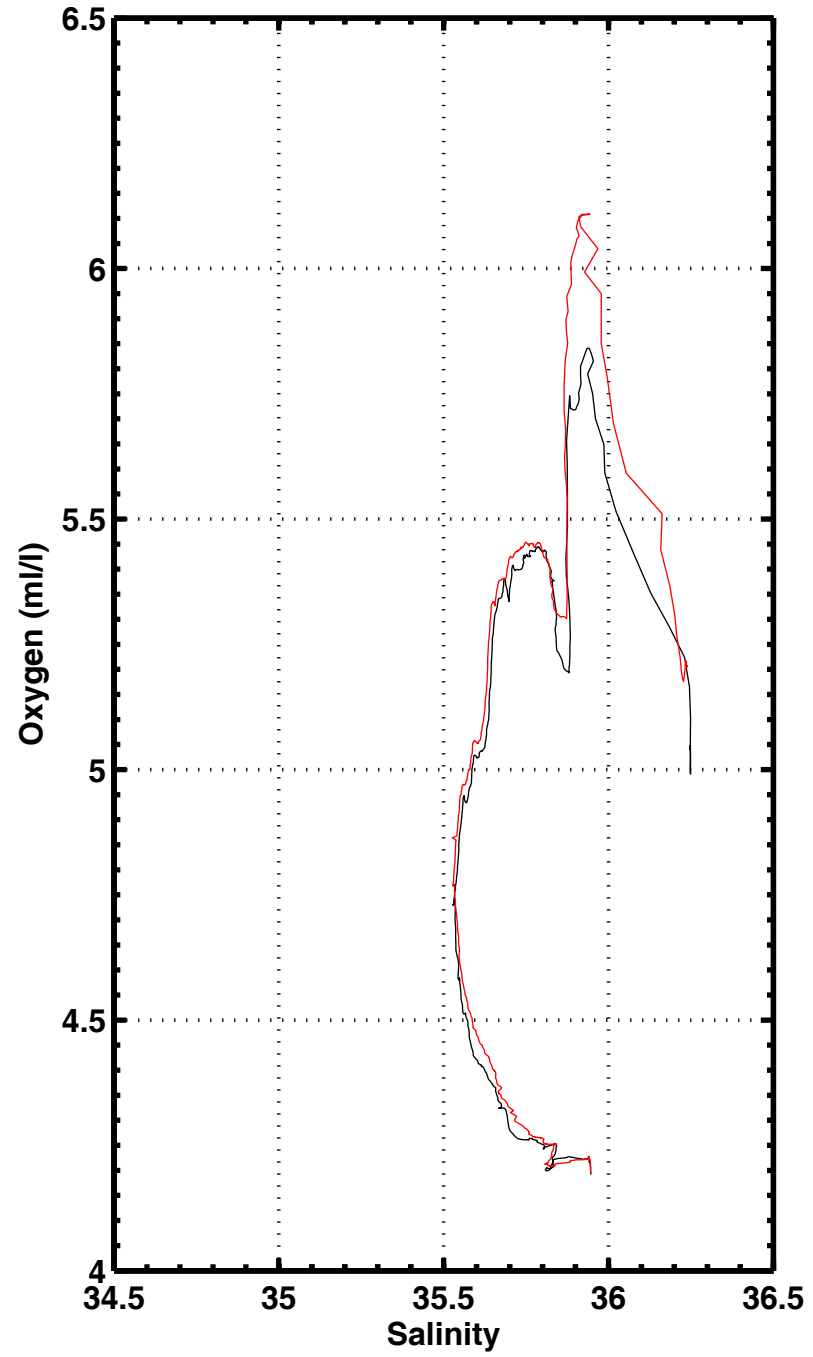
S-02 , station 3091
