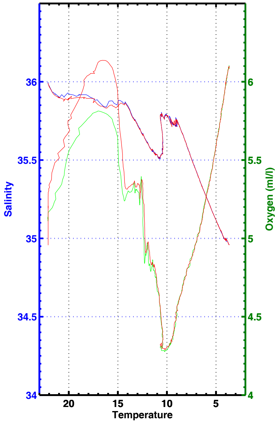
T-S , T-02 , station 3033
