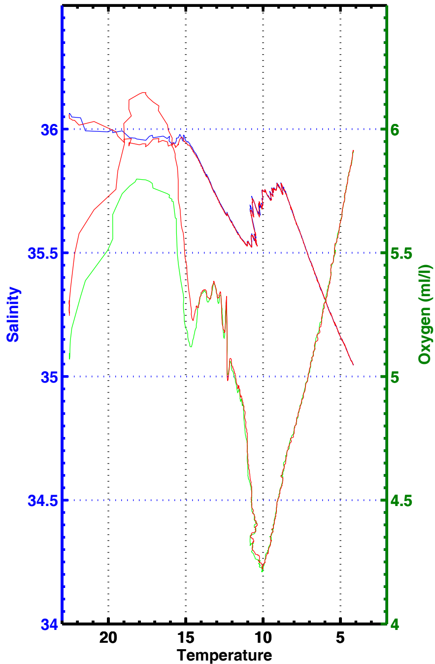
T-S , T-02 , station 3042
