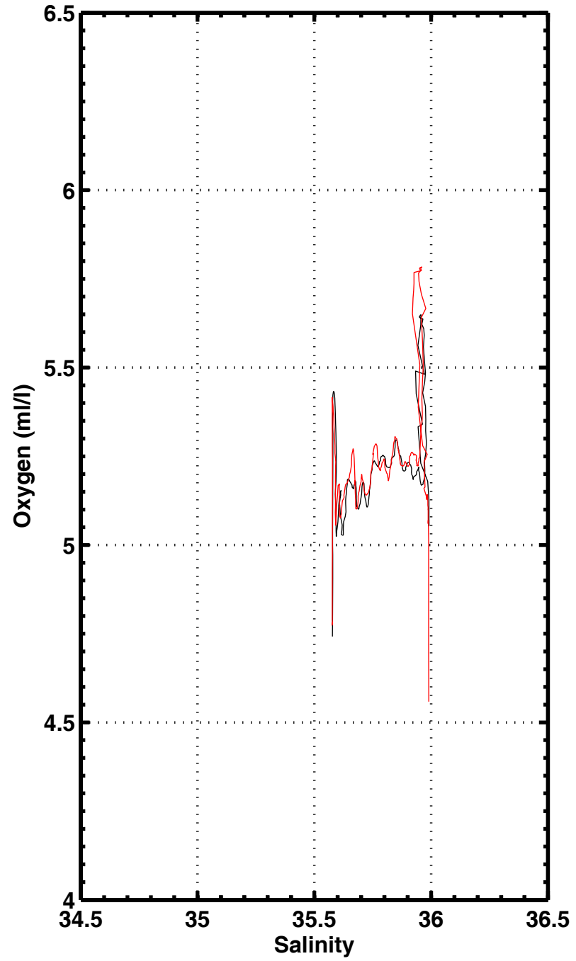
S-02 , station 3161
