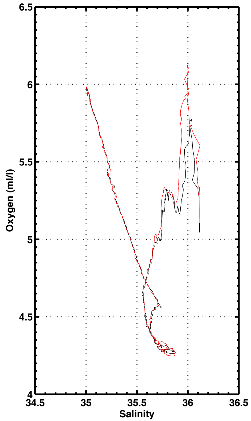
S-02 , station 3040
