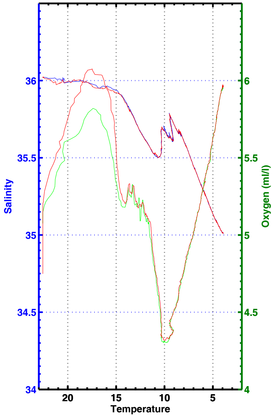
T-S , T-02 , station 3035
