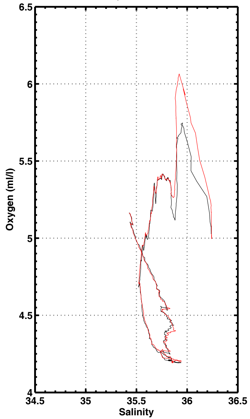
S-O2 , station 3087
