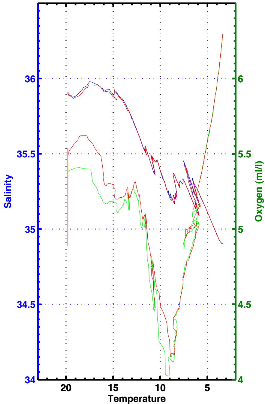
T-S , T-02 , station 3068
