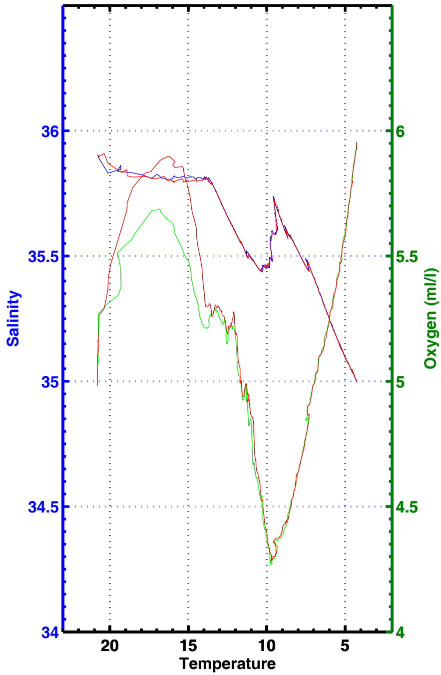
T-S , T-02 , station 3250
