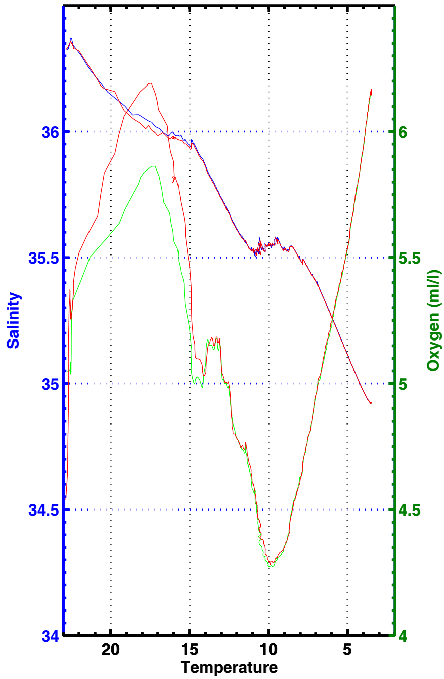
T-S , T-02 , station 3078
