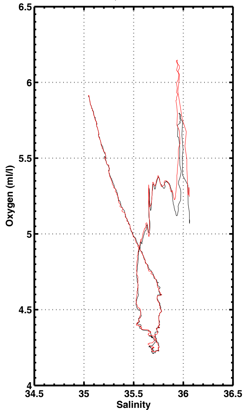
S-O2 , station 3042
