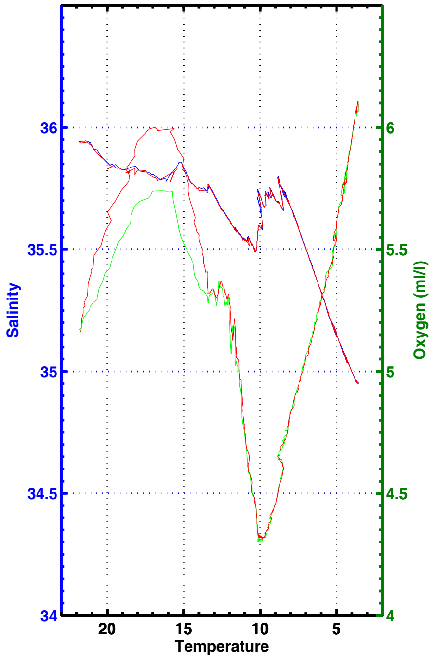
T-S , T-02 , station 3017
