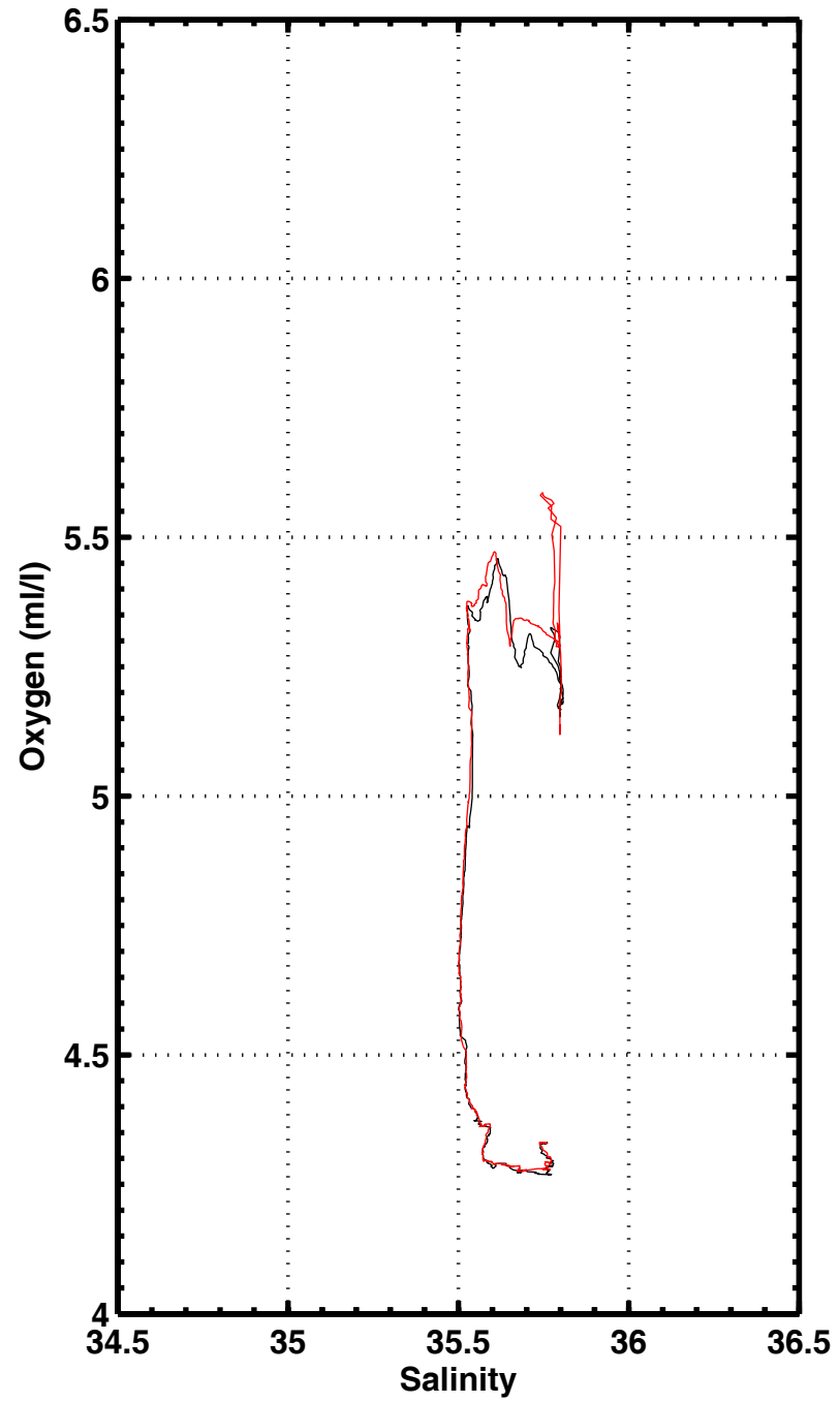
S-02 , station 3328
