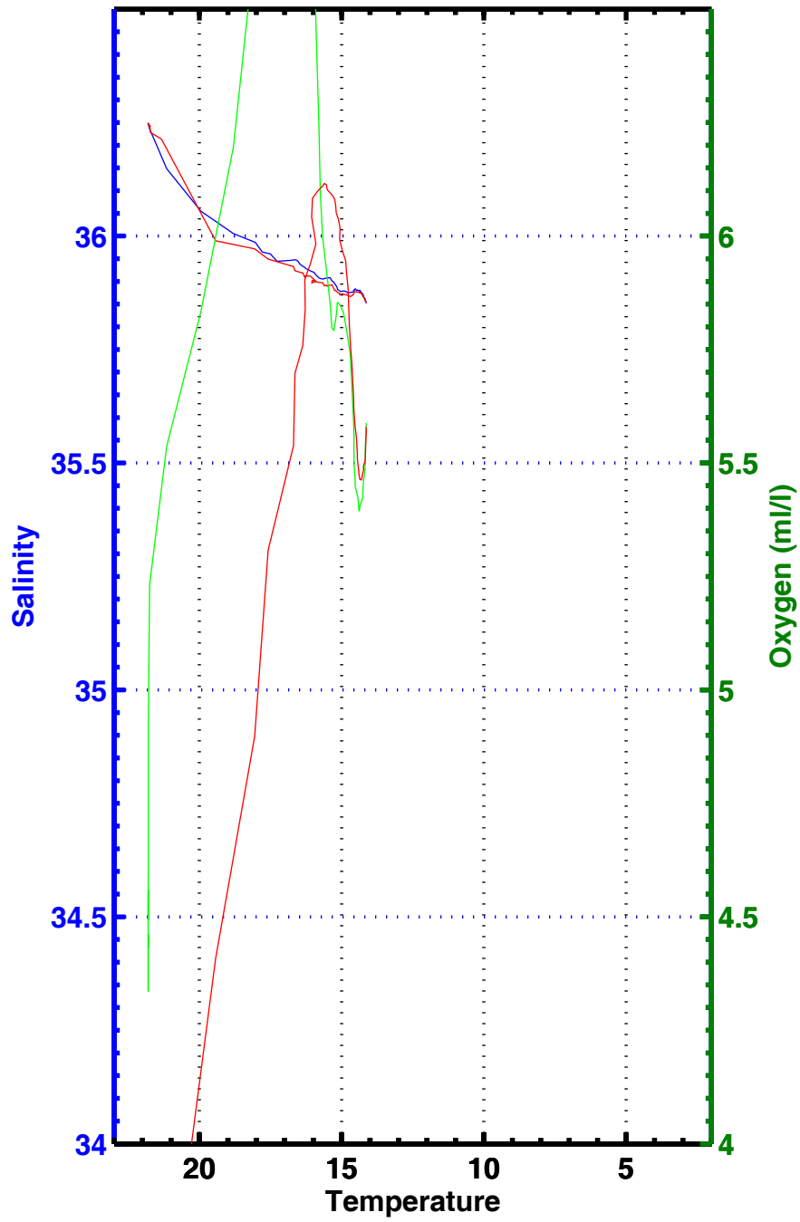
T-S , T-02 , station 3090
