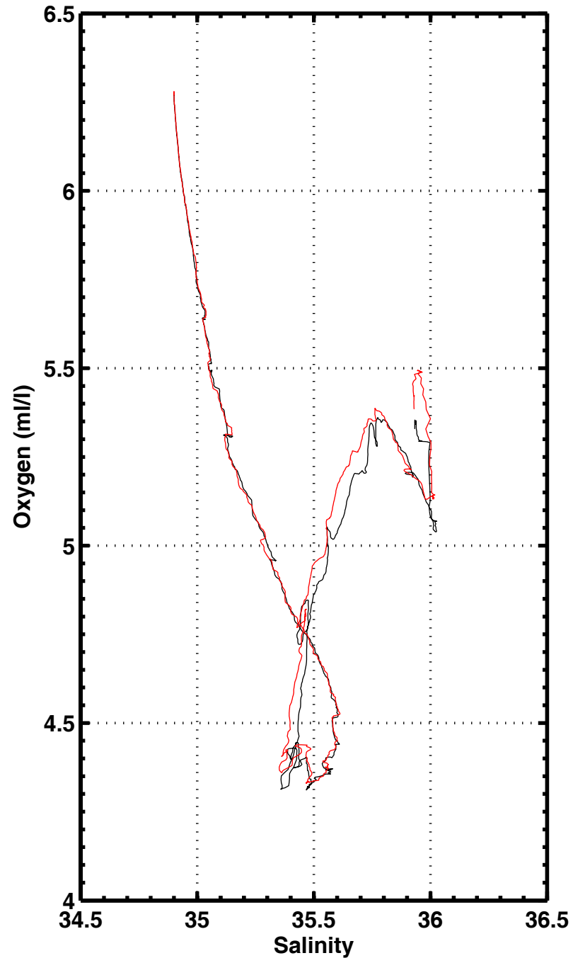
S-O2 , station 3063
