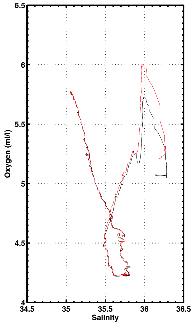
S-O2 , station 3083
