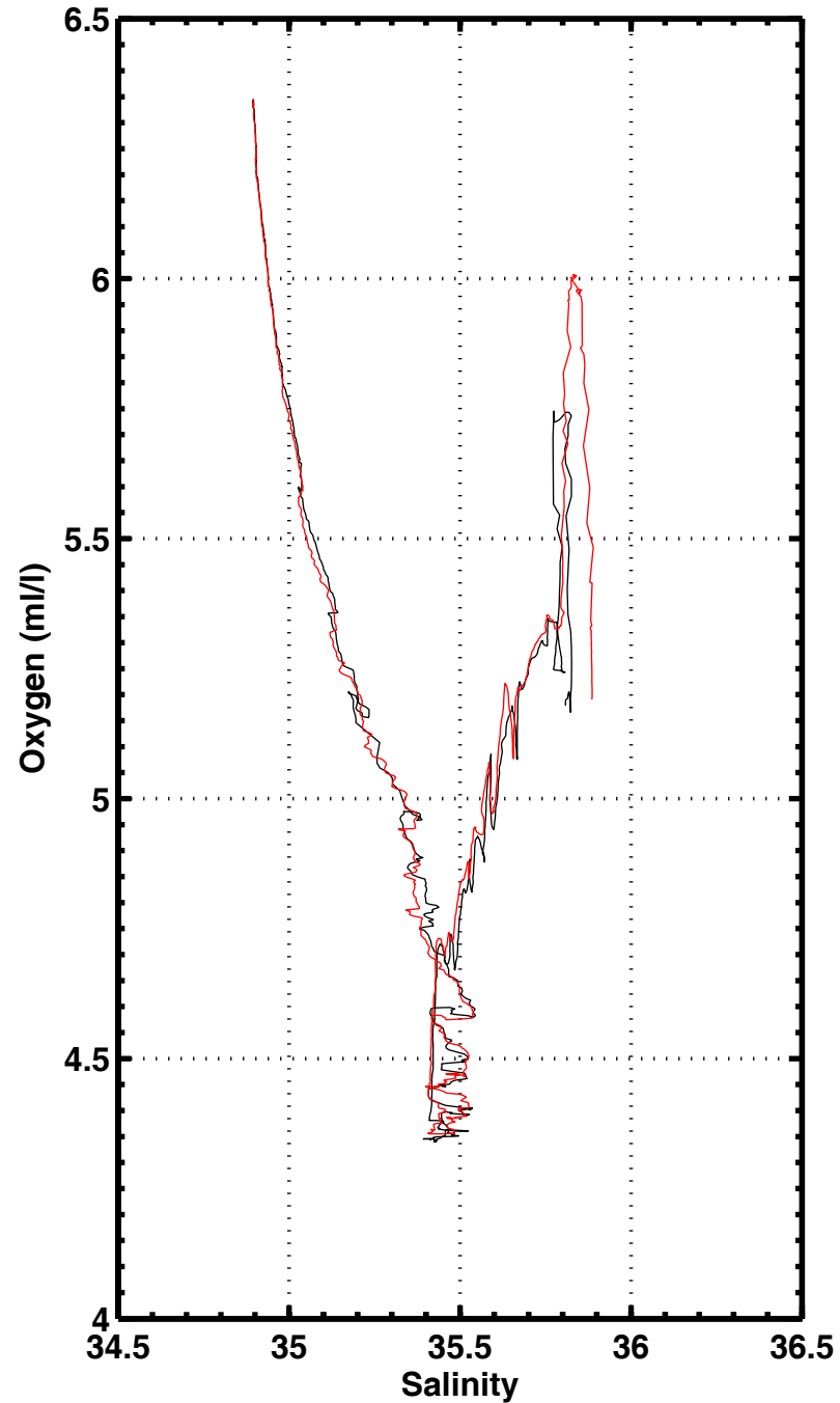
S-02 , station 3071
