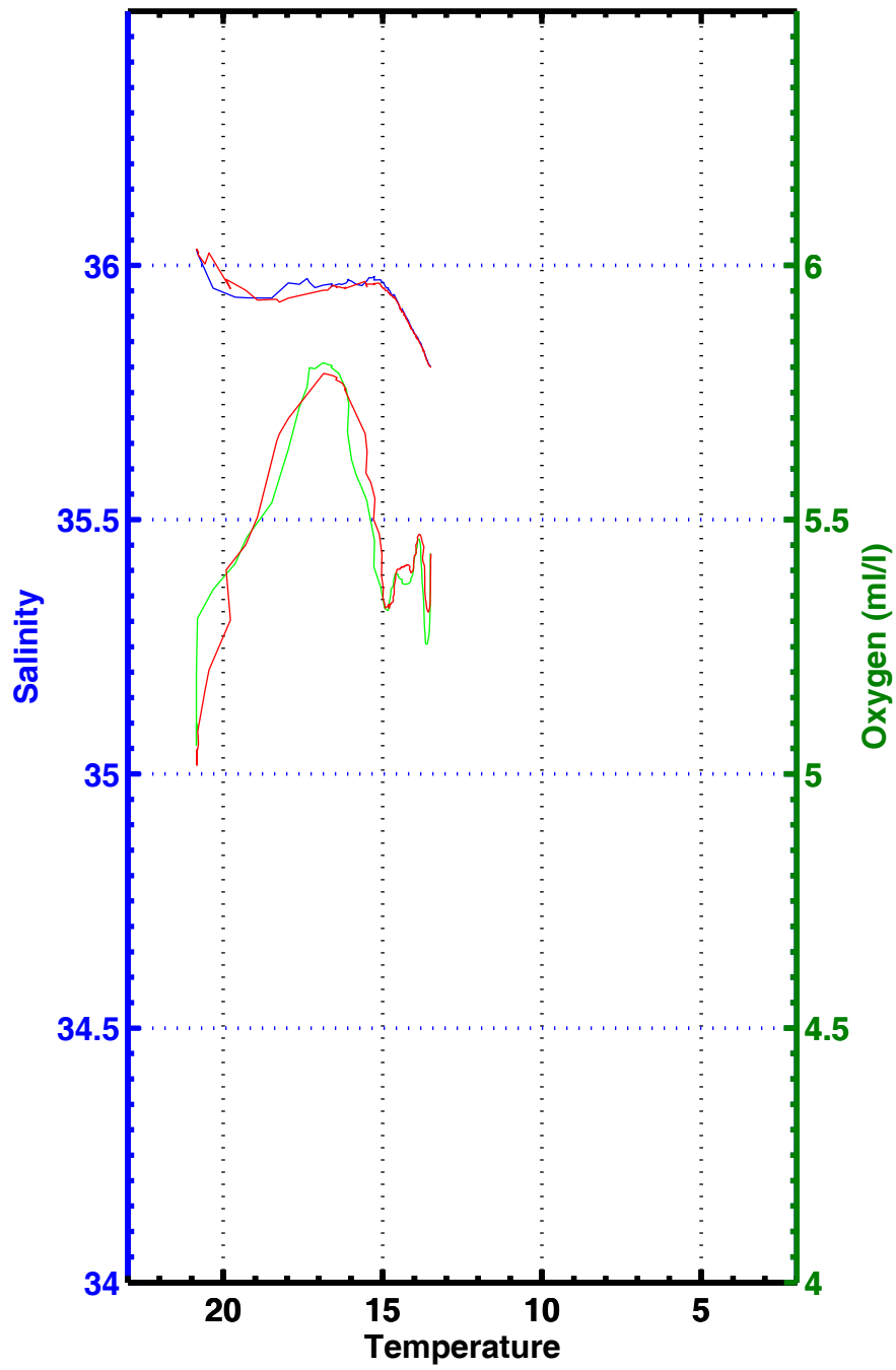
T-S , T-02 , station 3163
