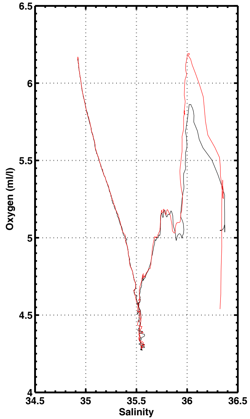
S-O2 , station 3078
