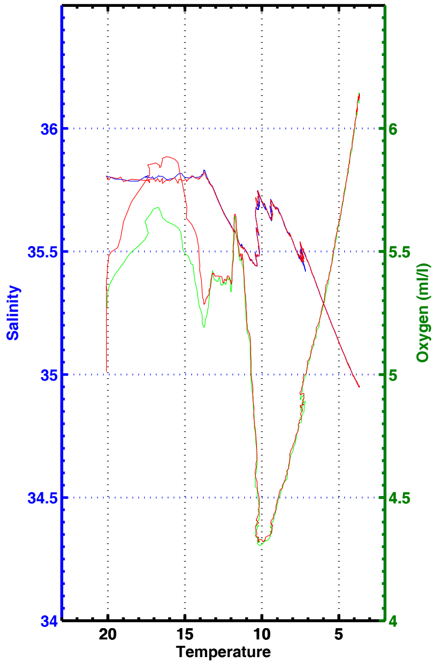
T-S , T-02 , station 3050
