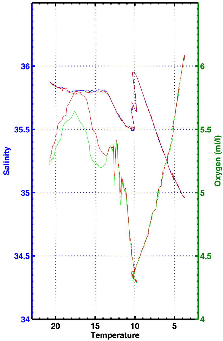
T-S , T-02 , station 3024
