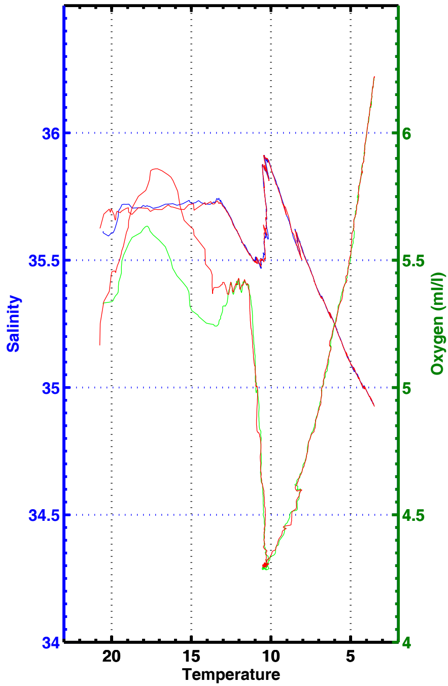
T-S , T-02 , station 3021
