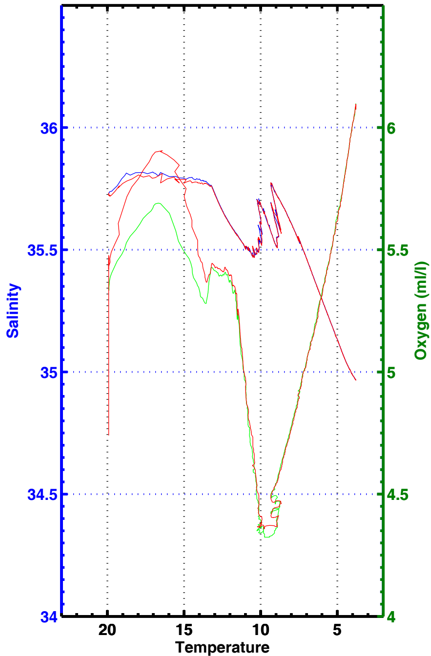
T-S , T-02 , station 3065
