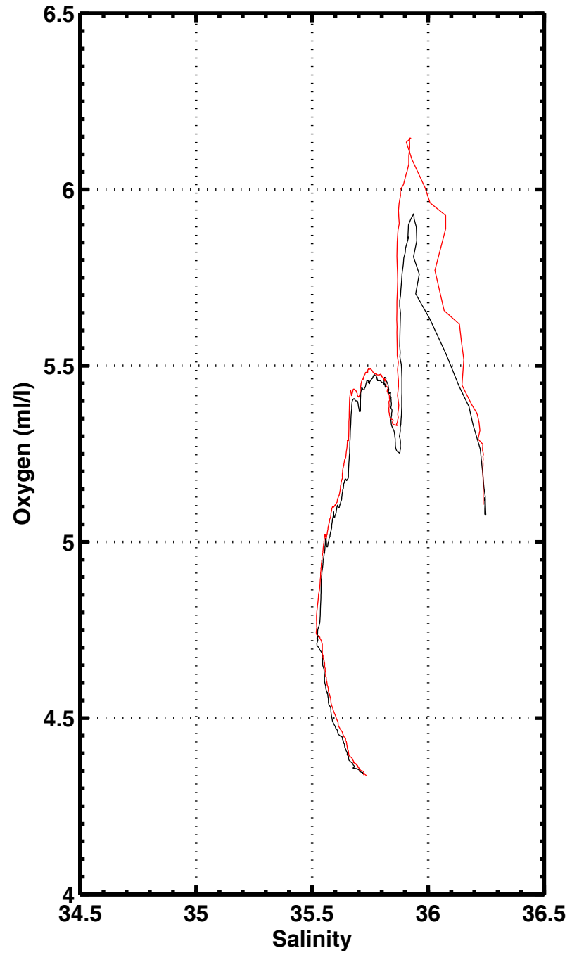
S-02 , station 3095
