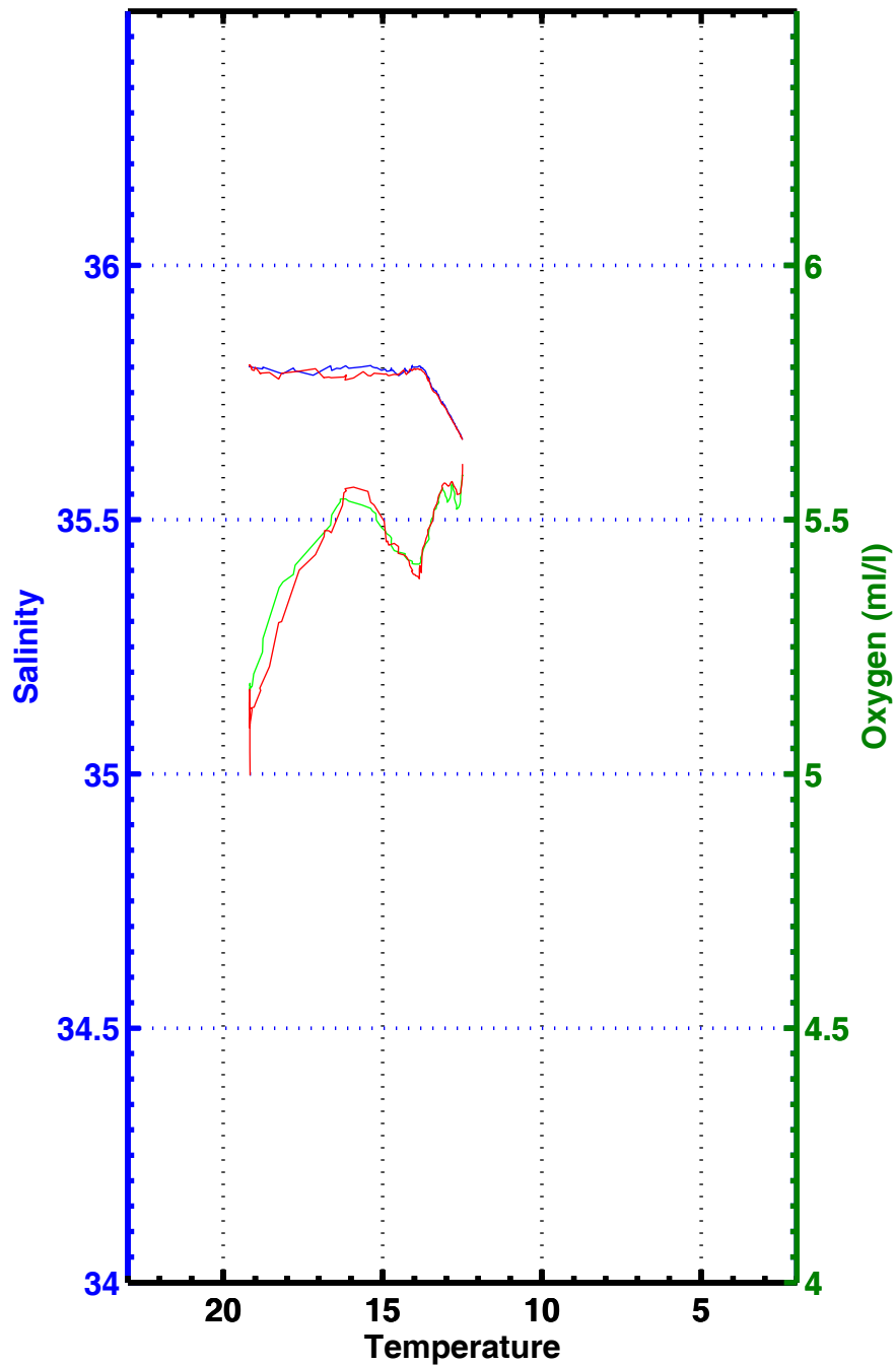
T-S , T-02 , station 3330
