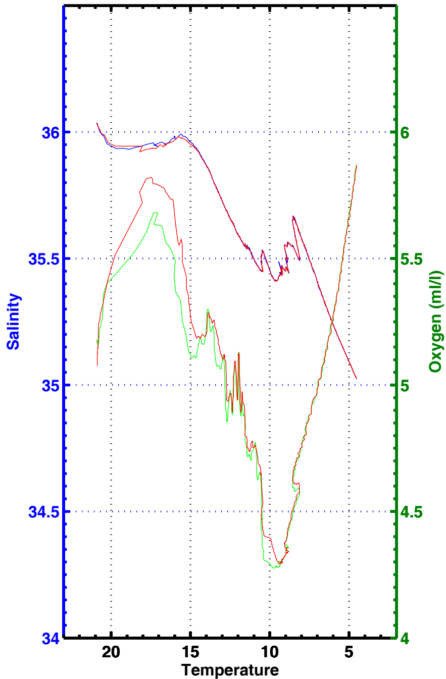
T-S , T-02 , station 3167
