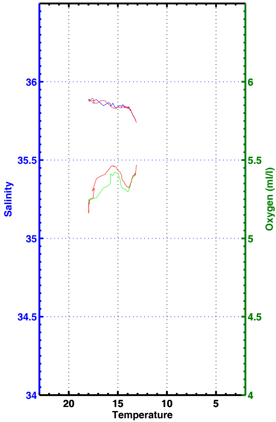
T-S , T-02 , station 3337
