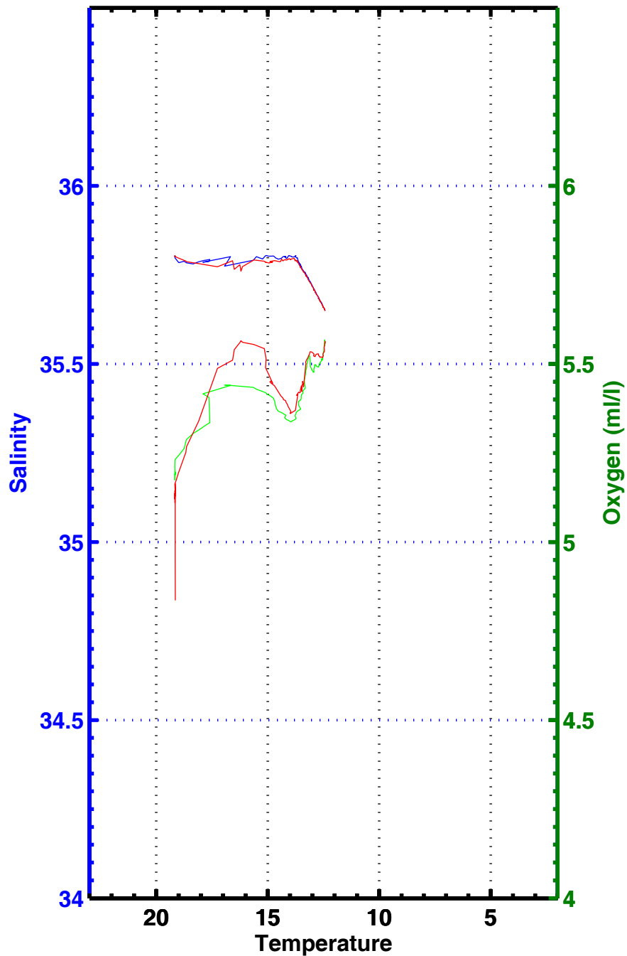
T-S , T-02 , station 3331
