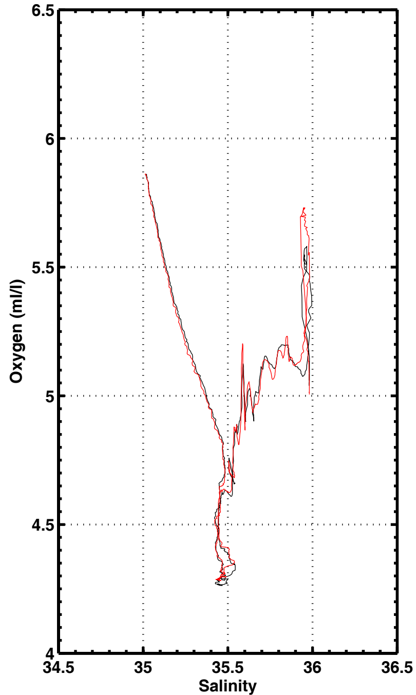
S-O2 , station 3155
