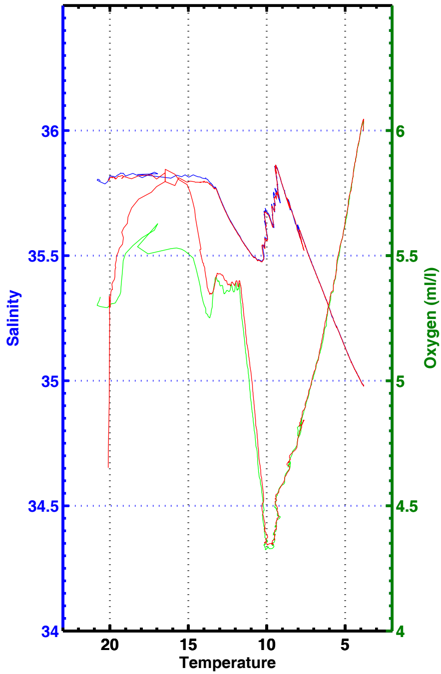
T-S , T-02 , station 3023
