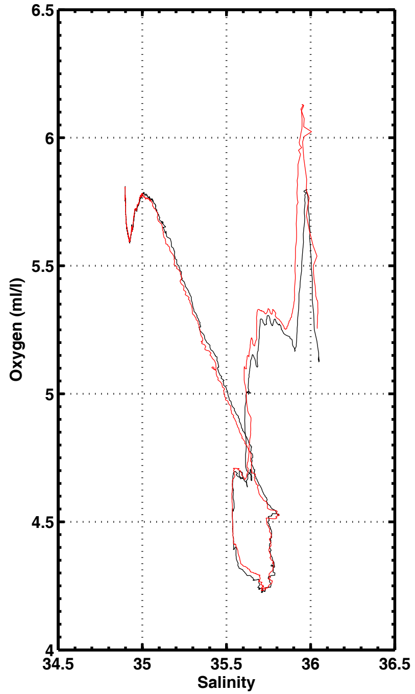
S-O2 , station 3036
