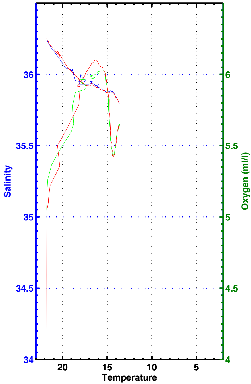
T-S , T-02 , station 3093
