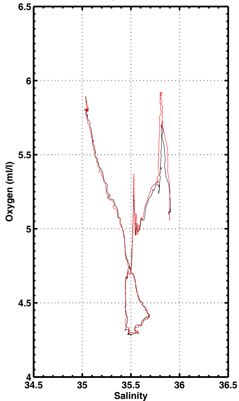
S-O2 , station 3251
