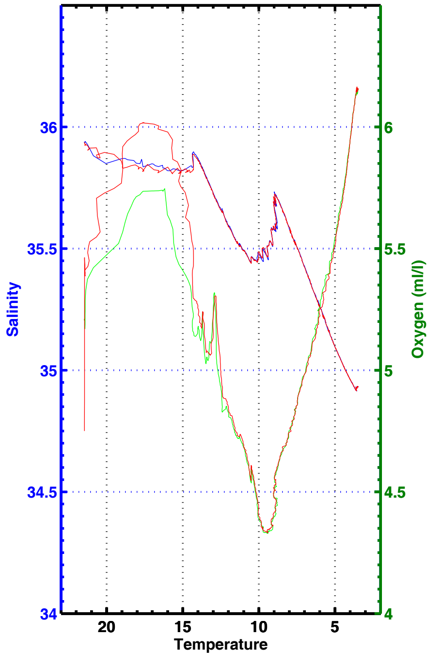
T-S , T-02 , station 3073
