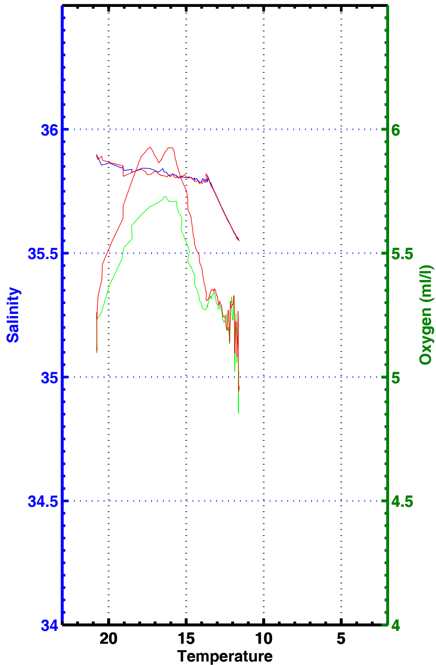
T-S , T-02 , station 3245
