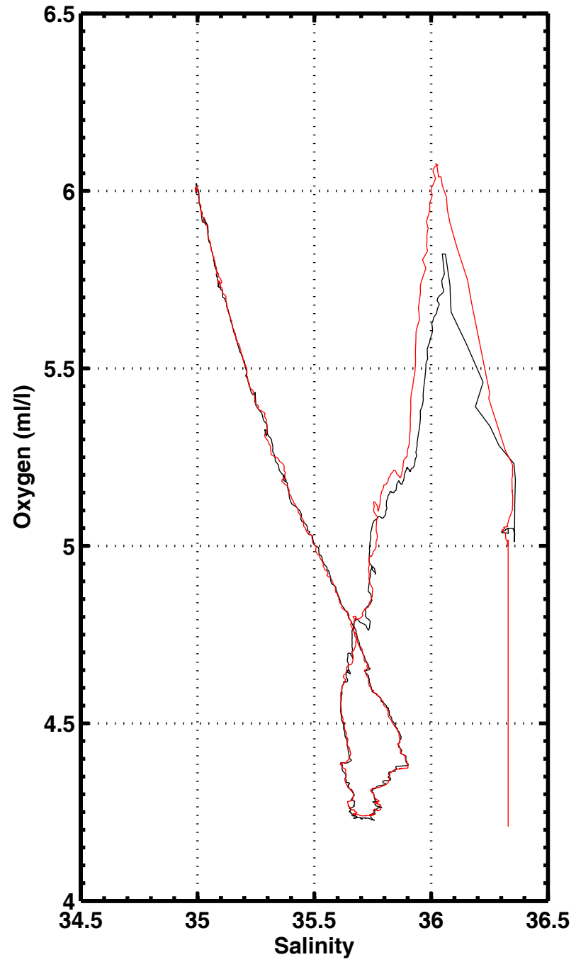
S-O2 , station 3081
