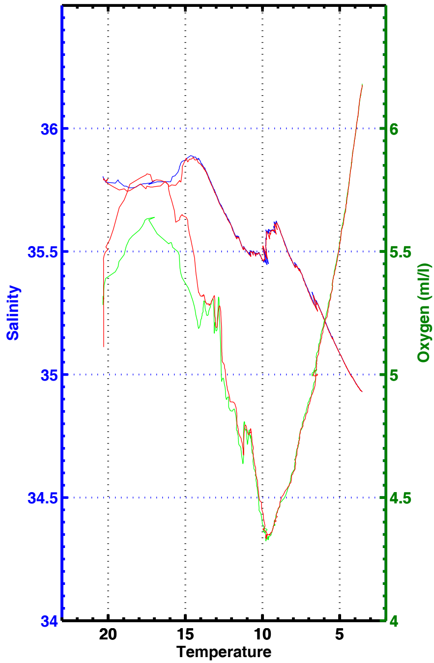
T-S , T-02 , station 3064
