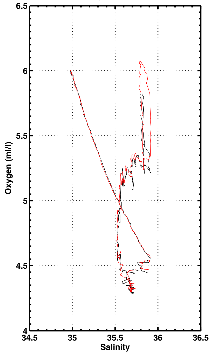
S-O2 , station 3008
