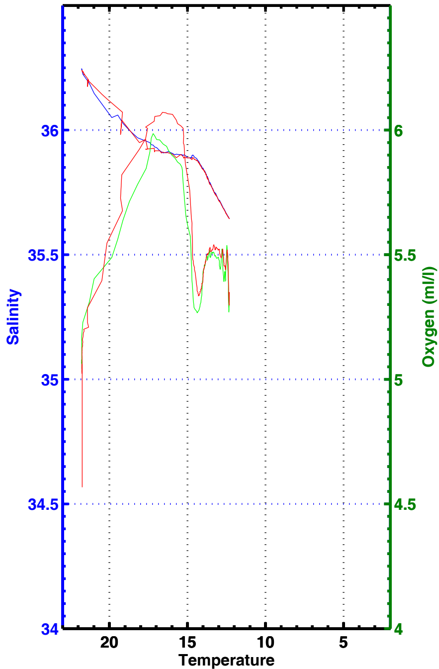
T-S , T-02 , station 3092
