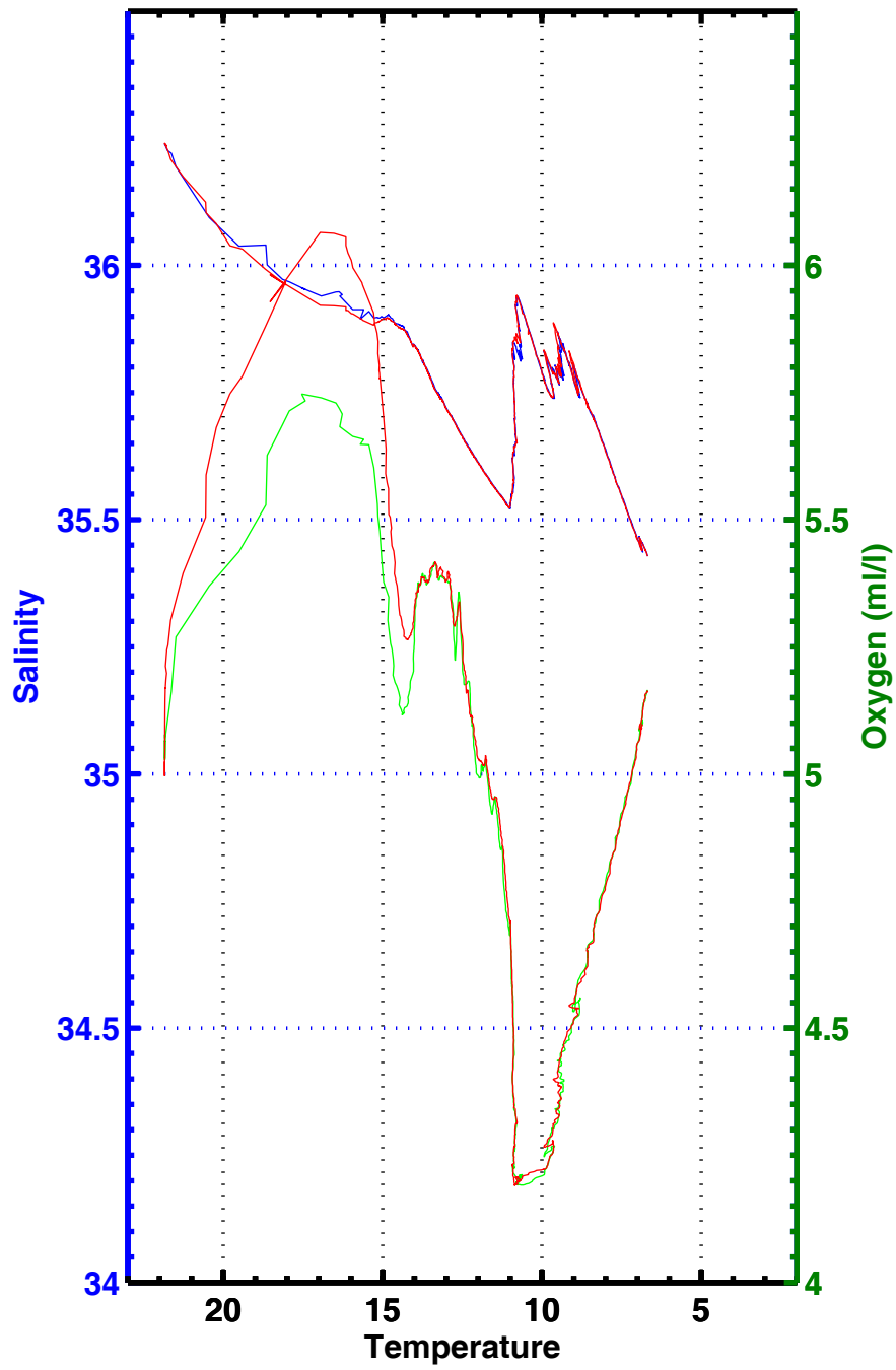
T-S , T-02 , station 3087
