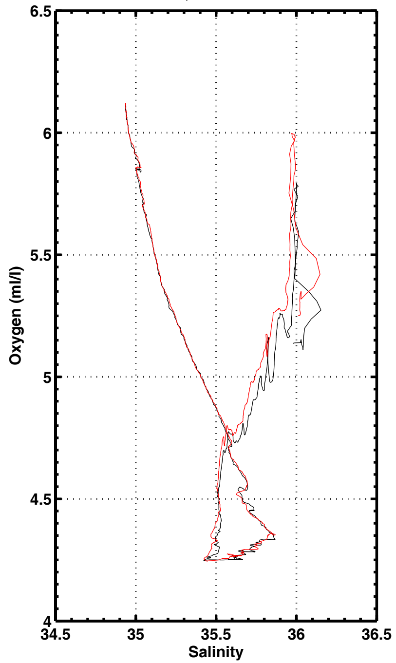
S-O2 , station 3080
