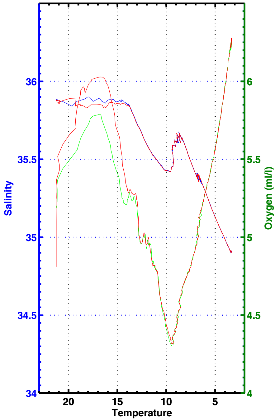
T-S , T-02 , station 3060
