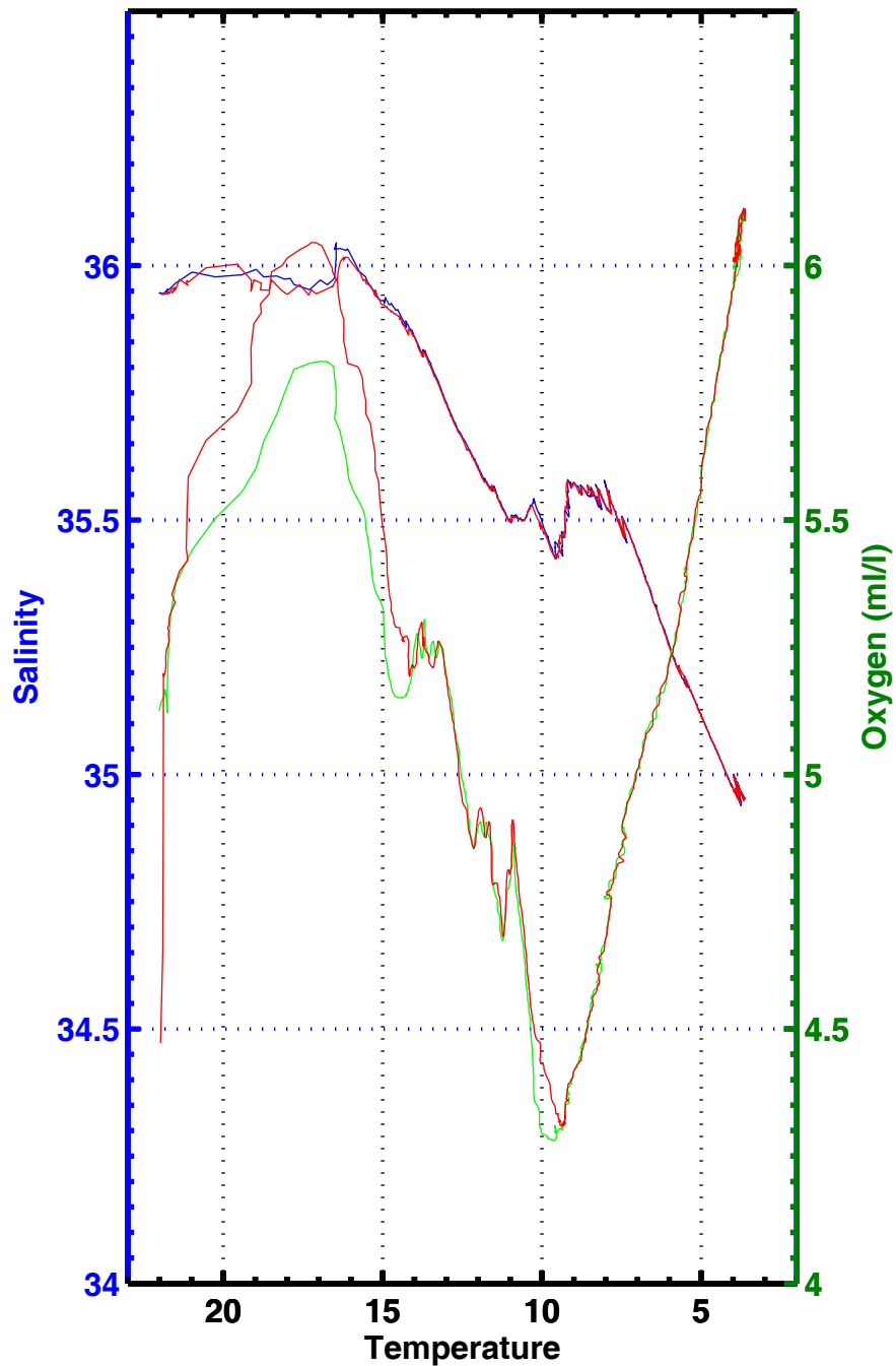
T-S , T-02 , station 3019
