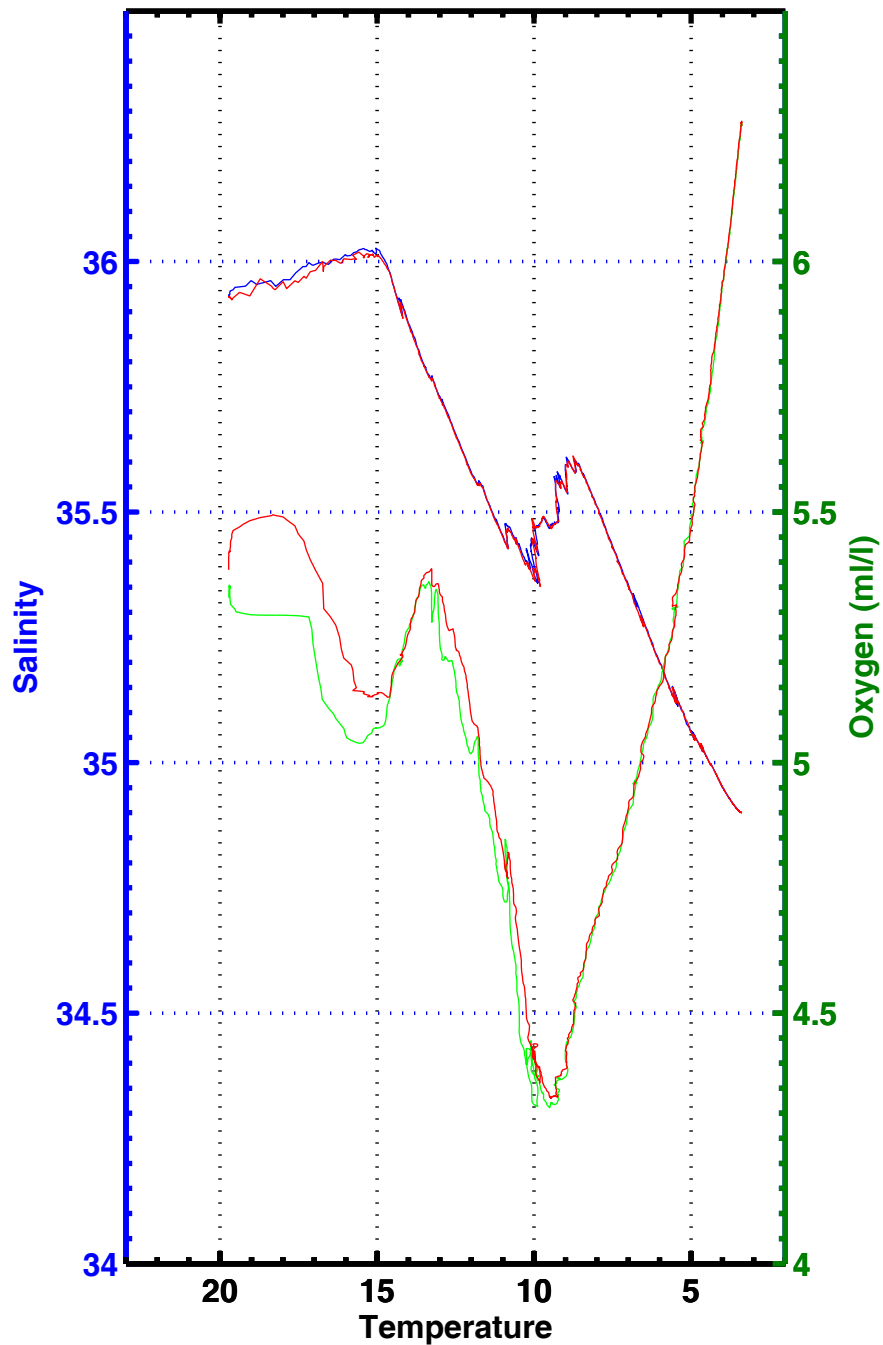
T-S , T-02 , station 3063
