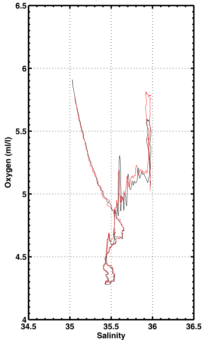
S-O2 , station 3157
