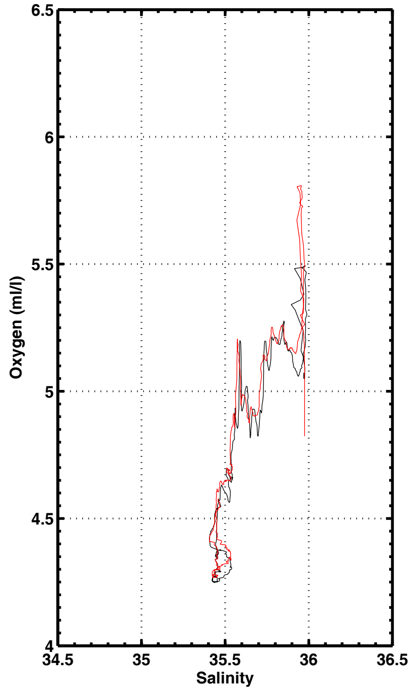
S-02 , station 3160
