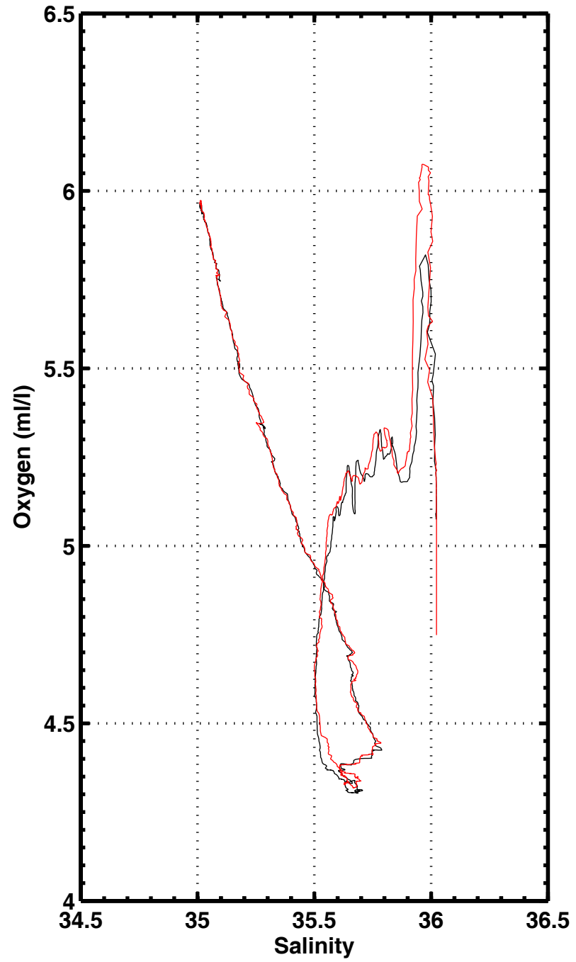
S-O2 , station 3035
