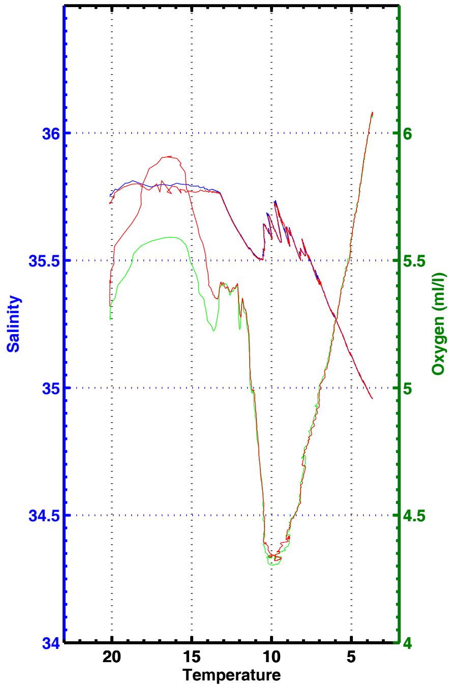
T-S , T-02 , station 3049
