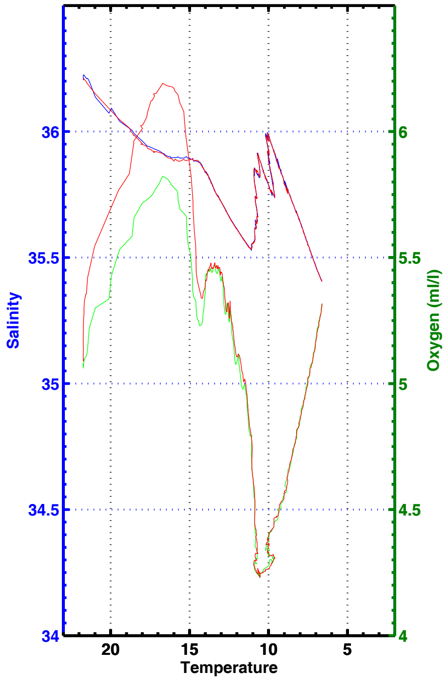
T-S , T-02 , station 3097
