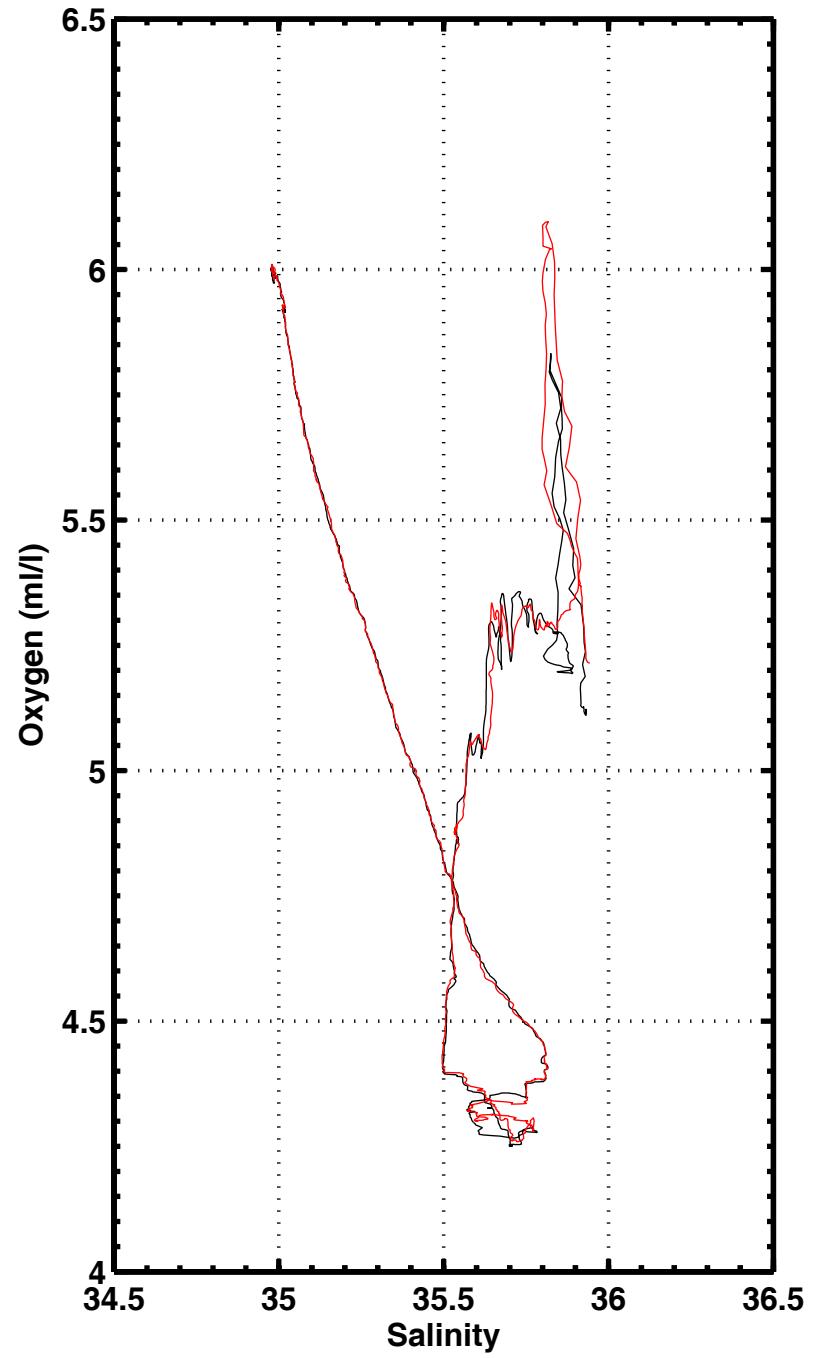
S-O2 , station 3015
