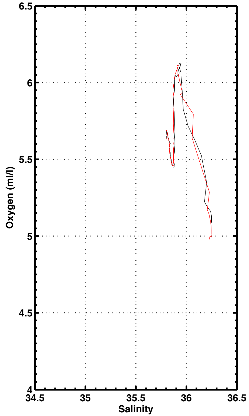
S-02 , station 3094
