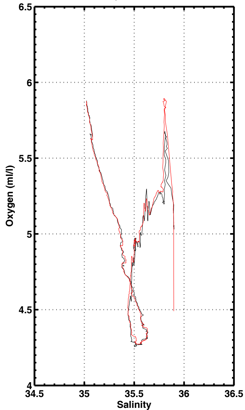
S-O2 , station 3243
