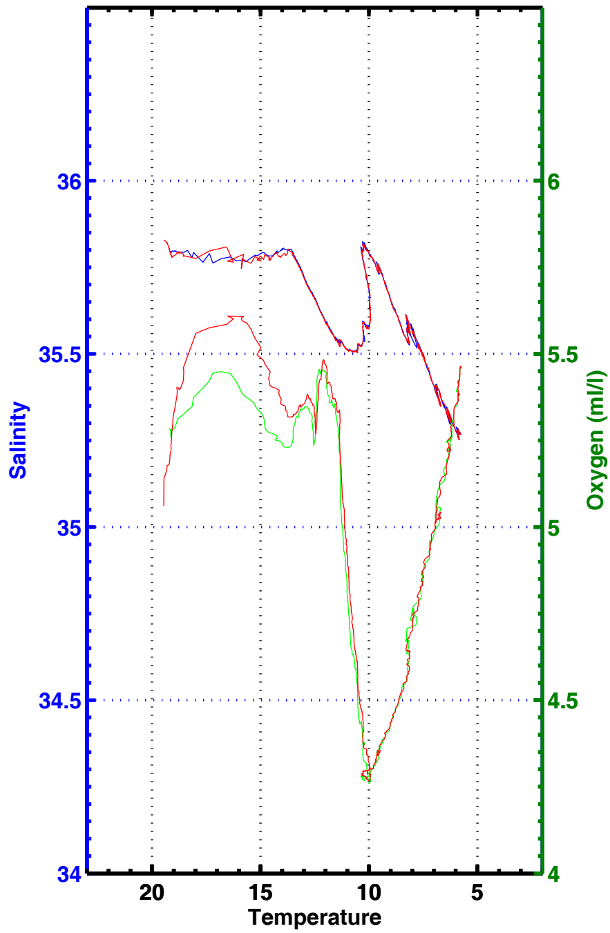
T-S , T-02 , station 3334
