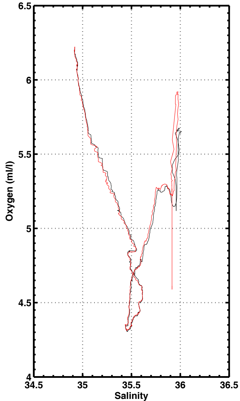
S-O2 , station 3048
