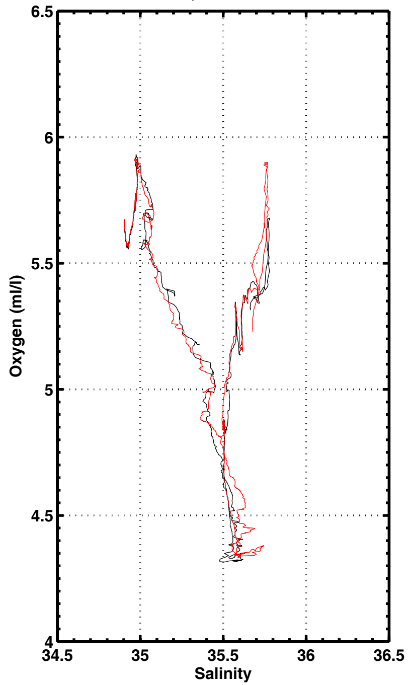
S-O2 , station 3004
