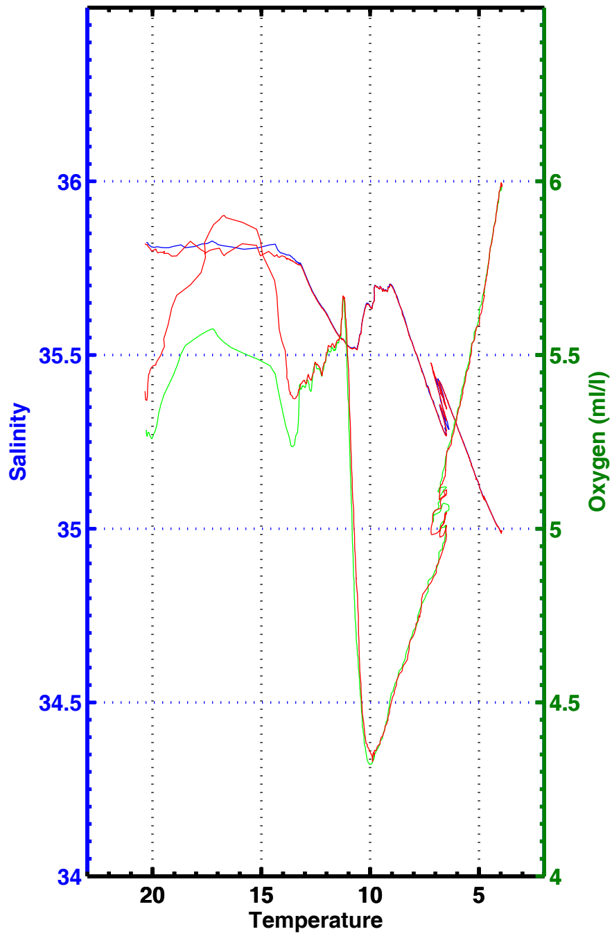
T-S , T-02 , station 3026
