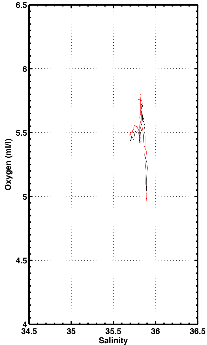
S-02 , station 3247
