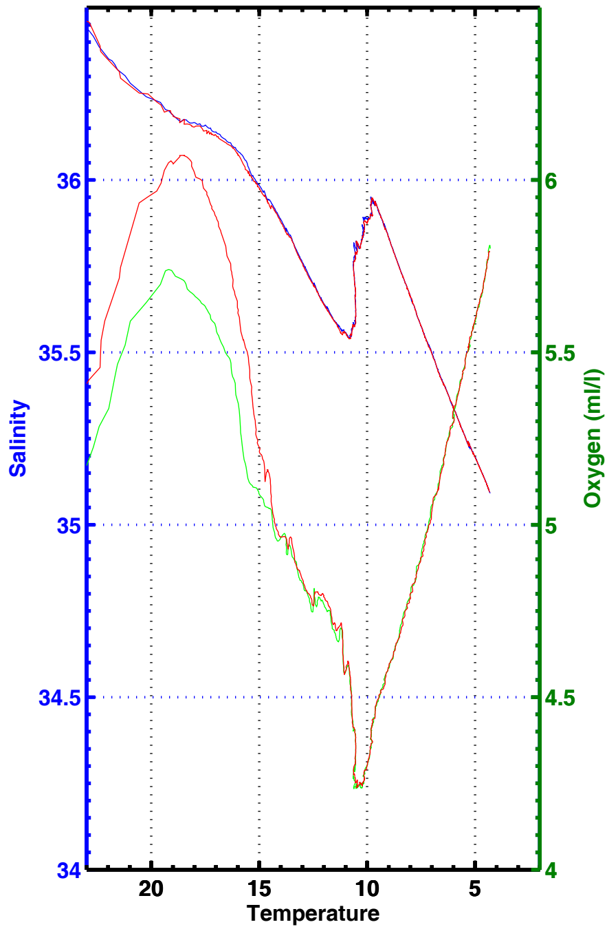
T-S , T-02 , station 3037
