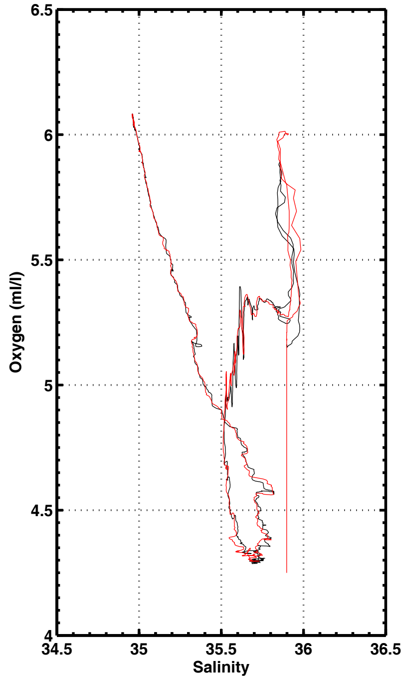
S-O2 , station 3032
