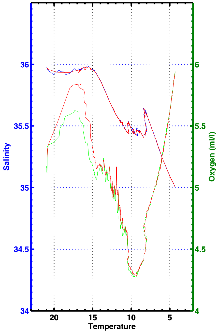
T-S , T-02 , station 3159
