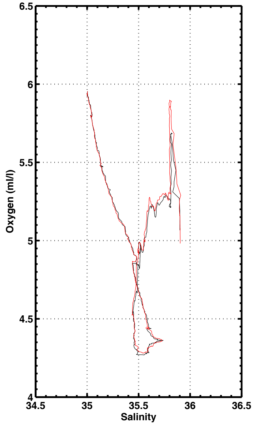
S-O2 , station 3250
