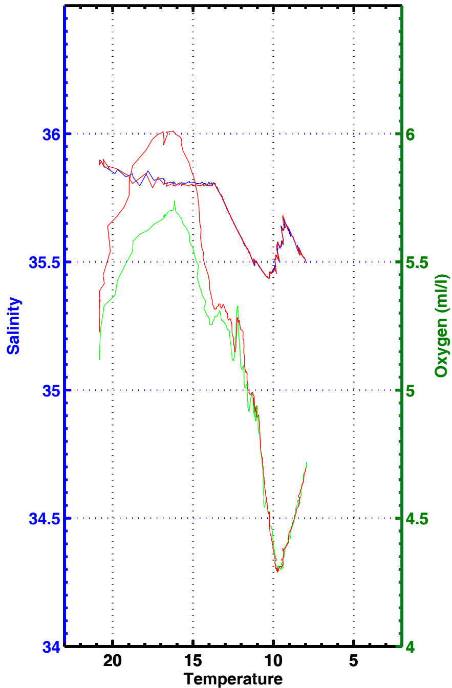
T-S , T-02 , station 3244
