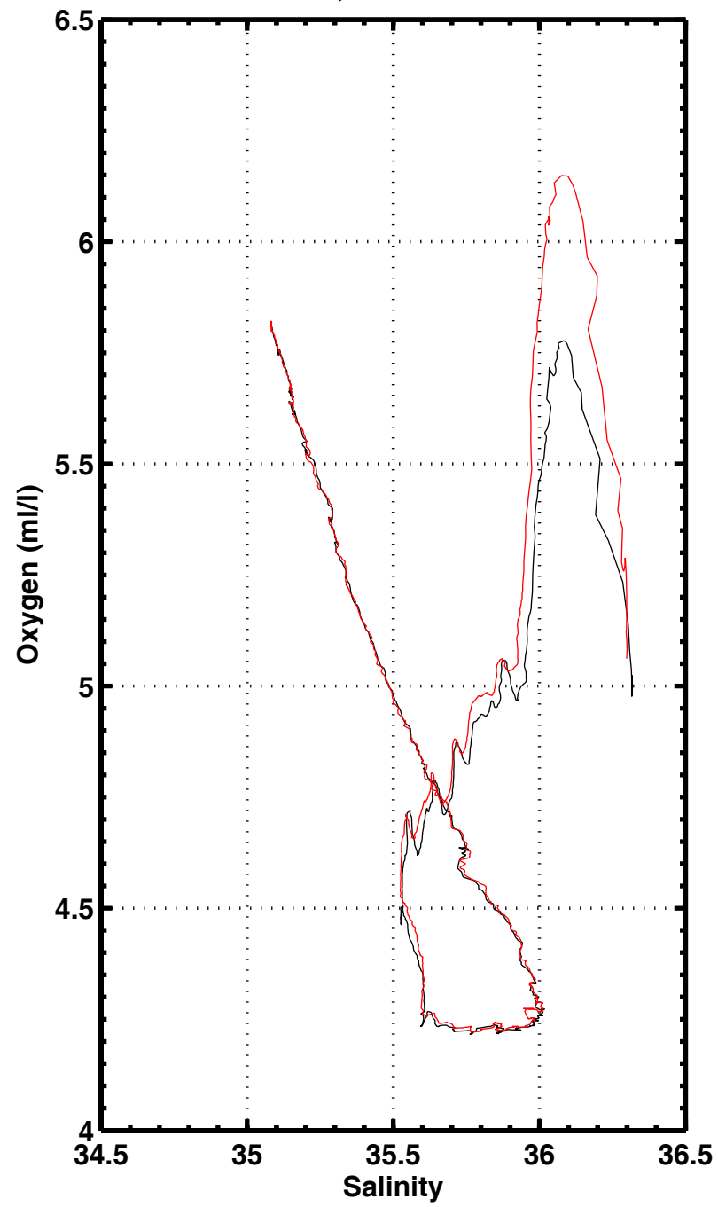
S-O2 , station 3038
