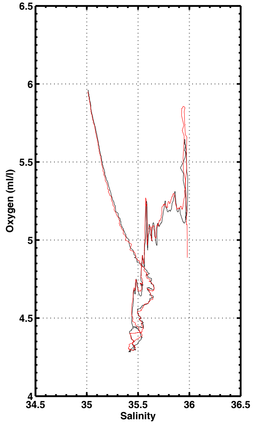
S-O2 , station 3166
