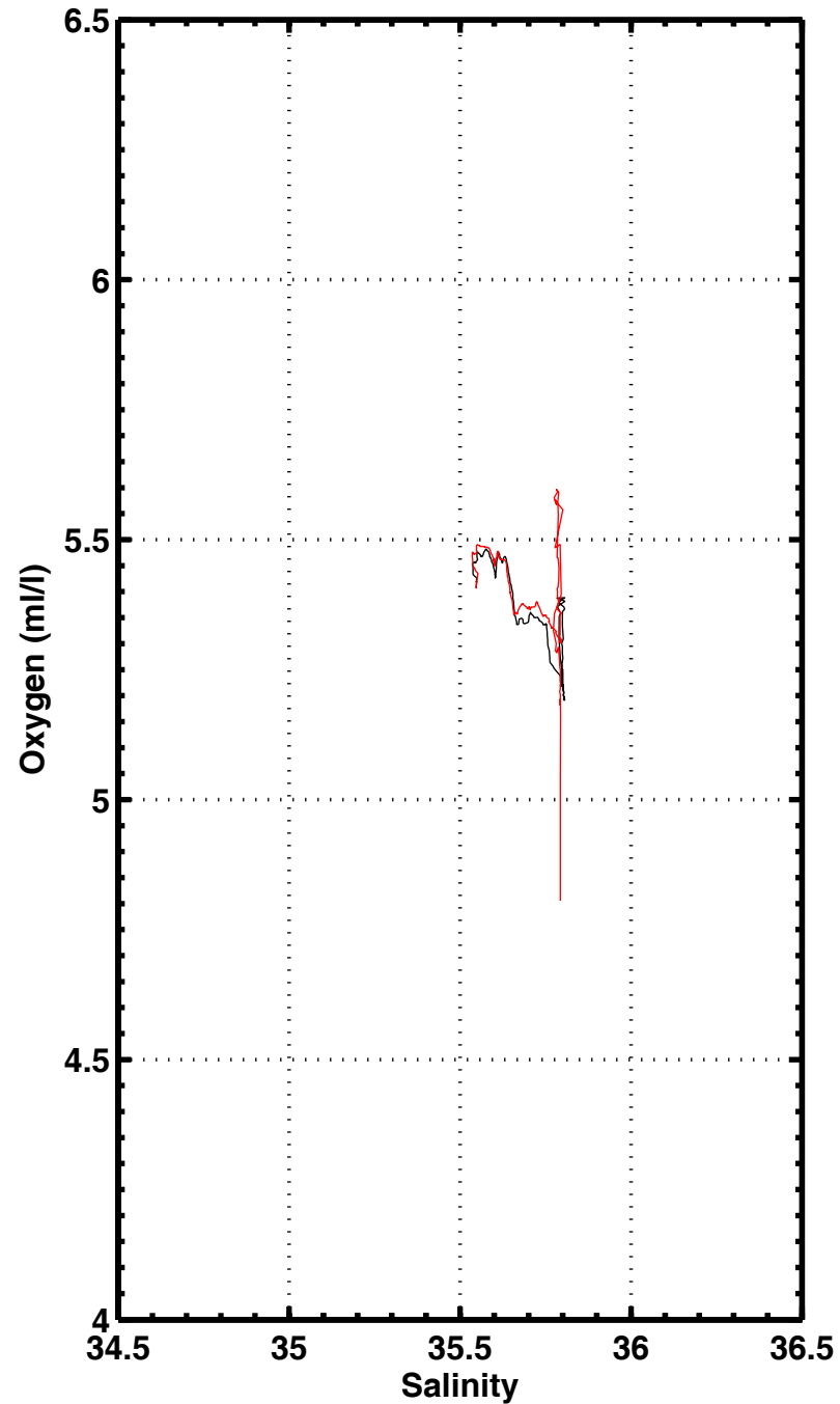
S-02 , station 3329
