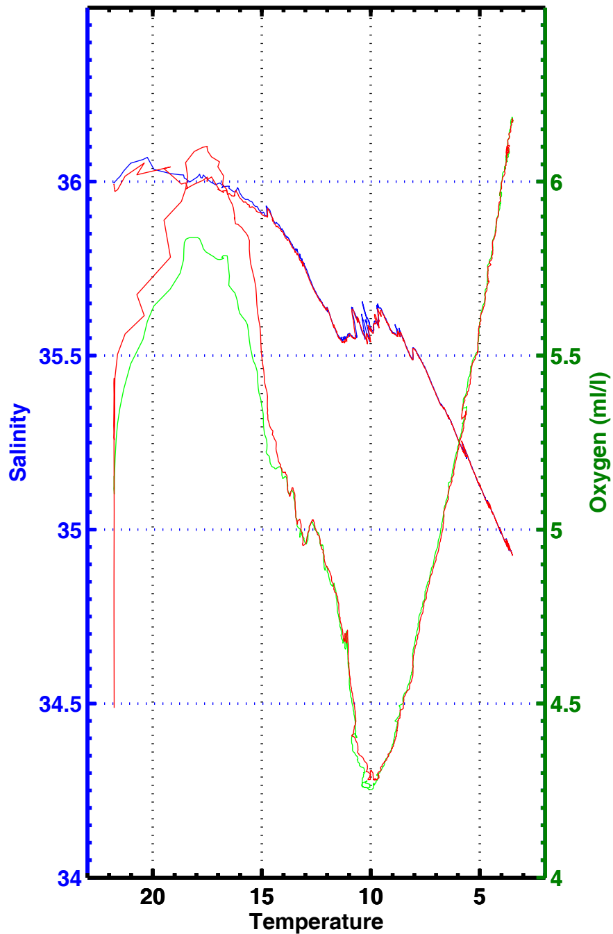
T-S , T-02 , station 3045
