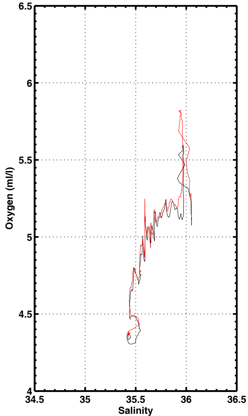
S-02 , station 3164
