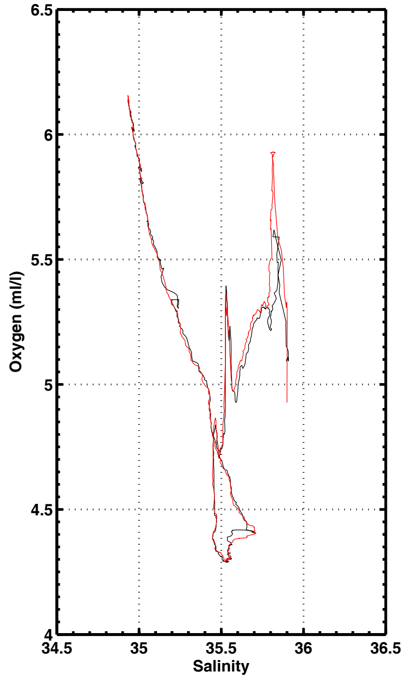
S-02 , station 3252
