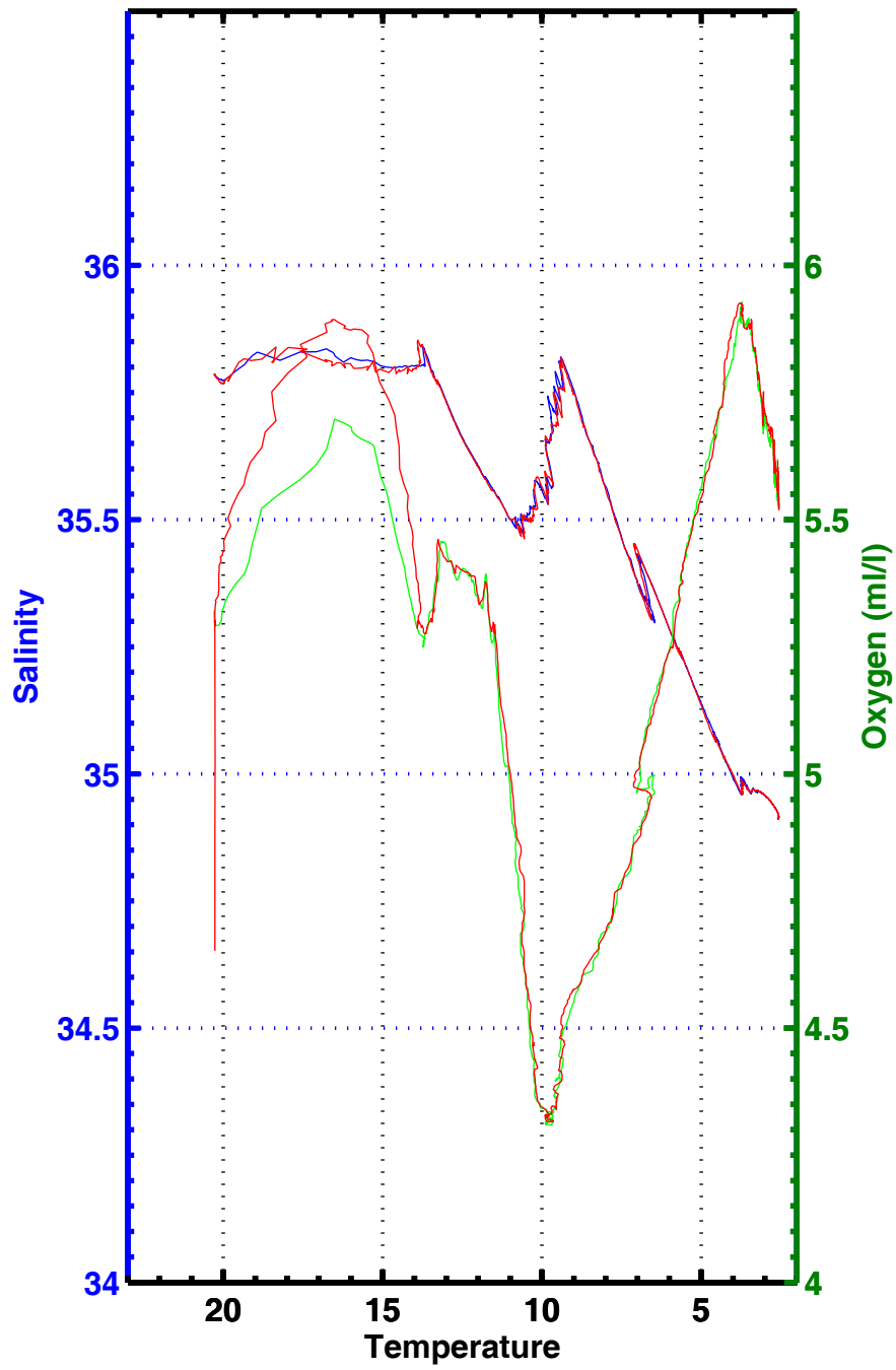
T-S , T-02 , station 3025
