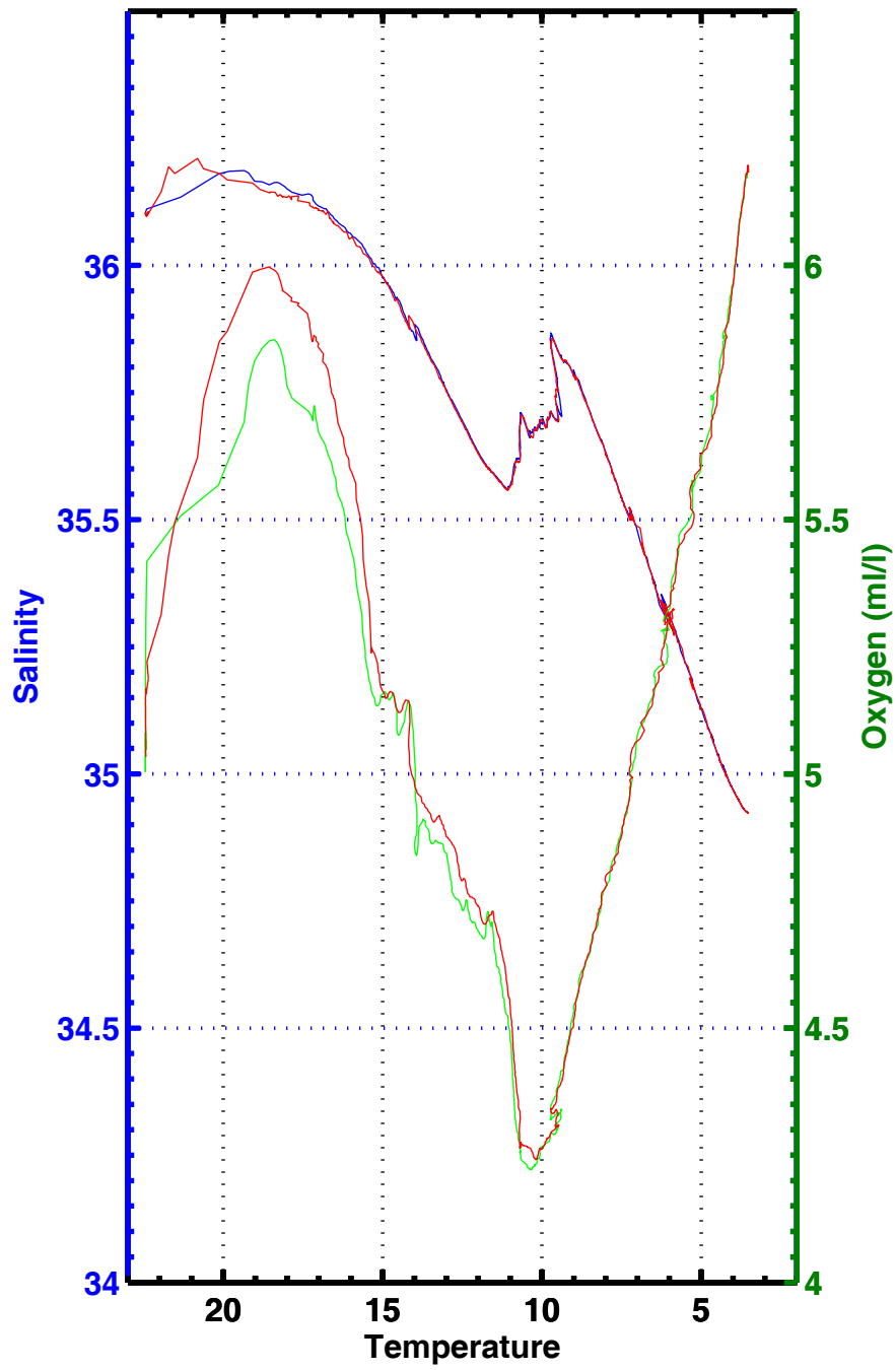
T-S , T-02 , station 3043
