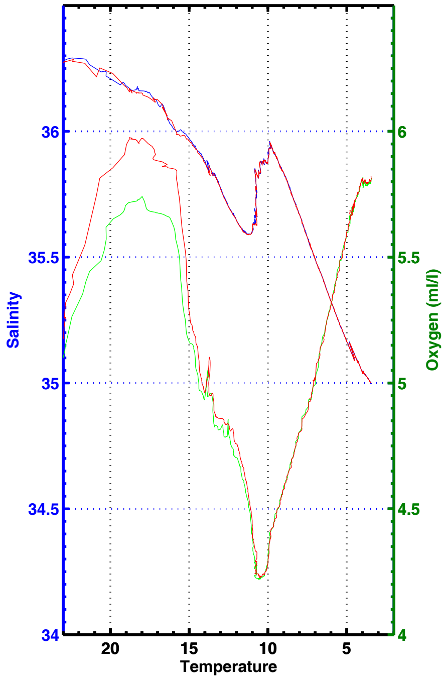
T-S , T-02 , station 3013
