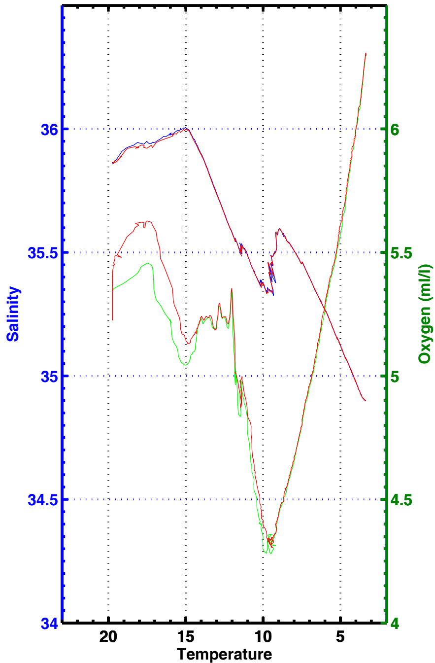
T-S , T-02 , station 3069
