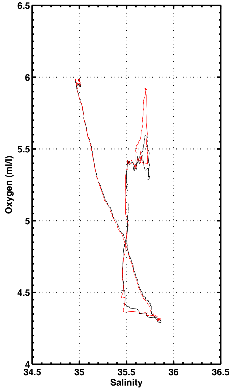
S-O2 , station 3028
