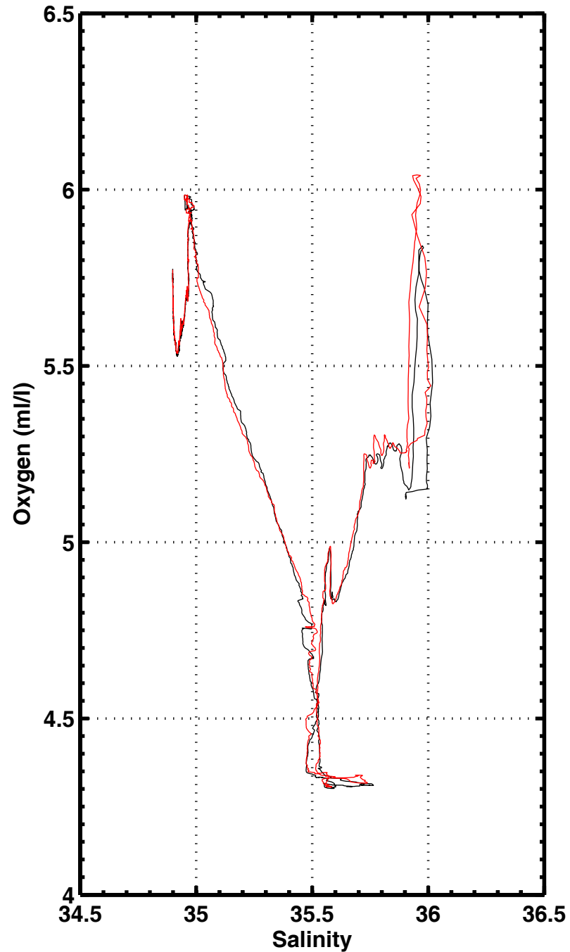
S-02 , station 3031
