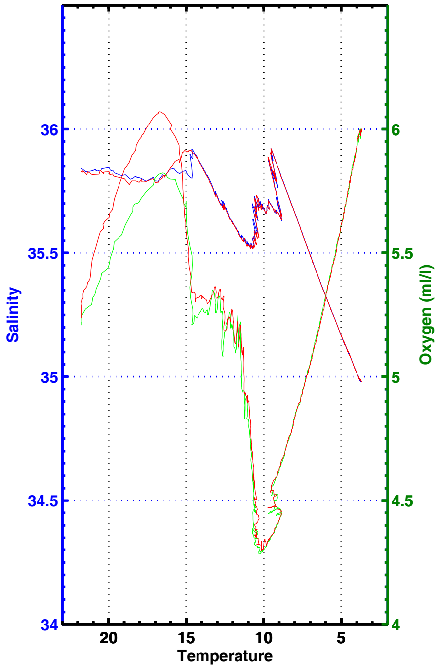
T-S , T-02 , station 3008
