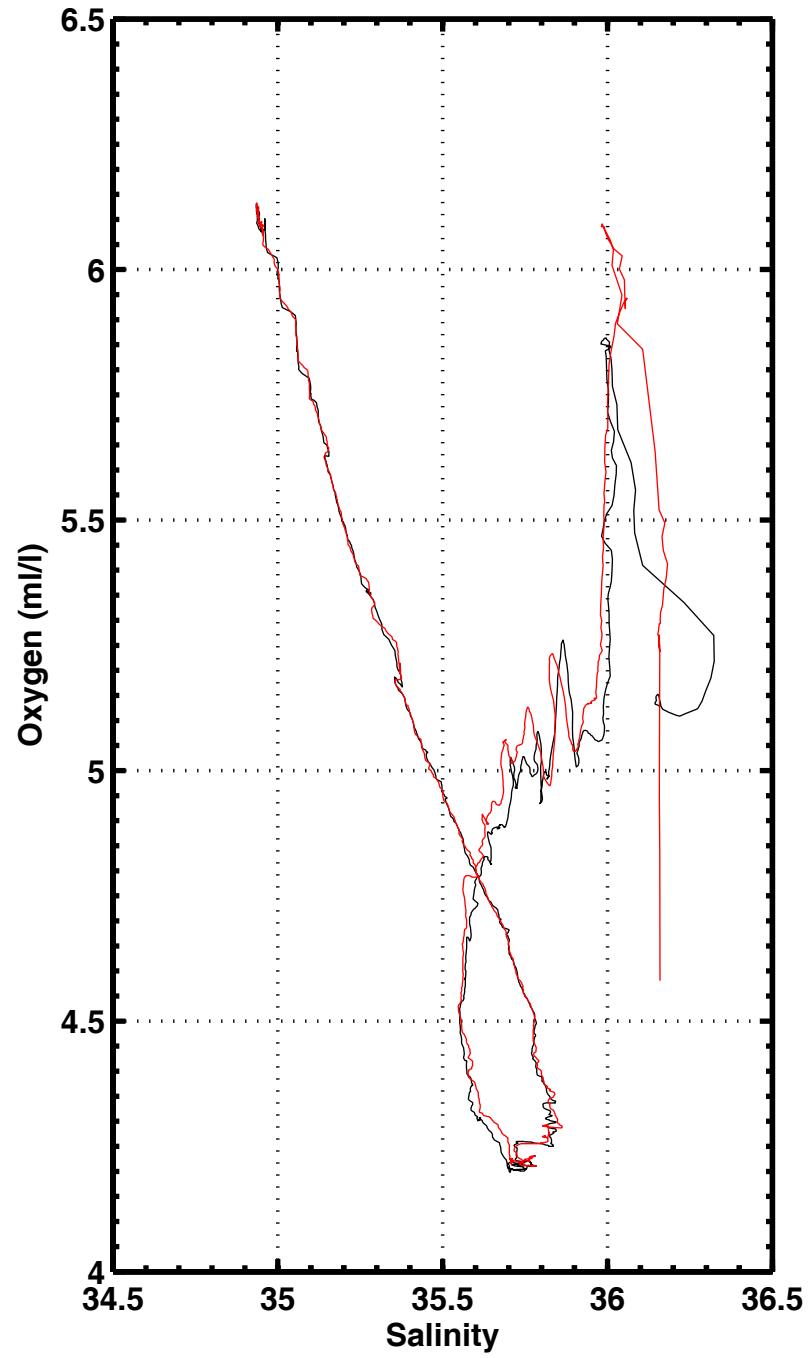
S-02 , station 3079
