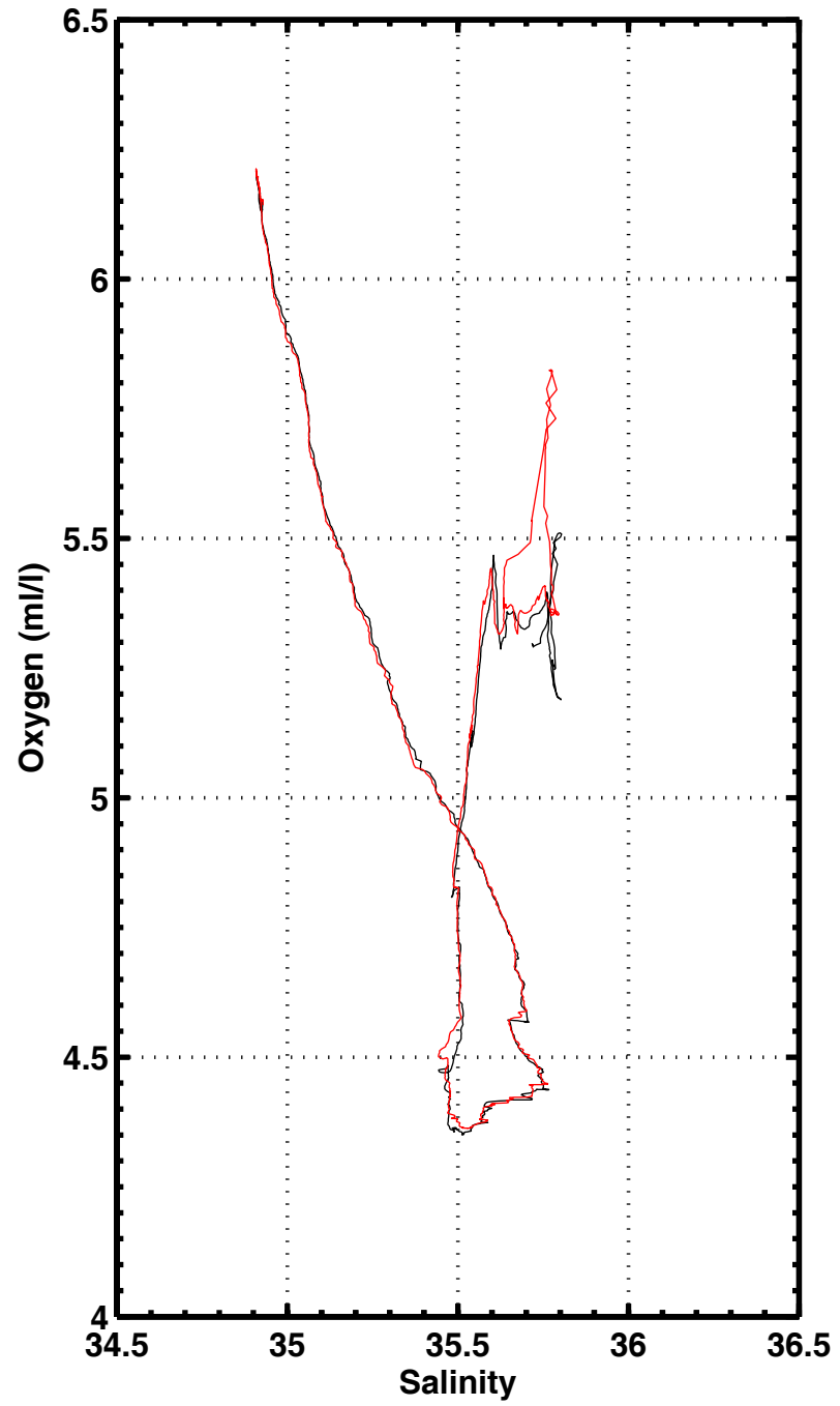
S-O2 , station 3002
