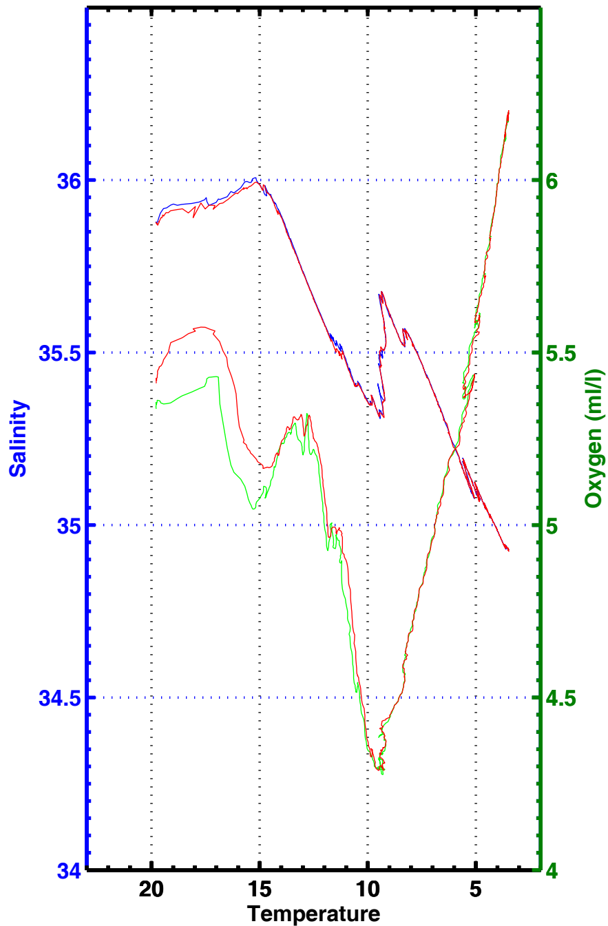
T-S , T-02 , station 3070
