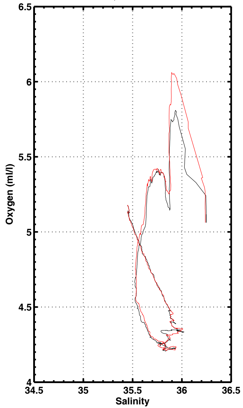
S-O2 , station 3089
