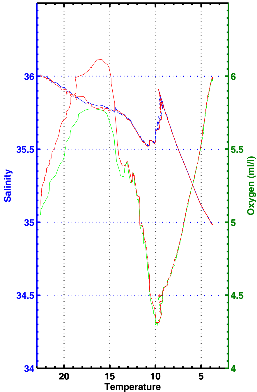
T-S , T-02 , station 3009
