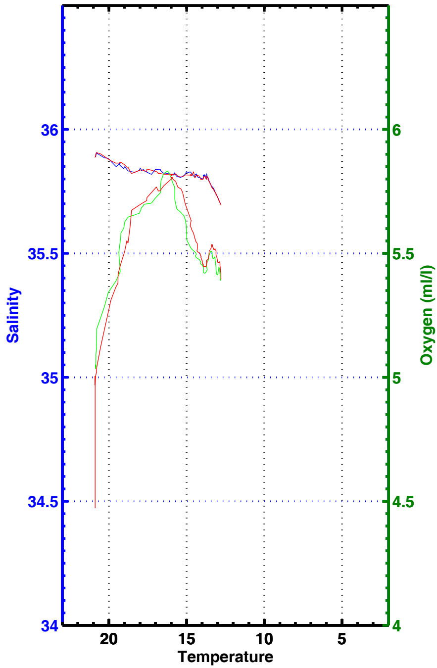
T-S , T-02 , station 3246
