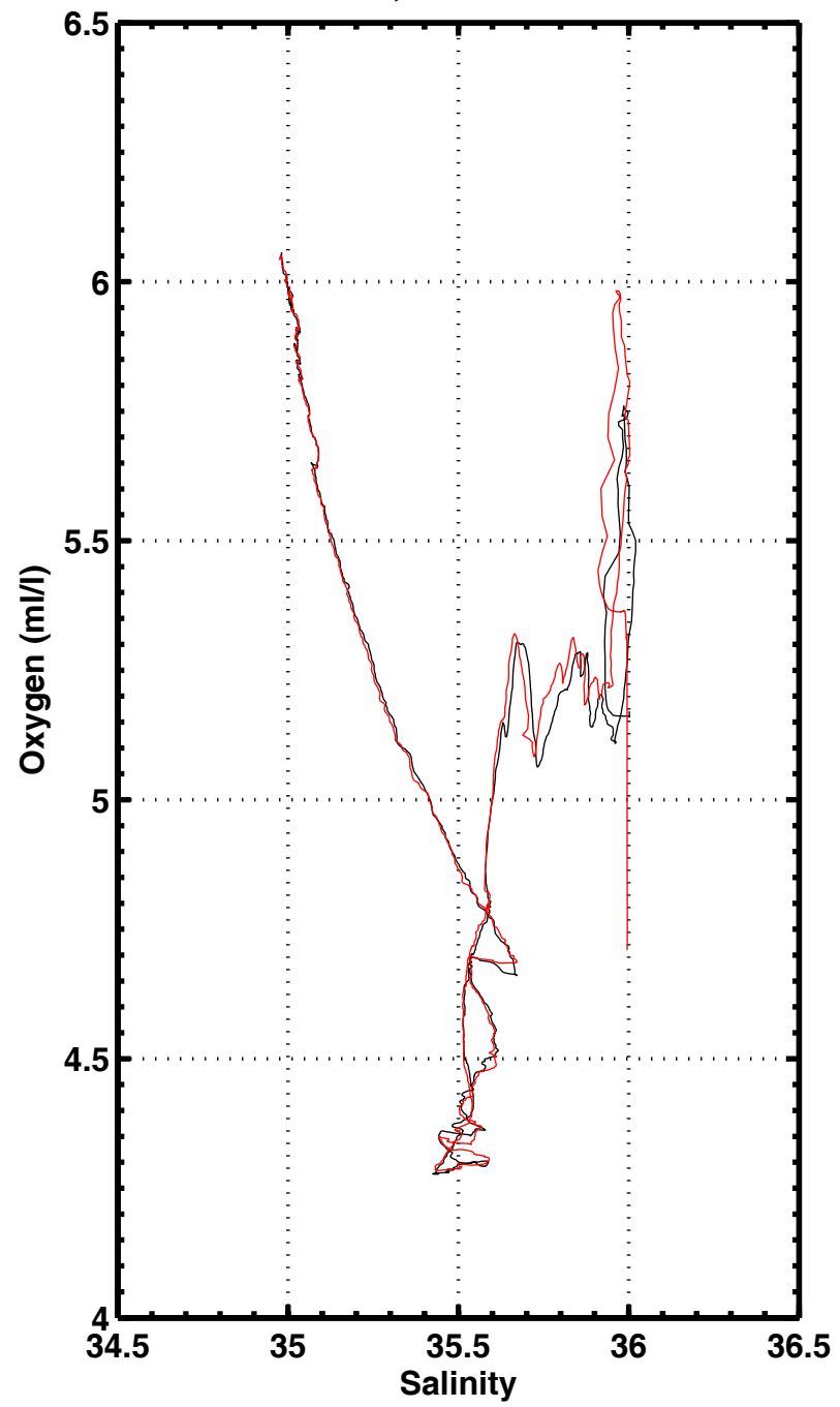
S-O2 , station 3077
