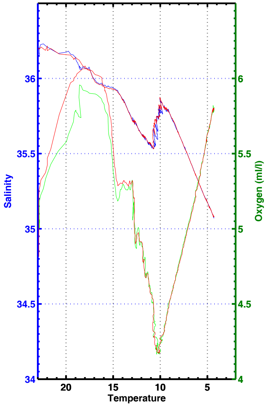
T-S , T-02 , station 3039
