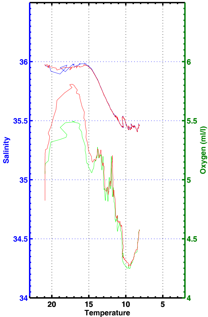
T-S , T-02 , station 3160
