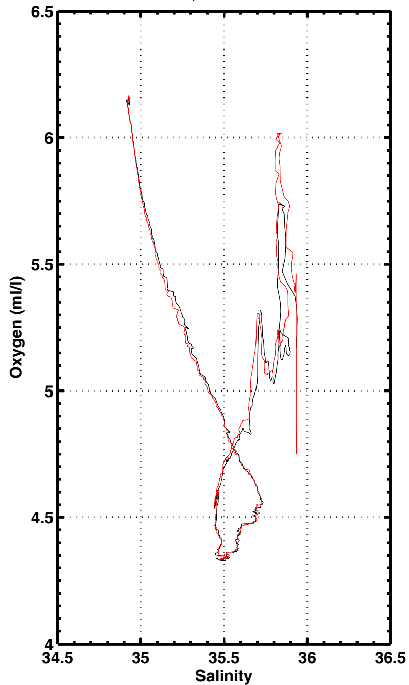
S-O2 , station 3073
