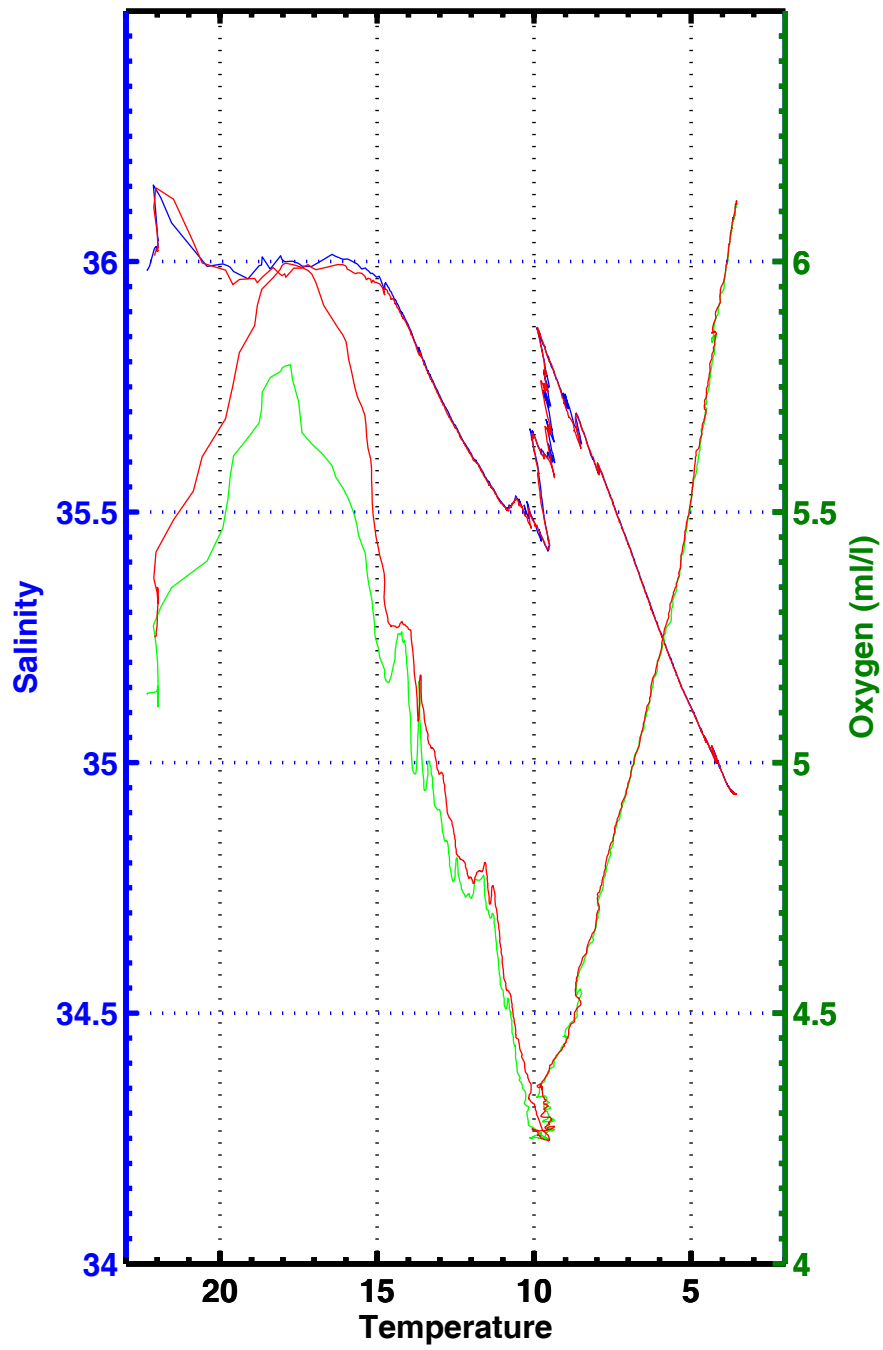
T-S , T-02 , station 3080
