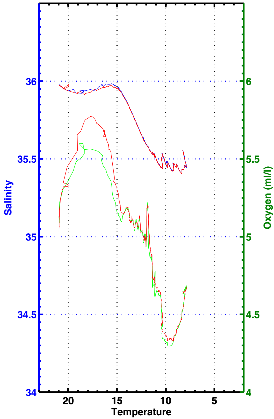
T-S , T-02 , station 3158
