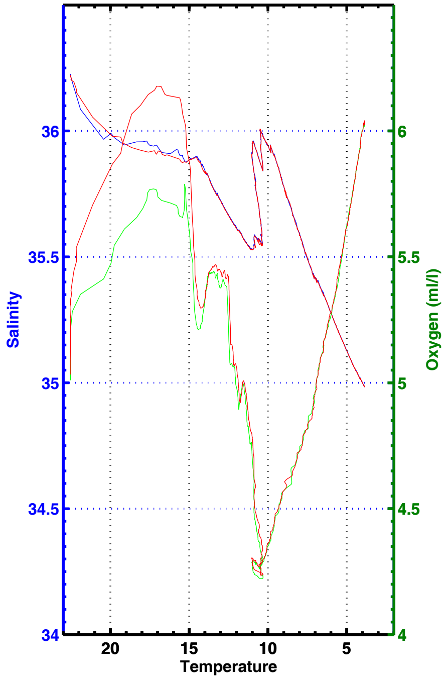
T-S , T-02 , station 3041
