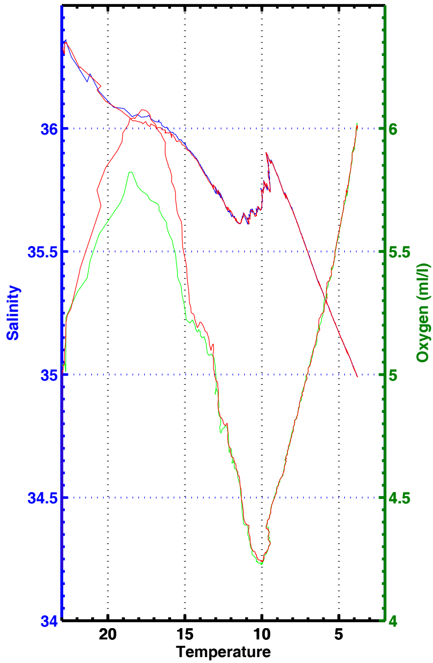
T-S , T-02 , station 3081
