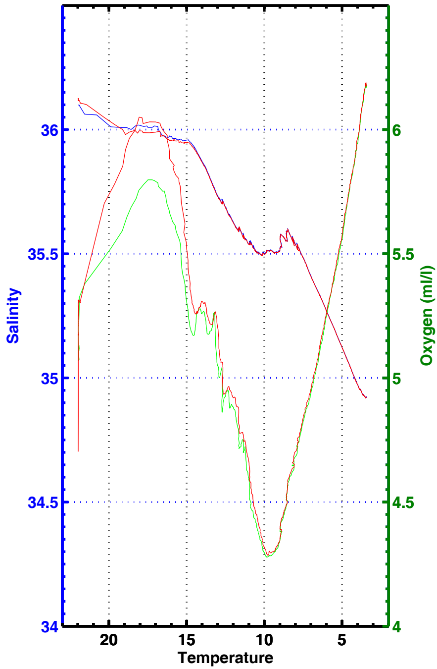
T-S , T-02 , station 3056
