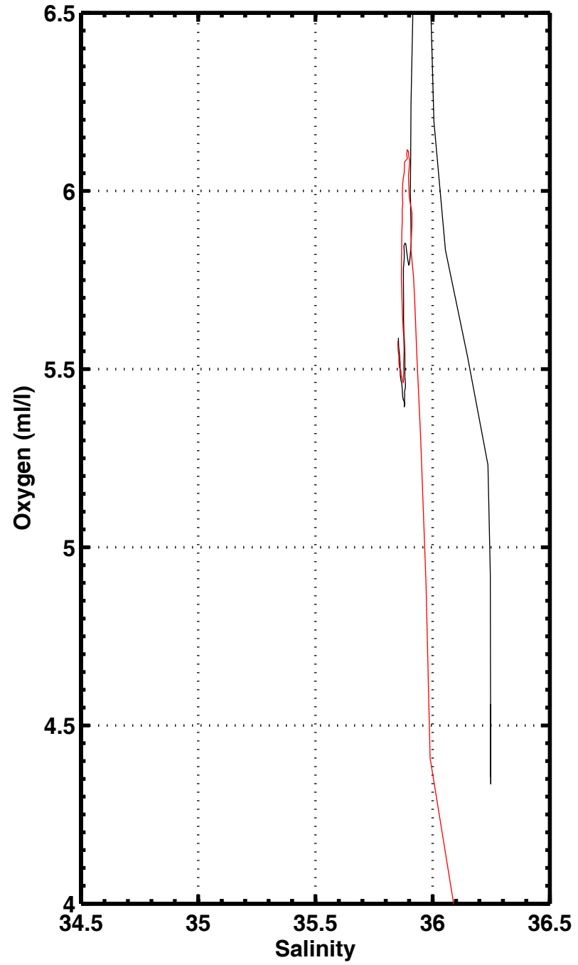
S-02 , station 3090
