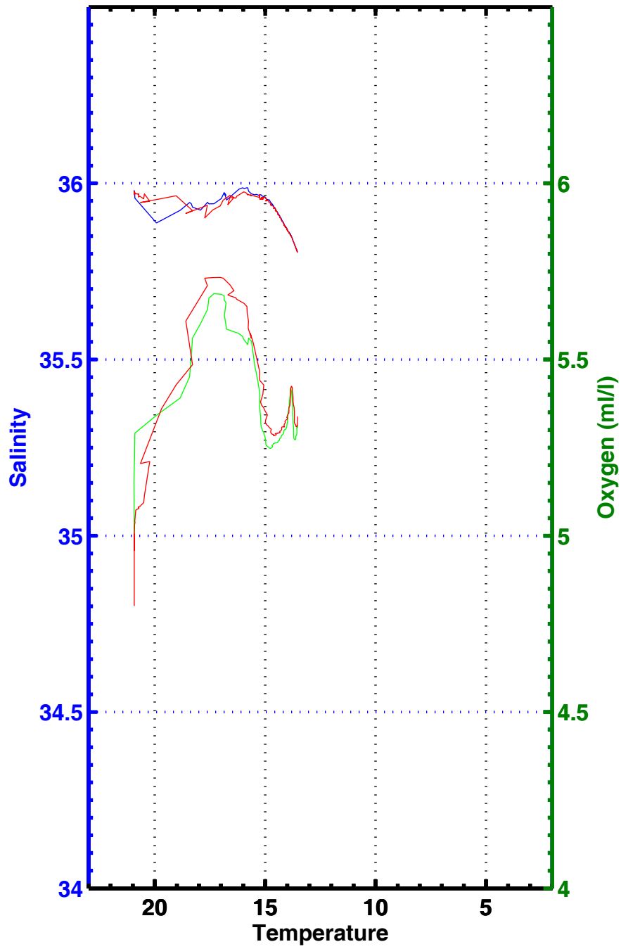
T-S , T-02 , station 3156
