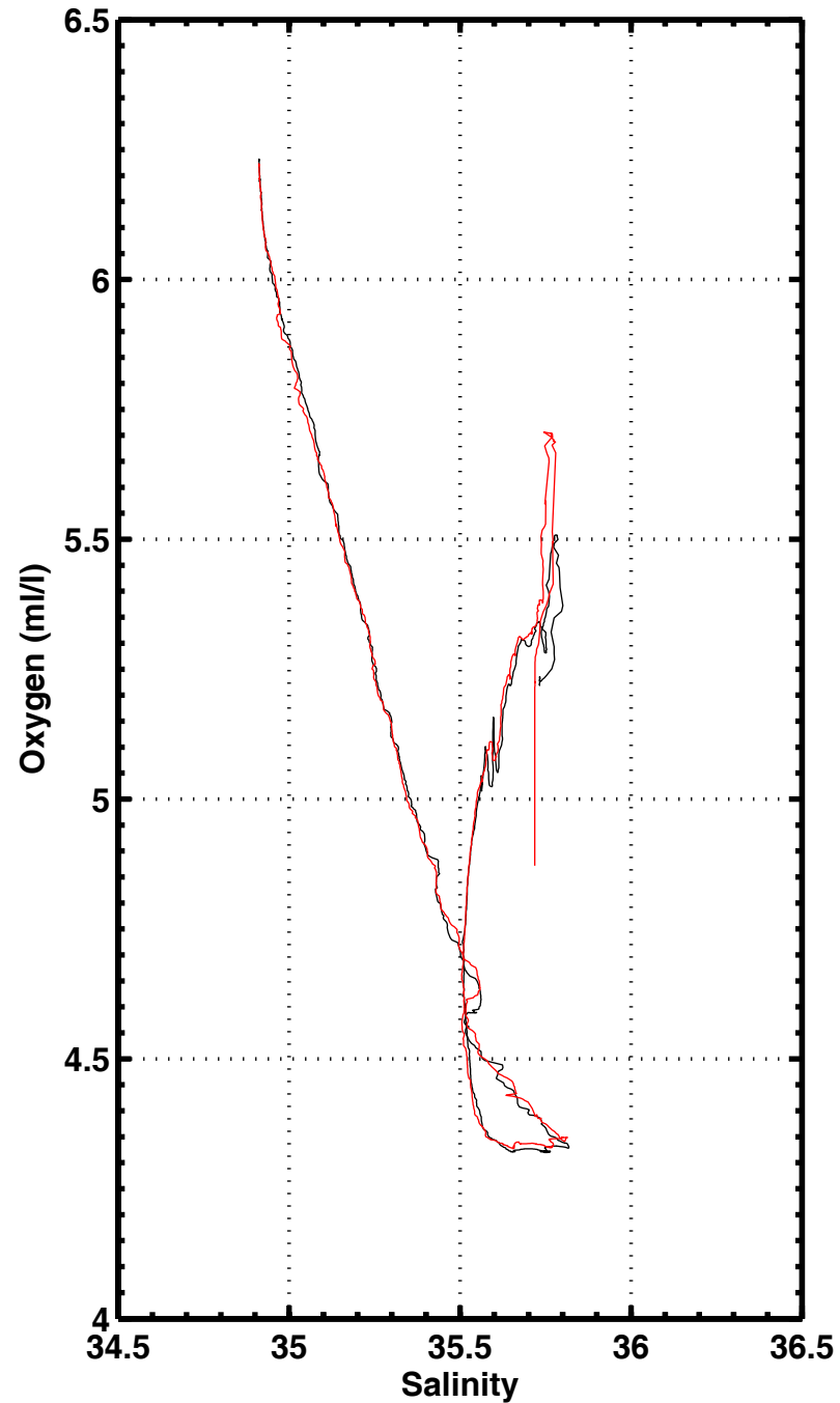
S-02 , station 3001
