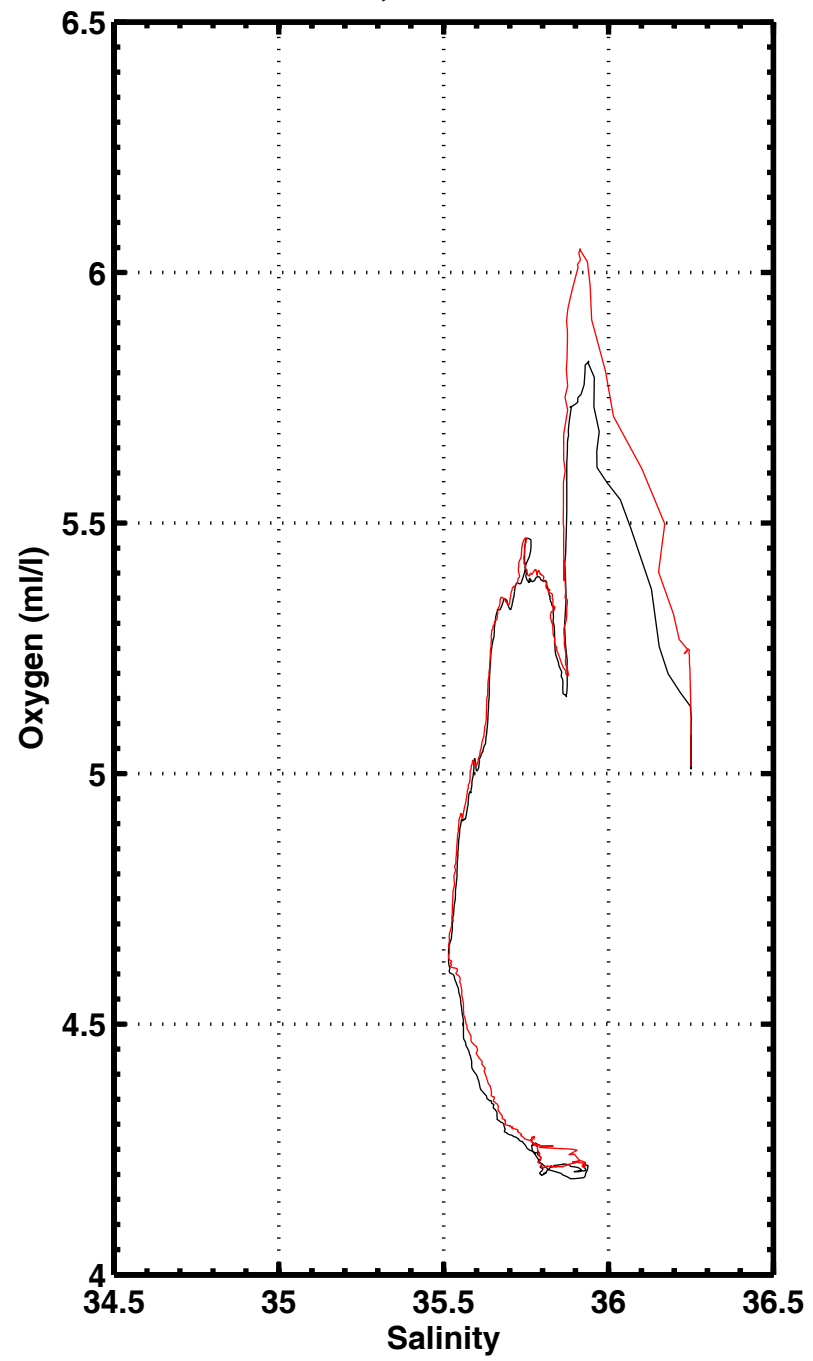
S-O2 , station 3088
