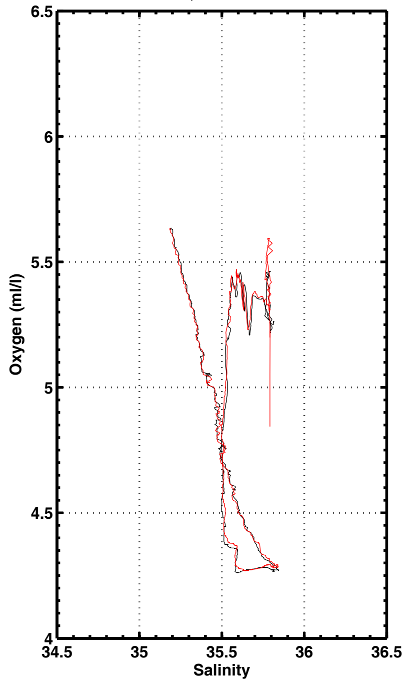
S-O2 , station 3335
