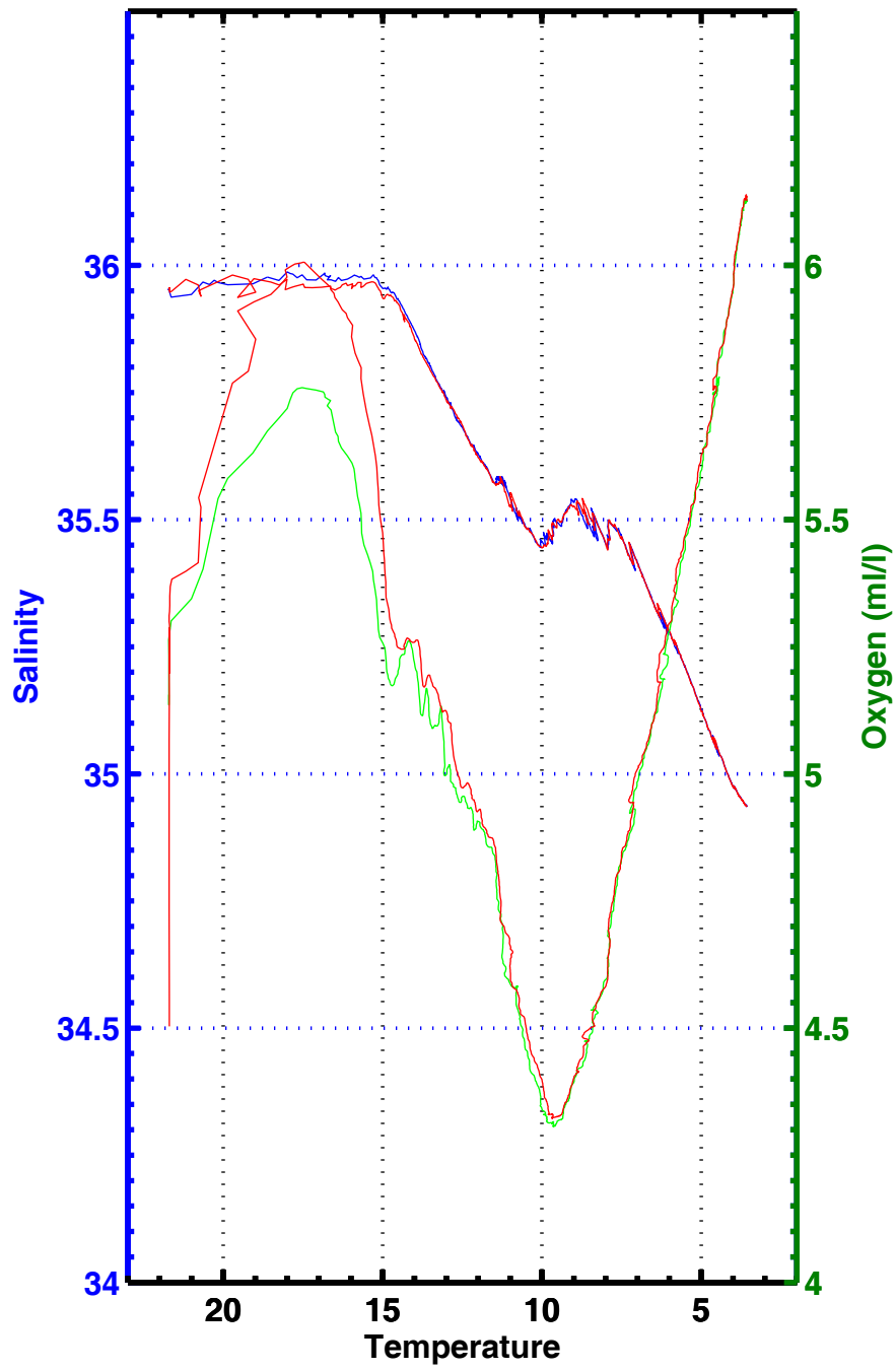
T-S , T-02 , station 3055
