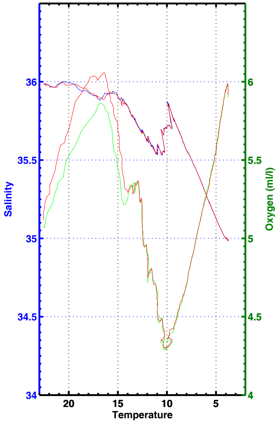
T-S , T-02 , station 3010
