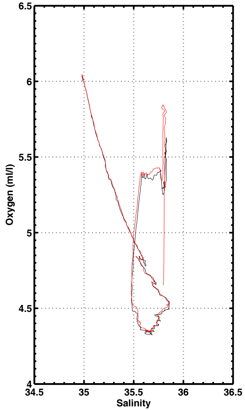
S-O2 , station 3023
