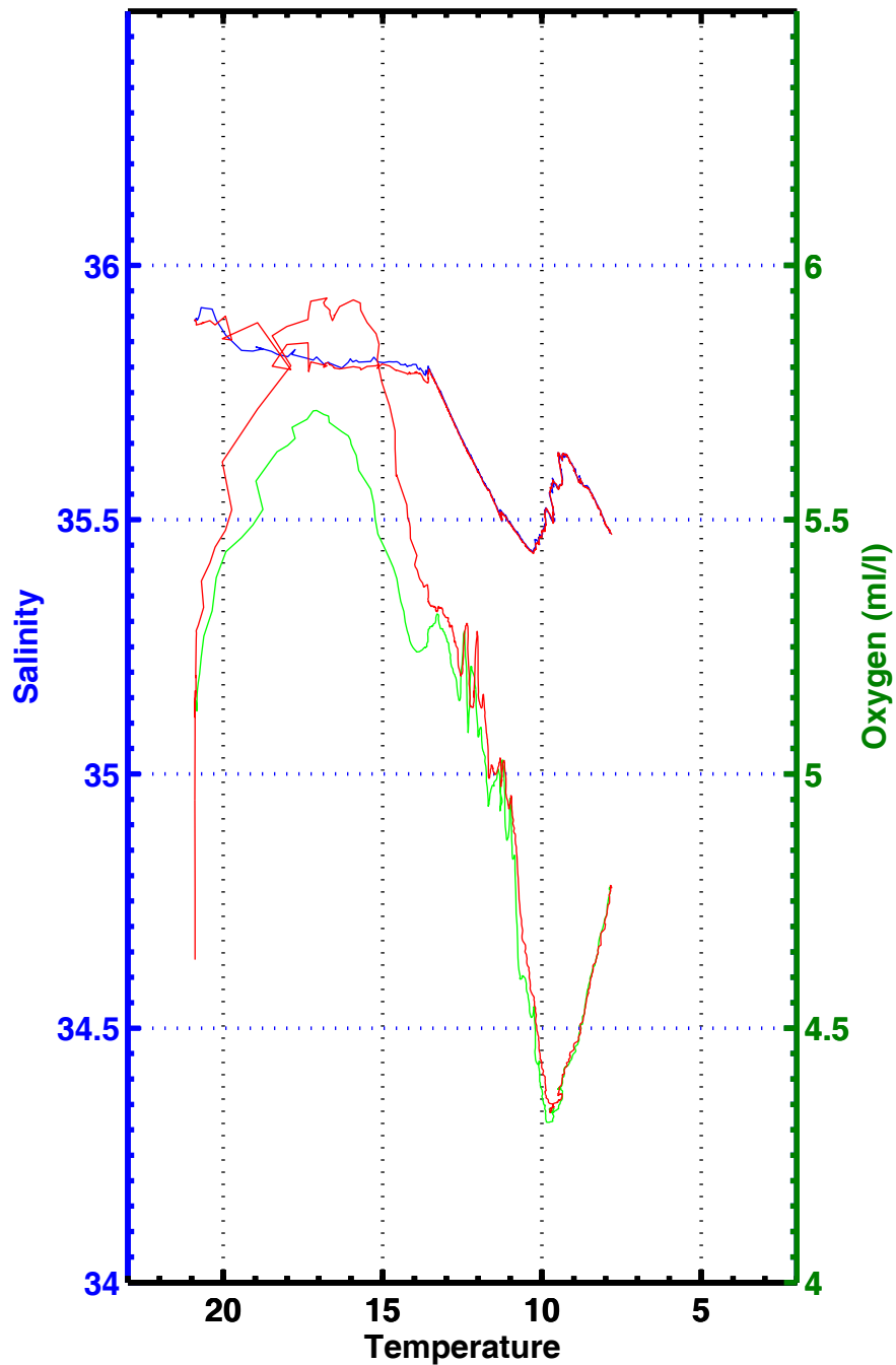
T-S , T-02 , station 3242
