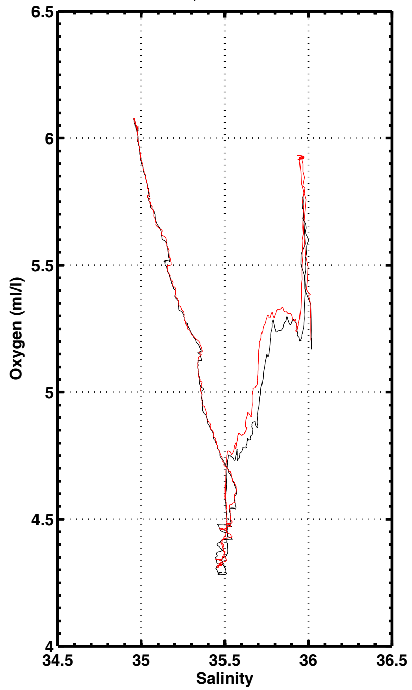
S-O2 , station 3054
