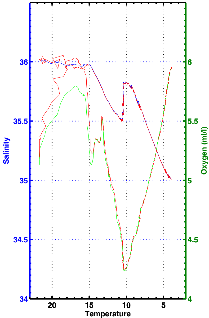
T-S , T-02 , station 3046
