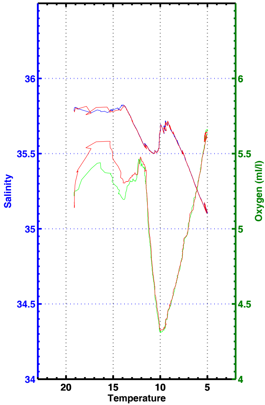
T-S , T-02 , station 3325
