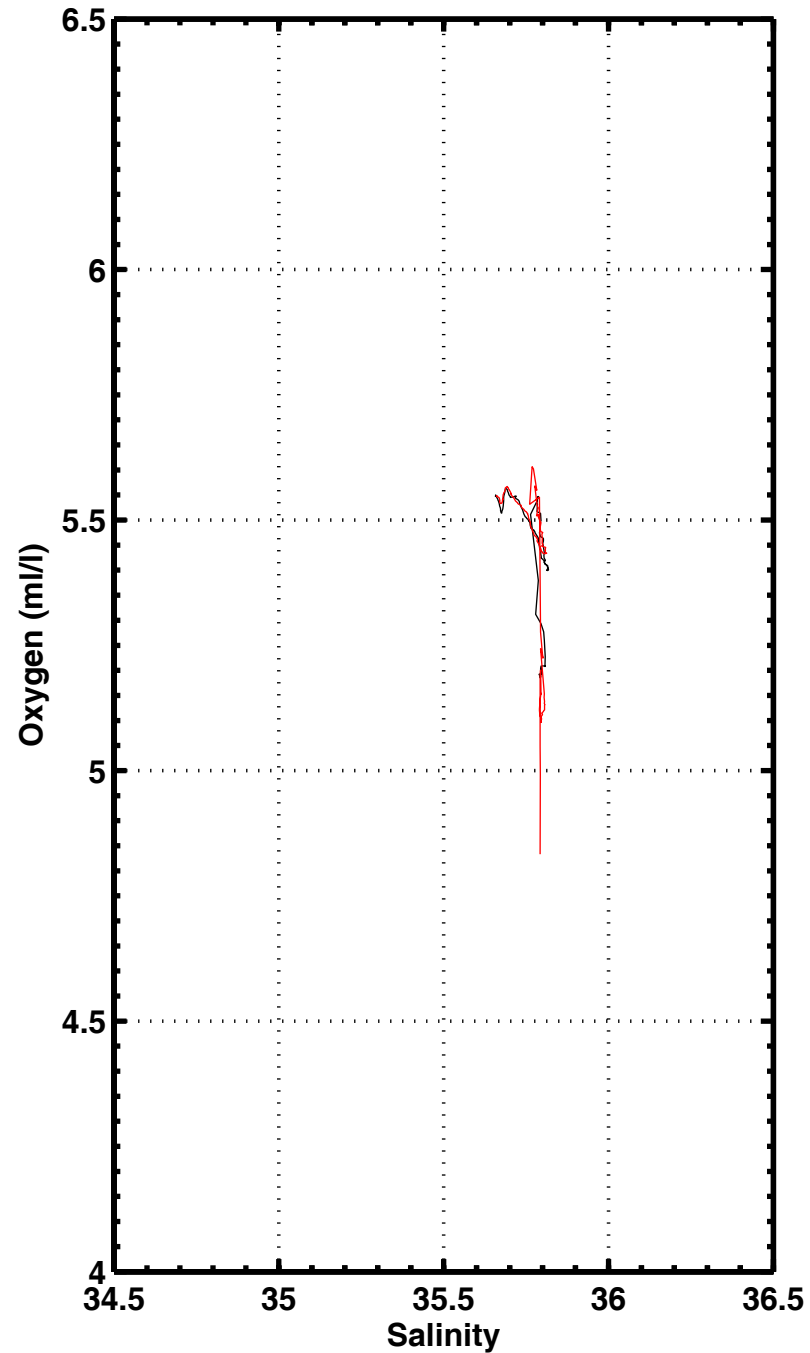
S-02 , station 3324
