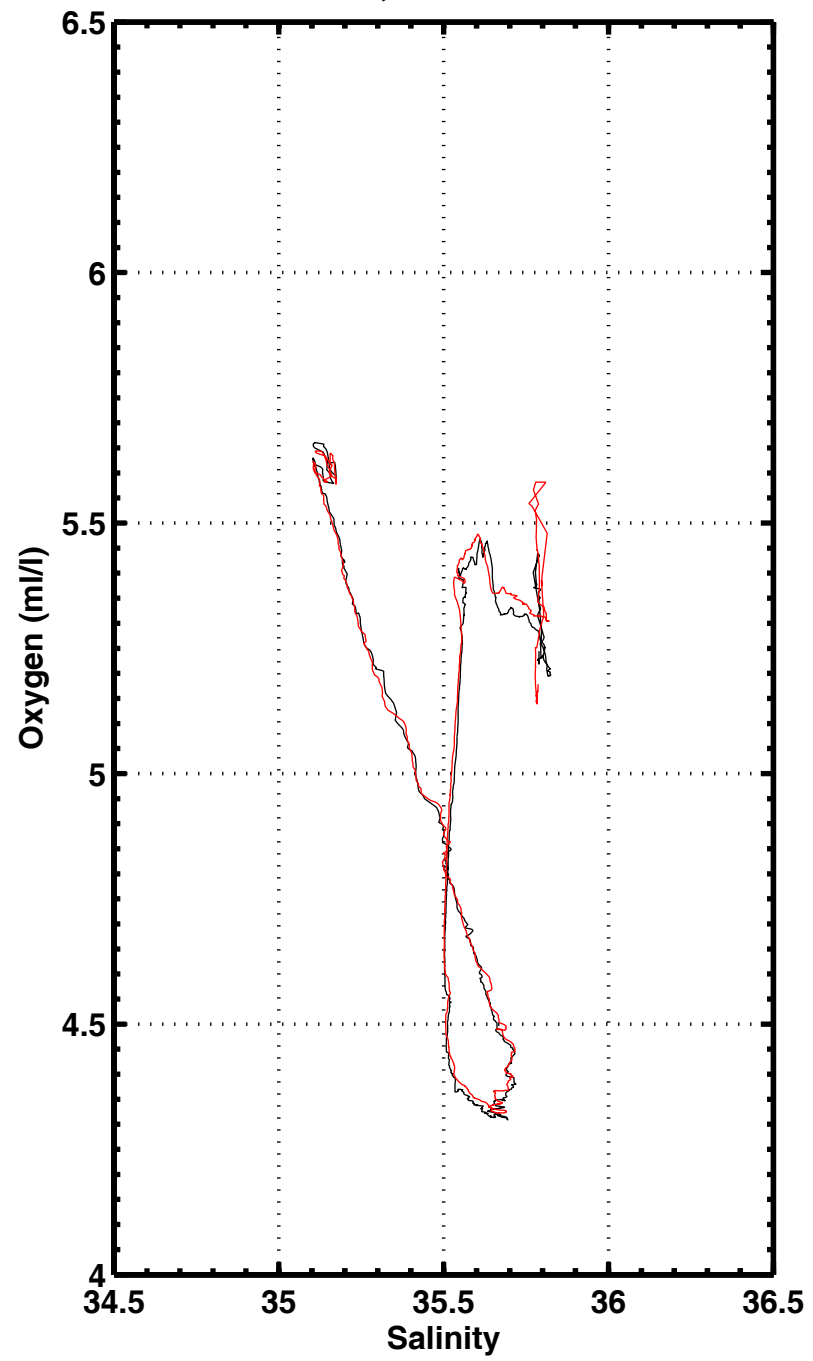
S-O2 , station 3325
