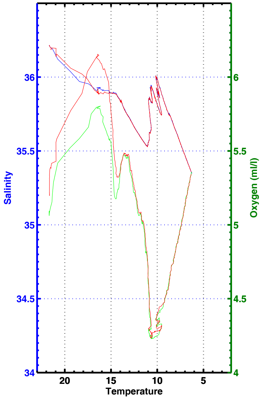
T-S , T-02 , station 3098
