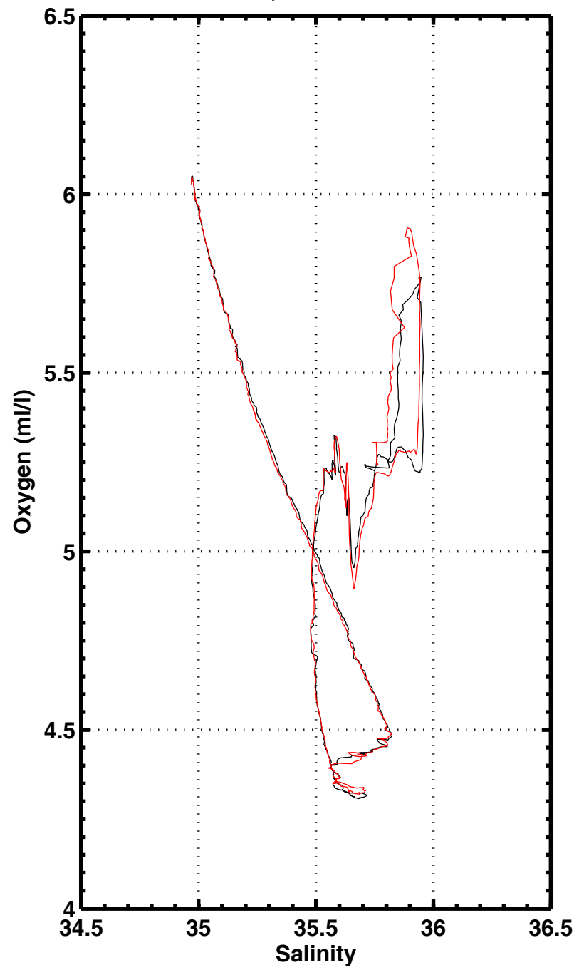
S-O2 , station 3020
