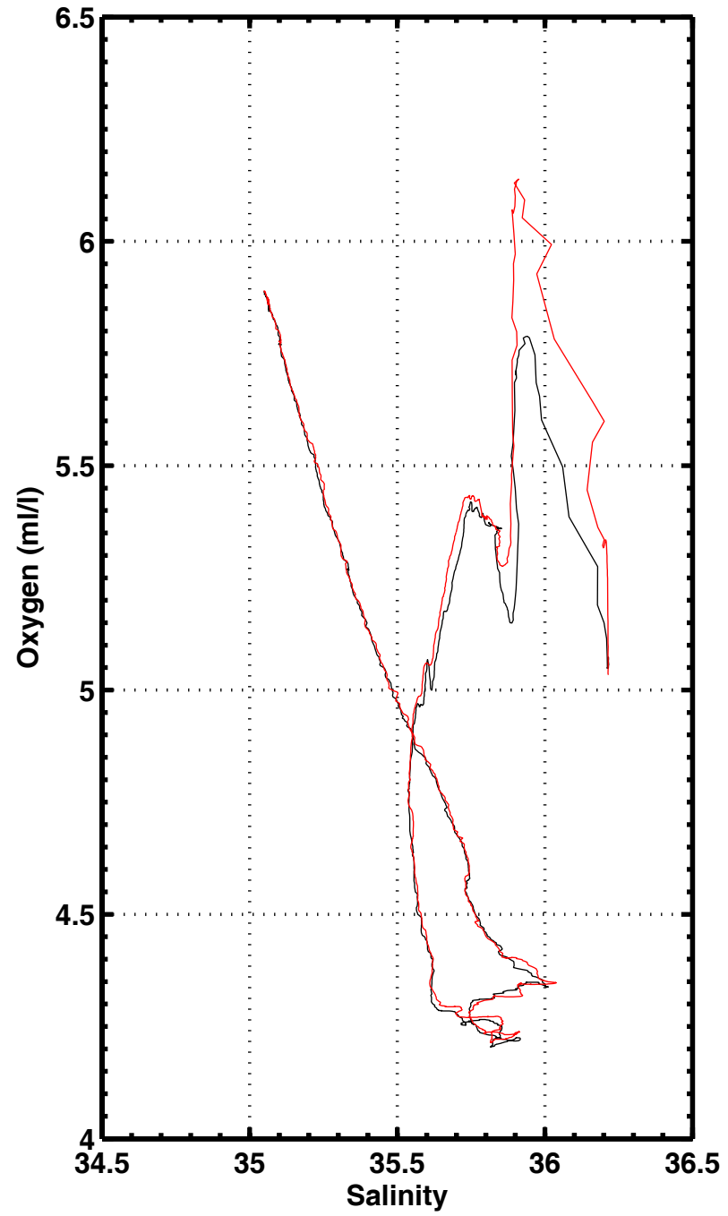
S-O2 , station 3099
