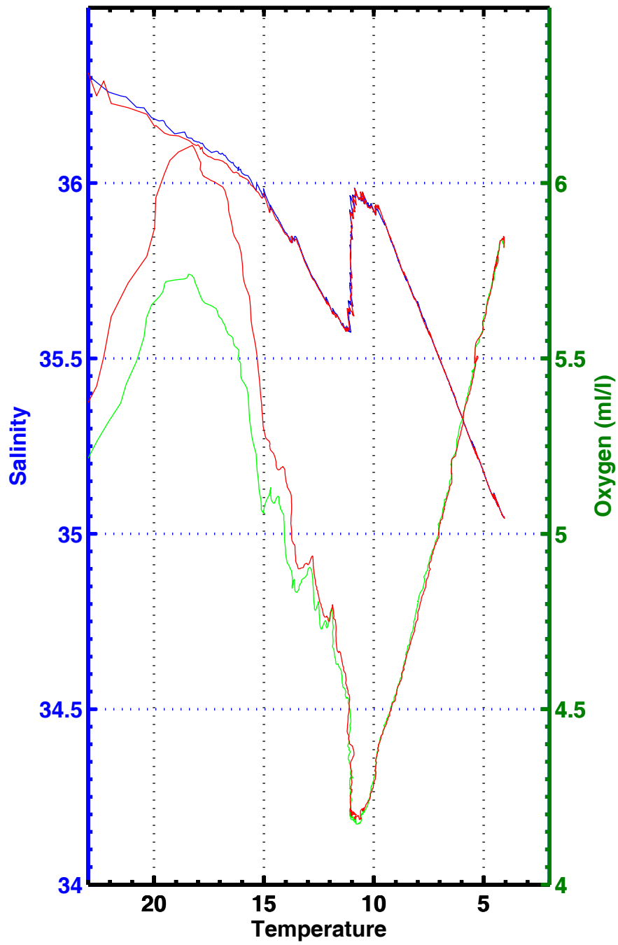
T-S , T-02 , station 3014
