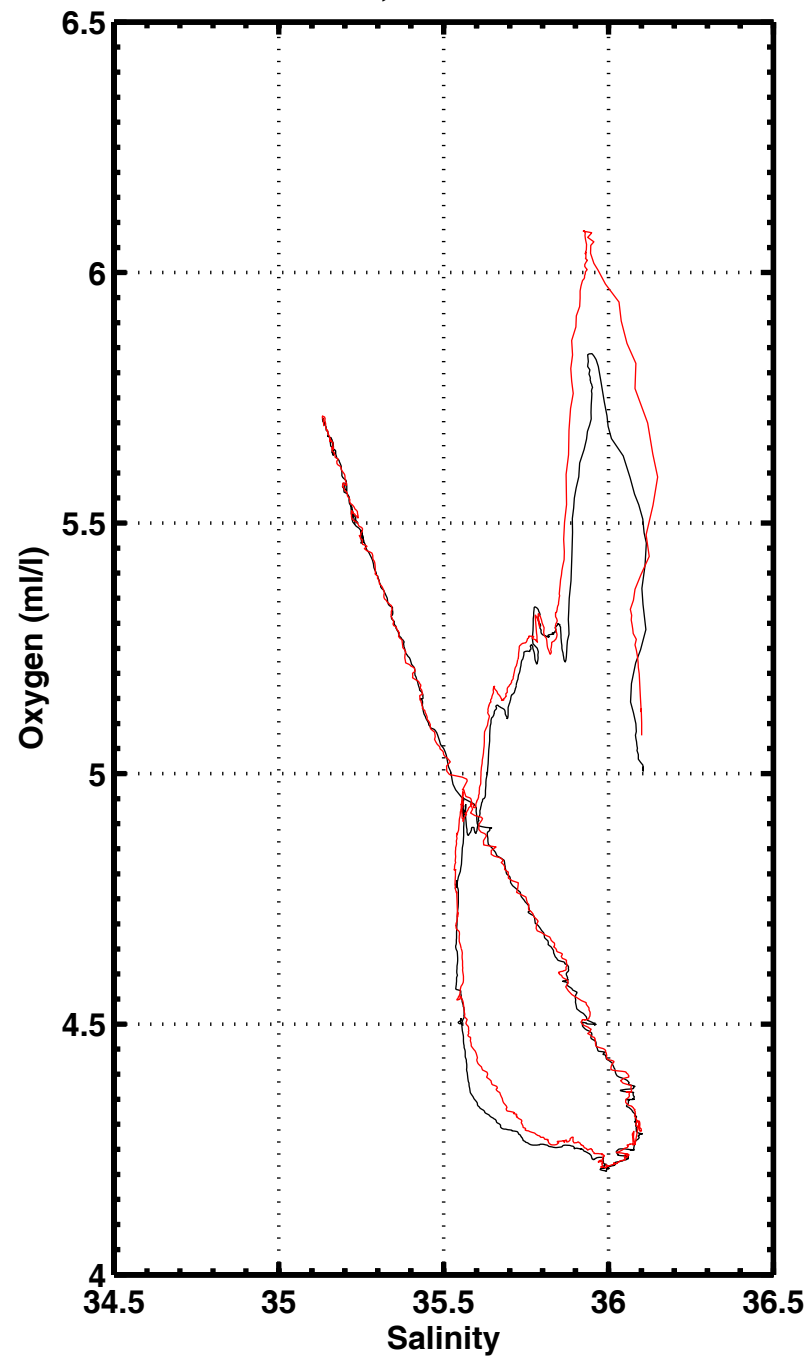
S-O2 , station 3012
