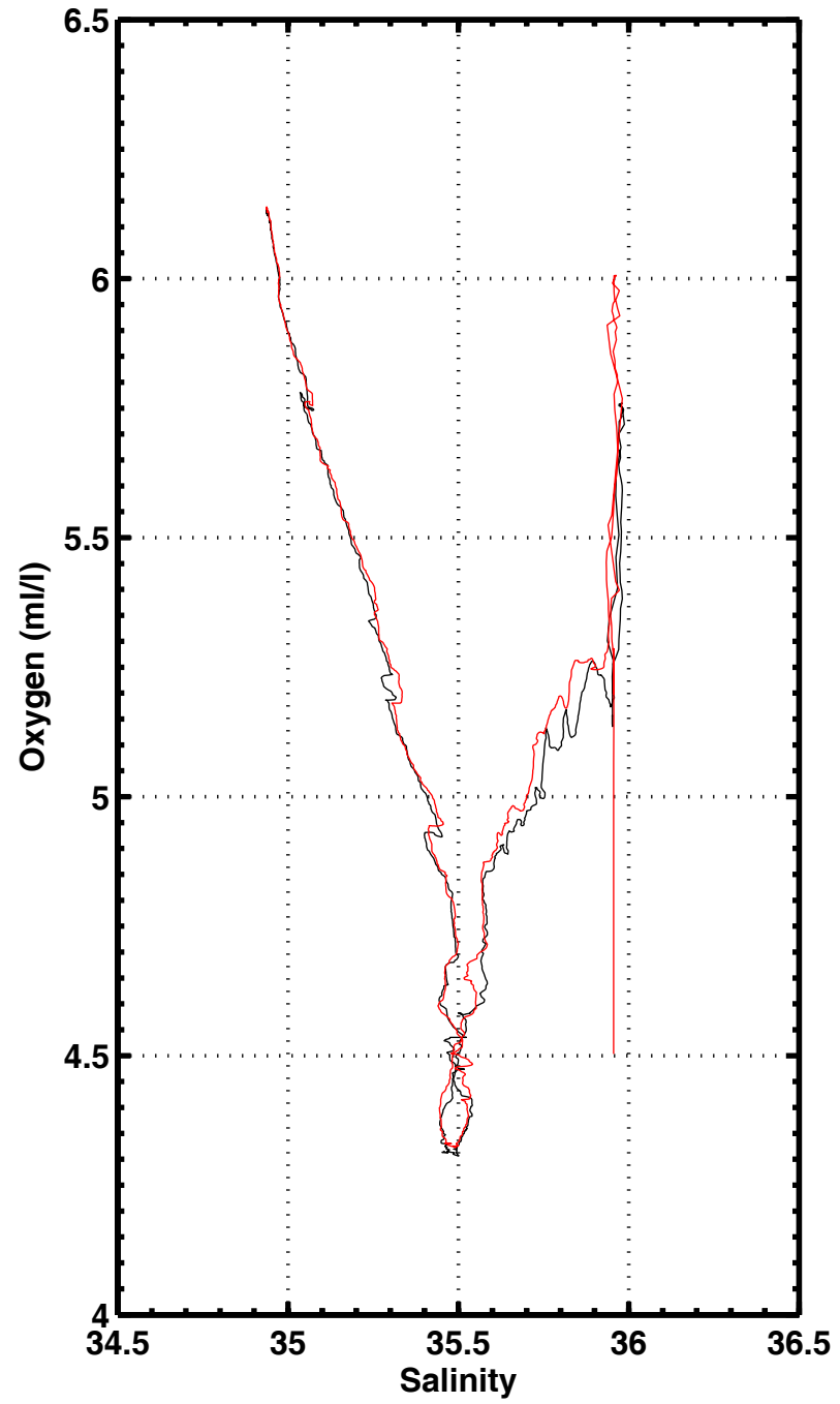
S-O2 , station 3055
