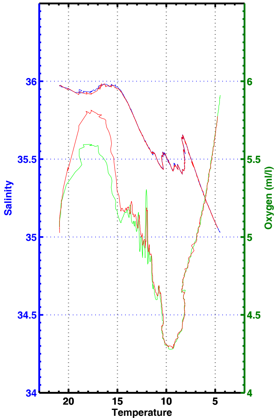
T-S , T-02 , station 3157
