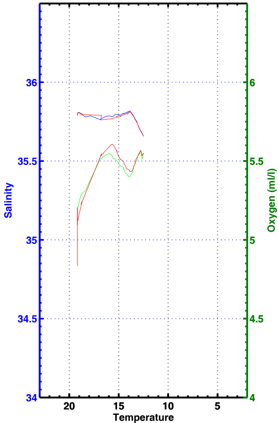
T-S , T-02 , station 3324
