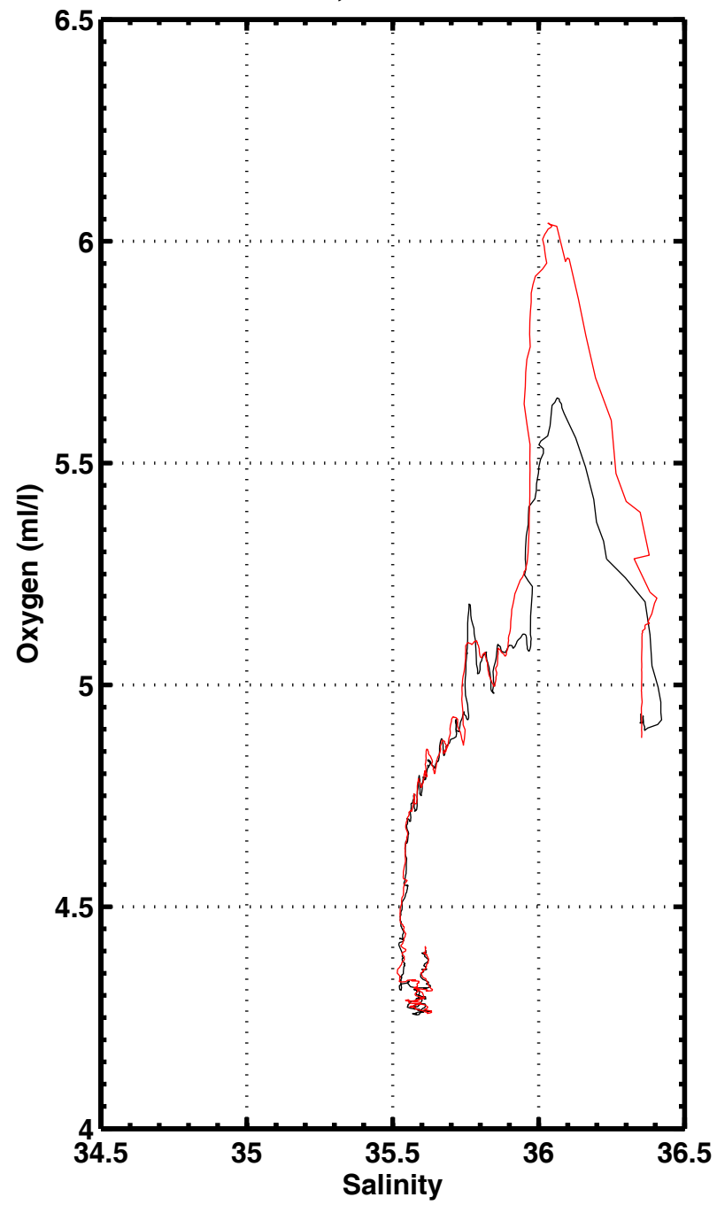
S-O2 , station 3084
