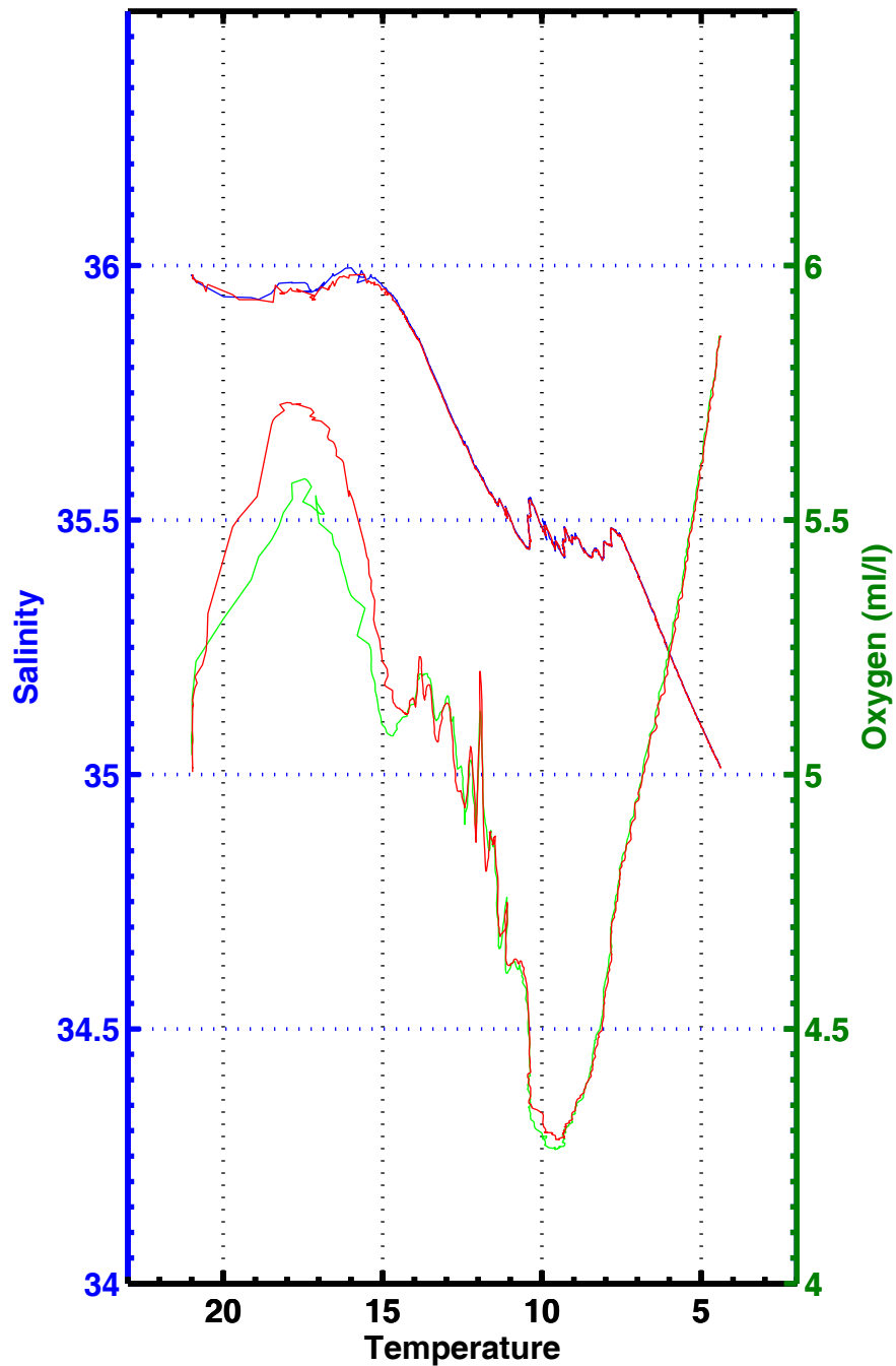
T-S , T-02 , station 3155
