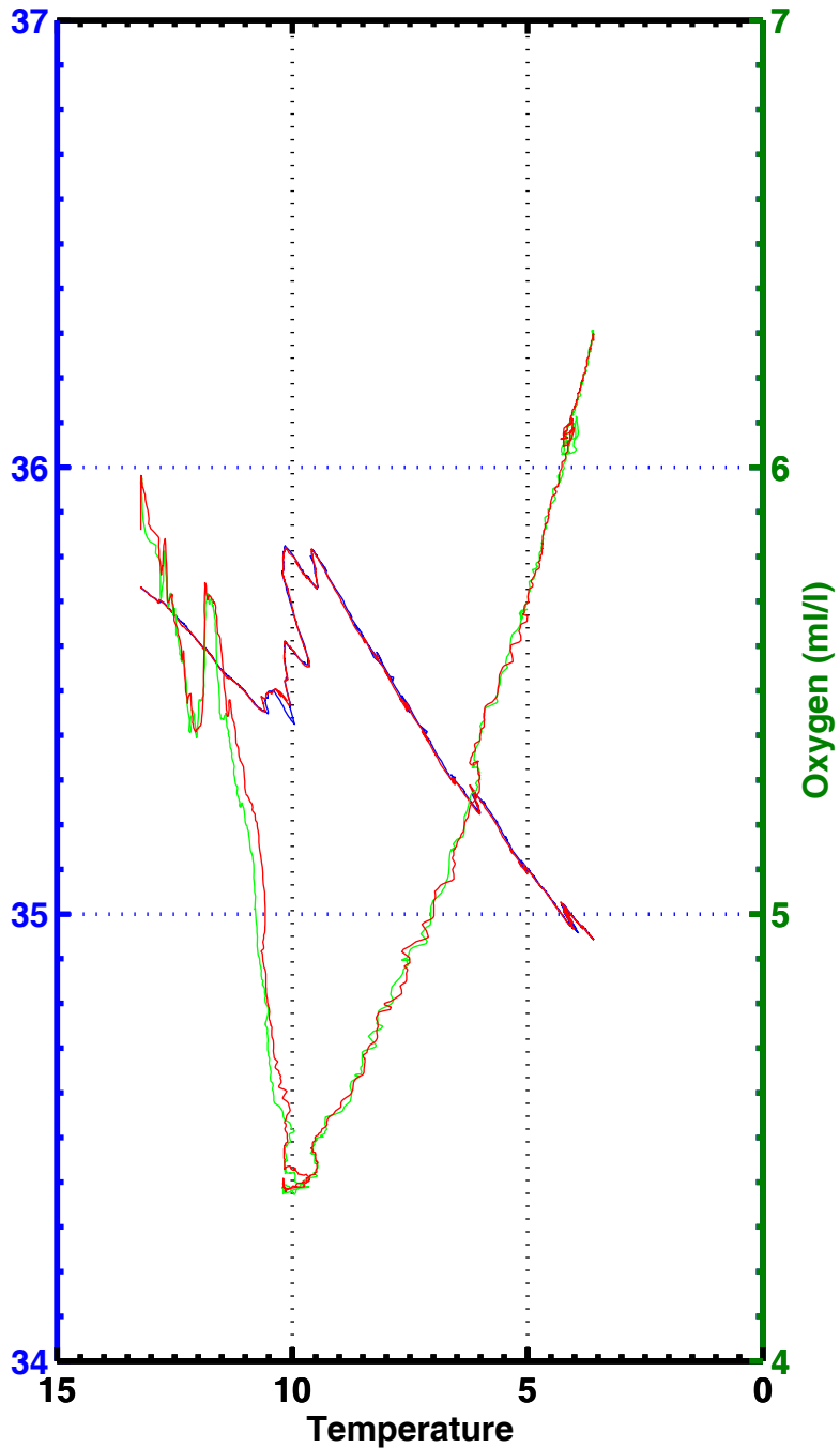
T-S , T-02 , station 2024
