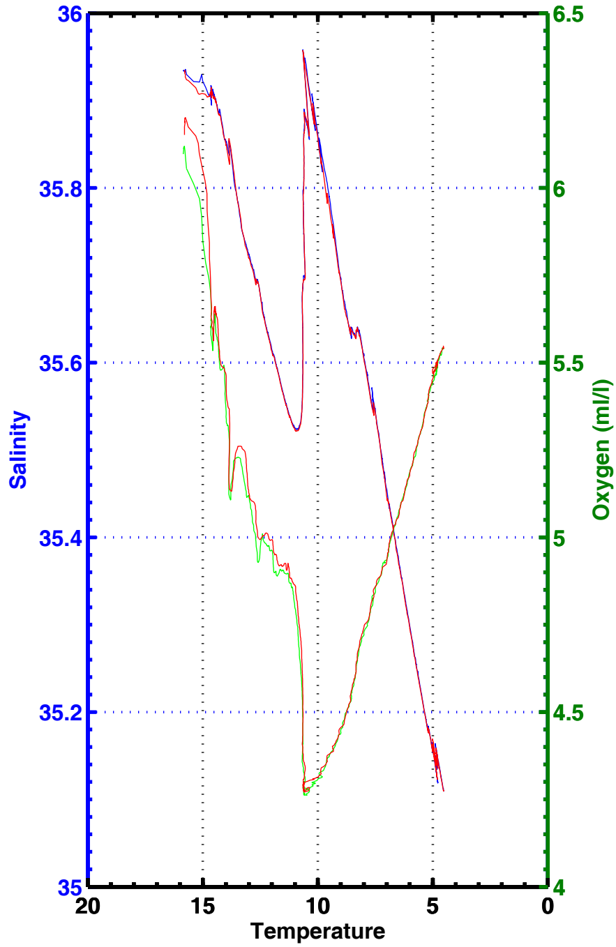
T-S , T-02 , station 2082
