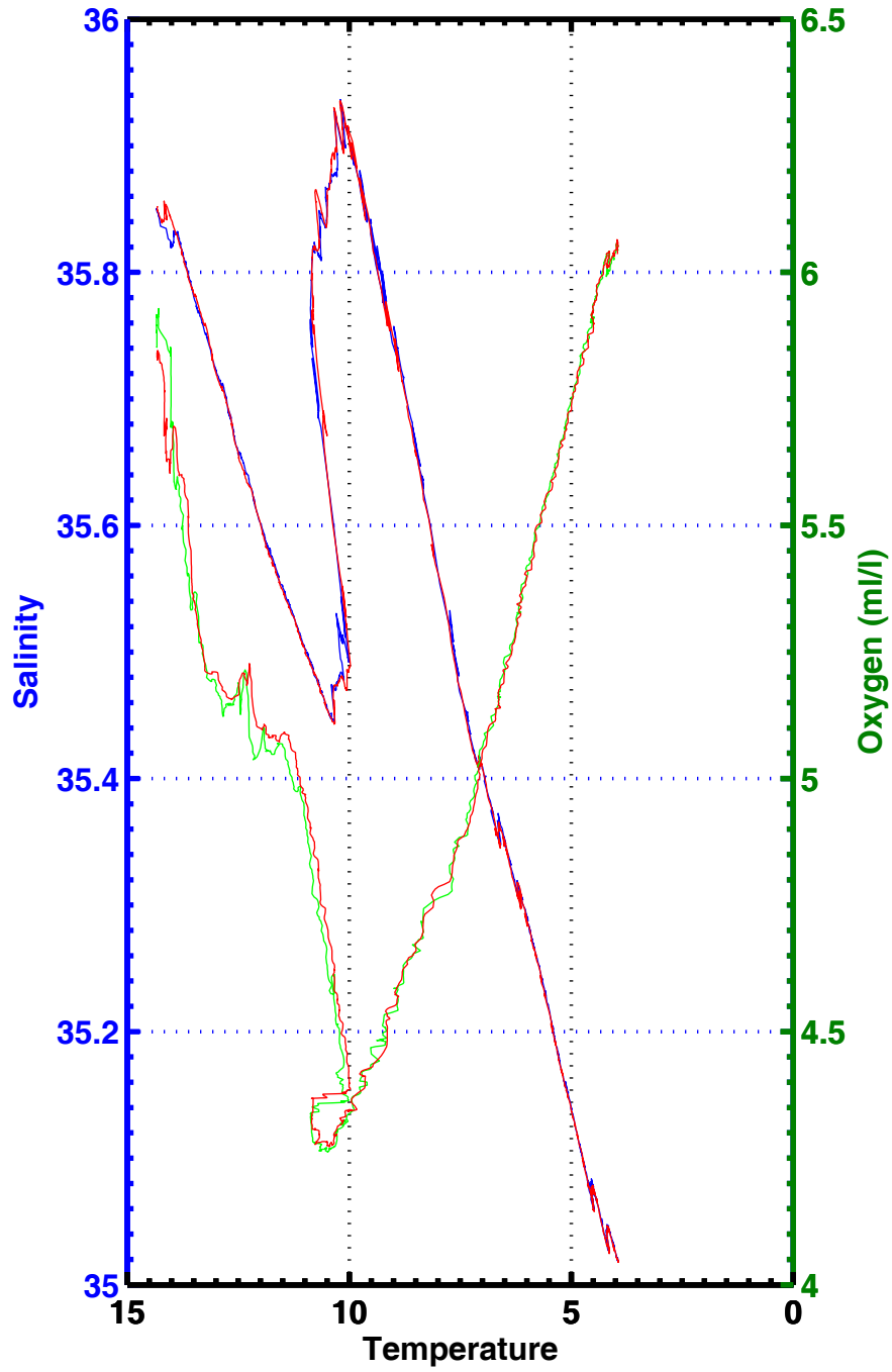
T-S , T-02 , station 2037
