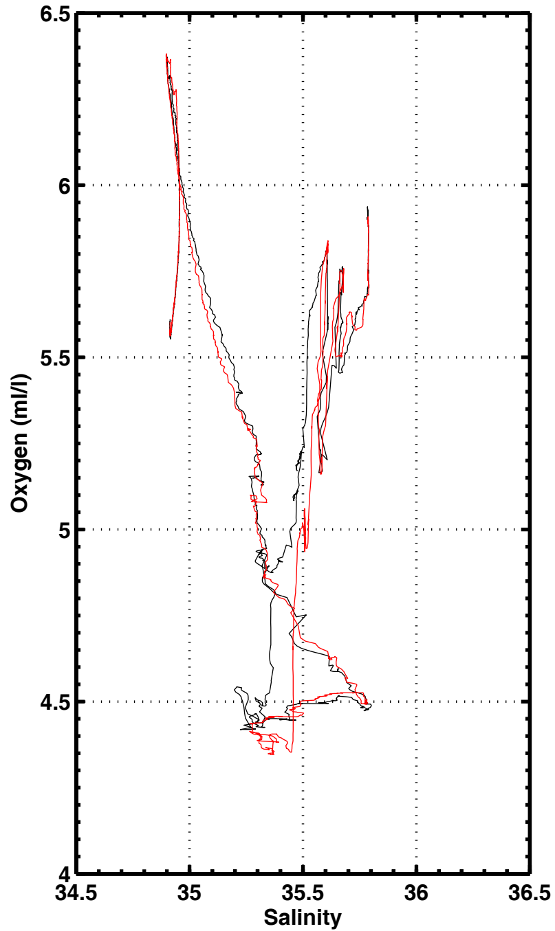
S-02 , station 2014
