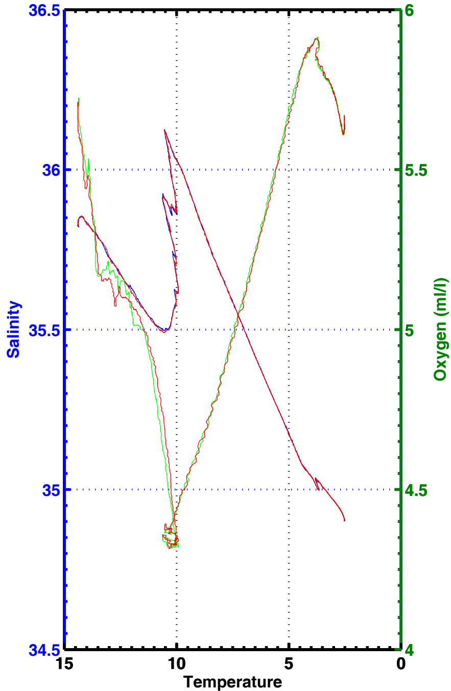
T-S , T-02 , station 2003
