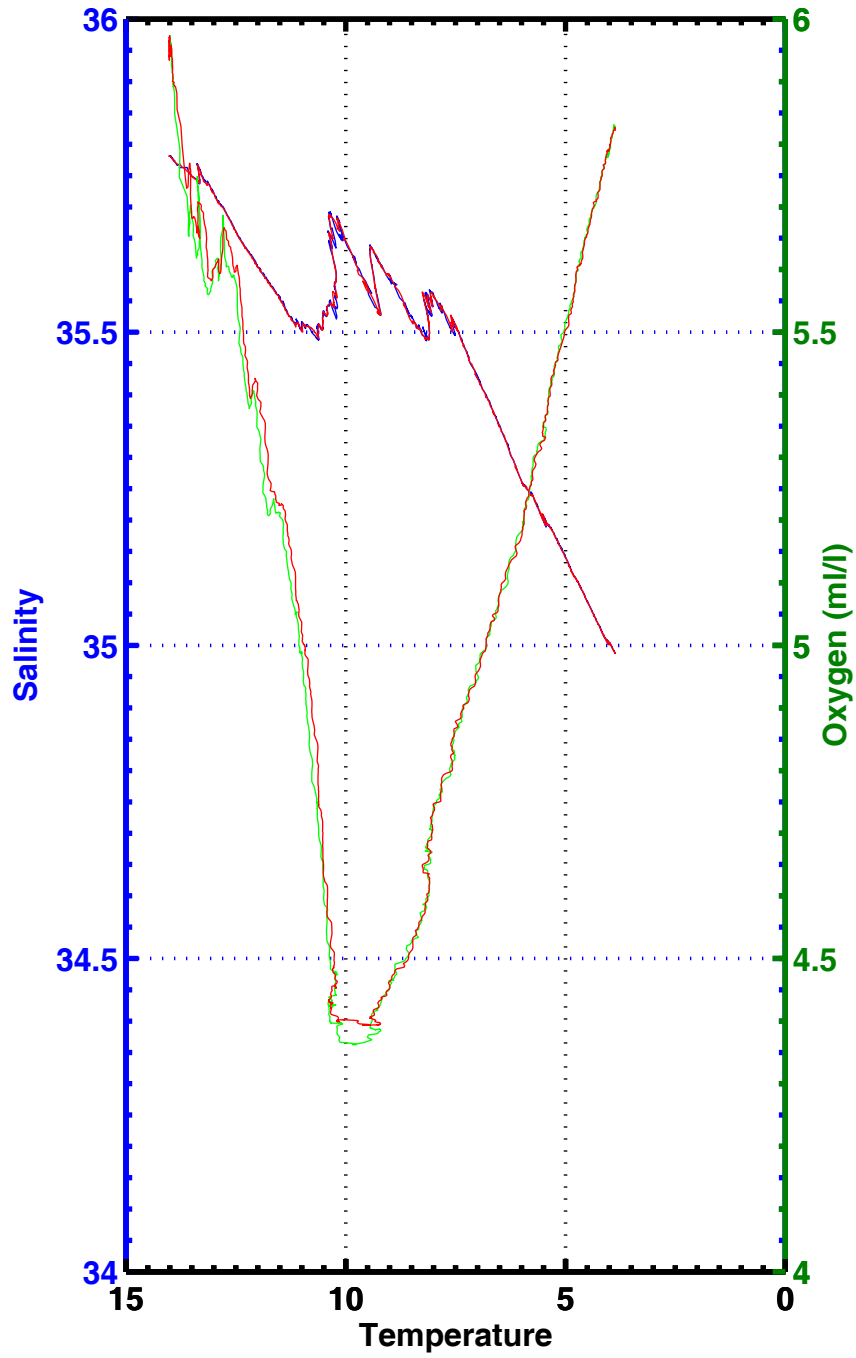
T-S , T-02 , station 2416
