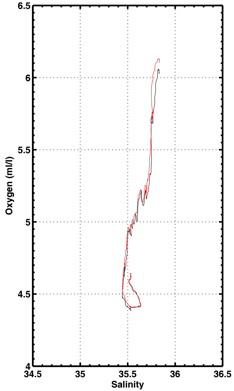
S-O2 , station 2172
