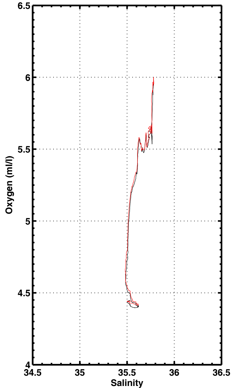
S-O2 , station 2413
