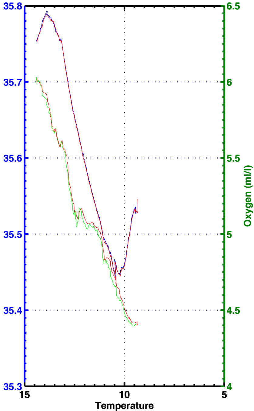
T-S , T-02 , station 2180
