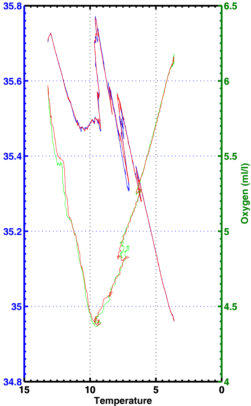
T-S , T-02 , station 2045
