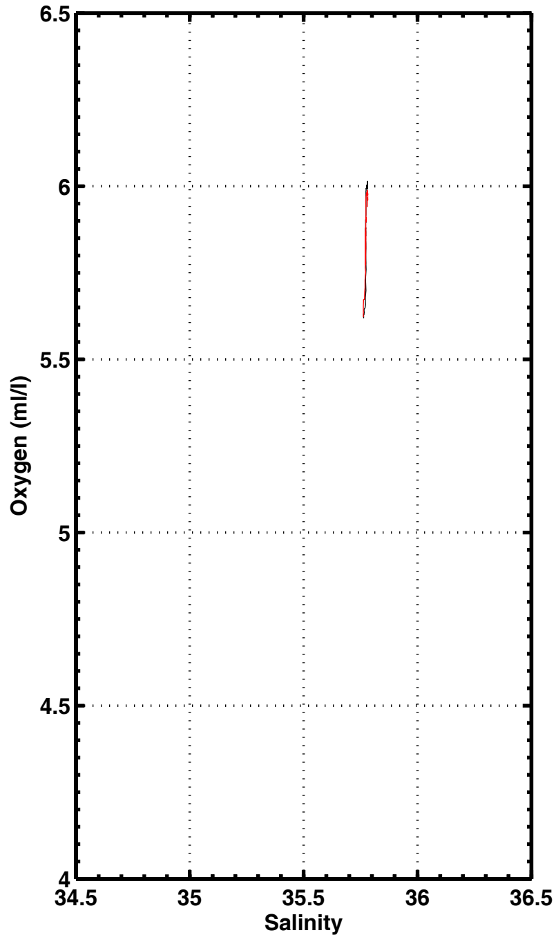
S-02, station 2409
