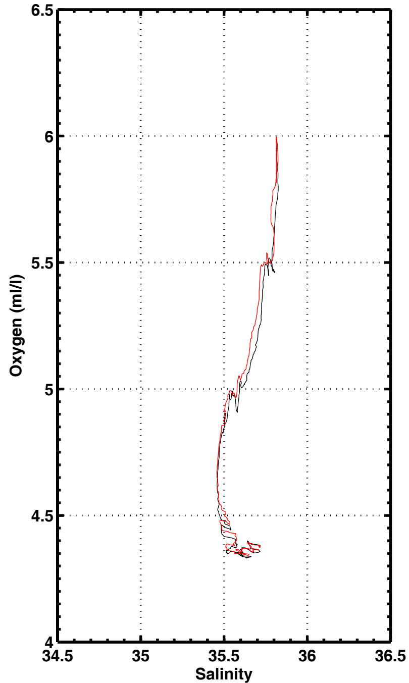
S-O2 , station 2276
