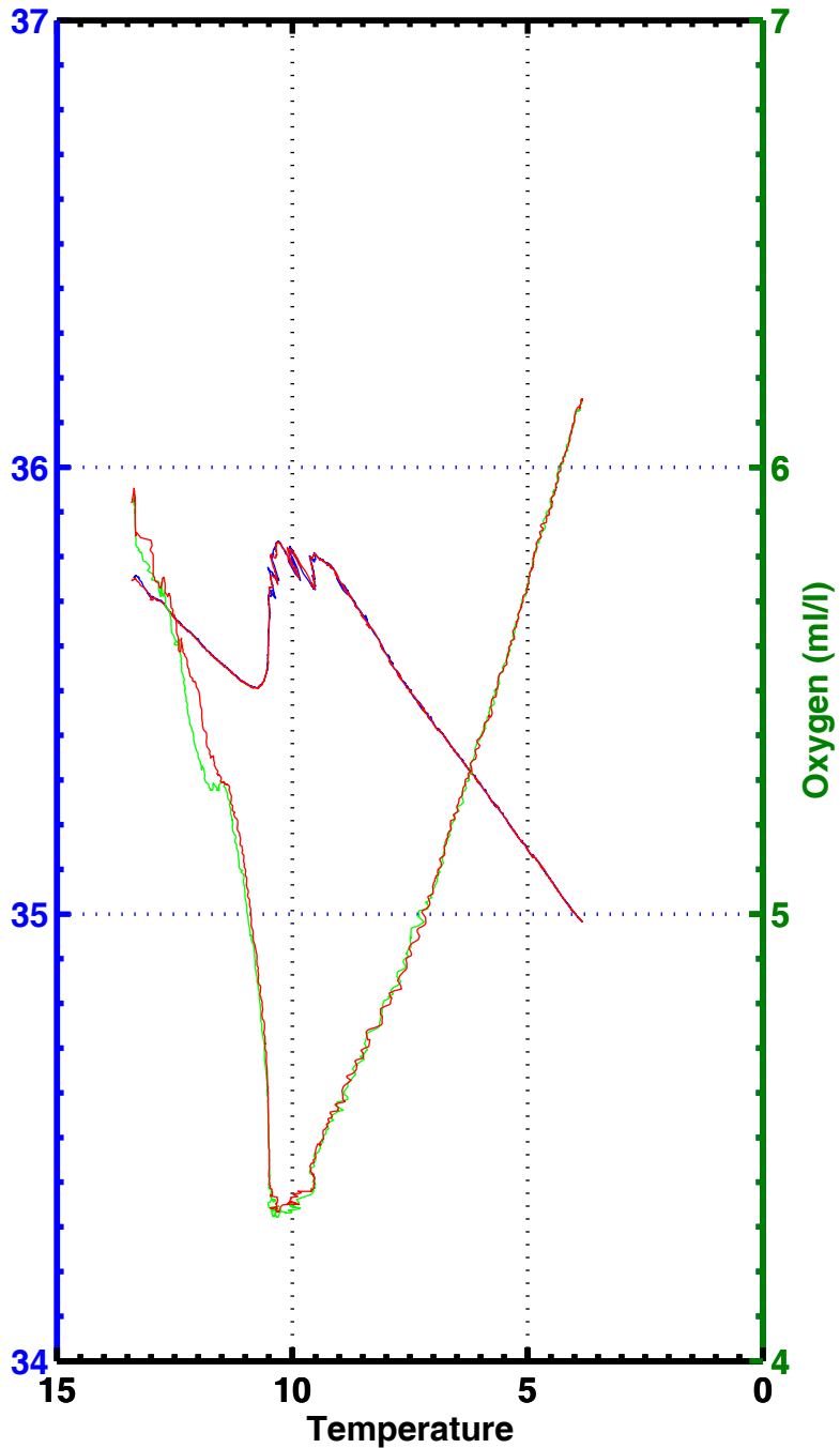
T-S , T-02 , station 2042
