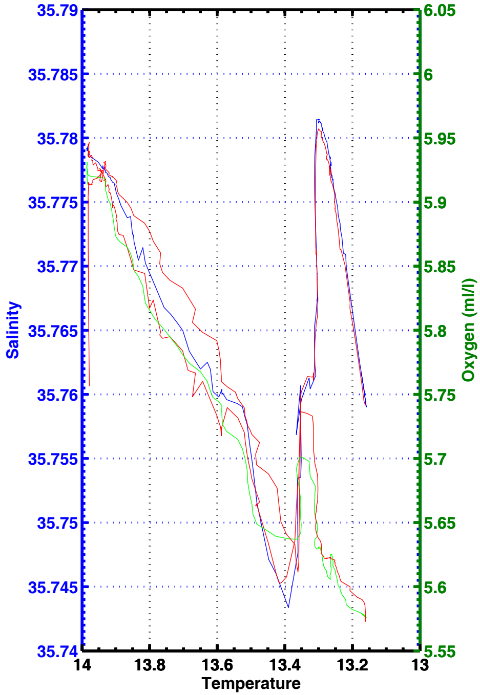
T-S , T-02 , station 2401
