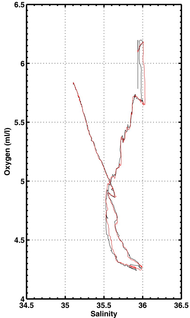
S-O2 , station 2078
