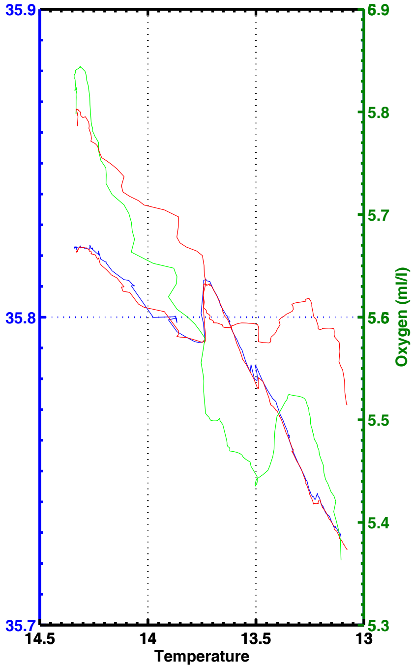
T-S , T-02 , station 2265
