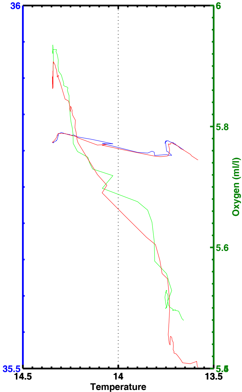
T-S , T-02 , station 2272
