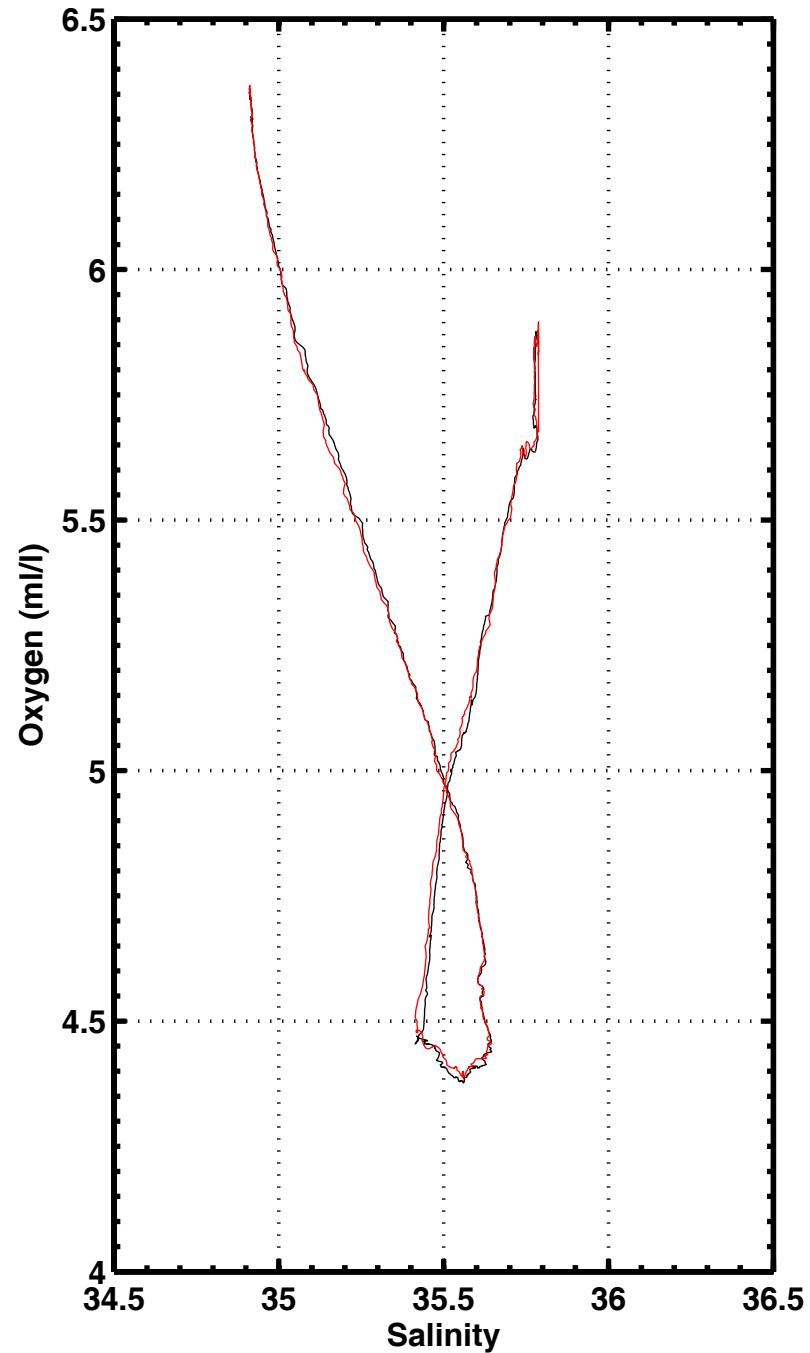
S-O2 , station 2055
