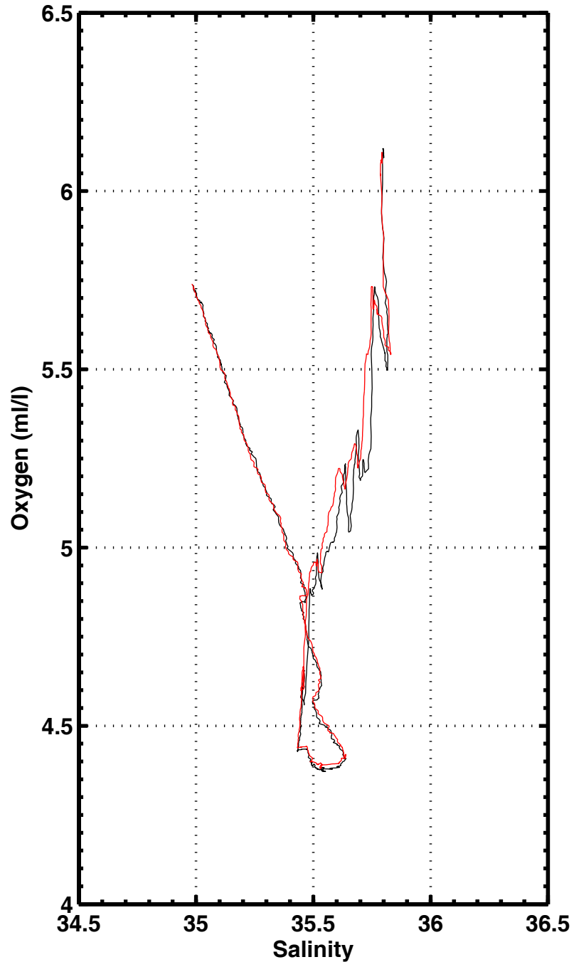
S-02 , station 2171
