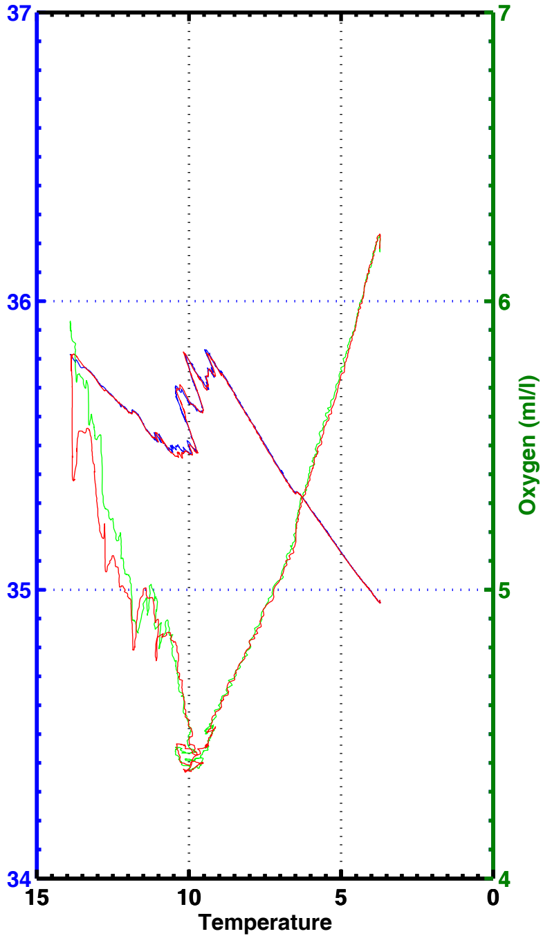
T-S , T-02 , station 2021
