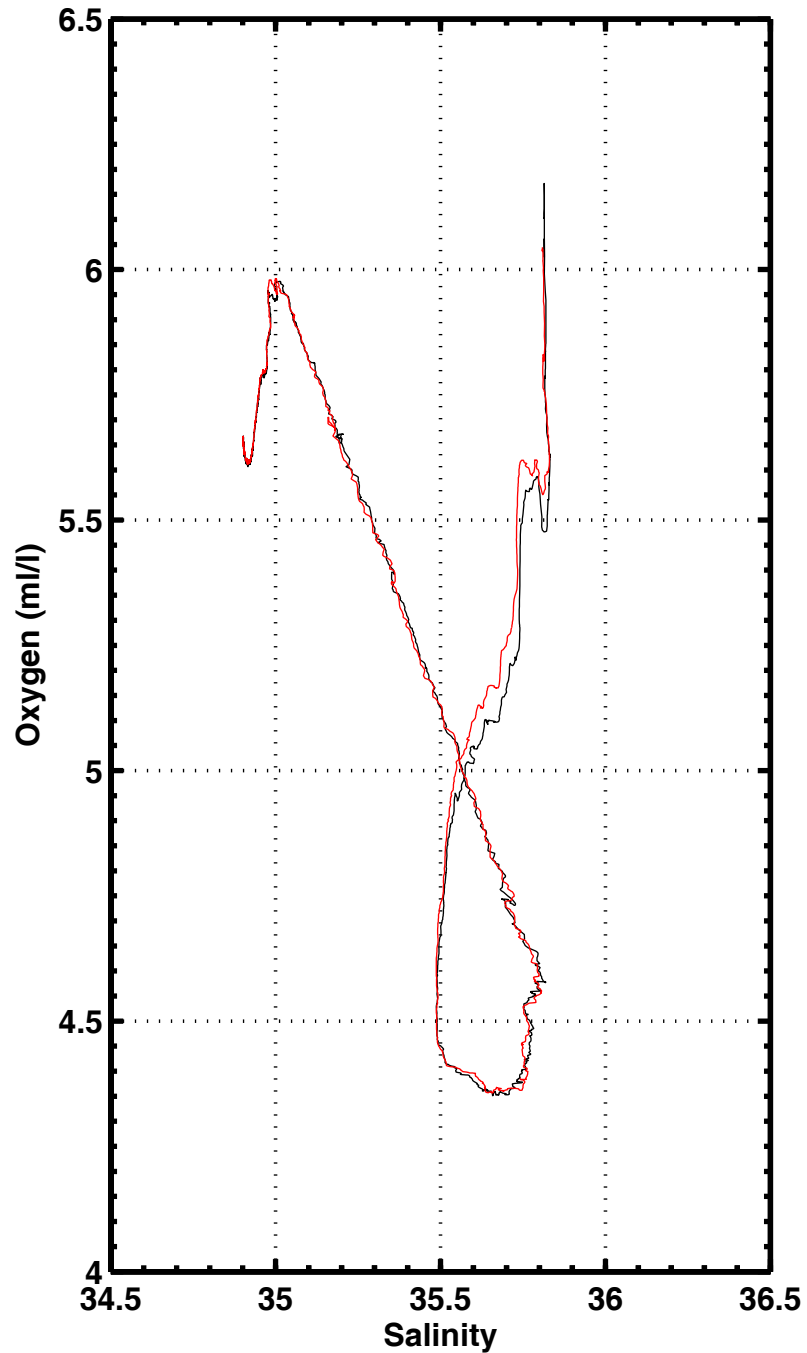
S-O2 , station 2034
