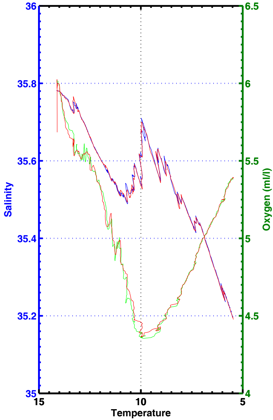
T-S , T-02 , station 2406
