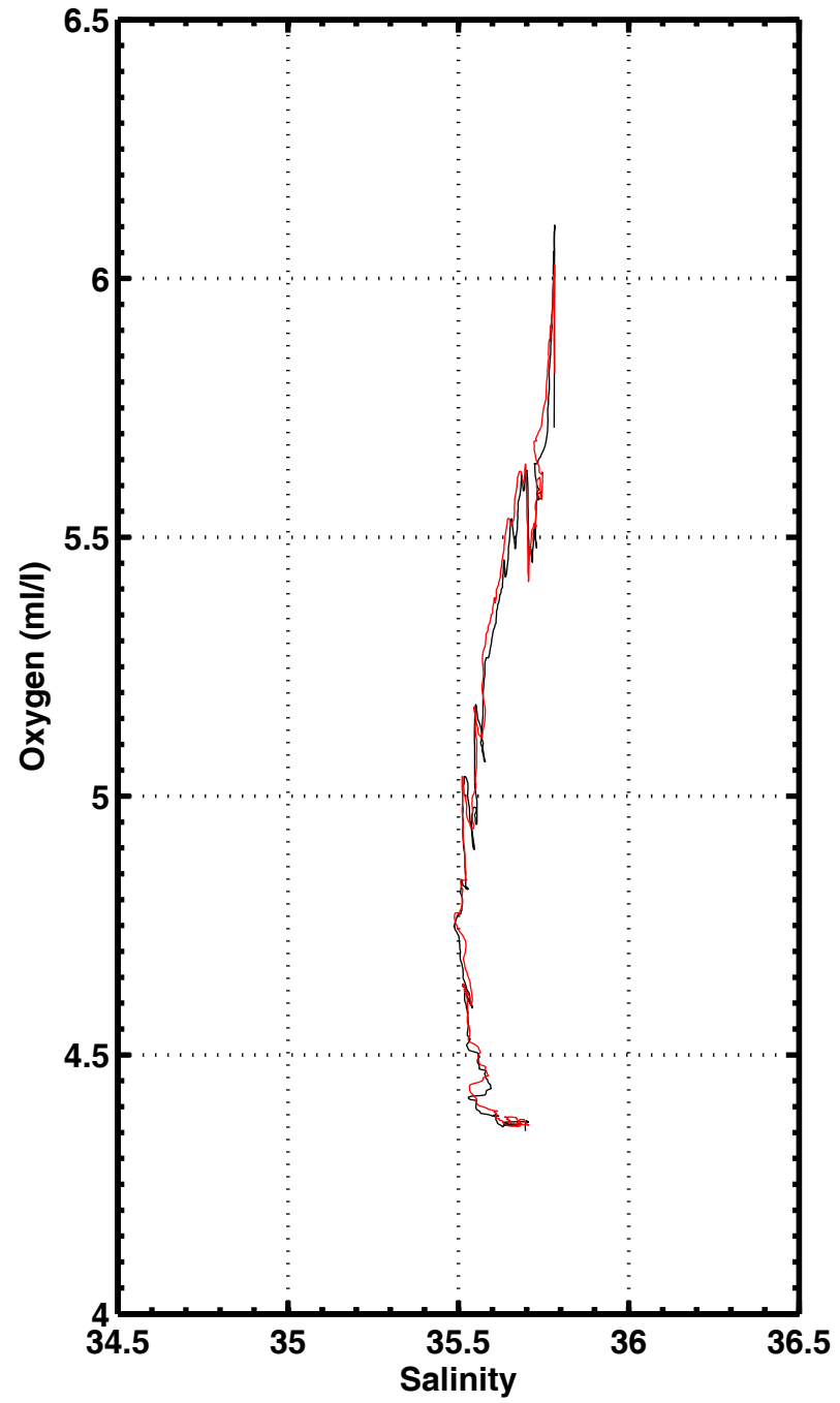
S-O2 , station 2405
