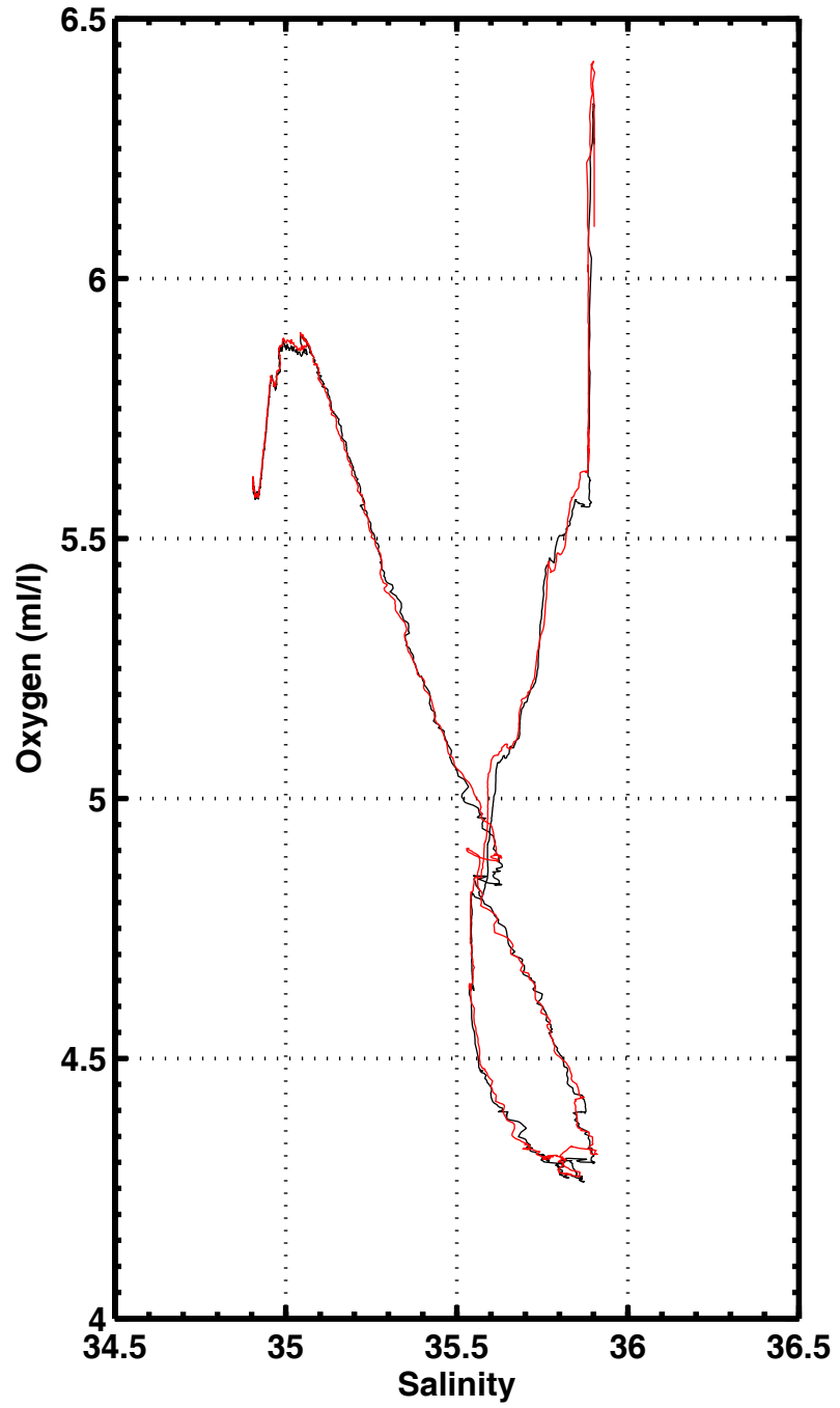
S-O2, station 2071
