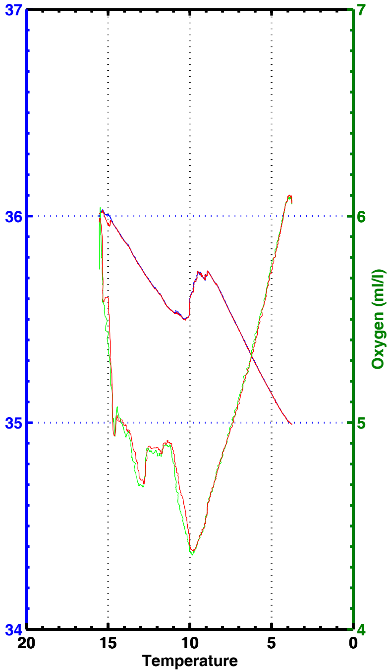
T-S, T-02, station 2033
