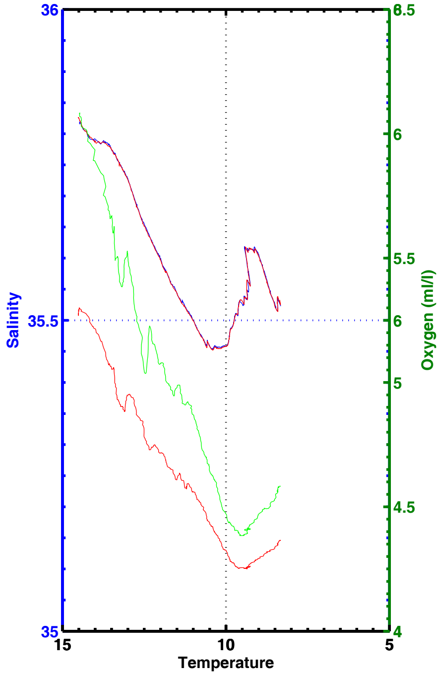
T-S , T-02 , station 2182
