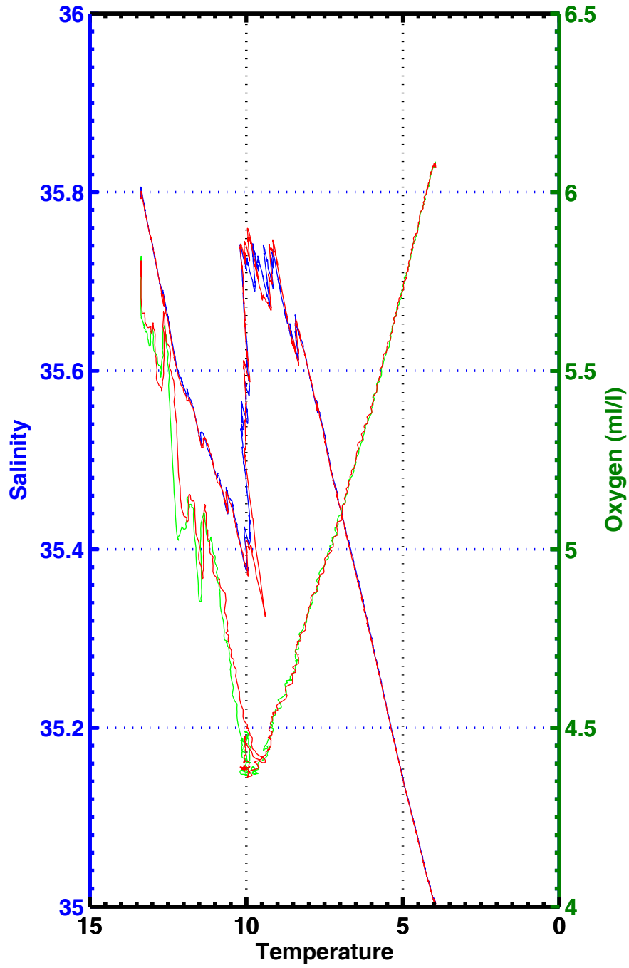
T-S , T-02 , station 2017
