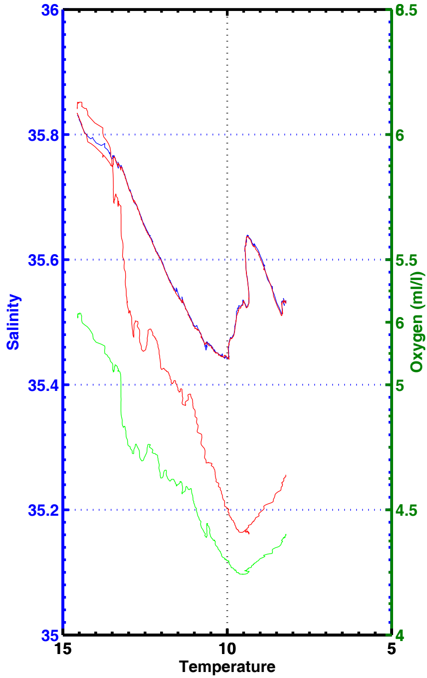
T-S , T-02 , station 2172
