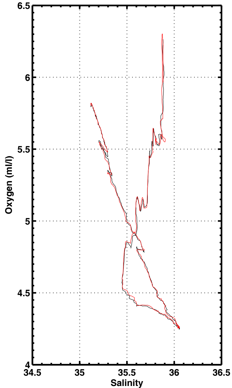
S-O2 , station 2079
