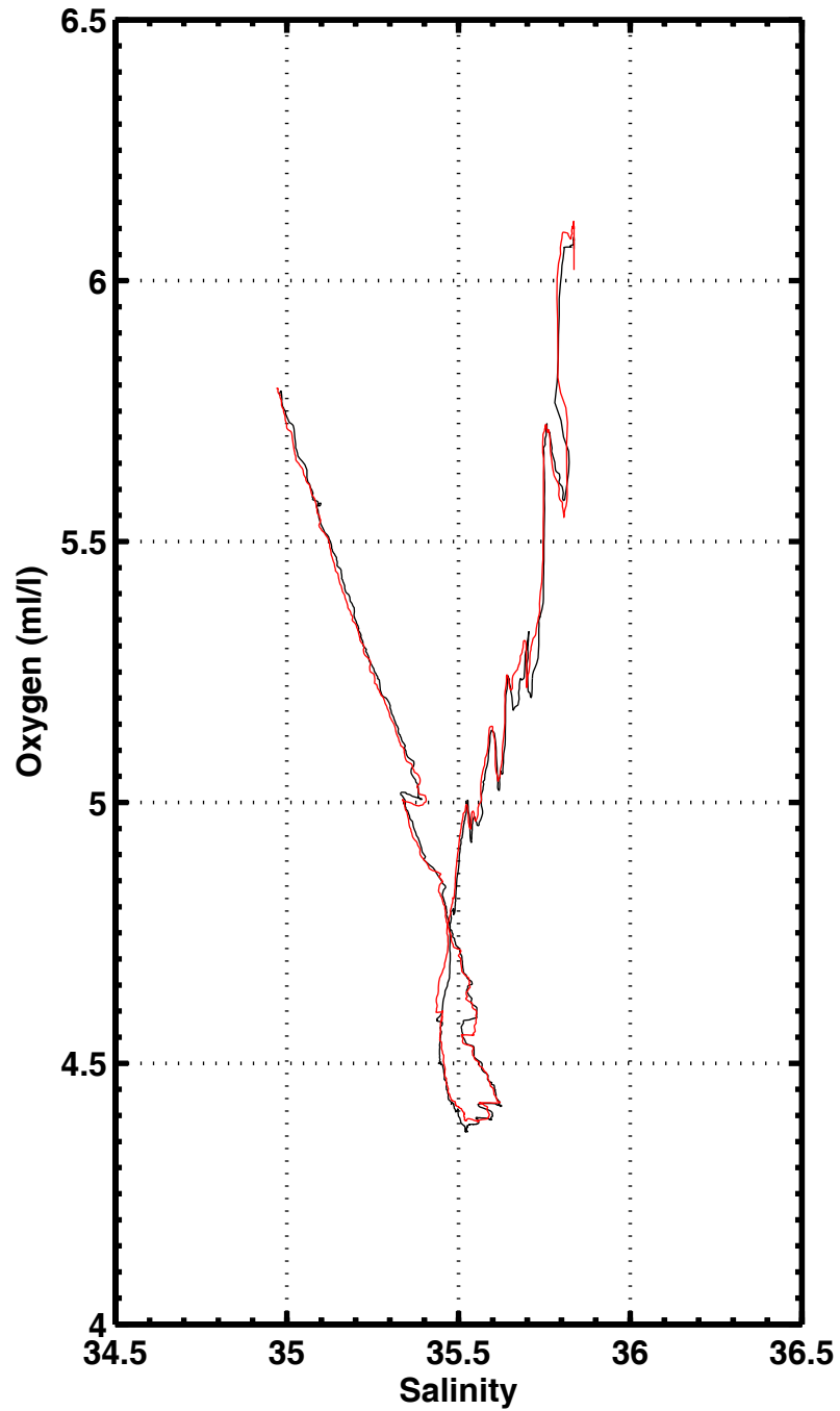
S-O2 , station 2174
