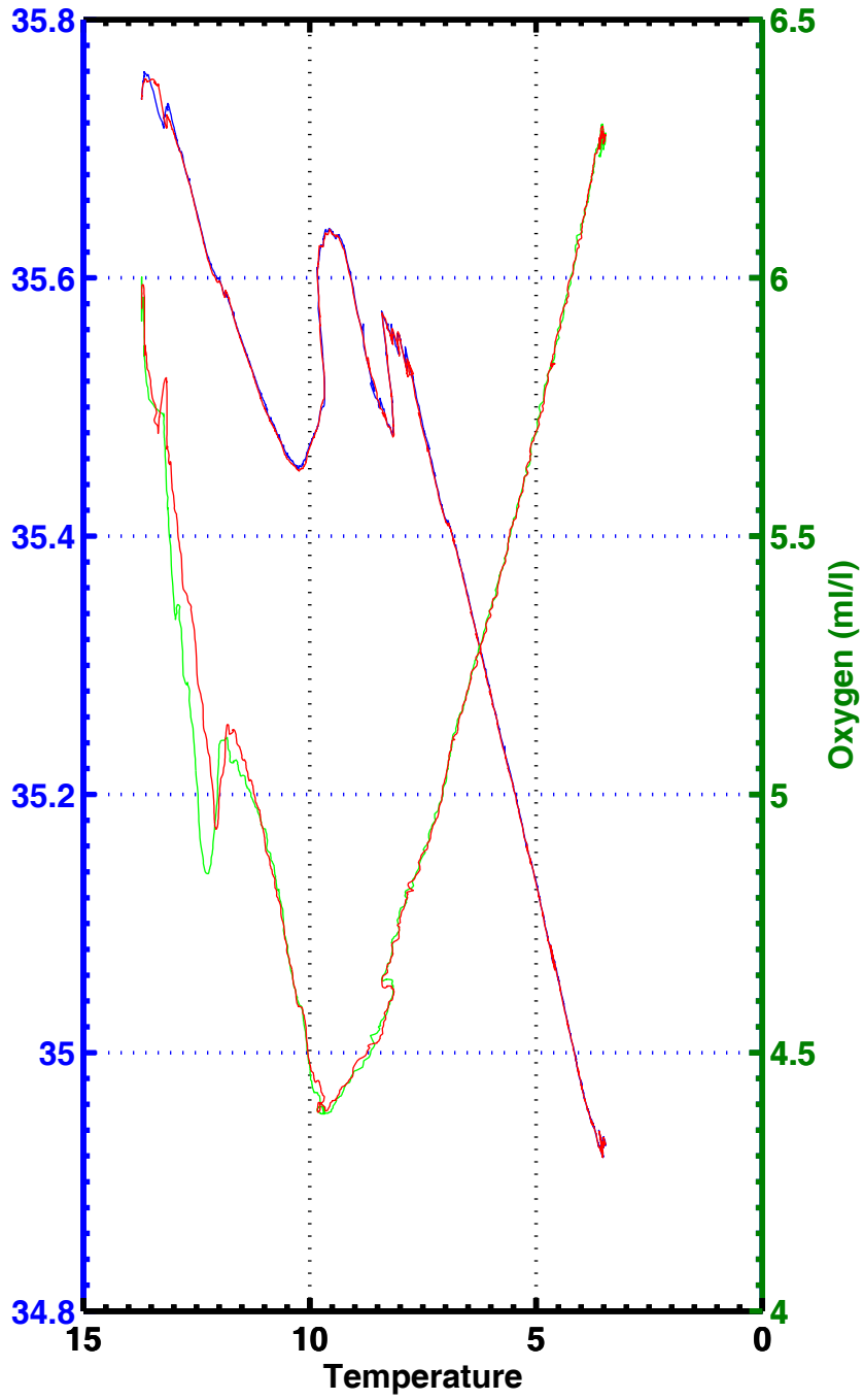
T-S , T-02 , station 2048
