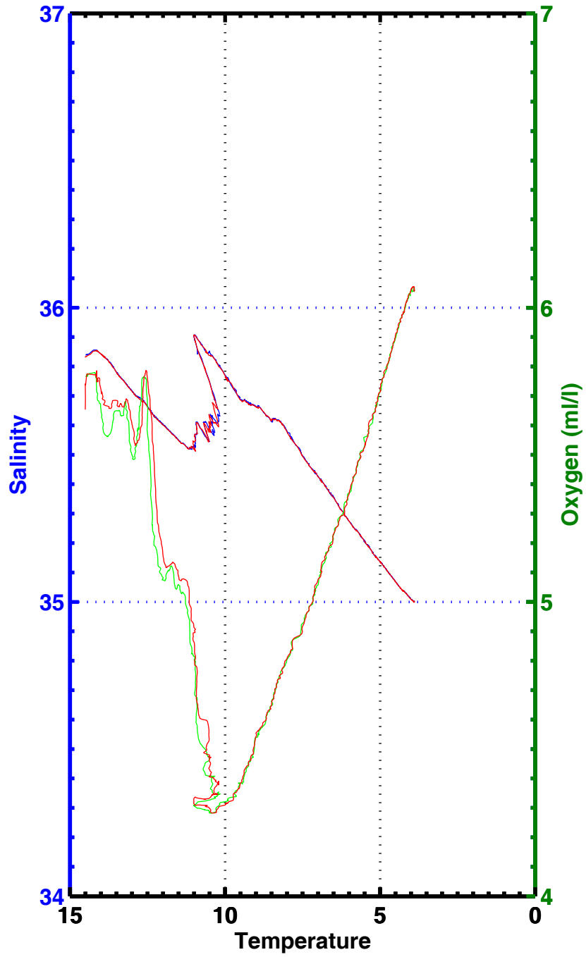
T-S , T-02 , station 2005
