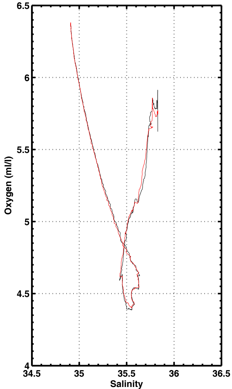
S-O2 , station 2054
