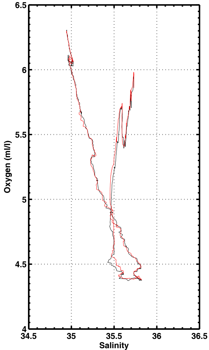
S-O2 , station 2024
