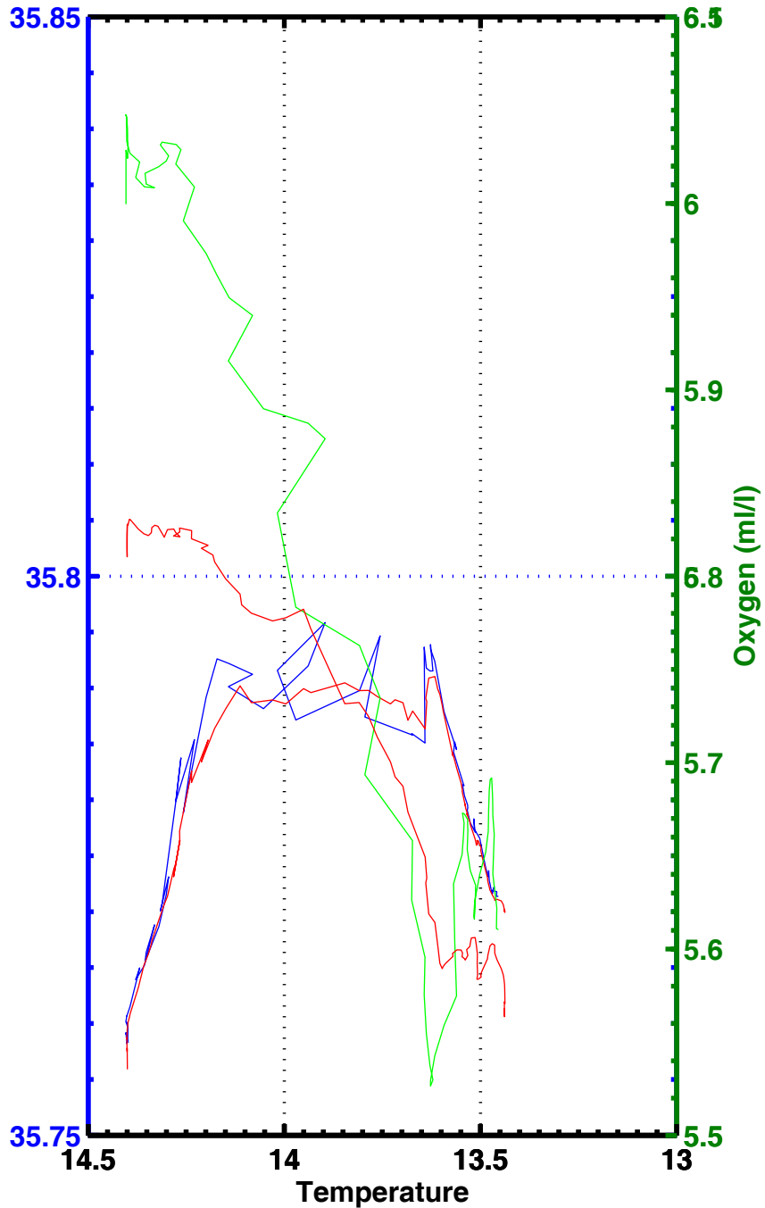
T-S , T-02 , station 2178
