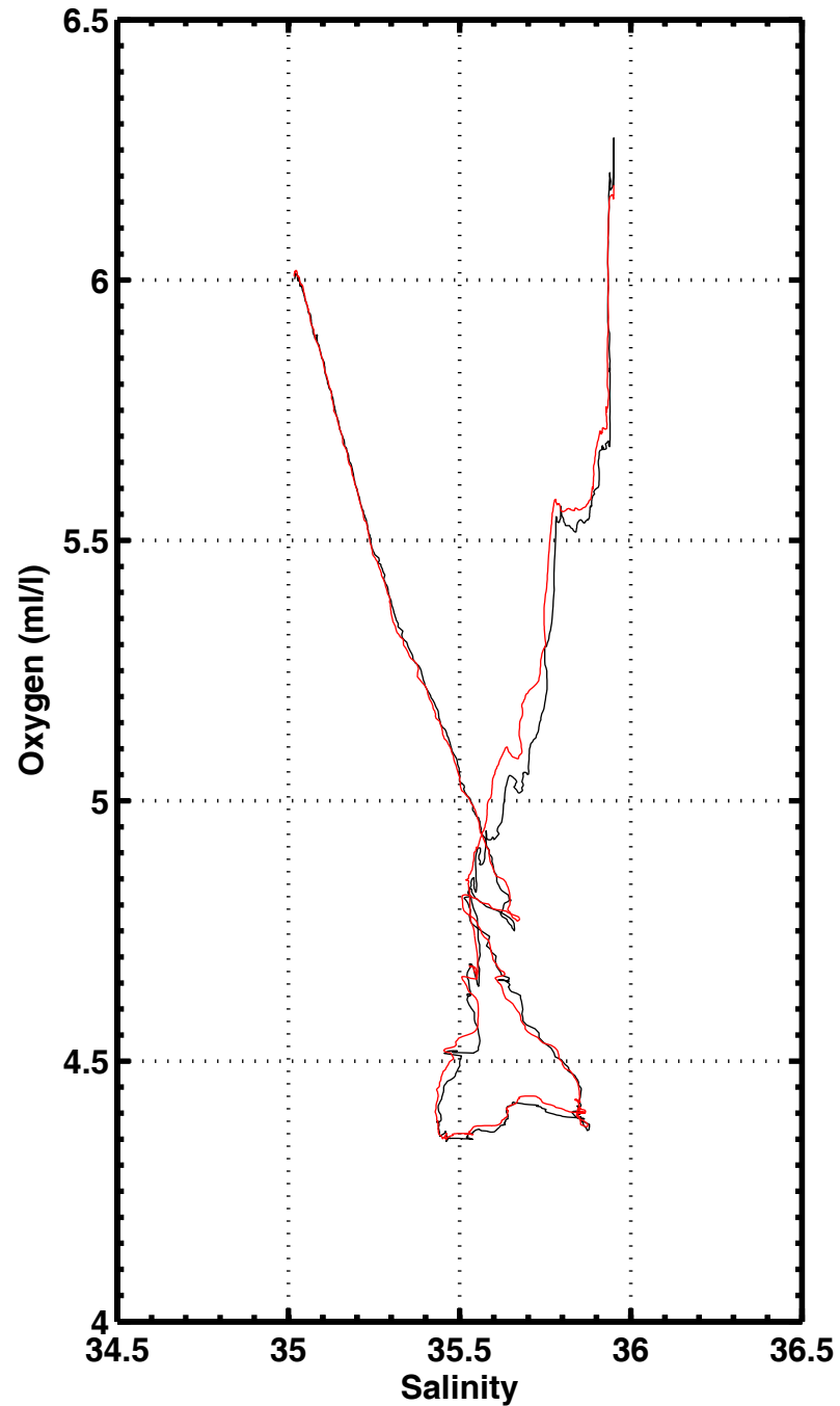
S-O2 , station 2074
