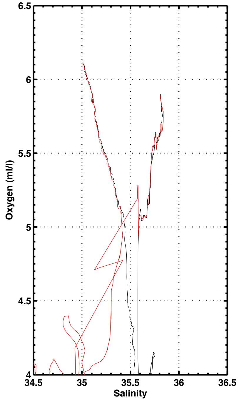
S-02 , station 2029
