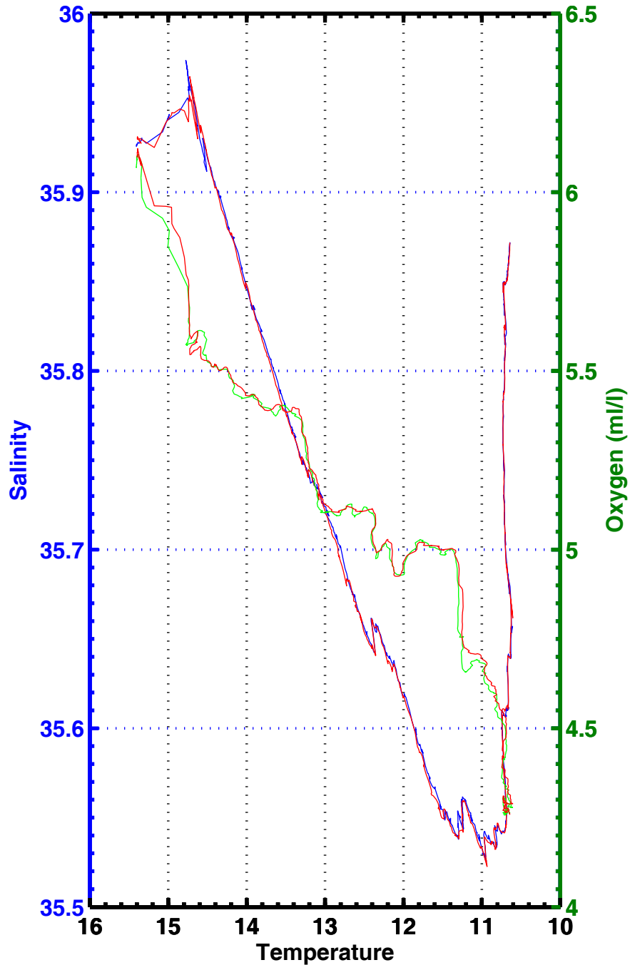
T-S , T-02 , station 2086
