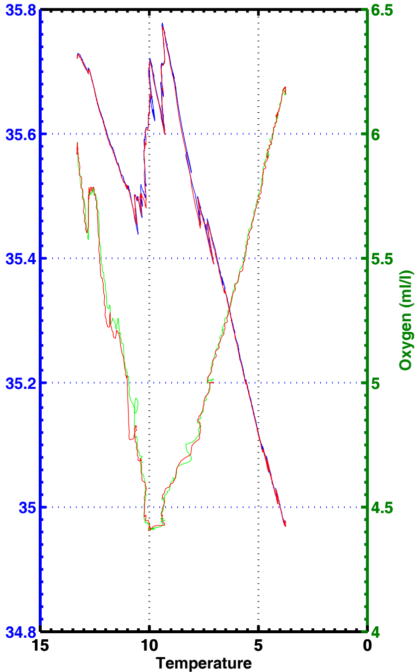
T-S , T-02 , station 2025
