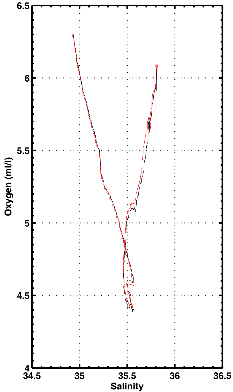
S-02 , station 2062
