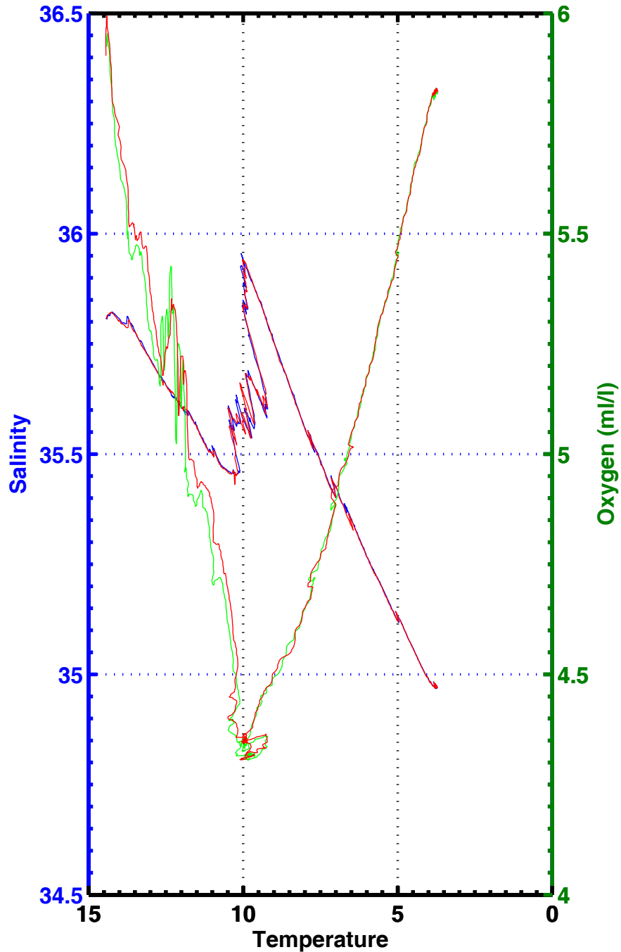
T-S , T-02 , station 2279
