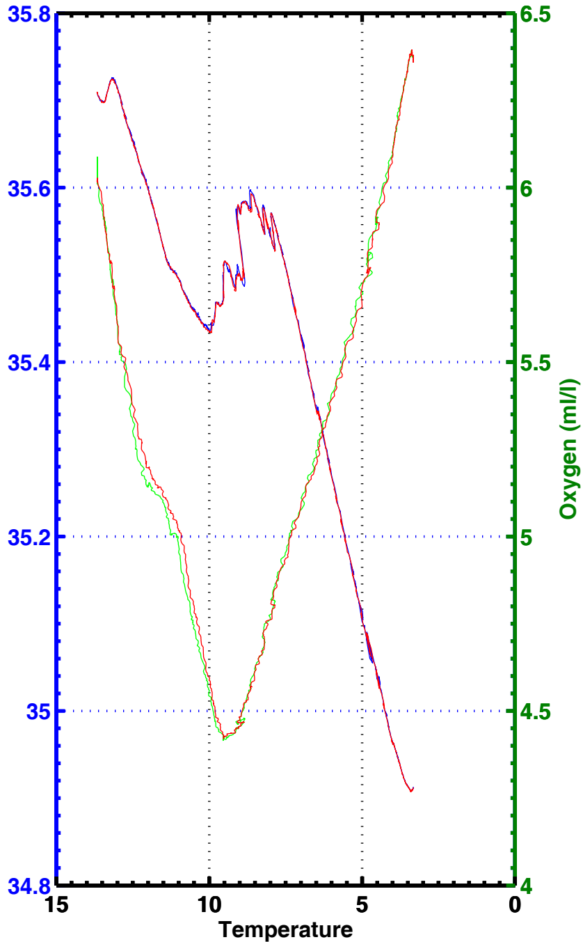
T-S , T-02 , station 2060
