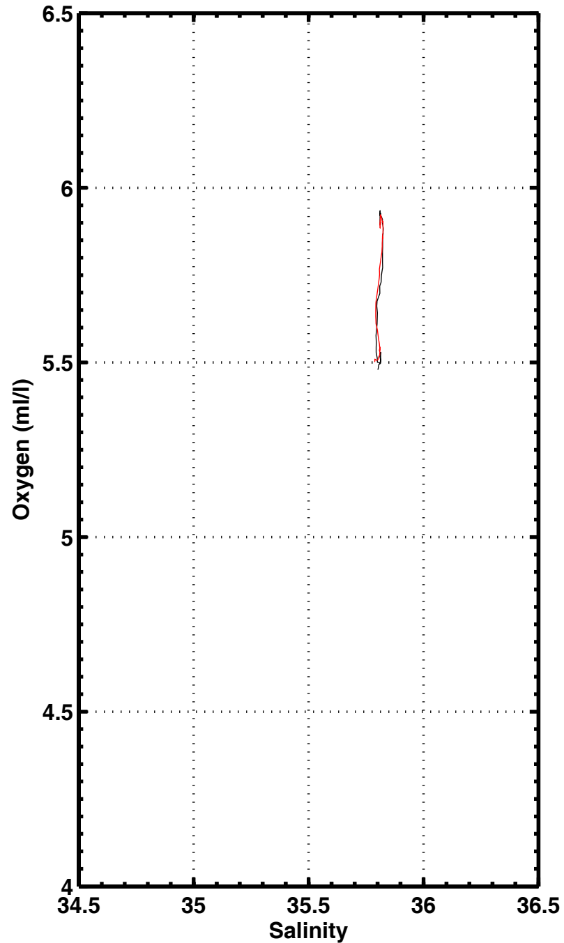
S-O2 , station 2272
