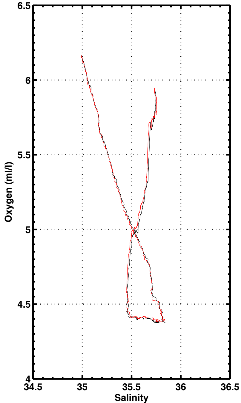
S-02 , station 2022
