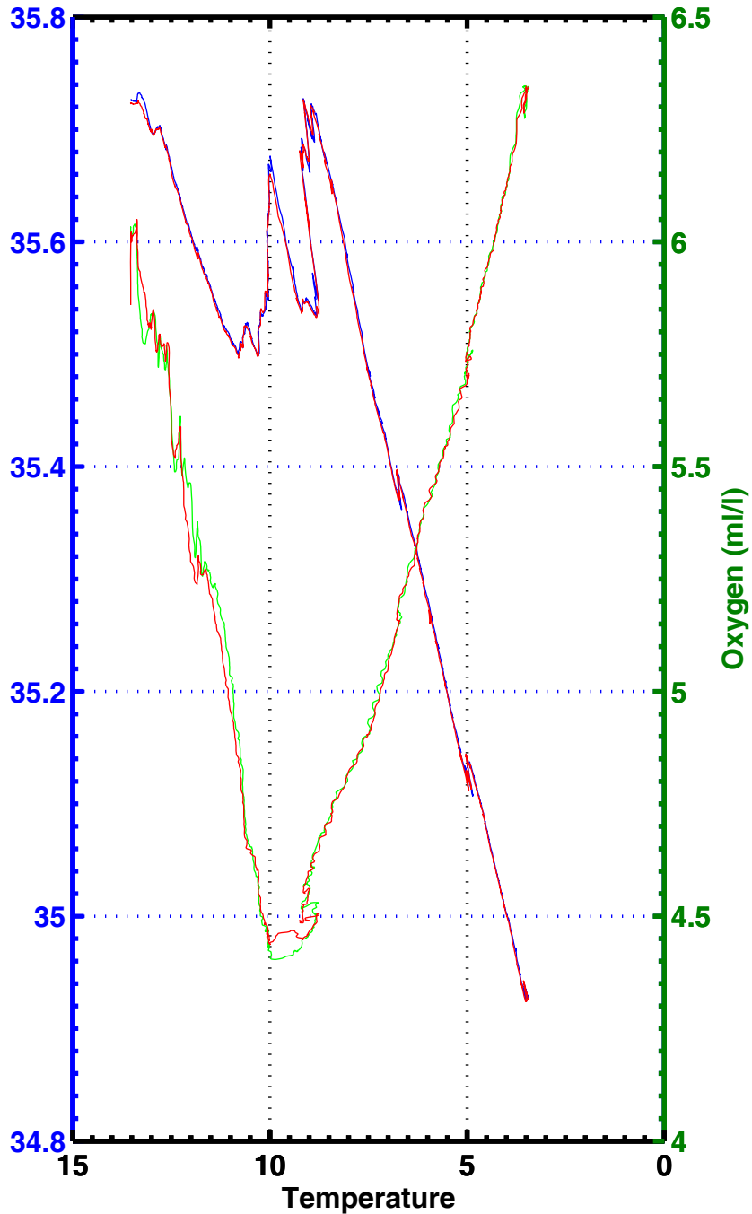
T-S , T-02 , station 2026
