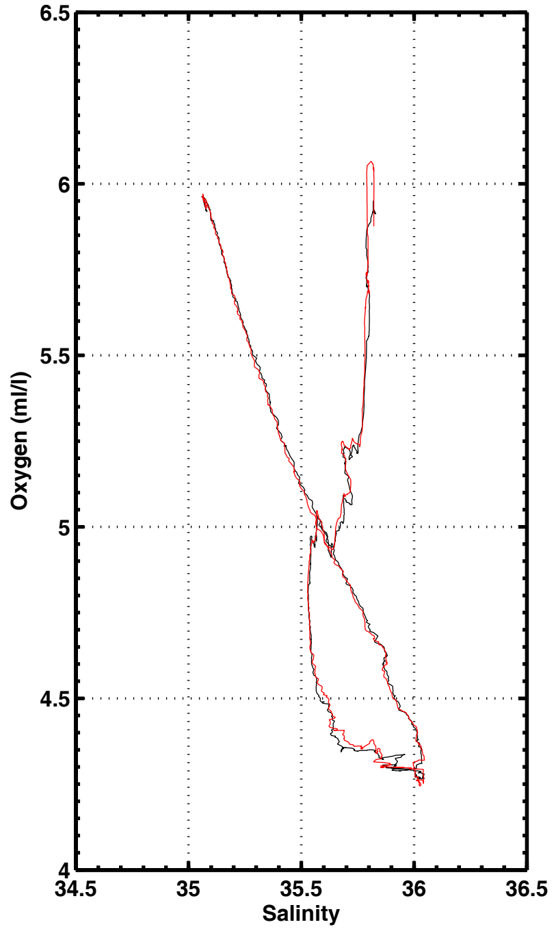
S-02 , station 2031
