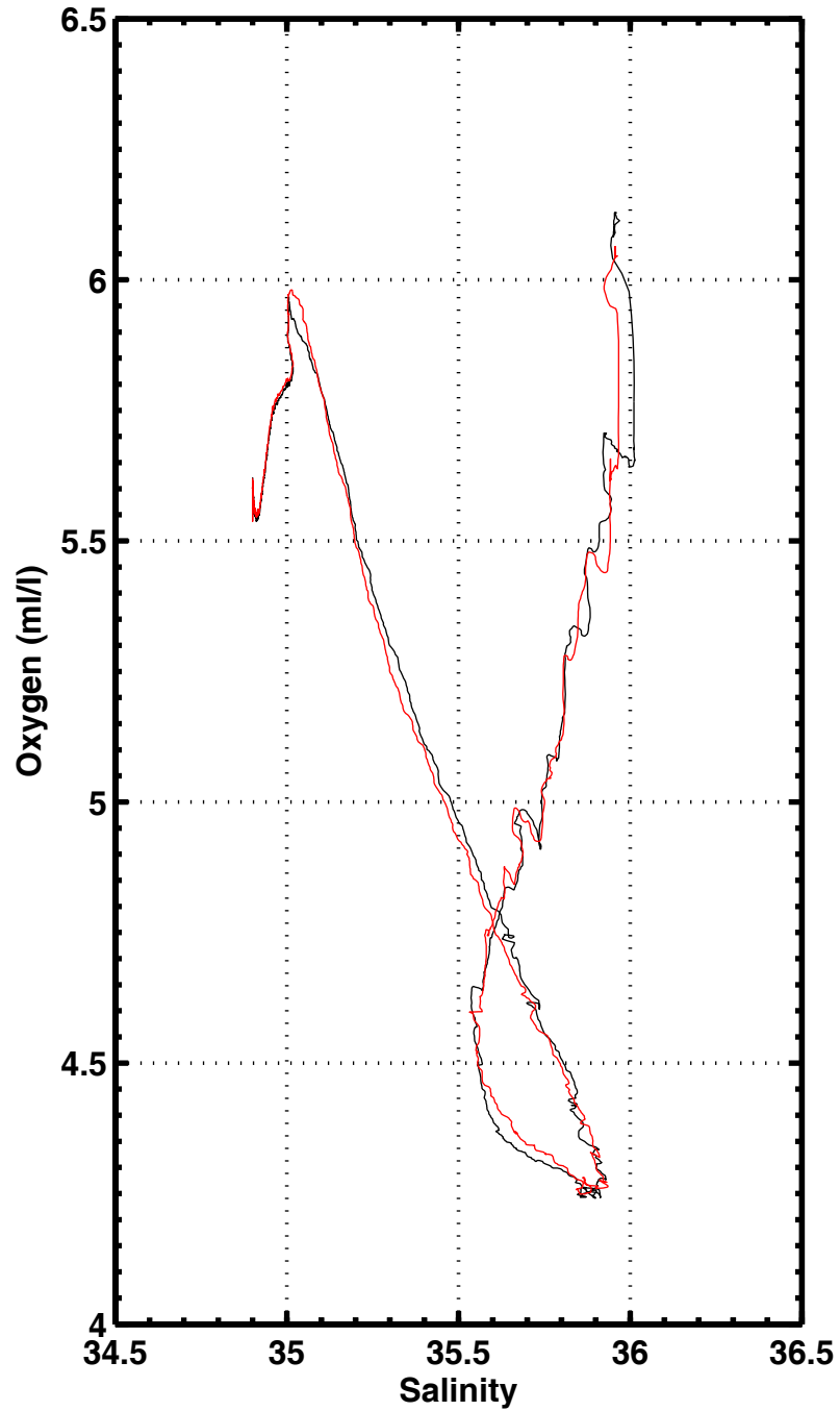
S-02, station 2076
