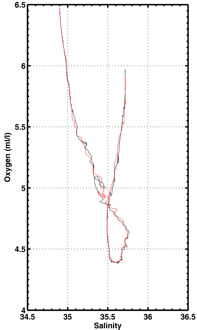
S-O2 , station 2019
