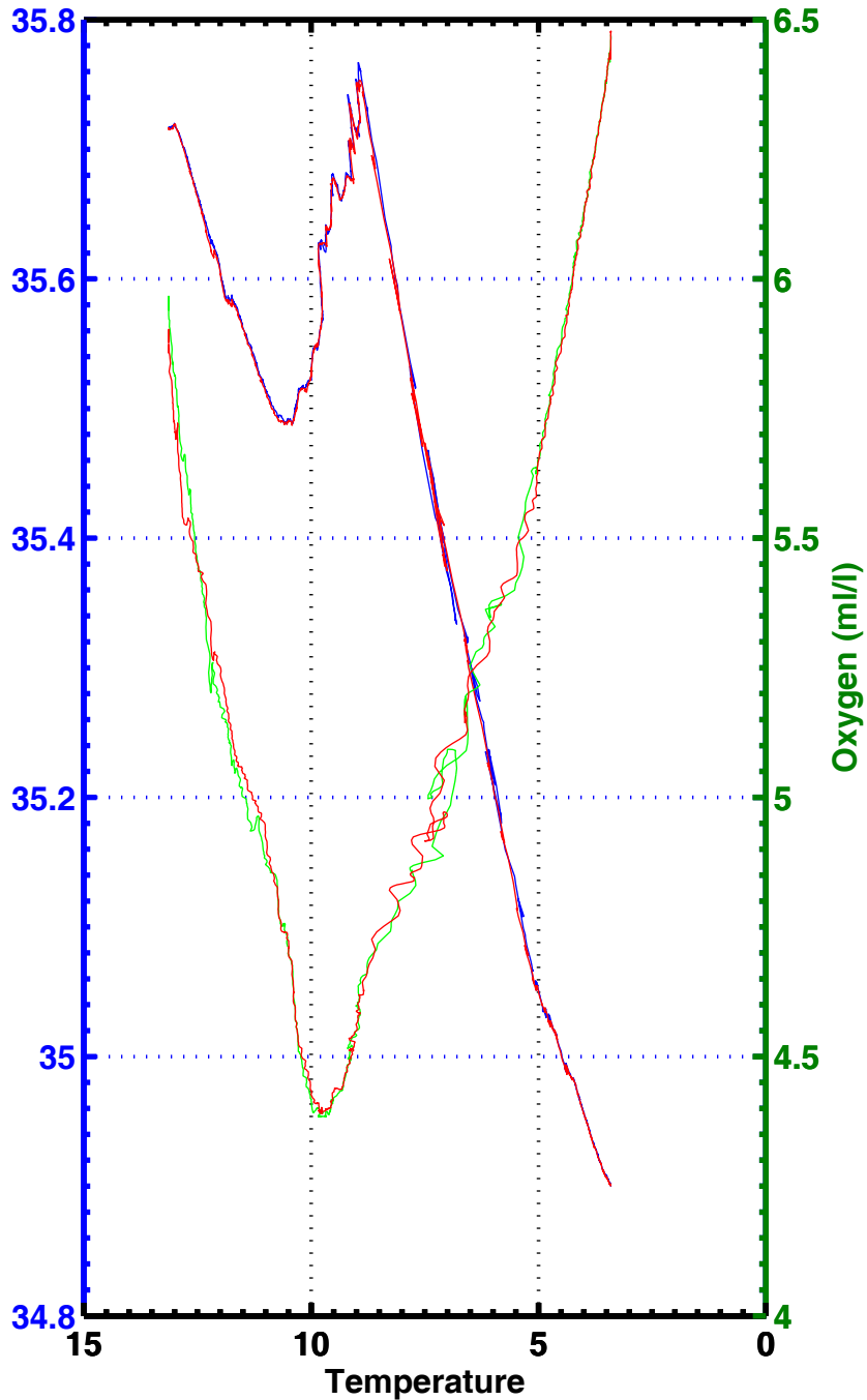
T-S , T-02 , station 2019
