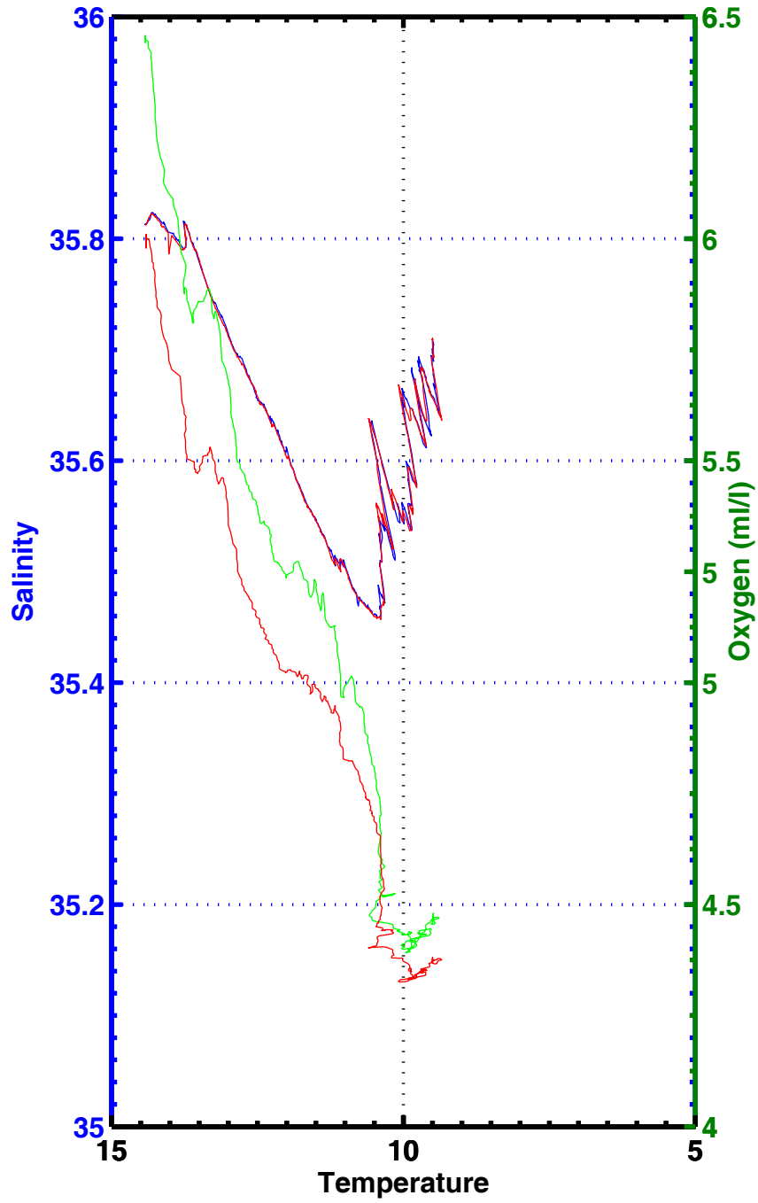
T-S , T-02 , station 2270
