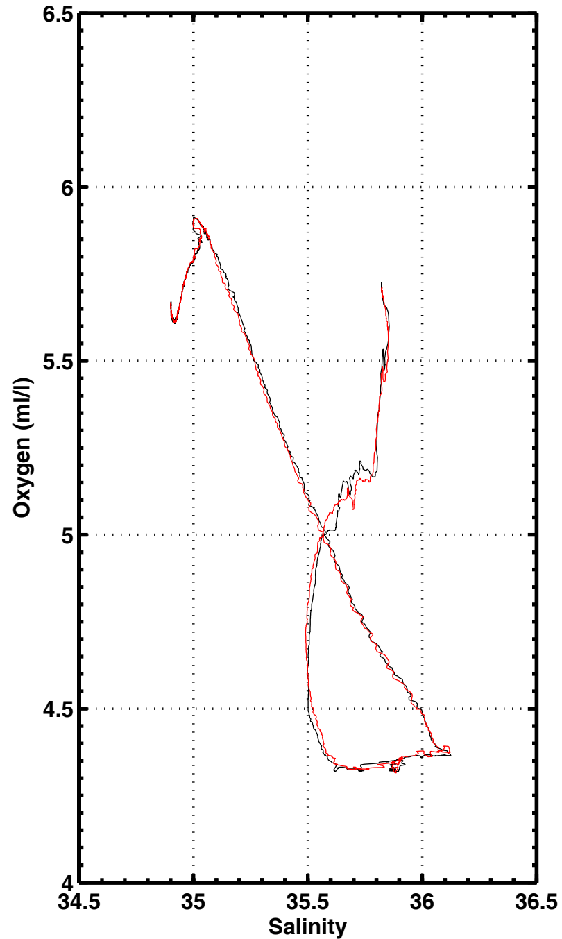
S-O2 , station 2003
