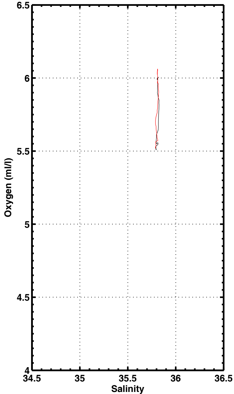
S-02 , station 2277
