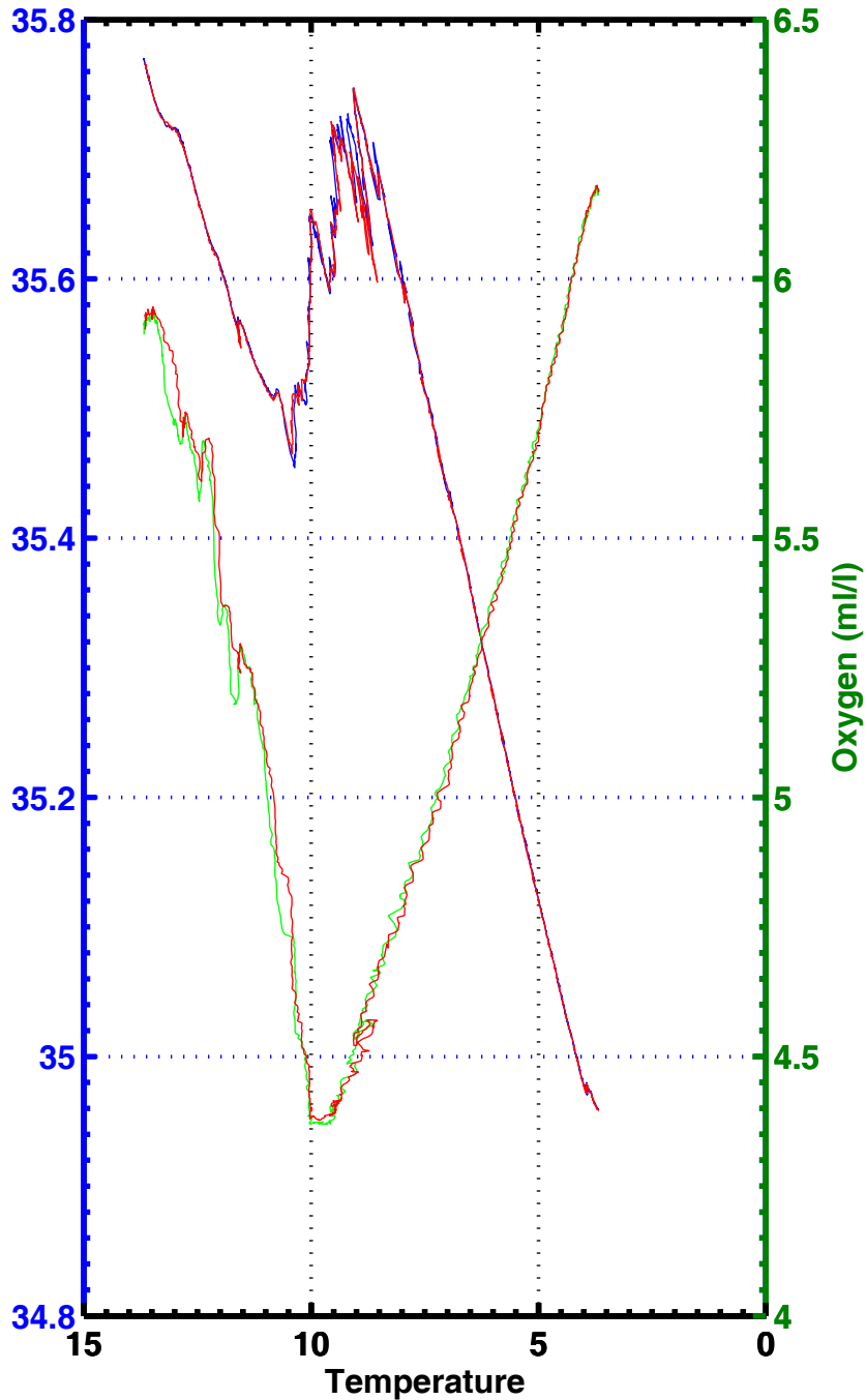
T-S , T-02 , station 2040
