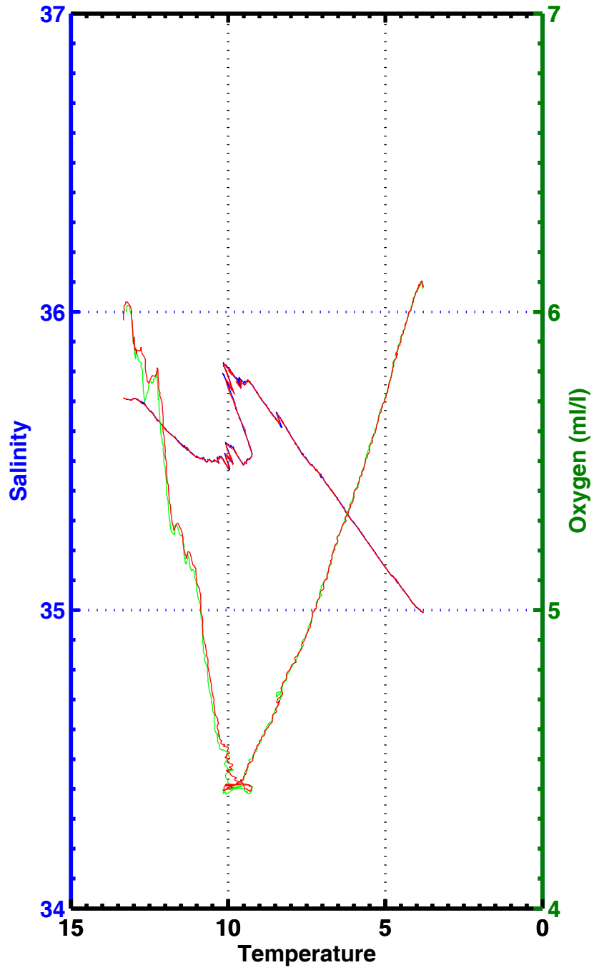
T-S , T-02 , station 2007
