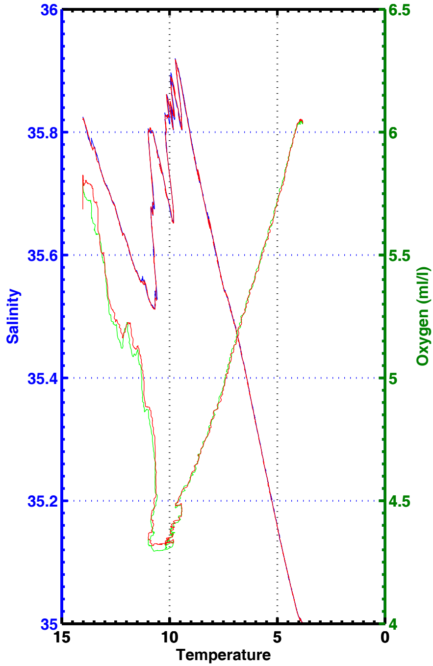
T-S , T-02 , station 2004
