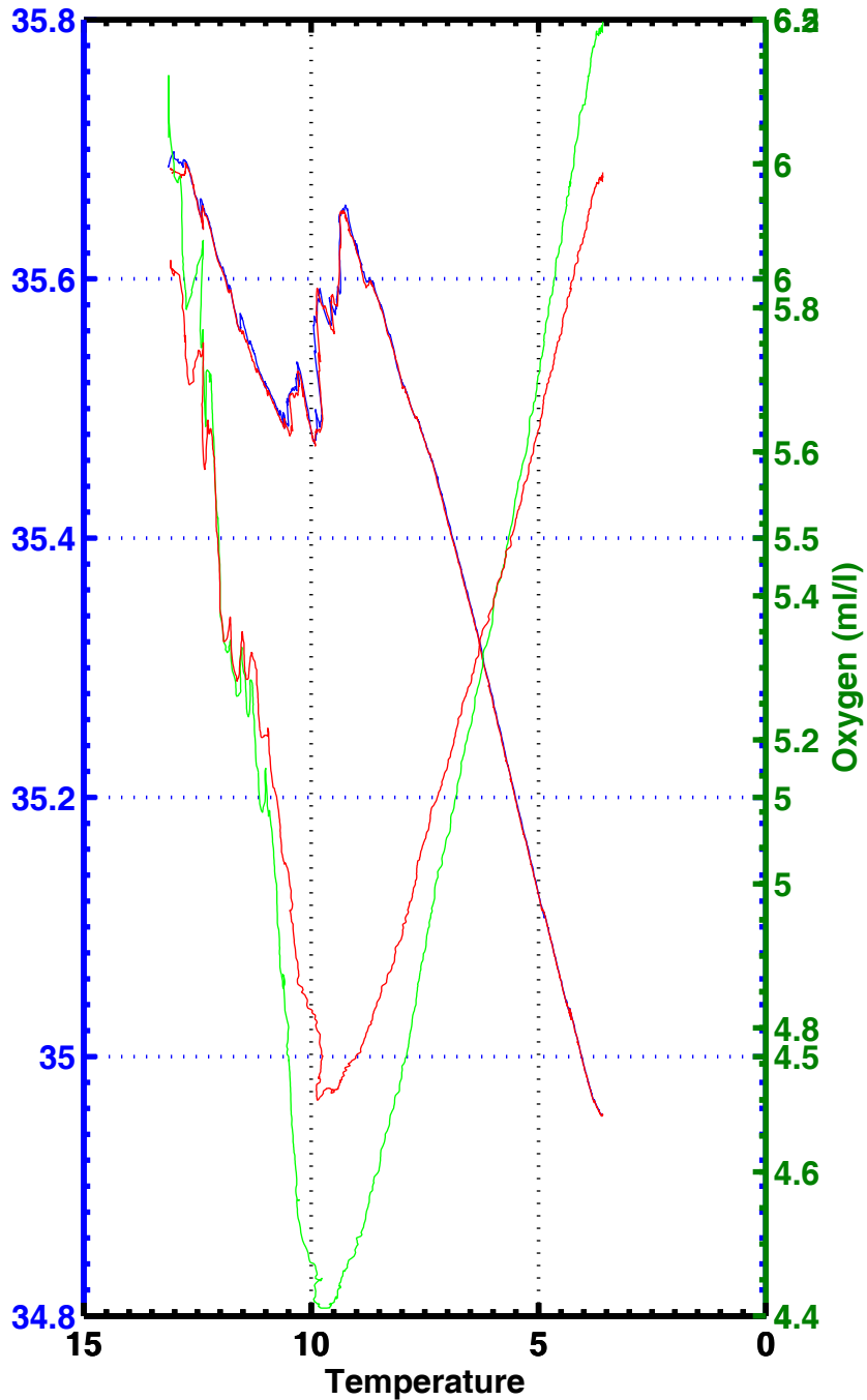
T-S , T-02 , station 2011
