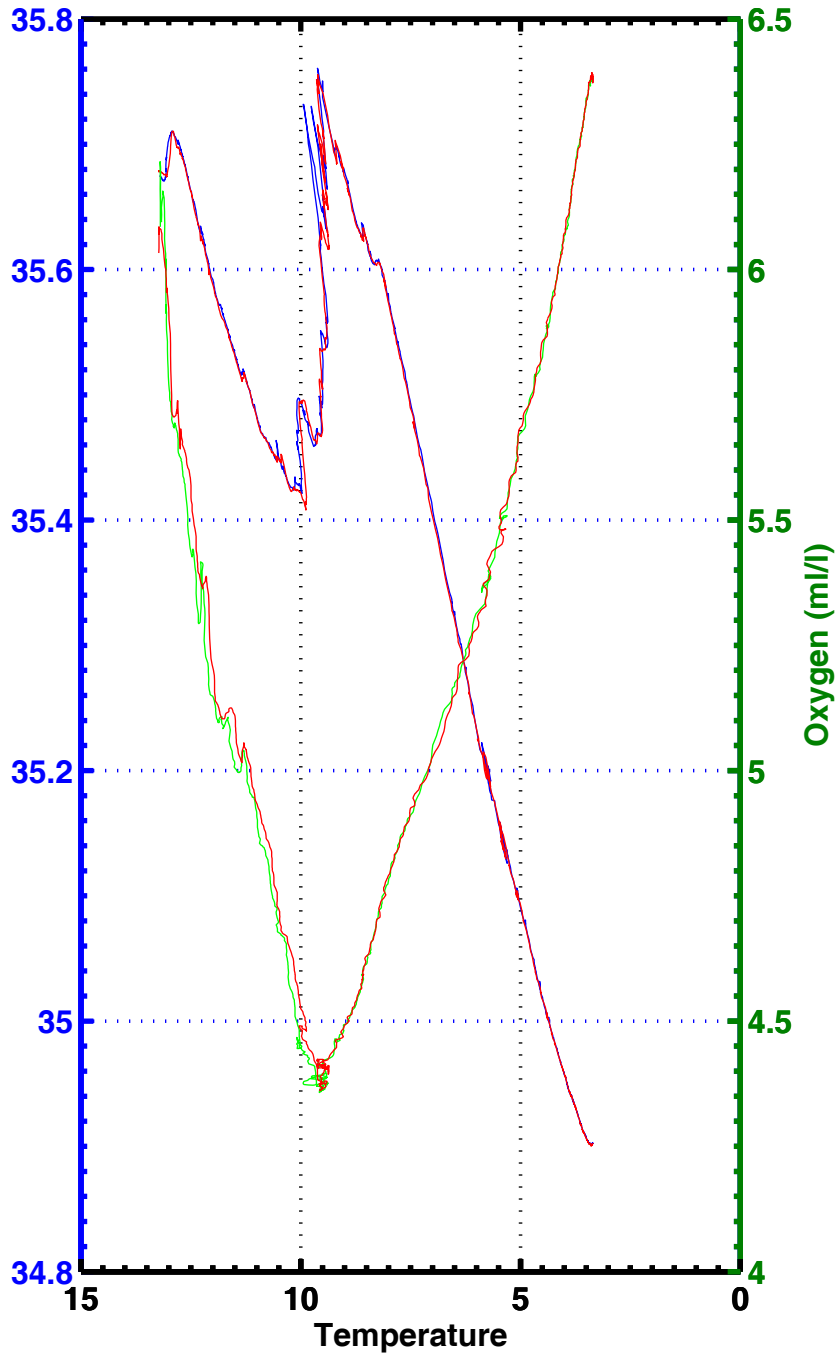
T-S , T-02 , station 2047
