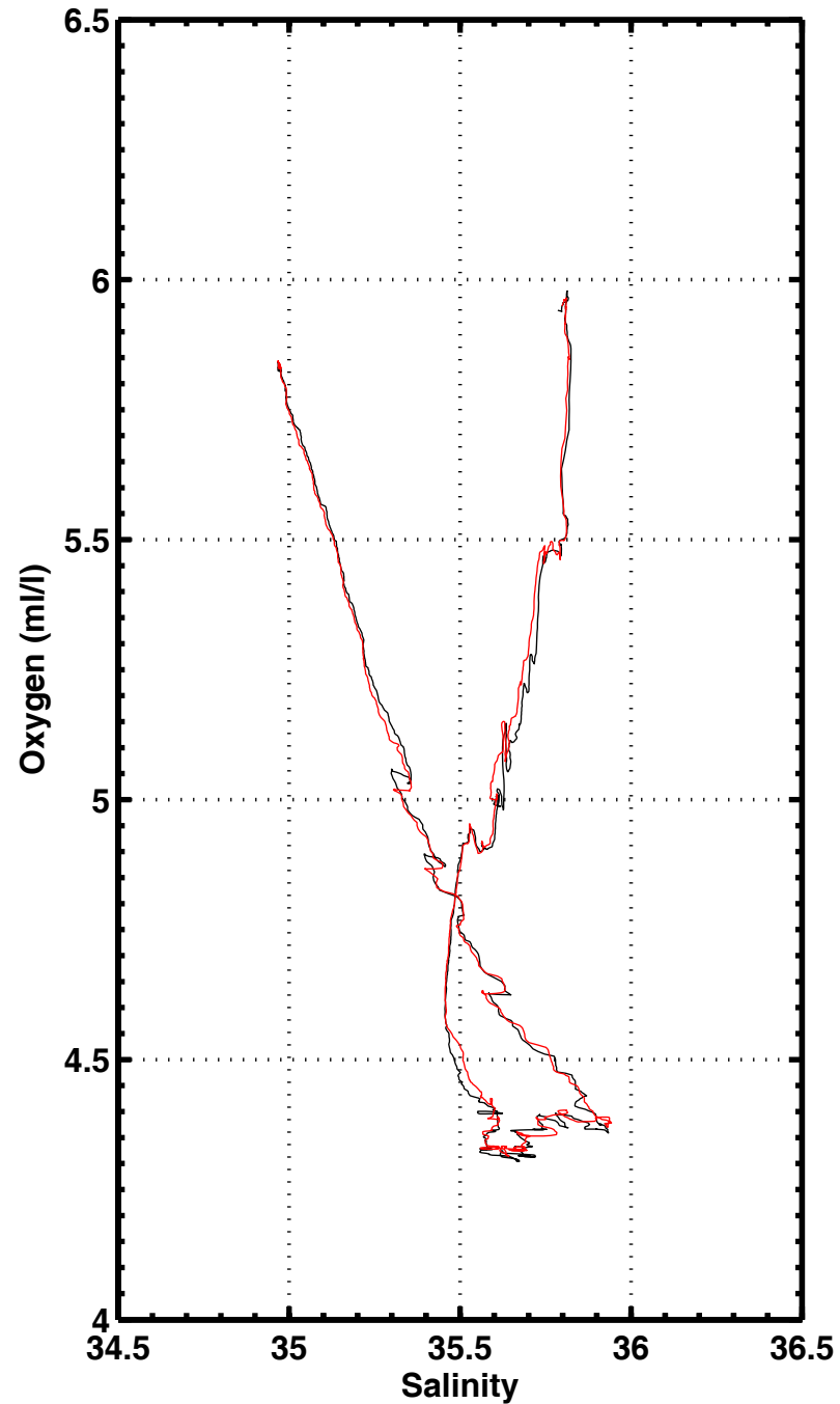
S-O2 , station 2278
