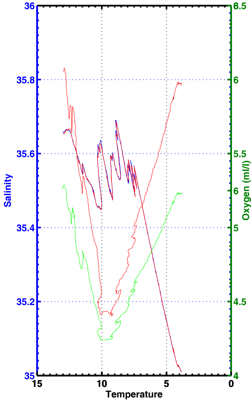
T-S , T-02 , station 2008
