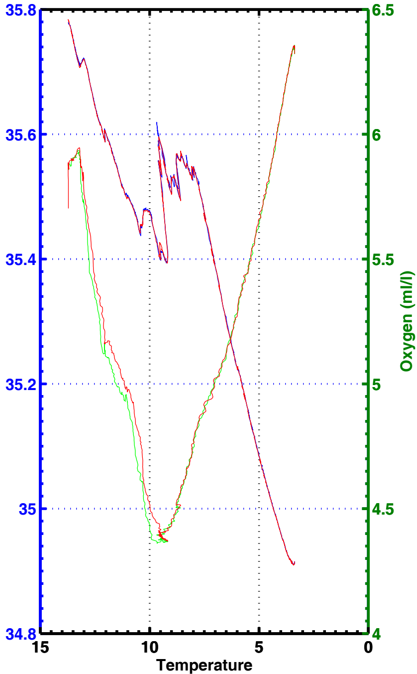
T-S , T-02 , station 2052
