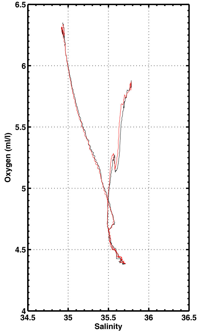
S-O2 , station 2023
