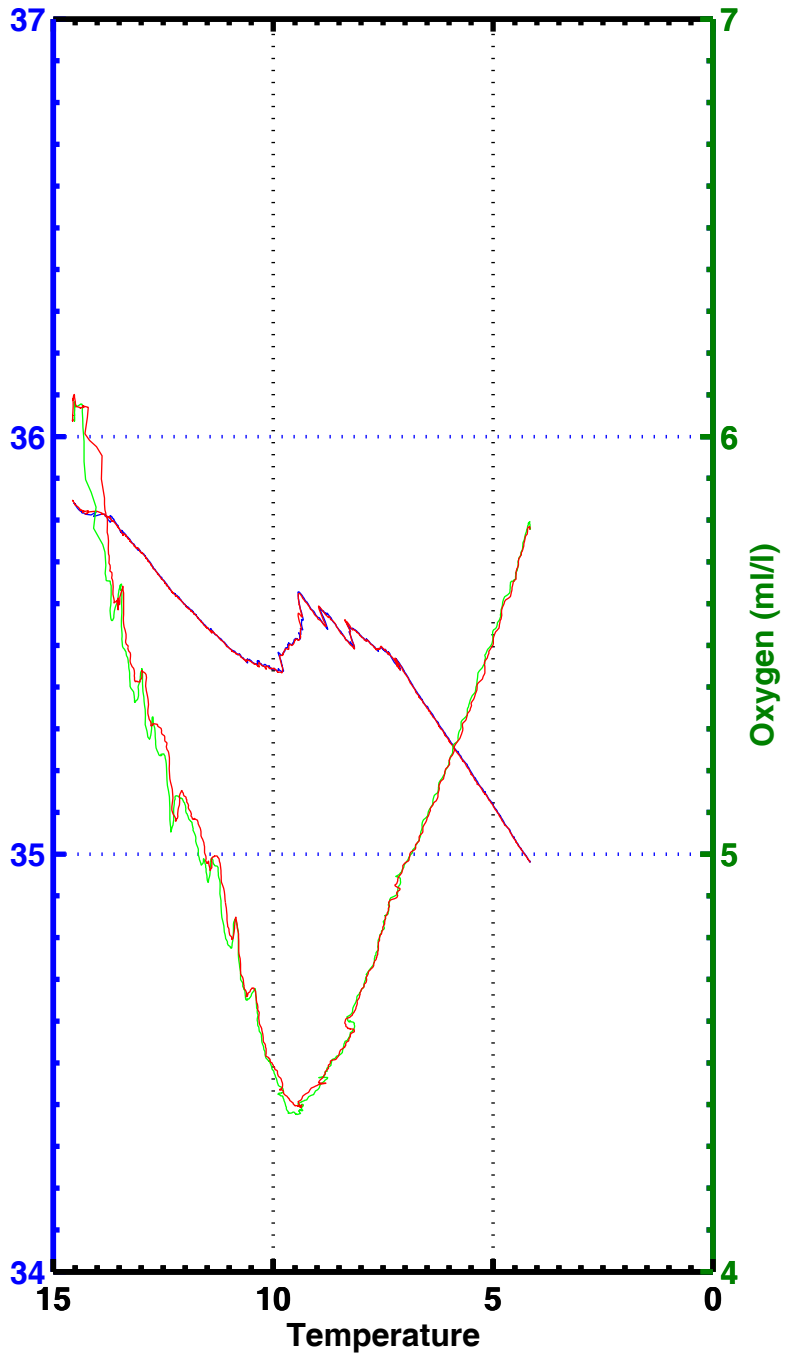
T-S , T-02 , station 2170
