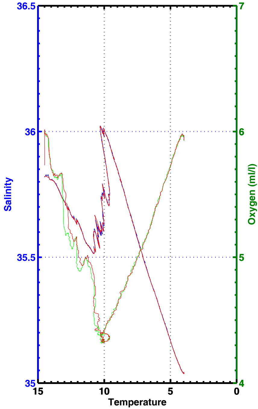
T-S , T-02 , station 2035
