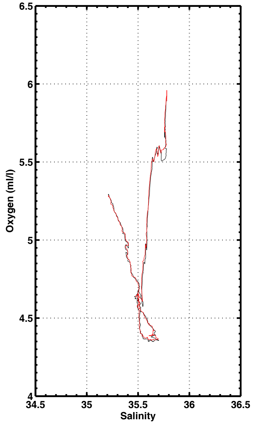
S-02 , station 2404
