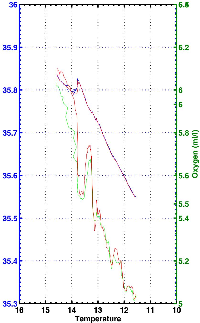
T-S , T-02 , station 2176
