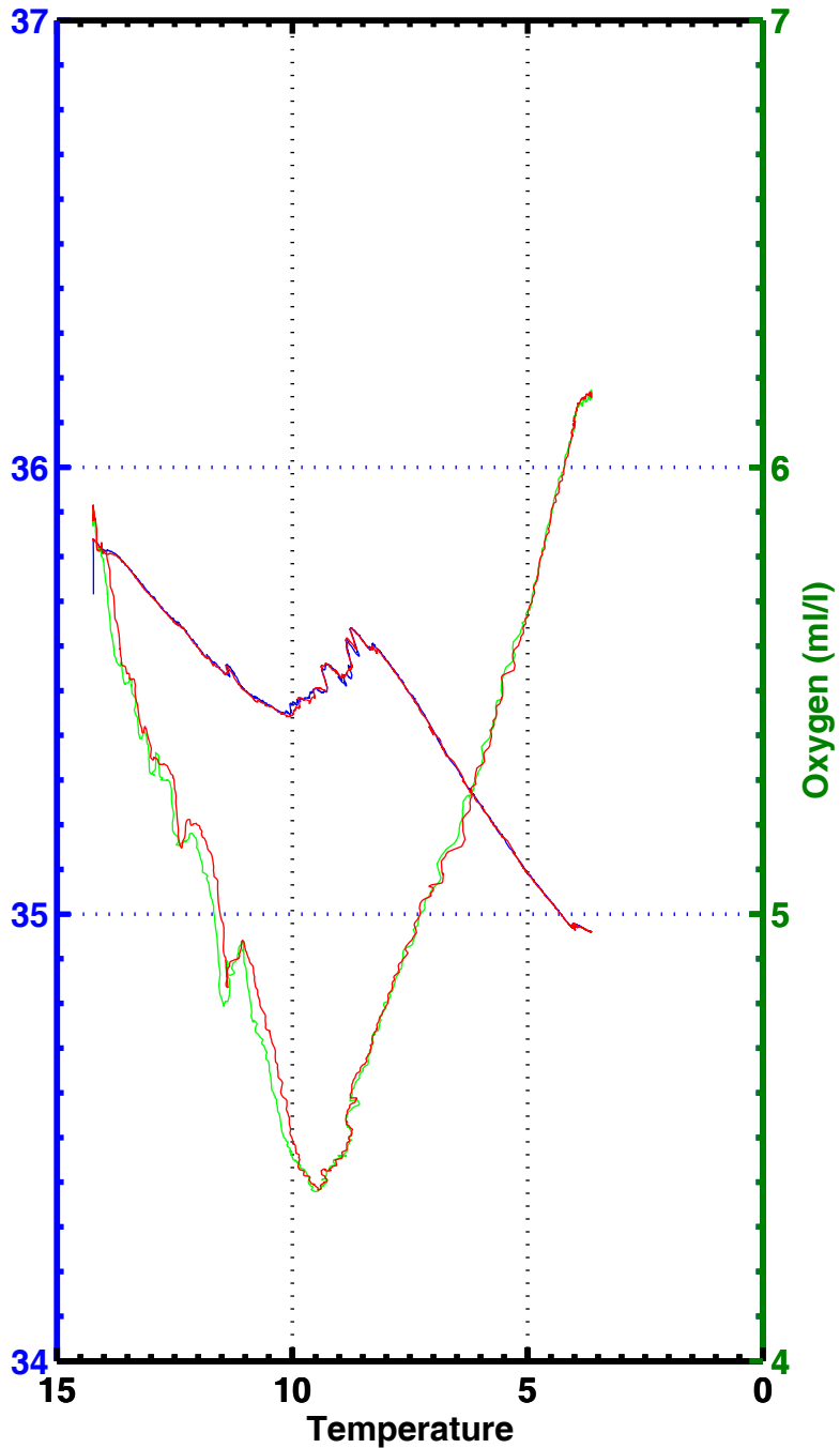
T-S , T-02 , station 2058
