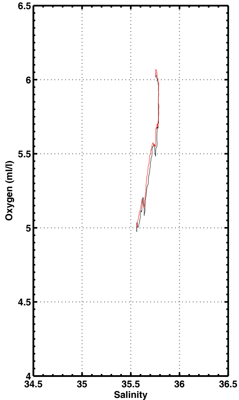
S-O2 , station 2179
