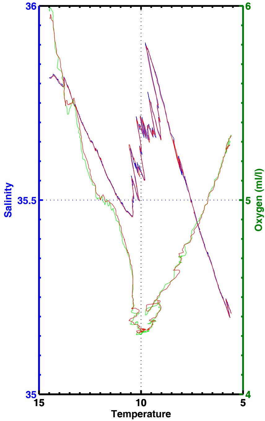
T-S , T-02 , station 2269
