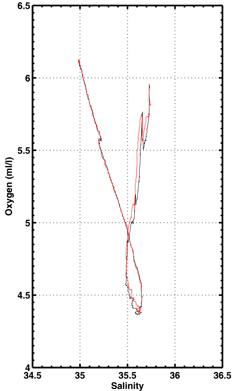
S-O2 , station 2016
