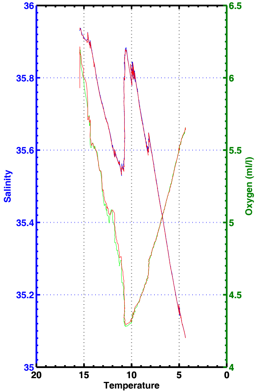
T-S , T-02 , station 2095
