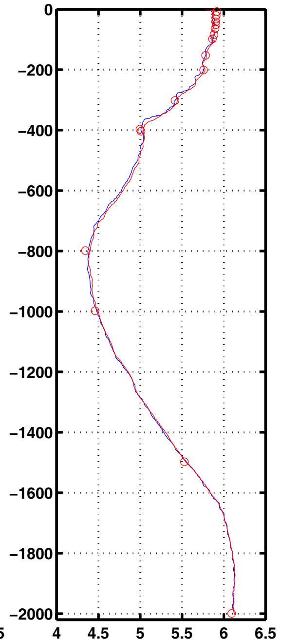
Oxyg 2020
