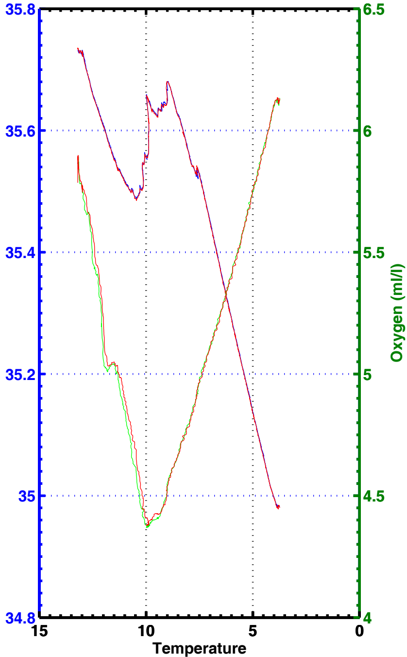
T-S , T-02 , station 2020
