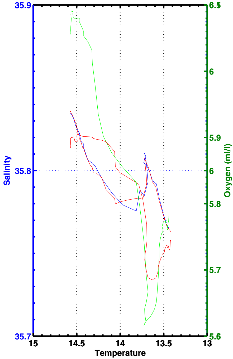
T-S , T-02 , station 2173
