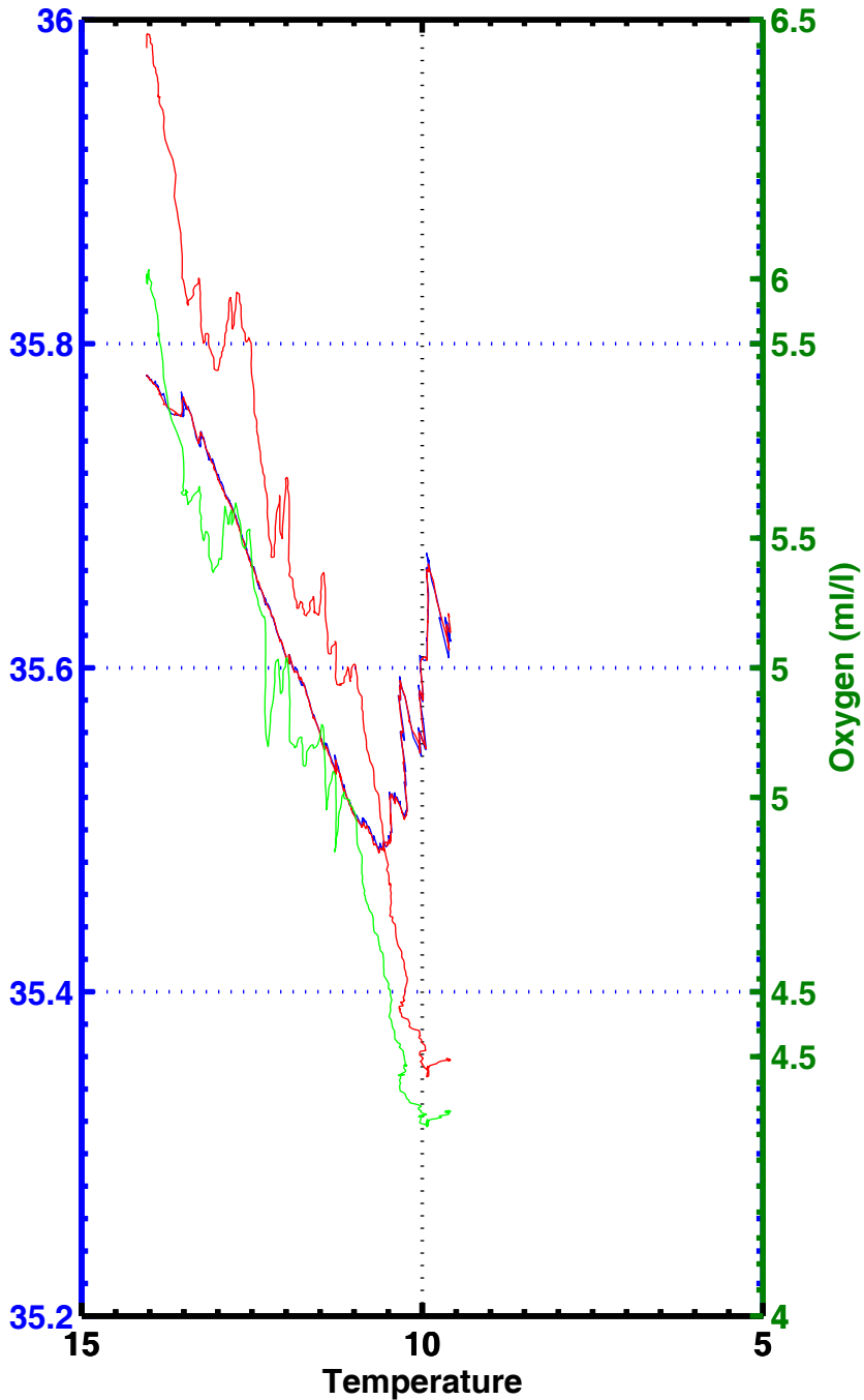
T-S , T-02 , station 2407
