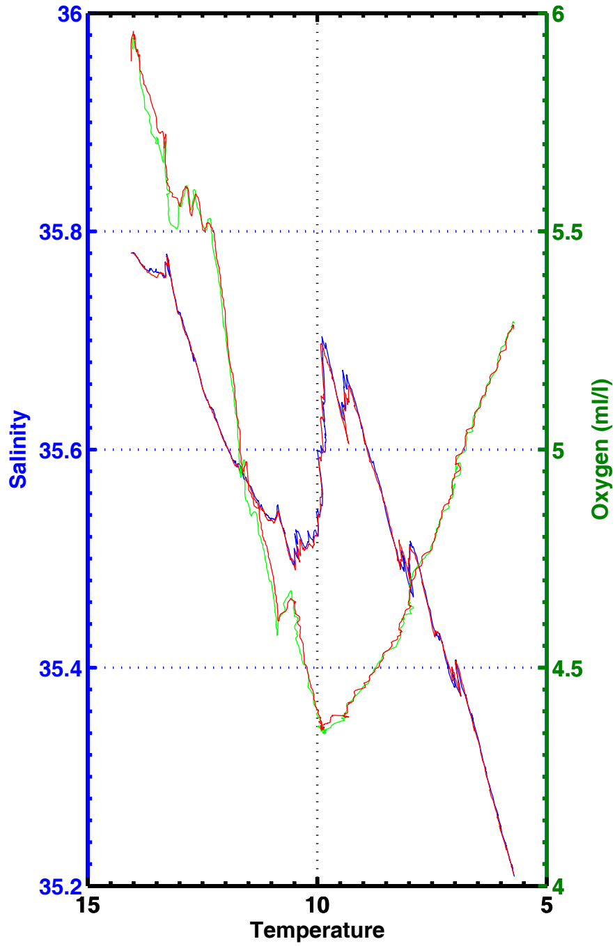
T-S , T-02 , station 2404
