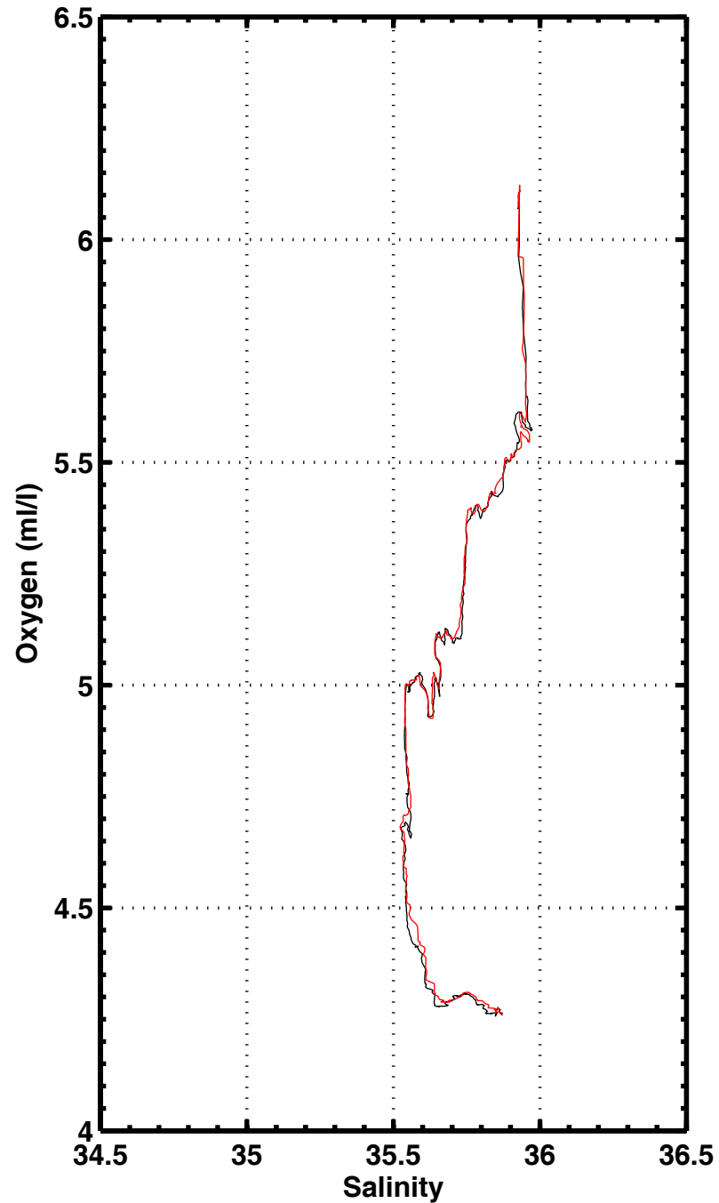
S-O2 , station 2086
