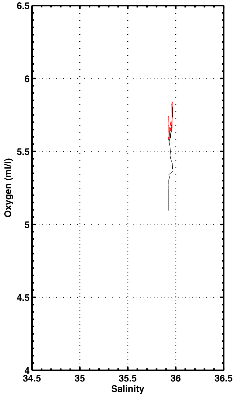
S-O2 , station 2090
