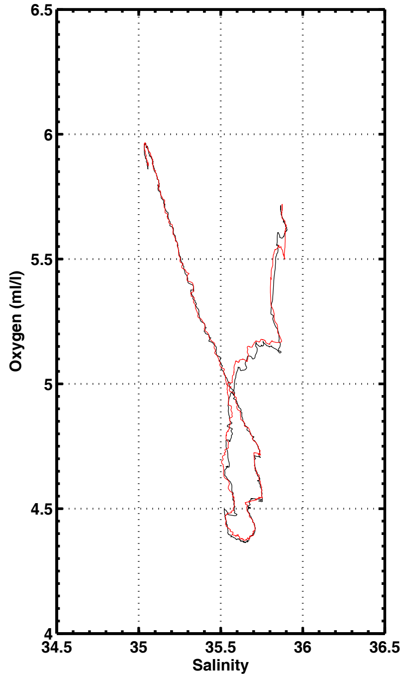
S-O2 , station 2002
