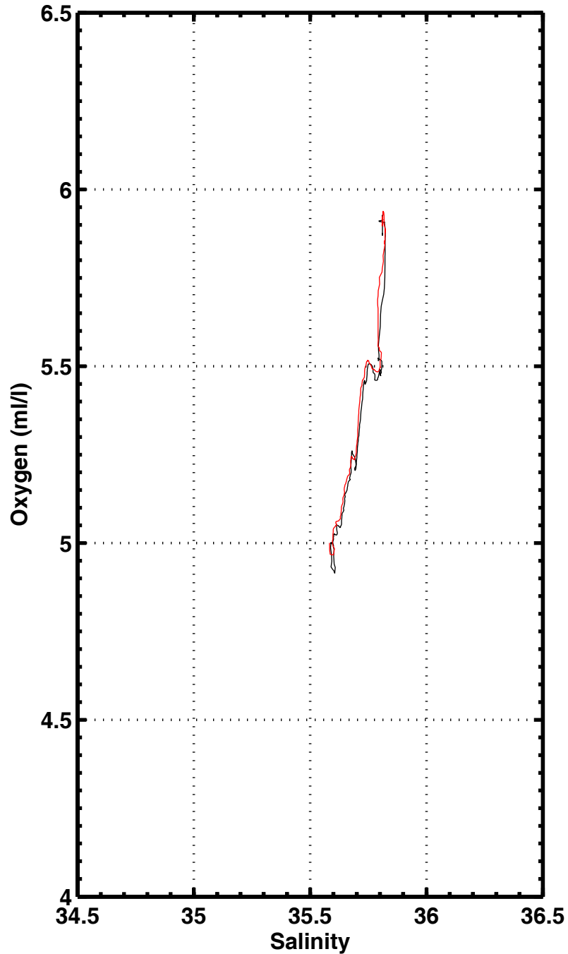
S-O2 , station 2273
