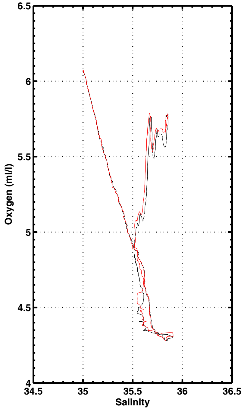
S-02 , station 2005
