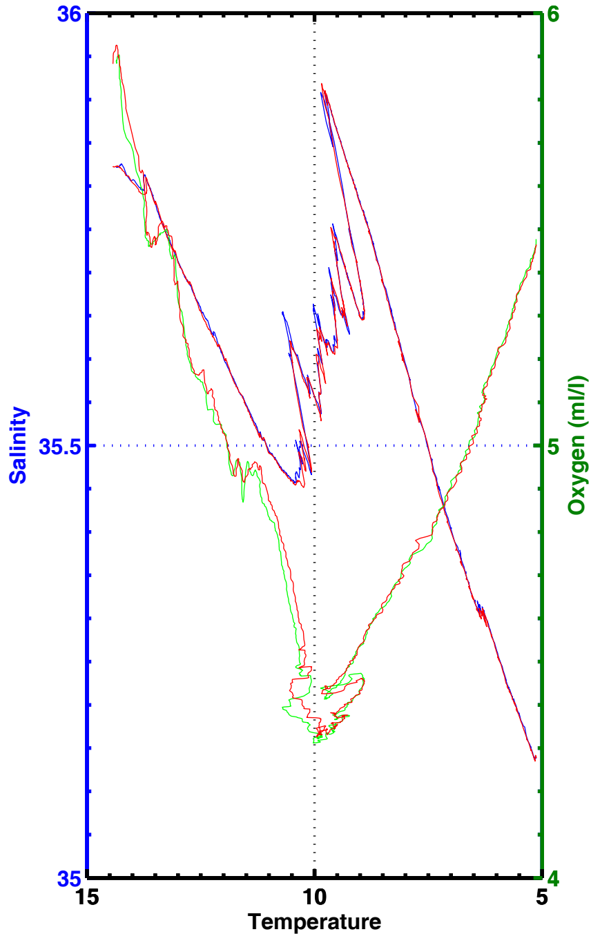
T-S , T-02 , station 2267
