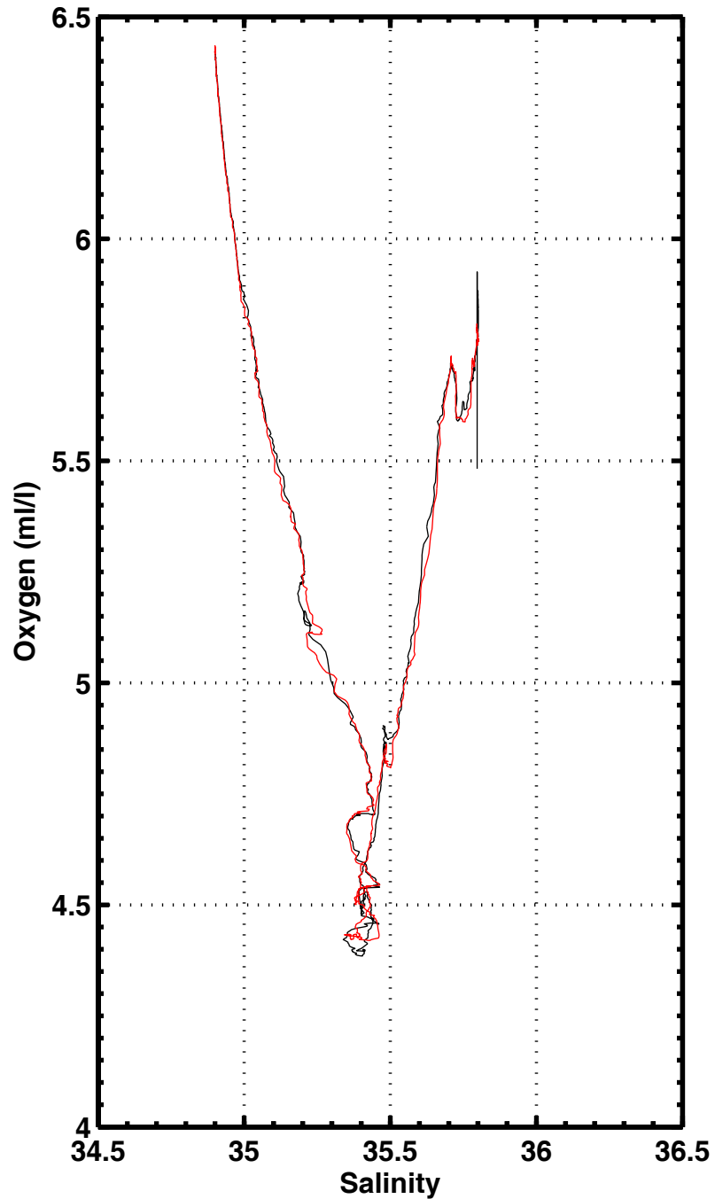
S-02 , station 2018
