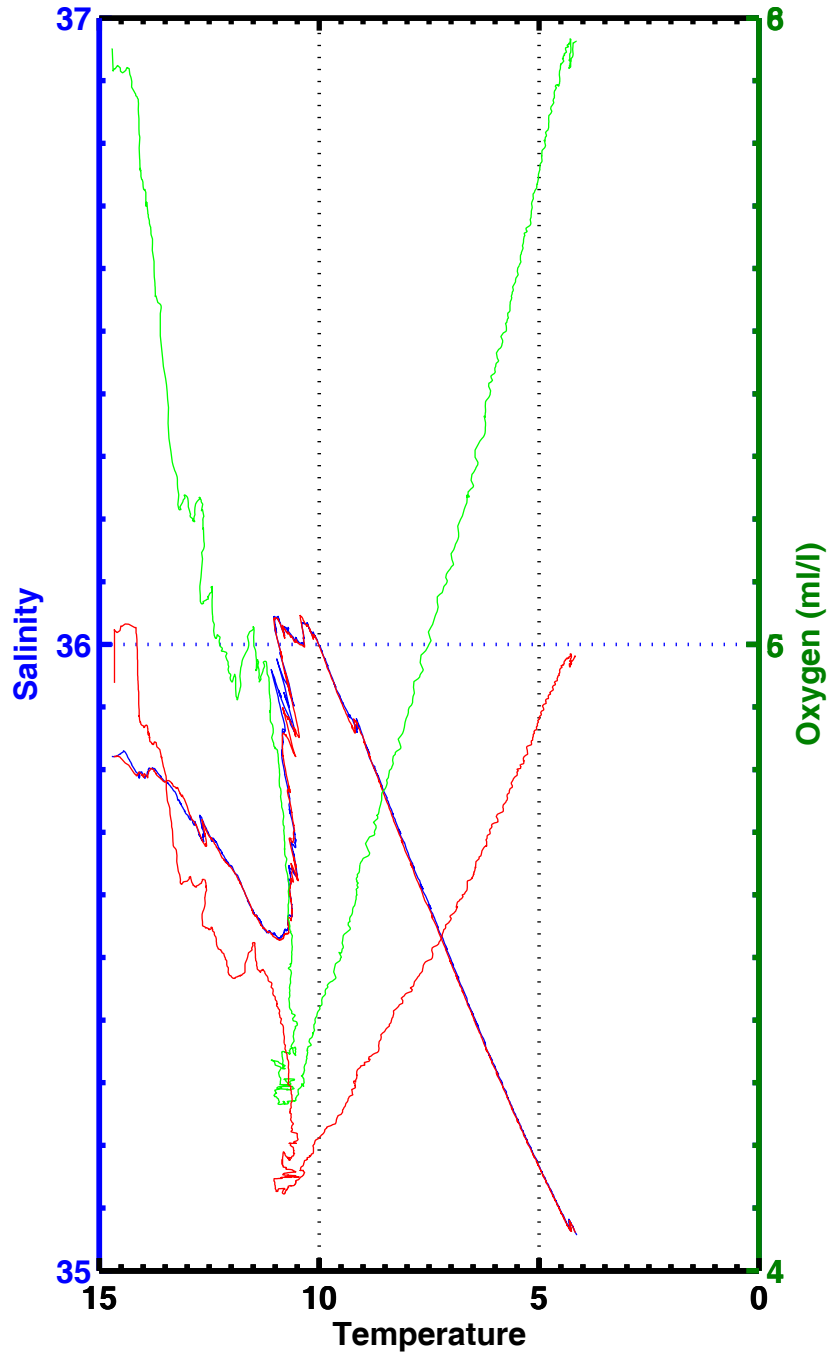
T-S , T-02 , station 2031
