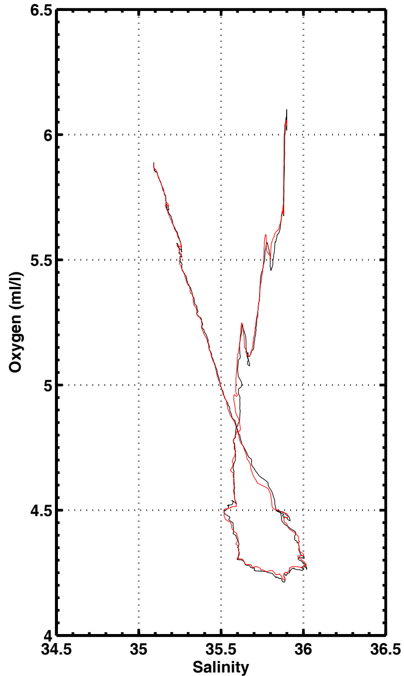
S-O2 , station 2077
