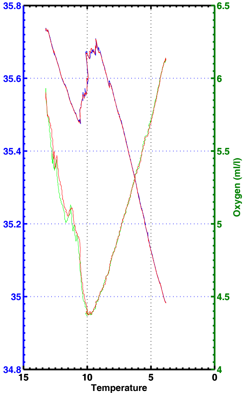
T-S , T-02 , station 2015
