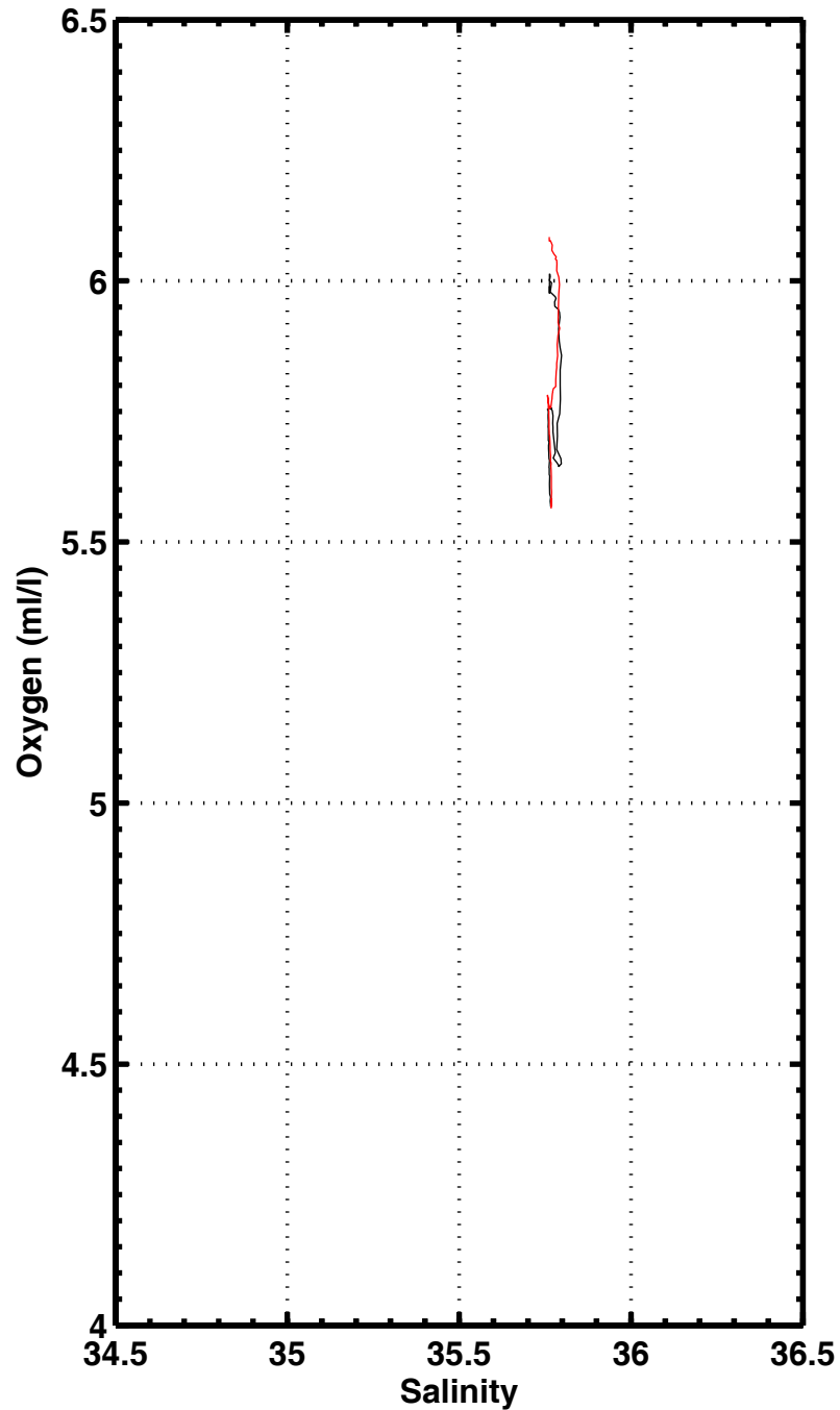
S-02 , station 2177
