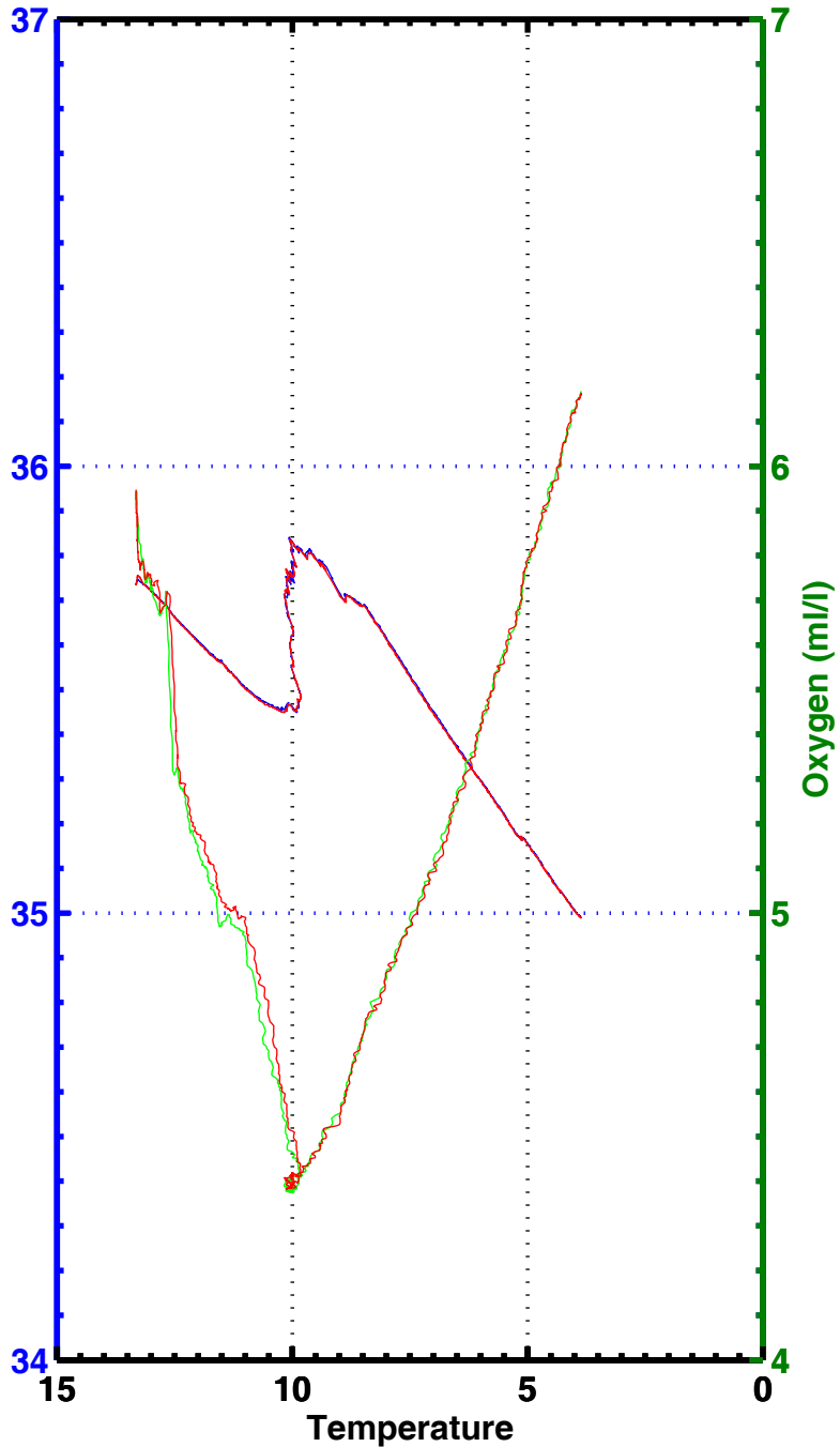
T-S , T-02 , station 2022
