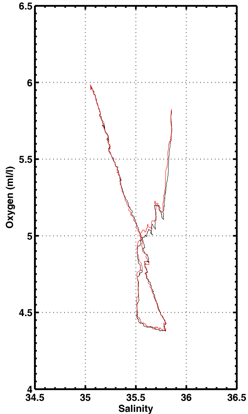
S-O2 , station 2001
