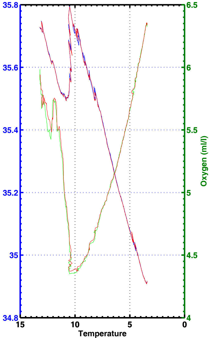
T-S , T-02 , station 2012
