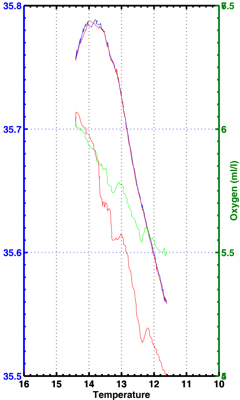
T-S , T-02 , station 2179
