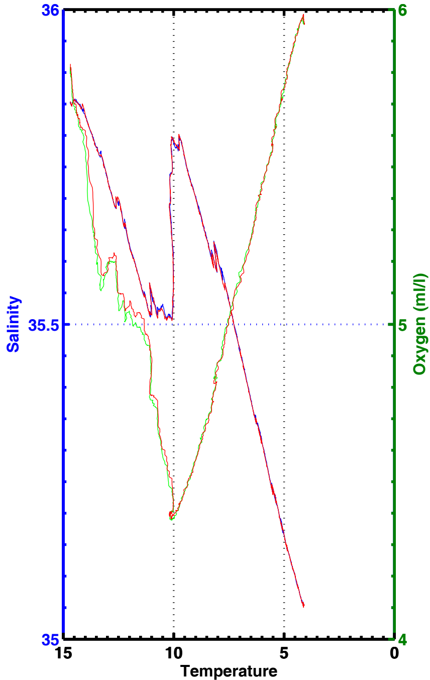
T-S , T-02 , station 2001
