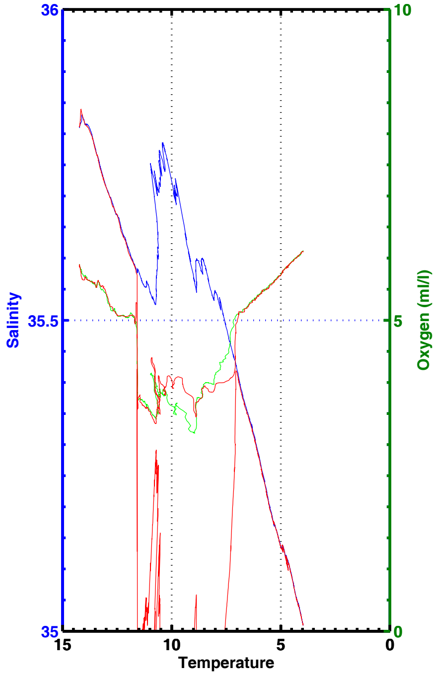
T-S , T-02 , station 2029
