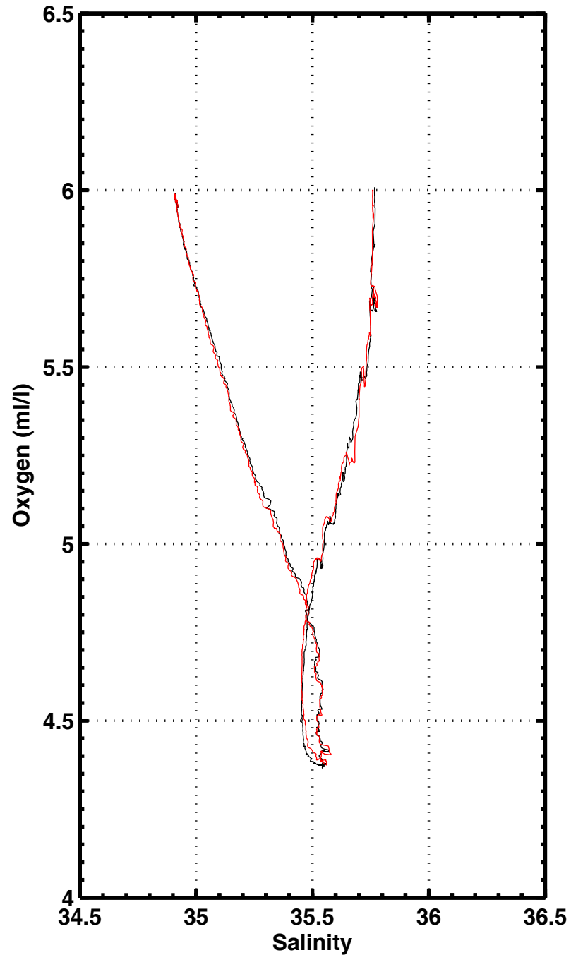
S-O2 , station 2184
