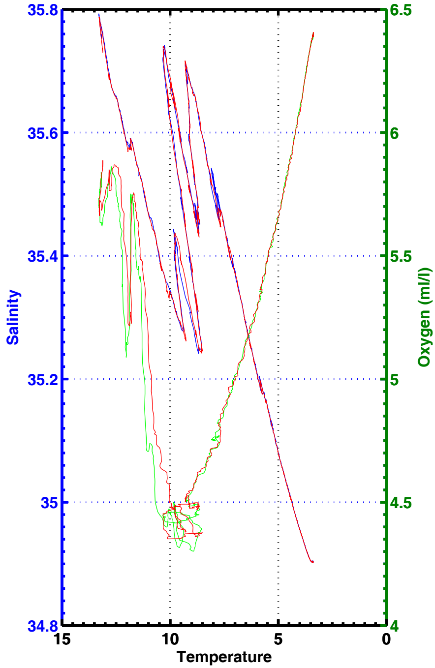
T-S , T-02 , station 2013
