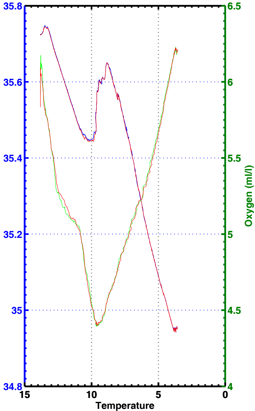
T-S , T-02 , station 2057
