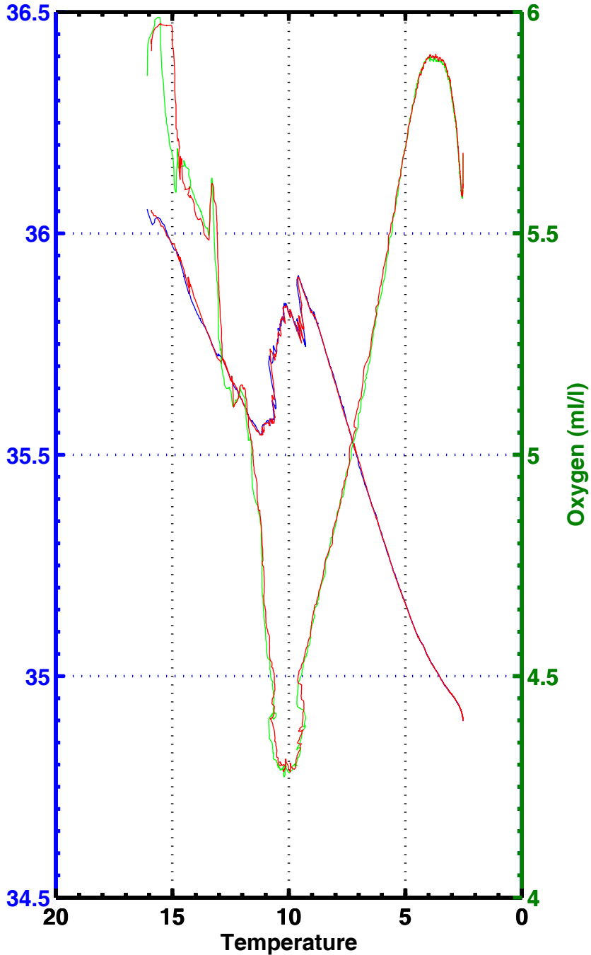
T-S , T-02 , station 2081
