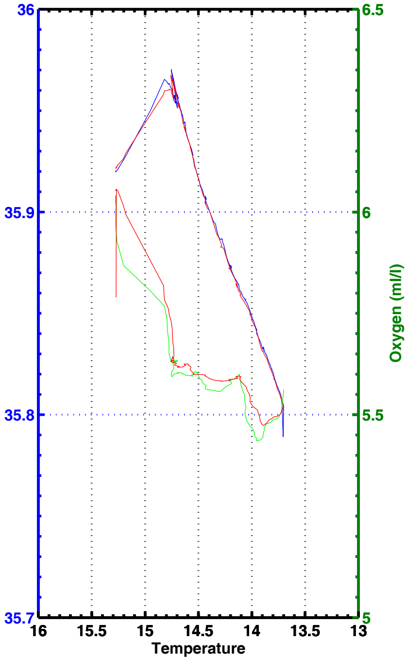
T-S , T-02 , station 2093
