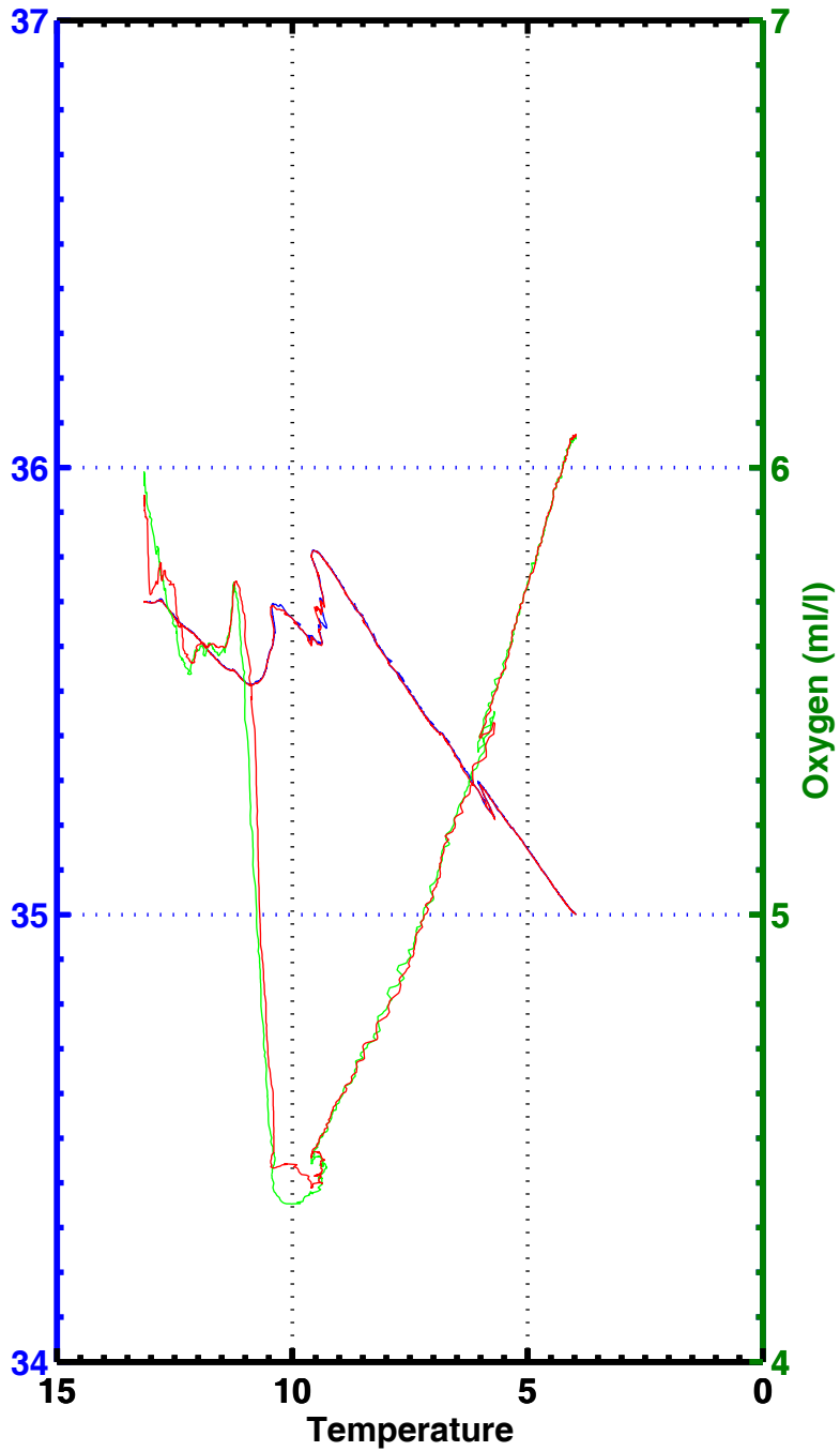
T-S , T-02 , station 2041
