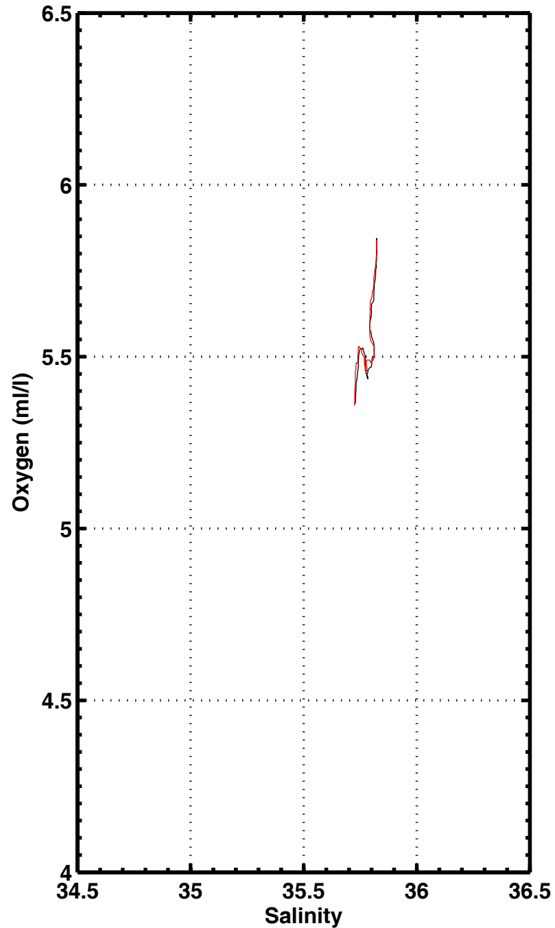
S-O2 , station 2265
