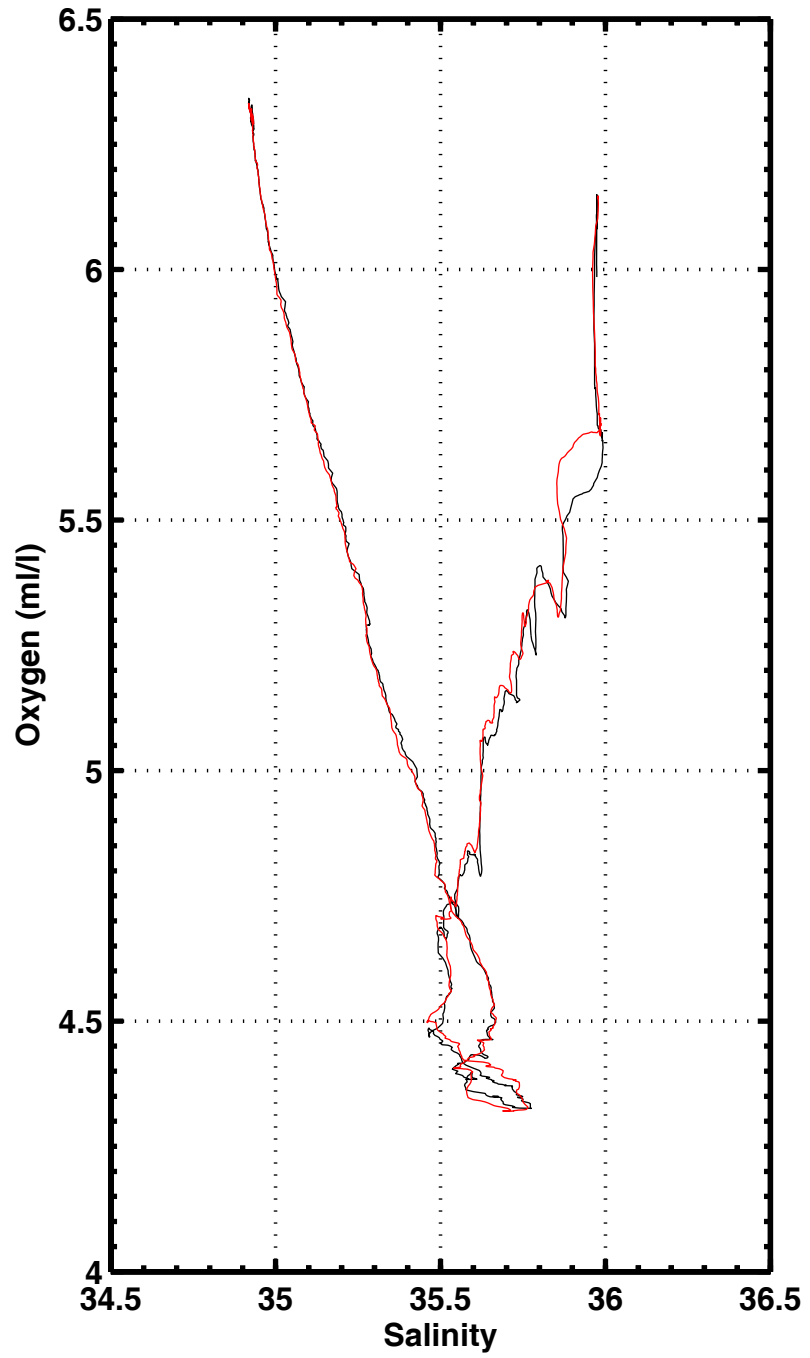
S-O2, station 2067
