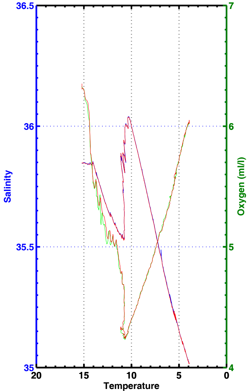
T-S , T-02 , station 2075
