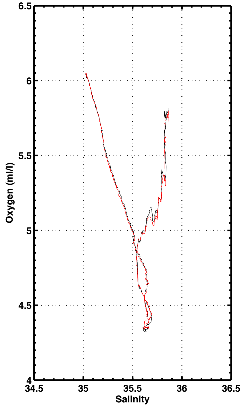
S-O2 , station 2036
