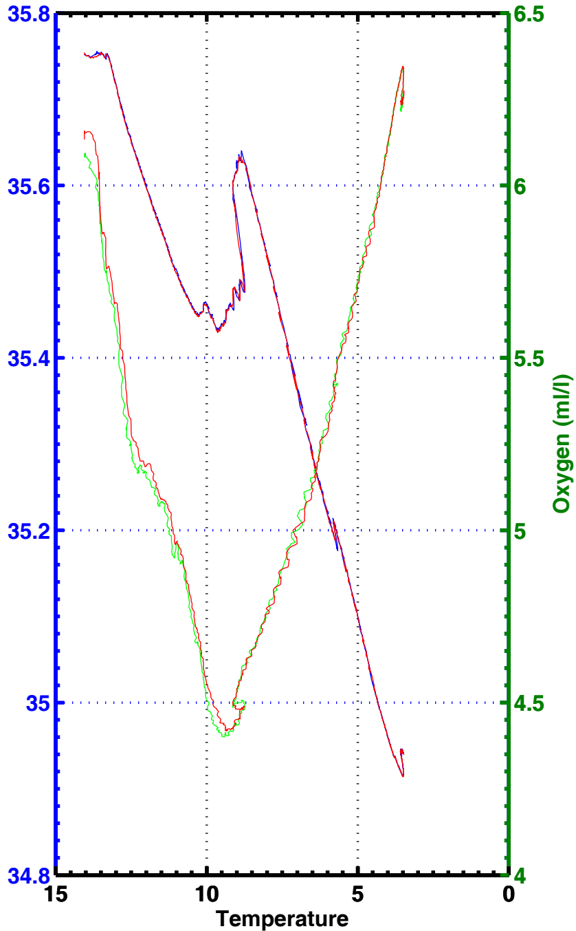
T-S , T-02 , station 2063
