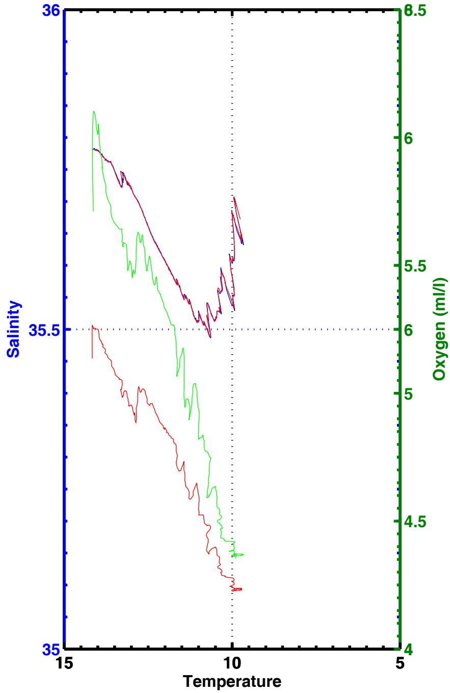
T-S , T-02 , station 2405
