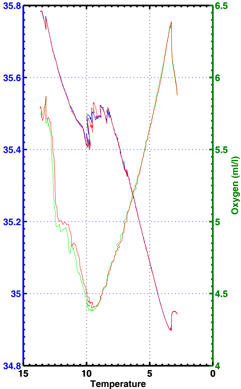
T-S , T-02 , station 2046
