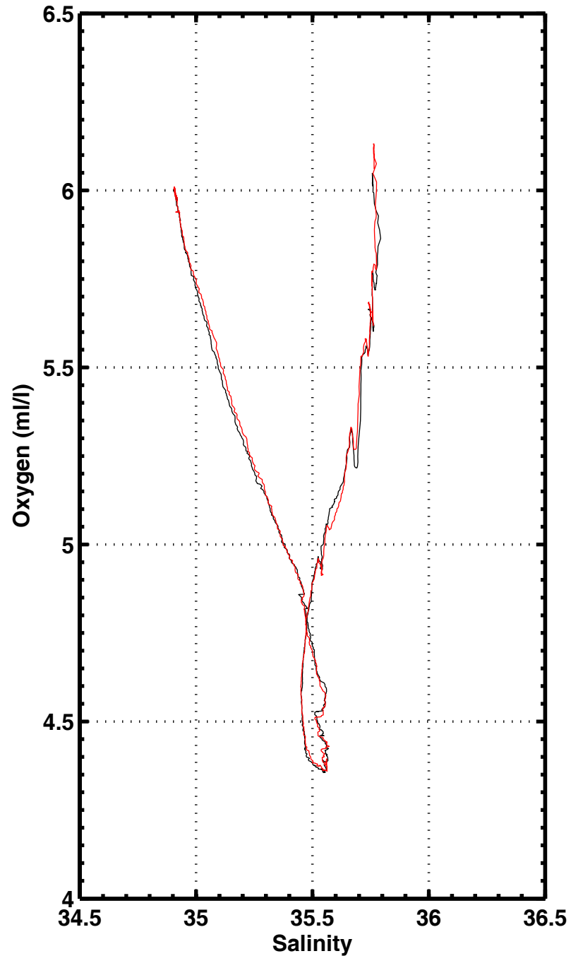
S-O2 , station 2183
