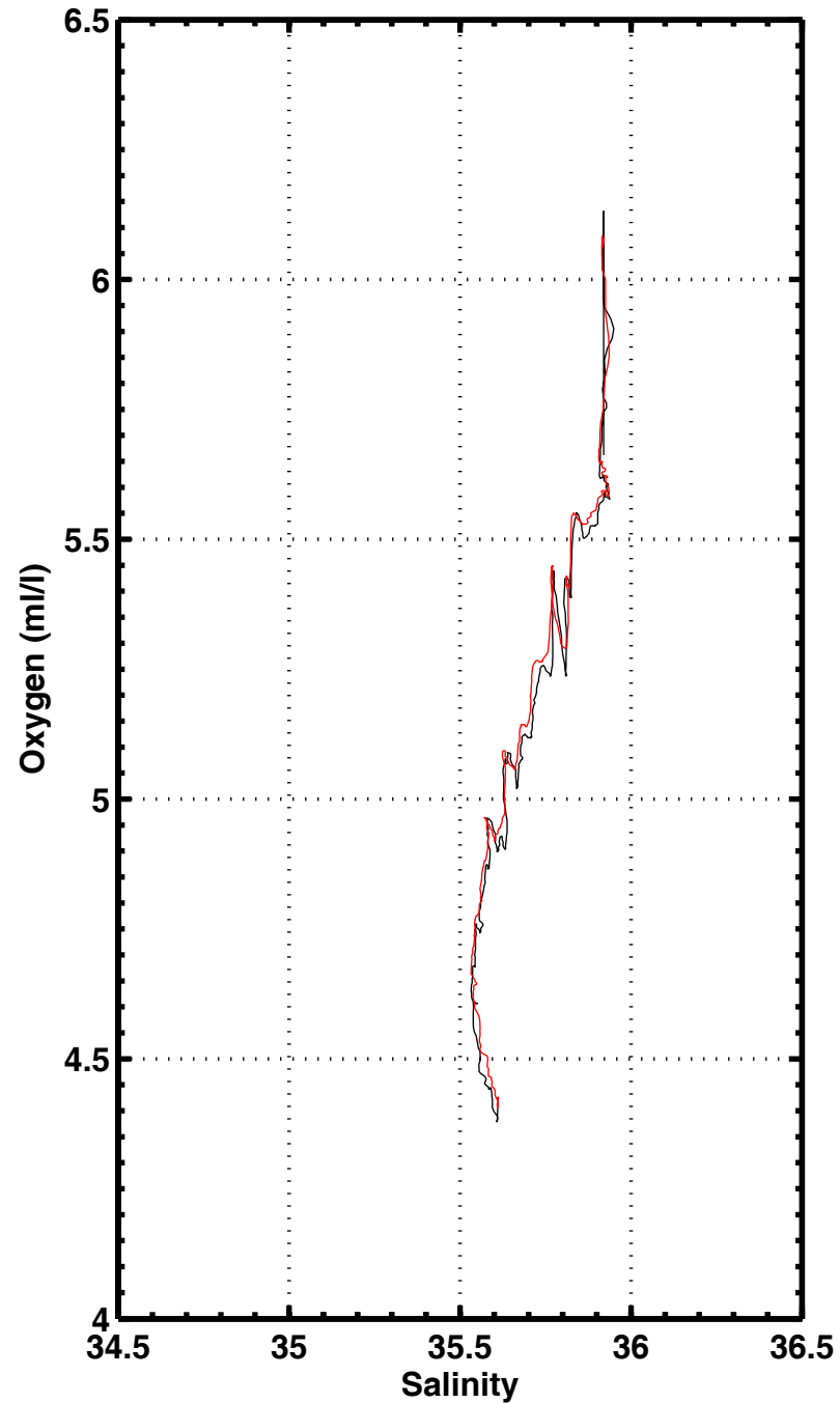
S-O2 , station 2092
