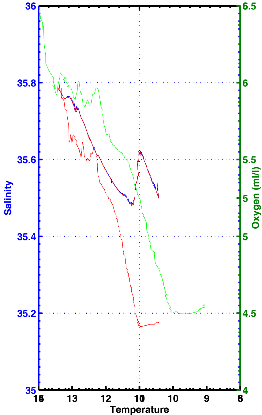
T-S , T-02 , station 2413
