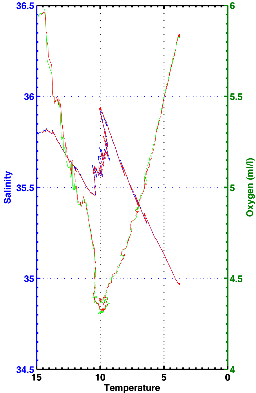
T-S , T-02 , station 2278
