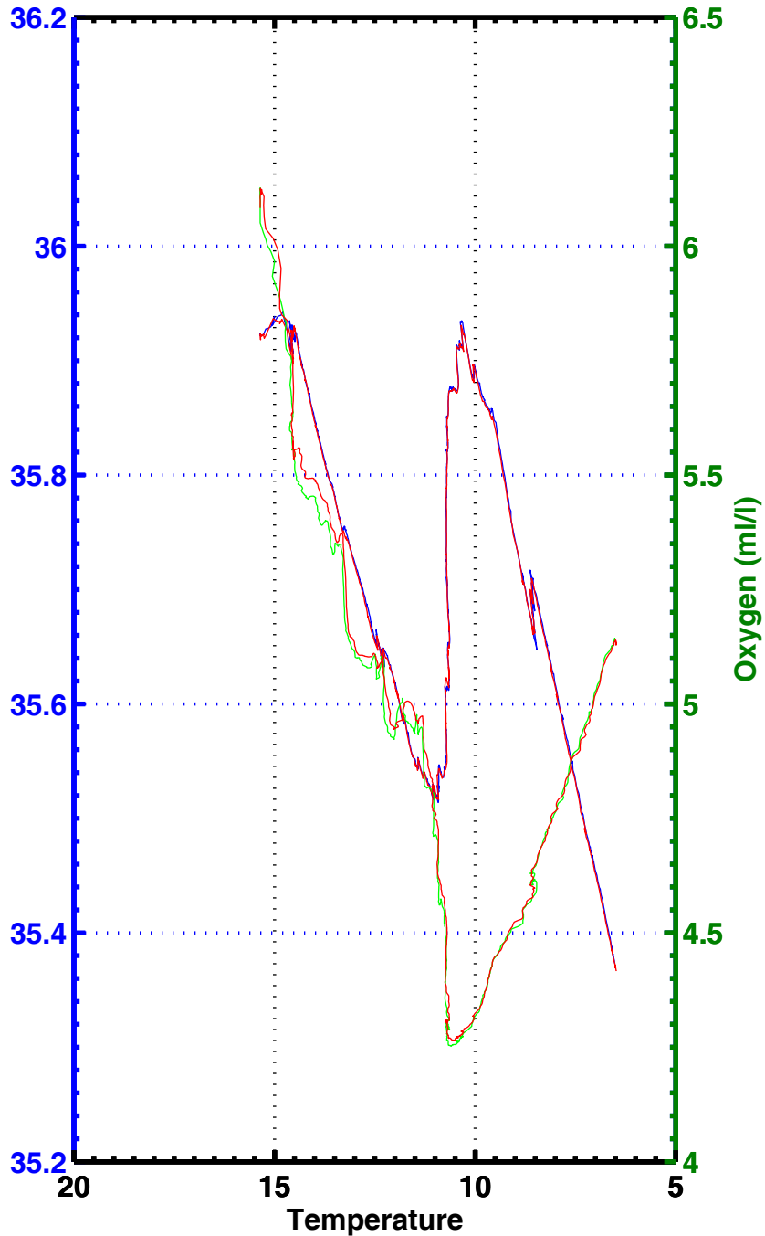
T-S , T-02 , station 2085
