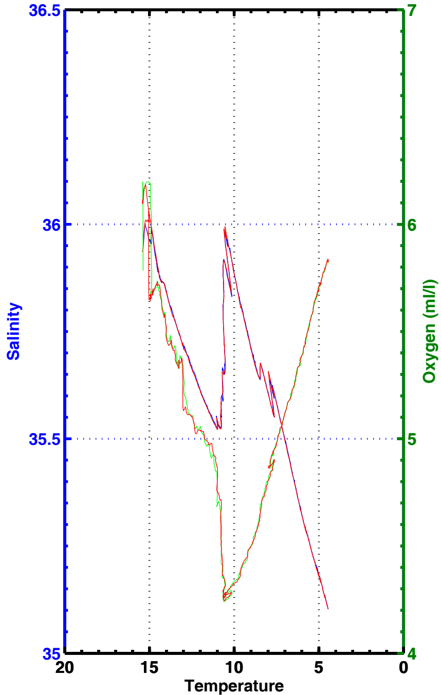
T-S , T-02 , station 2078
