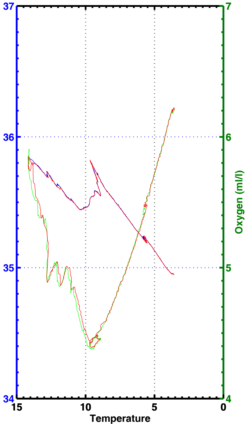
T-S , T-02 , station 2049
