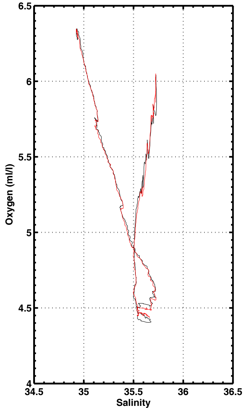
S-O2 , station 2026
