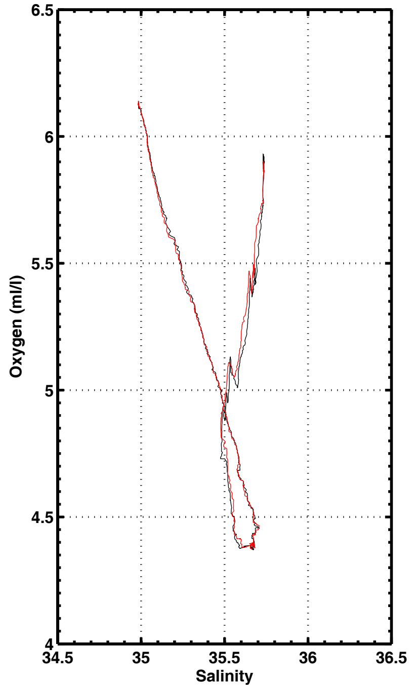
S-O2 , station 2015
