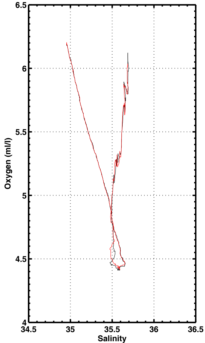
S-02 , station 2011
