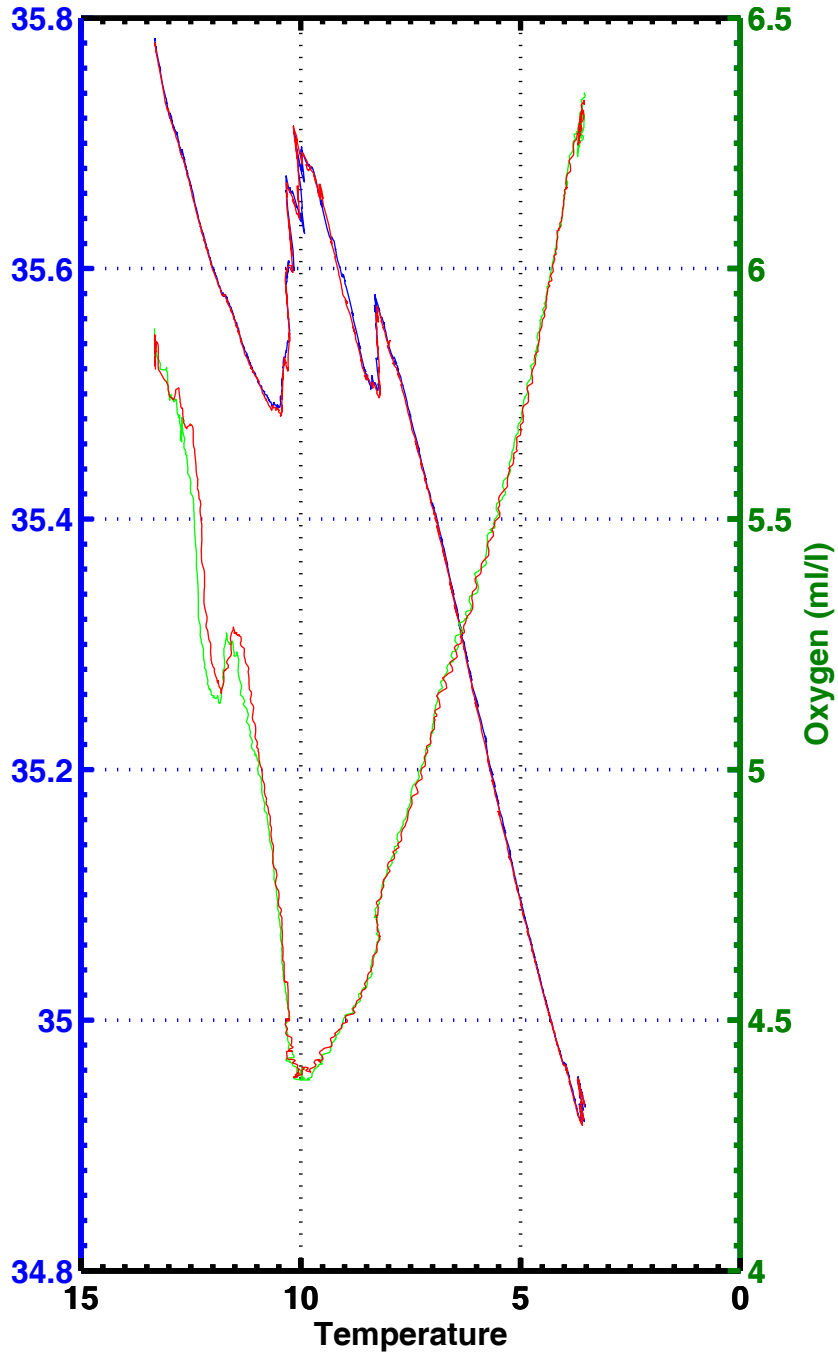
T-S , T-02 , station 2023
