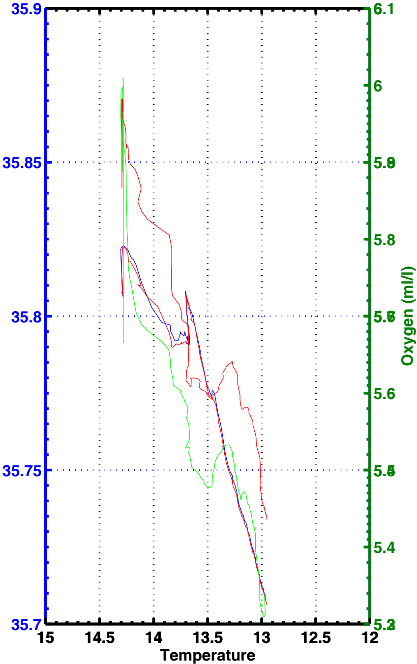
T-S , T-02 , station 2275
