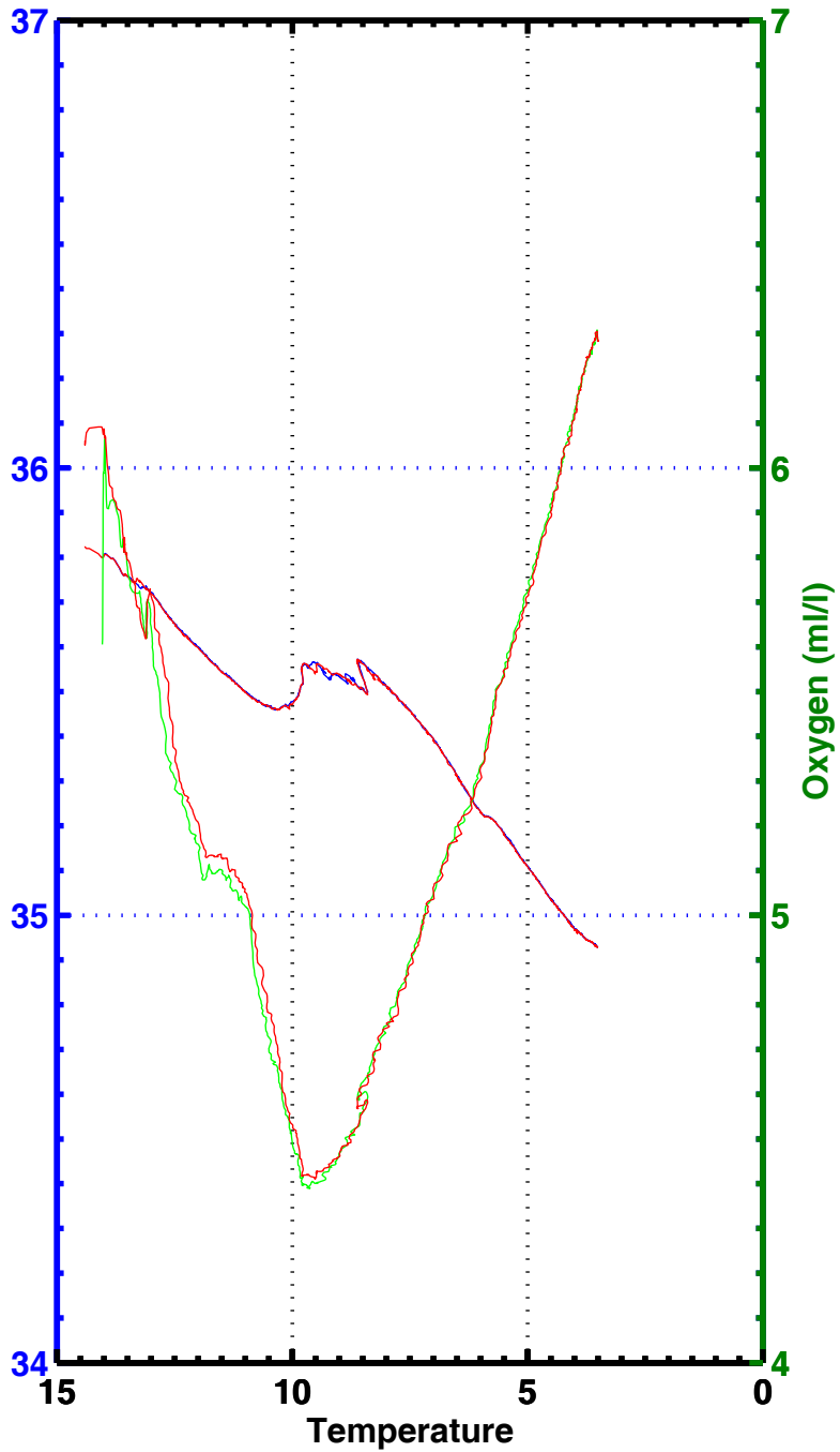
T-S , T-02 , station 2062
