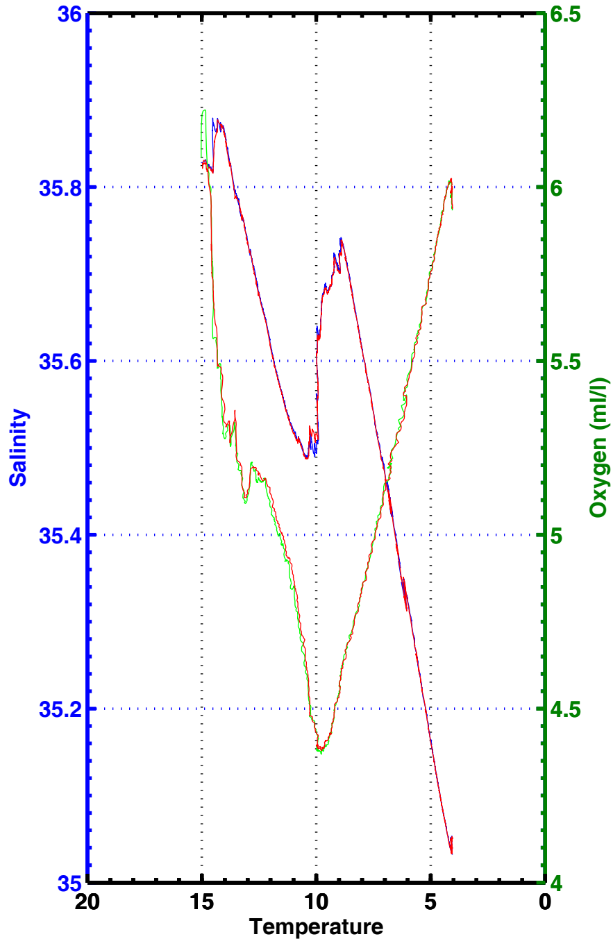
T-S , T-02 , station 2032
