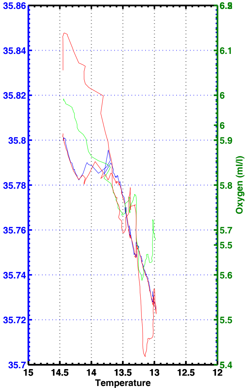
T-S , T-02 , station 2181
