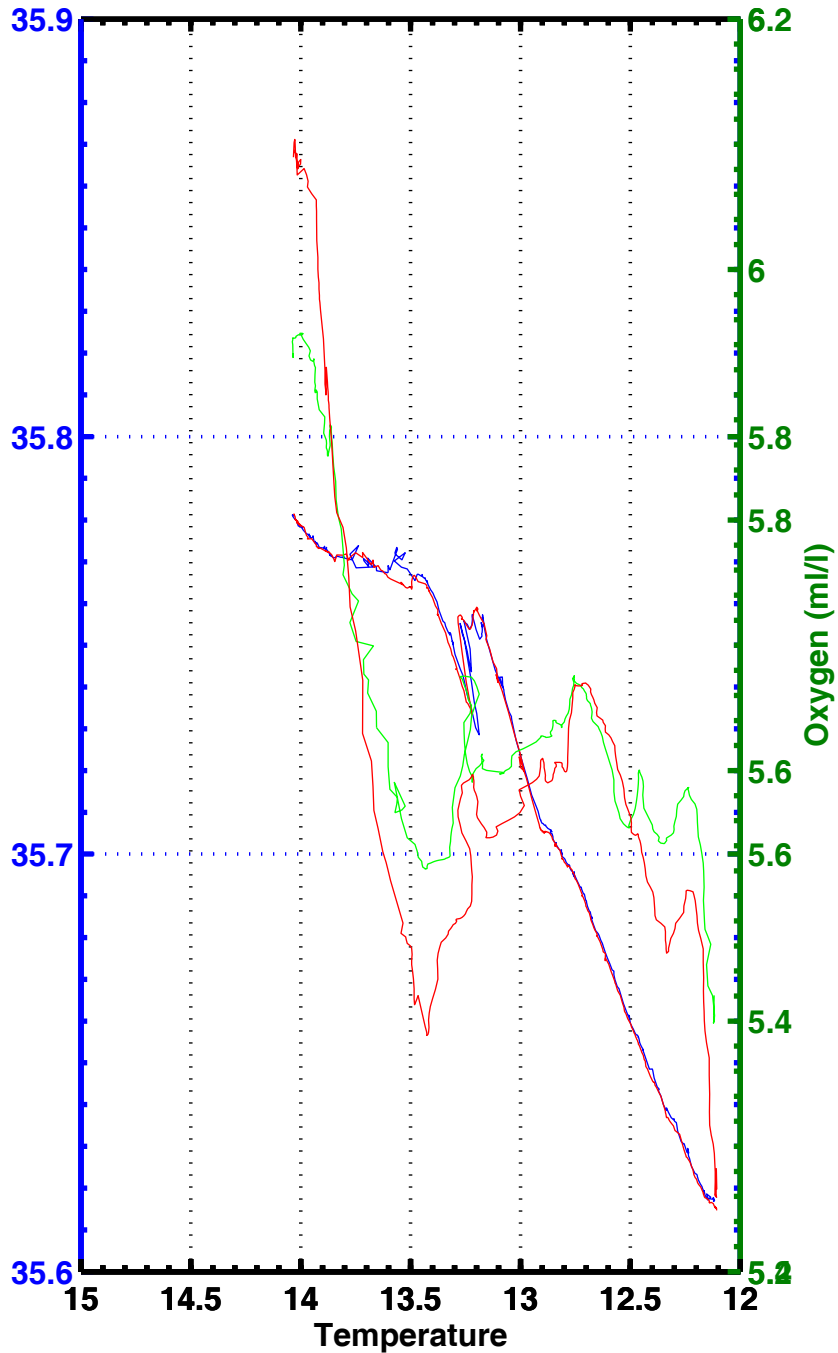
T-S , T-02 , station 2410
