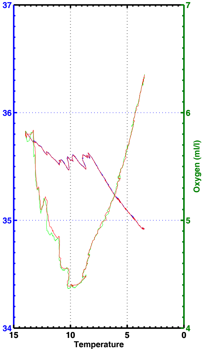
T-S , T-02 , station 2044
