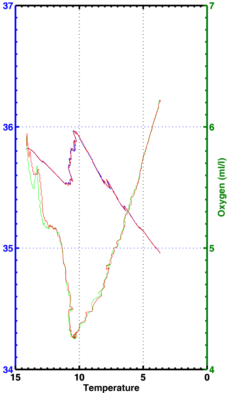
T-S , T-02 , station 2039
