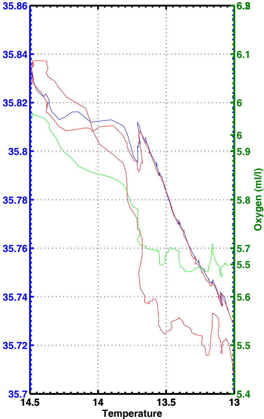
T-S , T-02 , station 2169
