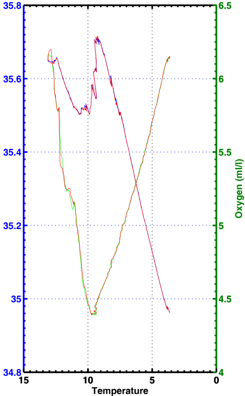
T-S , T-02 , station 2010
