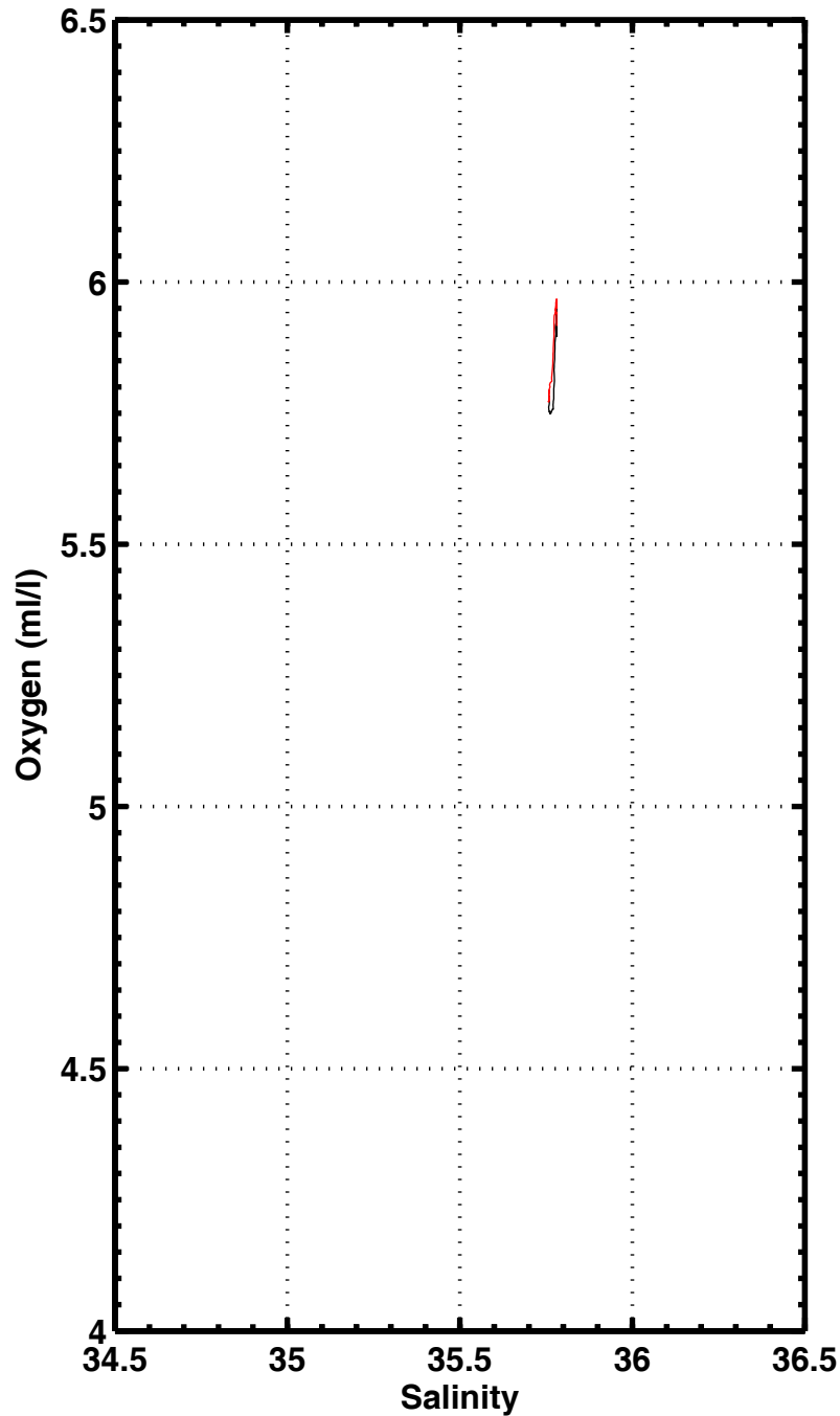
S-O2 , station 2415
