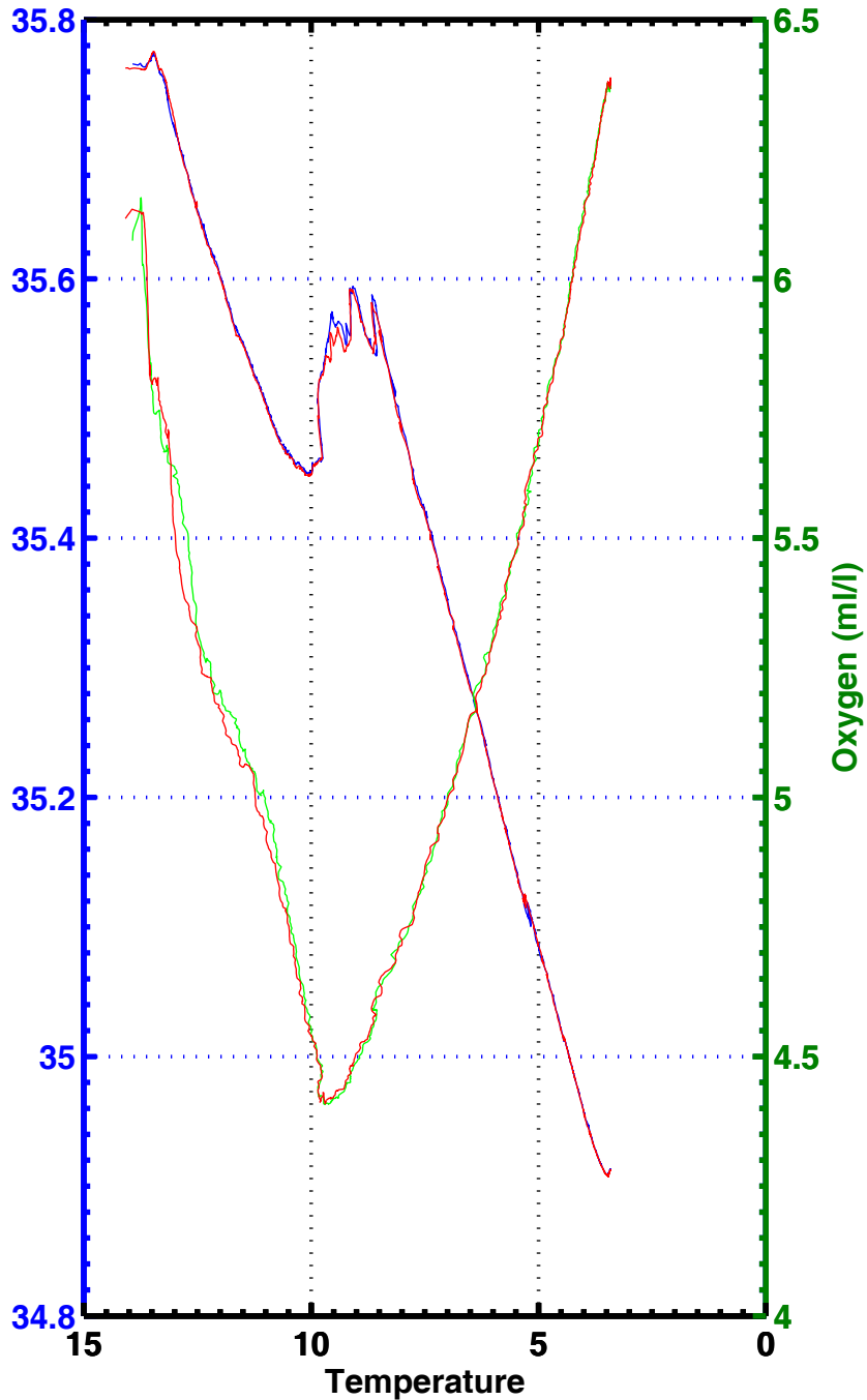
T-S , T-02 , station 2061
