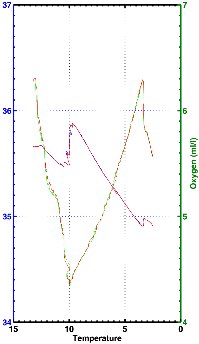
T-S , T-02 , station 2009
