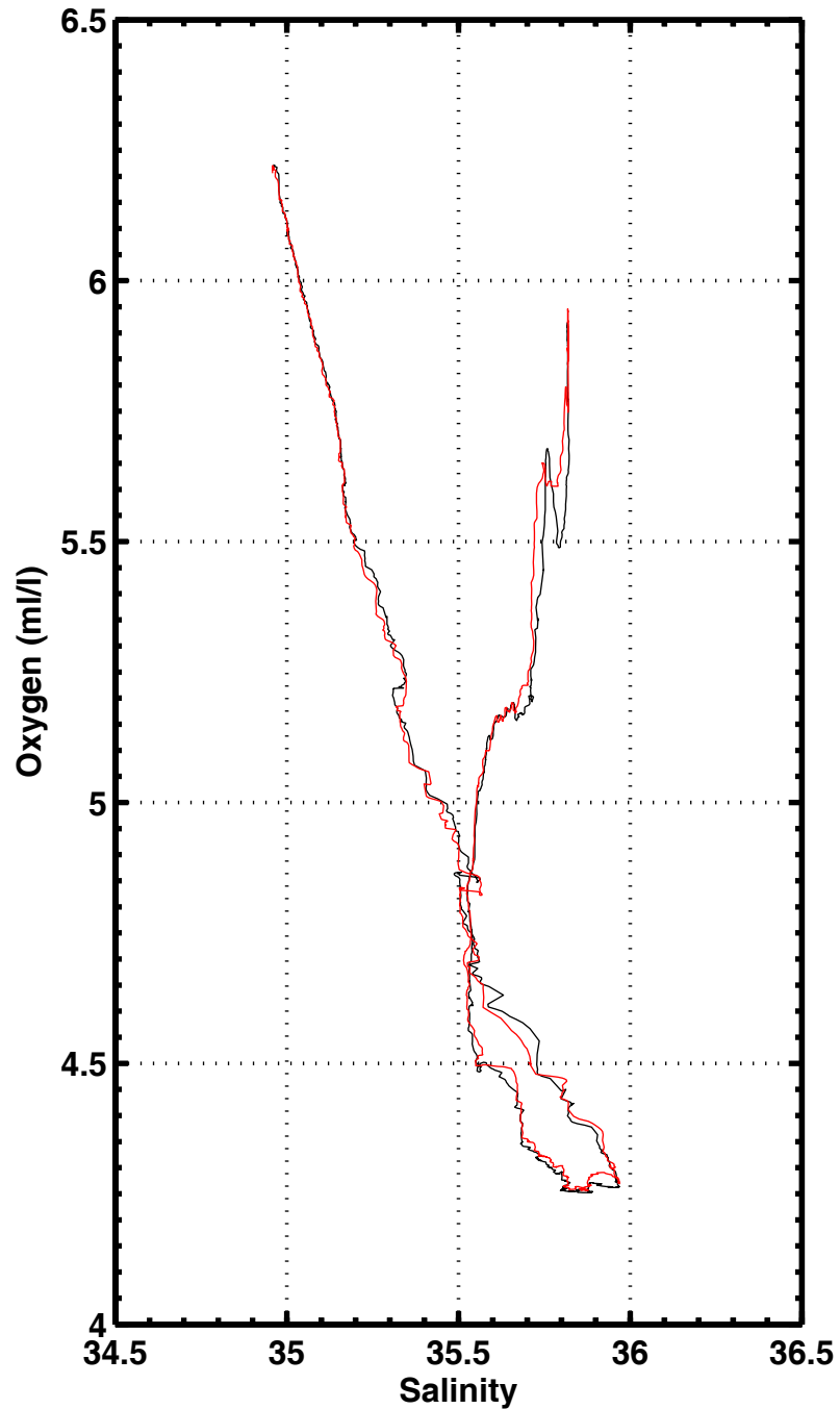
S-O2 , station 2039
