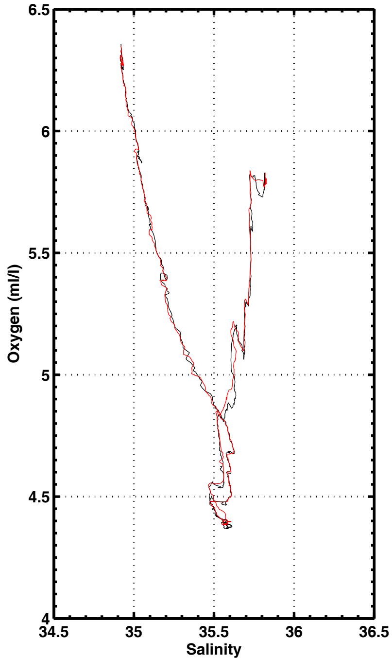
S-O2 , station 2044
