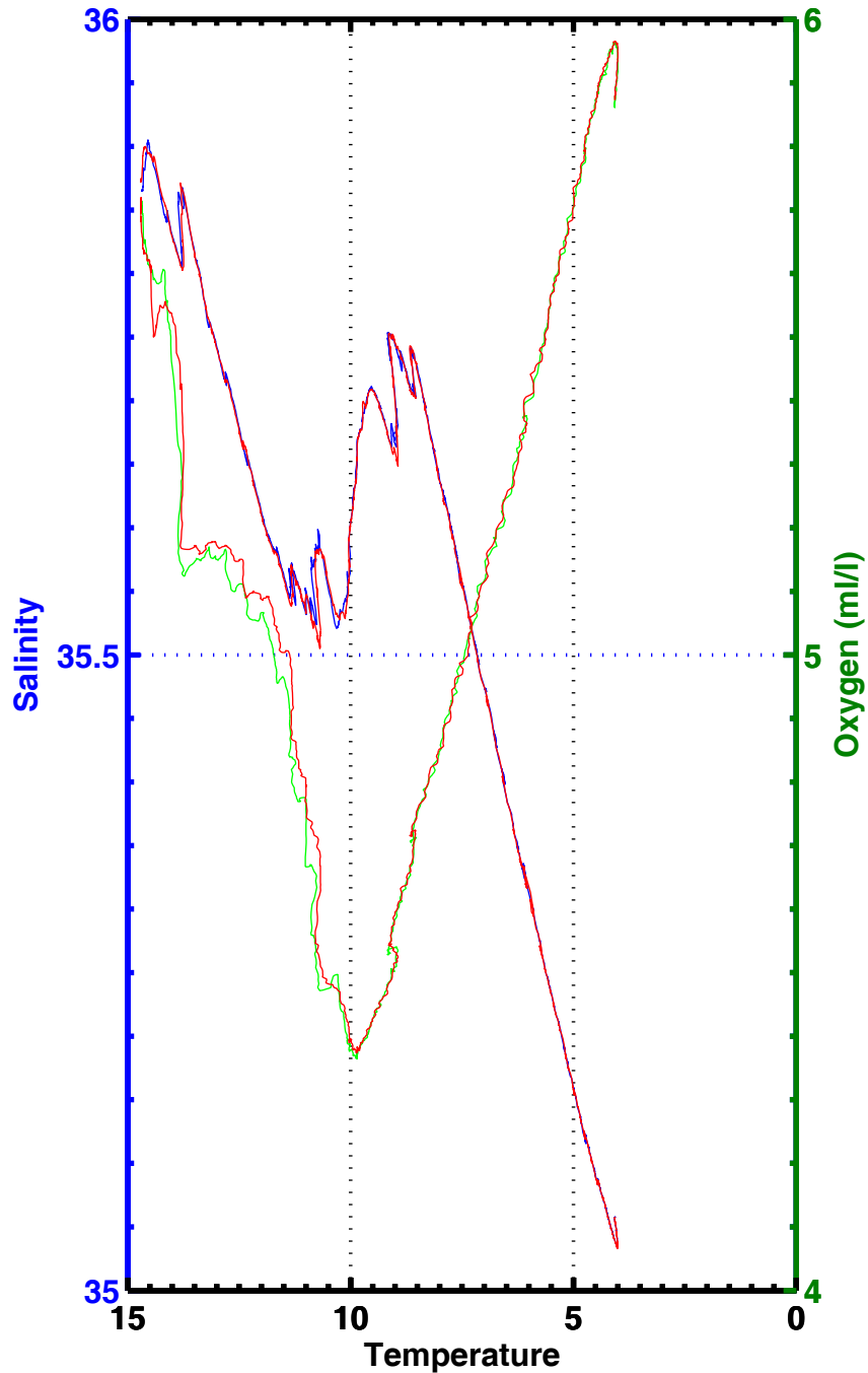
T-S , T-02 , station 2002
