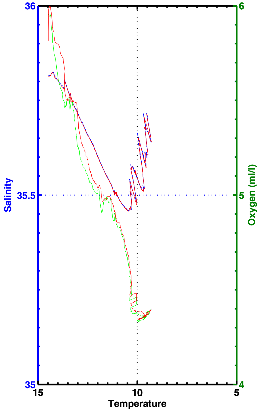
T-S , T-02 , station 2276
