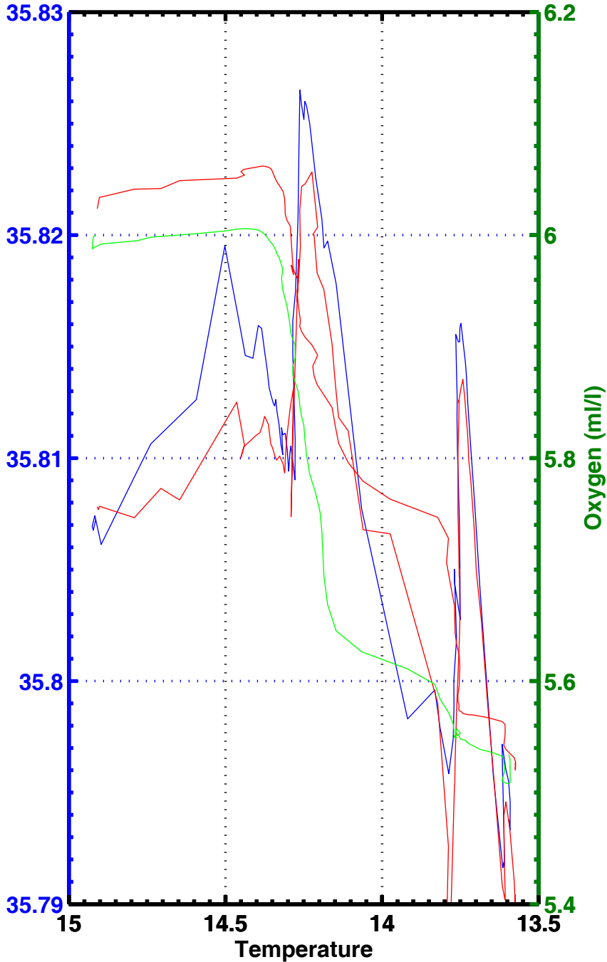
T-S , T-02 , station 2277
