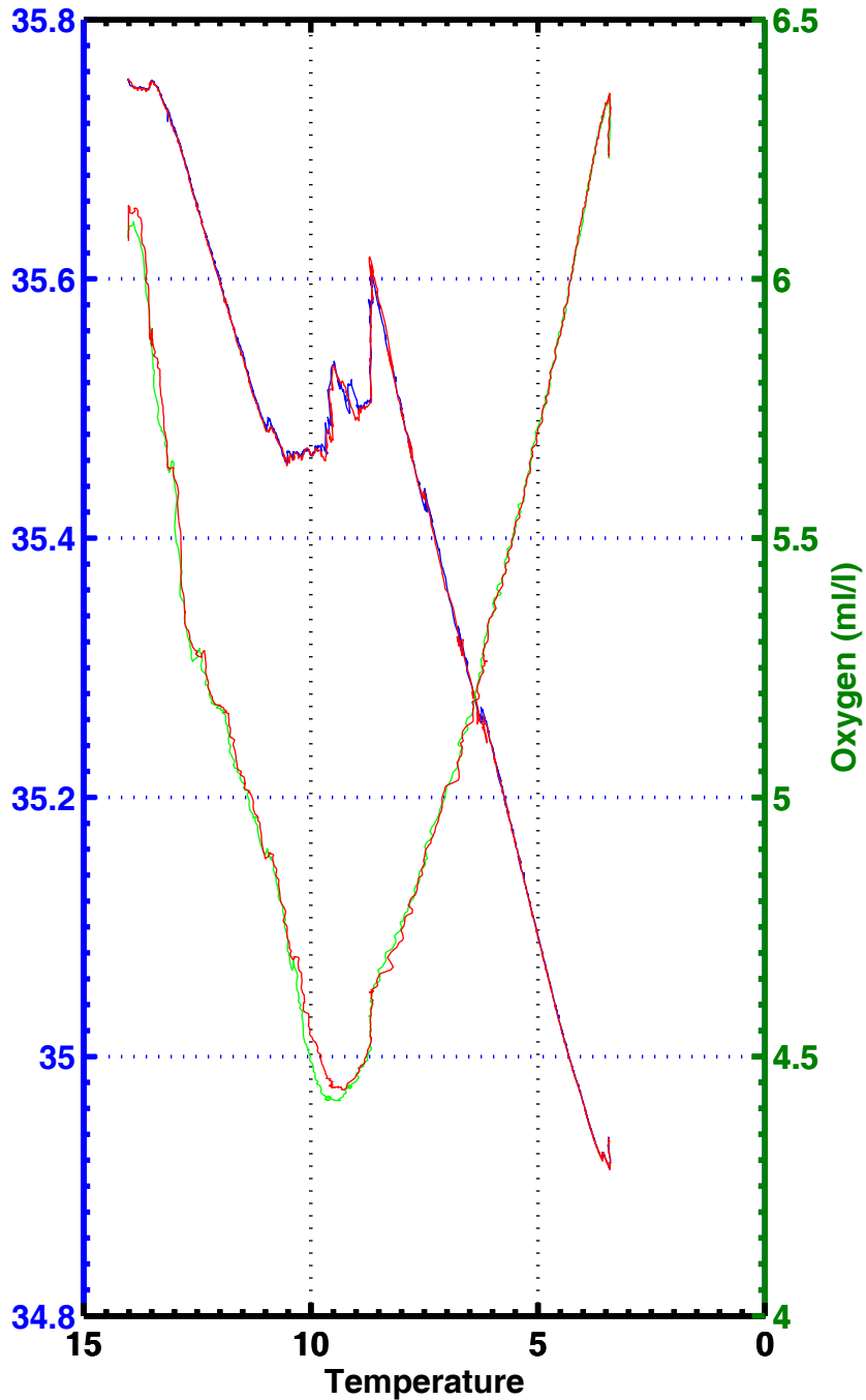
T-S , T-02 , station 2064
