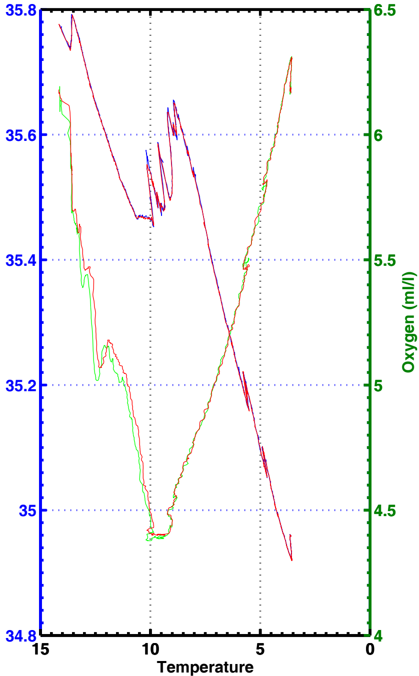
T-S , T-02 , station 2065
