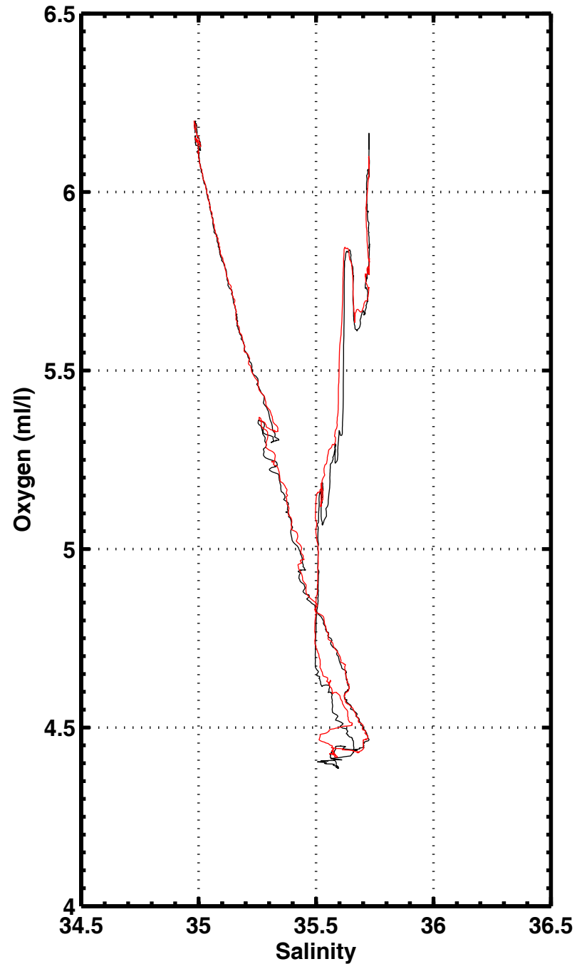
S-O2 , station 2027
