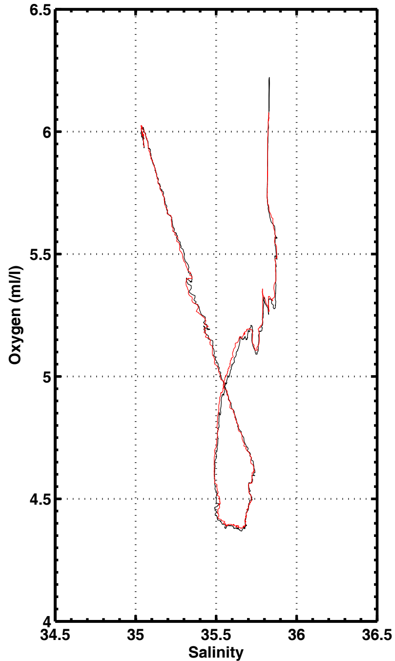
S-O2 , station 2032
