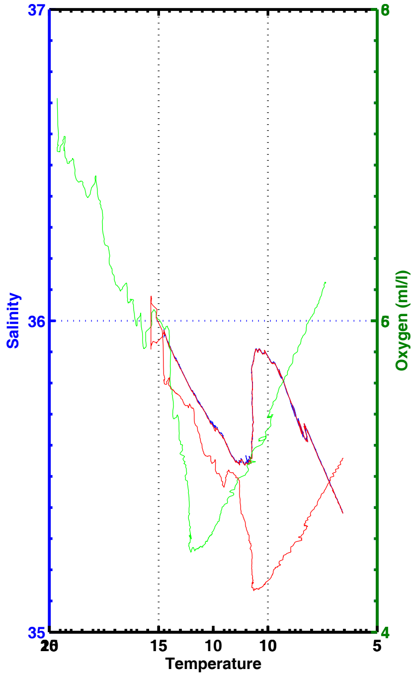
T-S , T-02 , station 2087
