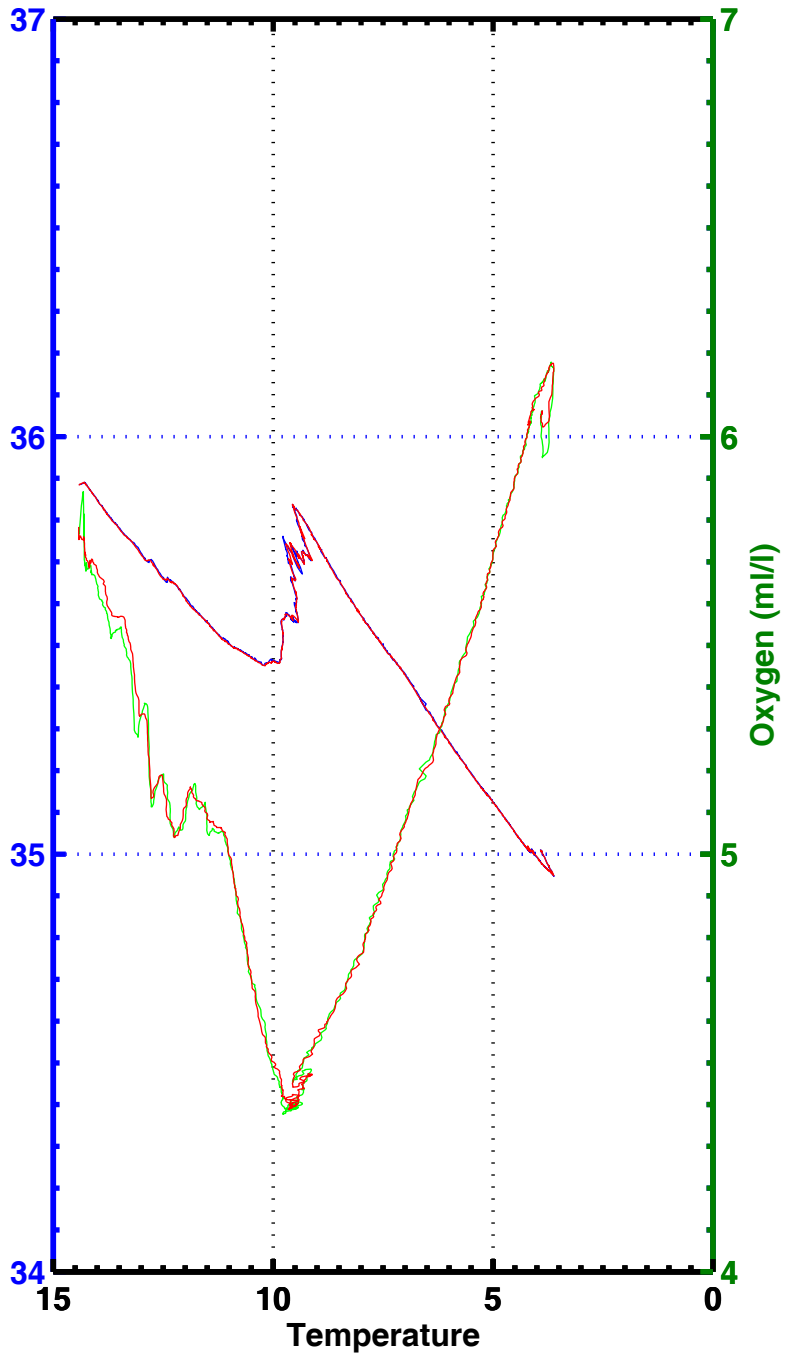
T-S , T-02 , station 2006
