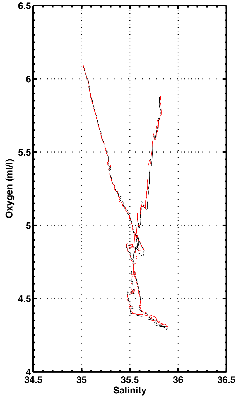
S-O2 , station 2028
