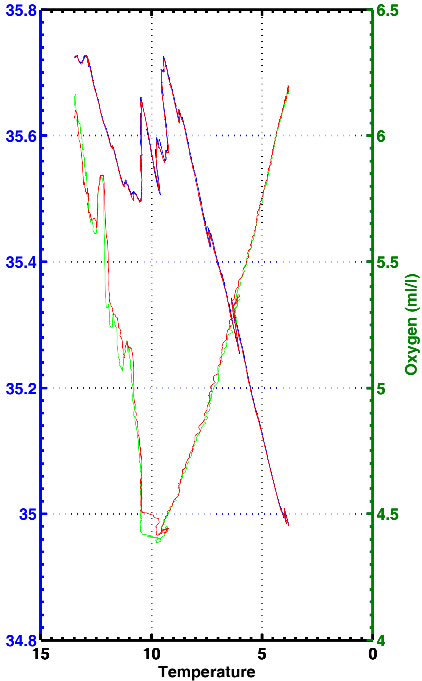
T-S , T-02 , station 2027
