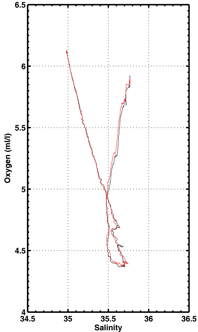
S-O2 , station 2043
