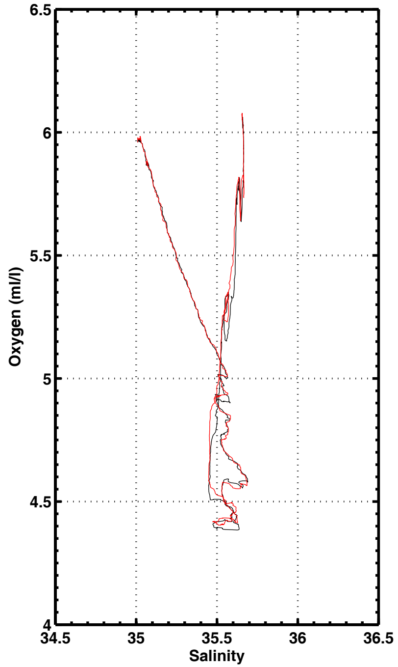
S-O2 , station 2008
