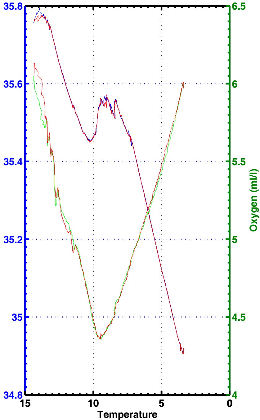
T-S , T-02 , station 2183
