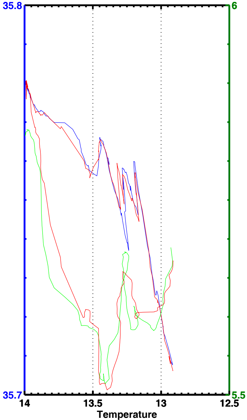
T-S , T-02 , station 2412
