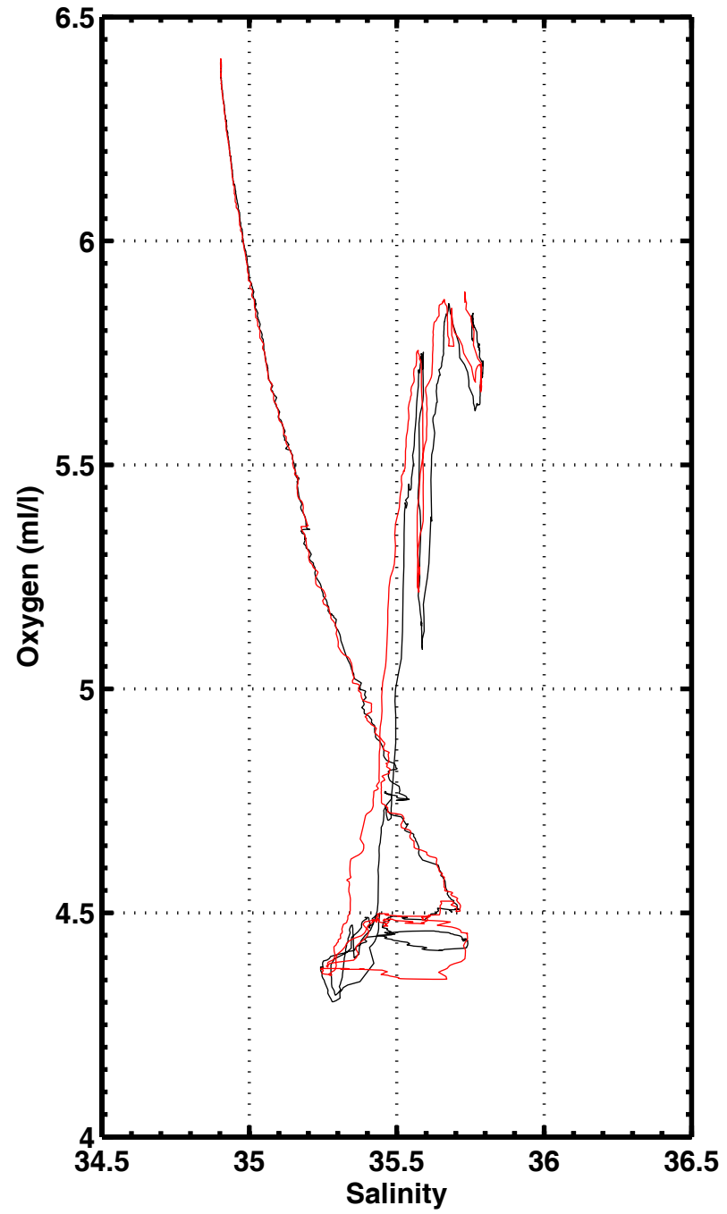
S-O2 , station 2013
