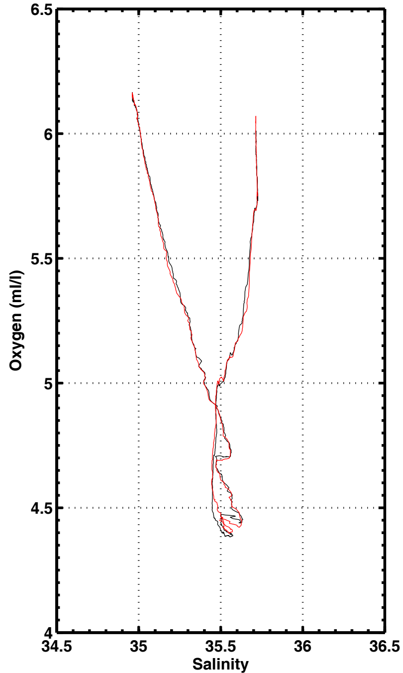
S-O2 , station 2051
