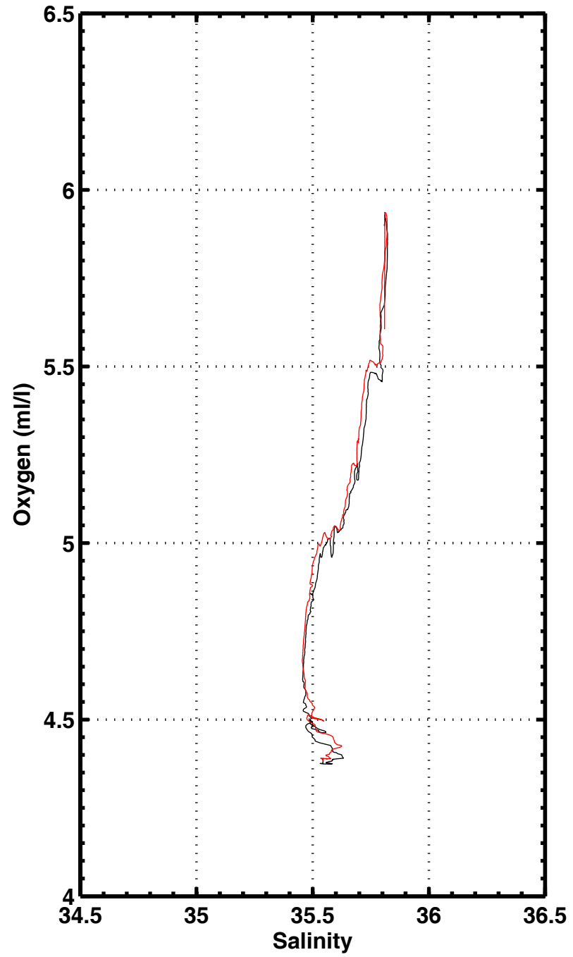
S-02 , station 2274
