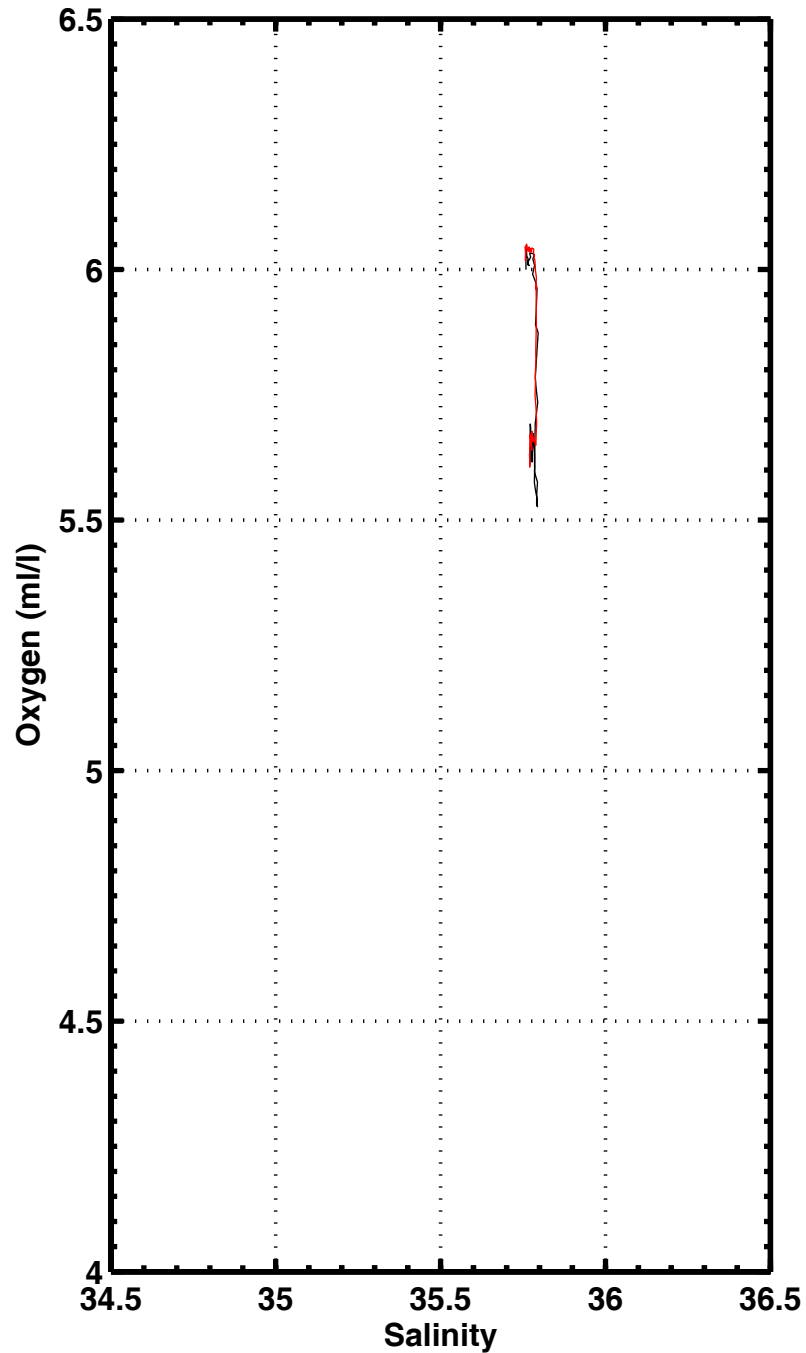
S-O2 , station 2178
