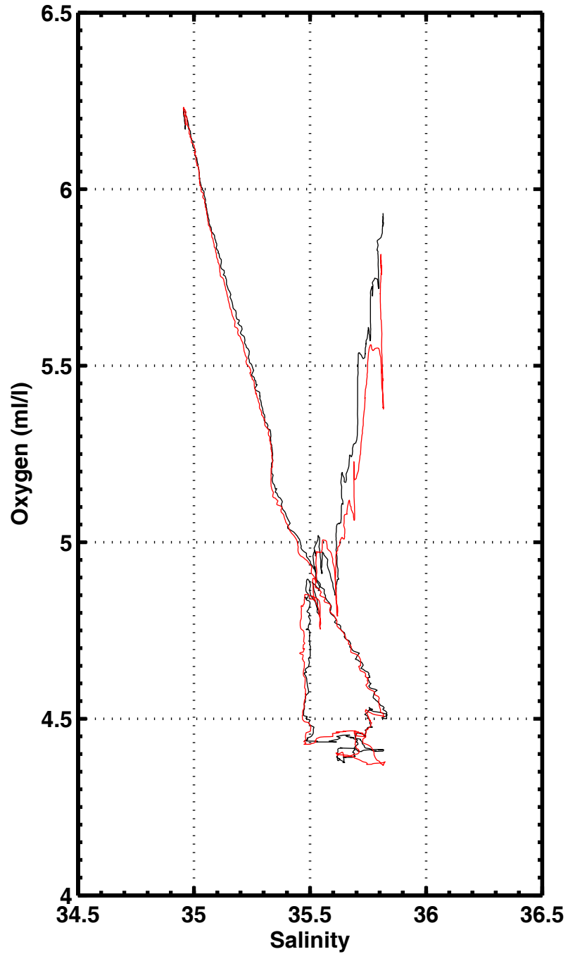
S-O2 , station 2021
