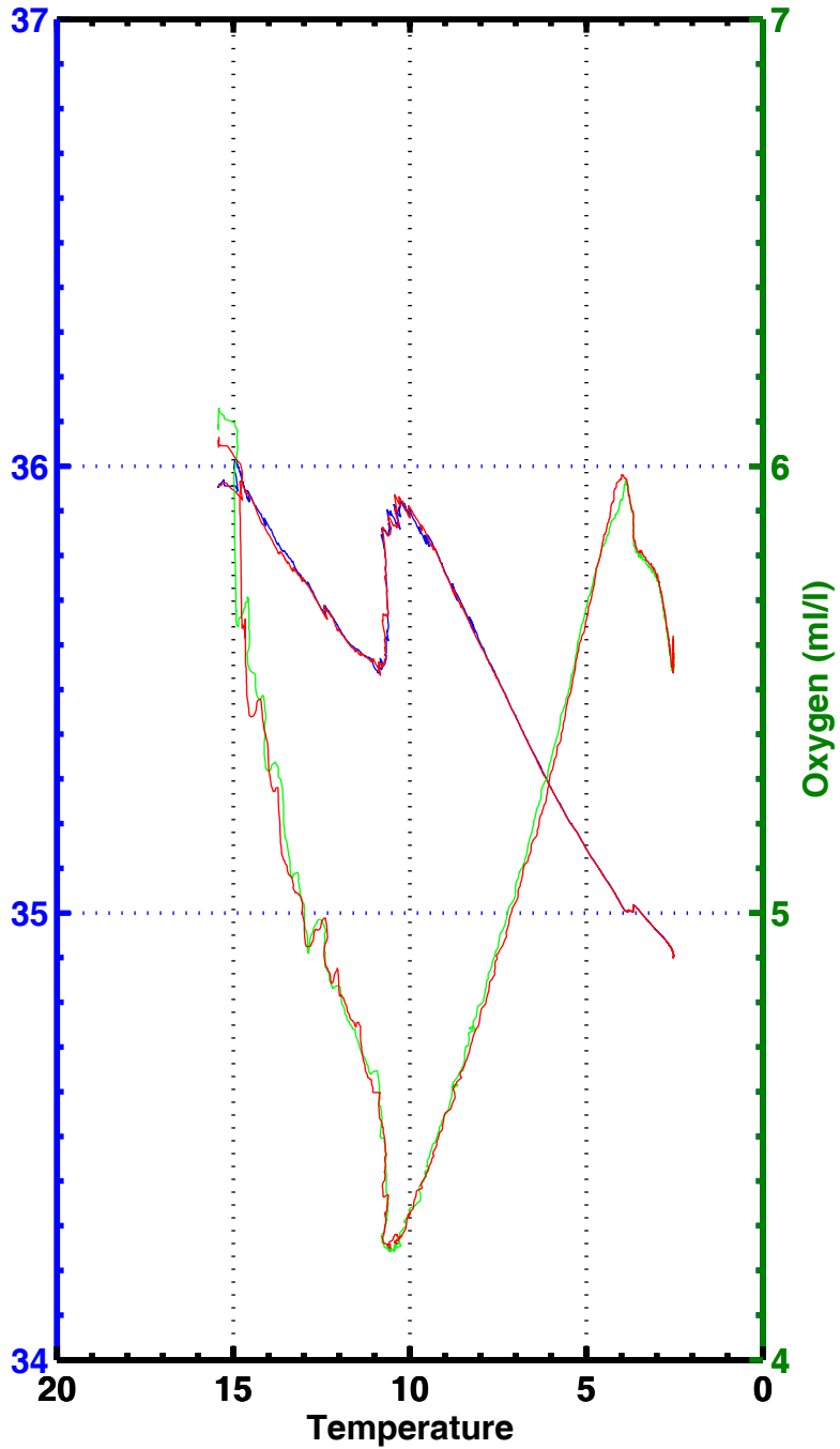
T-S, T-02, station 2076
