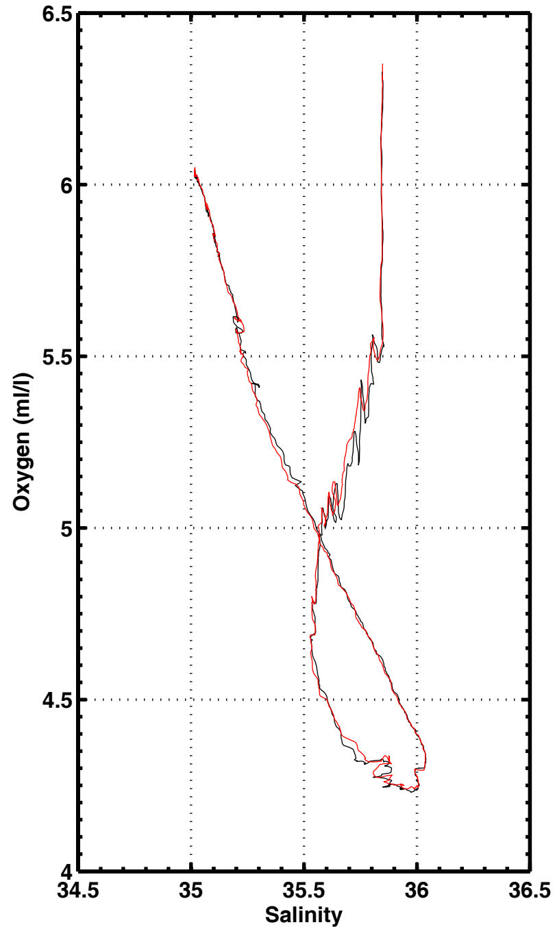
S-O2 , station 2075
