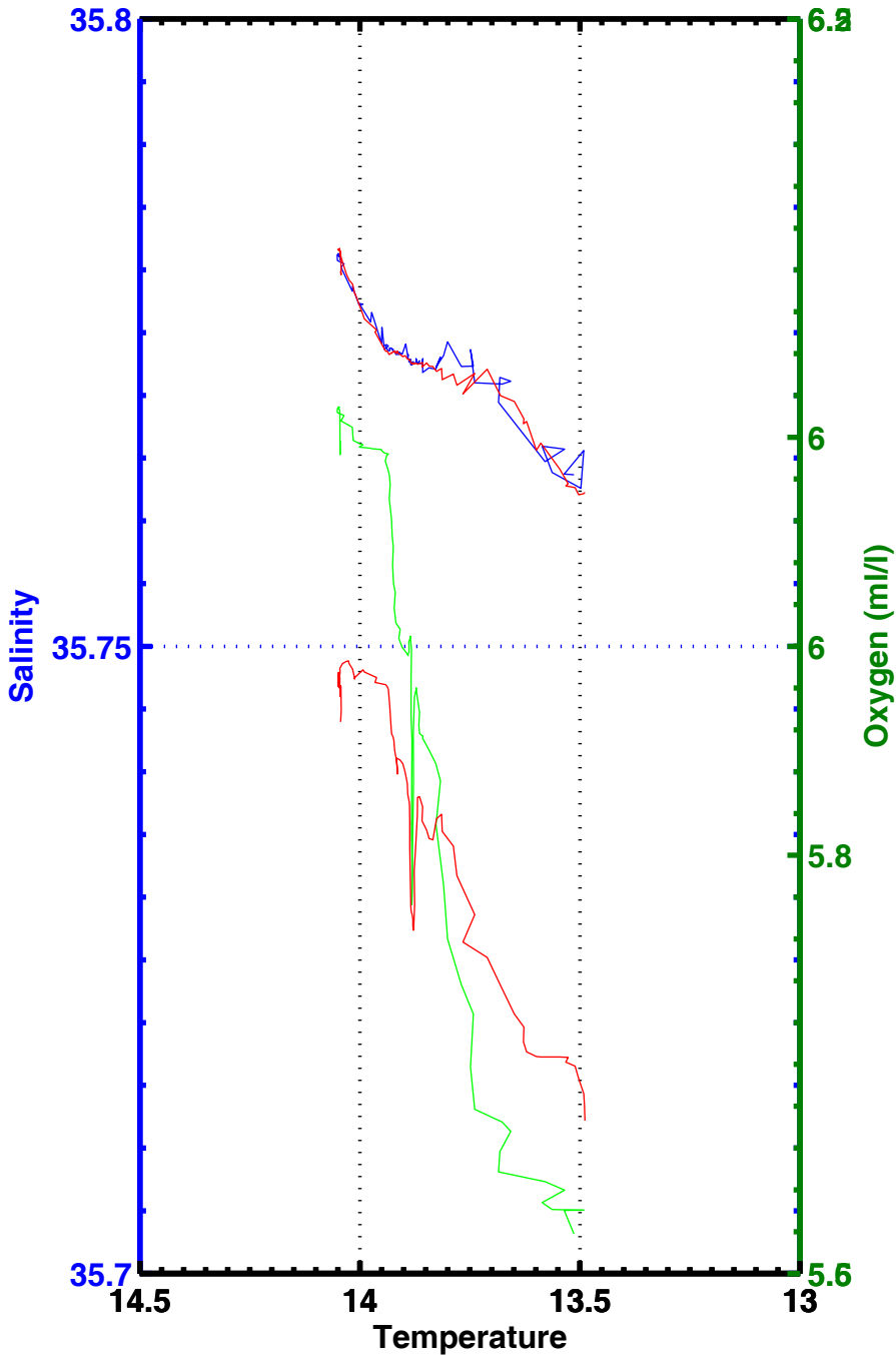
T-S, T-02, station 2409
