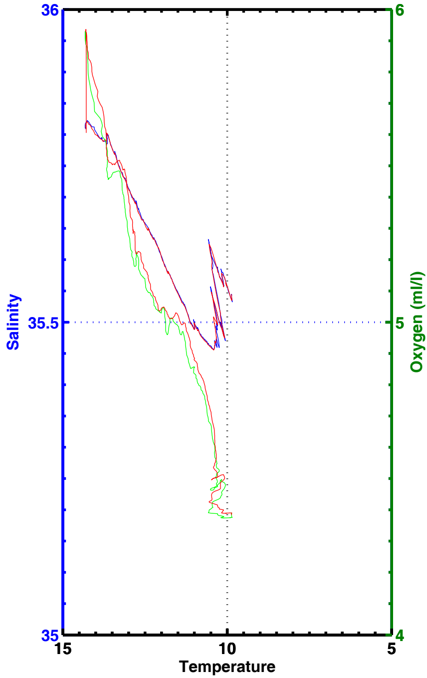
T-S , T-02 , station 2274
