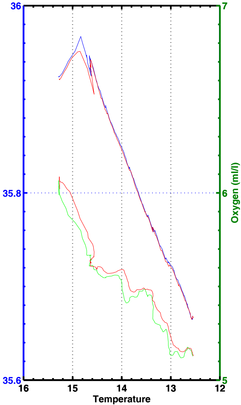
T-S , T-02 , station 2091
