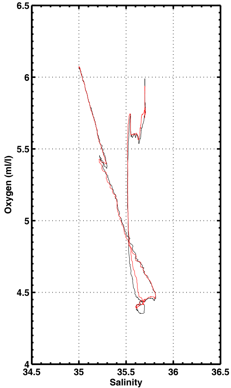
S-O2 , station 2041
