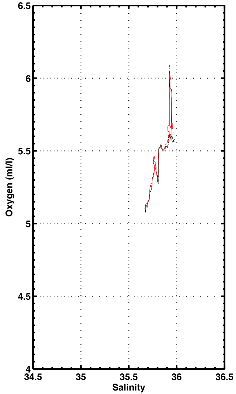
S-O2 , station 2089
