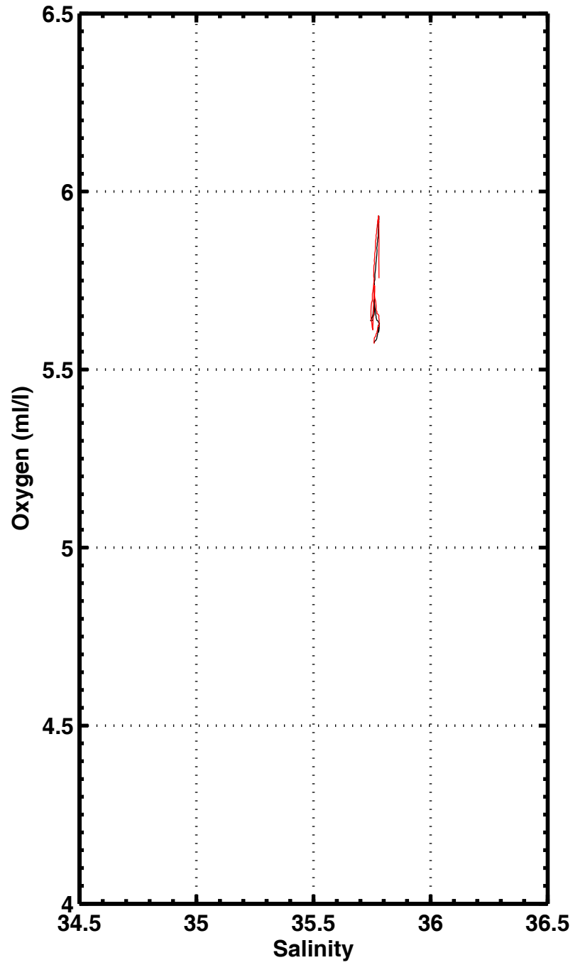
S-O2 , station 2401
