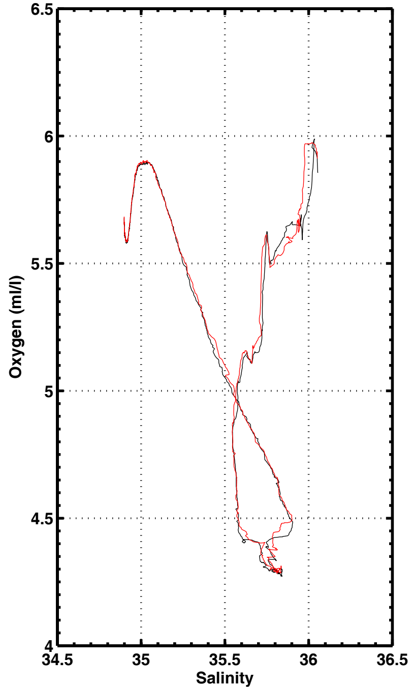
S-02 , station 2081
