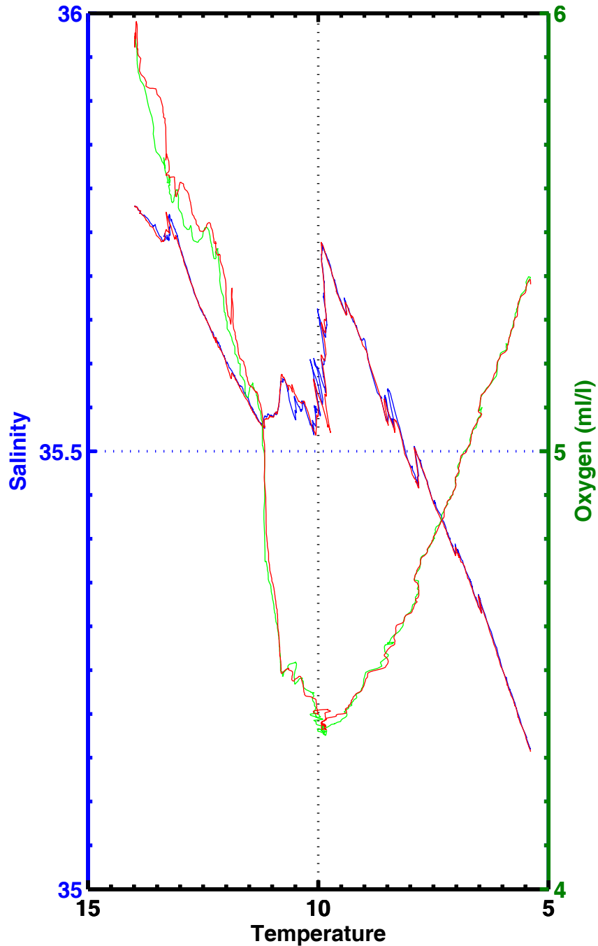
T-S , T-02 , station 2402
