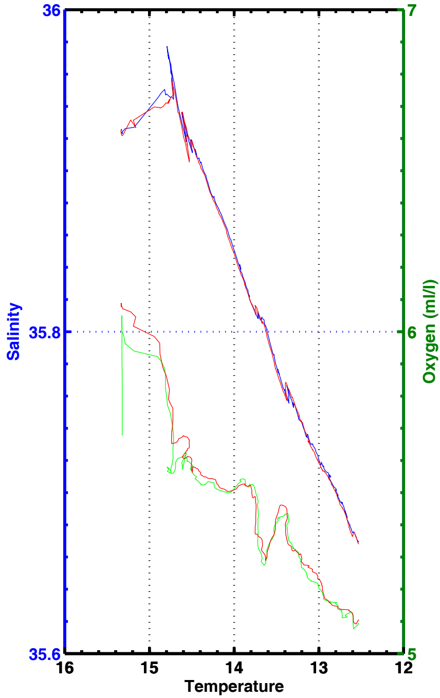
T-S , T-02 , station 2089
