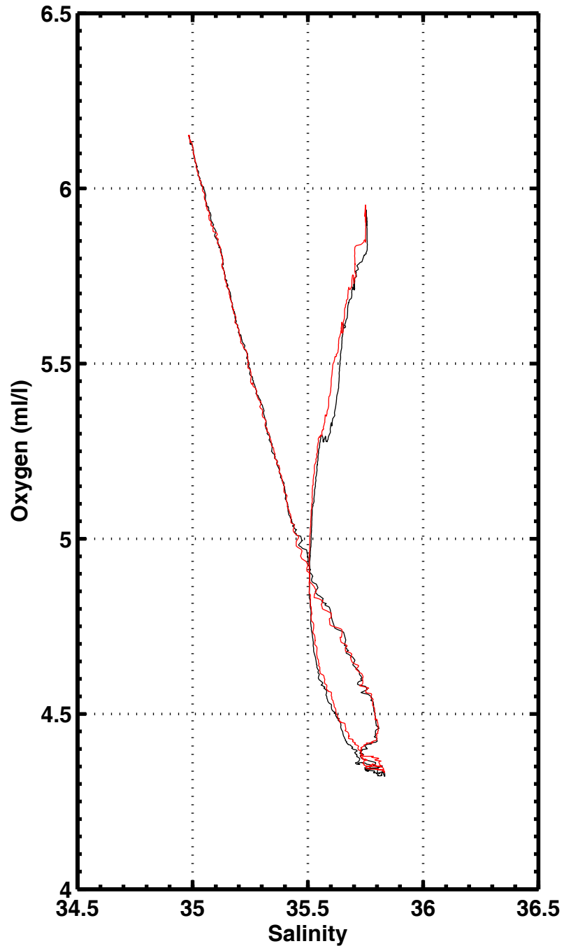
S-O2 , station 2042
