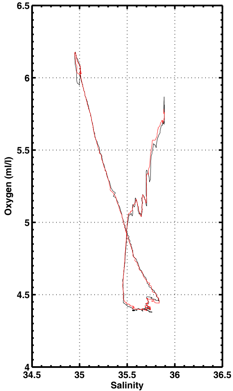
S-02 , station 2006
