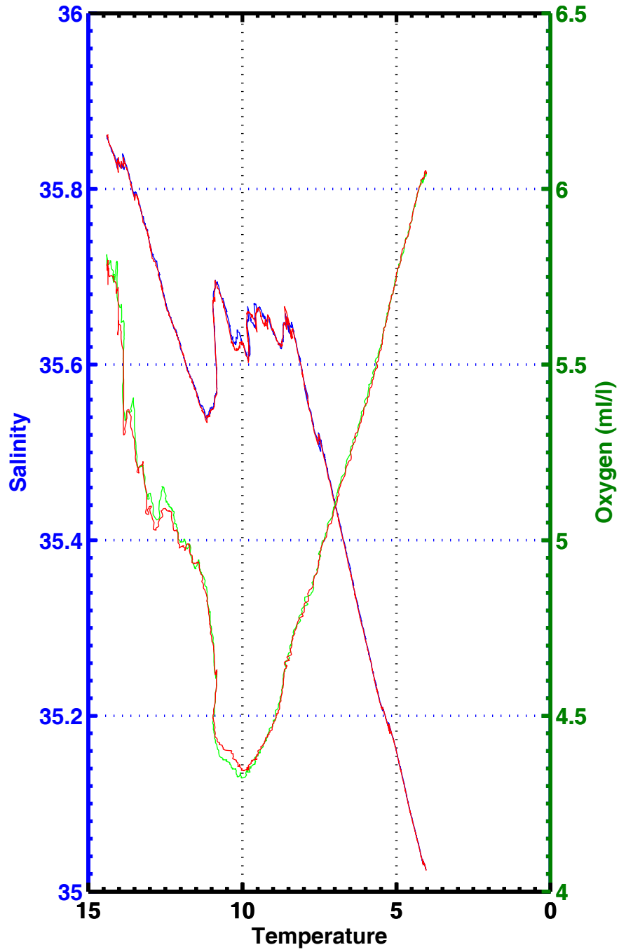
T-S , T-02 , station 2036
