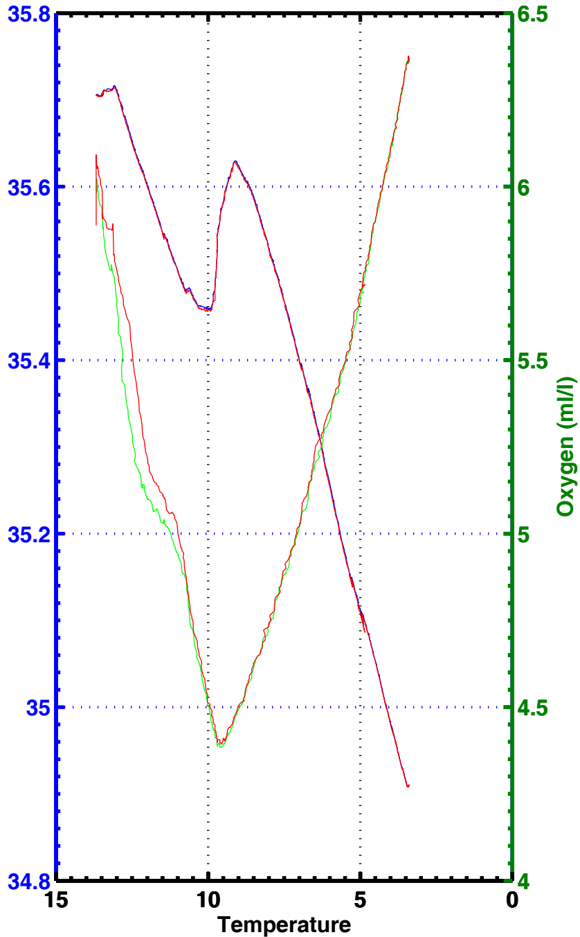
T-S , T-02 , station 2056
