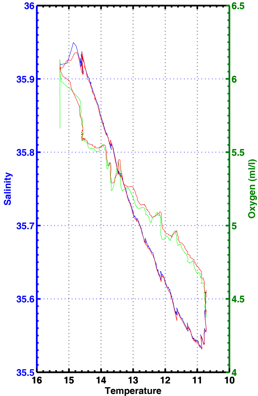
T-S , T-02 , station 2092
