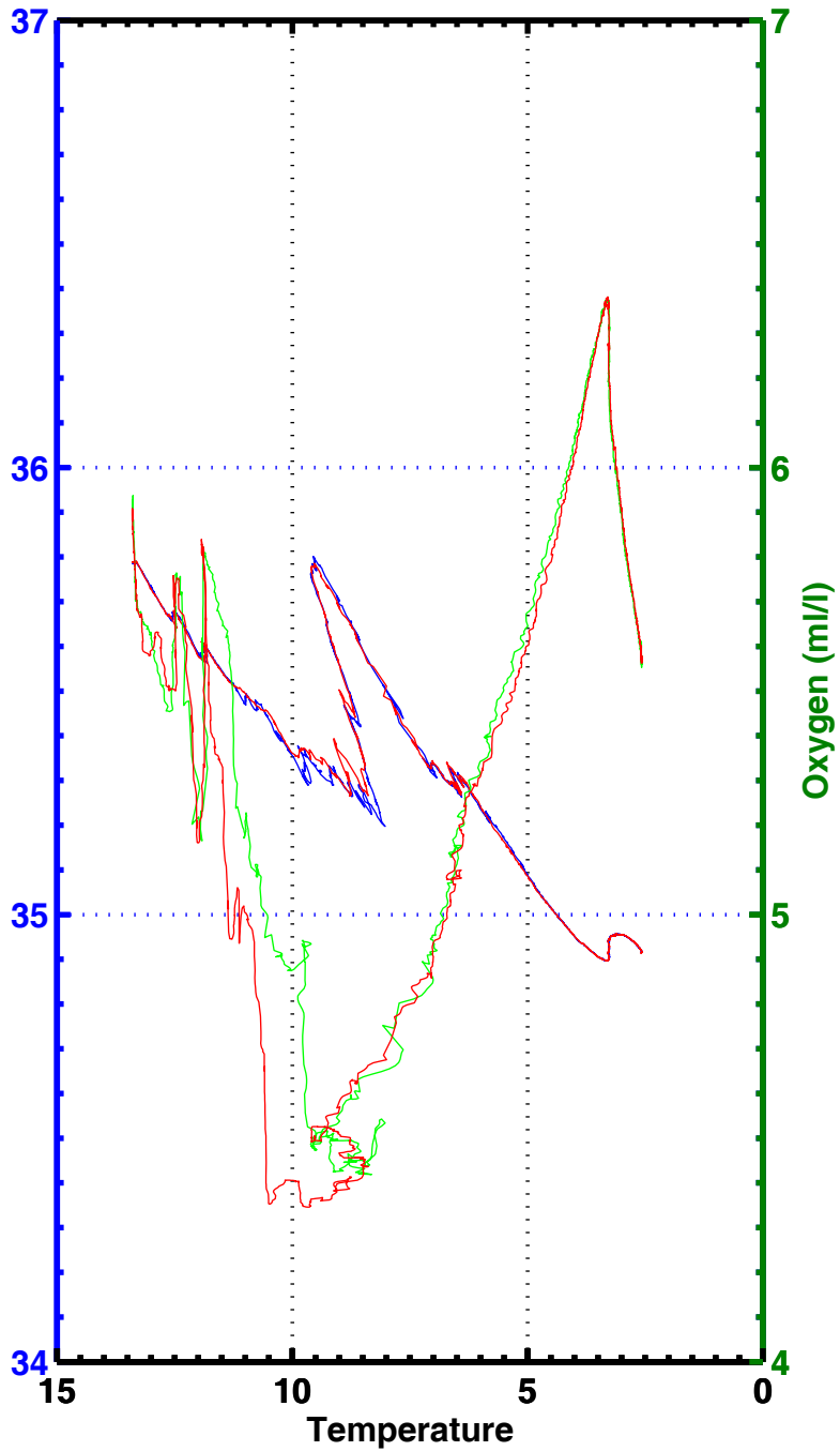
T-S , T-02 , station 2014
