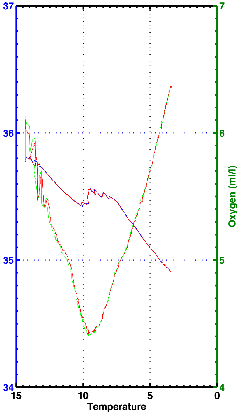
T-S , T-02 , station 2066
