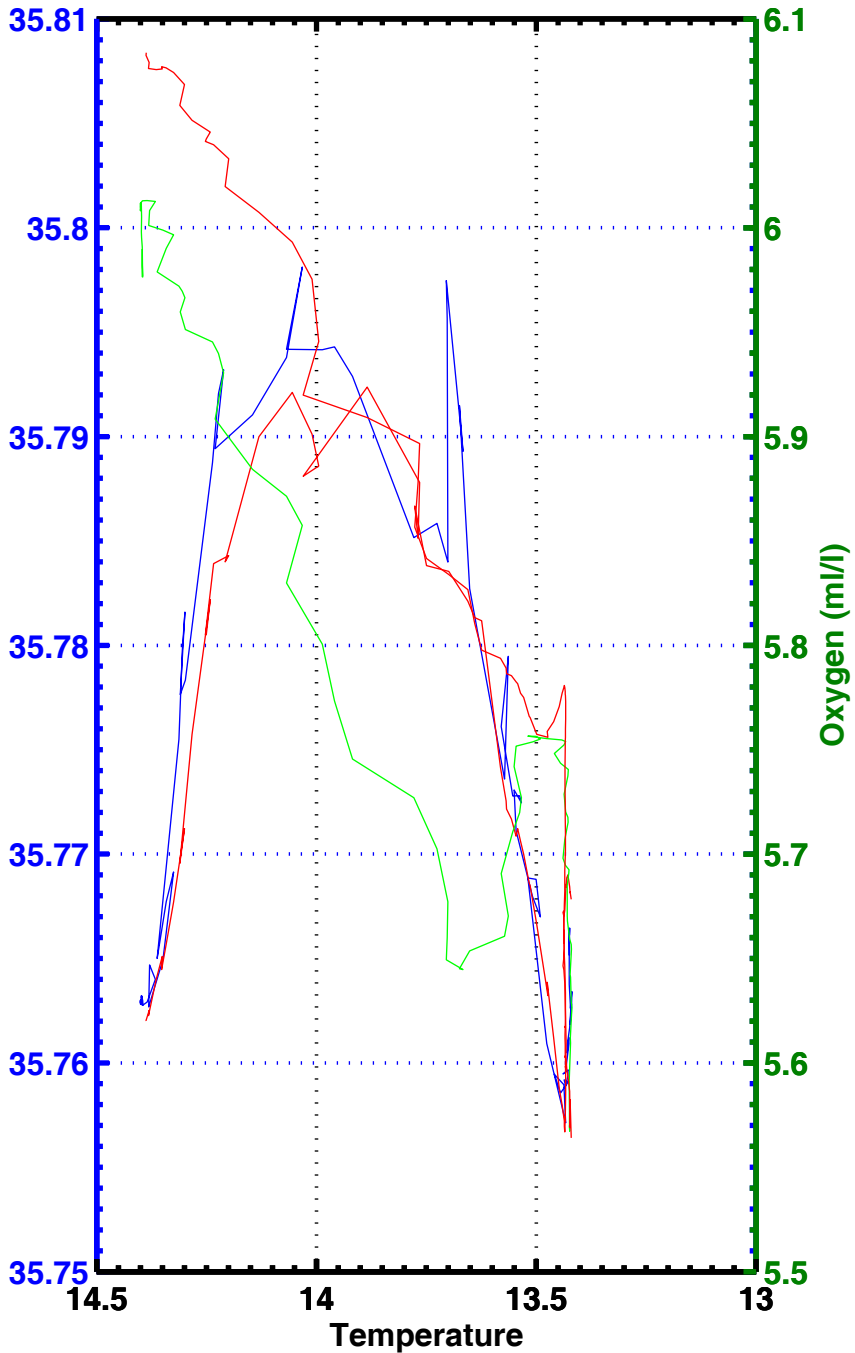
T-S, T-02 , station 2177
