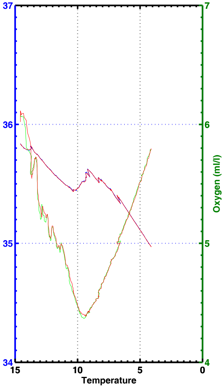
T-S , T-02 , station 2174
