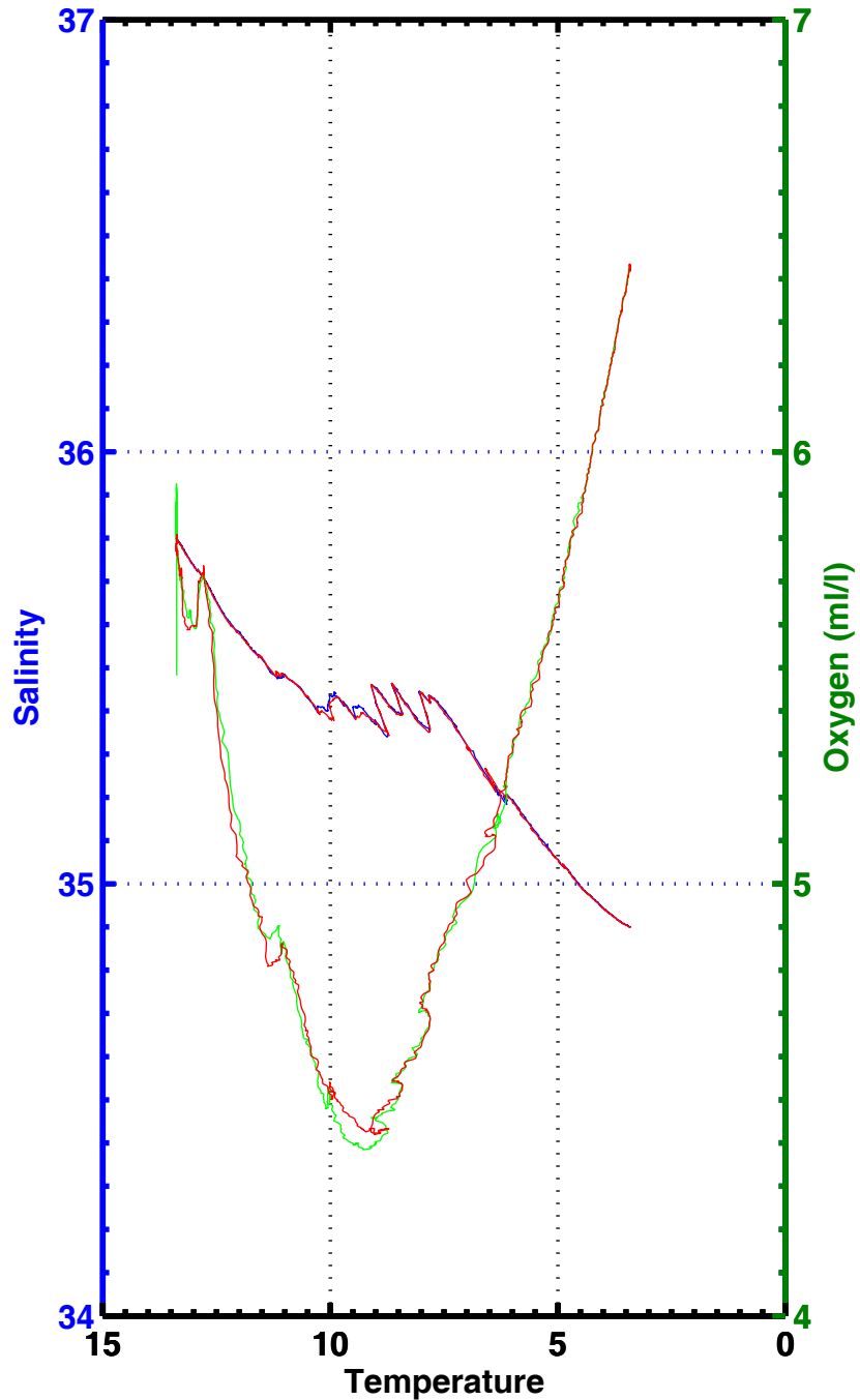
T-S , T-02 , station 2018
