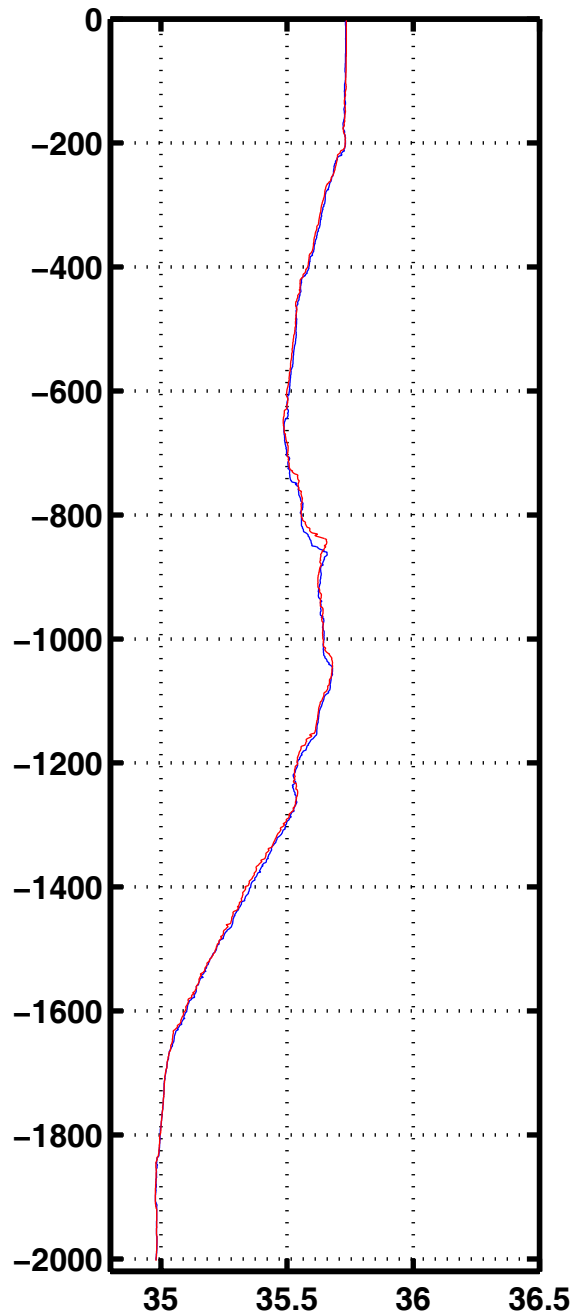
Sali 2020
