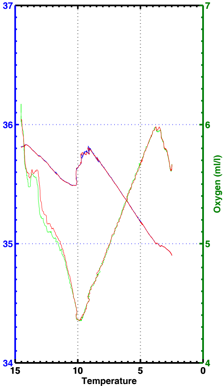
T-S , T-02 , station 2034
