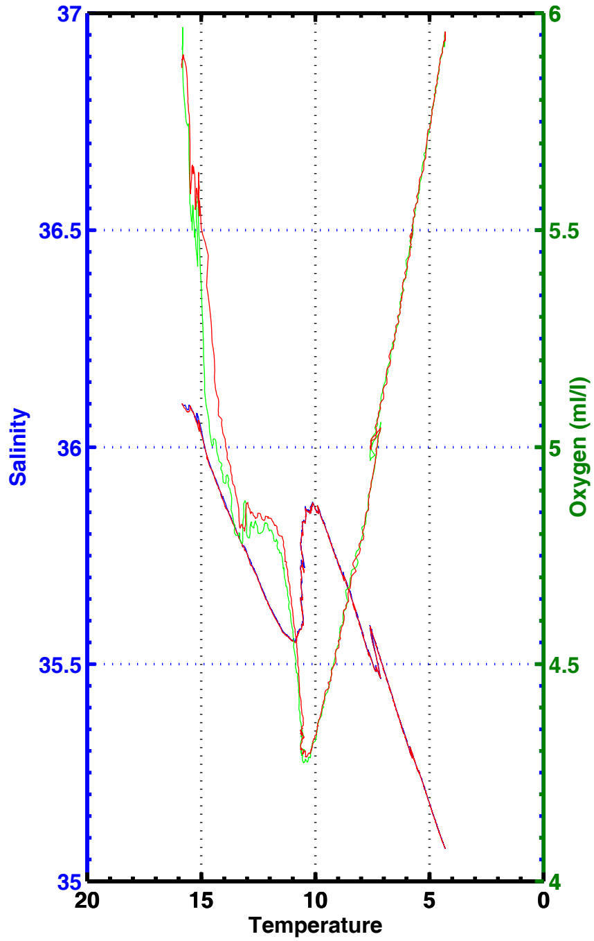
T-S , T-02 , station 2070
