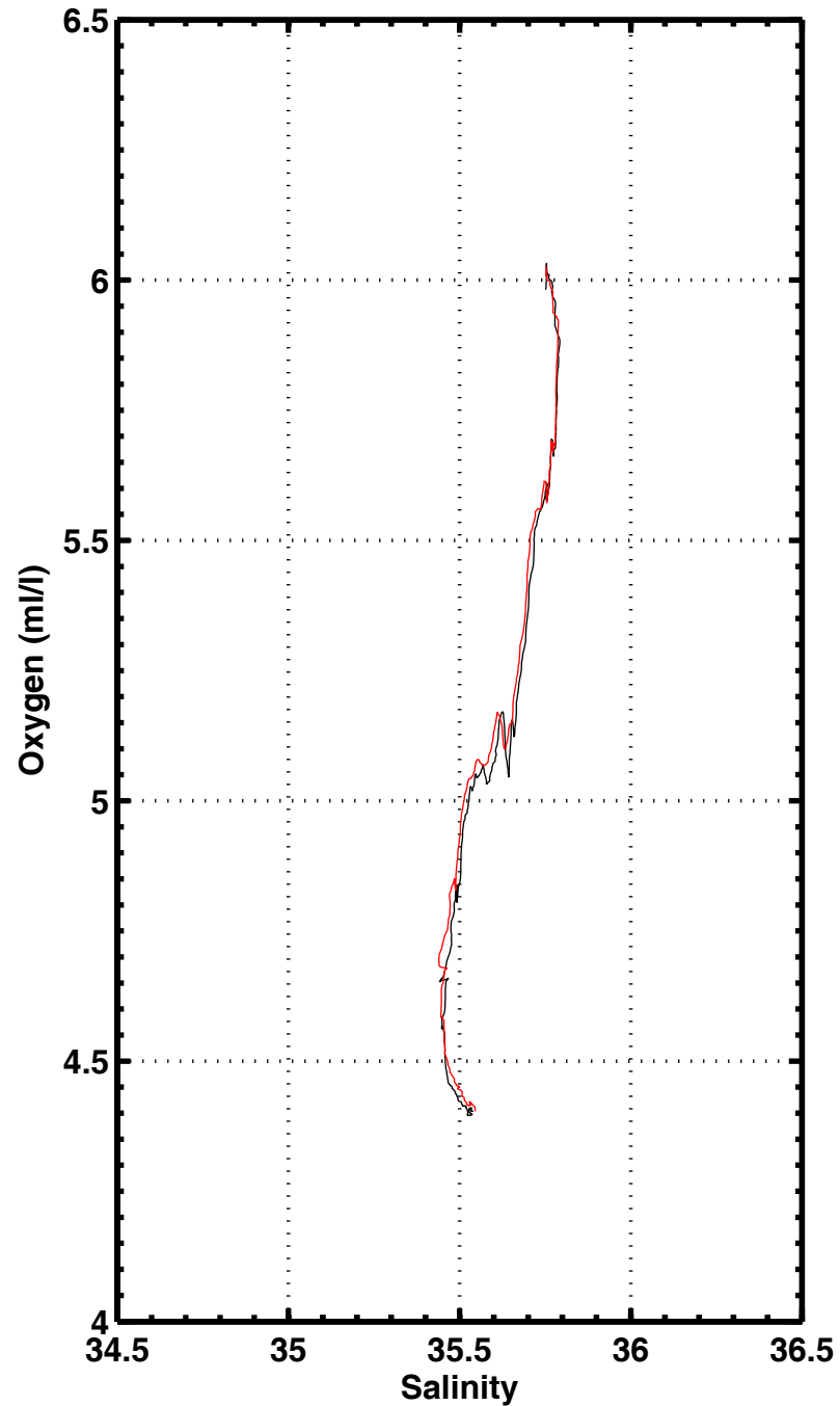
S-O2 , station 2180
