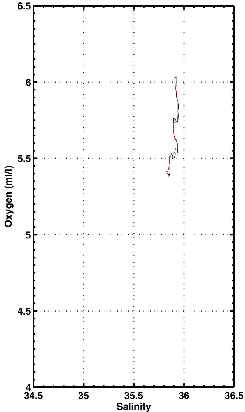
S-O2 , station 2083
