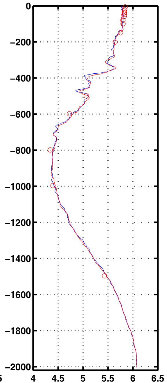
Oxyg 2017
