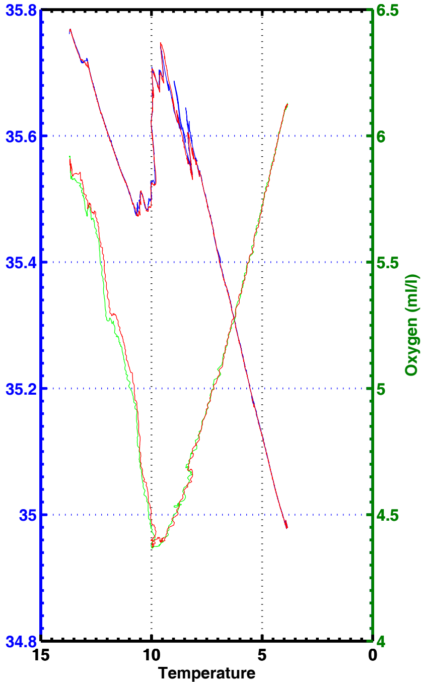
T-S , T-02 , station 2043
