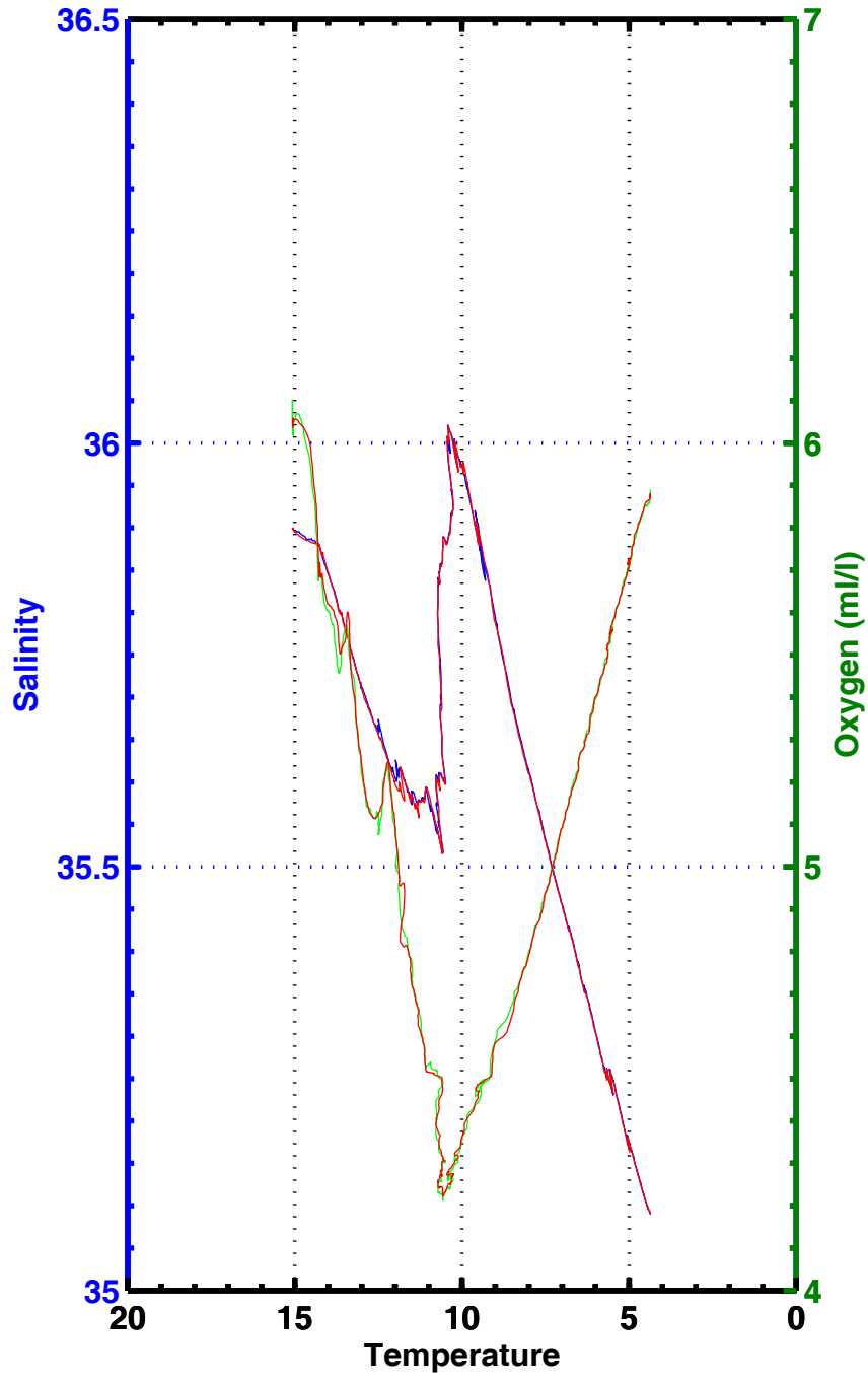
T-S , T-02 , station 2077
