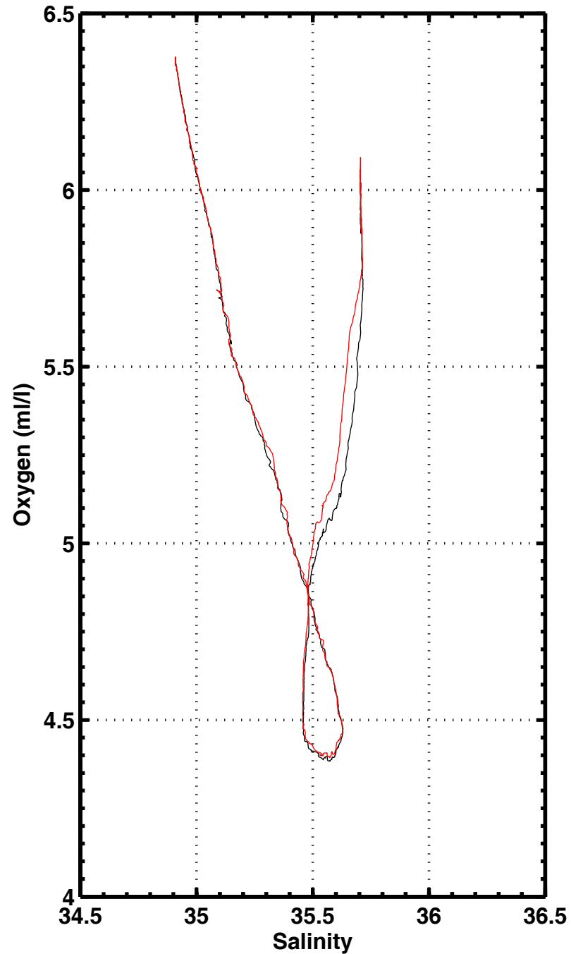
S-02 , station 2056
