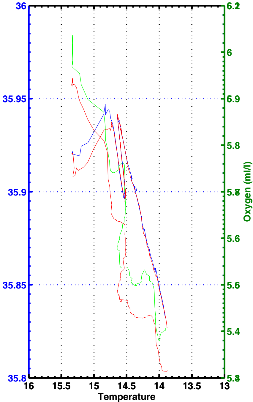
T-S , T-02 , station 2083
