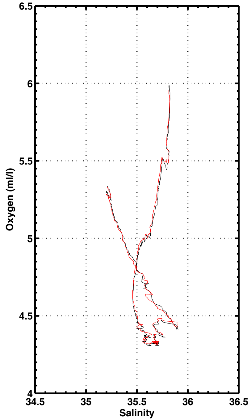
S-O2 , station 2269
