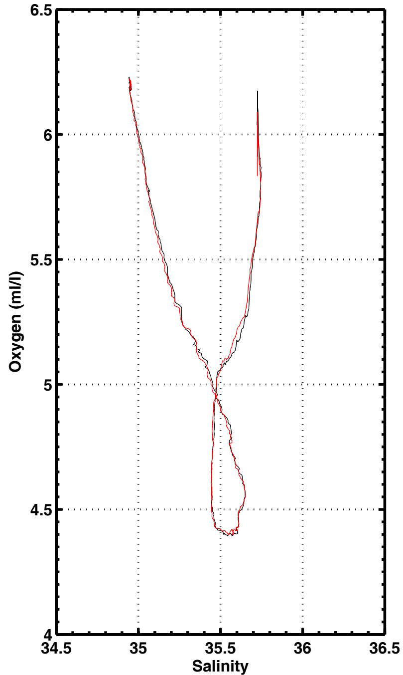
S-O2 , station 2057
