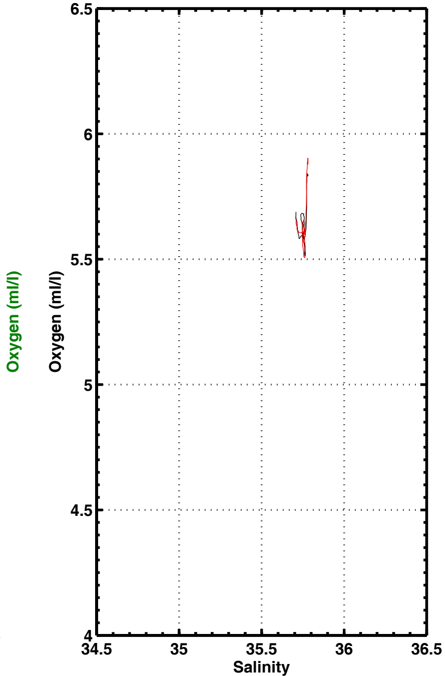
S-02 , station 2412
