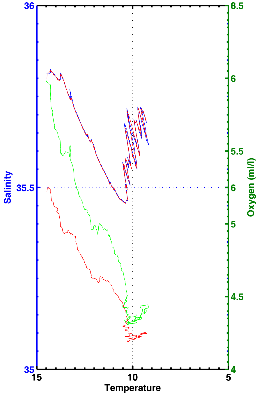
T-S , T-02 , station 2268
