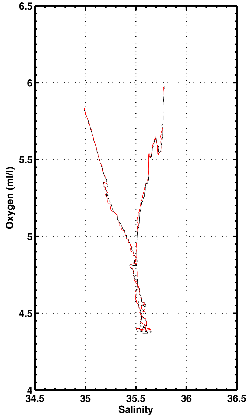
S-O2 , station 2414
