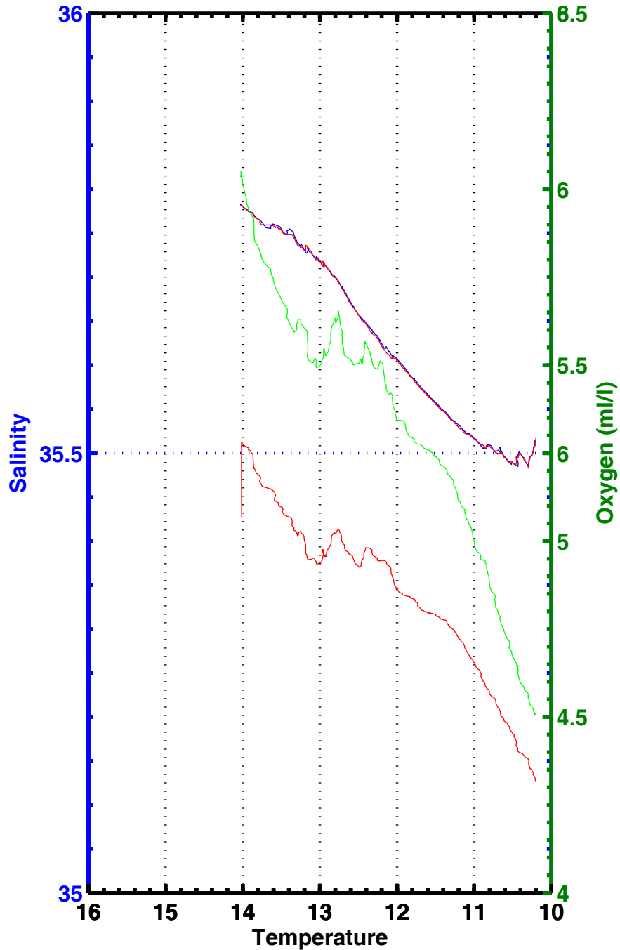
T-S , T-02 , station 2411
