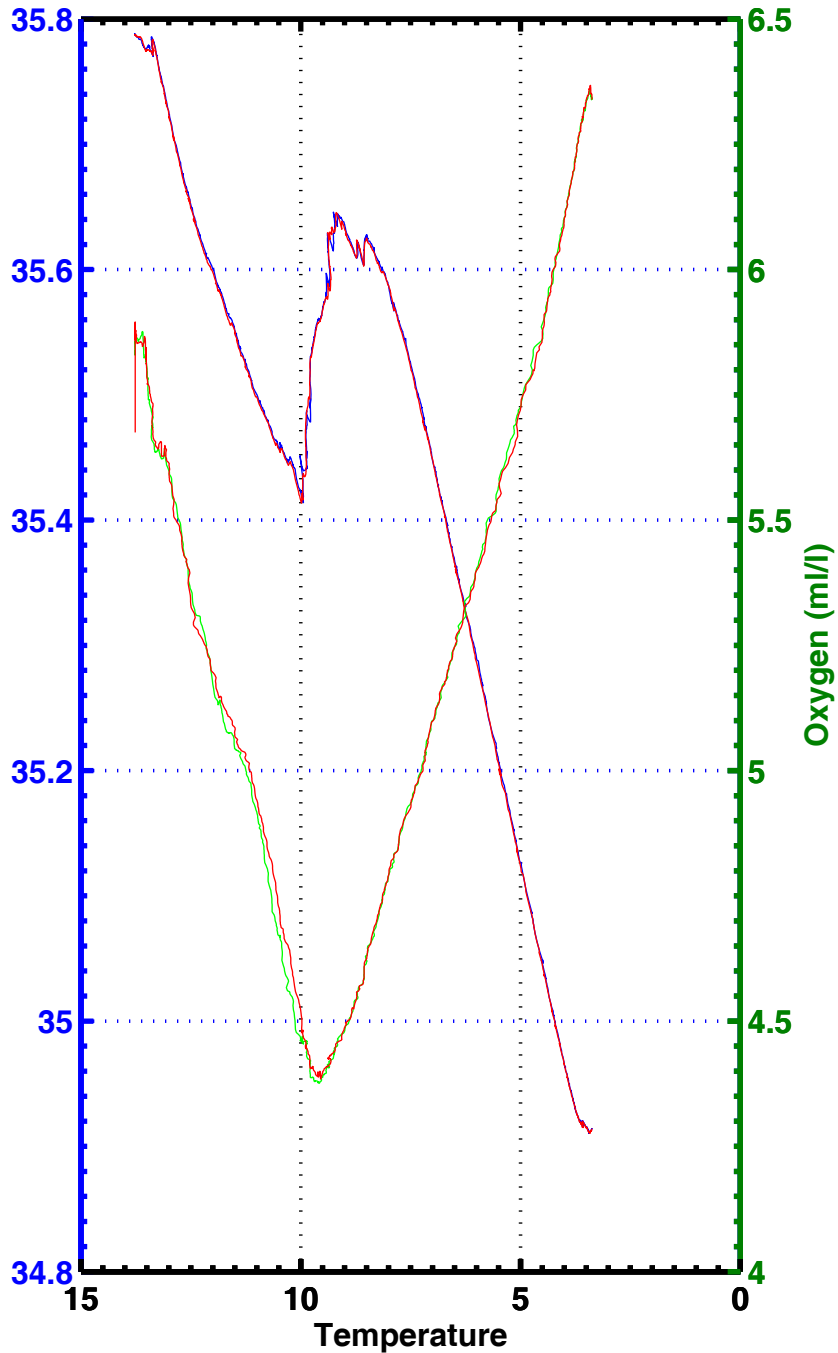
T-S , T-02 , station 2055
