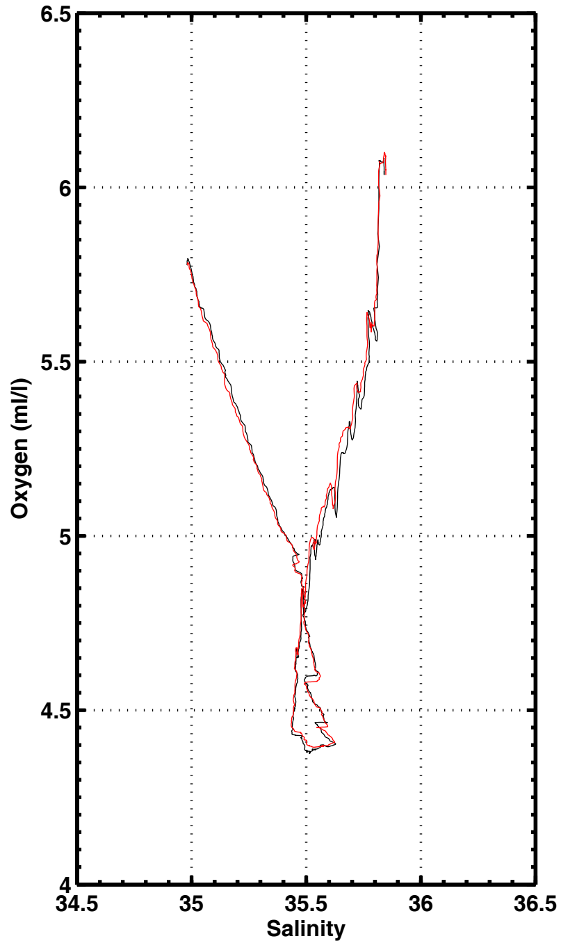
S-O2 , station 2170
