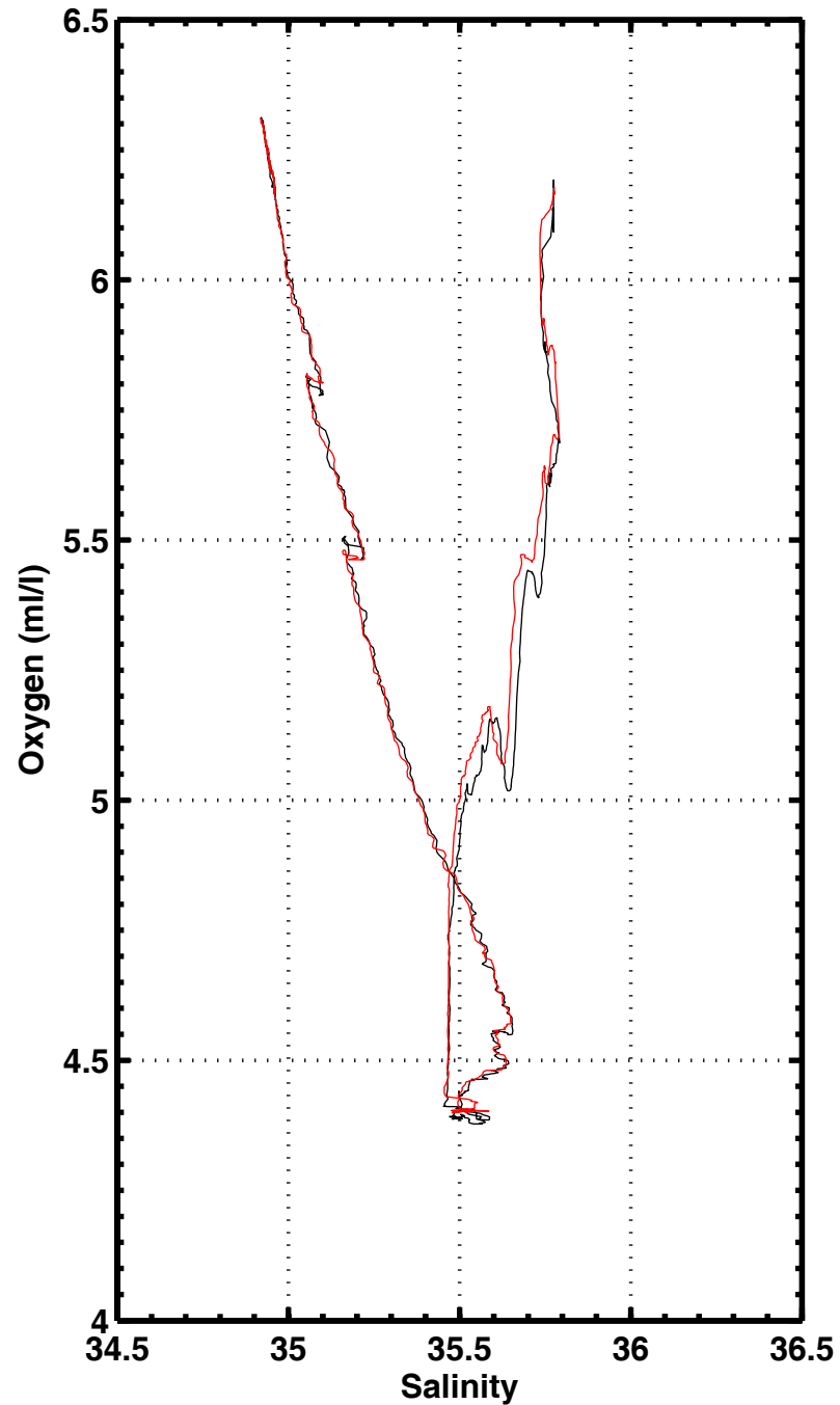
S-O2 , station 2065
