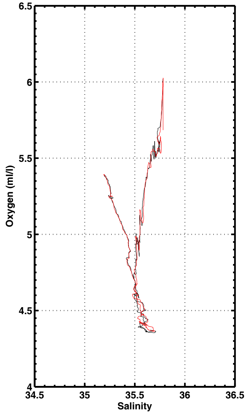
S-O2 , station 2406
