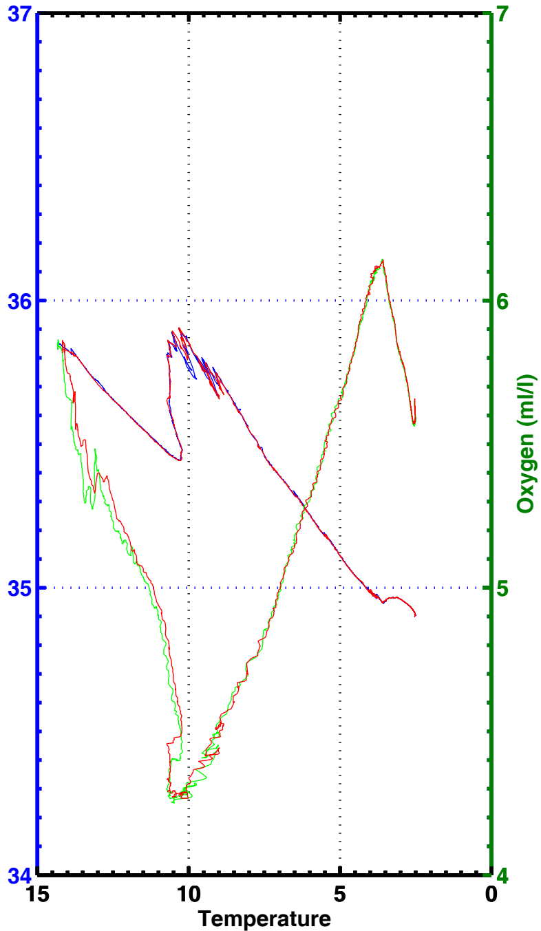
T-S , T-02 , station 2038
