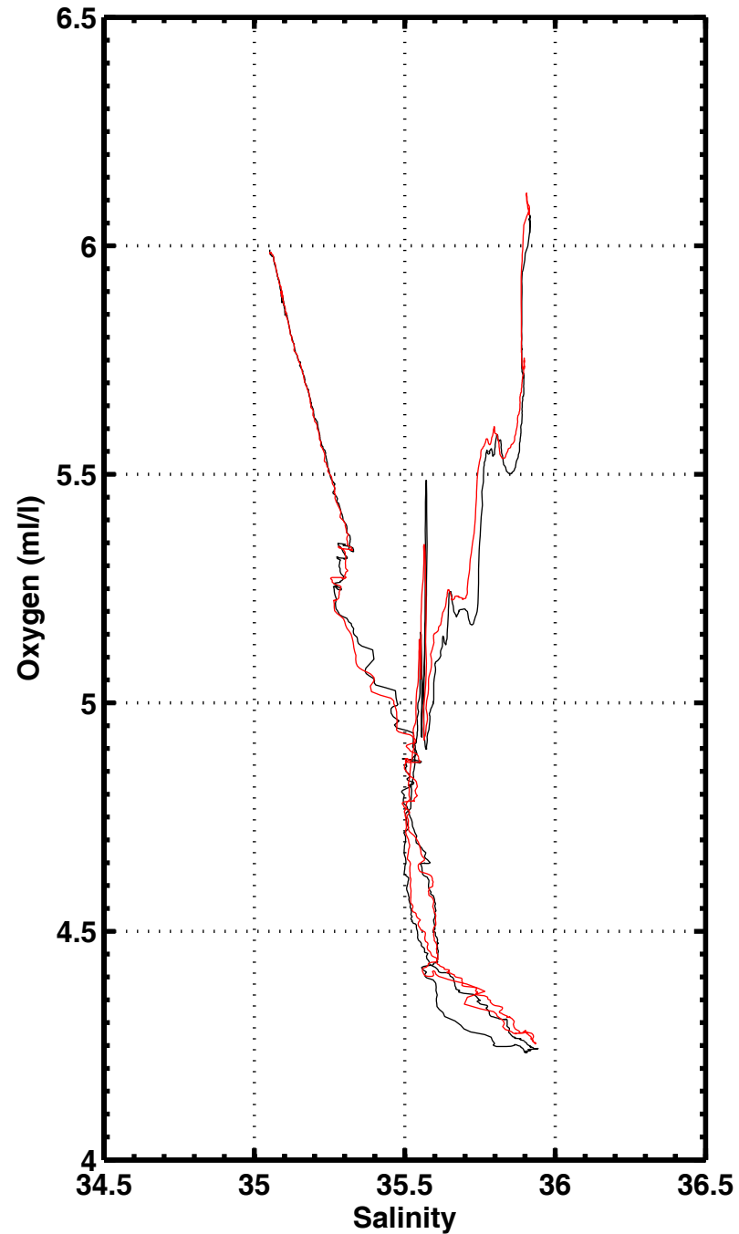
S-O2 , station 2072
