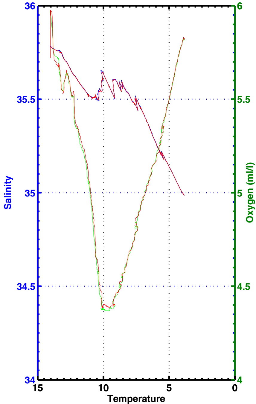
T-S , T-02 , station 2414
