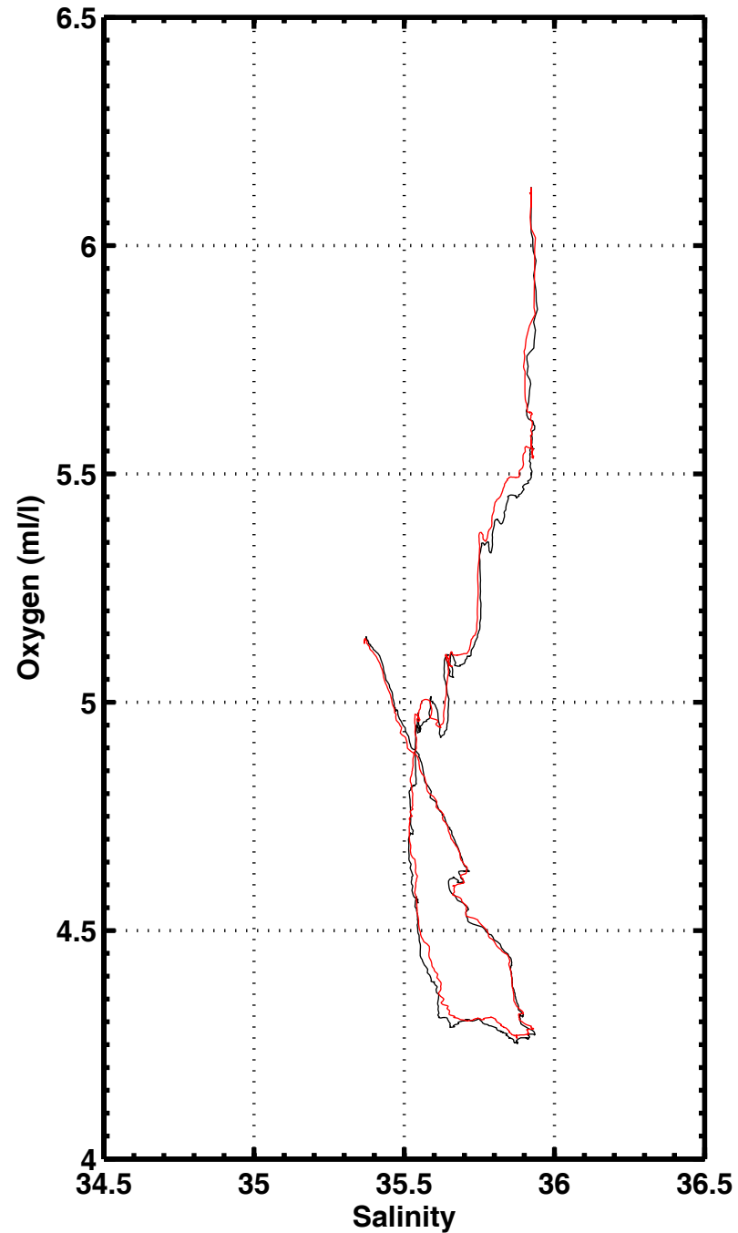
S-O2 , station 2085
