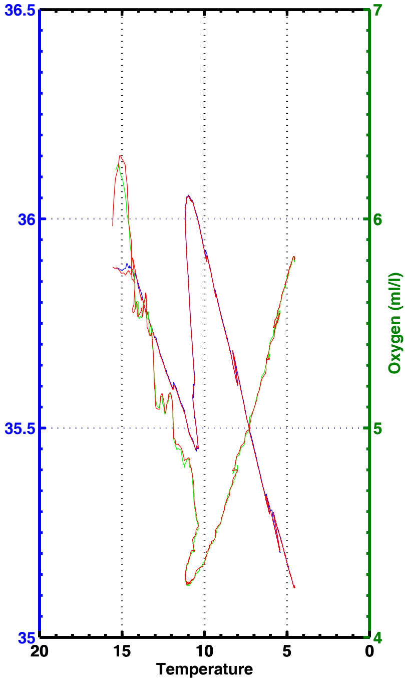
T-S , T-02 , station 2079
