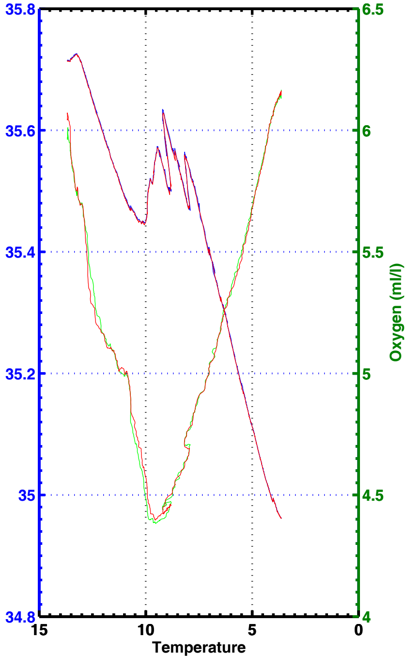
T-S , T-02 , station 2051
