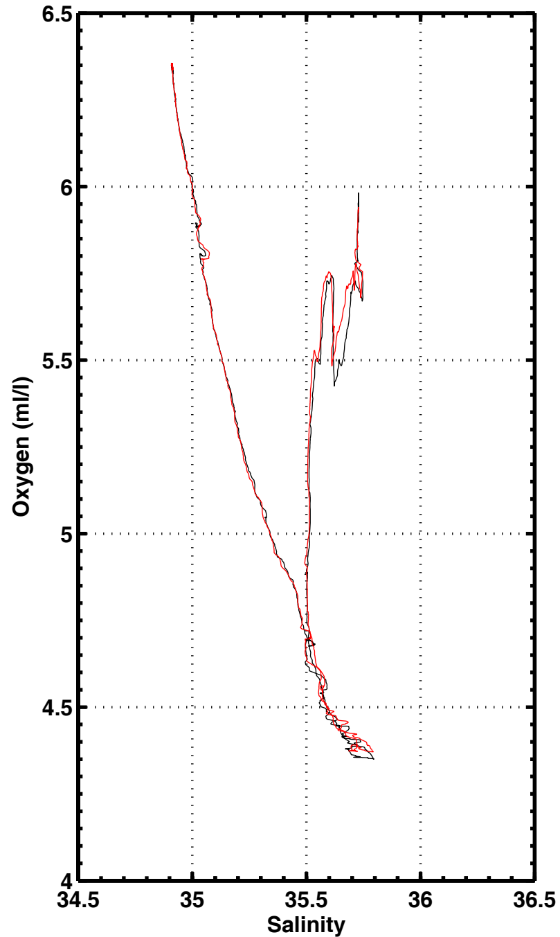
S-O2 , station 2012
