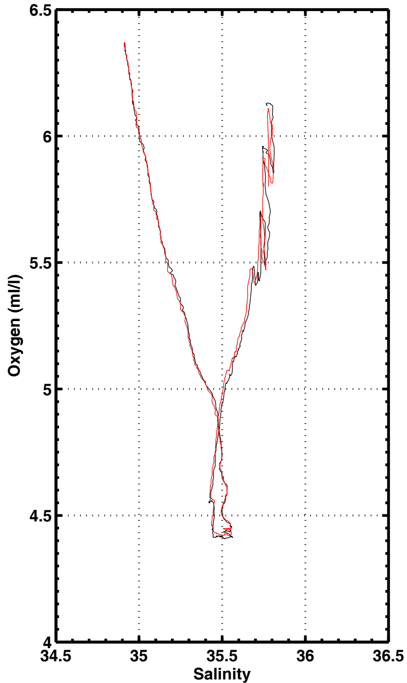
S-02 , station 2066
