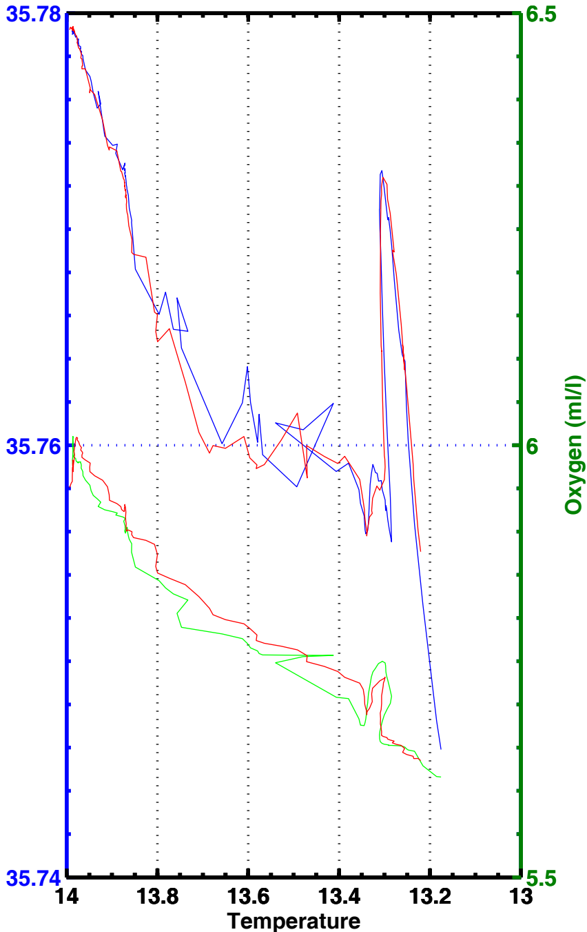
T-S , T-02 , station 2403
