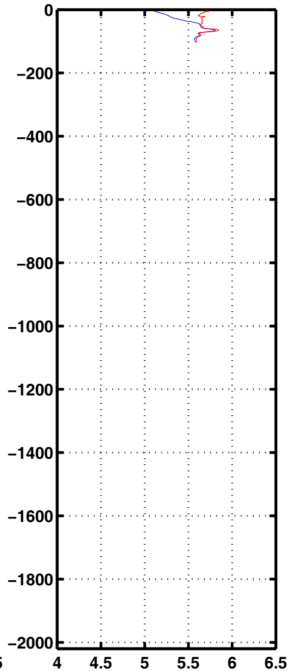
Oxyg 2090
