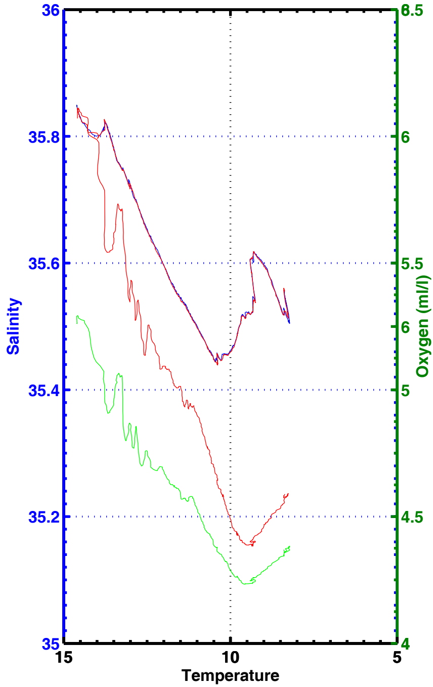
T-S , T-02 , station 2175
