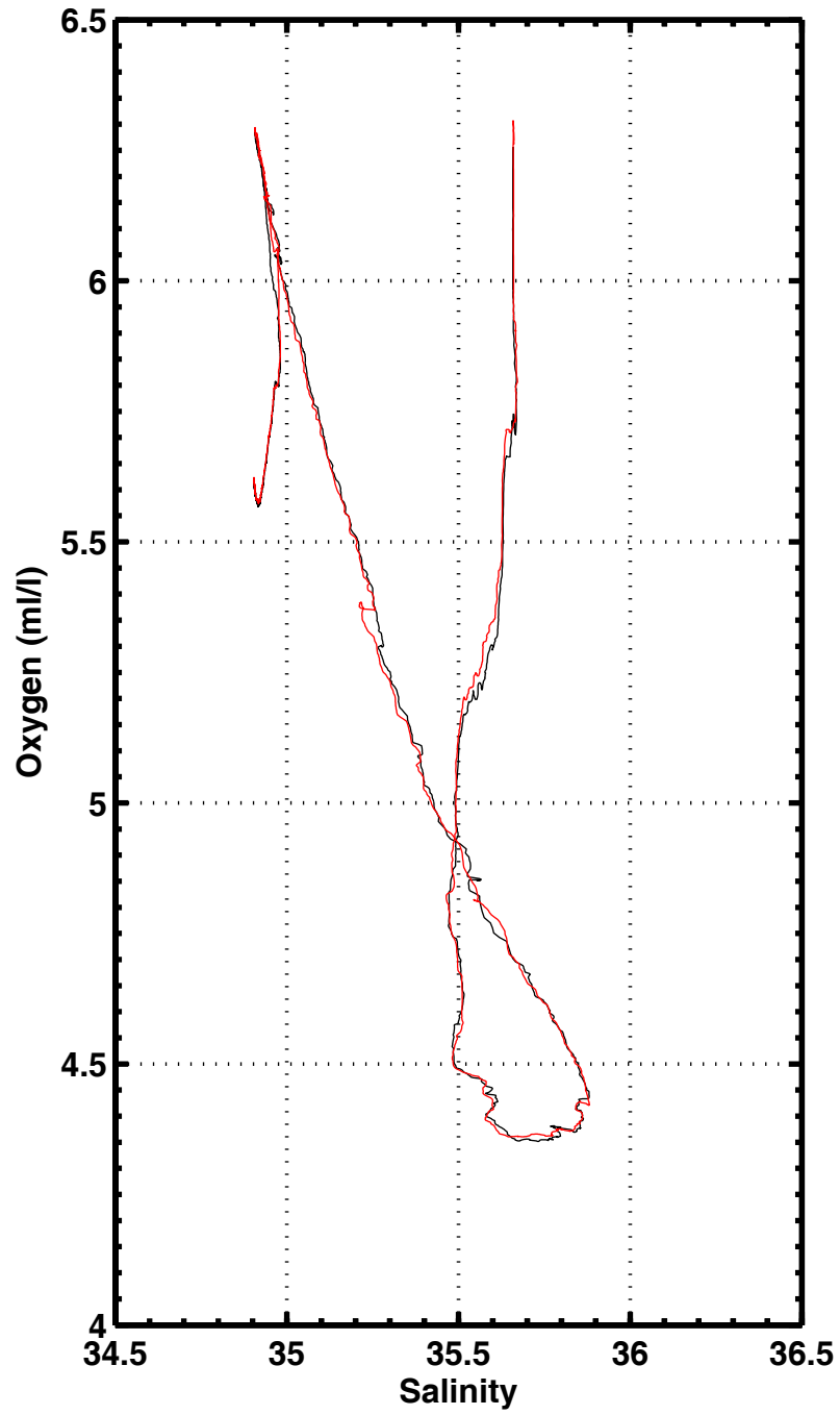
S-O2 , station 2009
