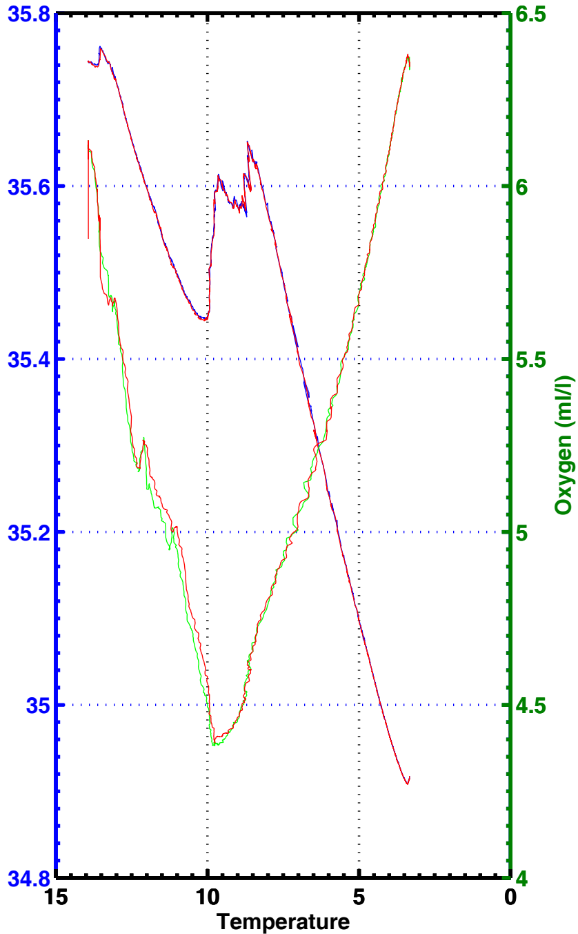
T-S , T-02 , station 2059
