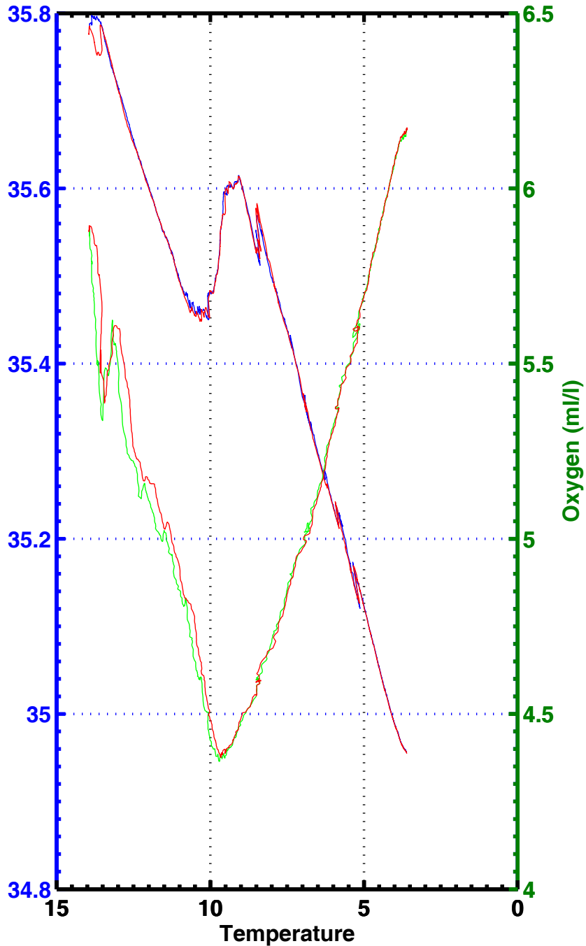
T-S , T-02 , station 2050
