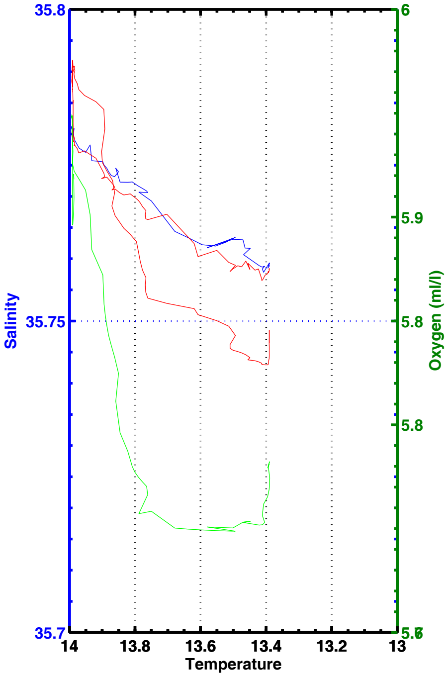
T-S , T-02 , station 2415
