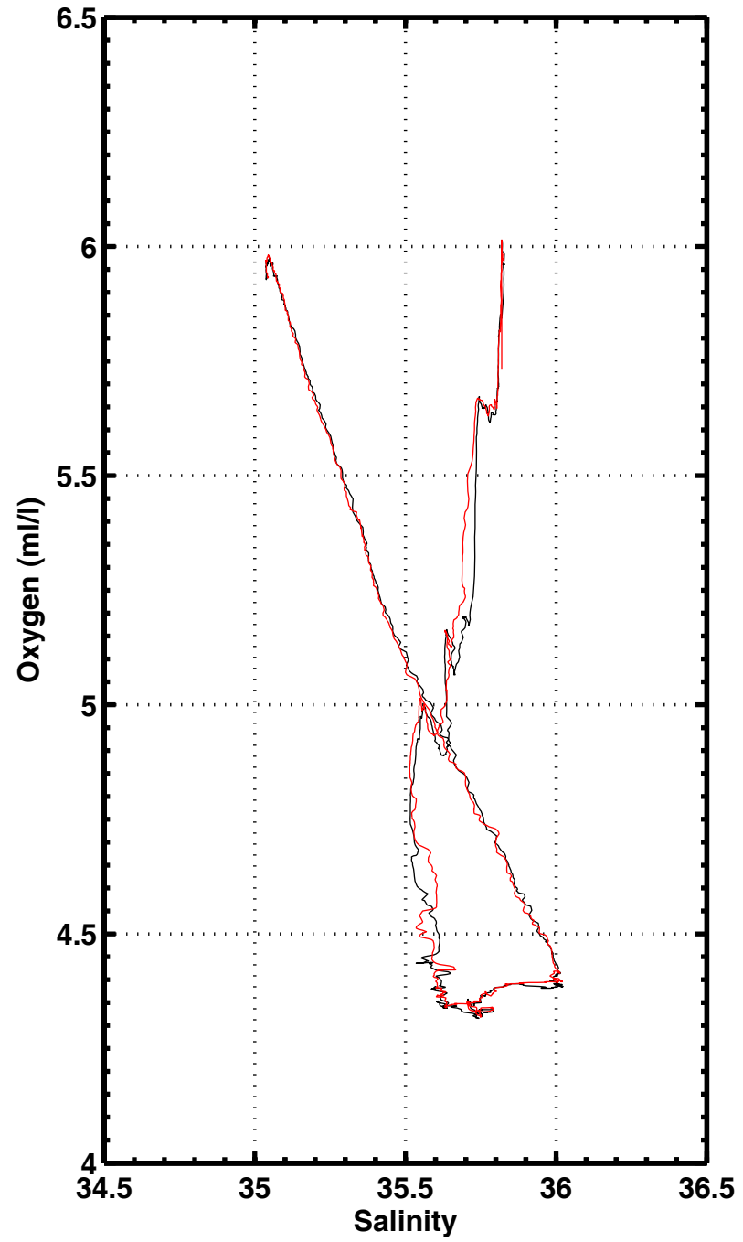
S-O2 , station 2035
