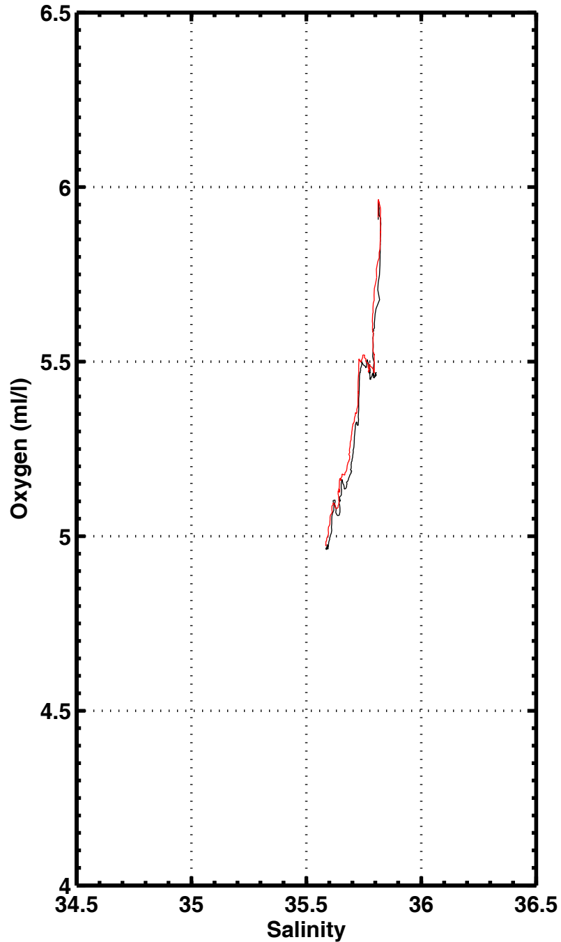
S-02, station 2271
