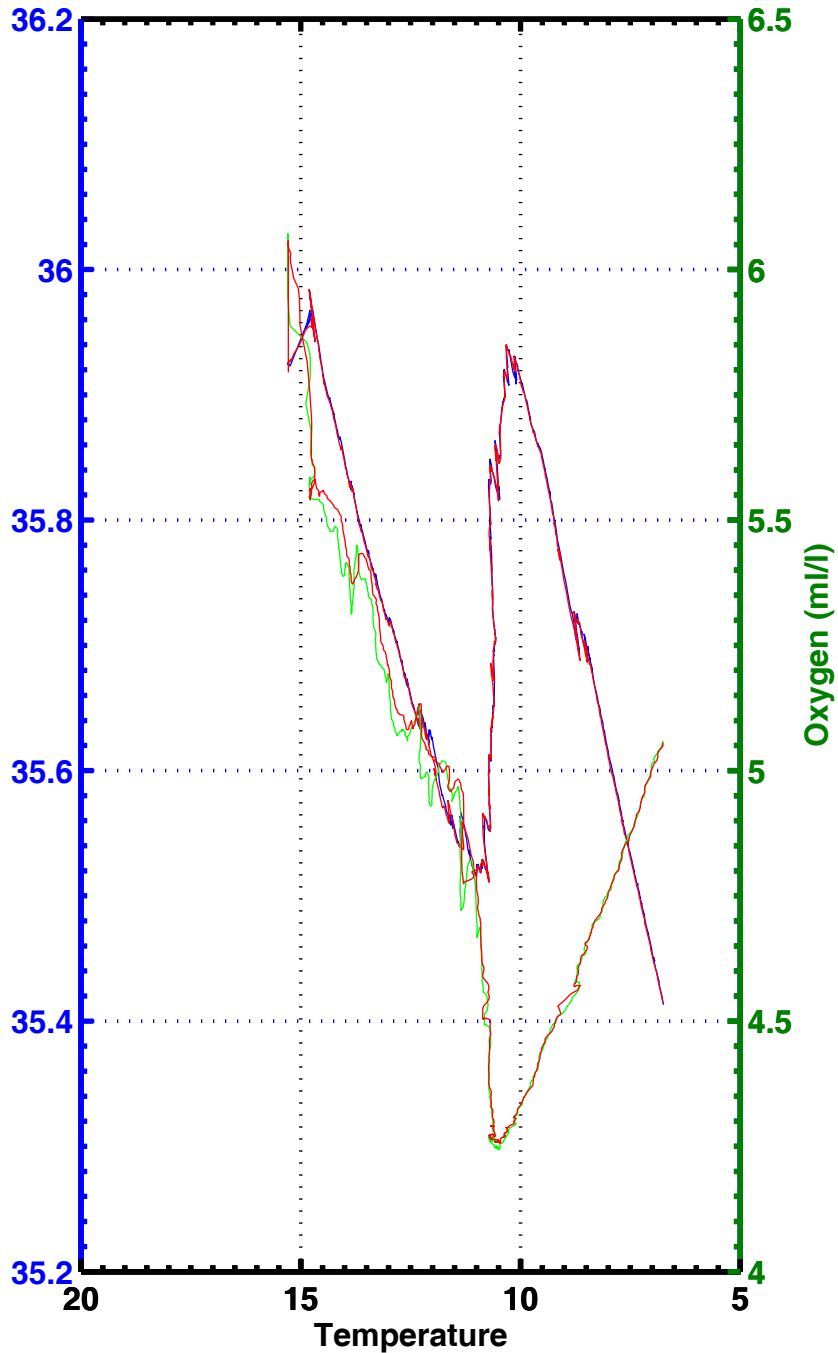
T-S , T-02 , station 2084
