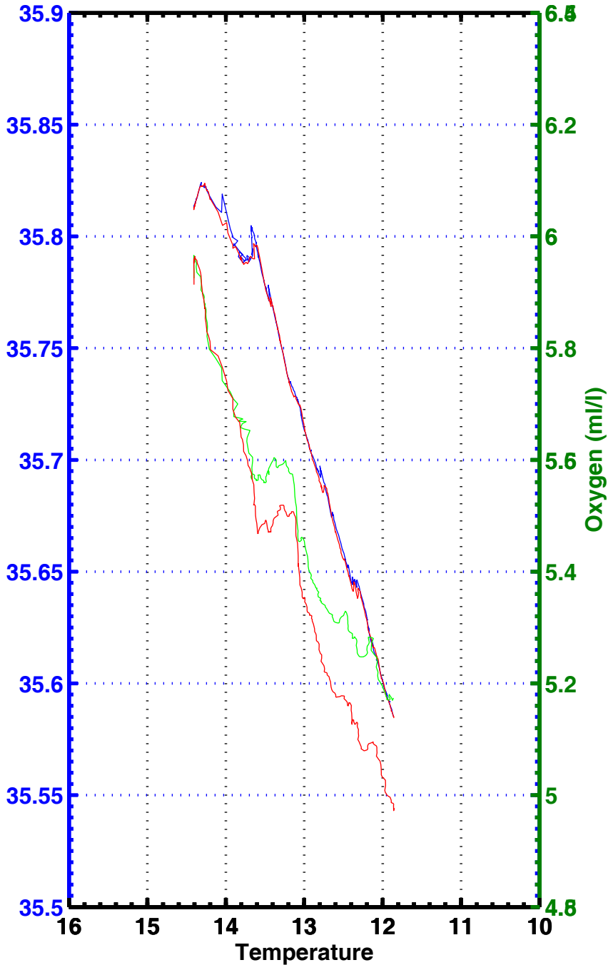
T-S, T-02, station 2271
