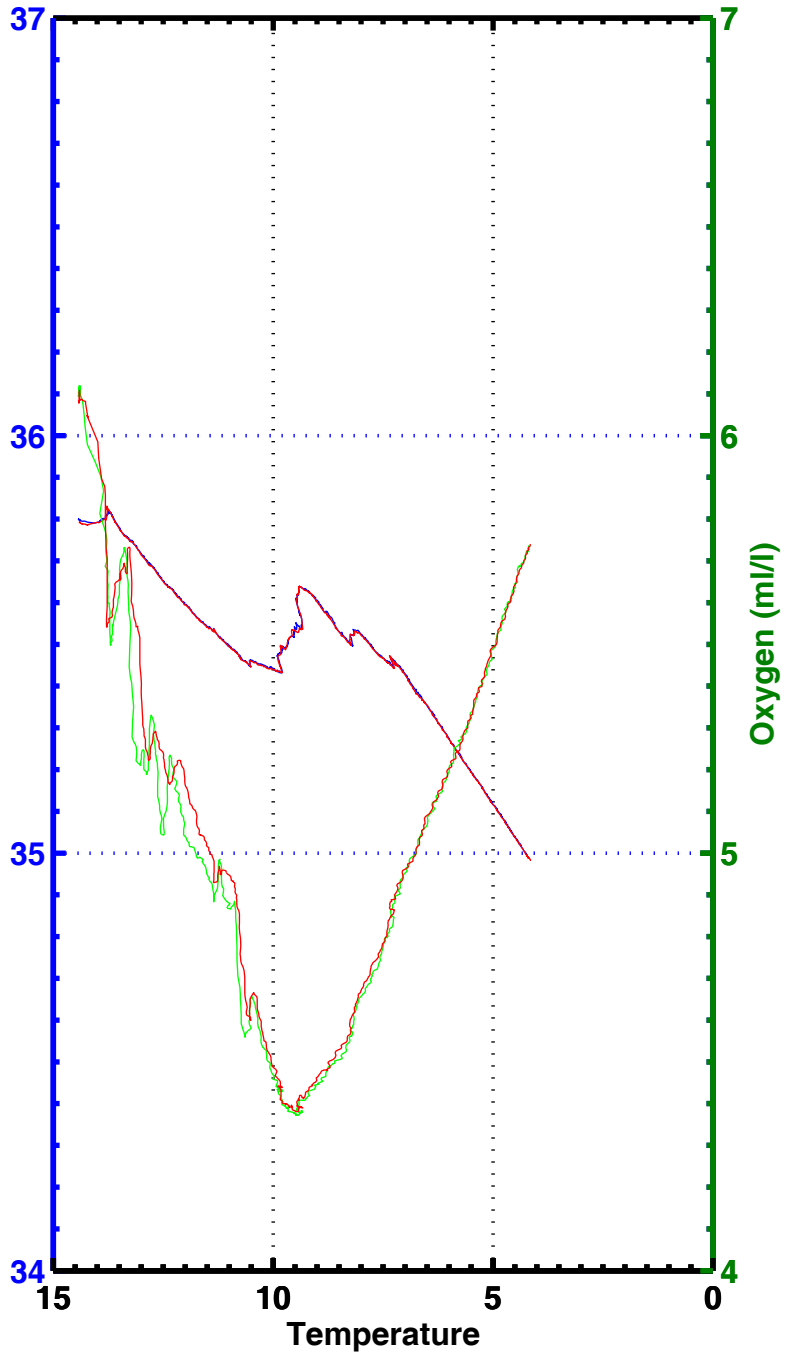
T-S , T-02 , station 2171
