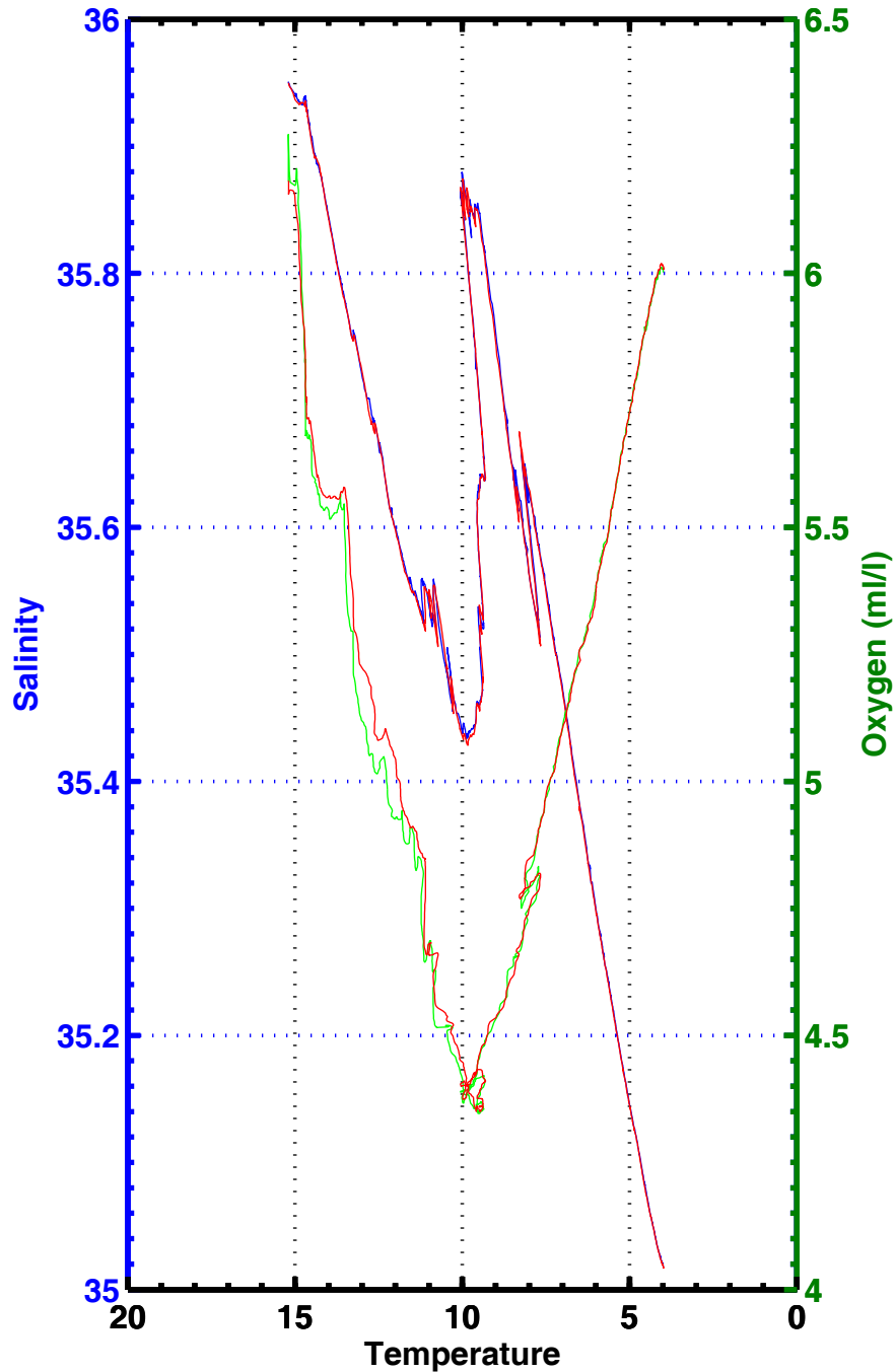
T-S , T-02 , station 2074
