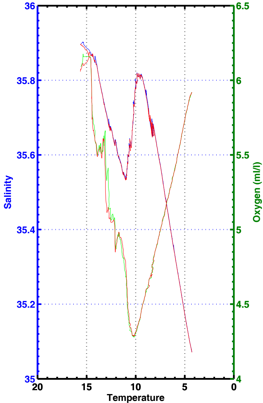
T-S , T-02 , station 2080
