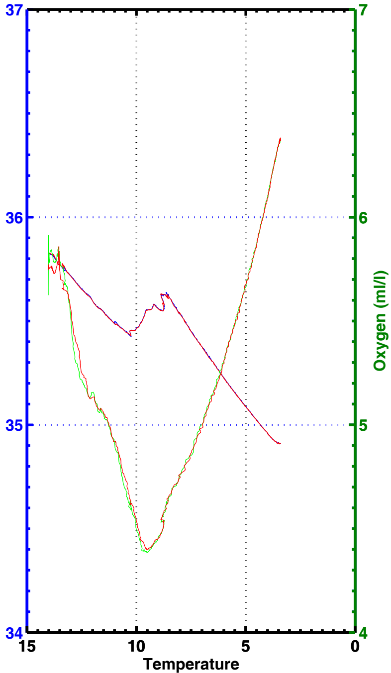
T-S , T-02 , station 2054
