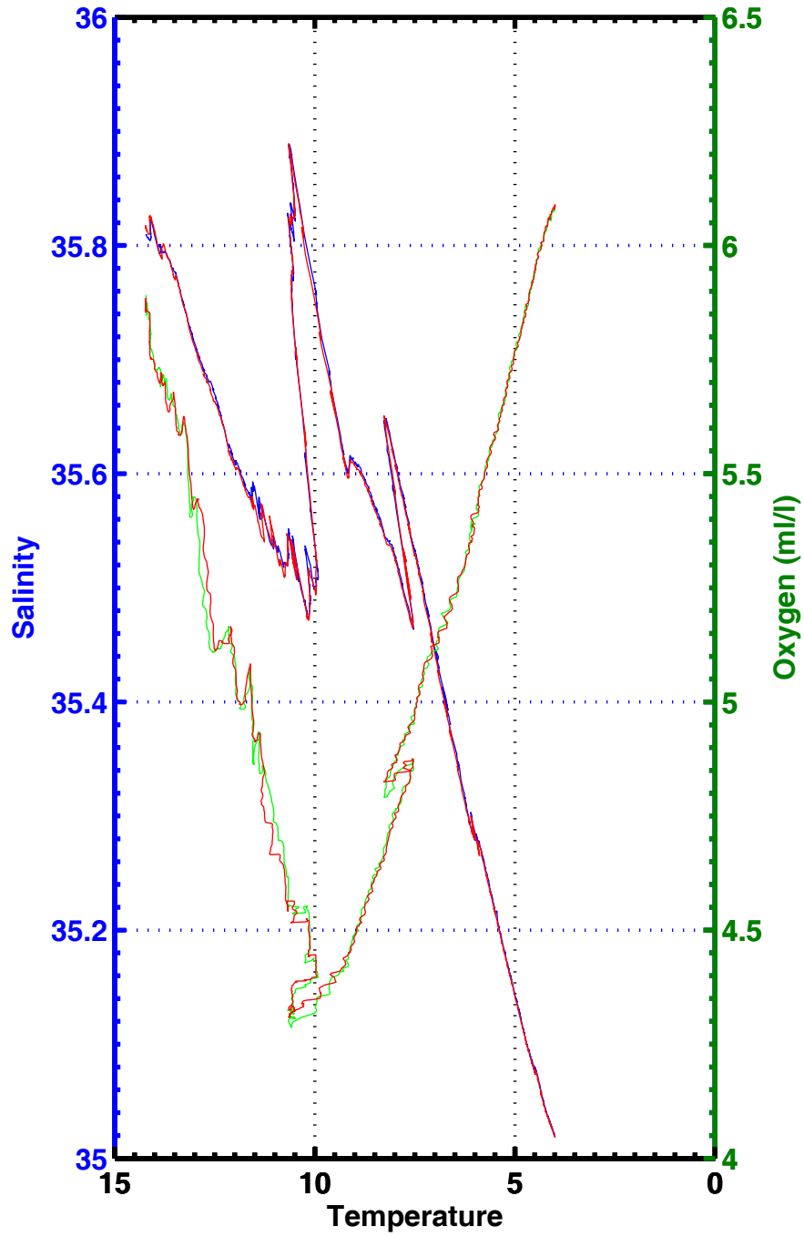
T-S , T-02 , station 2028
