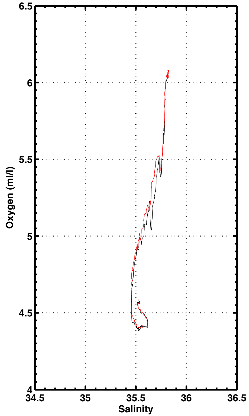
S-O2 , station 2182
