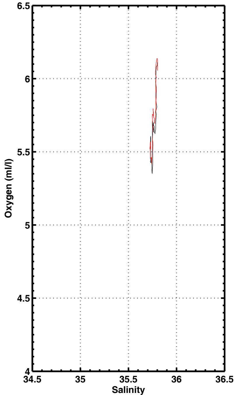
S-O2 , station 2181
