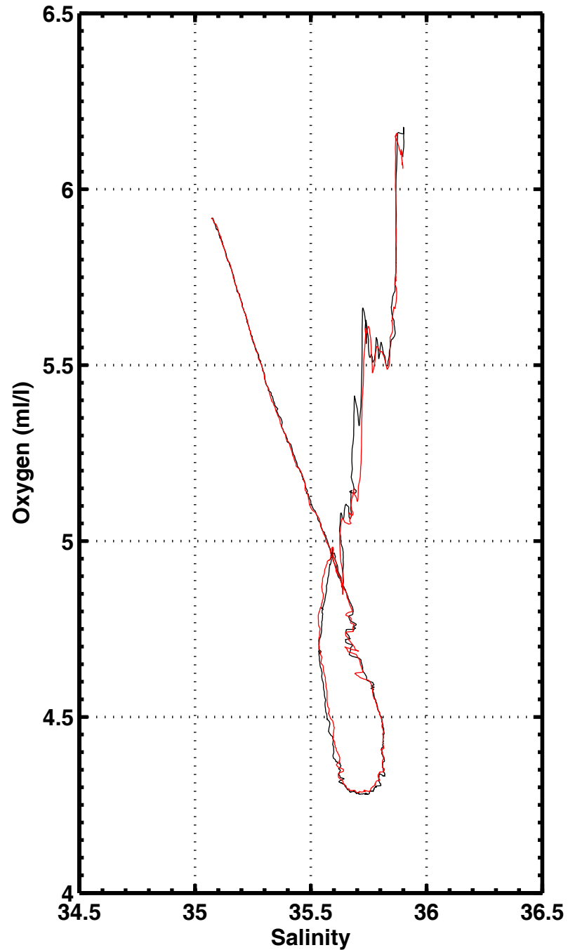
S-O2 , station 2080
