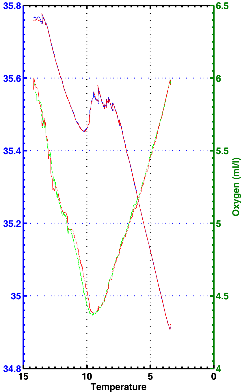
T-S , T-02 , station 2184
