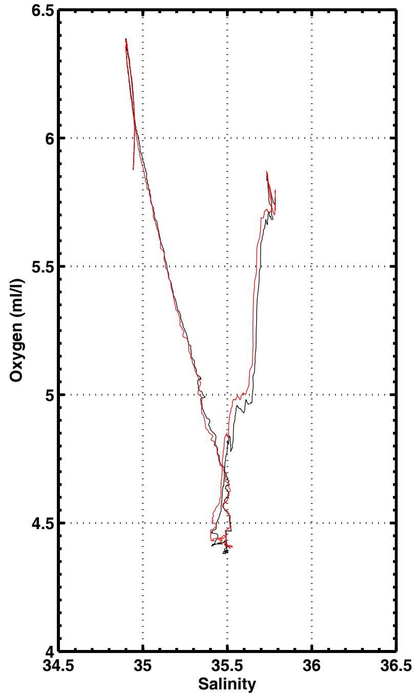
S-02 , station 2046
