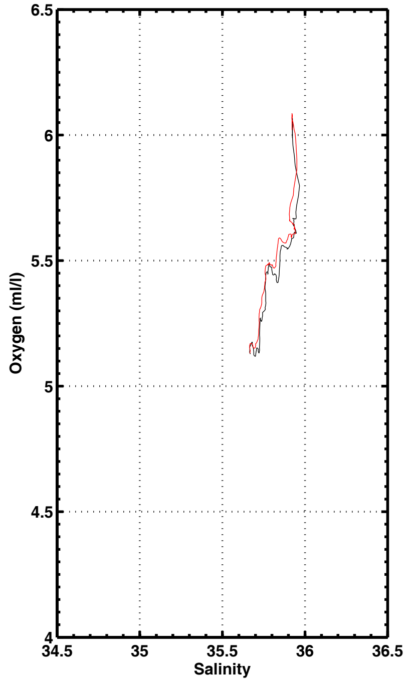
S-02 , station 2091
