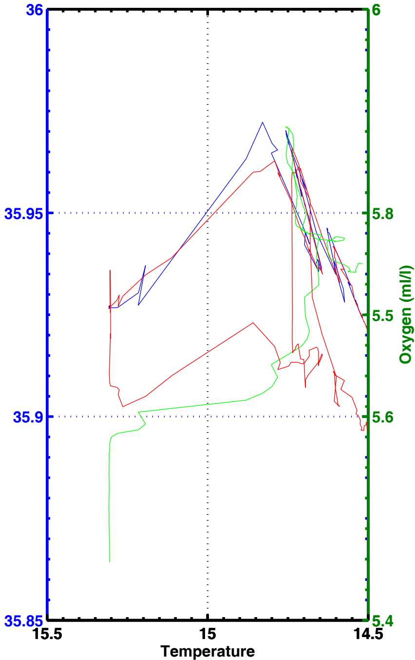
T-S , T-02 , station 2090
