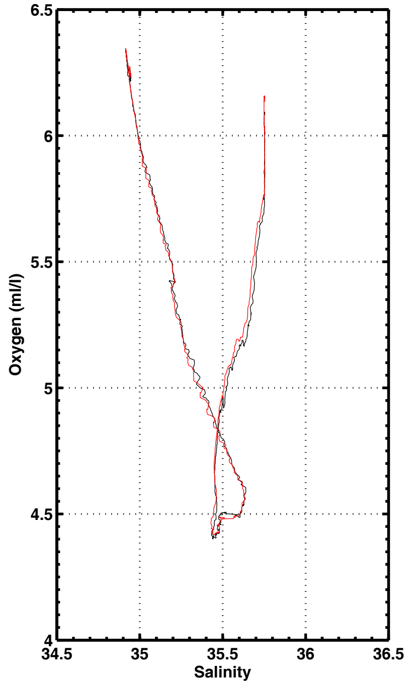
S-O2 , station 2063
