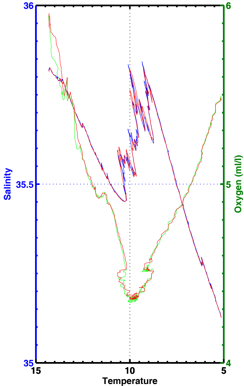
T-S , T-02 , station 2266
