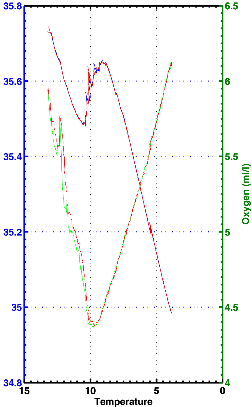
T-S , T-02 , station 2016
