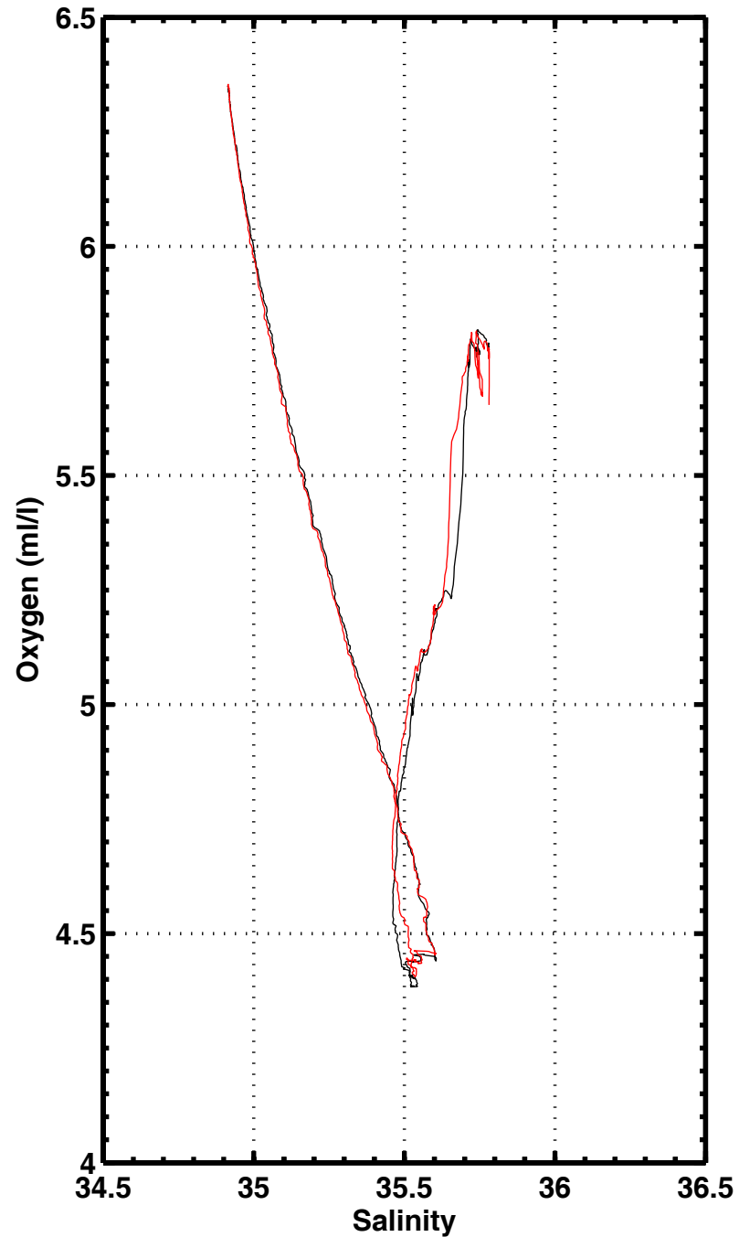
S-02 , station 1046
