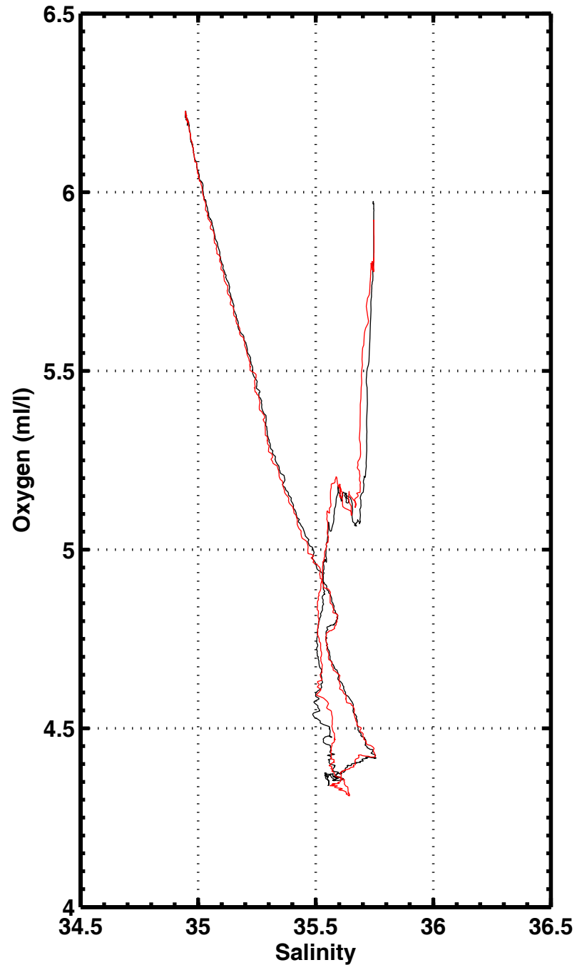
S-O2 , station 1039
