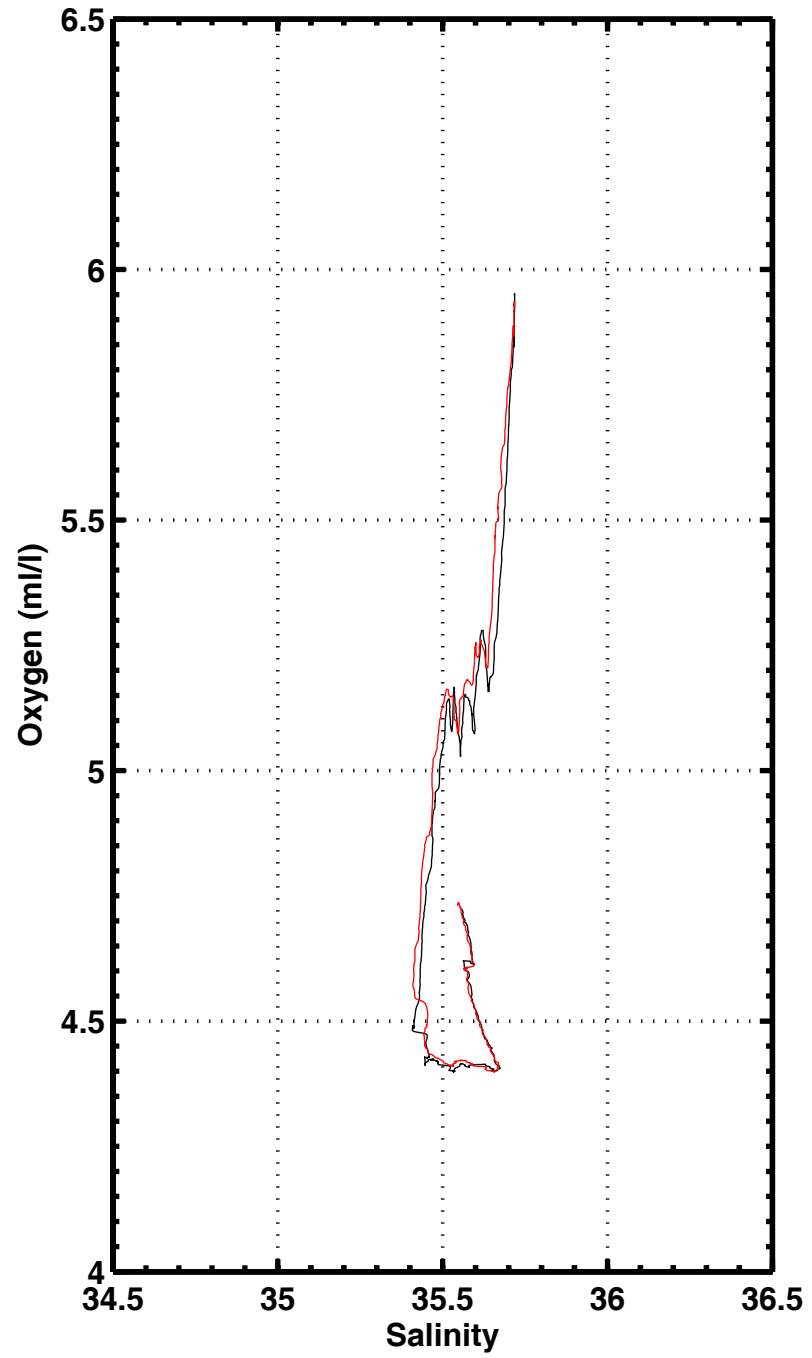
S-O2 , station 1134
