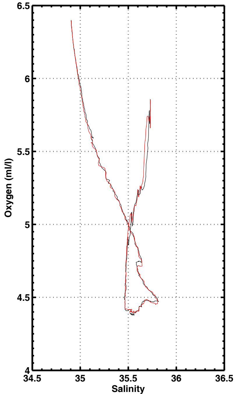
S-O2 , station 1043
