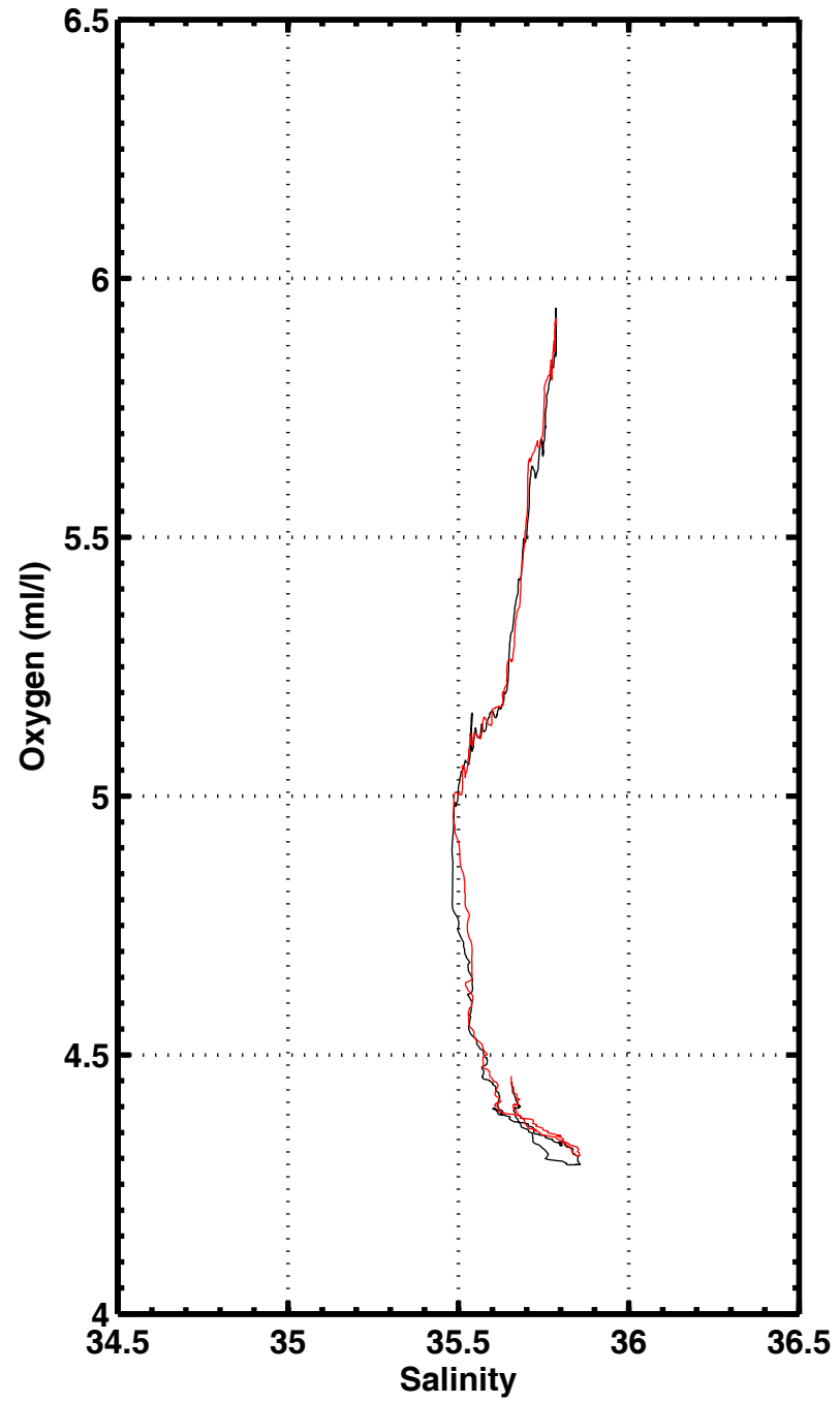
S-O2 , station 1196
