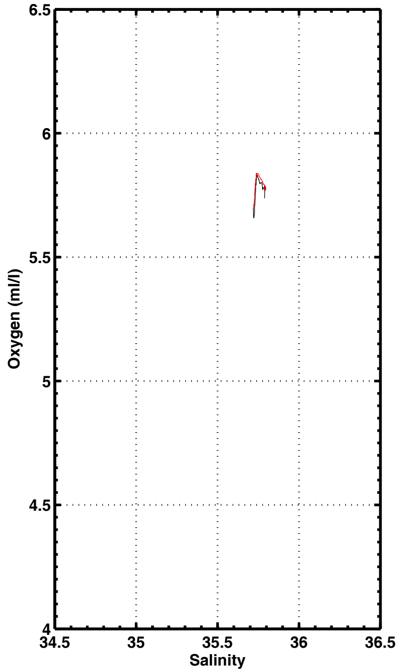
S-O2 , station 1112
