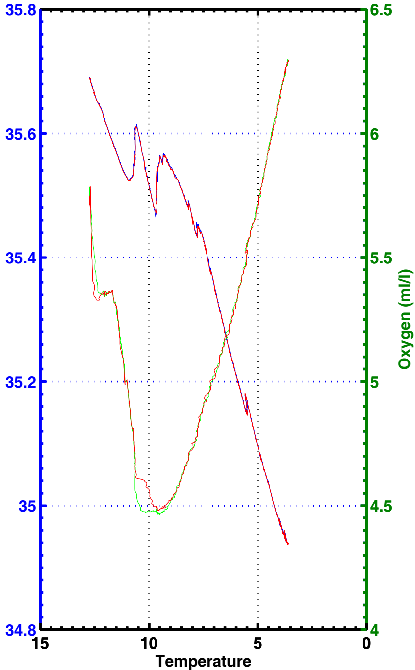
T-S , T-02 , station 1013
