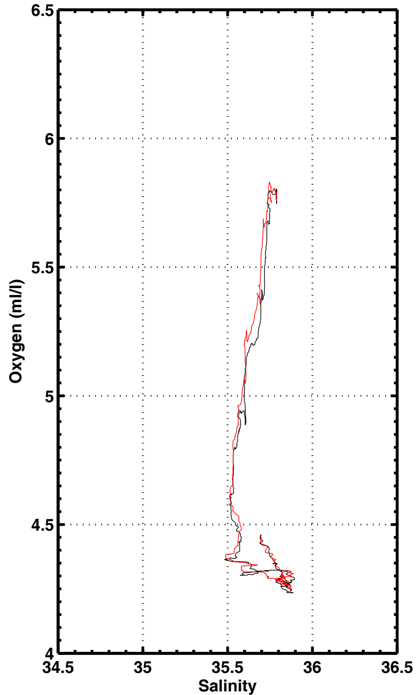
S-O2 , station 1113
