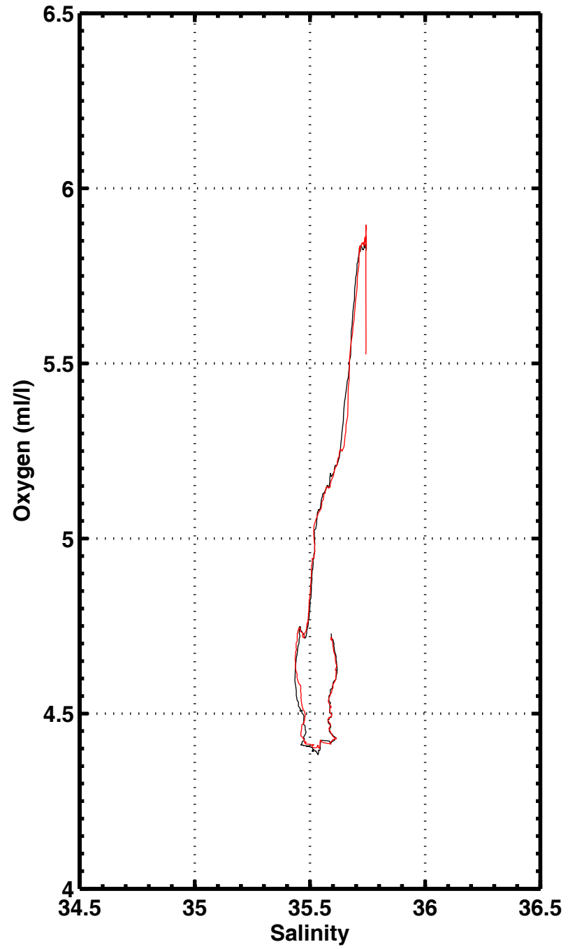
S-O2 , station 1132
