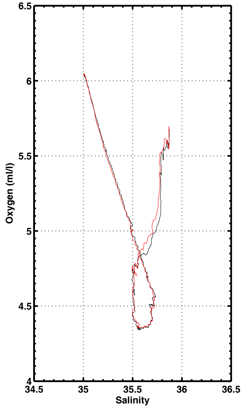
S-02 , station 1029
