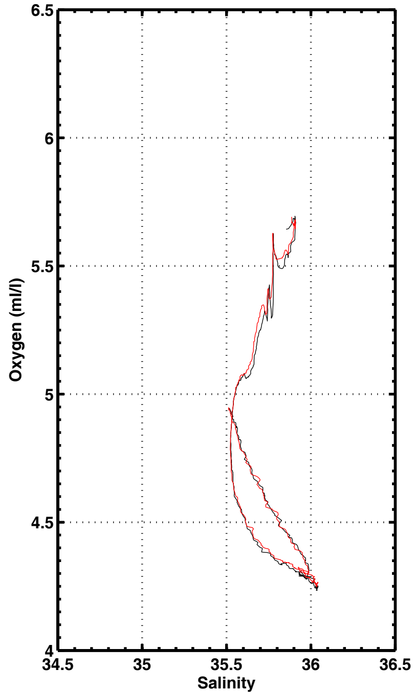
S-02 , station 1083
