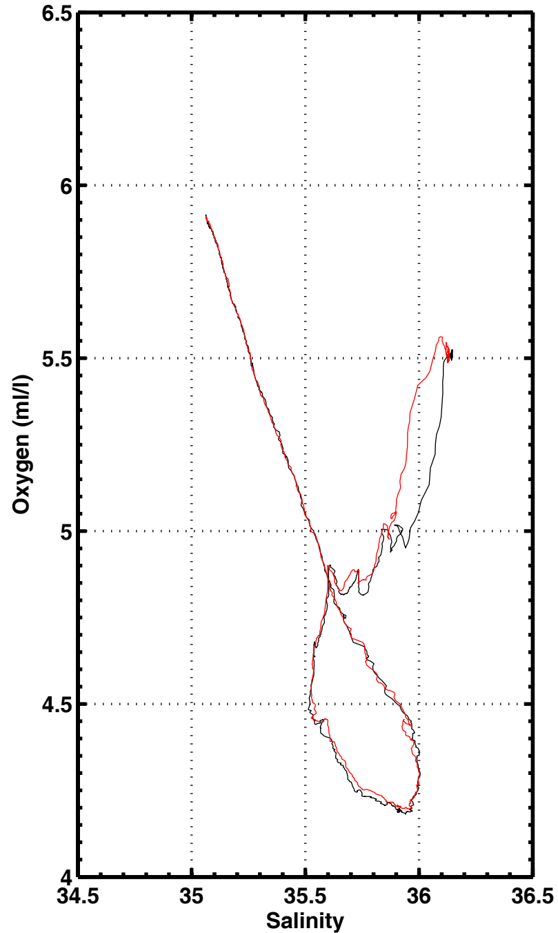
S-O2 , station 1077
