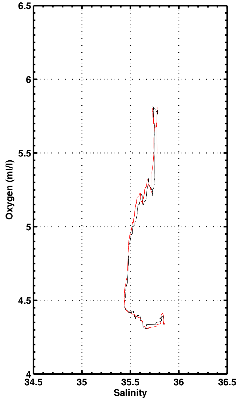
S-O2 , station 1157
