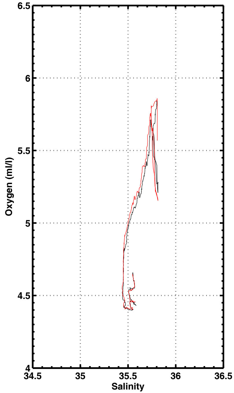
S-O2 , station 1153
