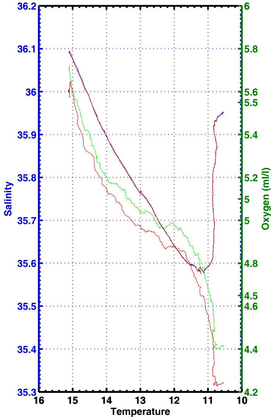
T-S , T-02 , station 1123
