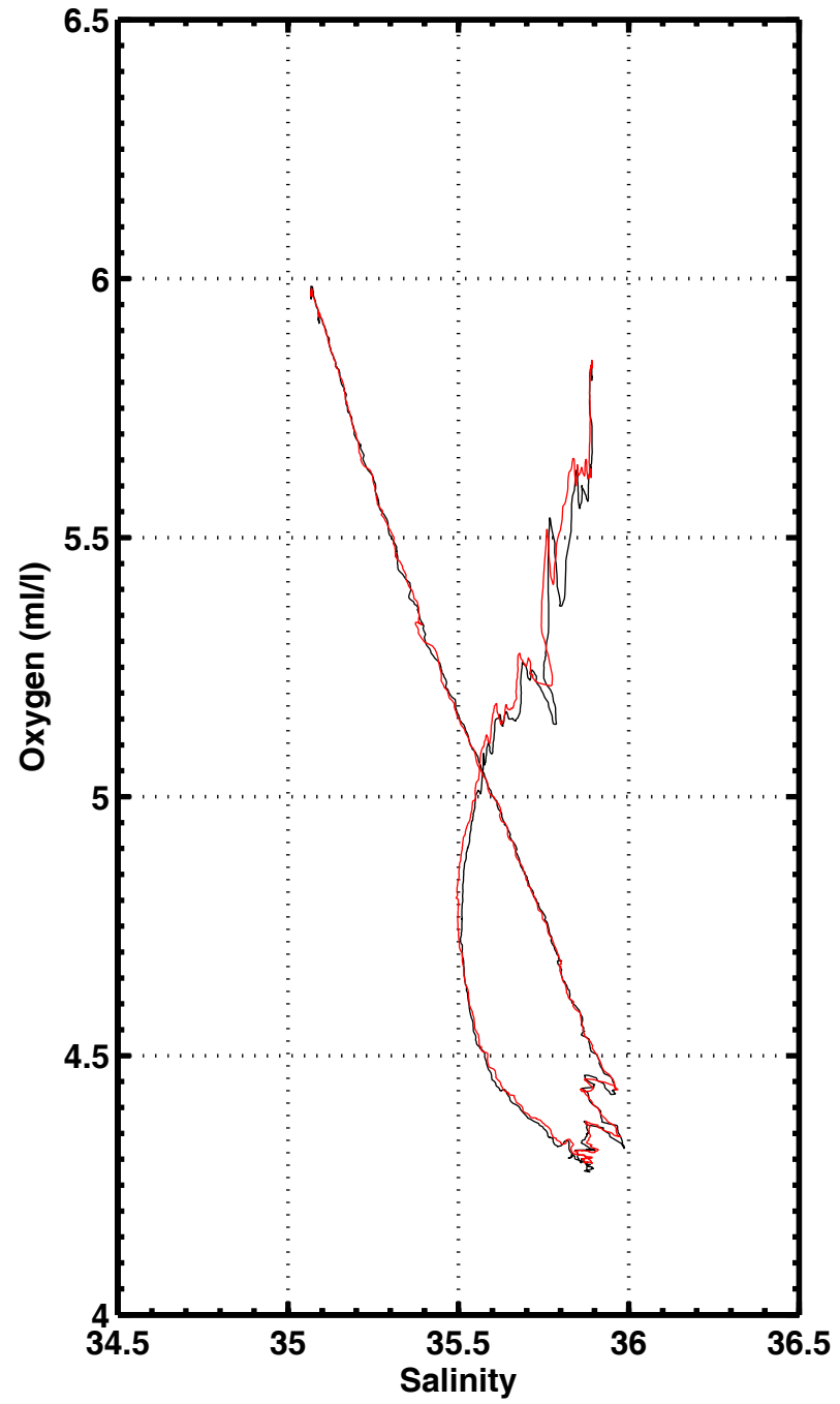
S-O2 , station 1053
