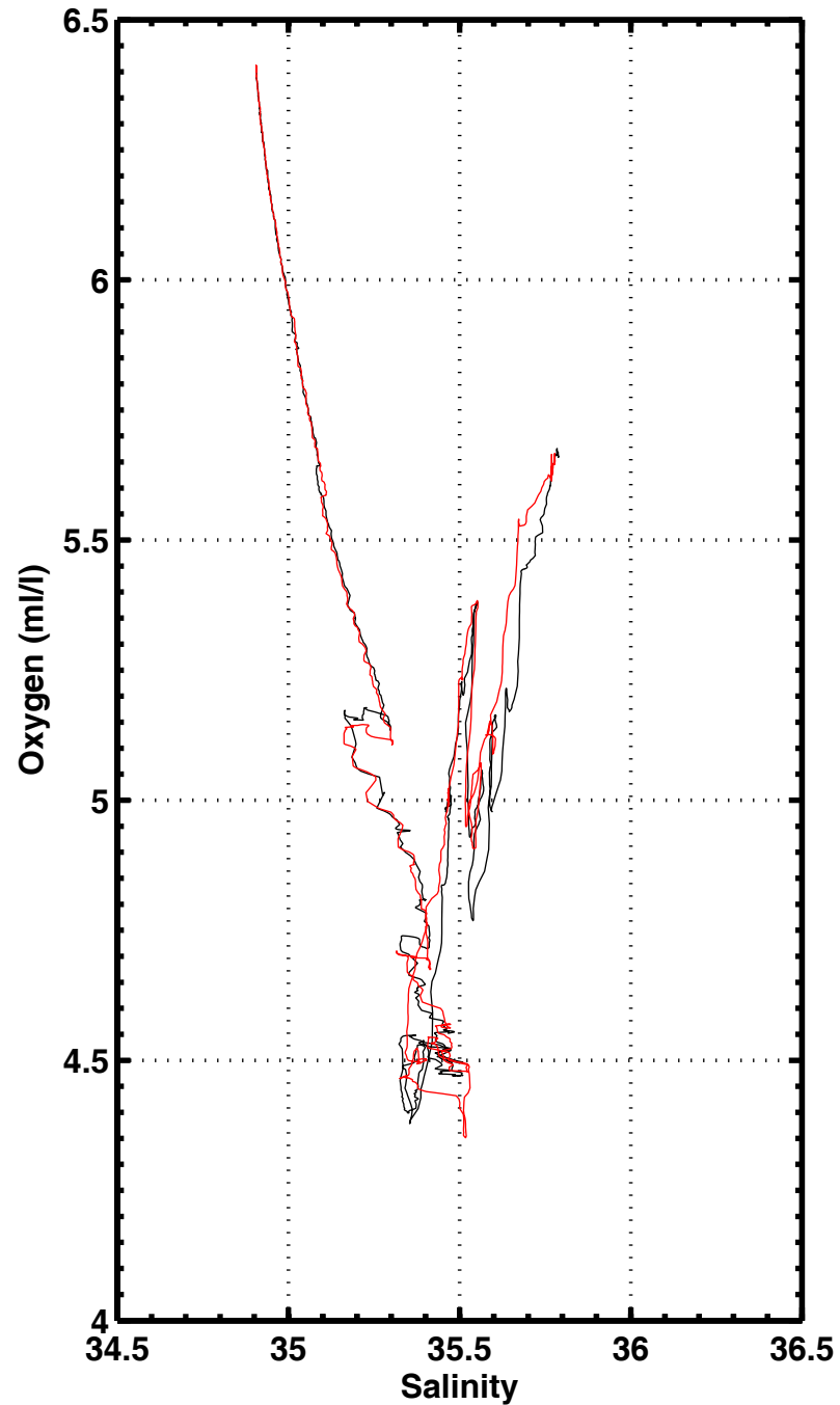
S-O2 , station 1016
