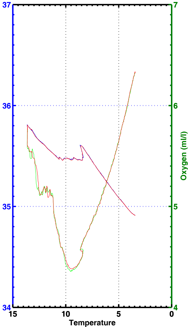
T-S , T-02 , station 1066
