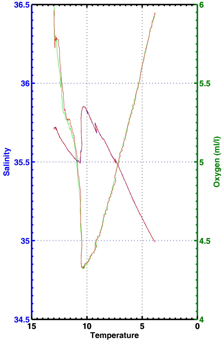
T-S , T-02 , station 1181
