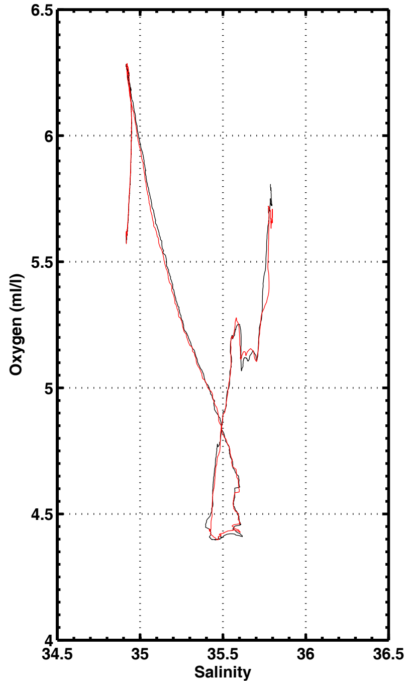
S-O2 , station 1045
