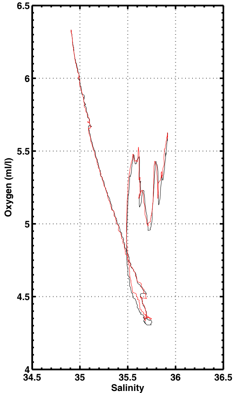
S-O2 , station 1071
