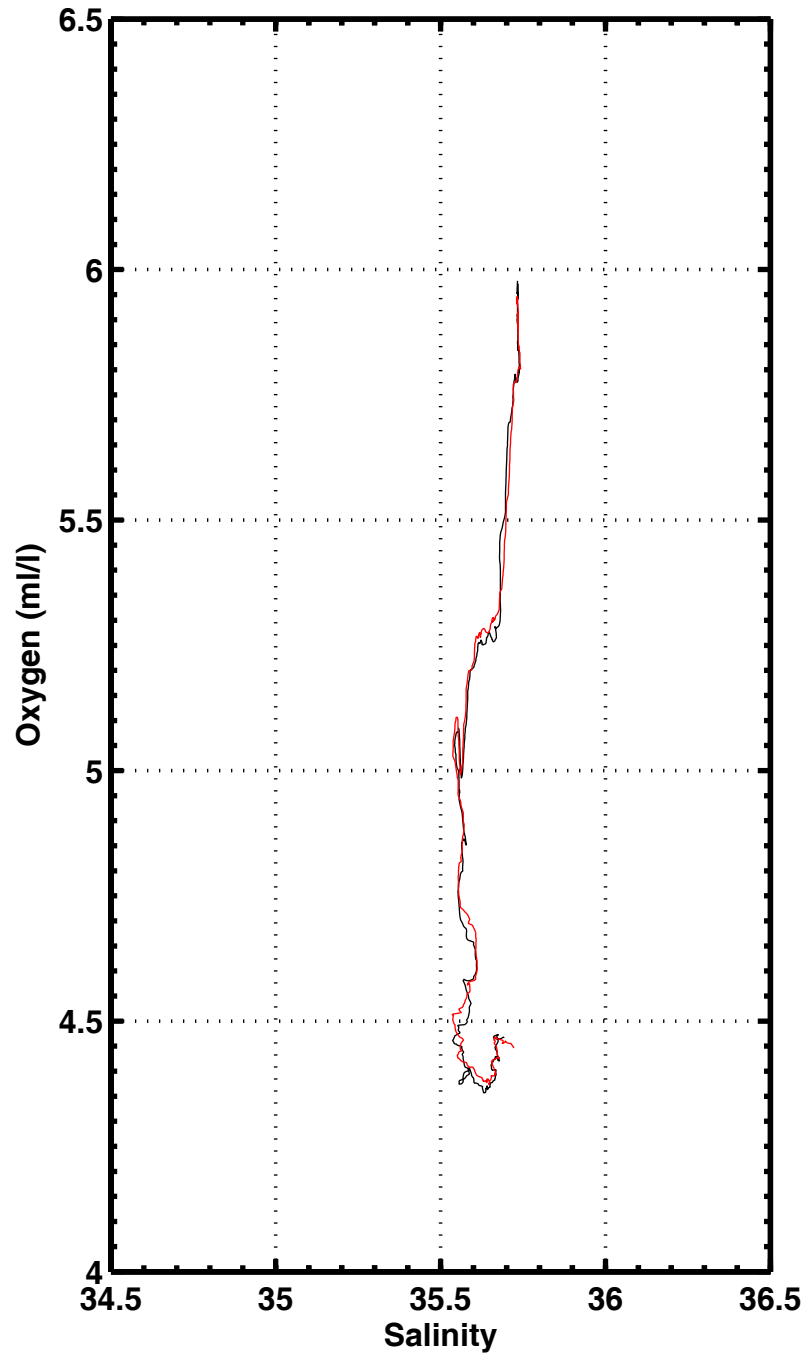
S-02 , station 1197
