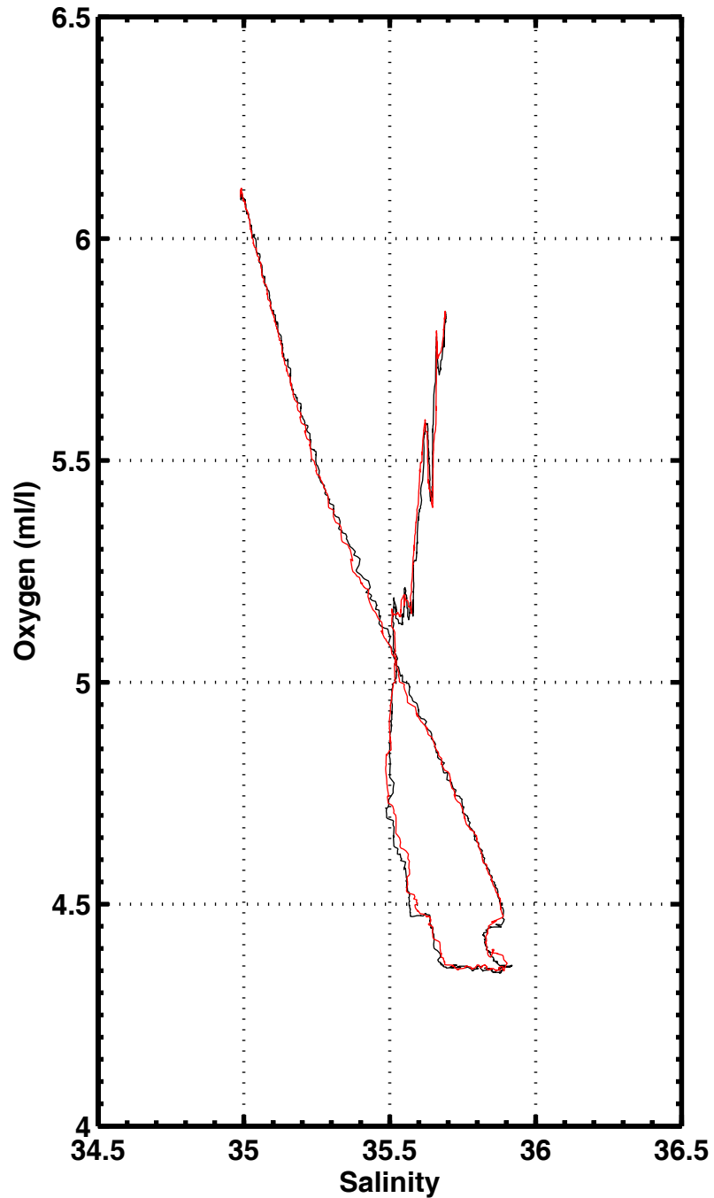
S-O2 , station 1008
