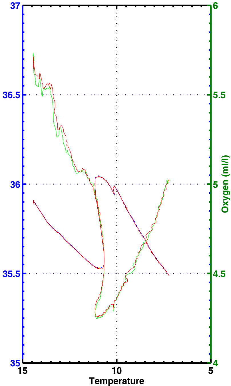
T-S , T-02 , station 1085
