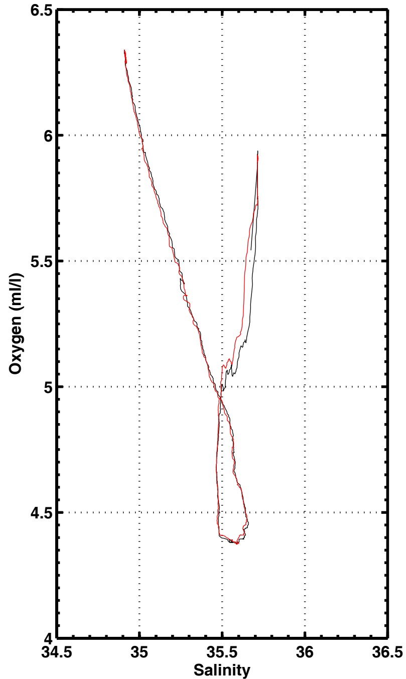
S-O2 , station 1063
