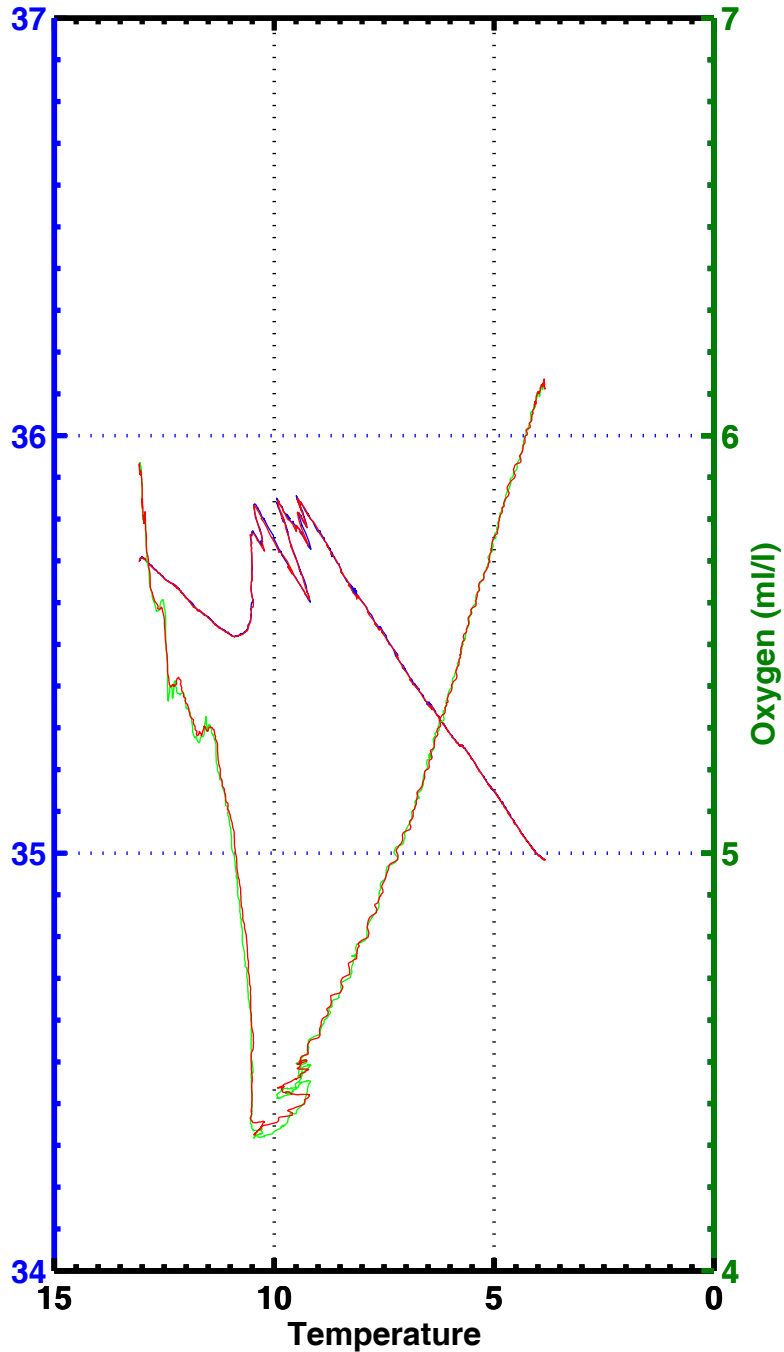
T-S , T-02 , station 1041
