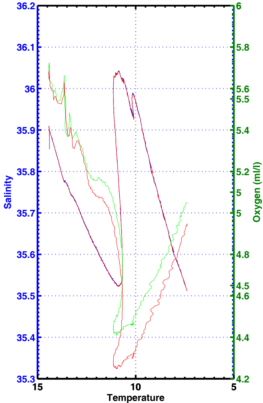
T-S , T-02 , station 1083
