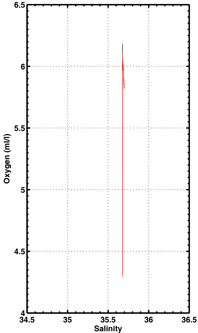
S-02 , station 1183
