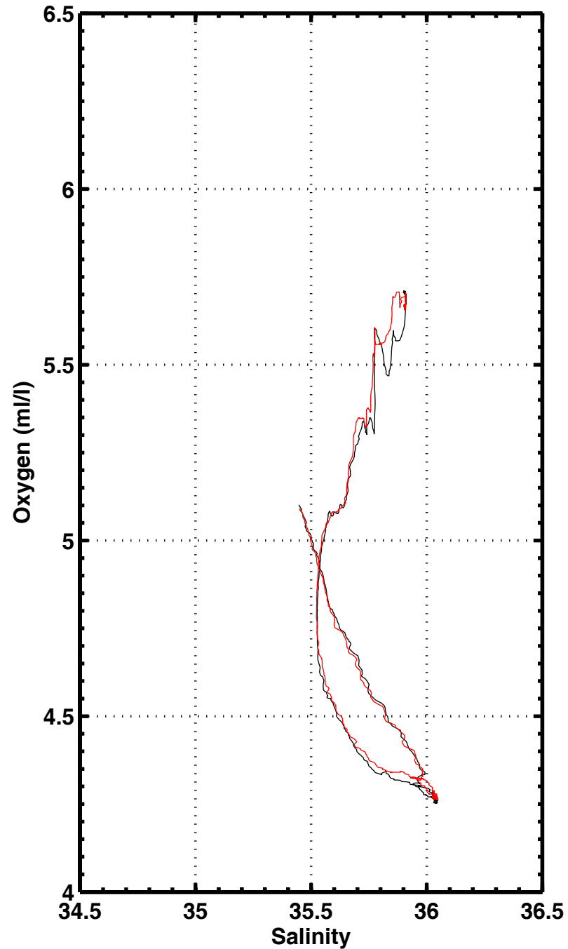
S-O2 , station 1082
