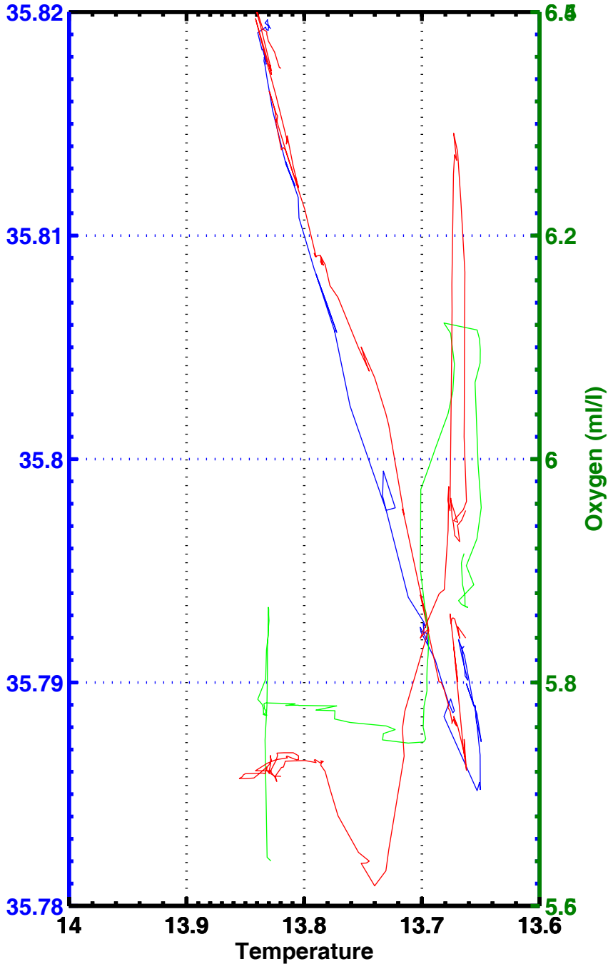
T-S , T-02 , station 1116
