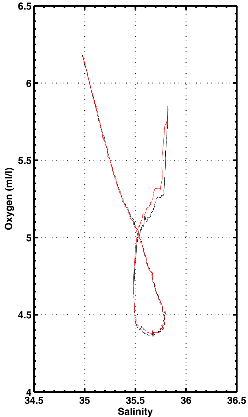
S-O2 , station 1030
