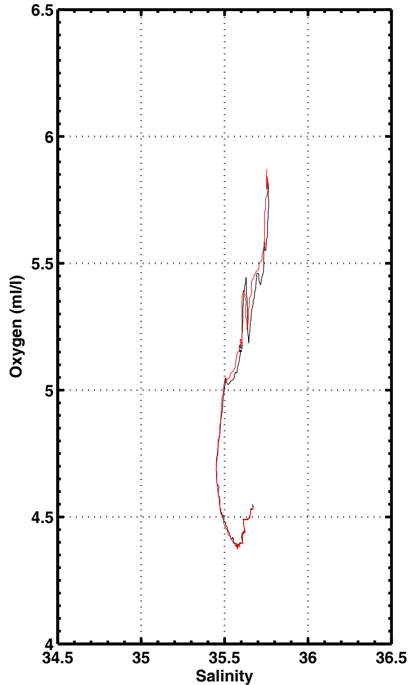
S-O2 , station 1130
