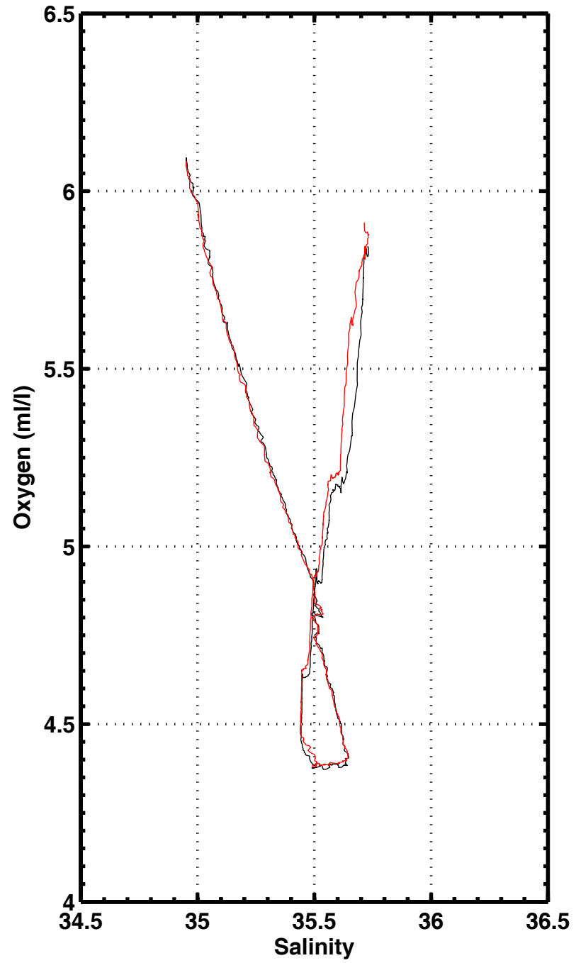
S-O2 , station 1139
