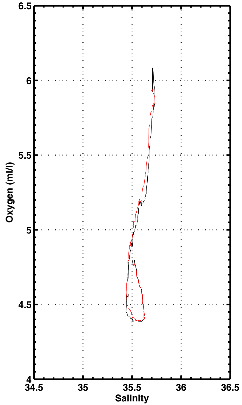
S-O2 , station 1142
