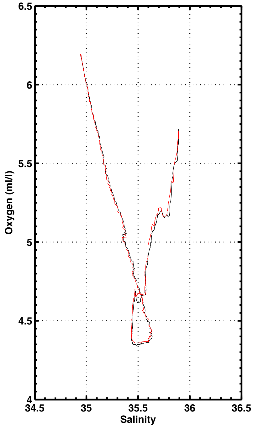
S-O2 , station 1072
