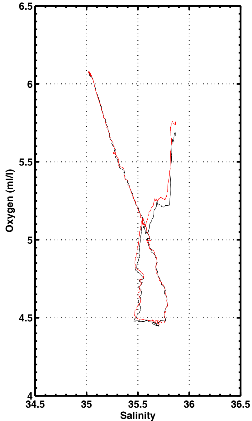
S-O2 , station 1001
