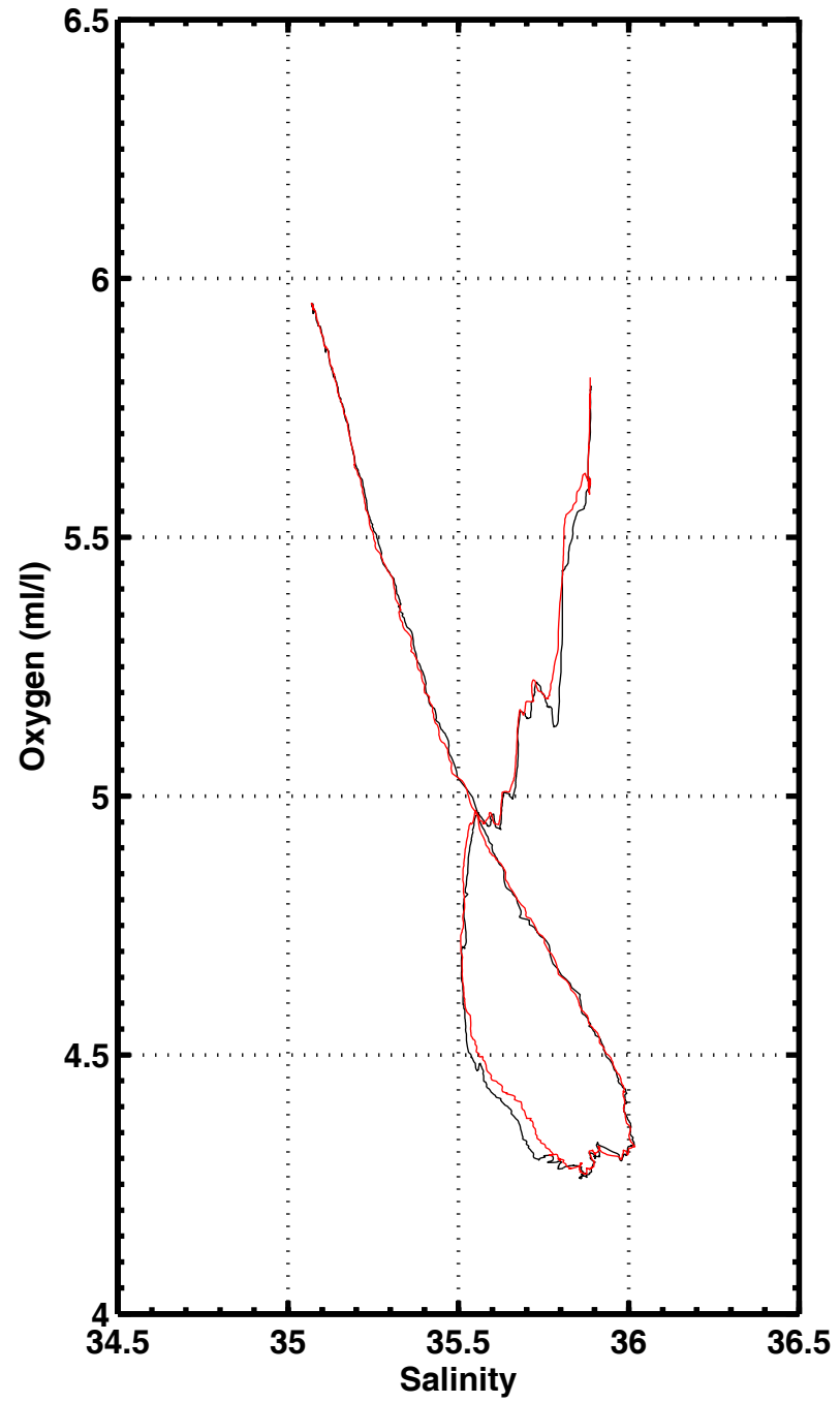
S-O2 , station 1059
