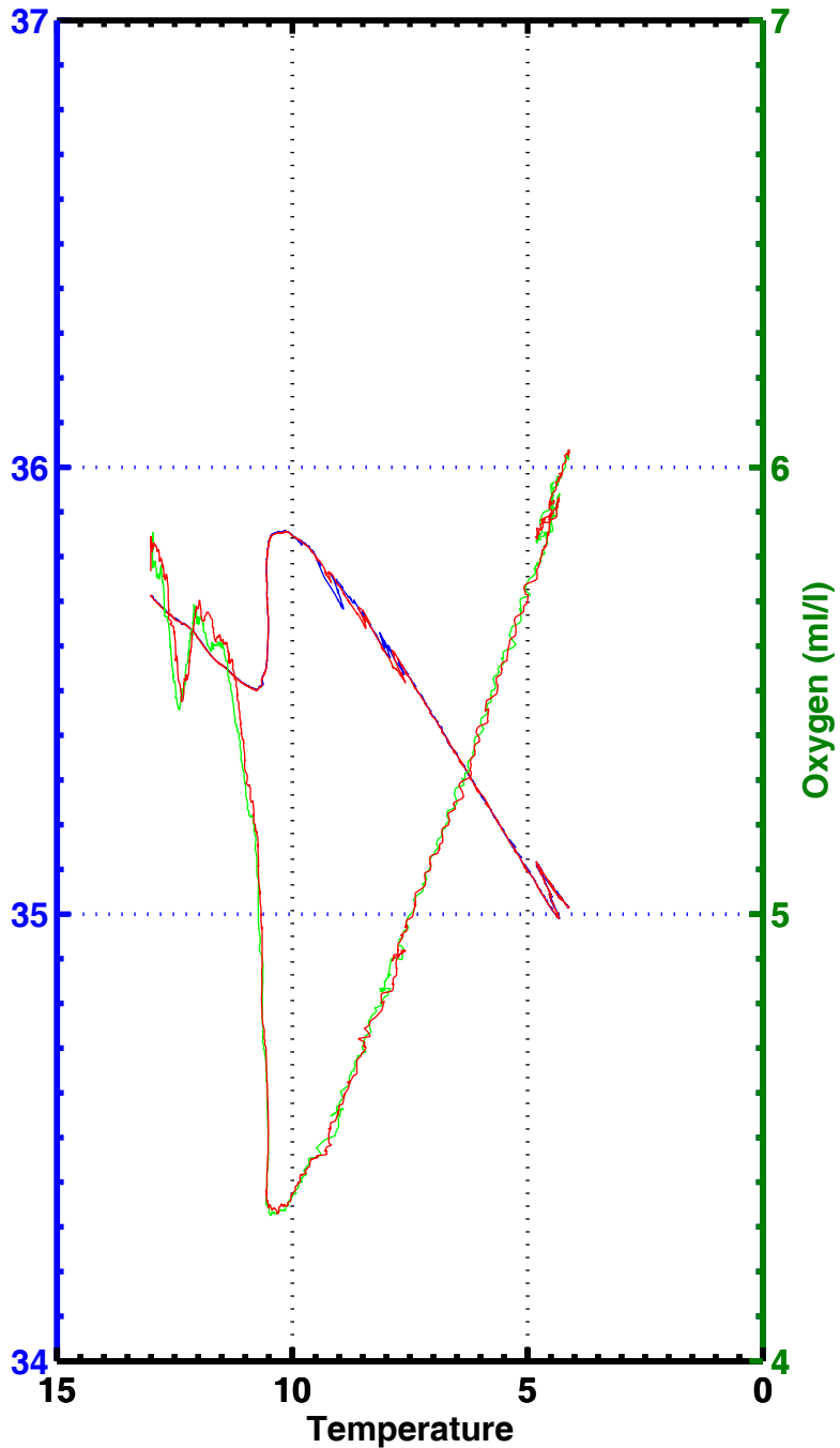
T-S , T-02 , station 1023
