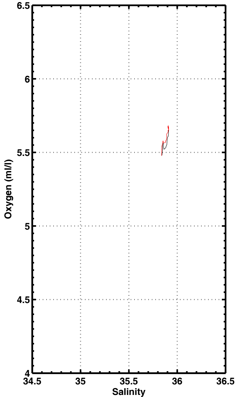
S-O2 , station 1081
