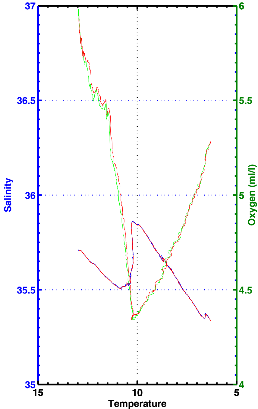
T-S , T-02 , station 1167
