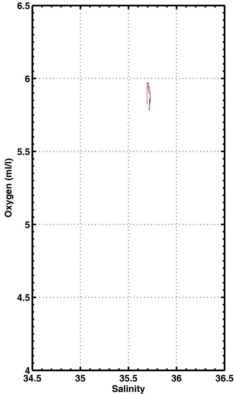
S-02 , station 1145
