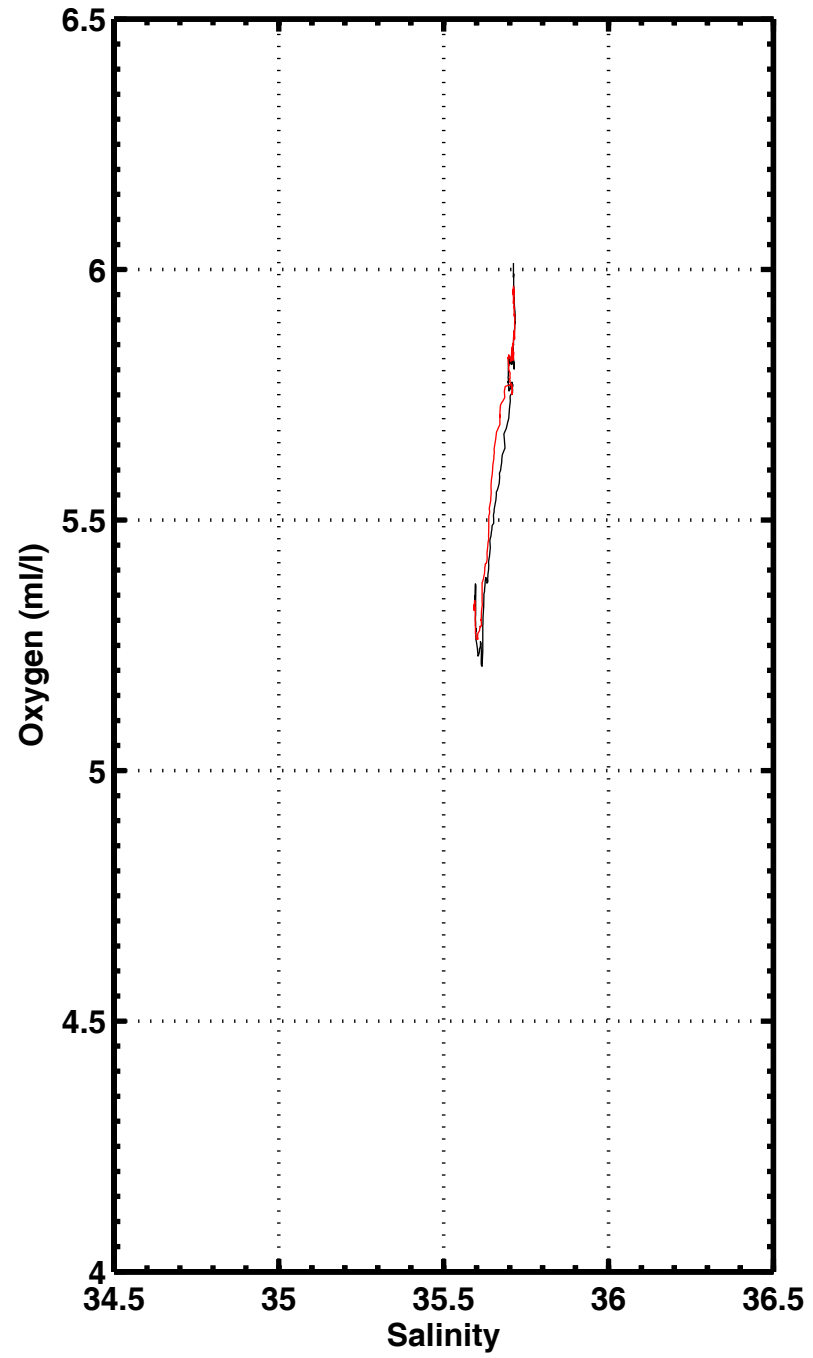
S-O2 , station 1173
