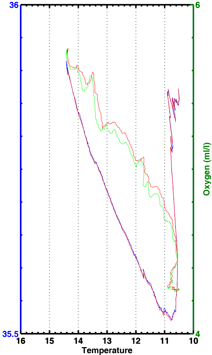
T-S , T-02 , station 1100
