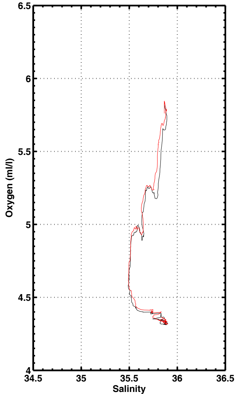
S-O2 , station 1206
