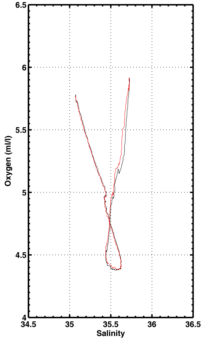
S-O2 , station 1140
