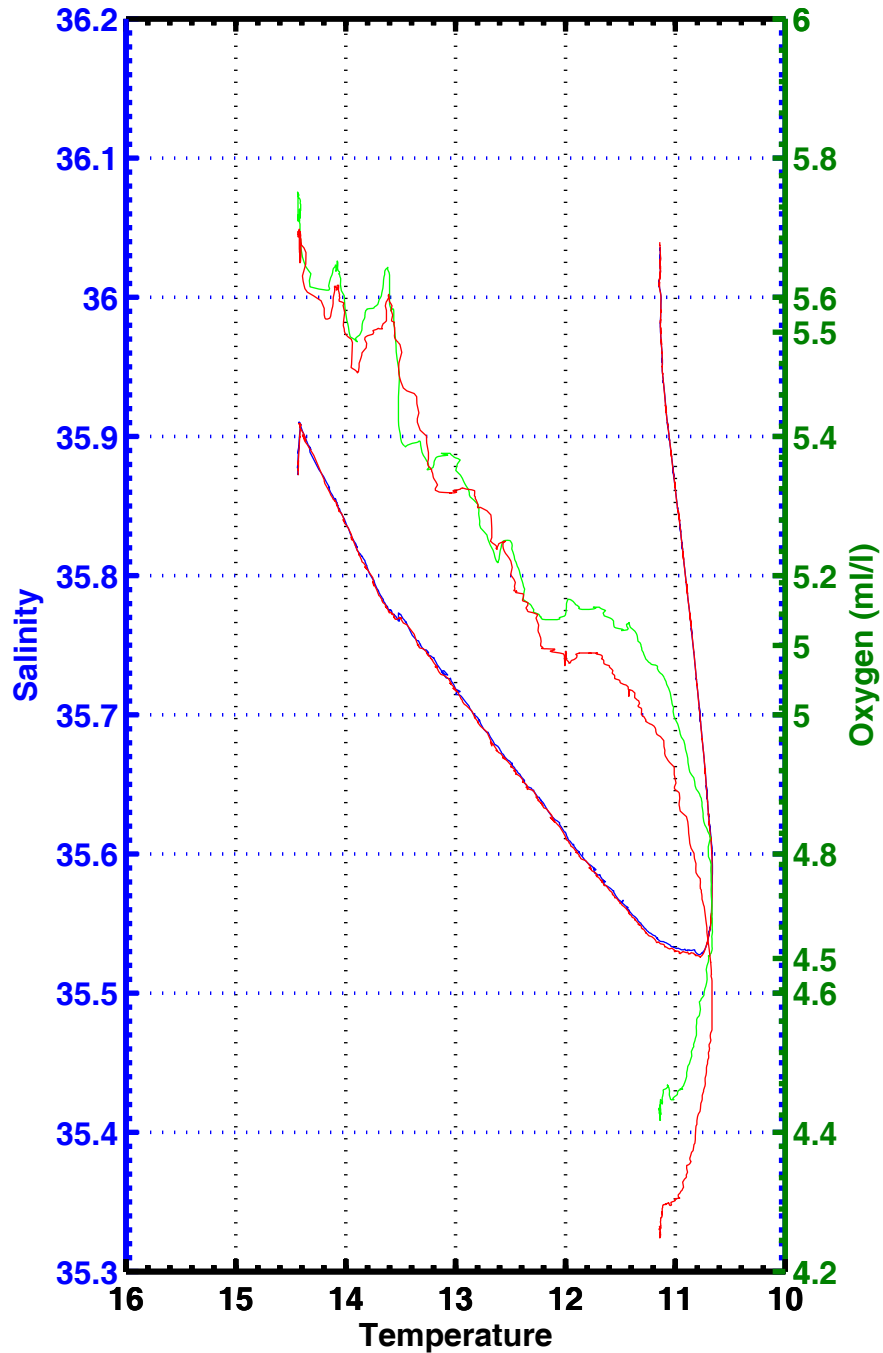
T-S , T-02 , station 1086
