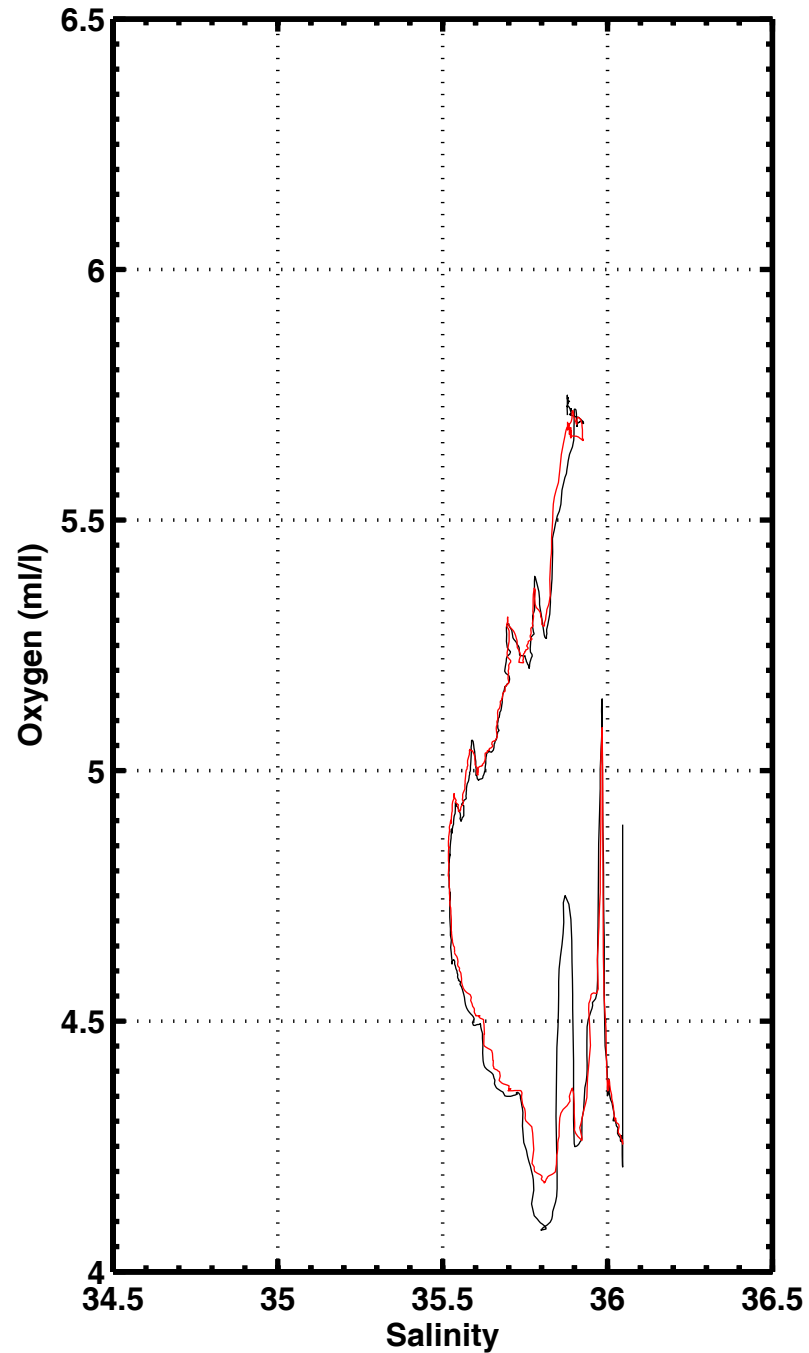
S-O2 , station 1097
