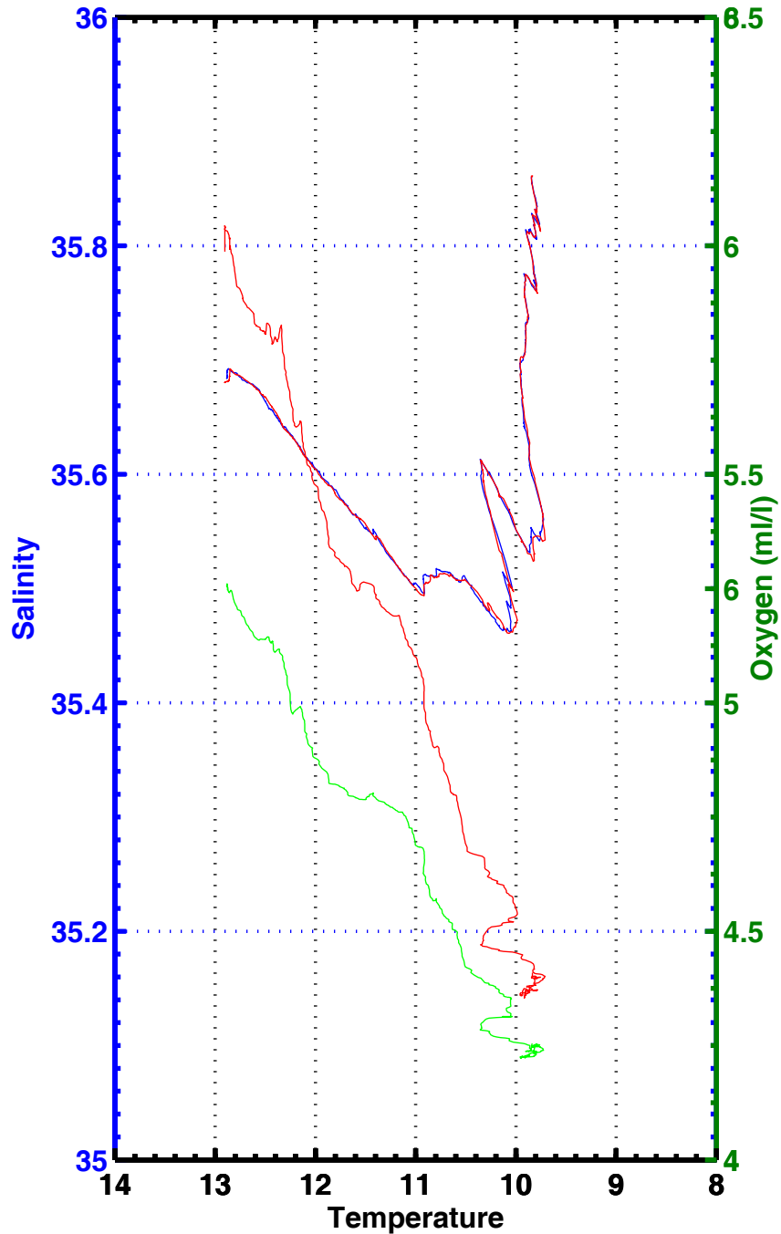
T-S , T-02 , station 1187
