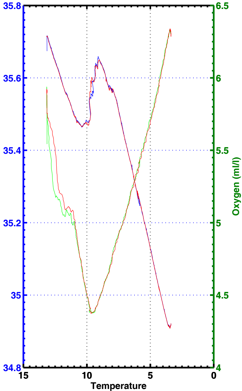
T-S , T-02 , station 1063
