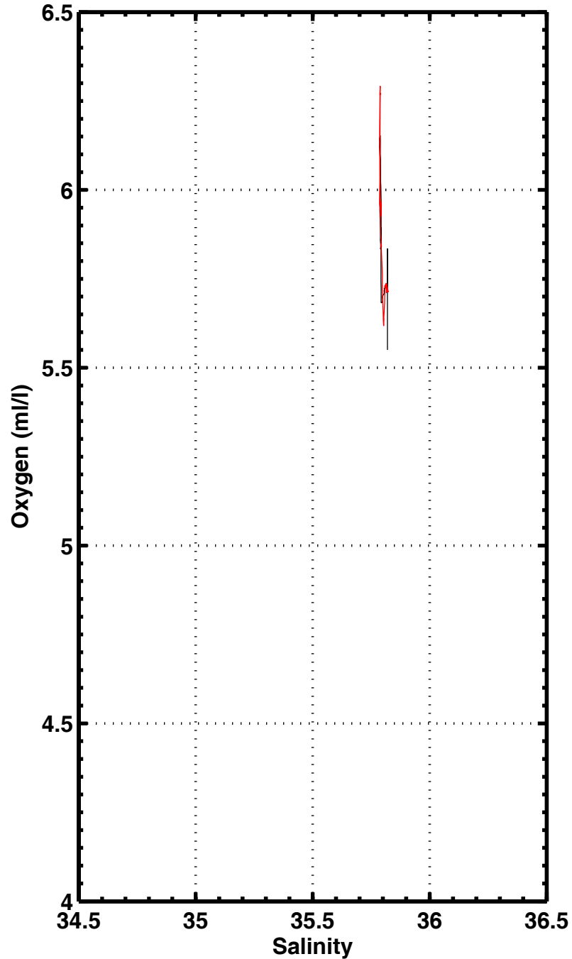
S-02 , station 1116
