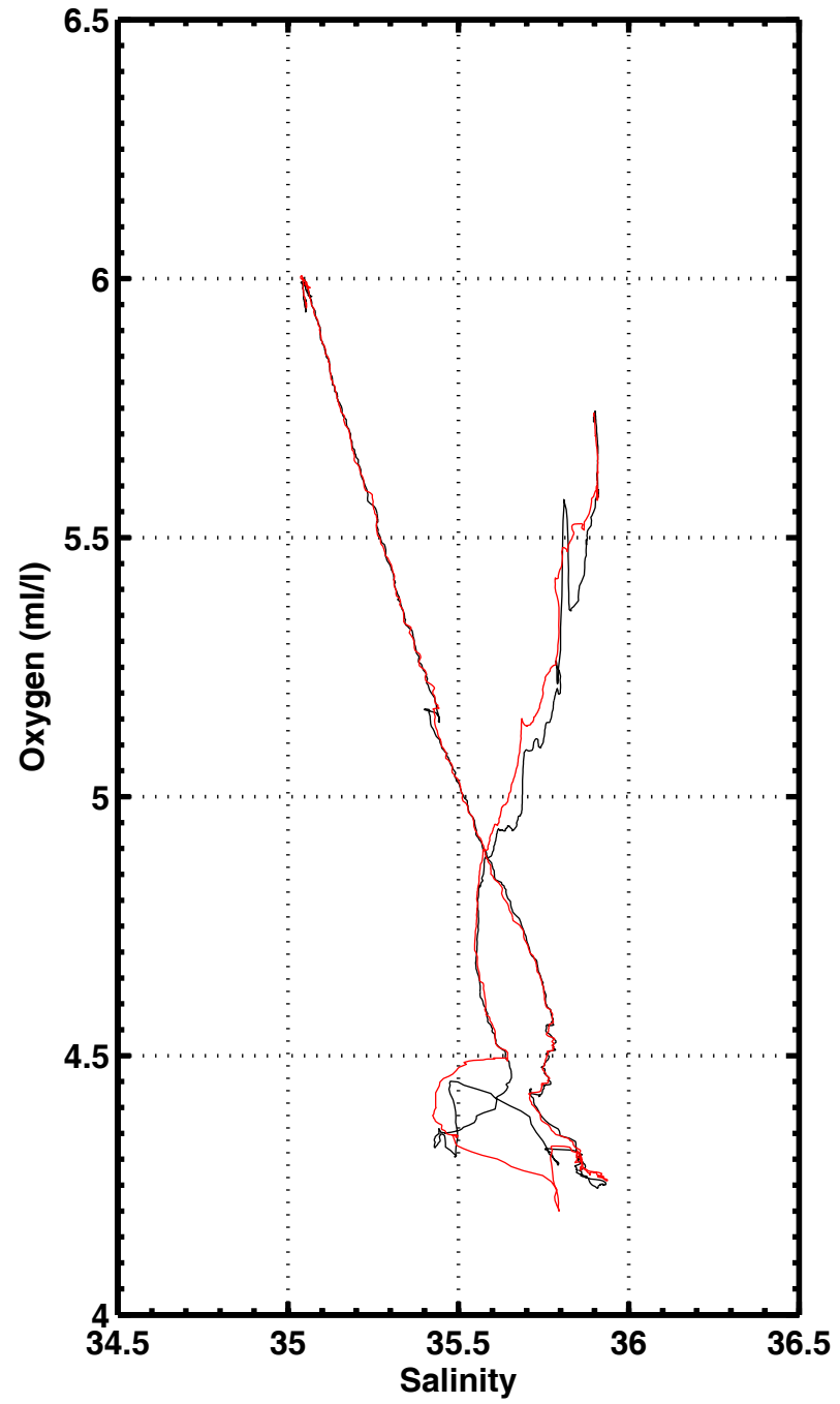
S-02 , station 1035
