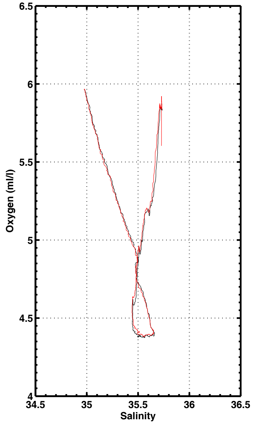
S-02 , station 1138
