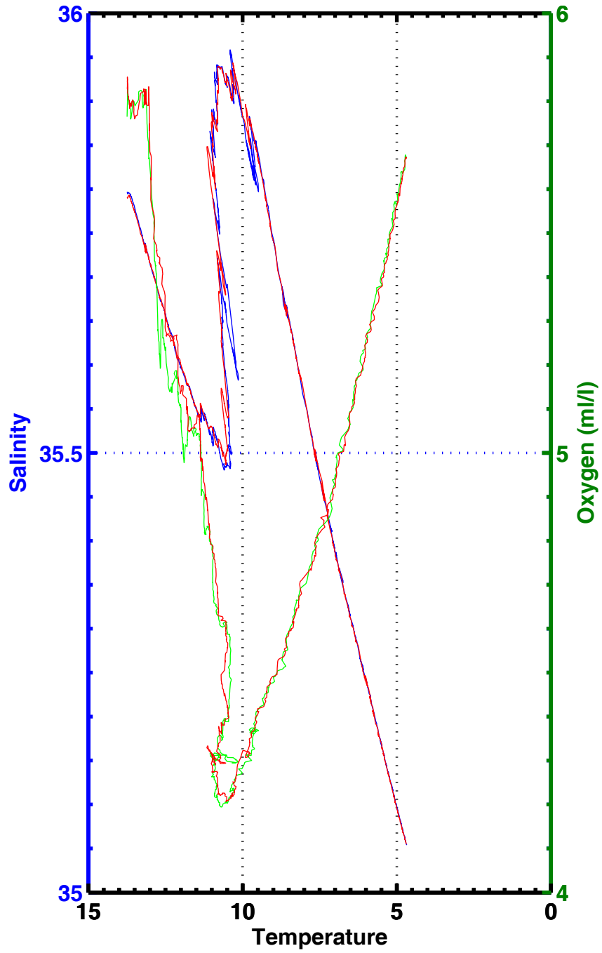
T-S , T-02 , station 1109
