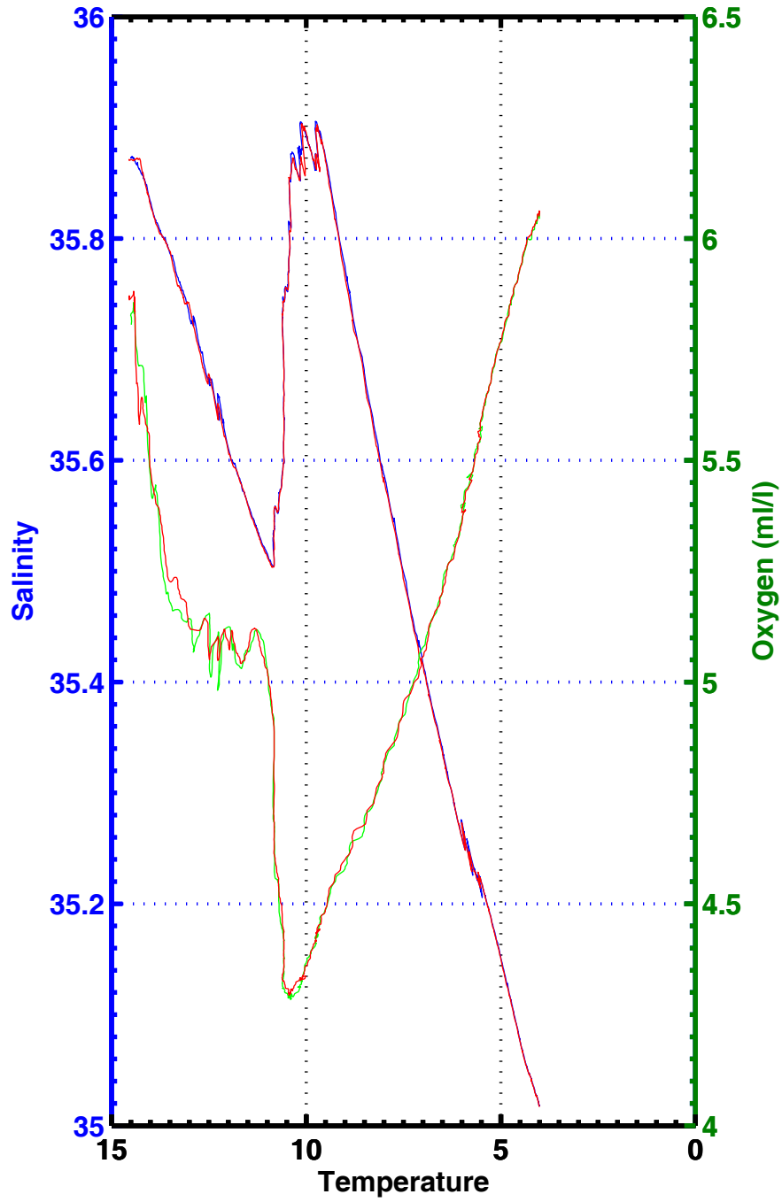
T-S , T-02 , station 1055
