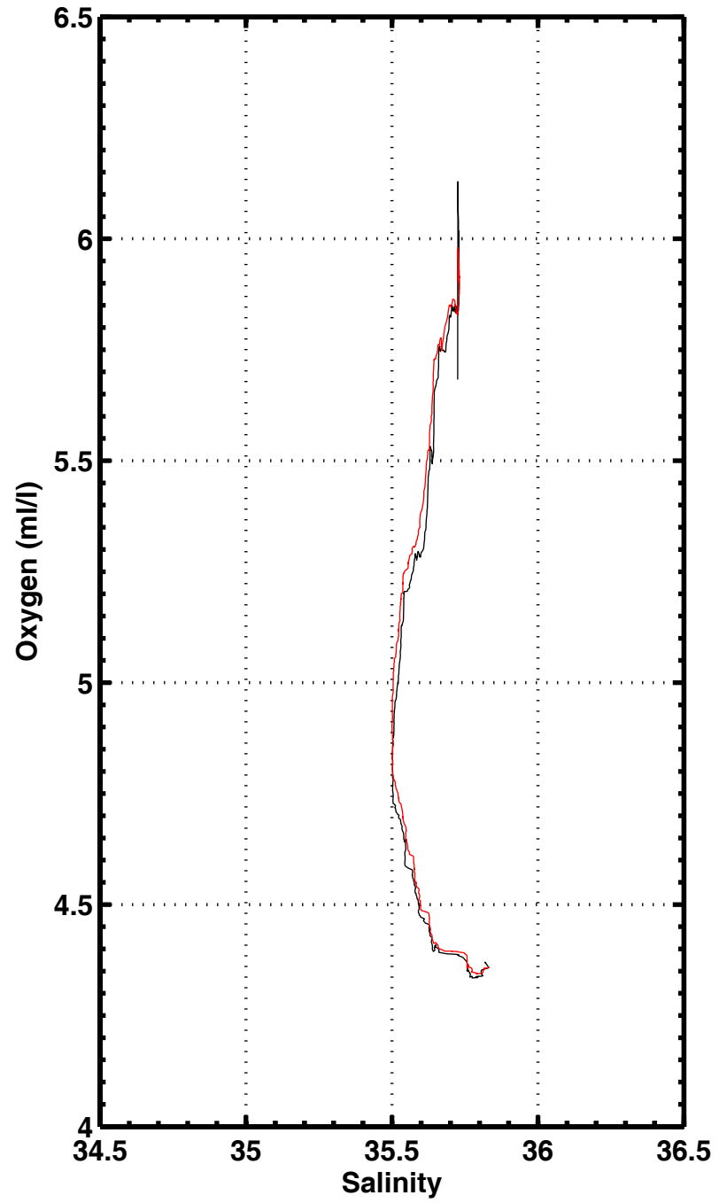
S-O2 , station 1163
