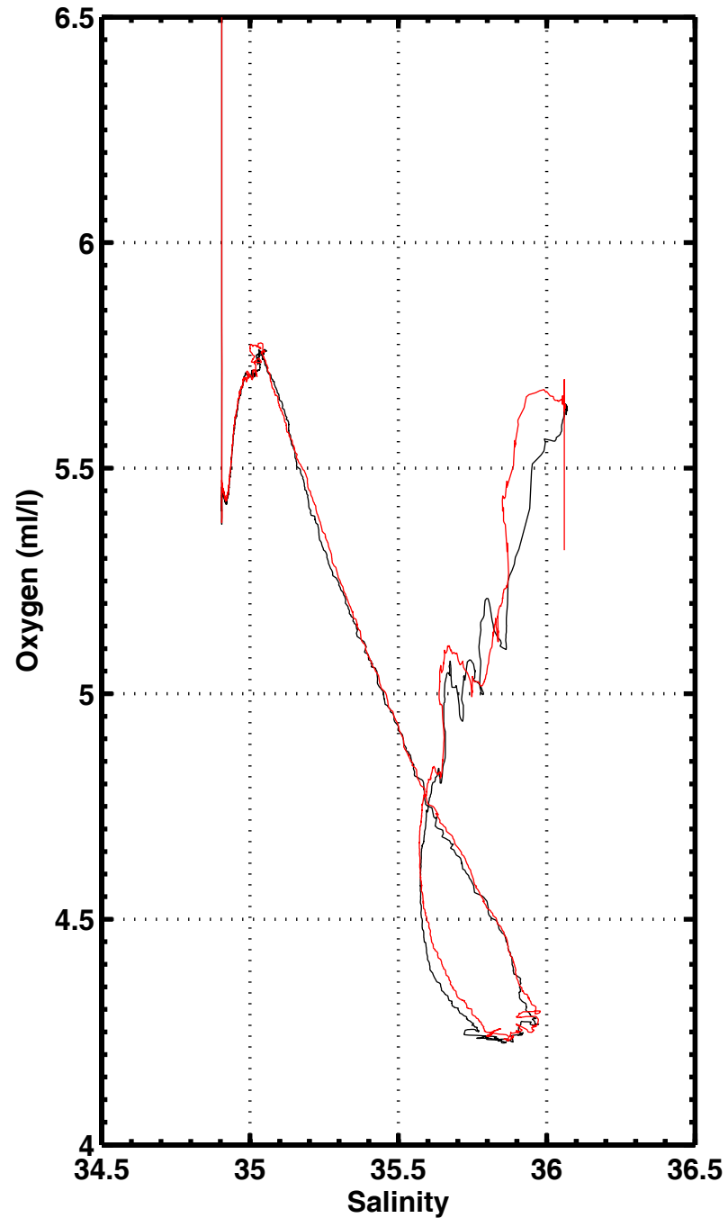
S-O2 , station 1124
