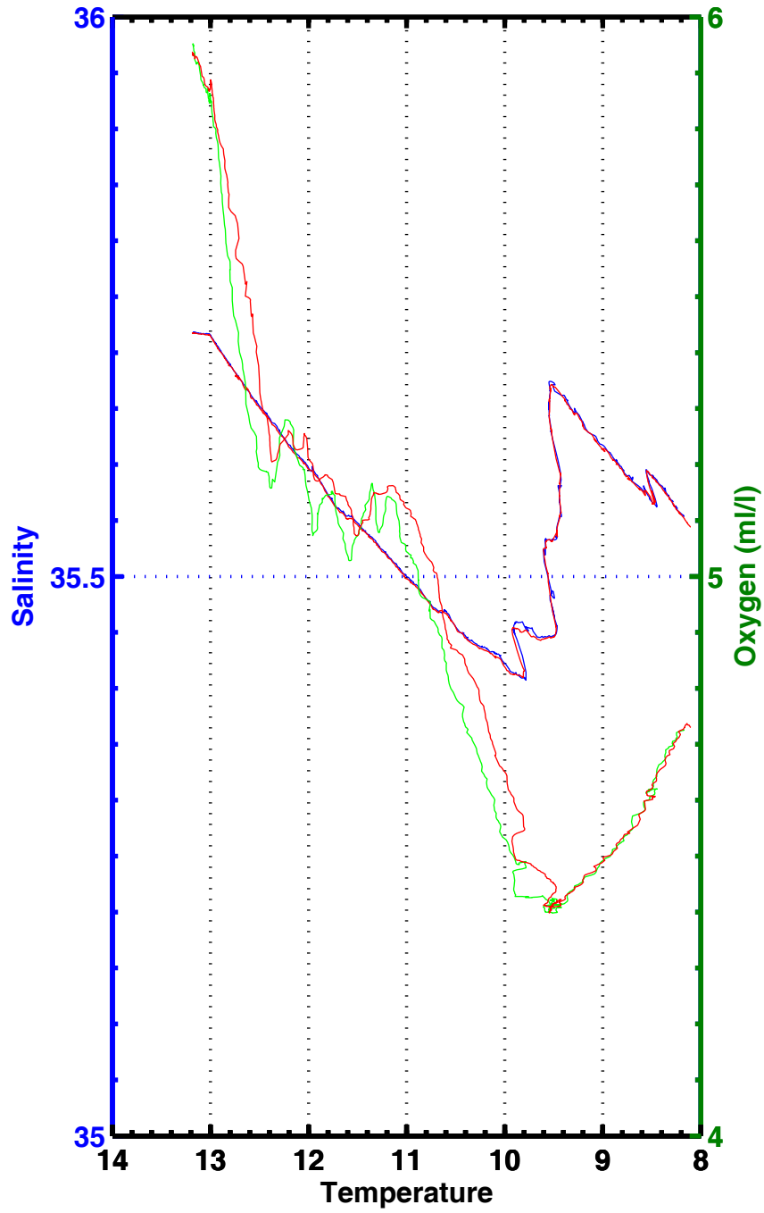
T-S , T-02 , station 1134
