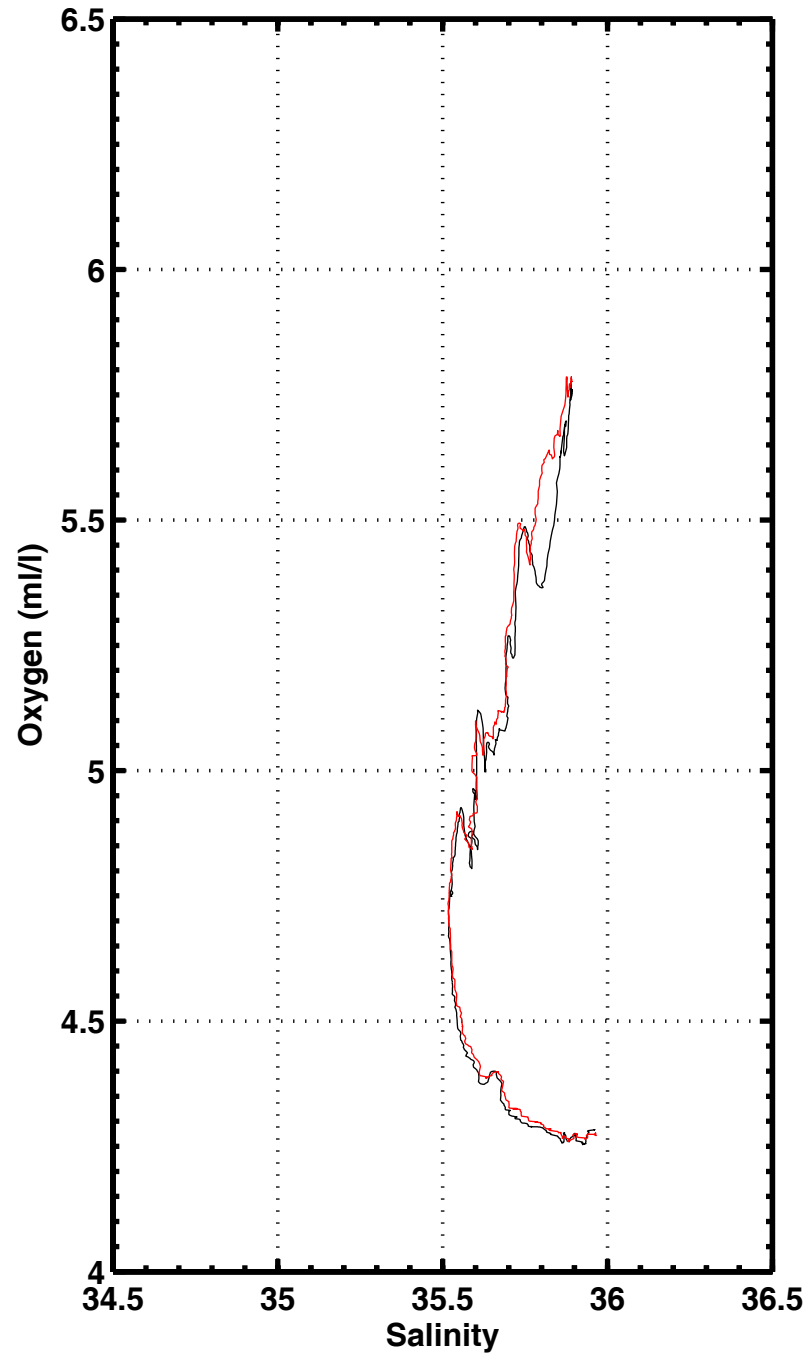
S-O2 , station 1096
