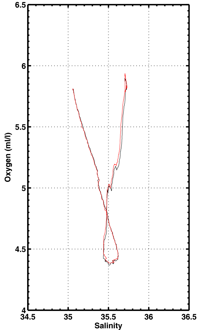
S-O2 , station 1148
