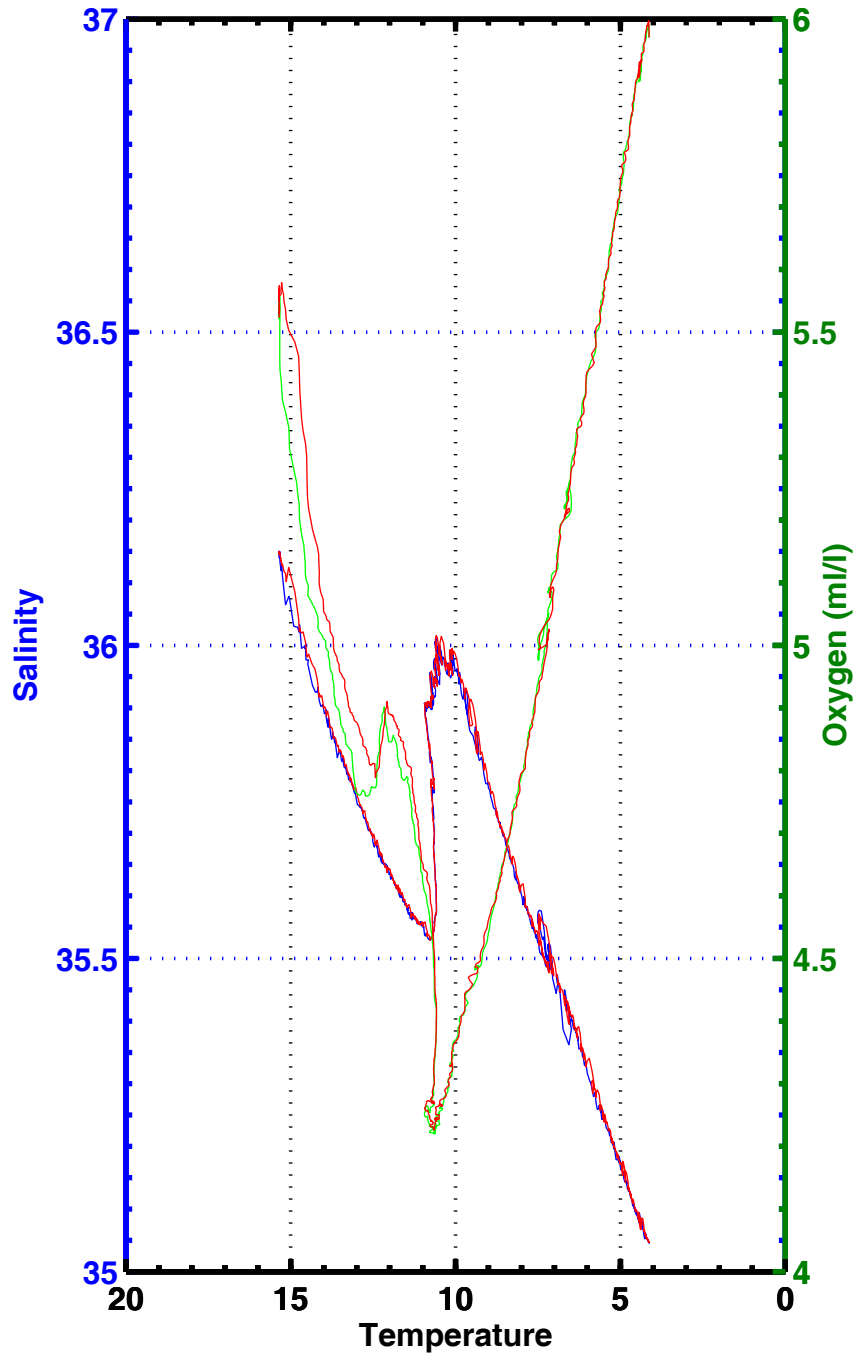
T-S , T-02 , station 1079
