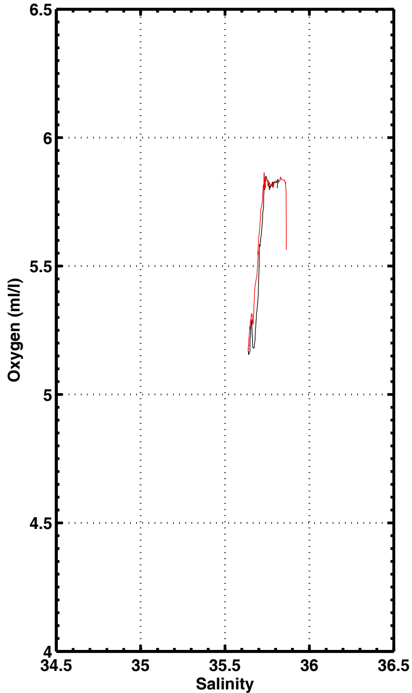
S-O2 , station 1111
