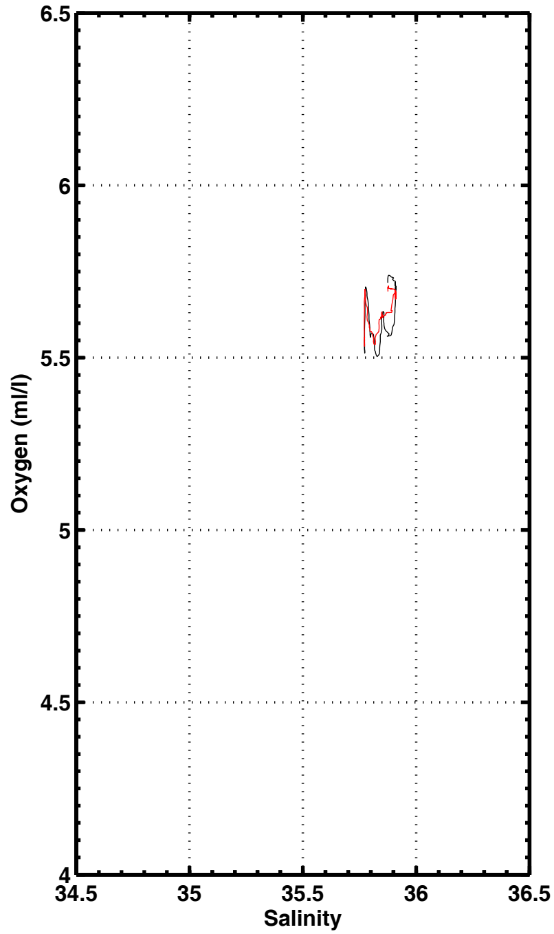
S-O2 , station 1087
