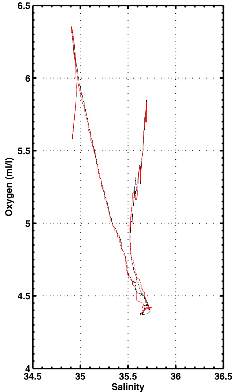
S-O2 , station 1014
