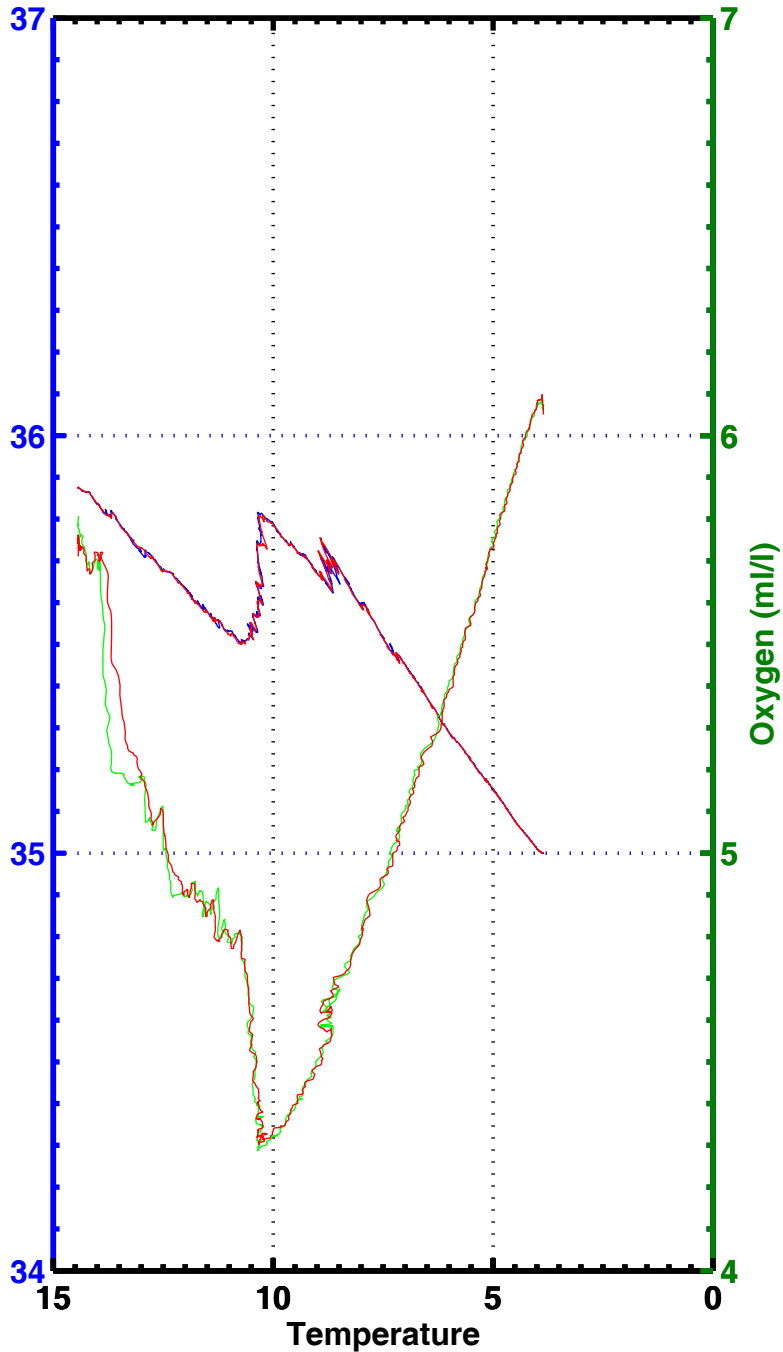
T-S , T-02 , station 1033
