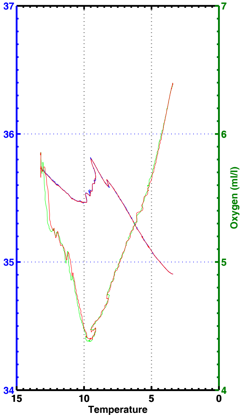
T-S , T-02 , station 1043
