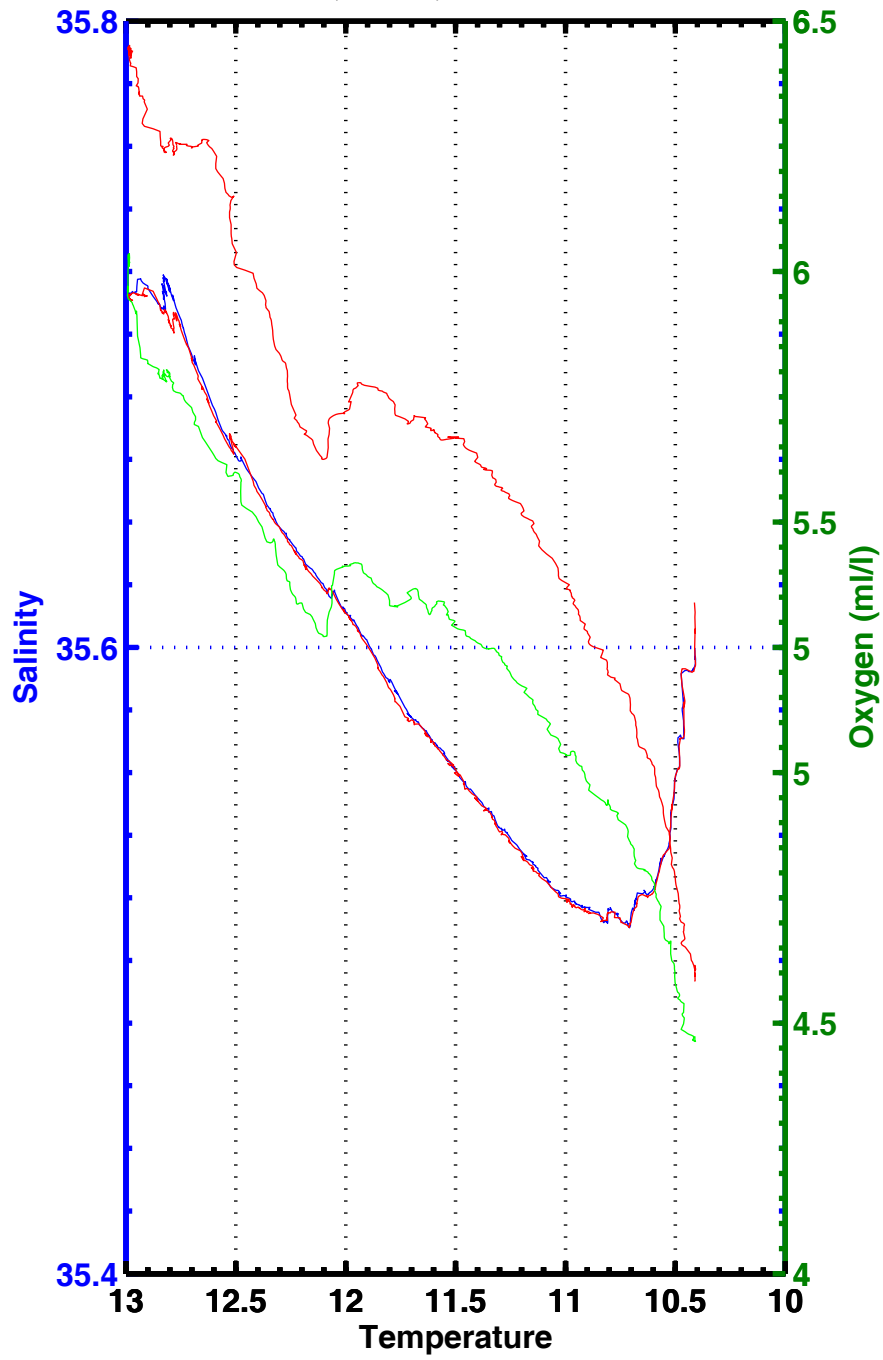
T-S , T-02 , station 1174
