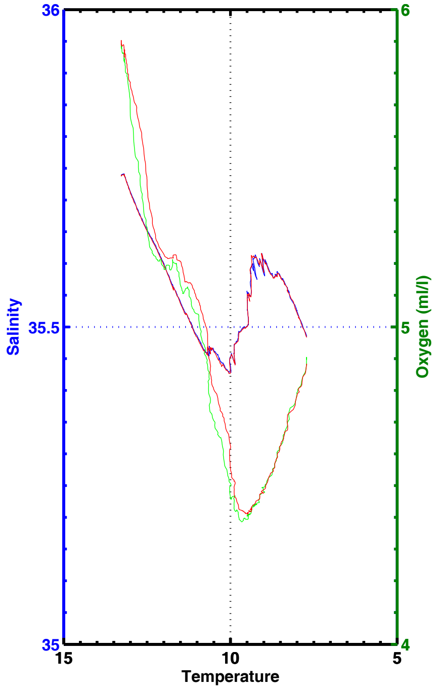
T-S , T-02 , station 1136
