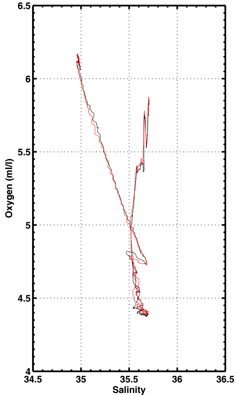
S-O2 , station 1024
