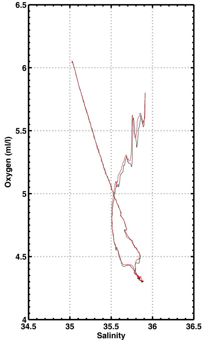
S-O2 , station 1054
