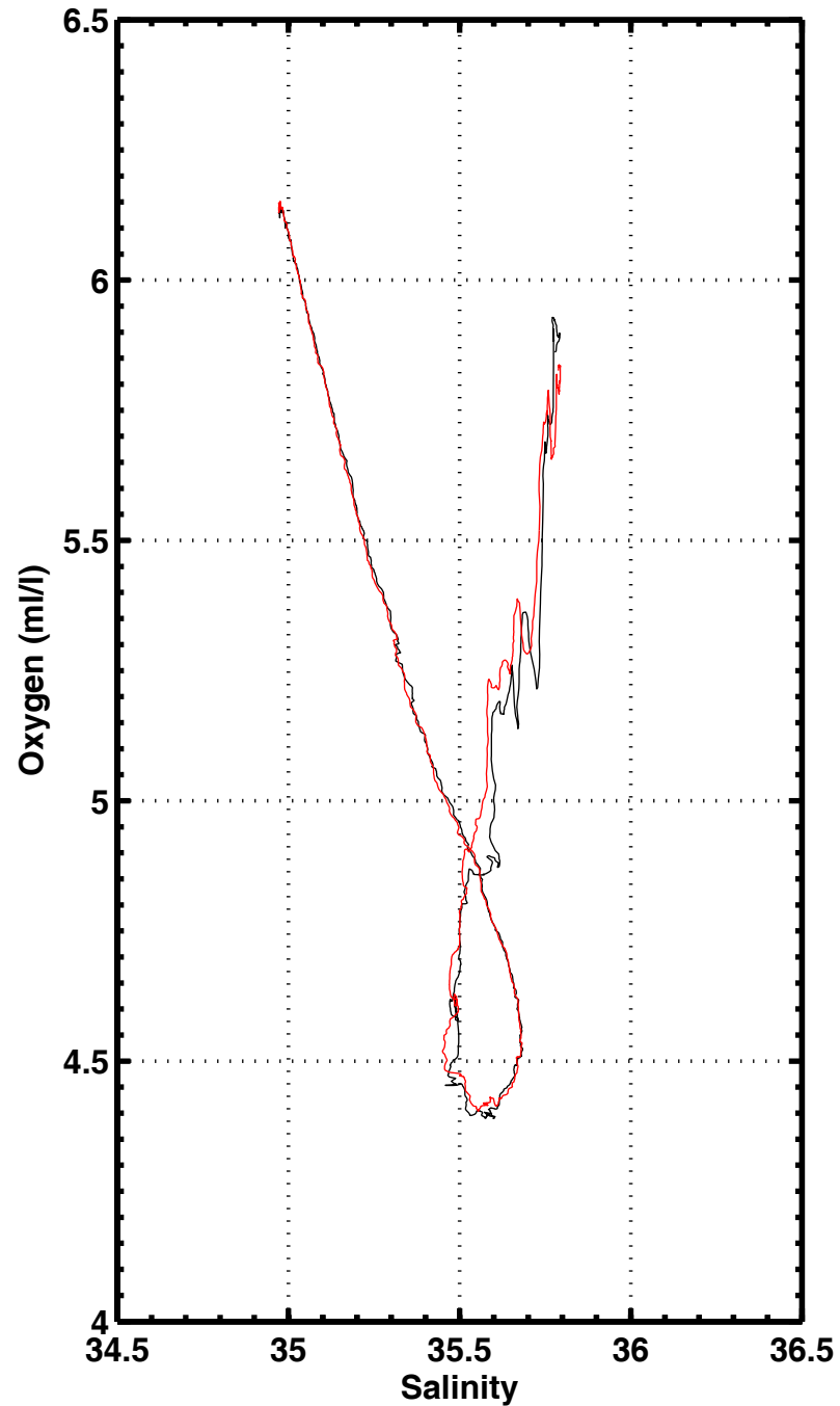
S-O2 , station 1048
