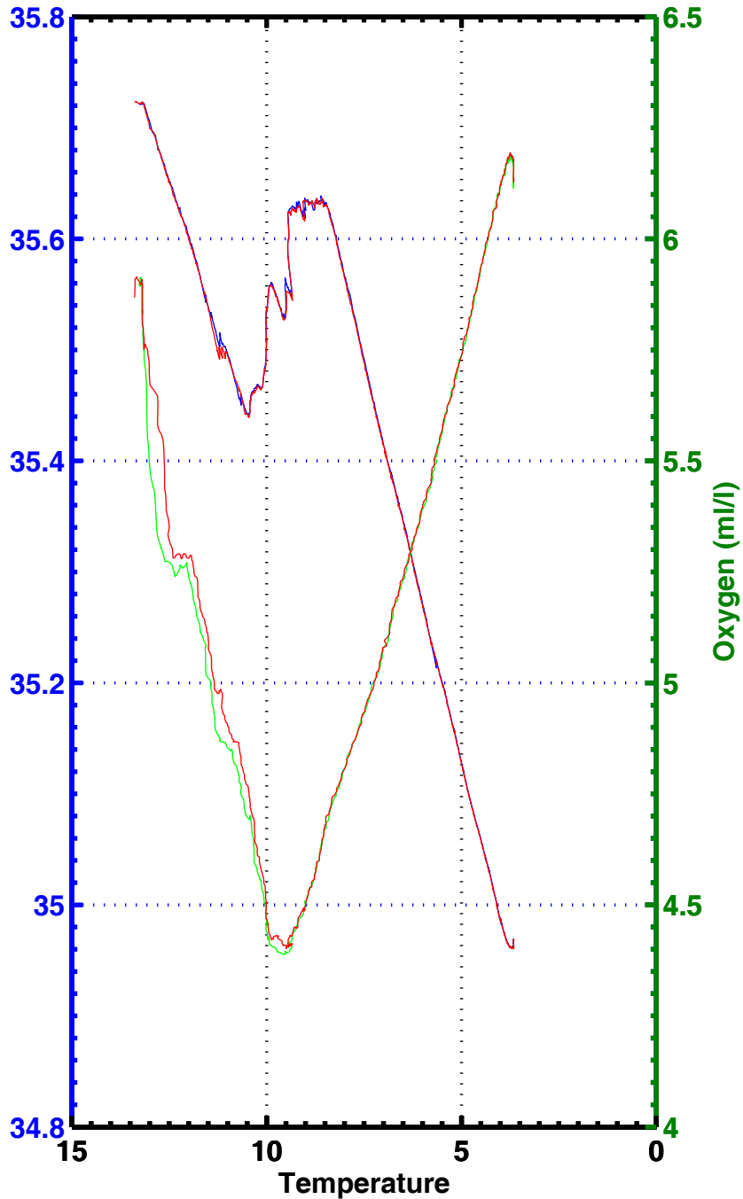
T-S , T-02 , station 1047
