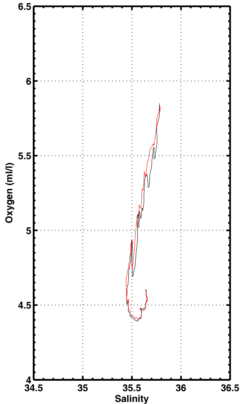
S-O2 , station 1127
