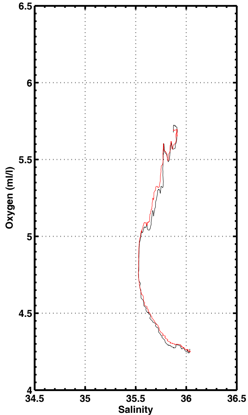
S-O2 , station 1086
