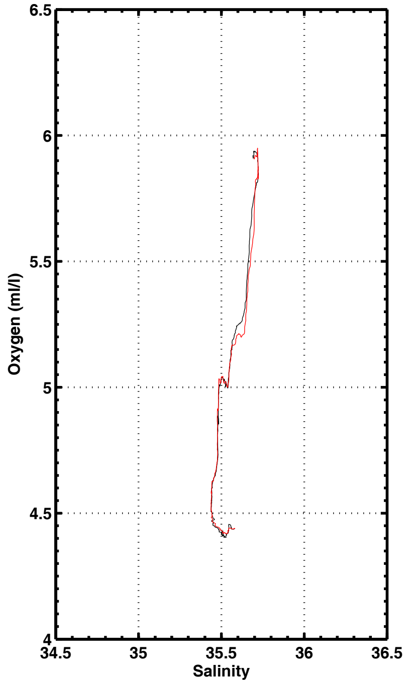
S-O2 , station 1147
