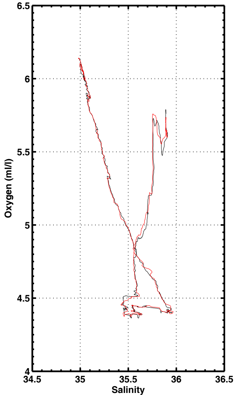
S-O2 , station 1036
