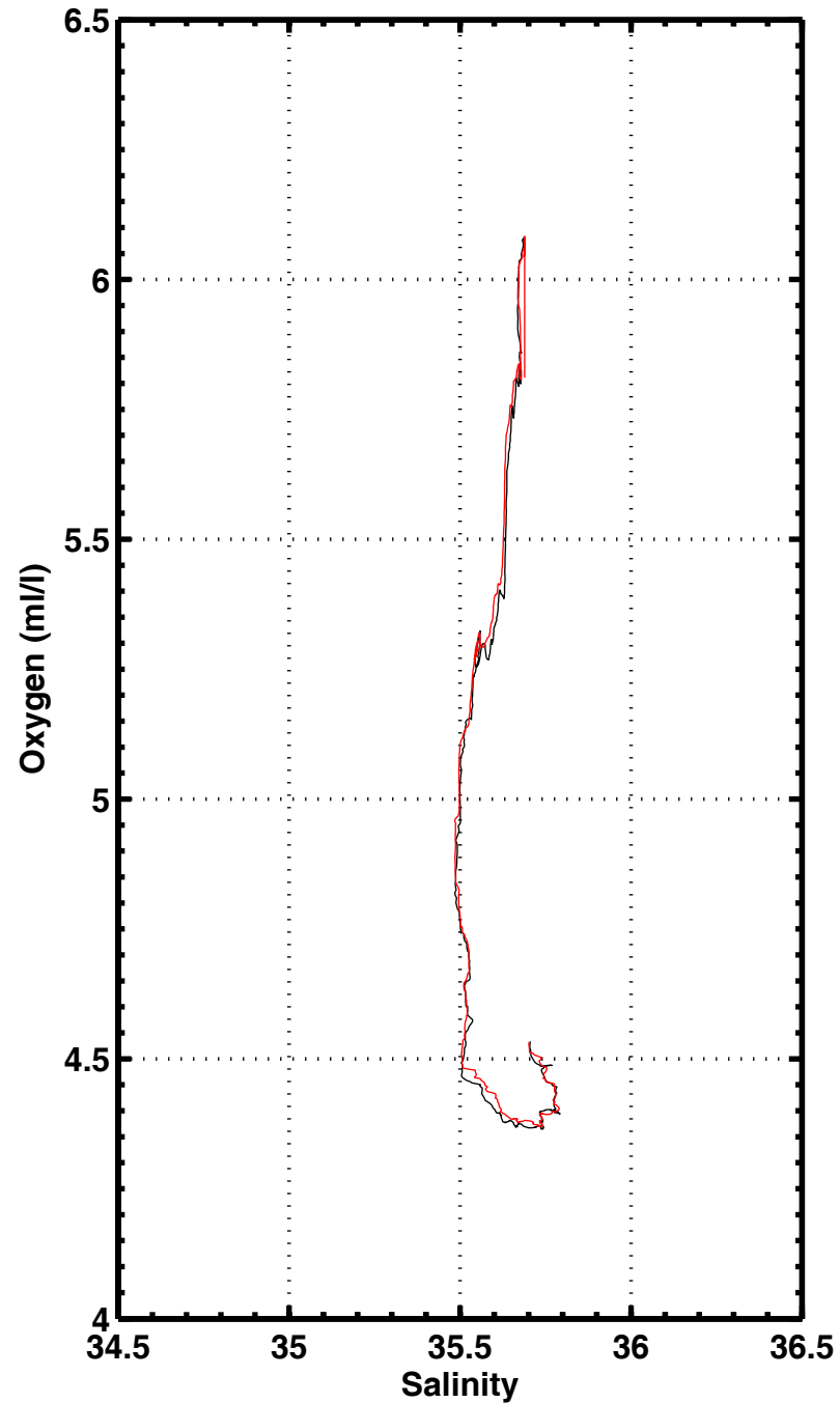
S-O2 , station 1188
