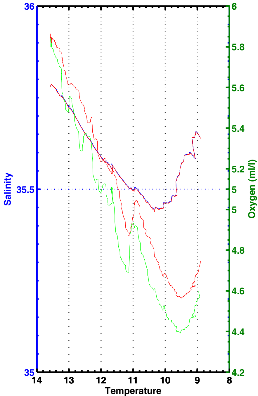
T-S , T-02 , station 1127
