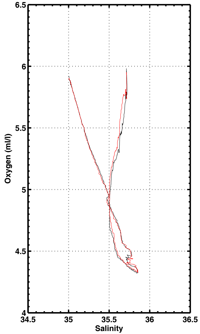
S-O2 , station 1177
