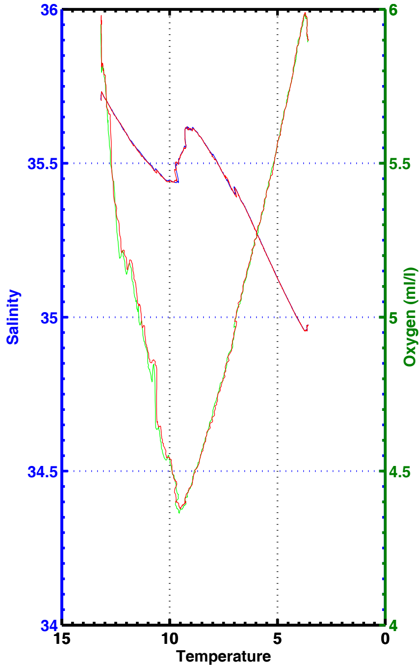
T-S , T-02 , station 1149
