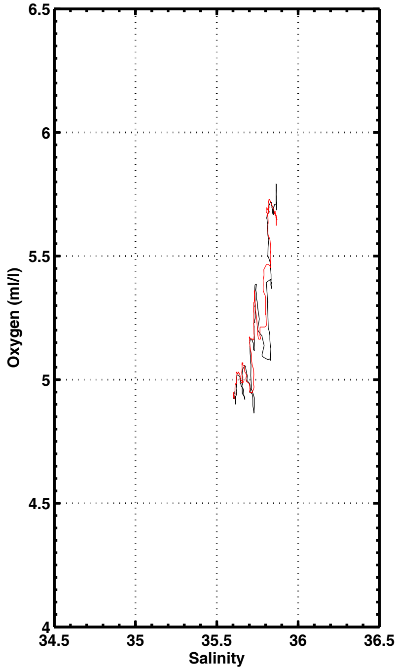
S-O2, station 1117
