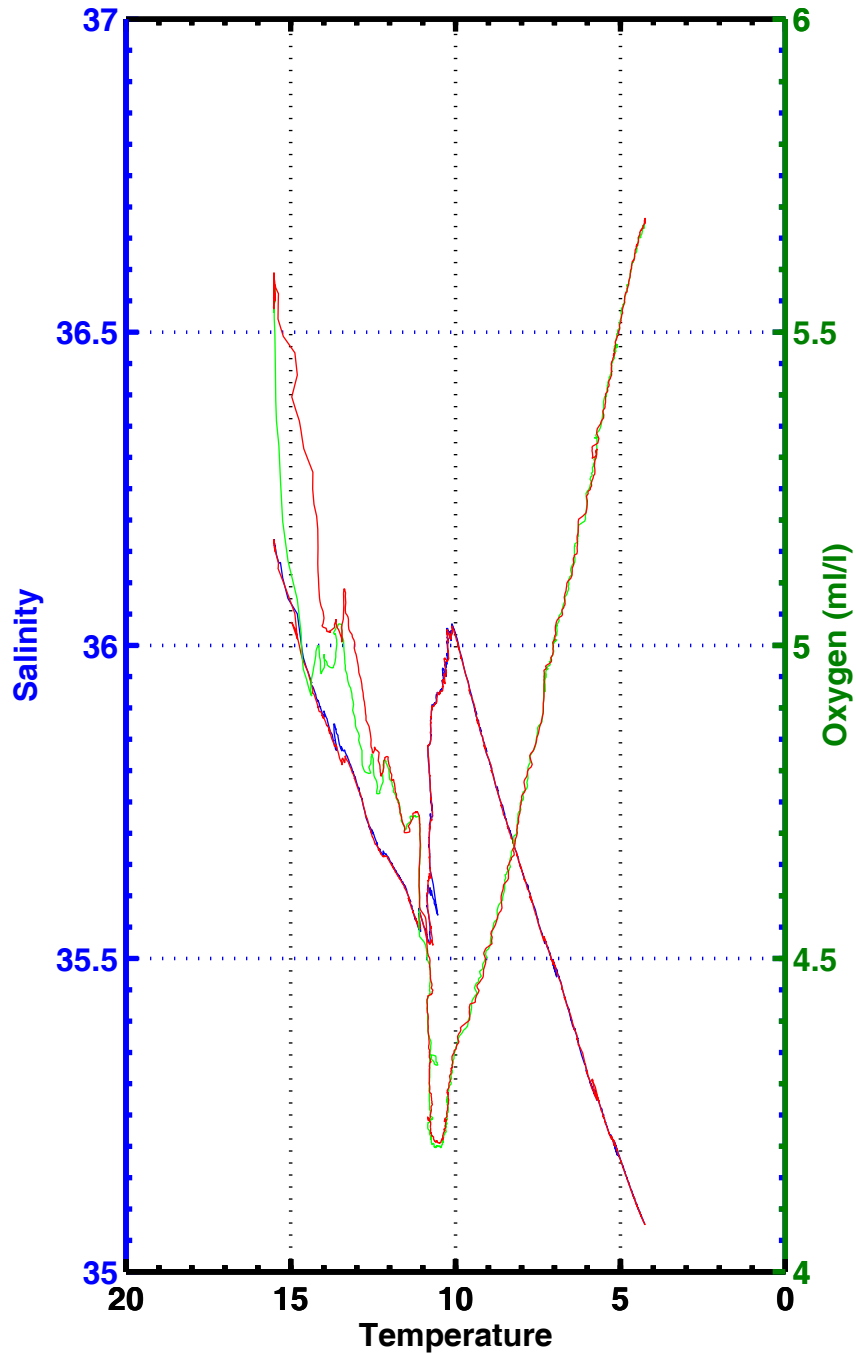
T-S , T-02 , station 1080
