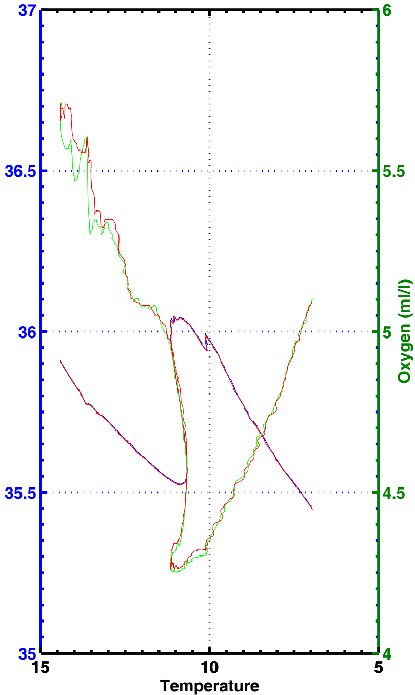
T-S , T-02 , station 1082
