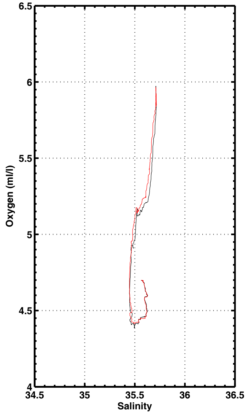
S-O2 , station 1152
