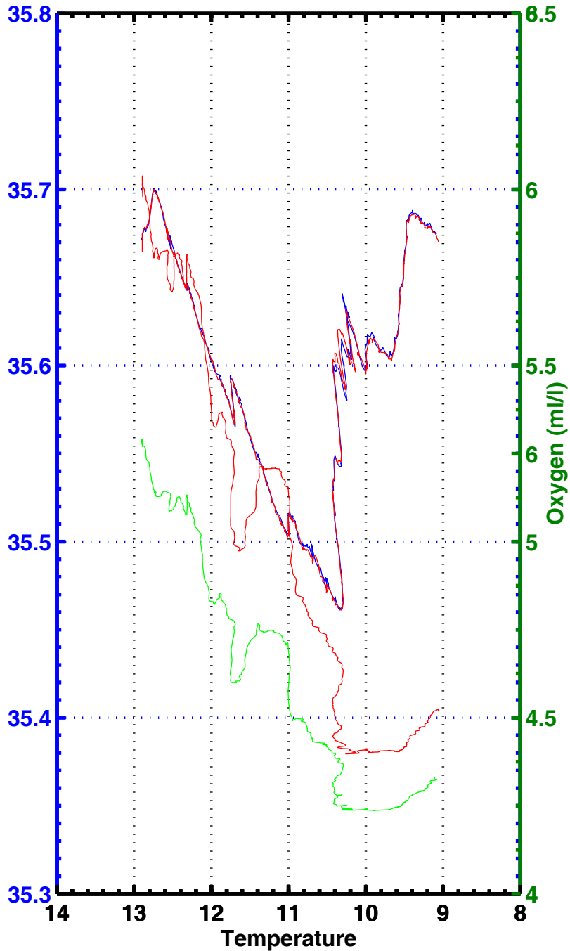
T-S , T-02 , station 1192
