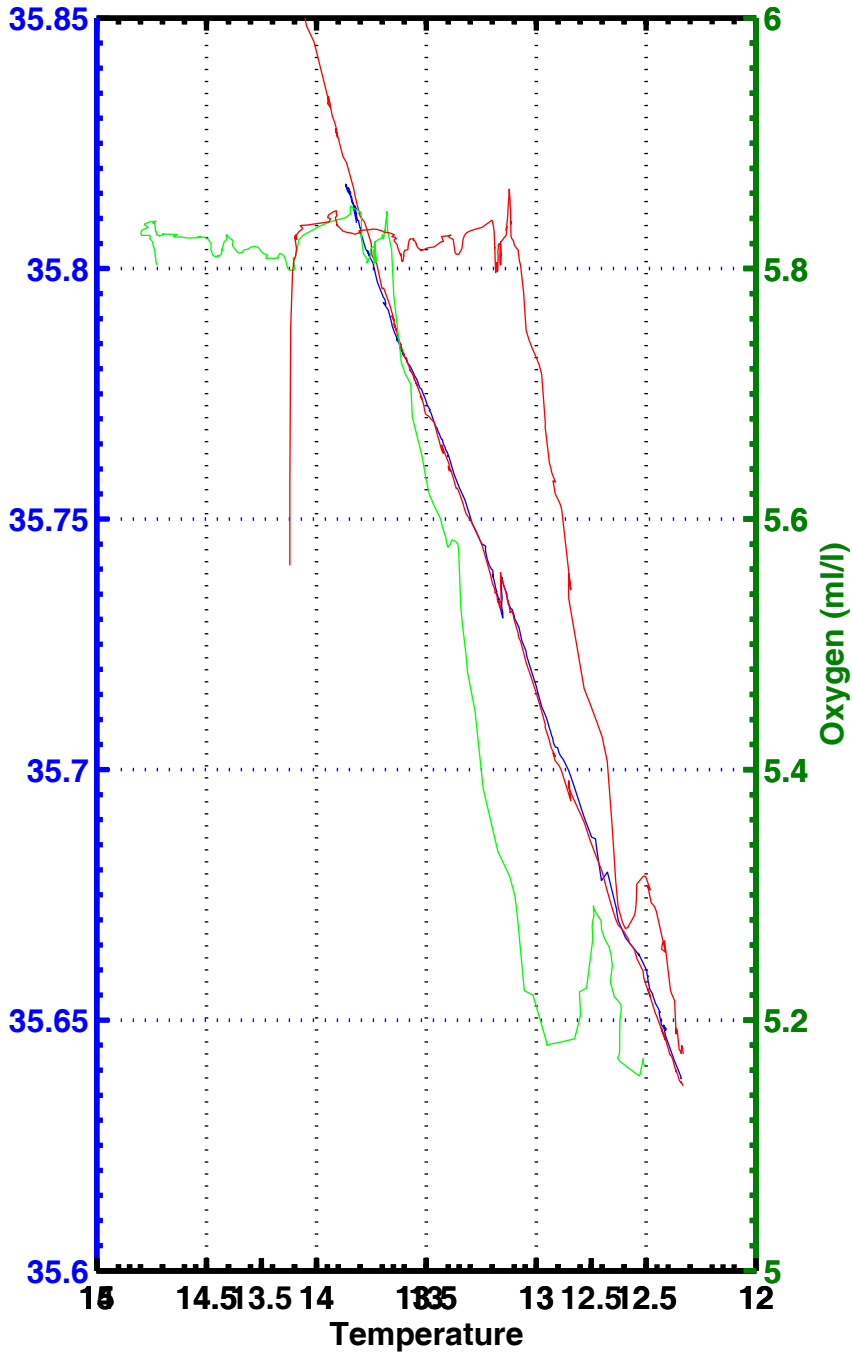
T-S , T-02 , station 1111
