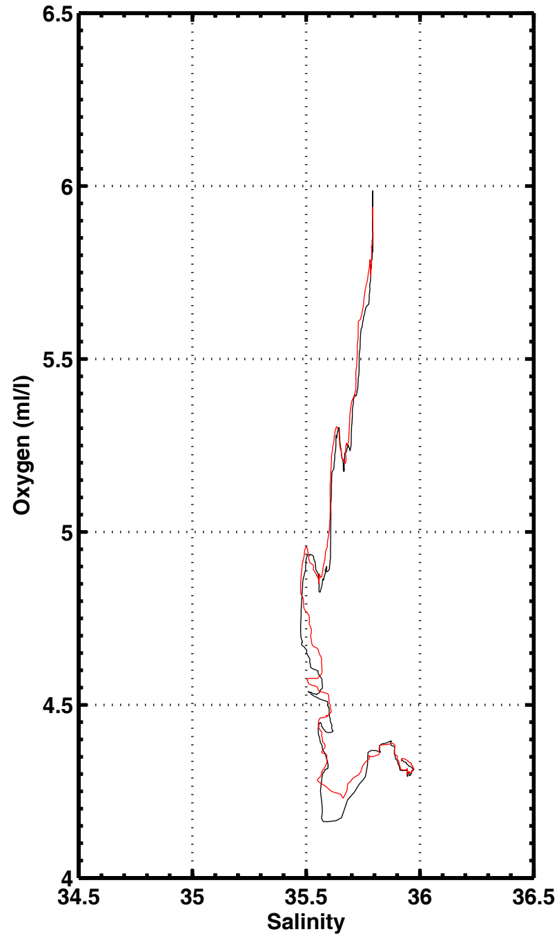
S-O2 , station 1200
