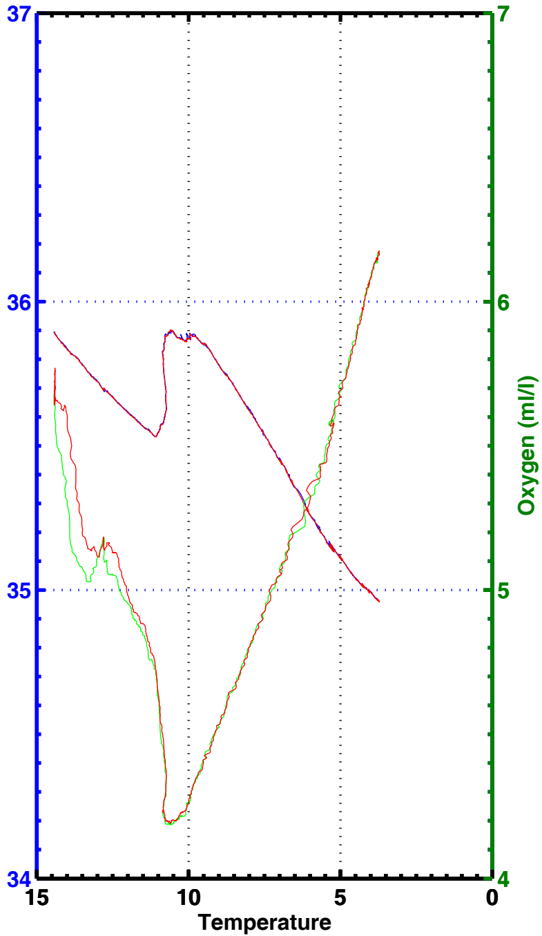
T-S , T-02 , station 1073
