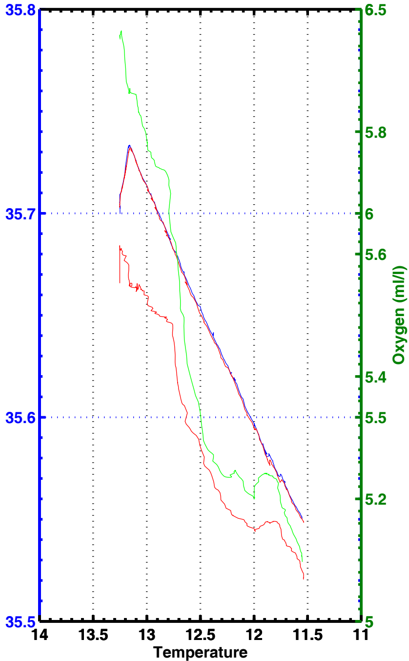
T-S , T-02 , station 1143
