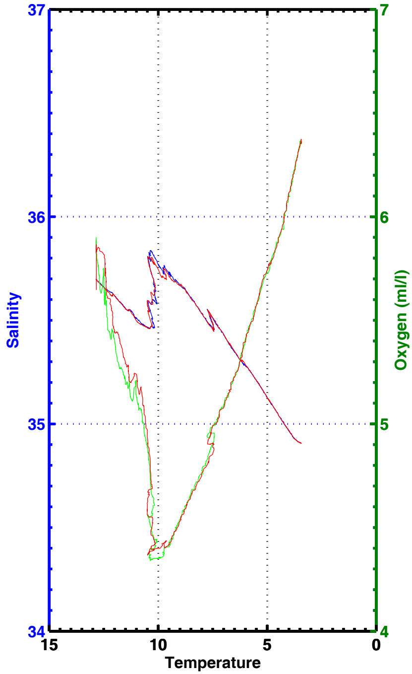
T-S , T-02 , station 1009
