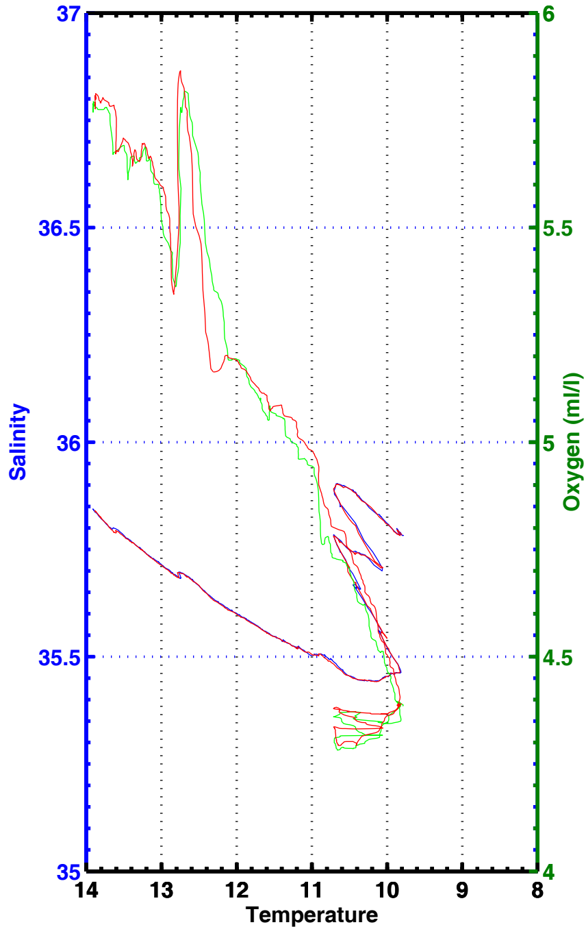
T-S , T-02 , station 1195
