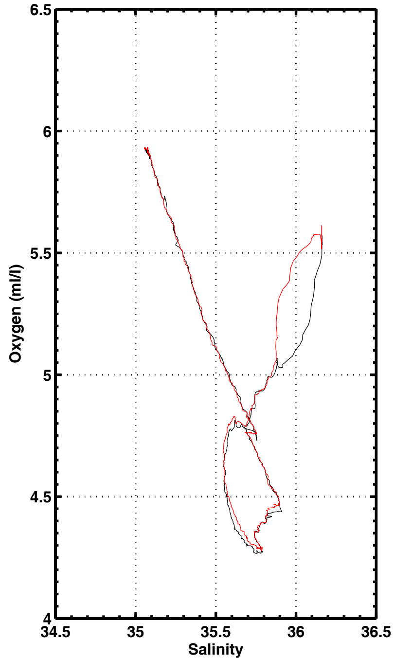
S-O2 , station 1078
