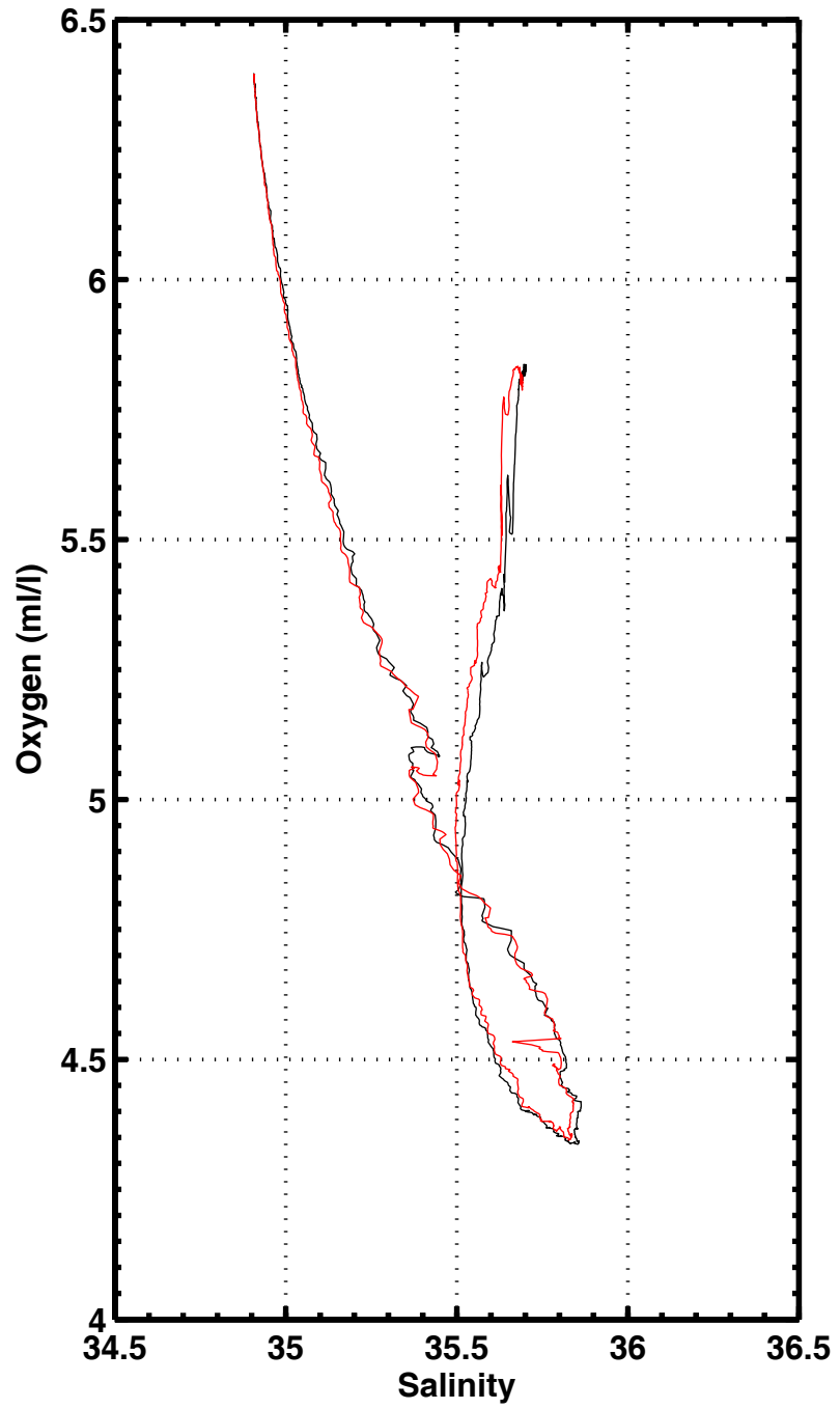
S-O2 , station 1010
