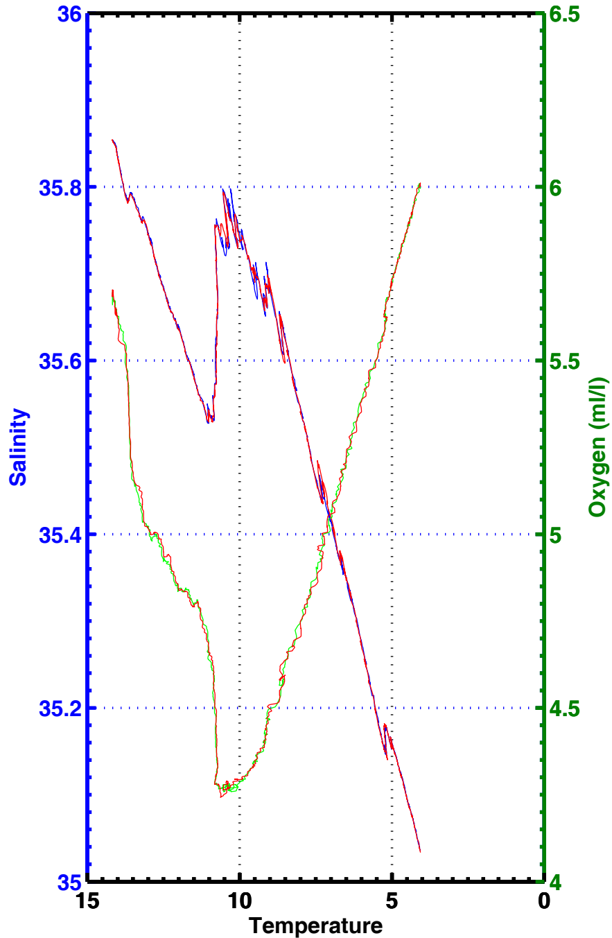
T-S , T-02 , station 1028
