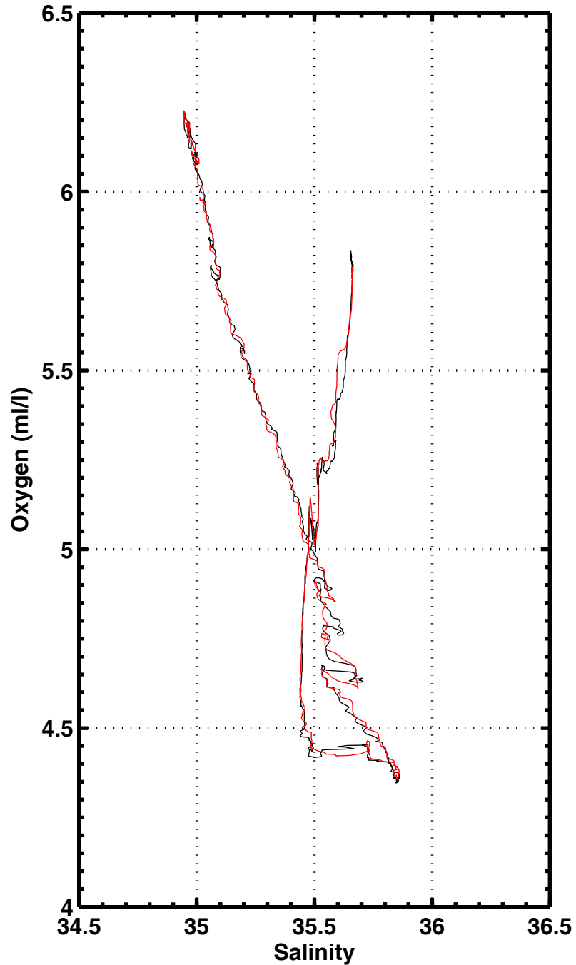
S-02, station 1011
