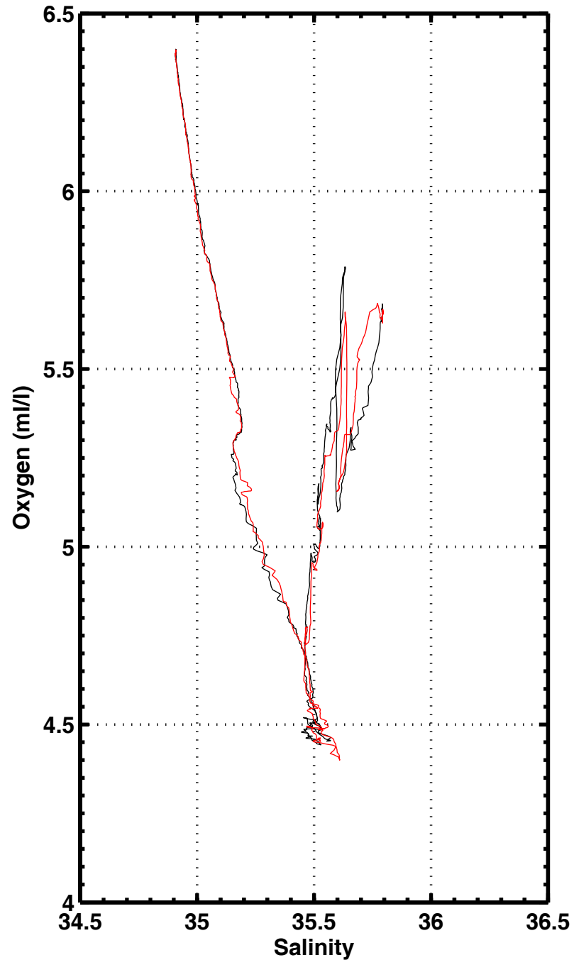
S-O2 , station 1017
