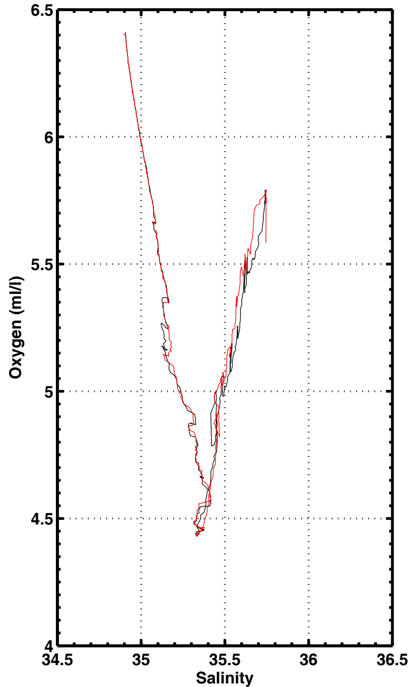
S-O2 , station 1018
