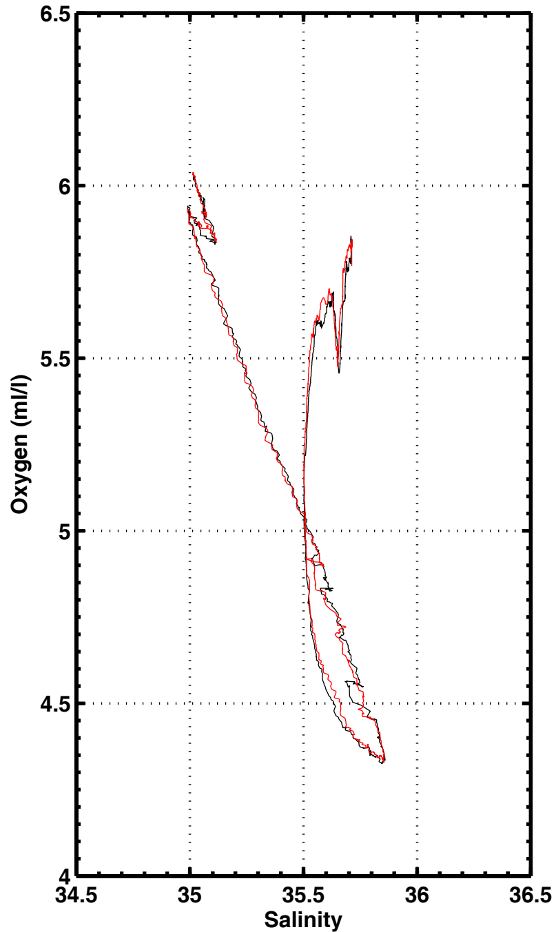
S-O2 , station 1023
