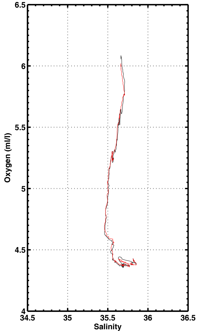
S-O2 , station 1186
