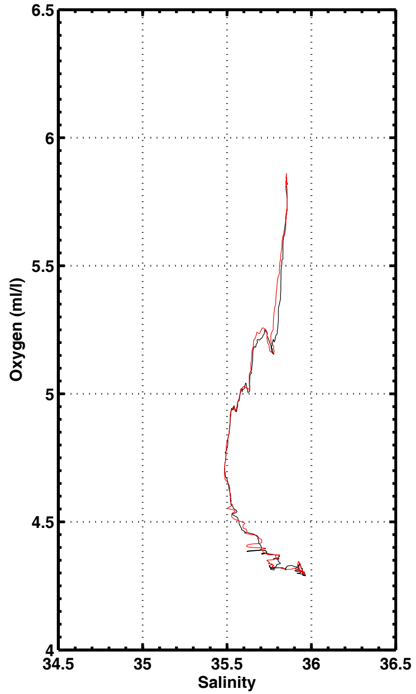
S-O2 , station 1205
