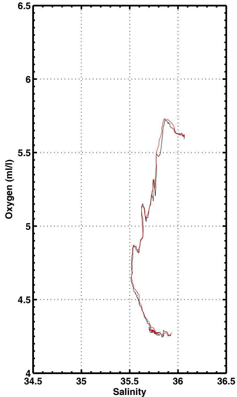
S-O2 , station 1102
