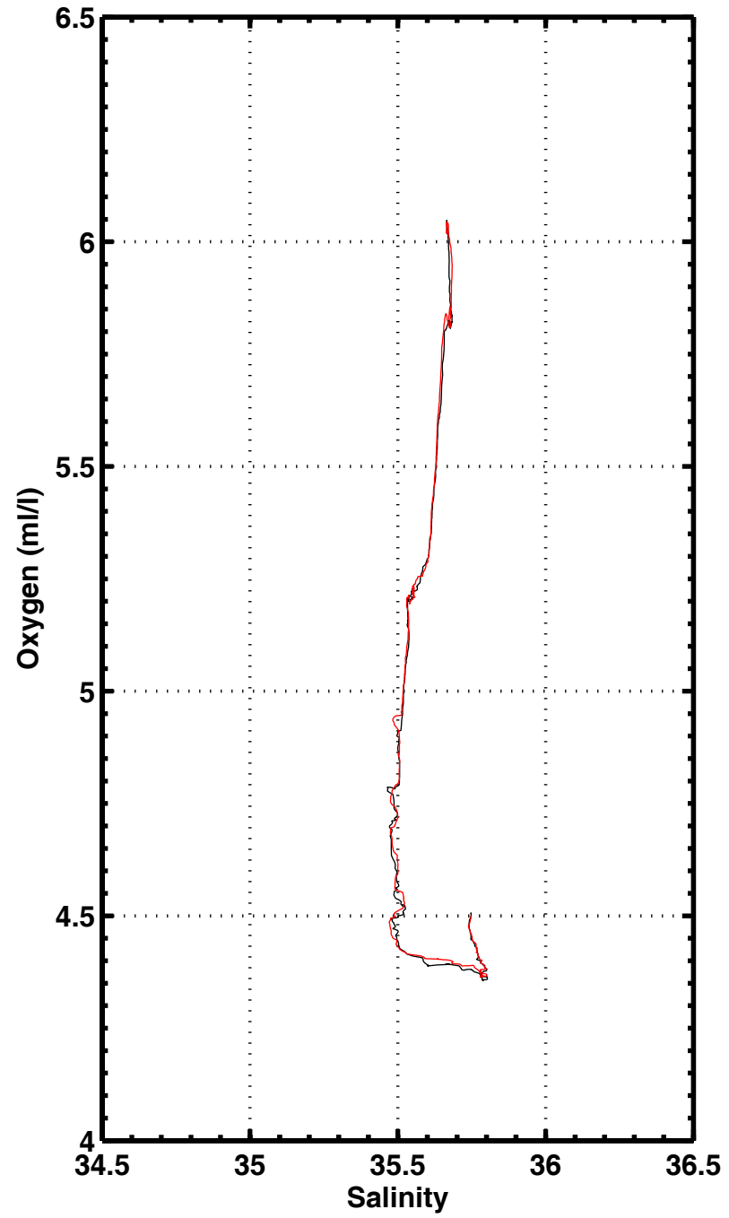
S-O2 , station 1190
