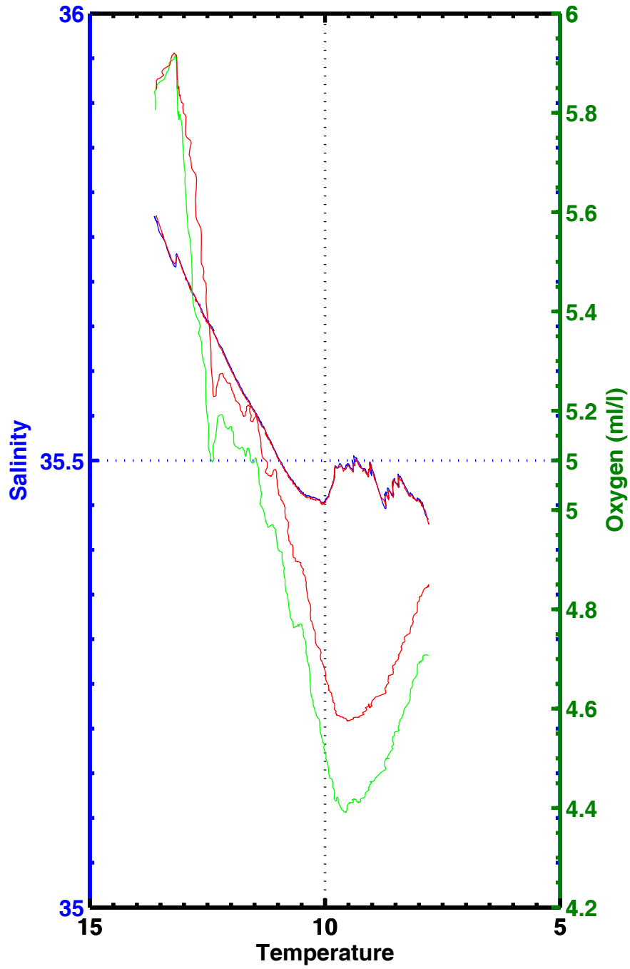
T-S , T-02 , station 1105
