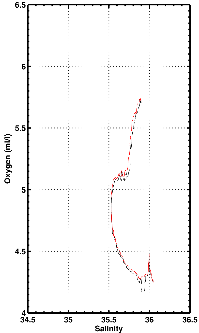
S-O2 , station 1098
