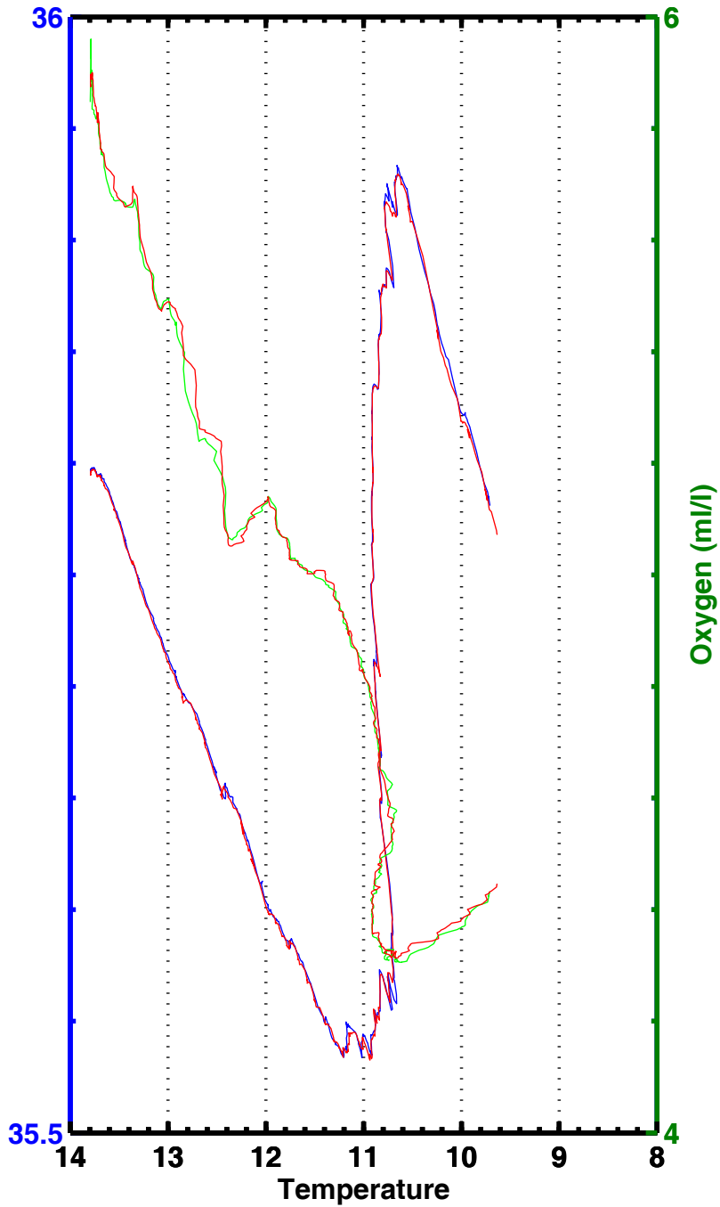
T-S , T-02 , station 1201
