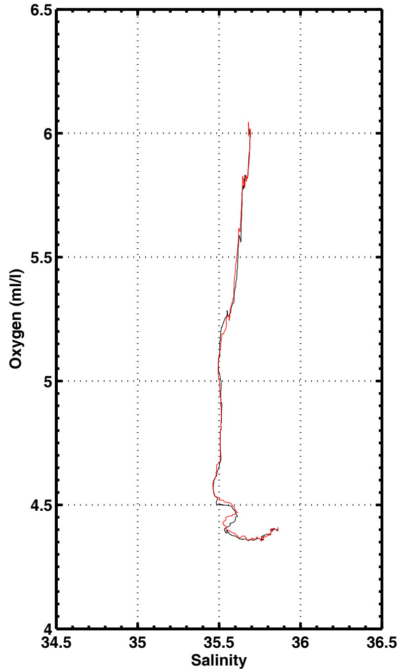
S-O2 , station 1187
