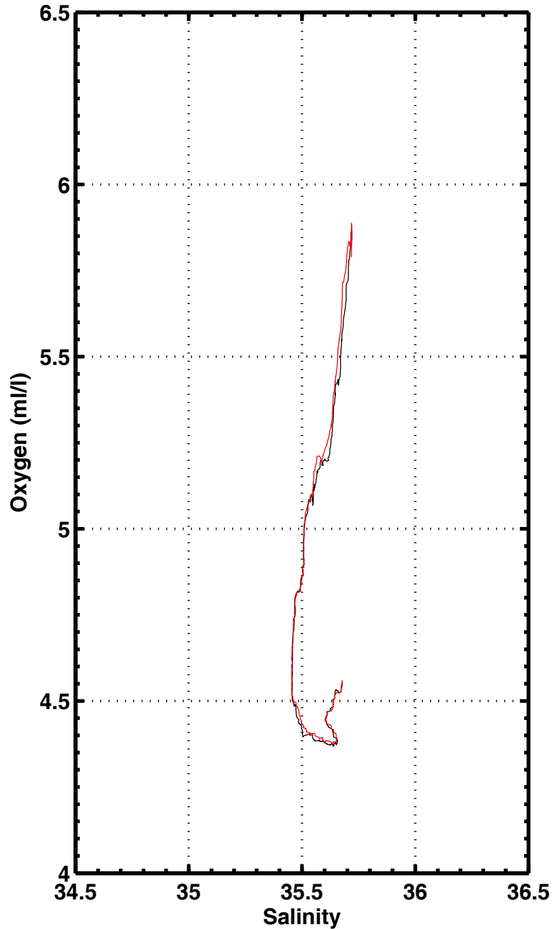
S-02 , station 1131
