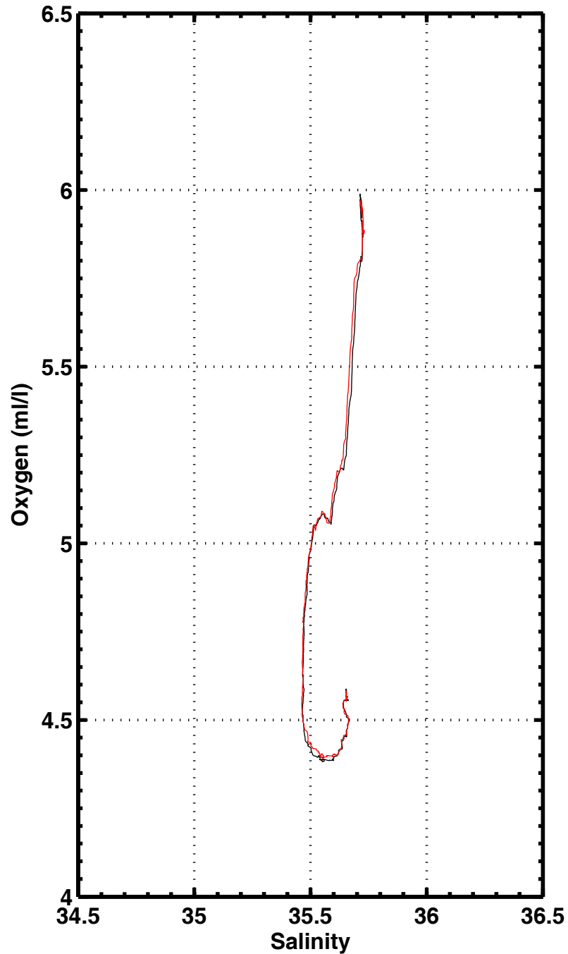
S-O2 , station 1106
