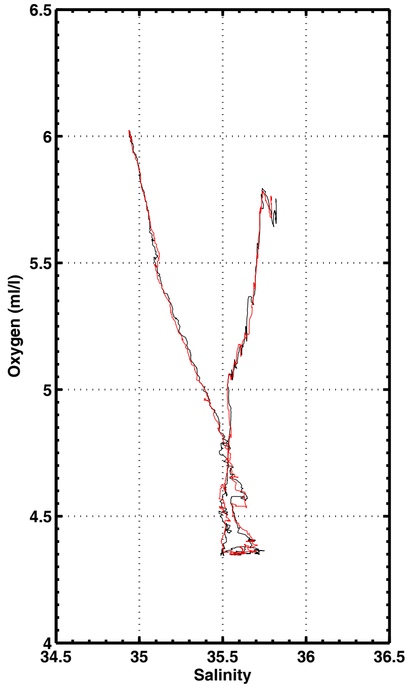
S-O2 , station 1115
