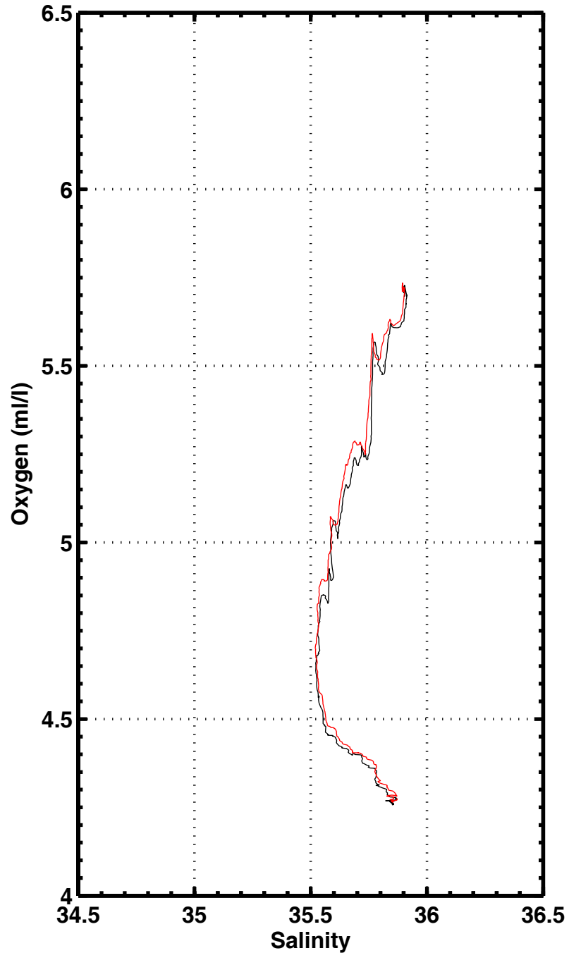
S-O2 , station 1100
