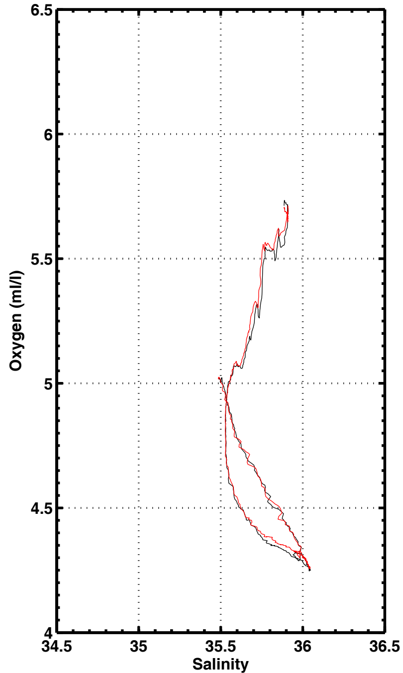
S-O2 , station 1085
