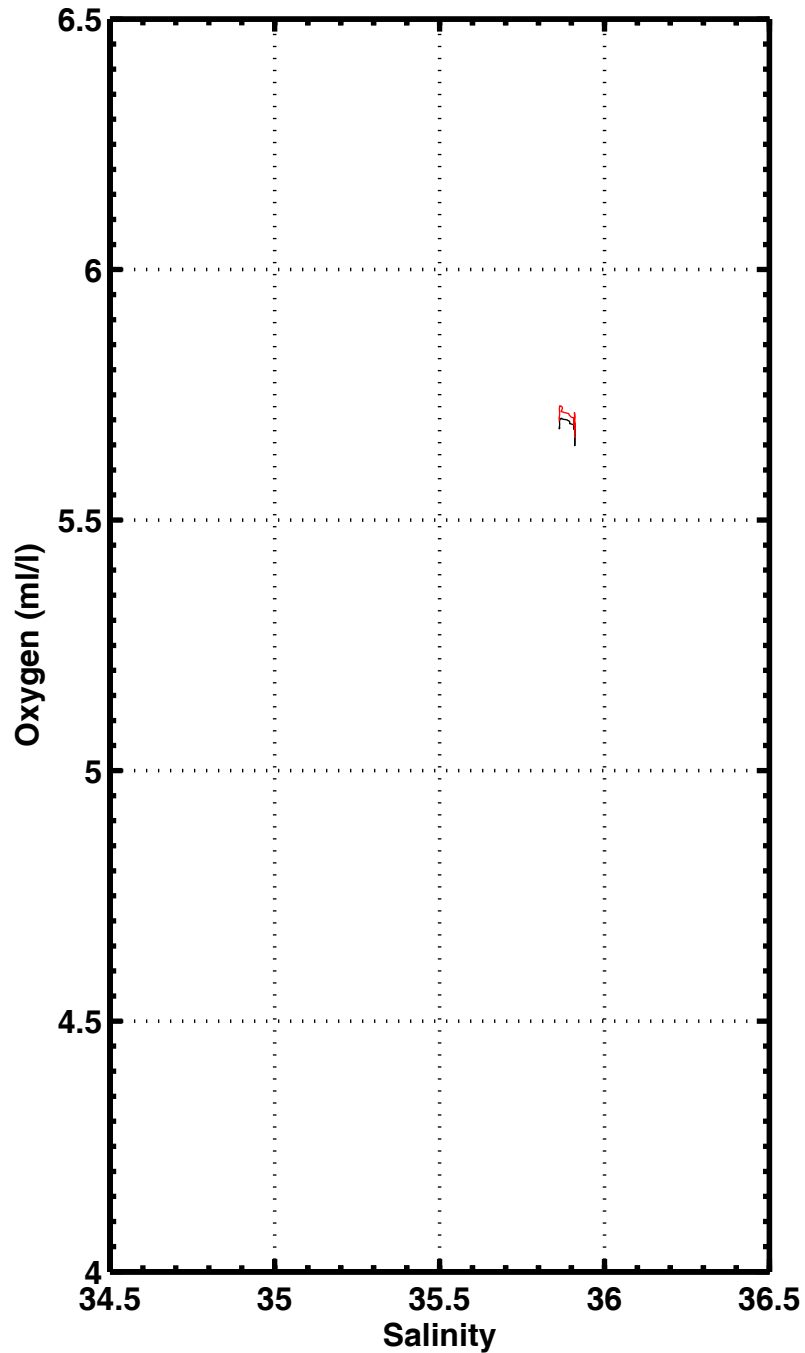
S-O2, station 1088
