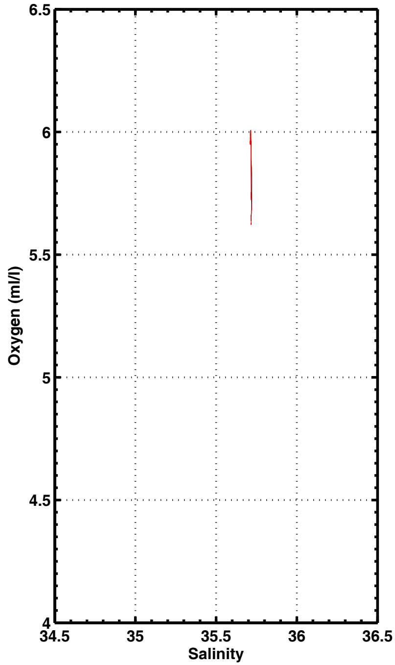
S-O2 , station 1172
