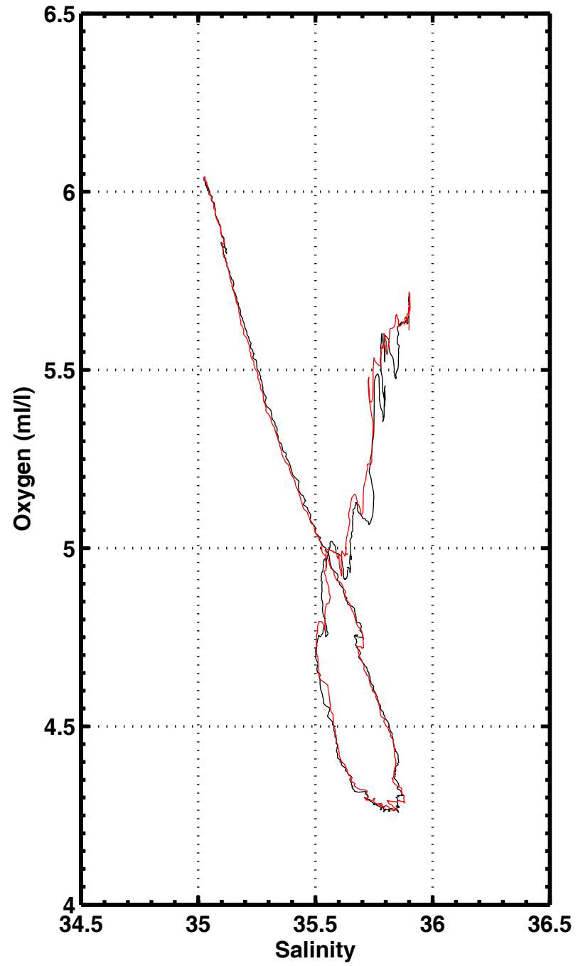
S-O2 , station 1034
