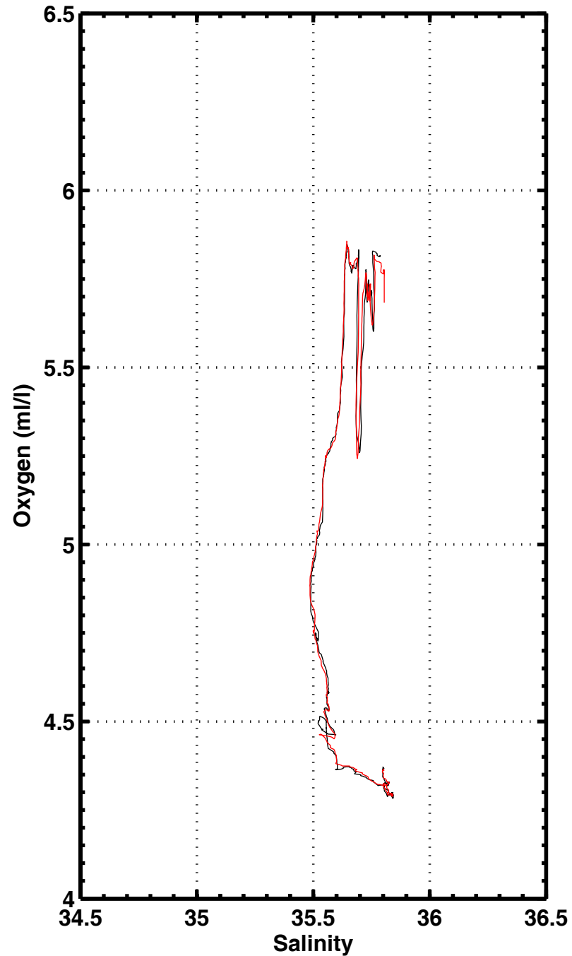
S-O2 , station 1194
