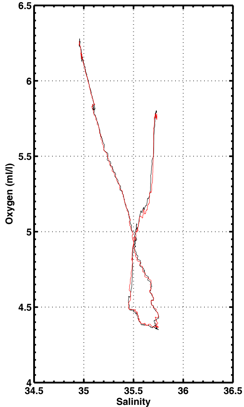
S-O2 , station 1021
