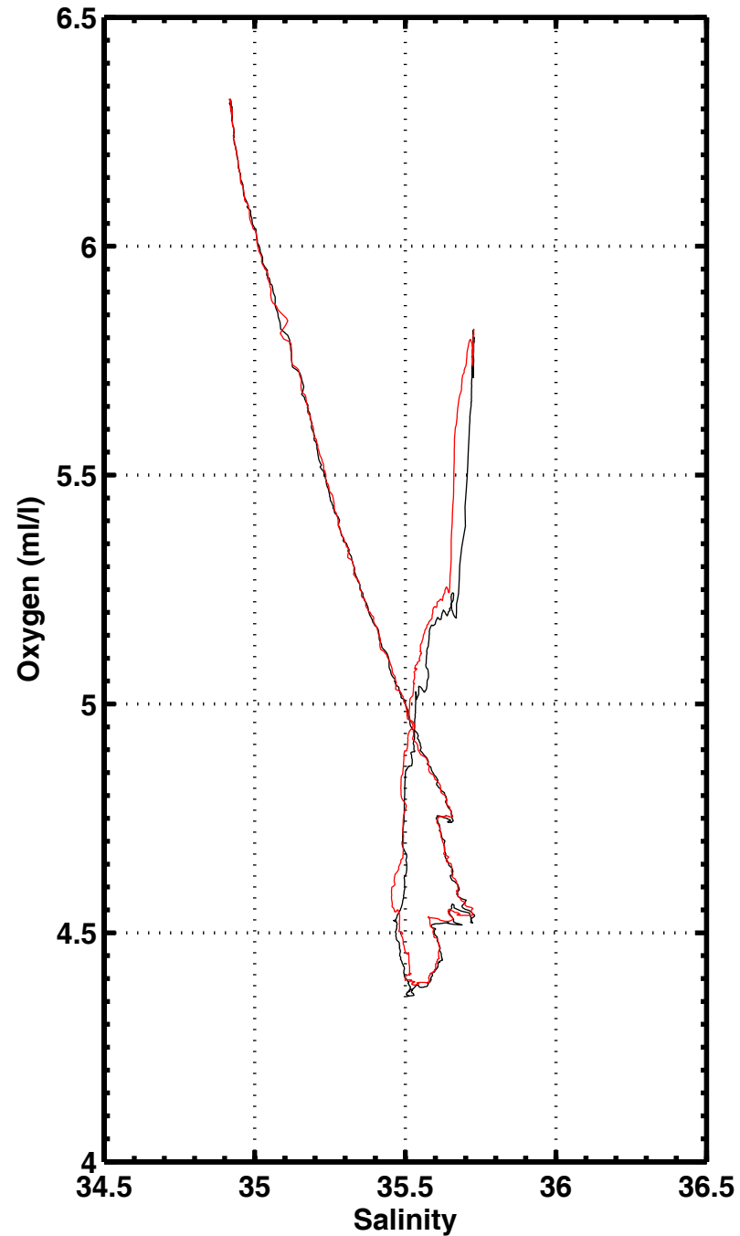
S-O2 , station 1042
