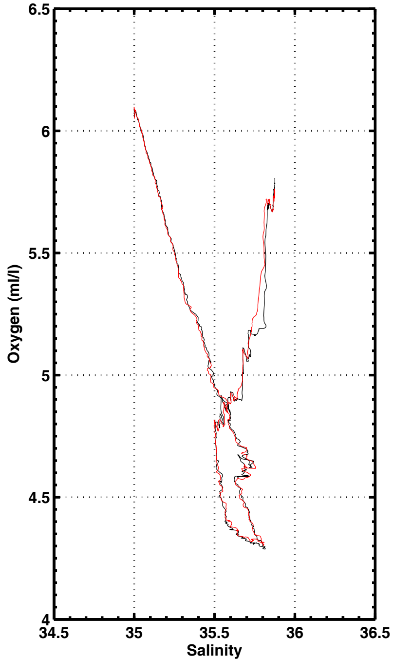
S-O2 , station 1033
