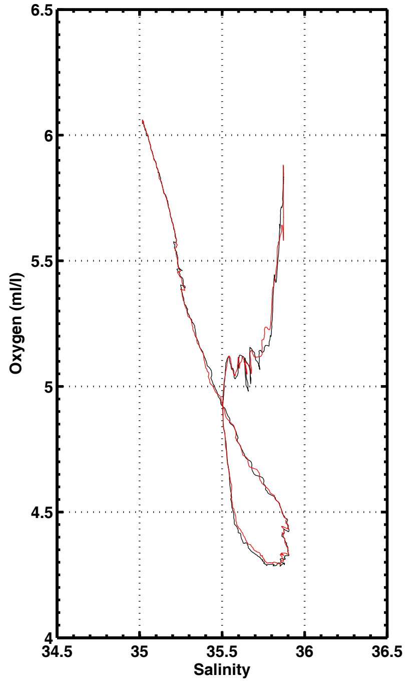
S-O2 , station 1055
