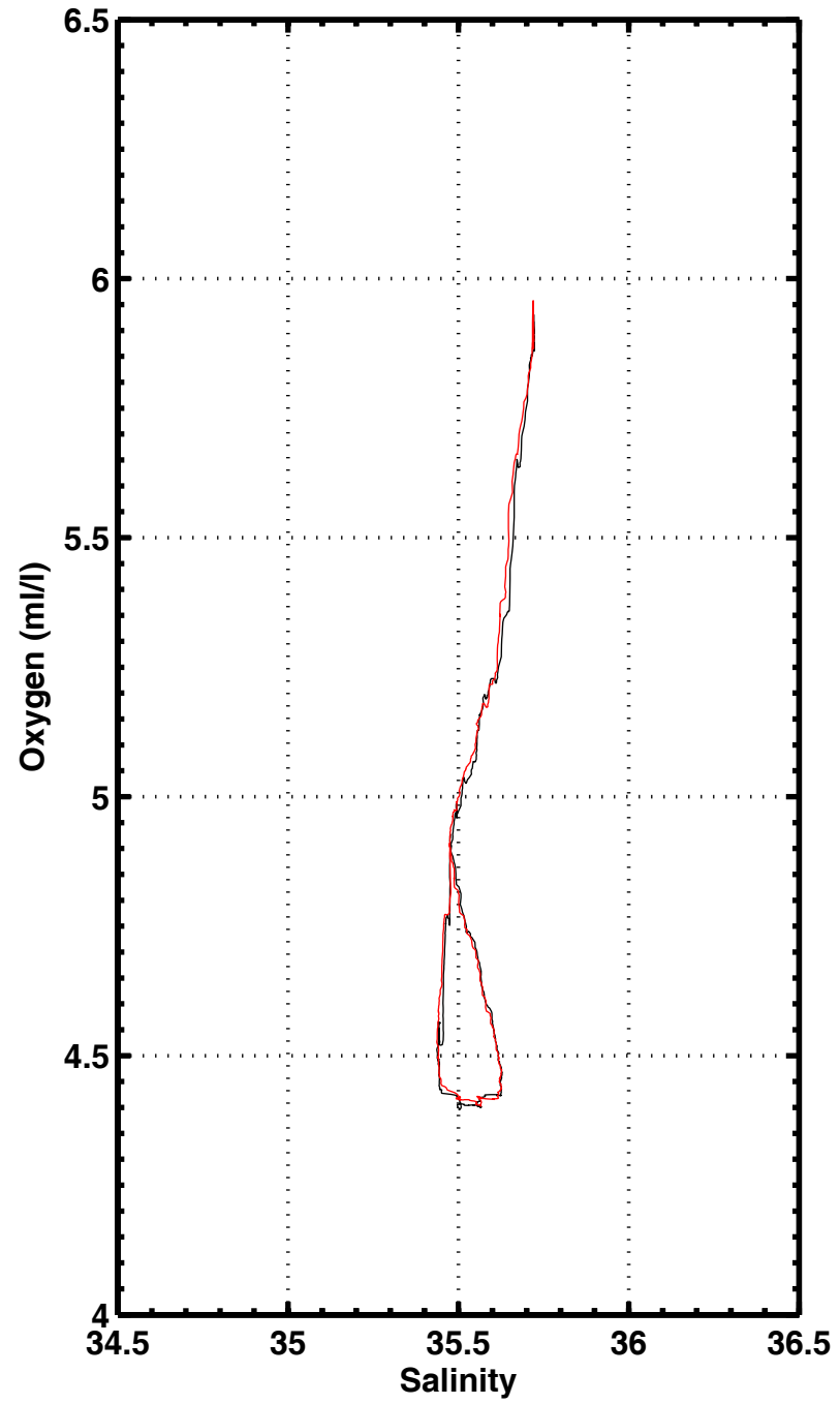
S-02 , station 1135
