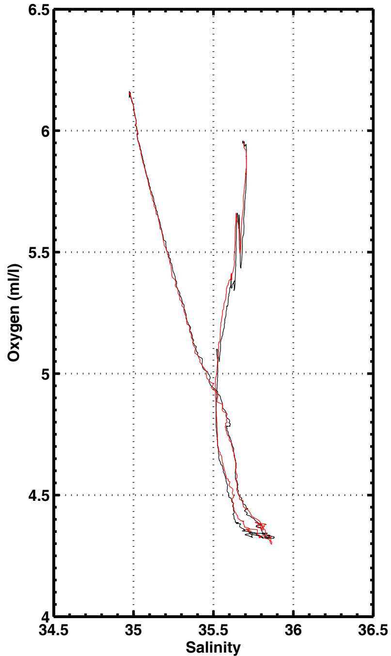
S-O2 , station 1040
