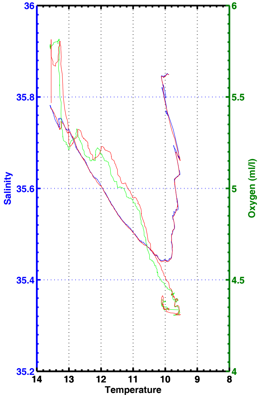
T-S , T-02 , station 1157
