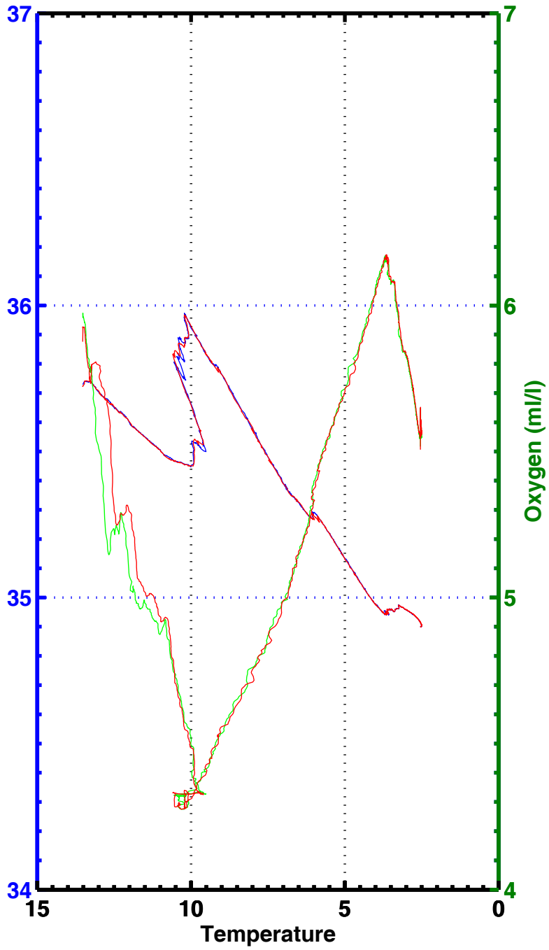
T-S , T-02 , station 1037
