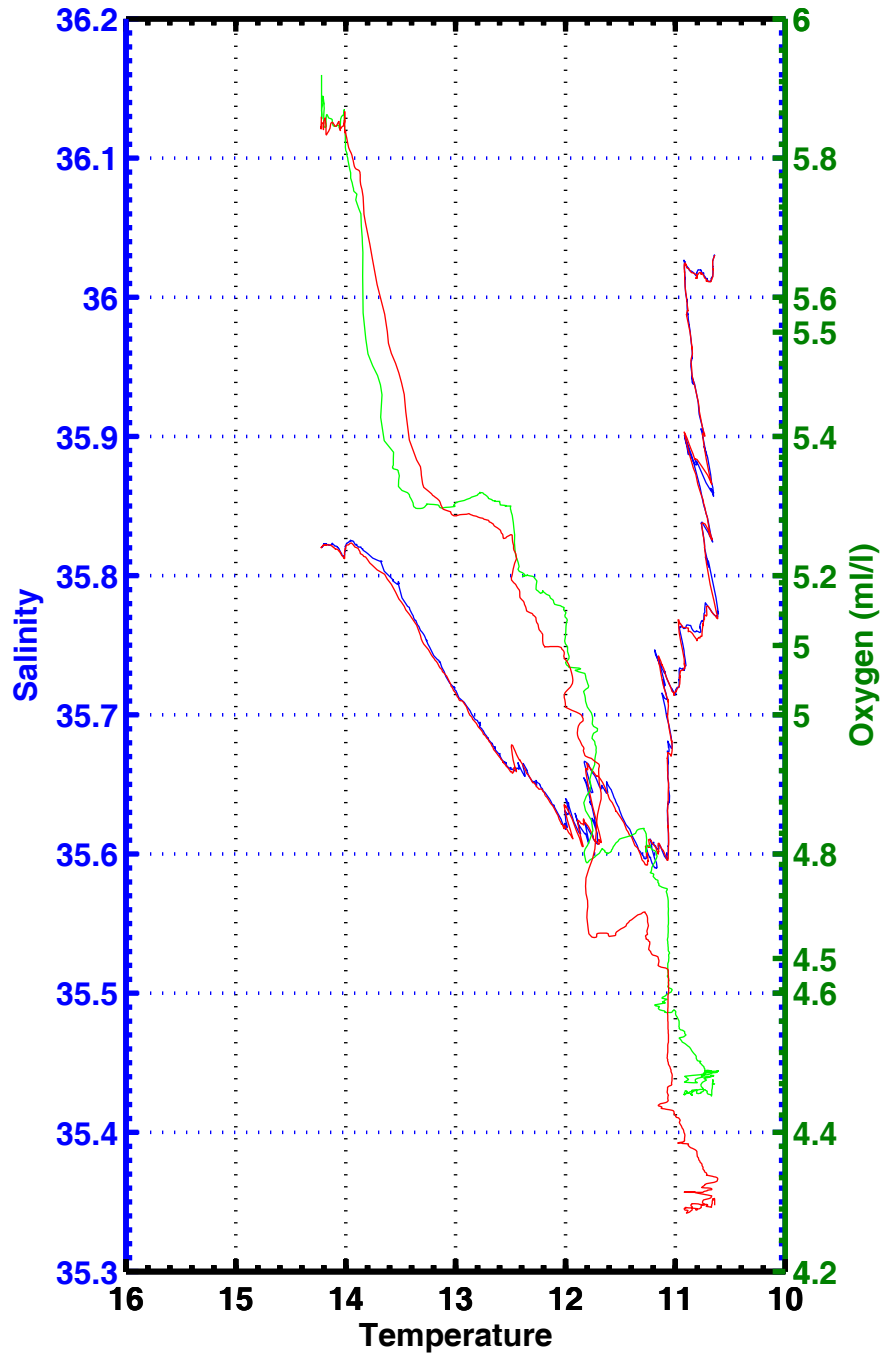
T-S , T-02 , station 1203
