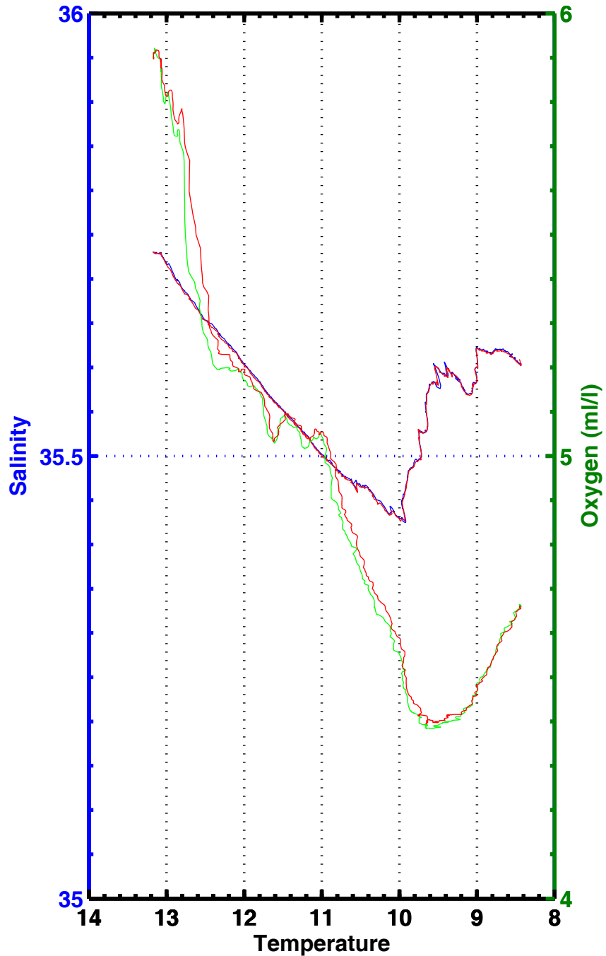
T-S , T-02 , station 1107
