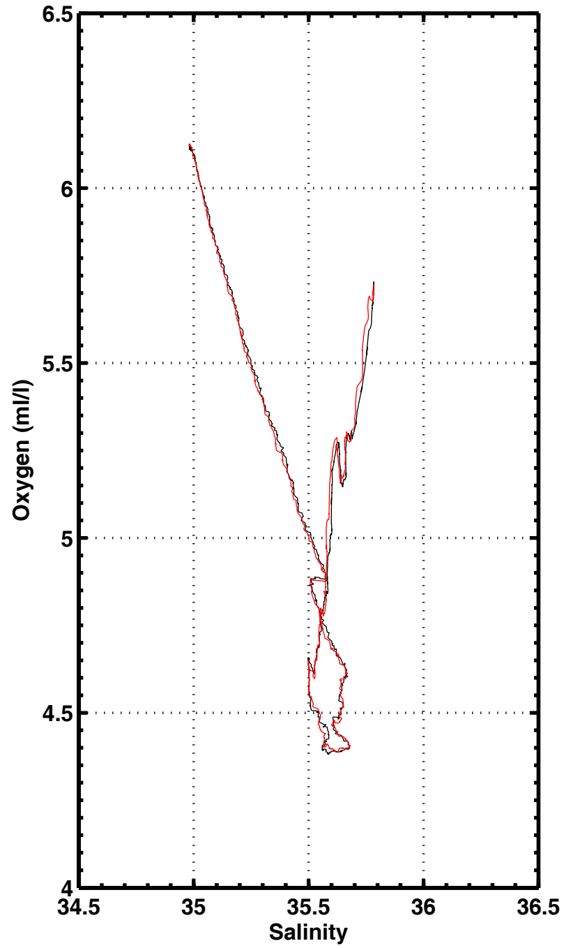
S-O2 , station 1007
