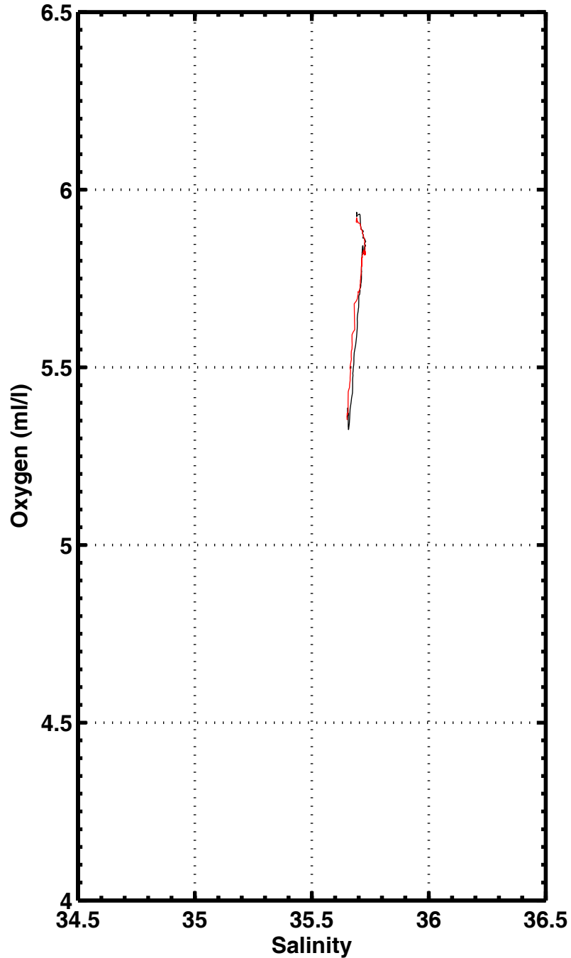
S-O2, station 1144
