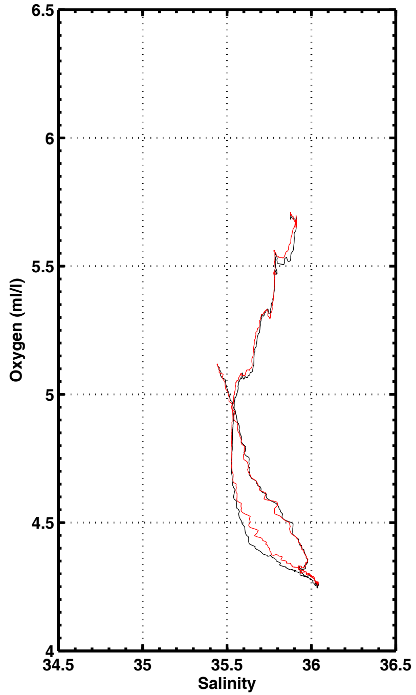
S-02 , station 1092
