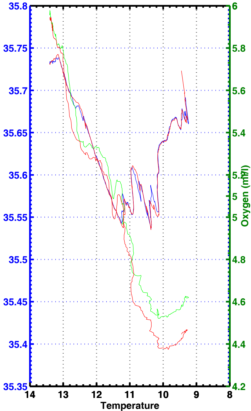
T-S , T-02 , station 1197
