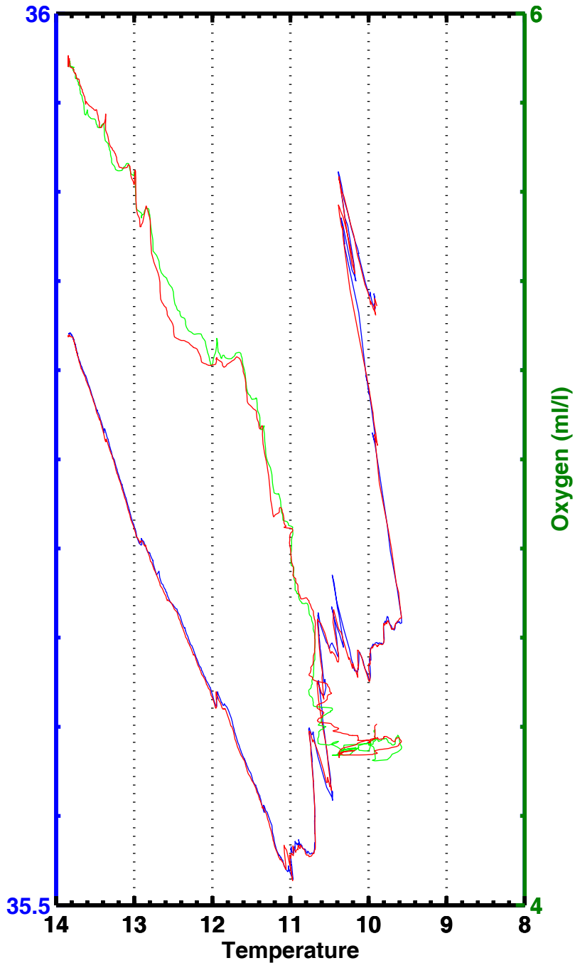
T-S , T-02 , station 1199
