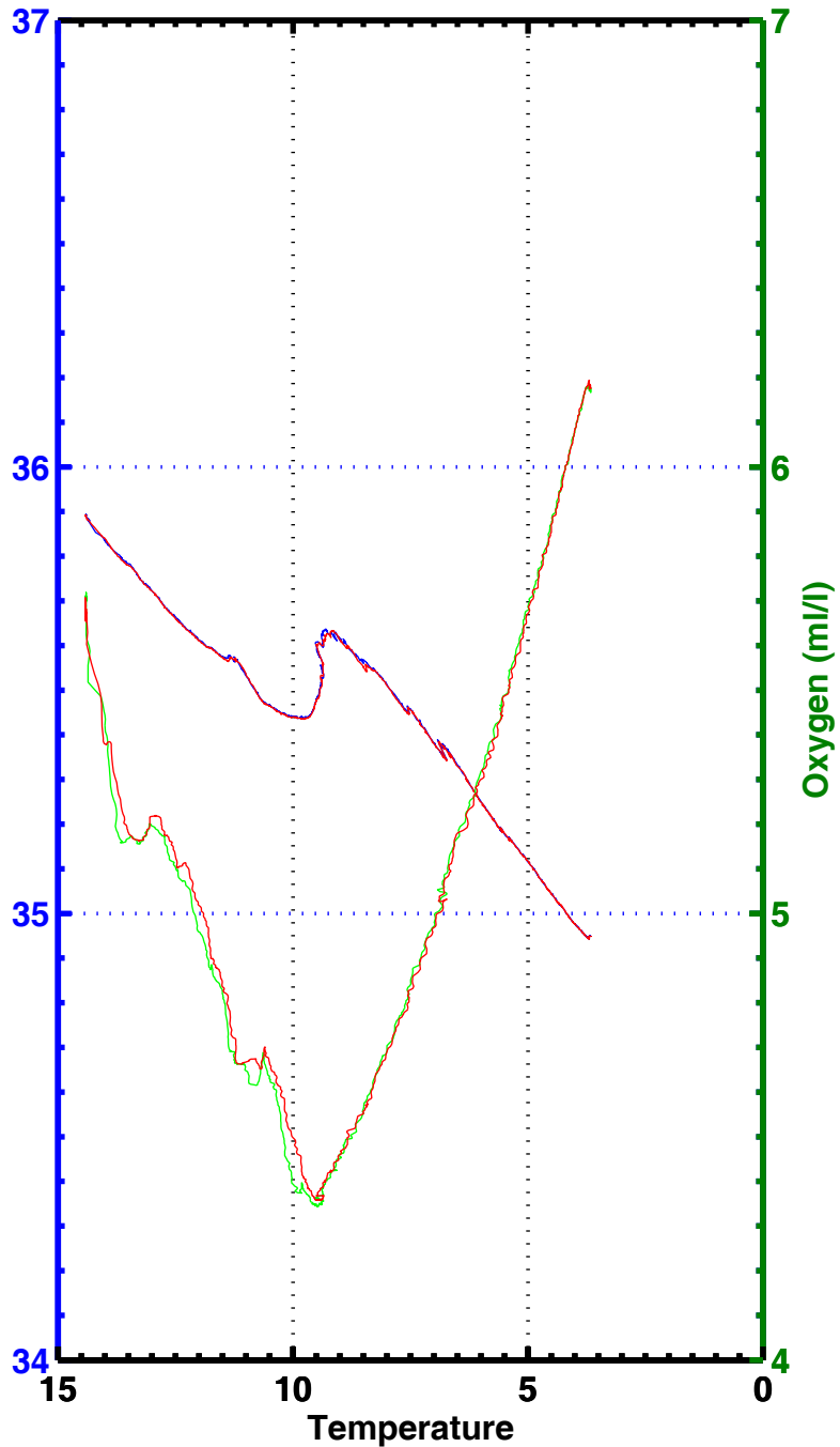
T-S , T-02 , station 1072
