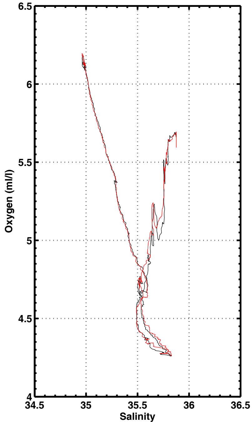
S-O2 , station 1027
