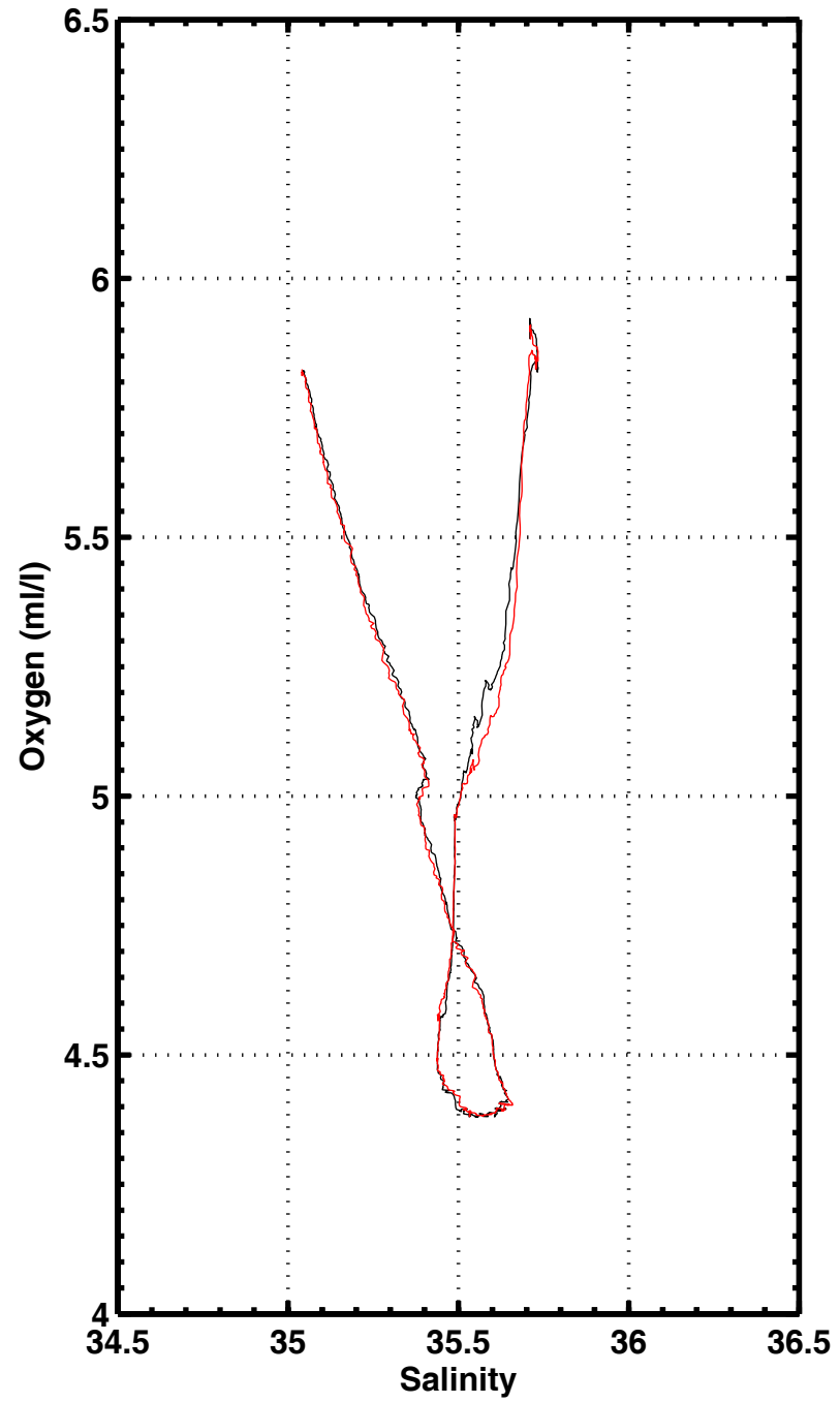
S-O2 , station 1141
