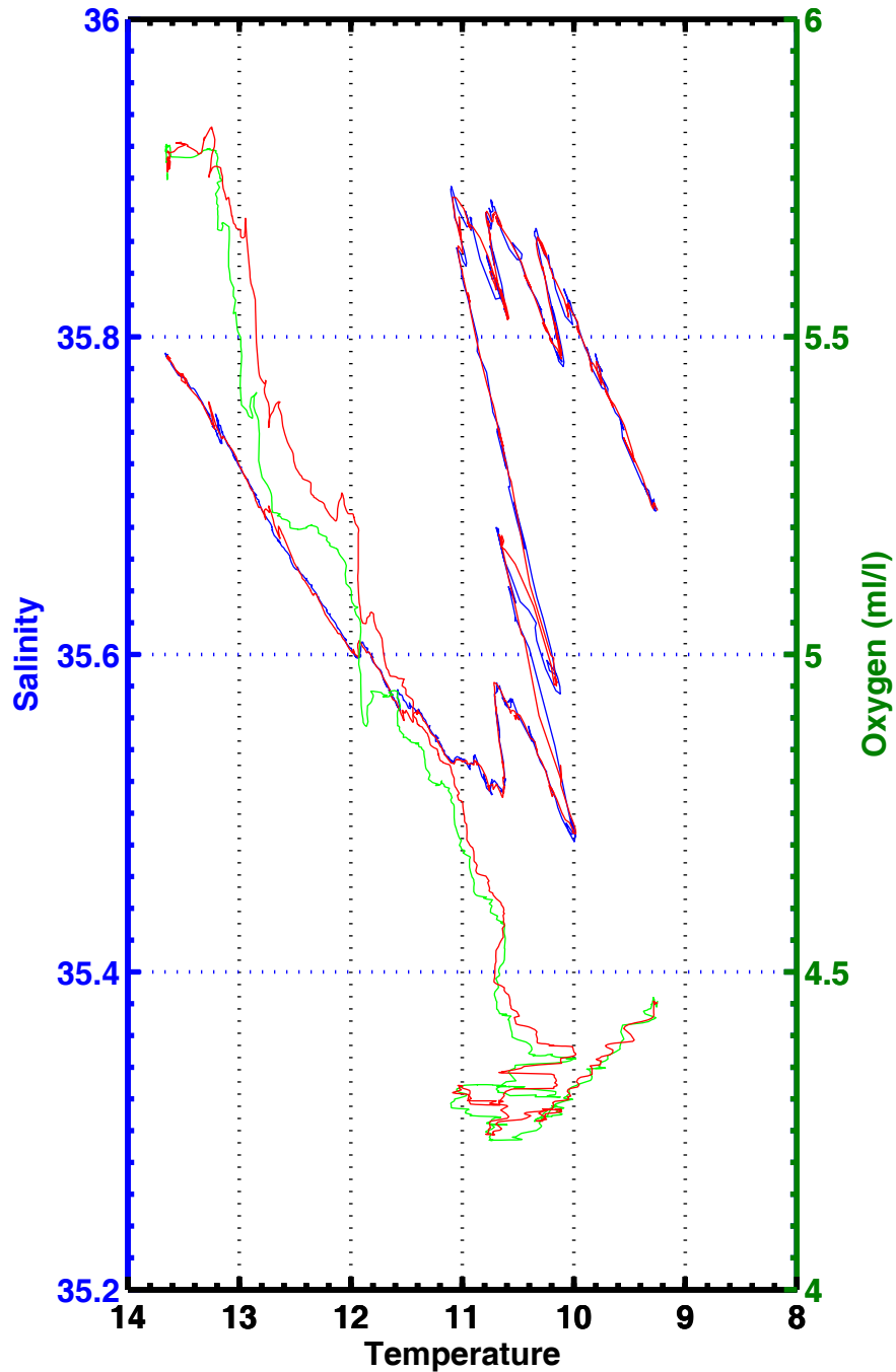
T-S , T-02 , station 1113
