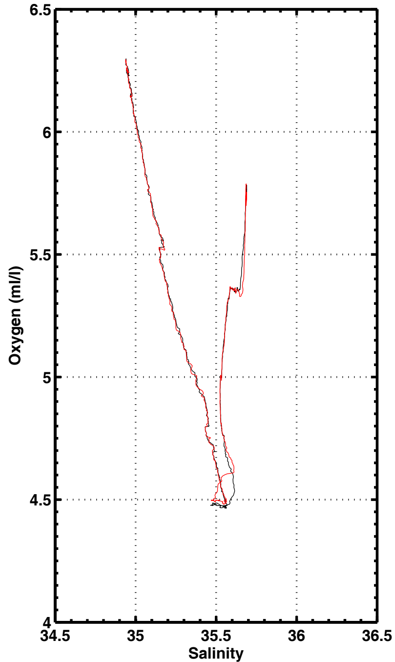
S-O2 , station 1013
