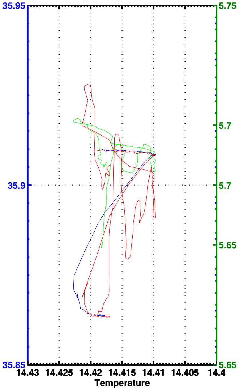
T-S, T-02, station 1088
