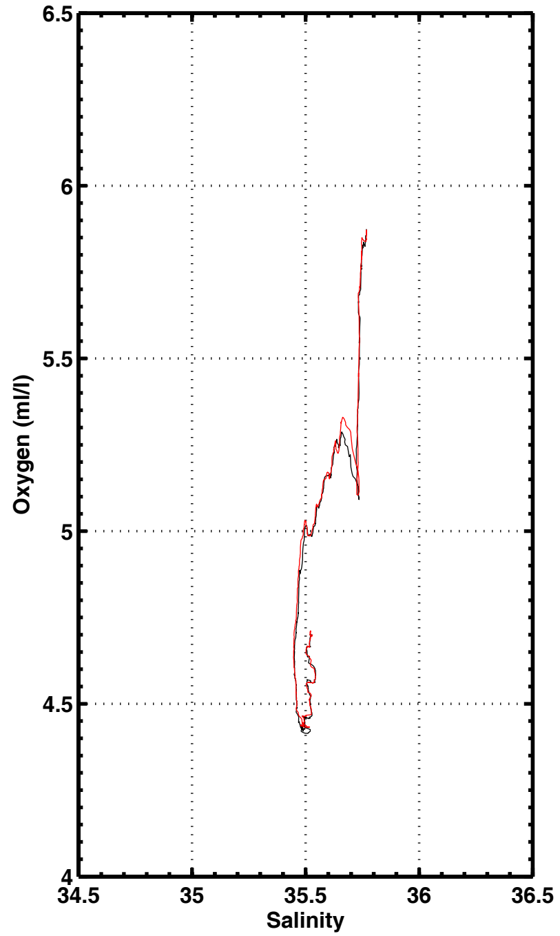
S-O2 , station 1154
