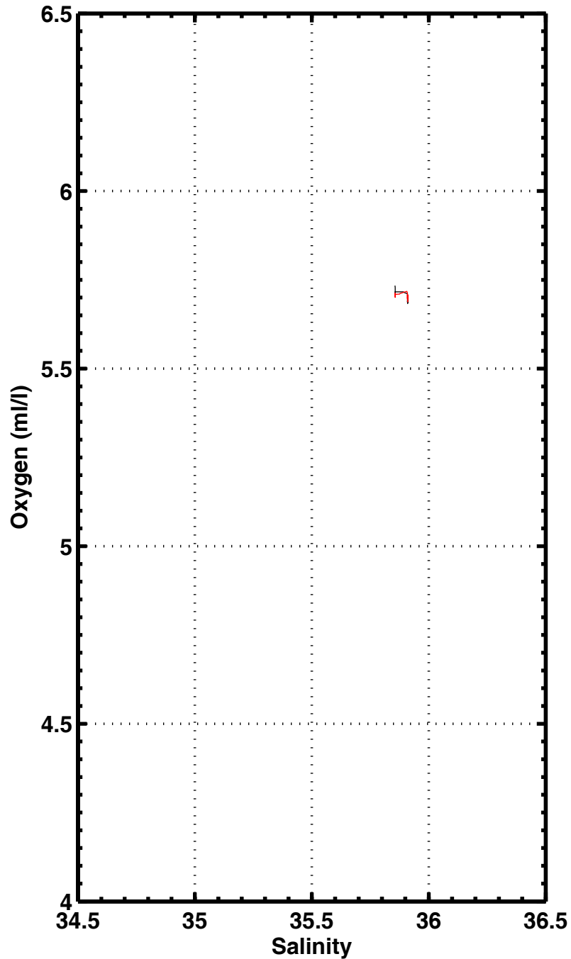
S-O2 , station 1089
