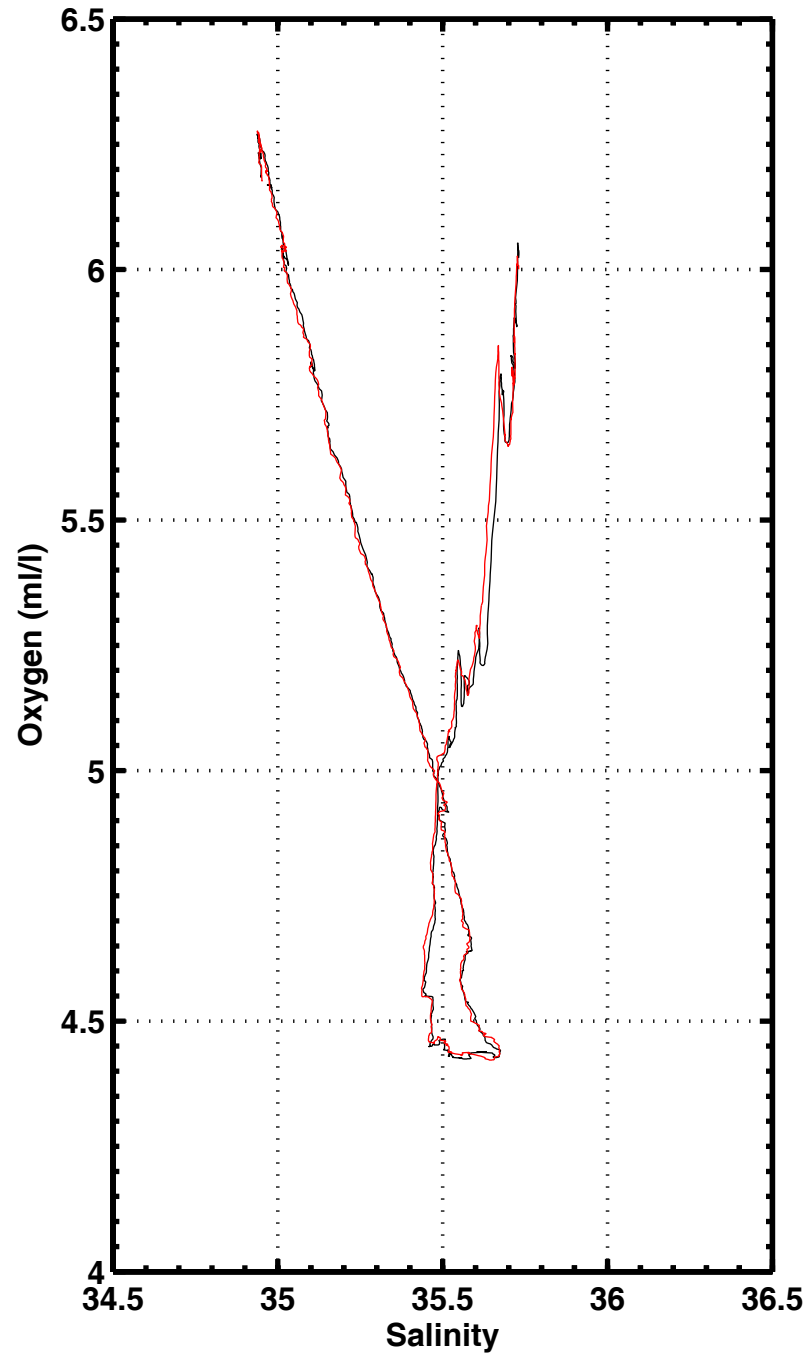
S-02 , station 1049
