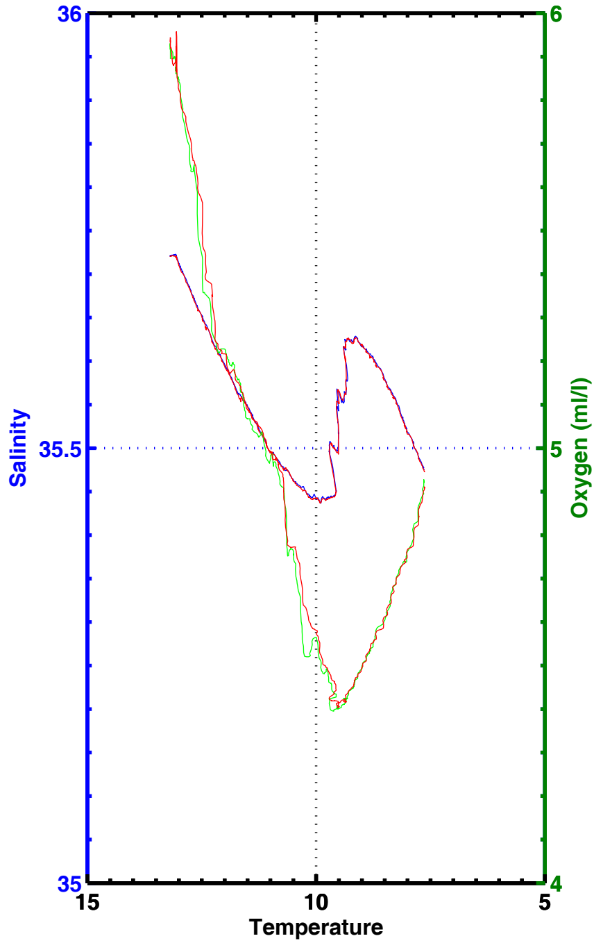
T-S , T-02 , station 1135
