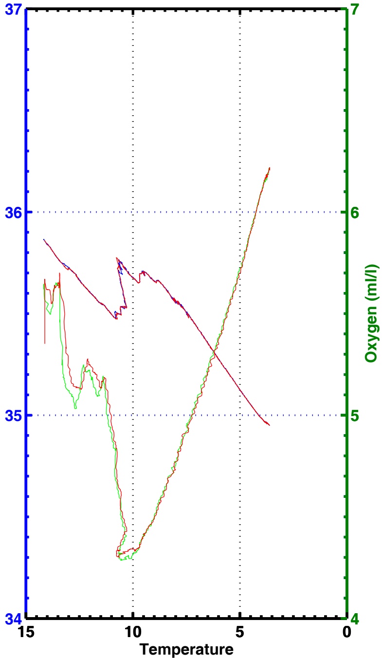
T-S , T-02 , station 1026
