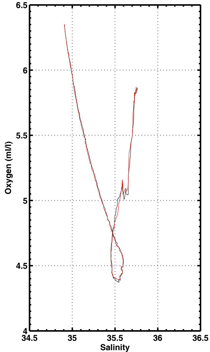
S-O2 , station 1065
