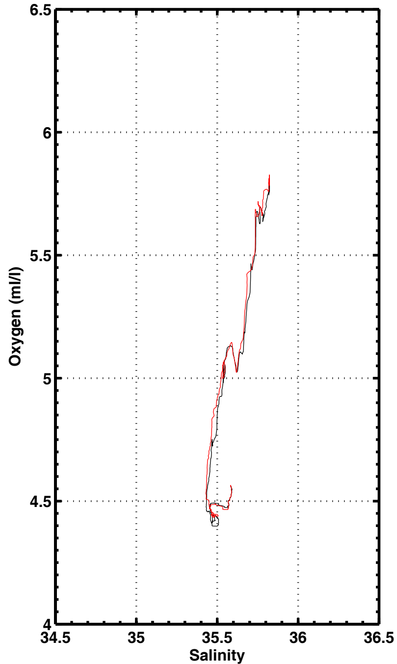
S-O2 , station 1126
