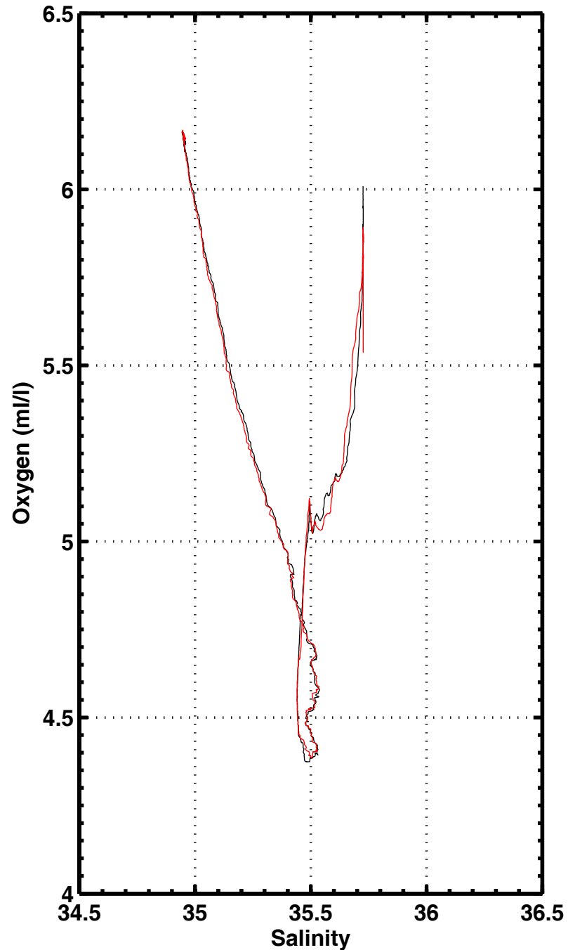
S-O2 , station 1068
