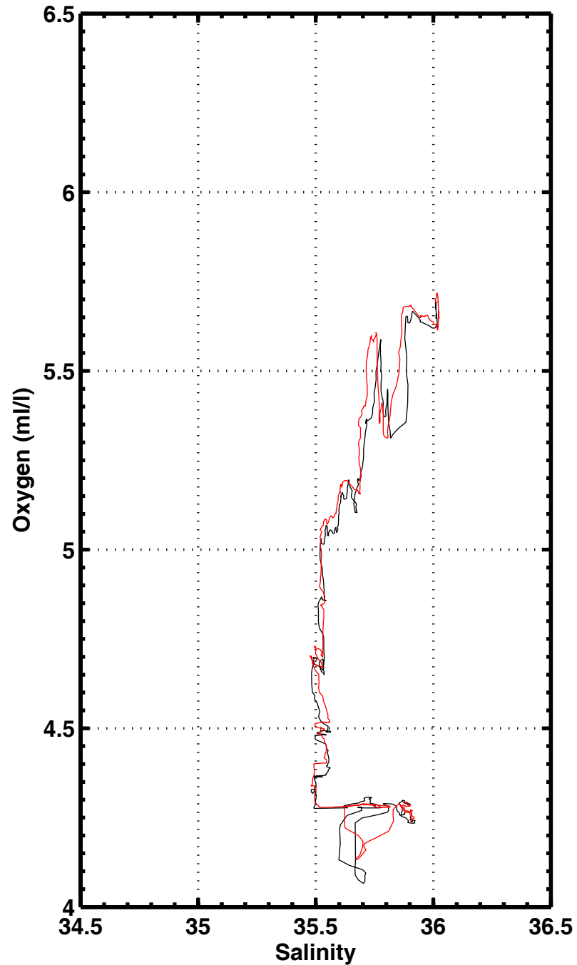
S-02 , station 1103
