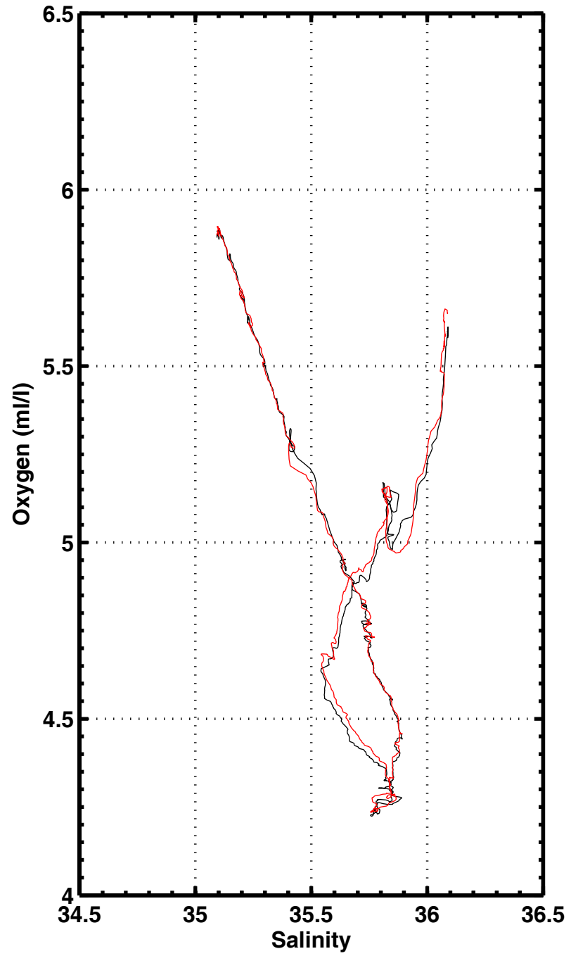
S-O2 , station 1057
