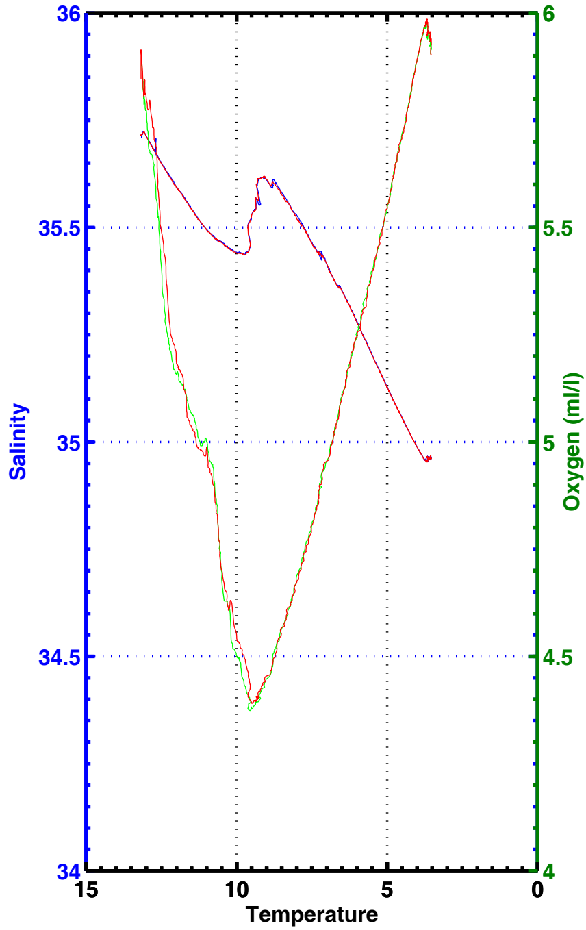
T-S , T-02 , station 1150
