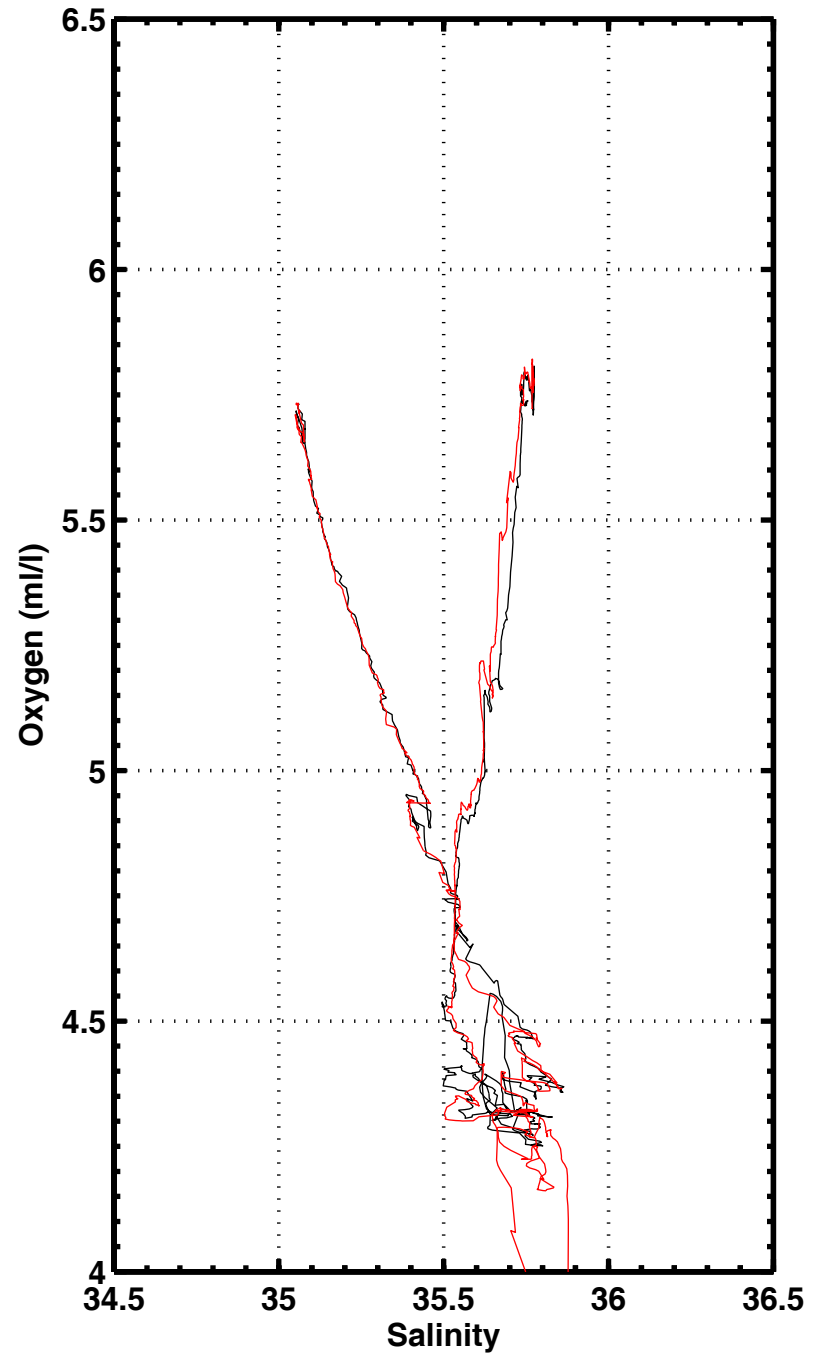
S-02 , station 1114
