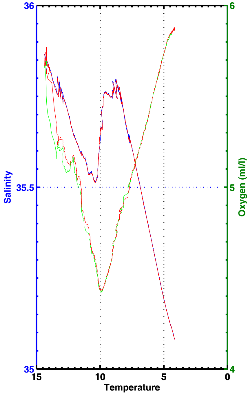
T-S , T-02 , station 1002
