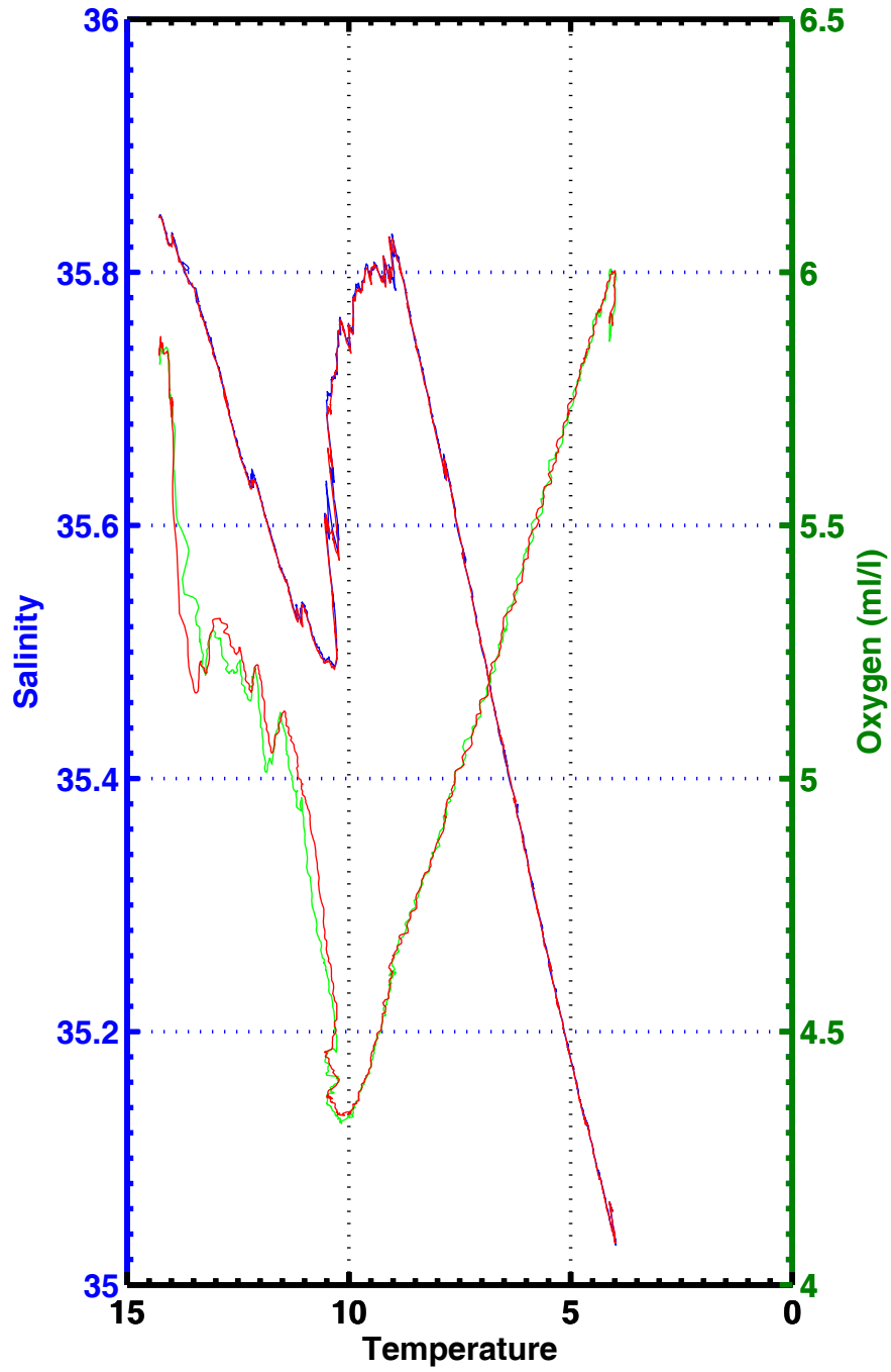
T-S , T-02 , station 1031
