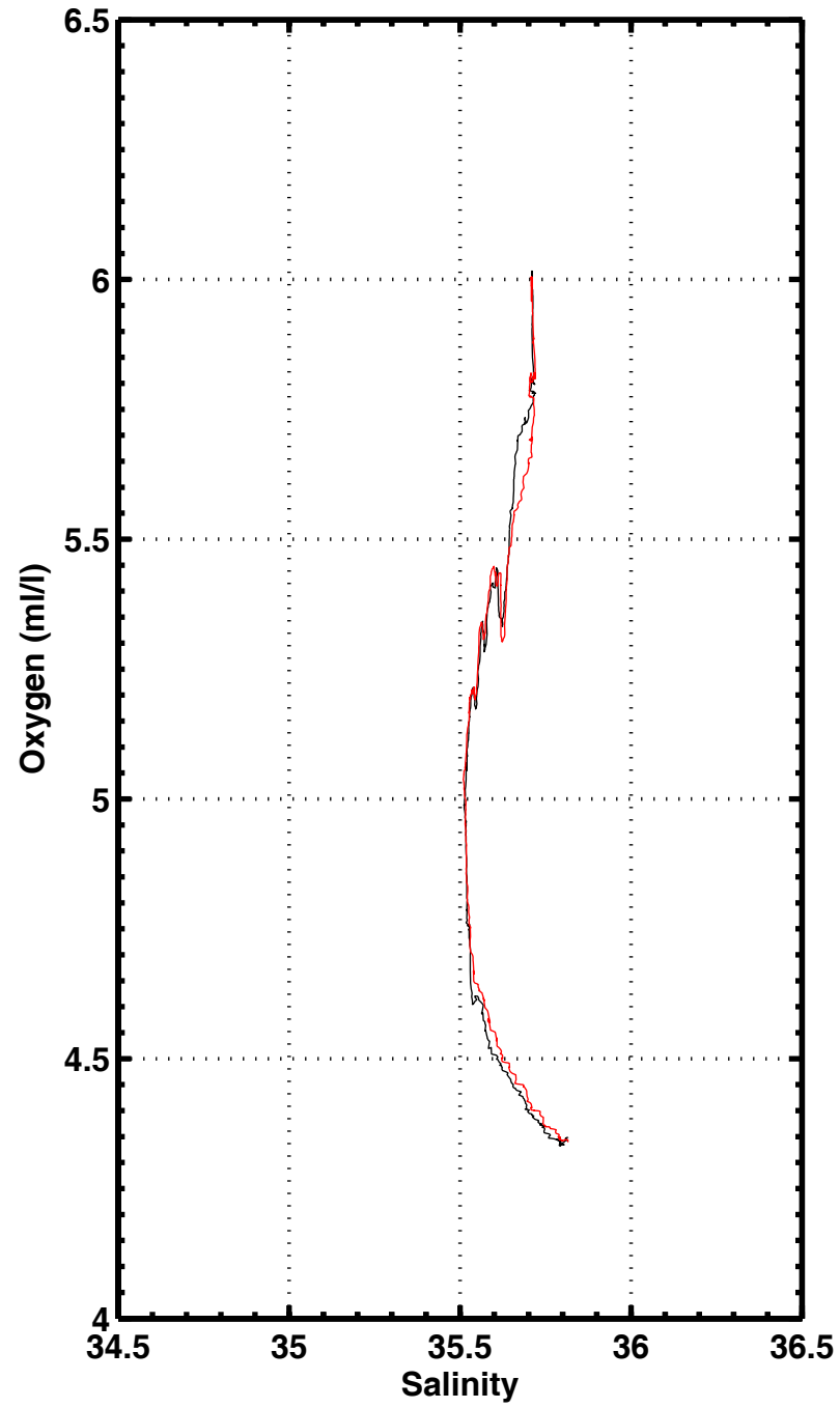
S-O2 , station 1169
