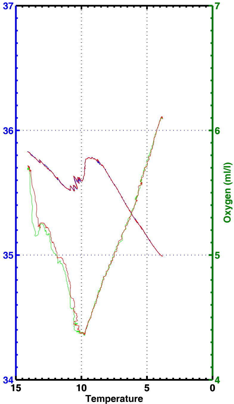
T-S , T-02 , station 1004
