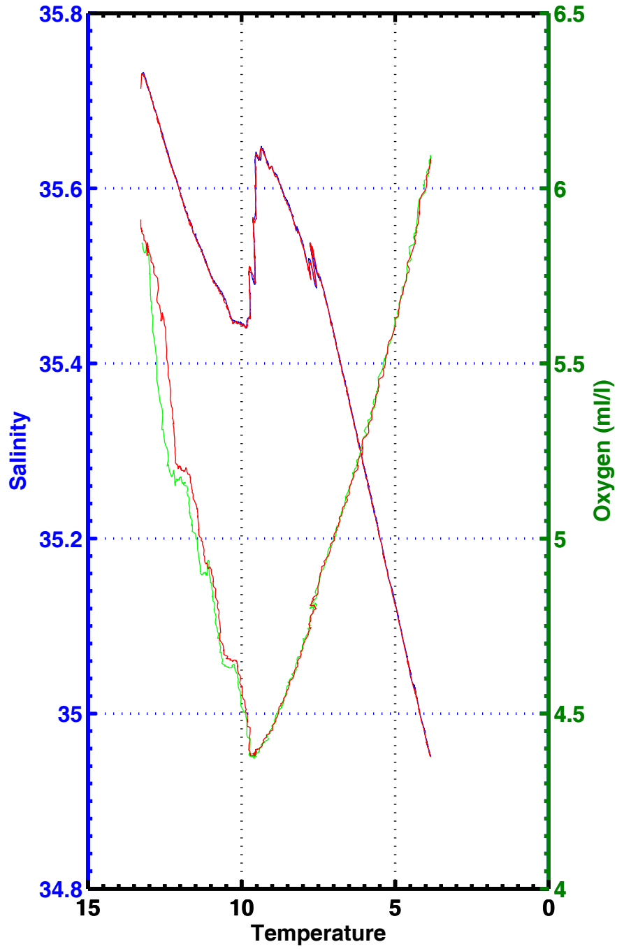
T-S , T-02 , station 1139
