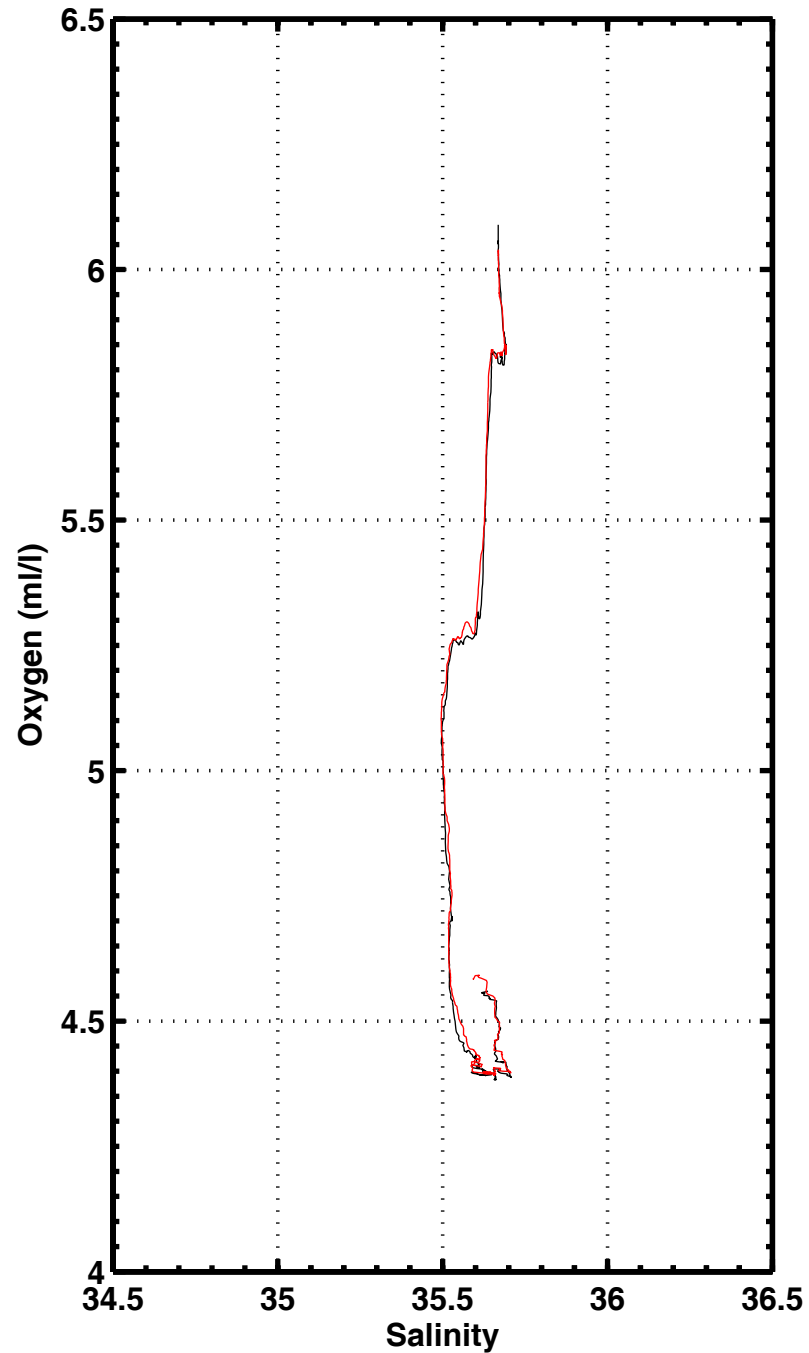
S-O2 , station 1189
