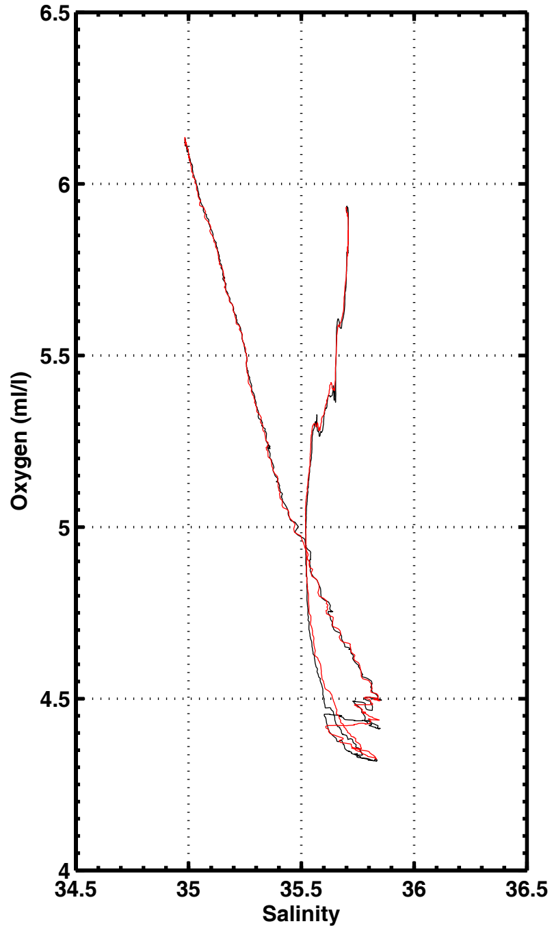
S-O2 , station 1041
