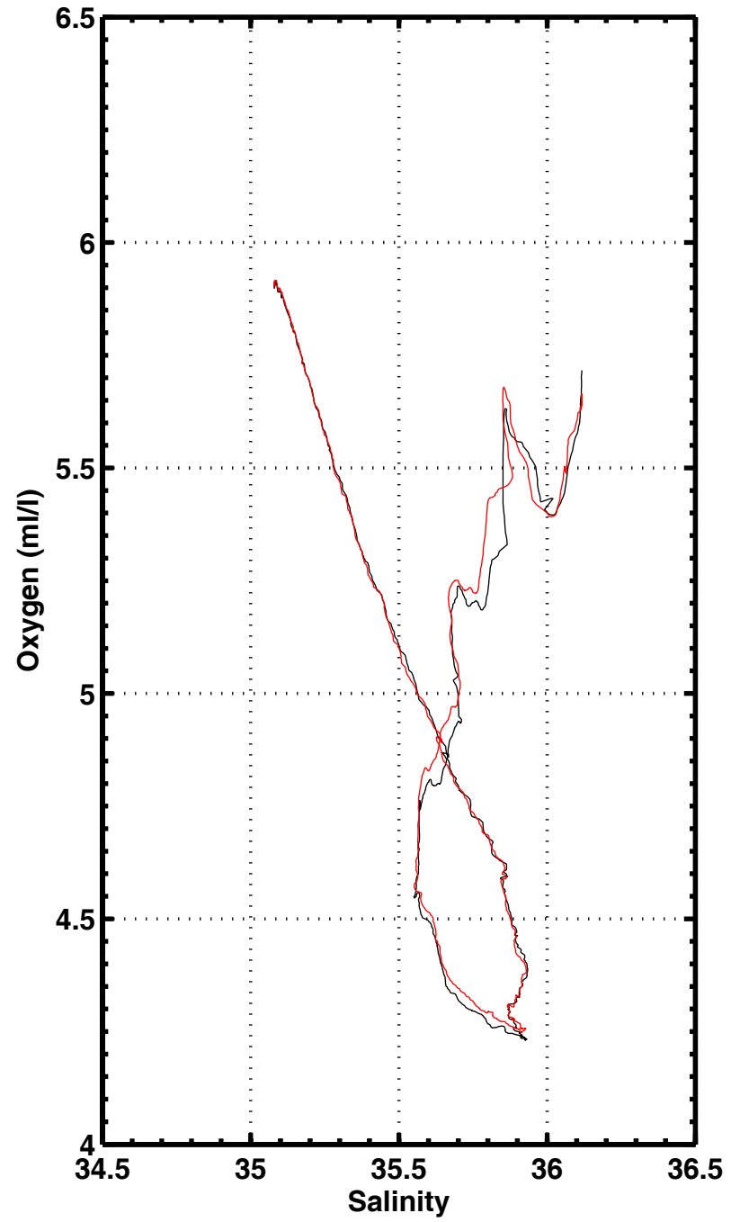
S-O2 , station 1056
