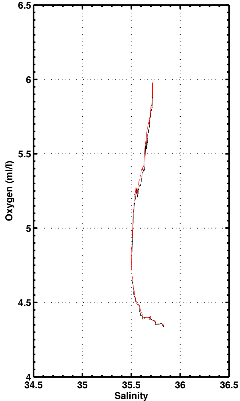
S-02 , station 1161
