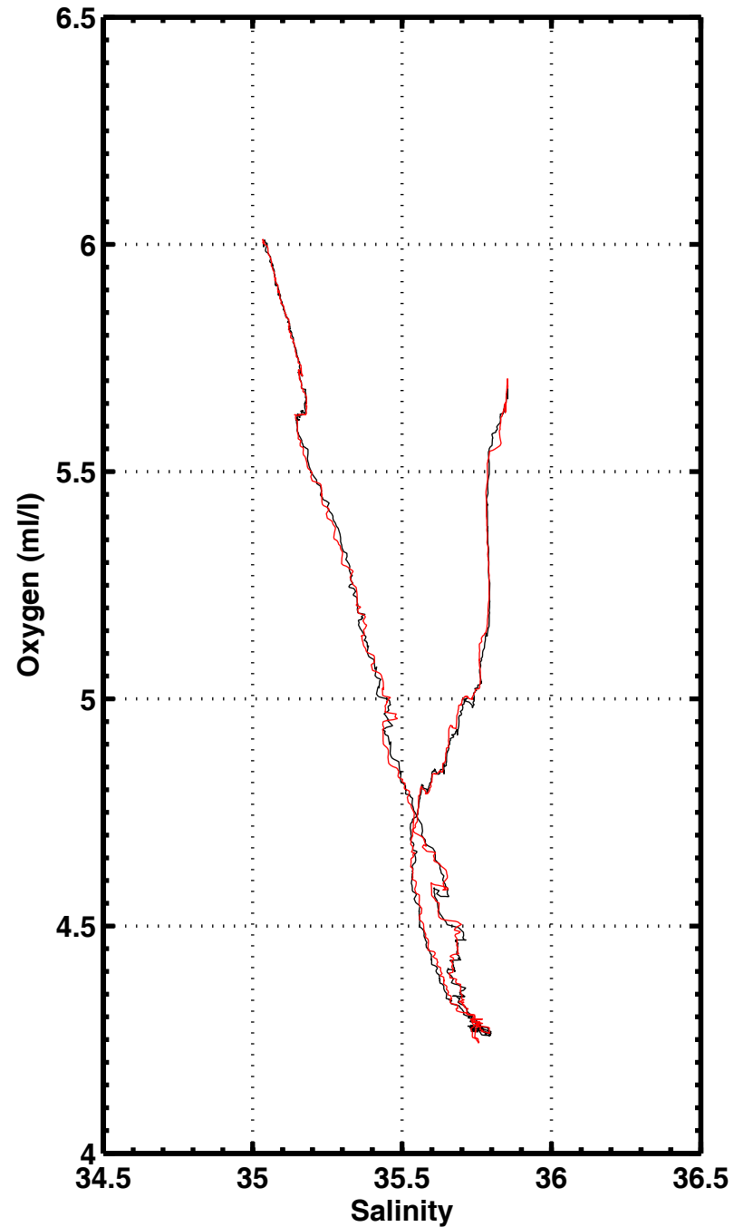
S-O2 , station 1028
