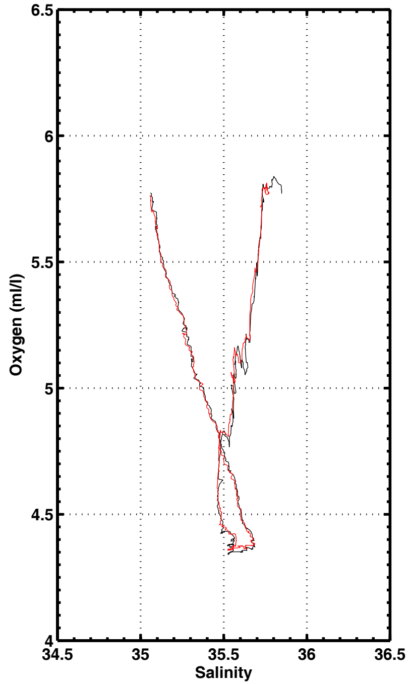
S-O2 , station 1119
