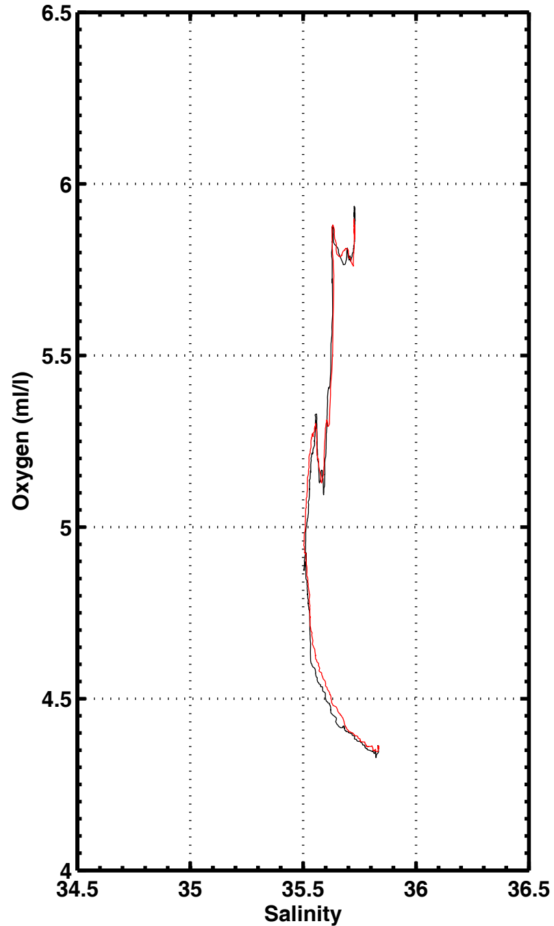
S-02 , station 1164
