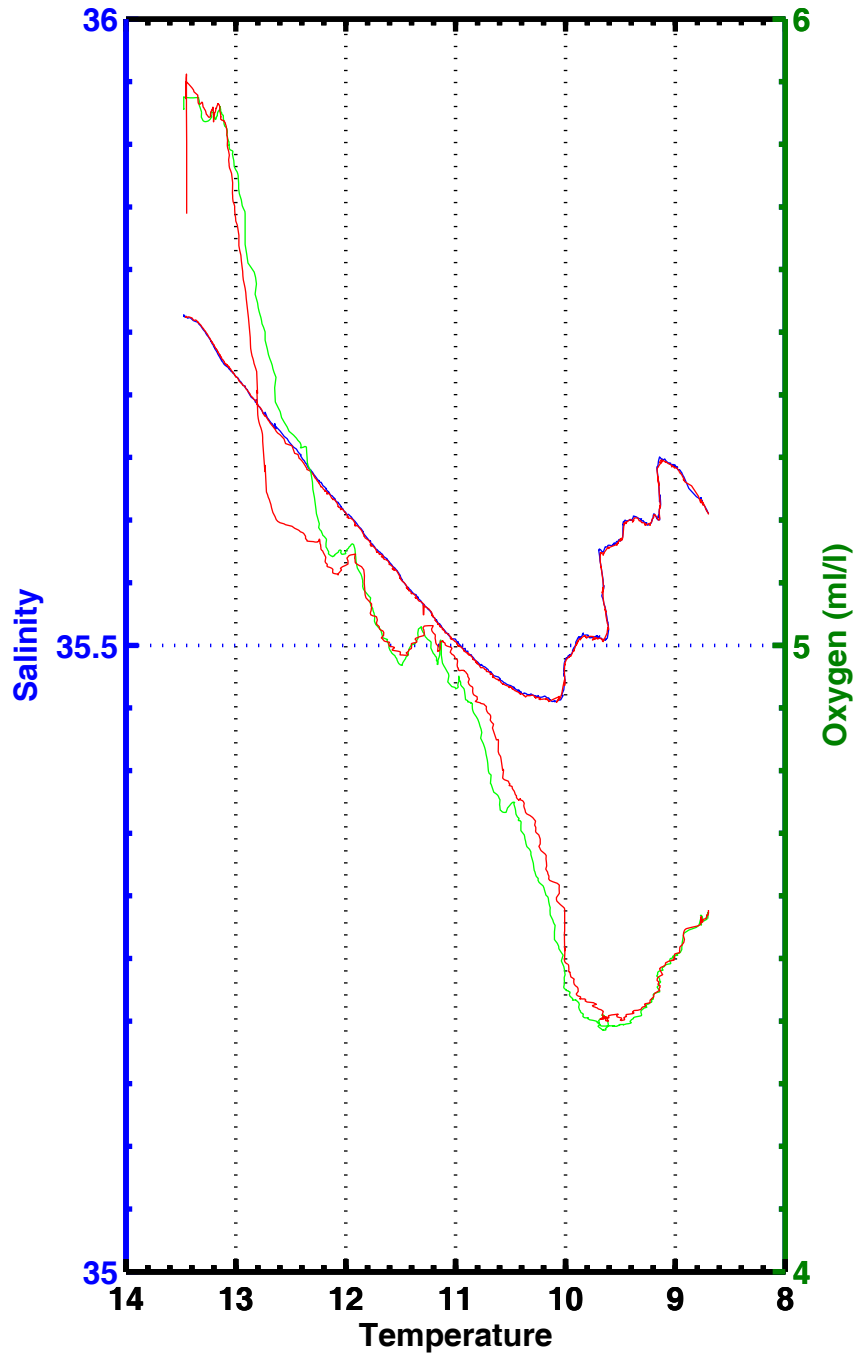
T-S , T-02 , station 1128
