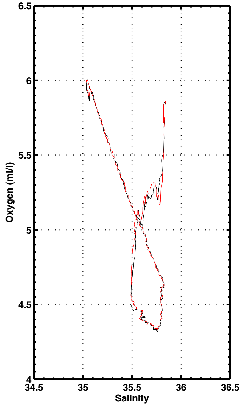
S-O2 , station 1031
