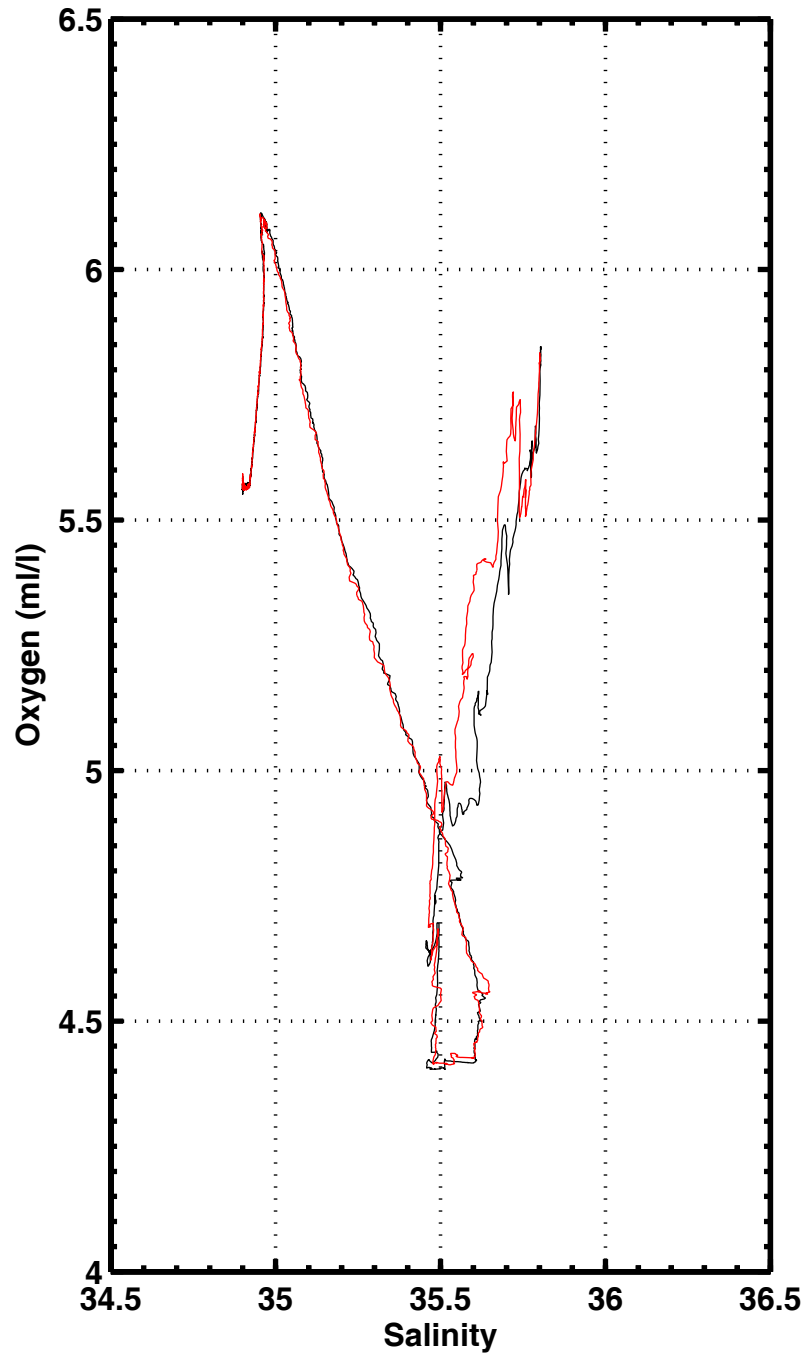
S-02 , station 1051
