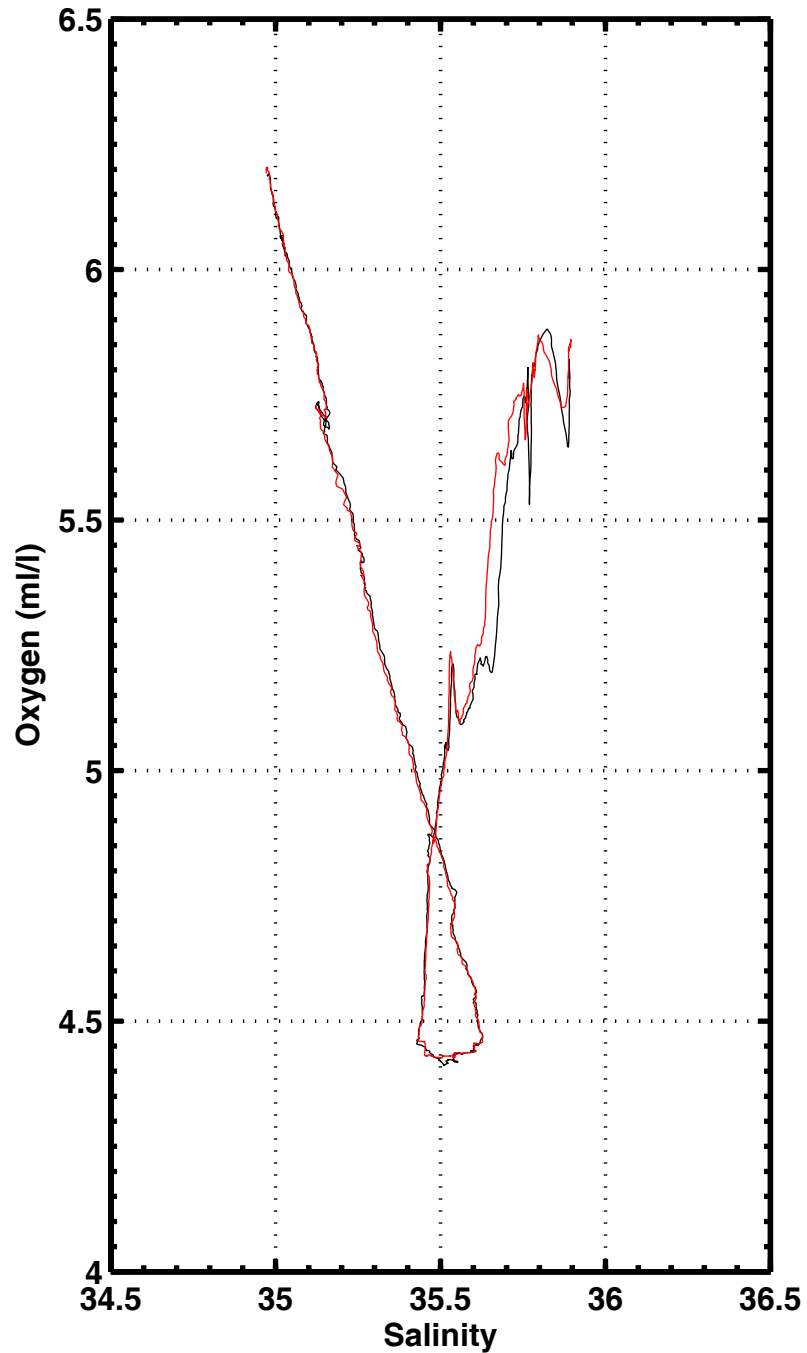
S-O2 , station 1052
