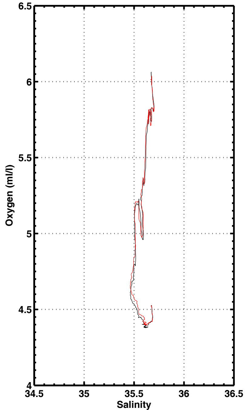
S-O2 , station 1192
