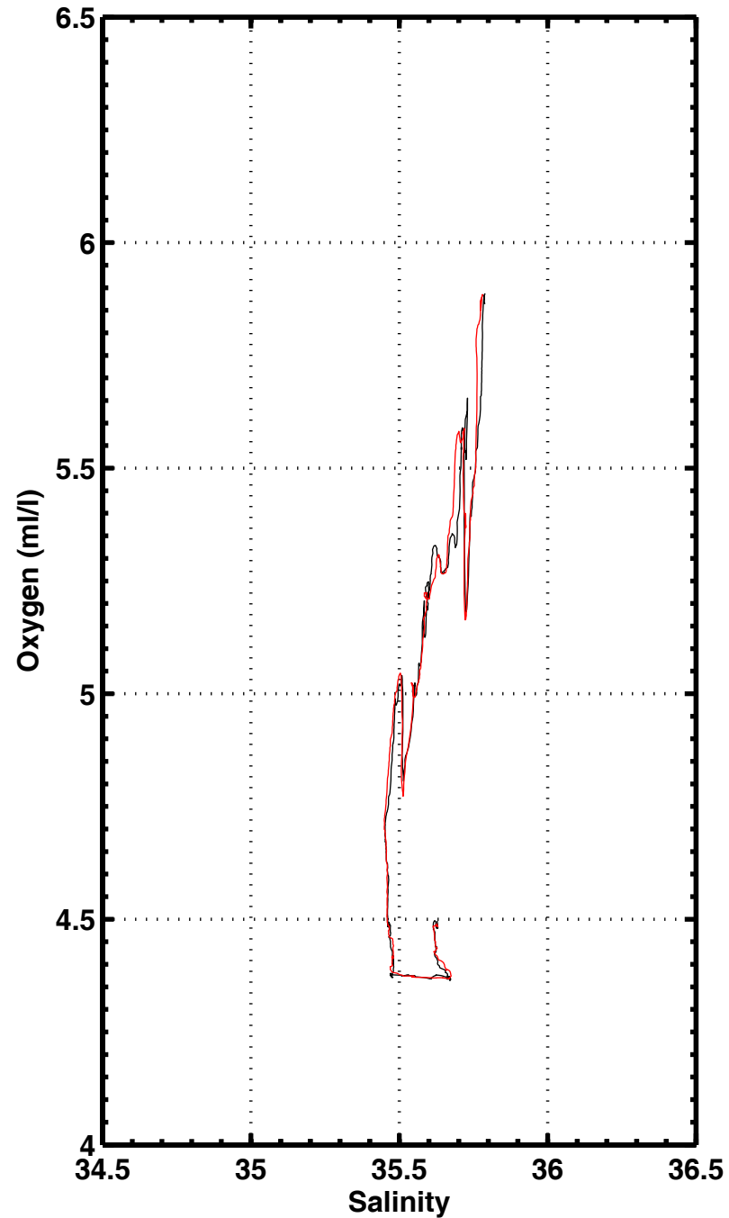
S-O2 , station 1104
