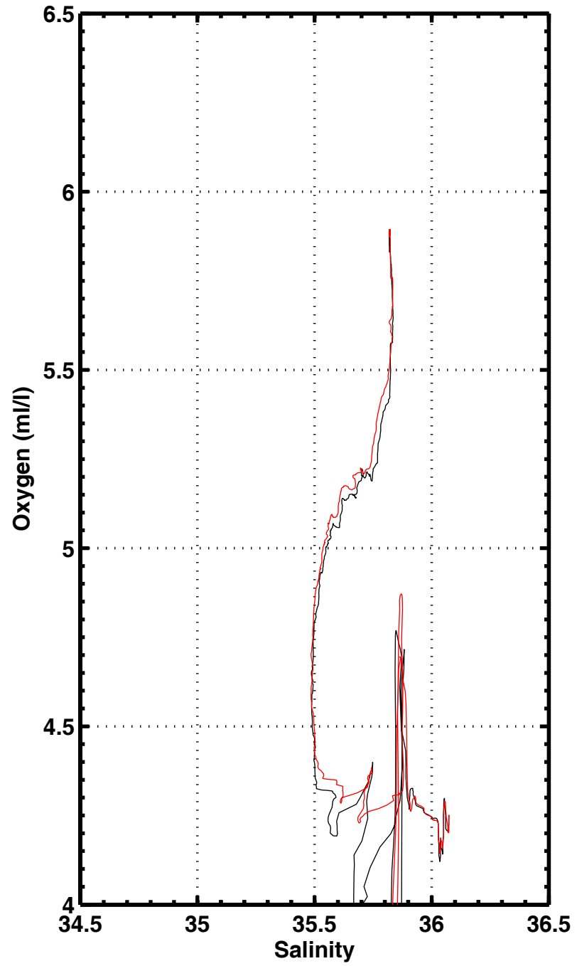
S-O2 , station 1204
