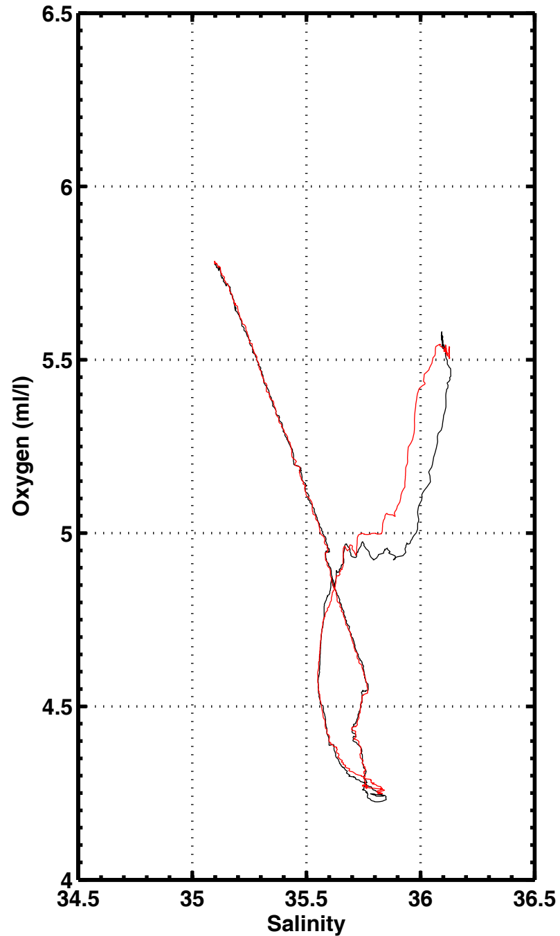
S-O2 , station 1076
