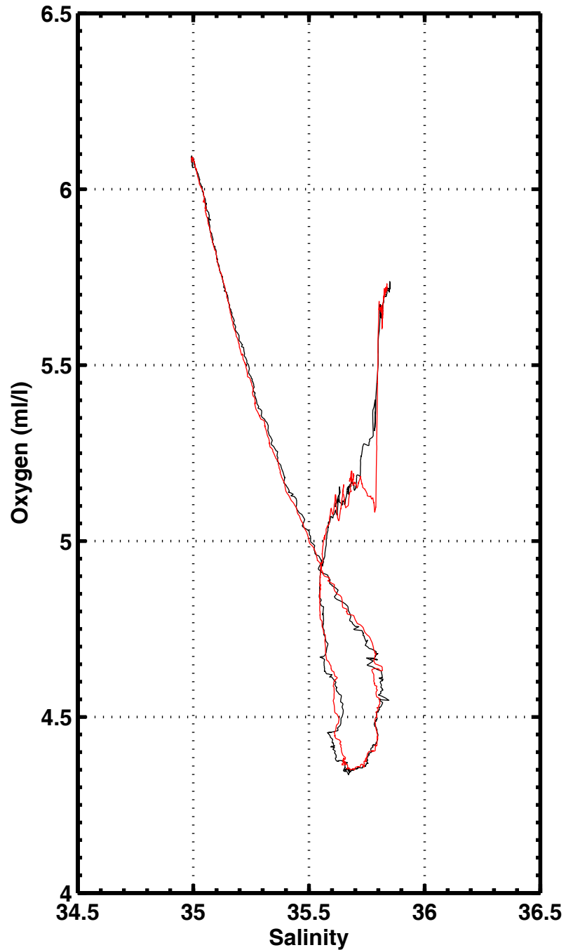
S-O2 , station 1005
