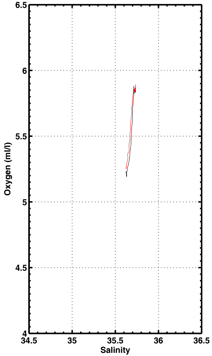
S-O2 , station 1137
