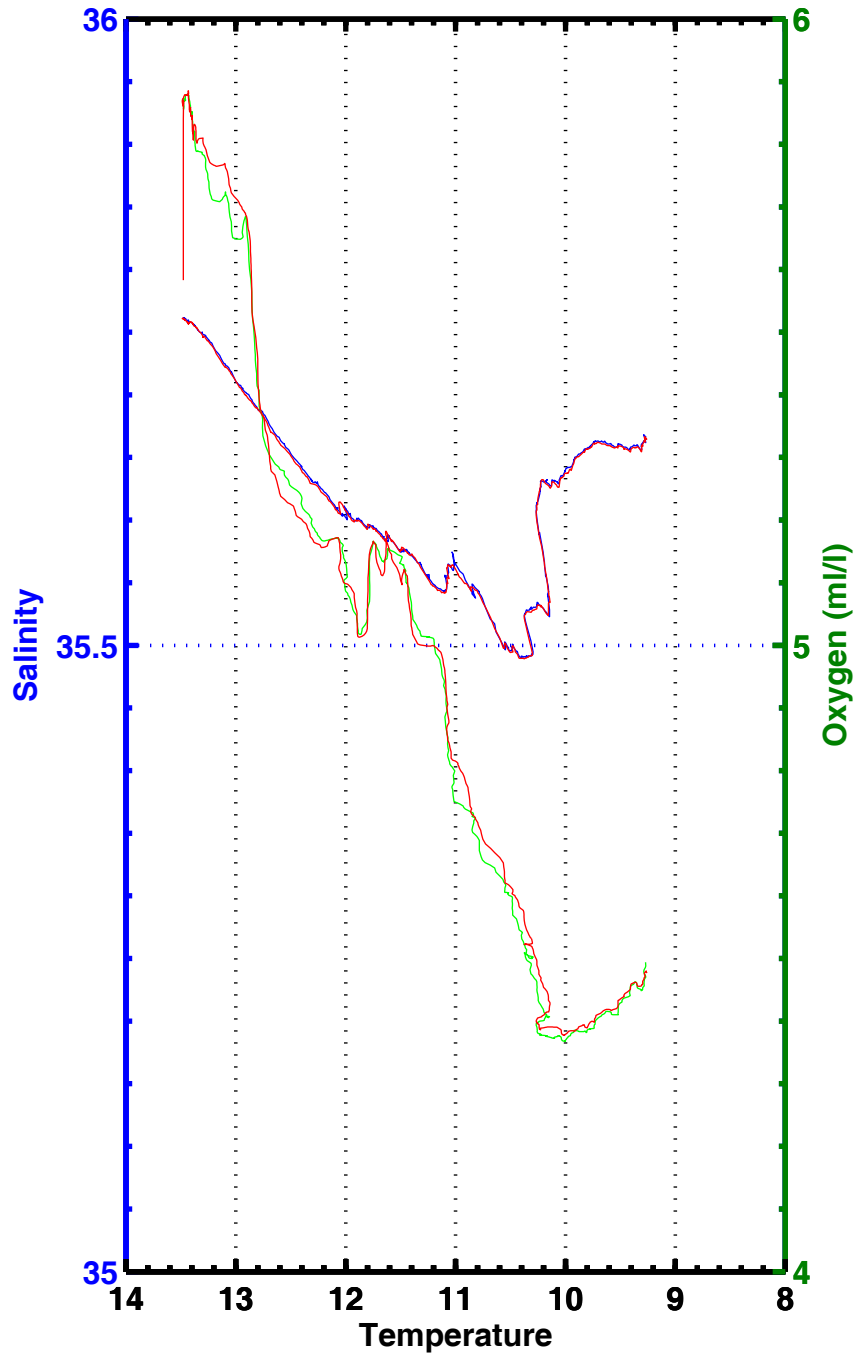
T-S , T-02 , station 1198
