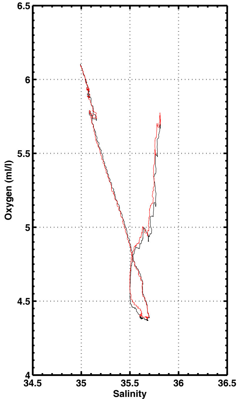
S-02 , station 1006
