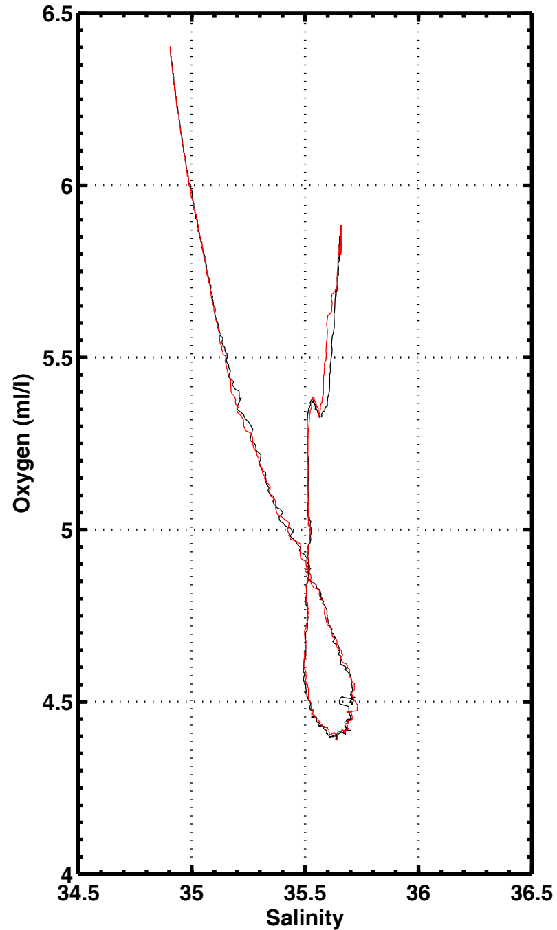
S-O2 , station 1012
