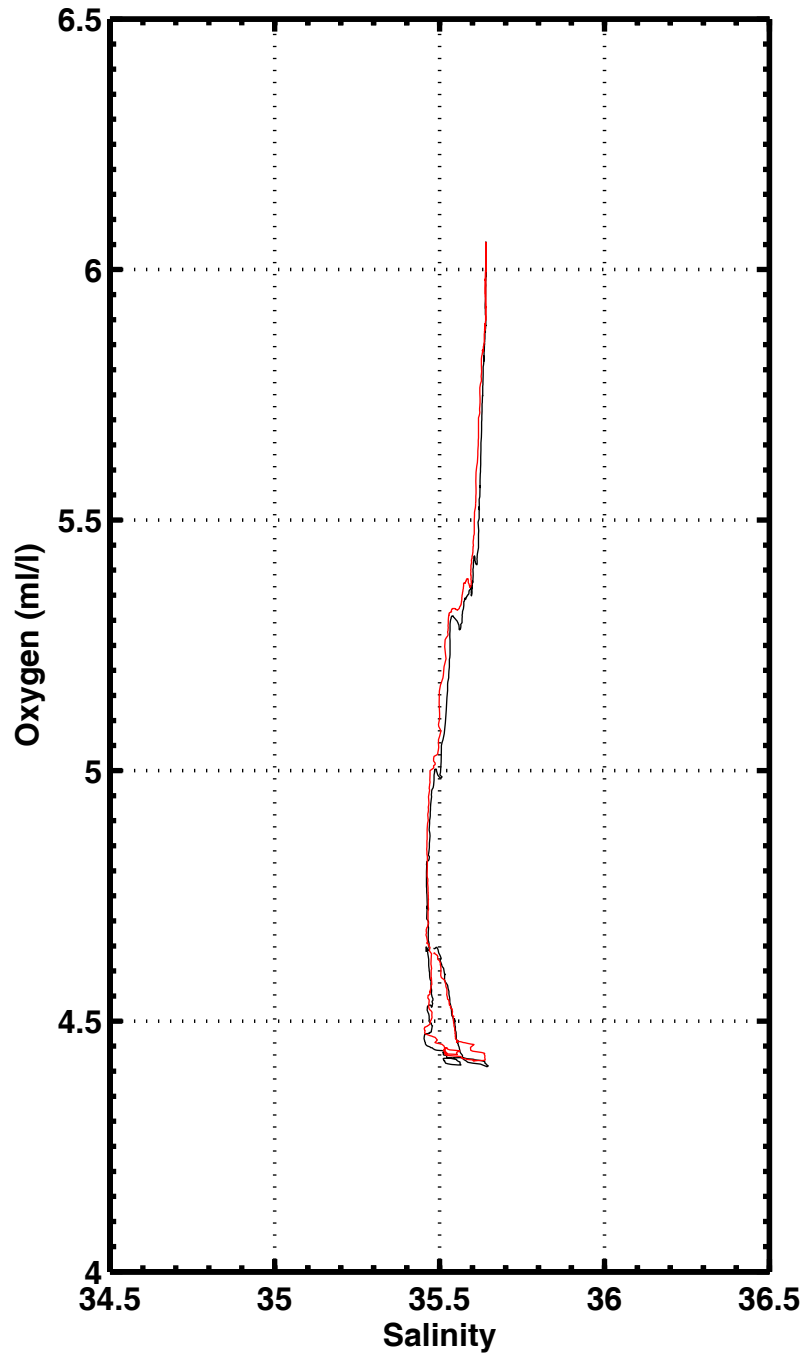
S-O2 , station 1165
