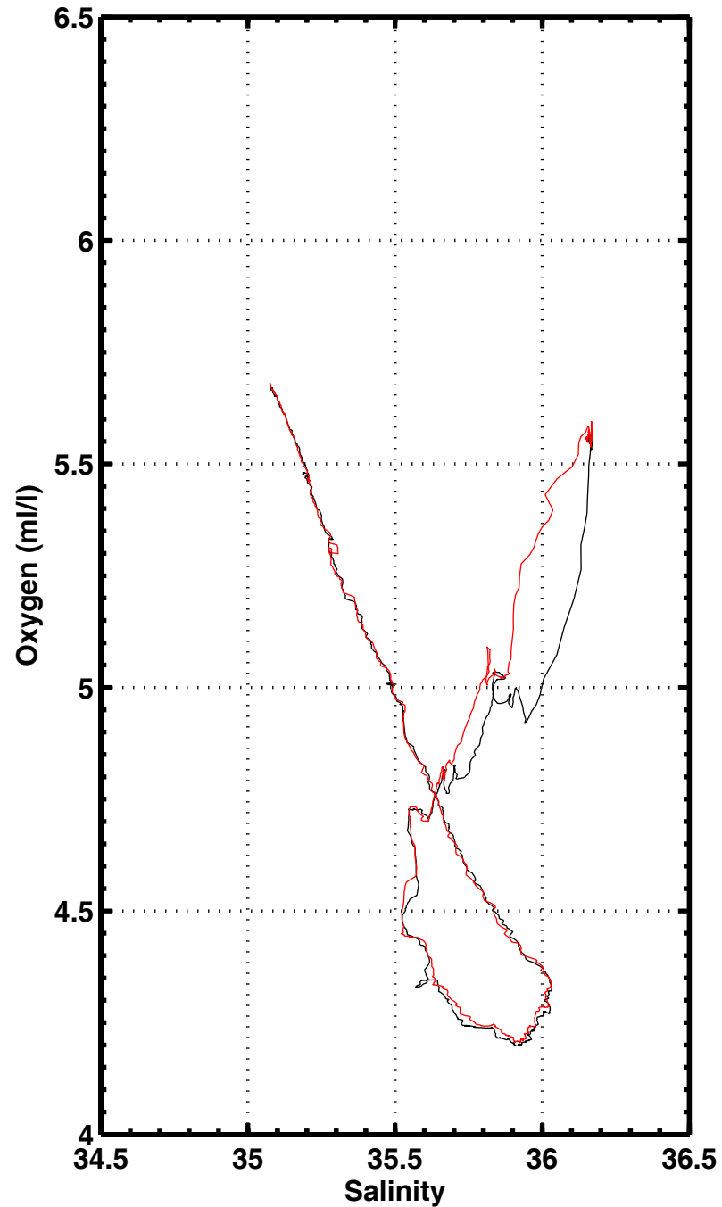
S-O2 , station 1080
