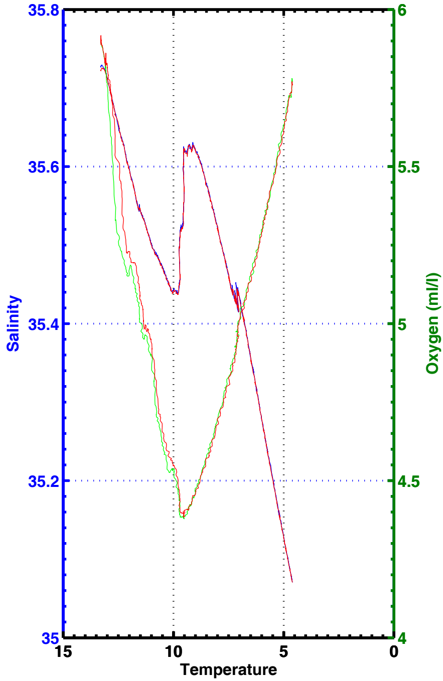
T-S , T-02 , station 1140
