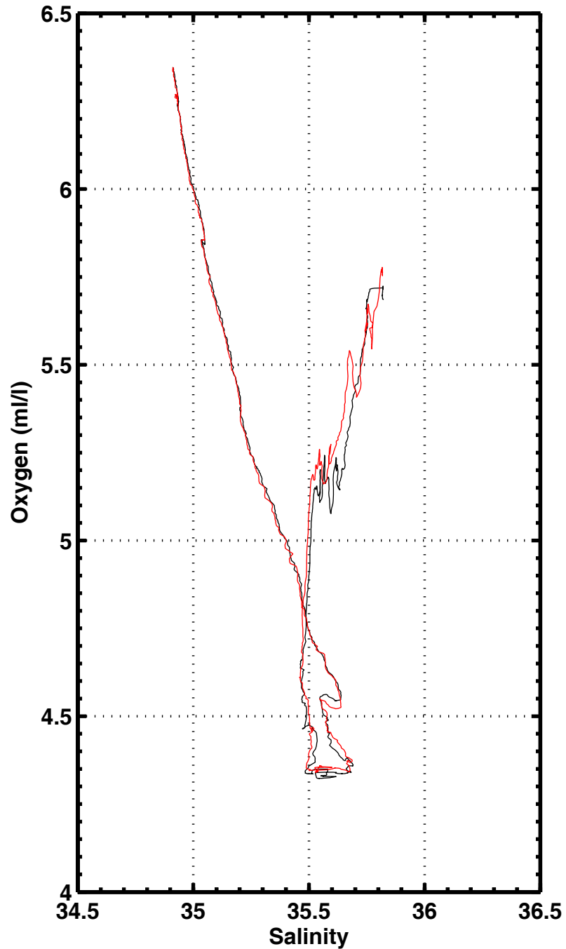
S-O2 , station 1069
