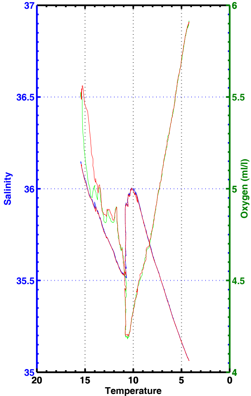
T-S , T-02 , station 1077
