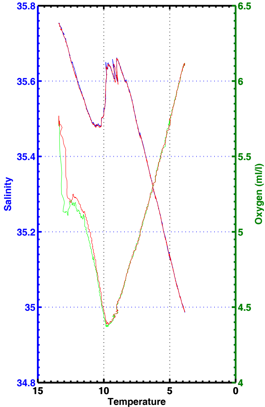
T-S , T-02 , station 1025
