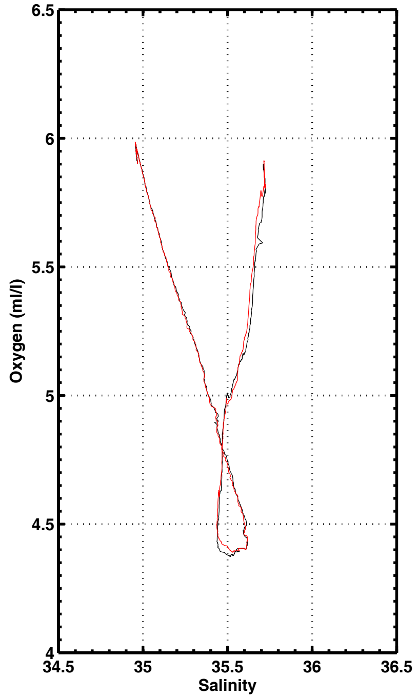
S-O2 , station 1150
