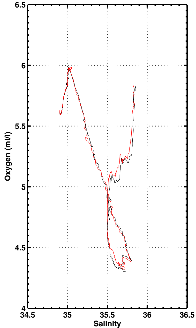
S-O2 , station 1032
