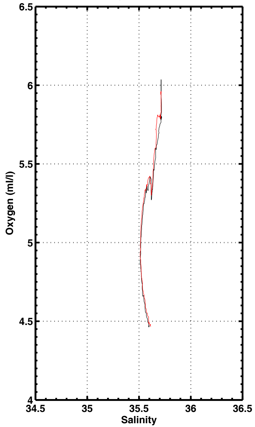
S-O2 , station 1174
