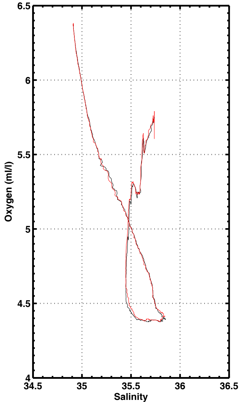
S-O2 , station 1020
