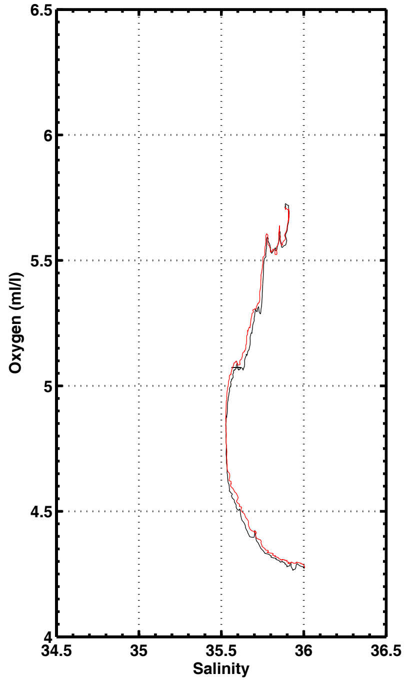
S-O2 , station 1084
