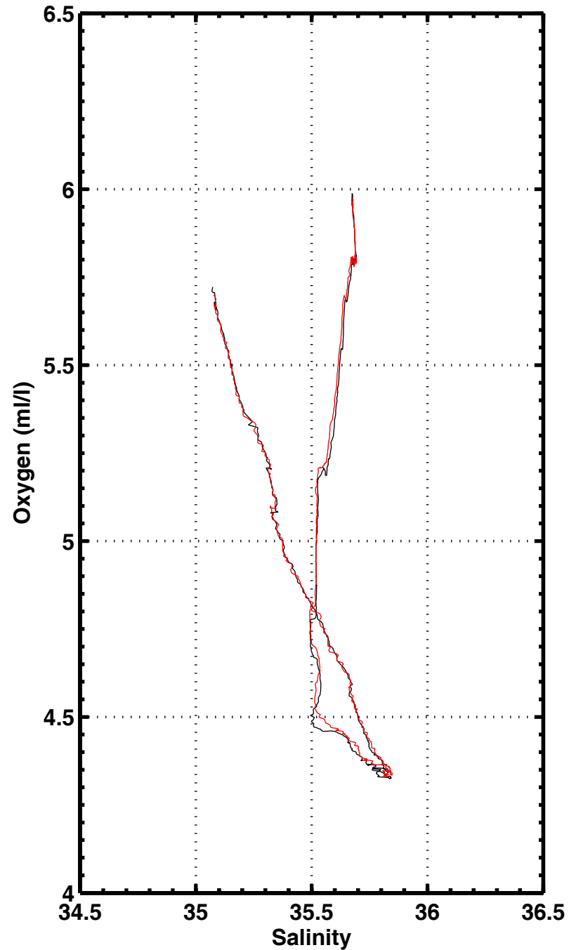
S-O2 , station 1185
