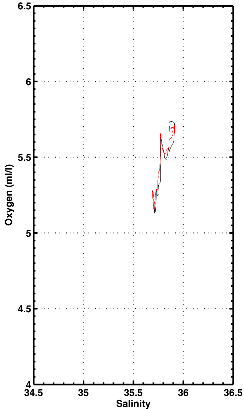
S-O2 , station 1090
