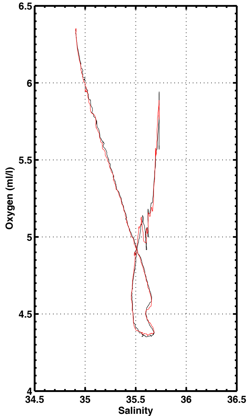
S-O2 , station 1064
