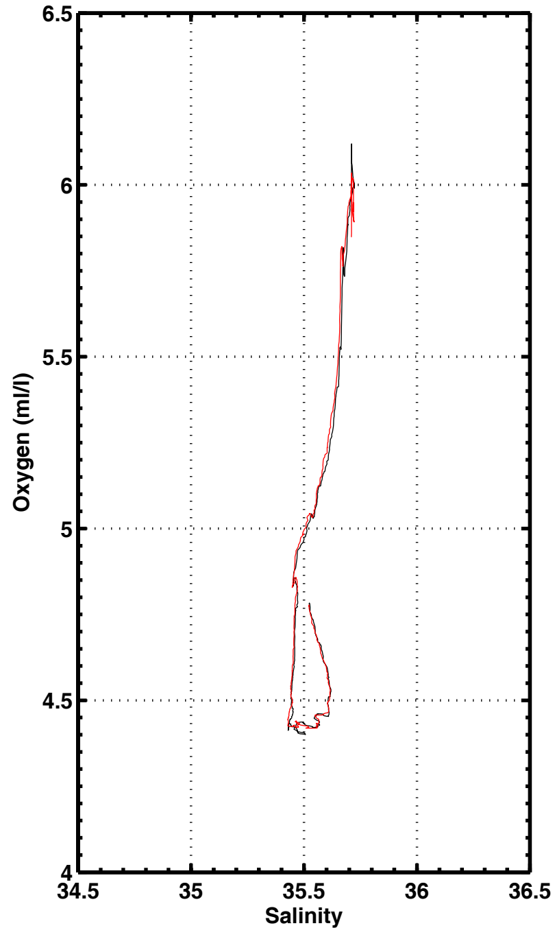
S-O2 , station 1151
