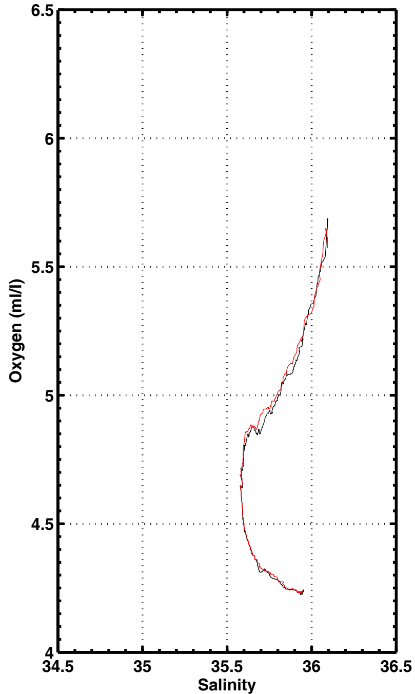
S-O2 , station 1123
