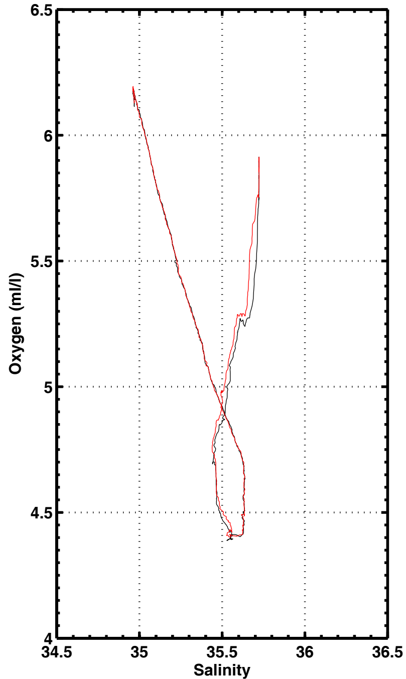
S-O2 , station 1047
