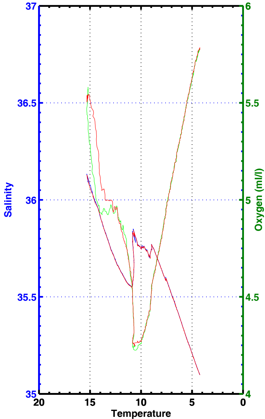
T-S , T-02 , station 1076
