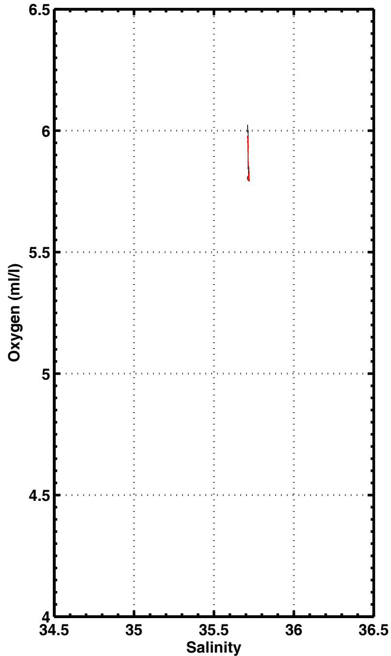
S-02 , station 1171
