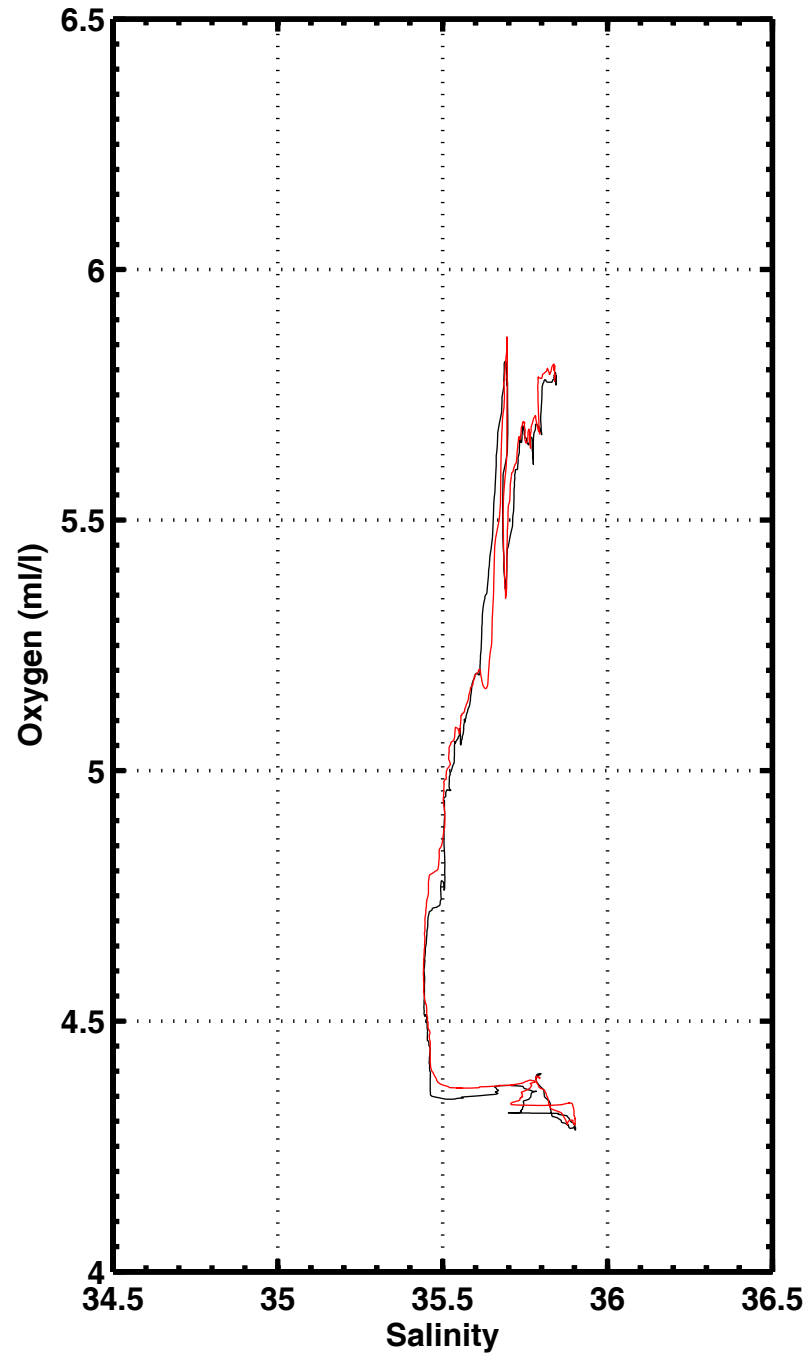
S-O2 , station 1195
