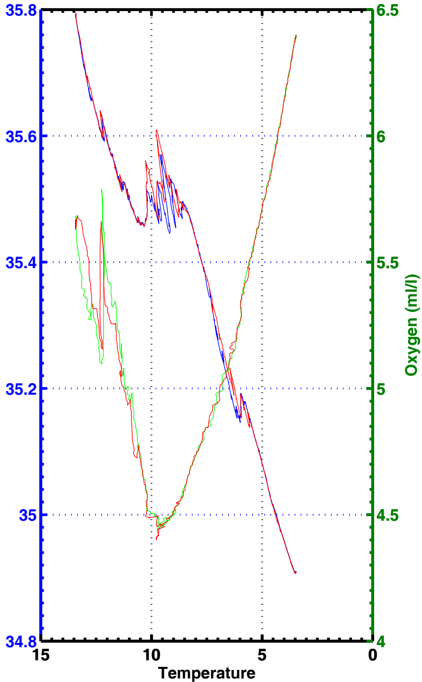
T-S , T-02 , station 1017
