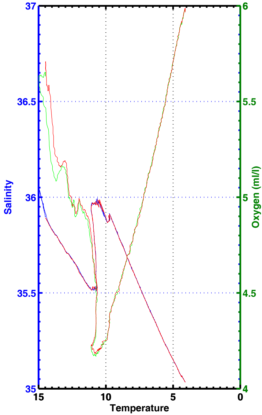
T-S , T-02 , station 1075
