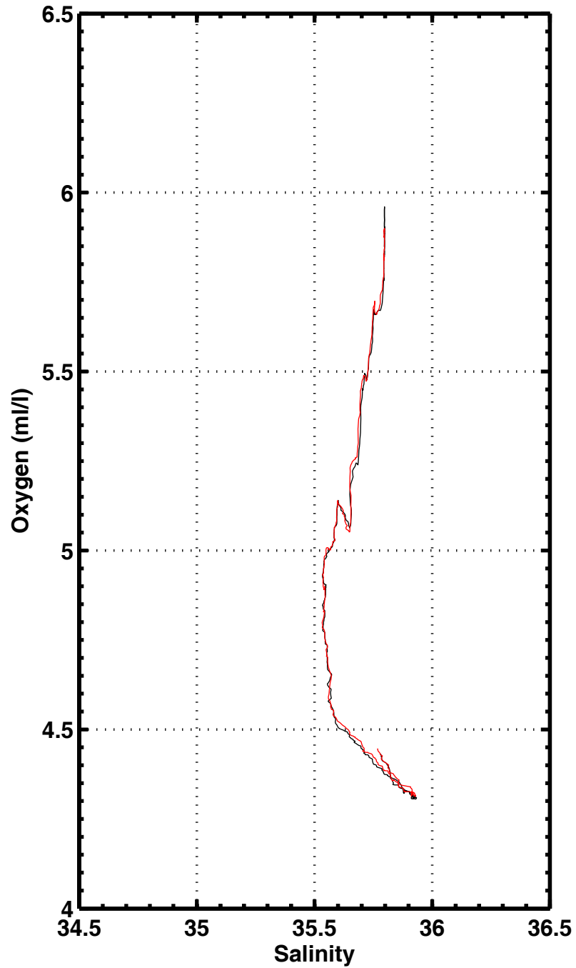
S-02 , station 1201
