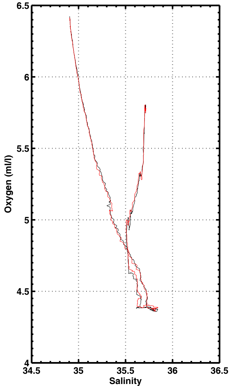
S-O2 , station 1015
