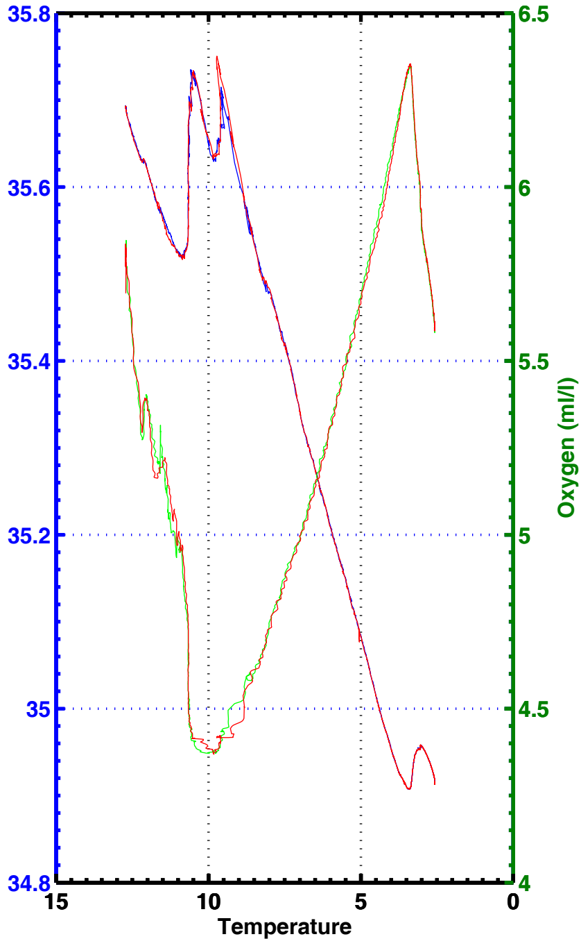
T-S , T-02 , station 1014
