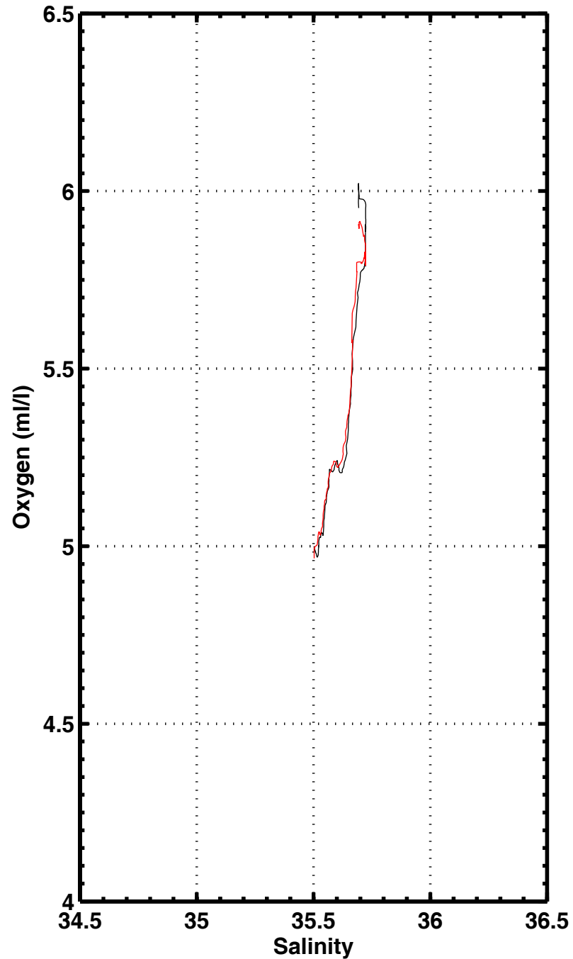
S-O2 , station 1146
