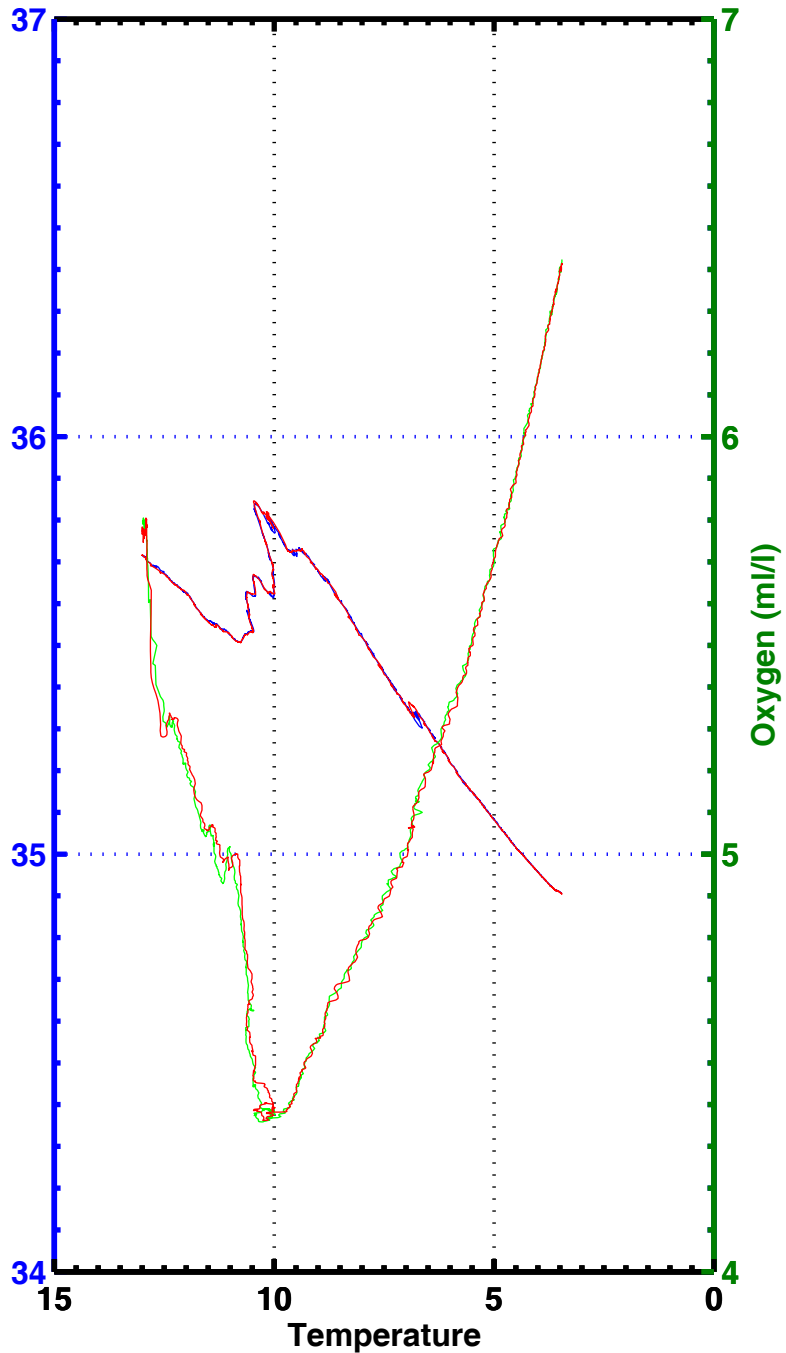
T-S , T-02 , station 1015
