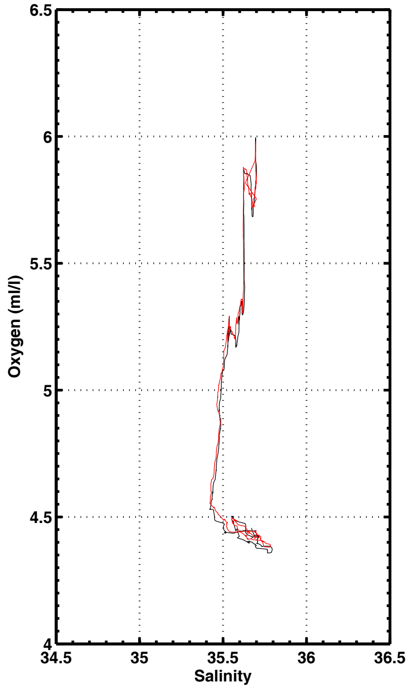
S-O2 , station 1158
