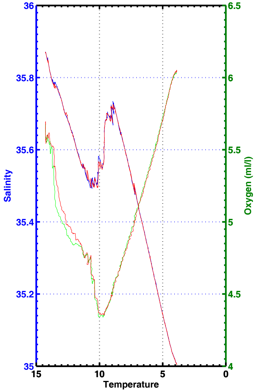
T-S , T-02 , station 1029
