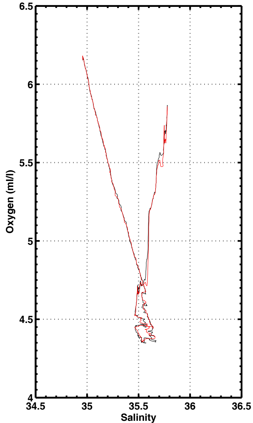
S-O2 , station 1038
