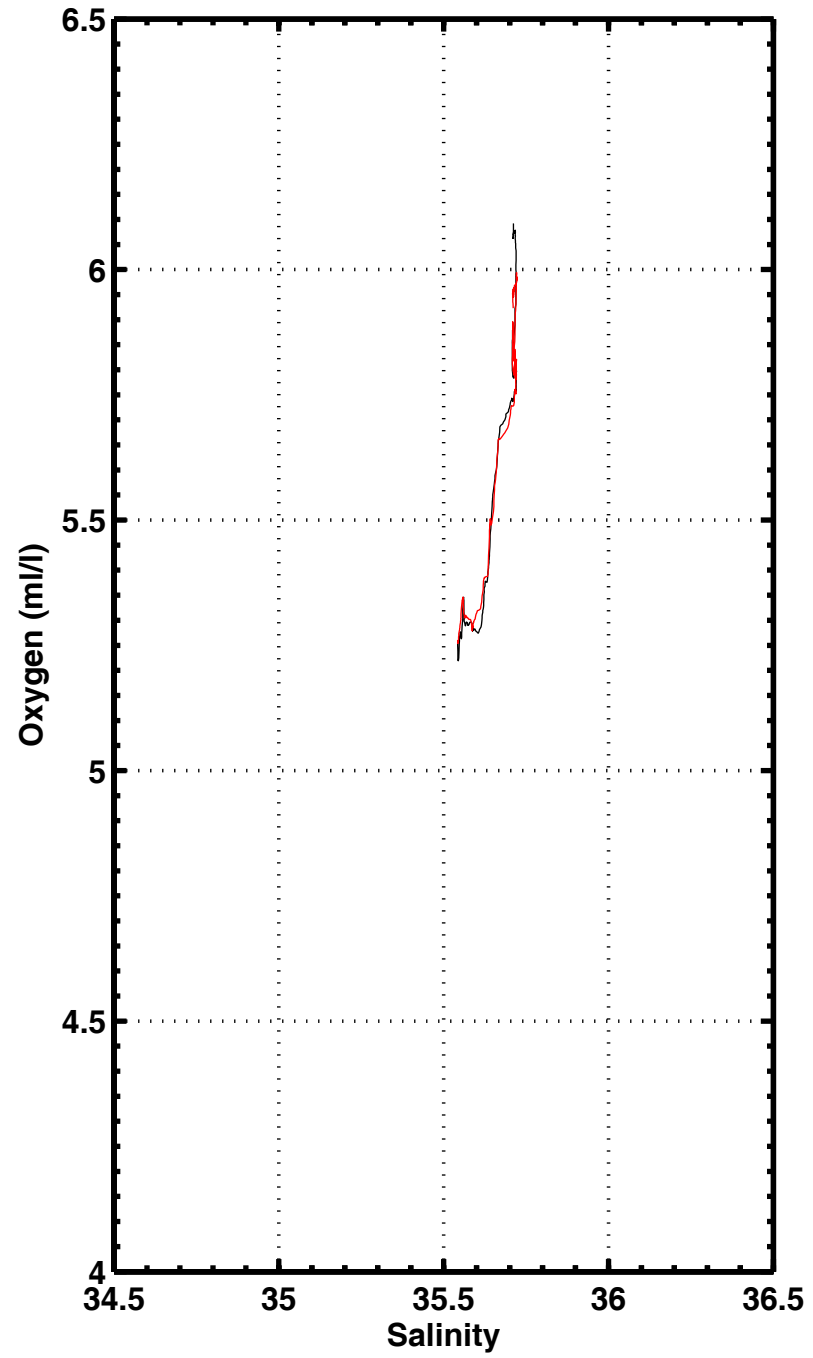
S-O2 , station 1179
