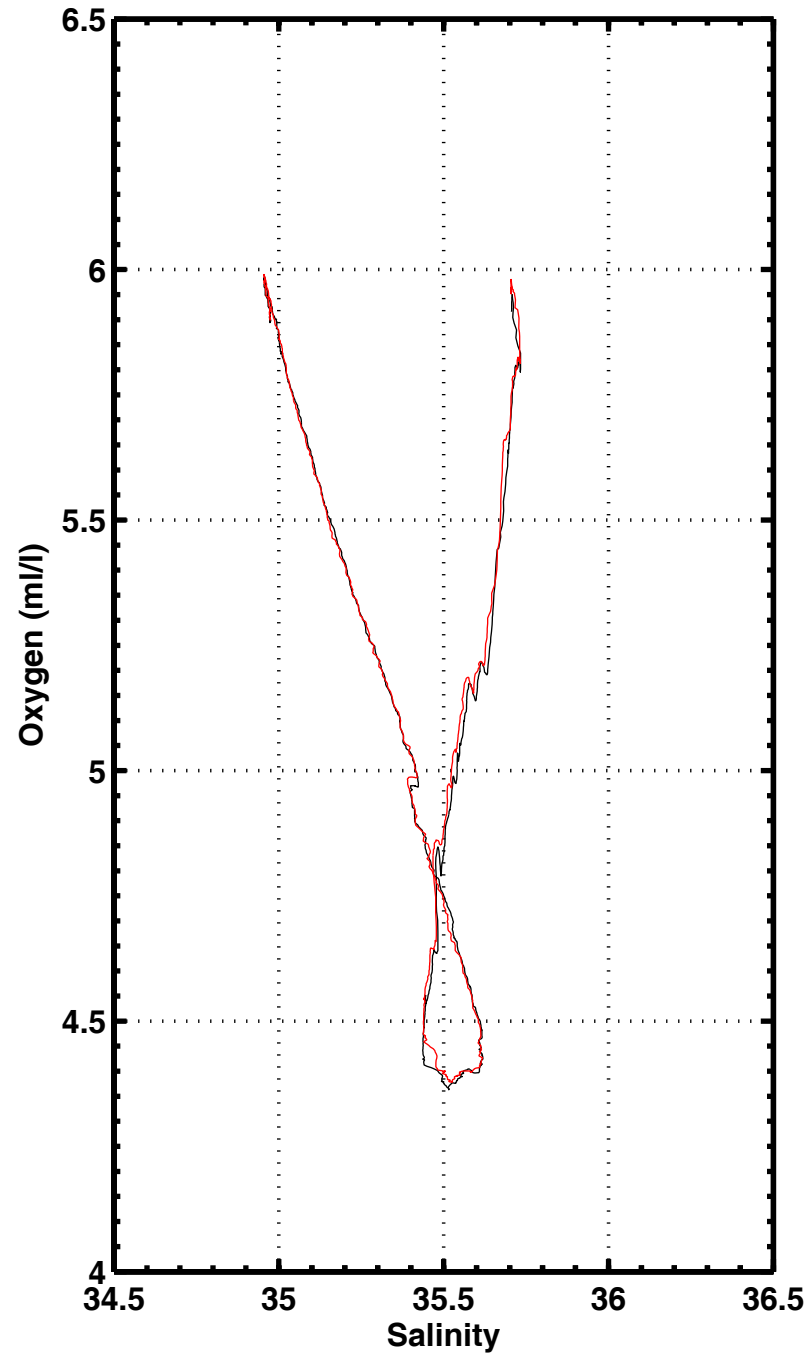
S-O2 , station 1149
