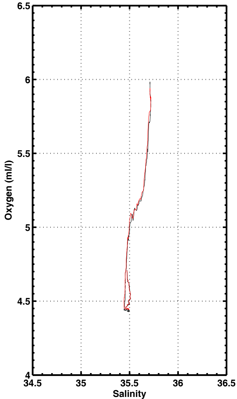
S-O2 , station 1155
