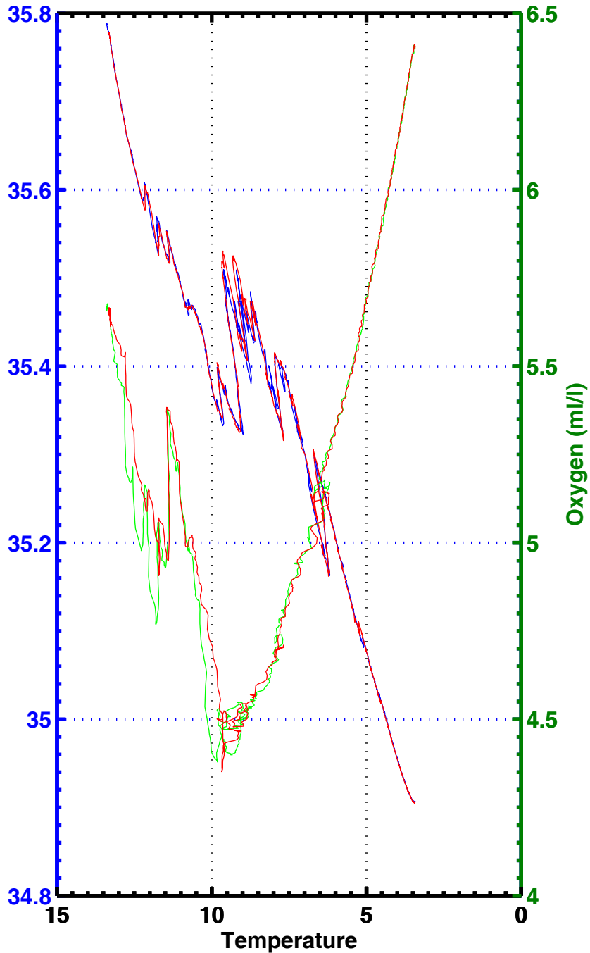
T-S , T-02 , station 1016
