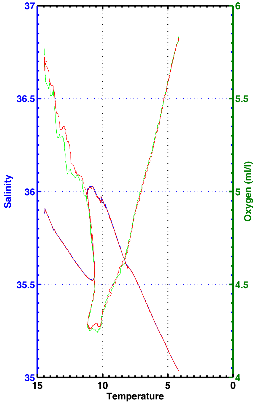
T-S , T-02 , station 1093
