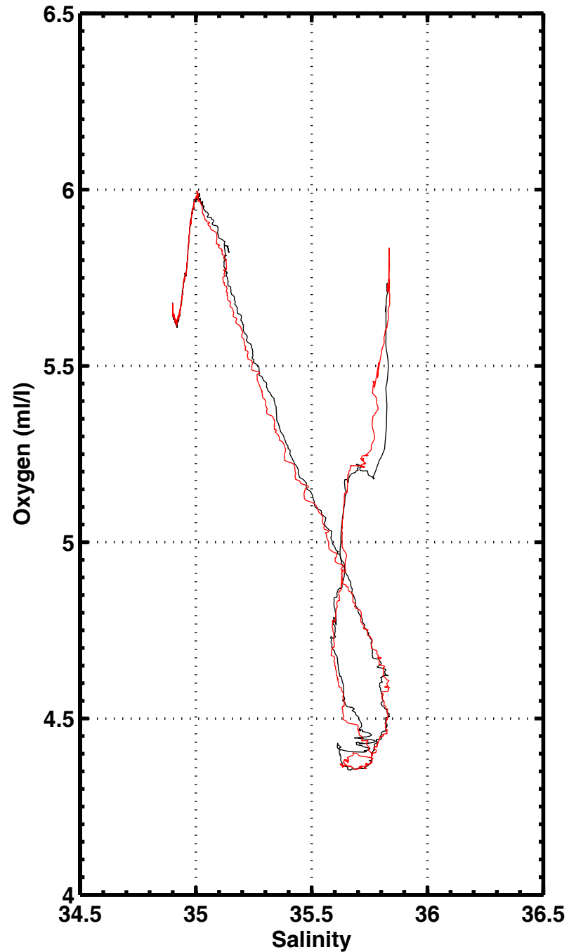
S-O2 , station 1003
