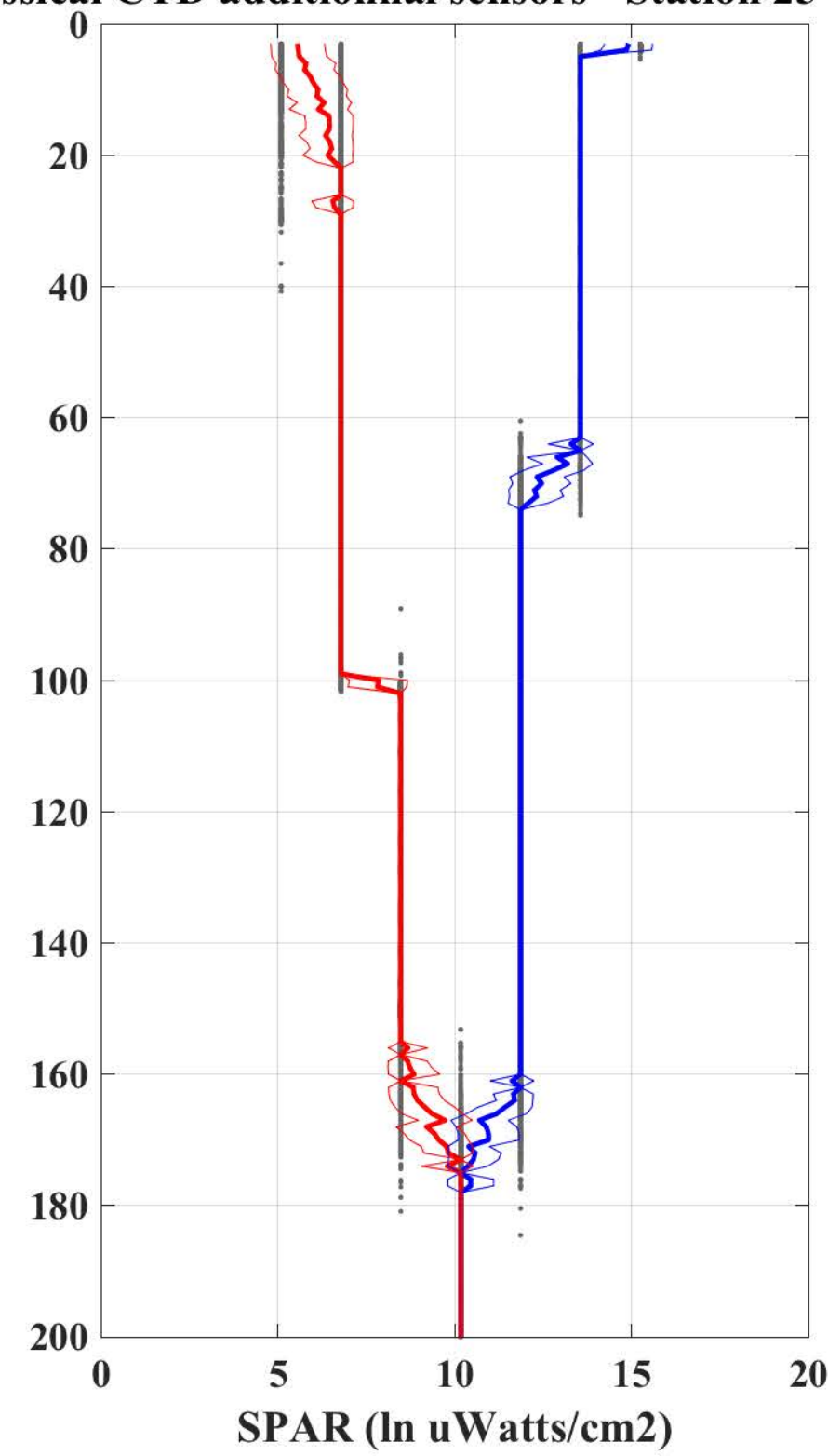
Classical CTD additional sensors - Station 25 - Cast 3
