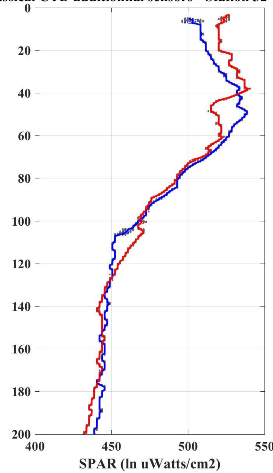
Classical CTD additional sensors - Station 32 - Cast 9
