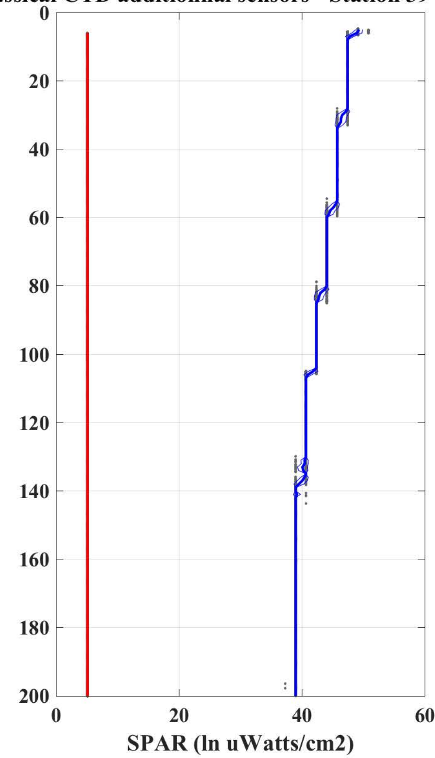
Classical CTD additional sensors - Station 39 - Cast 1
