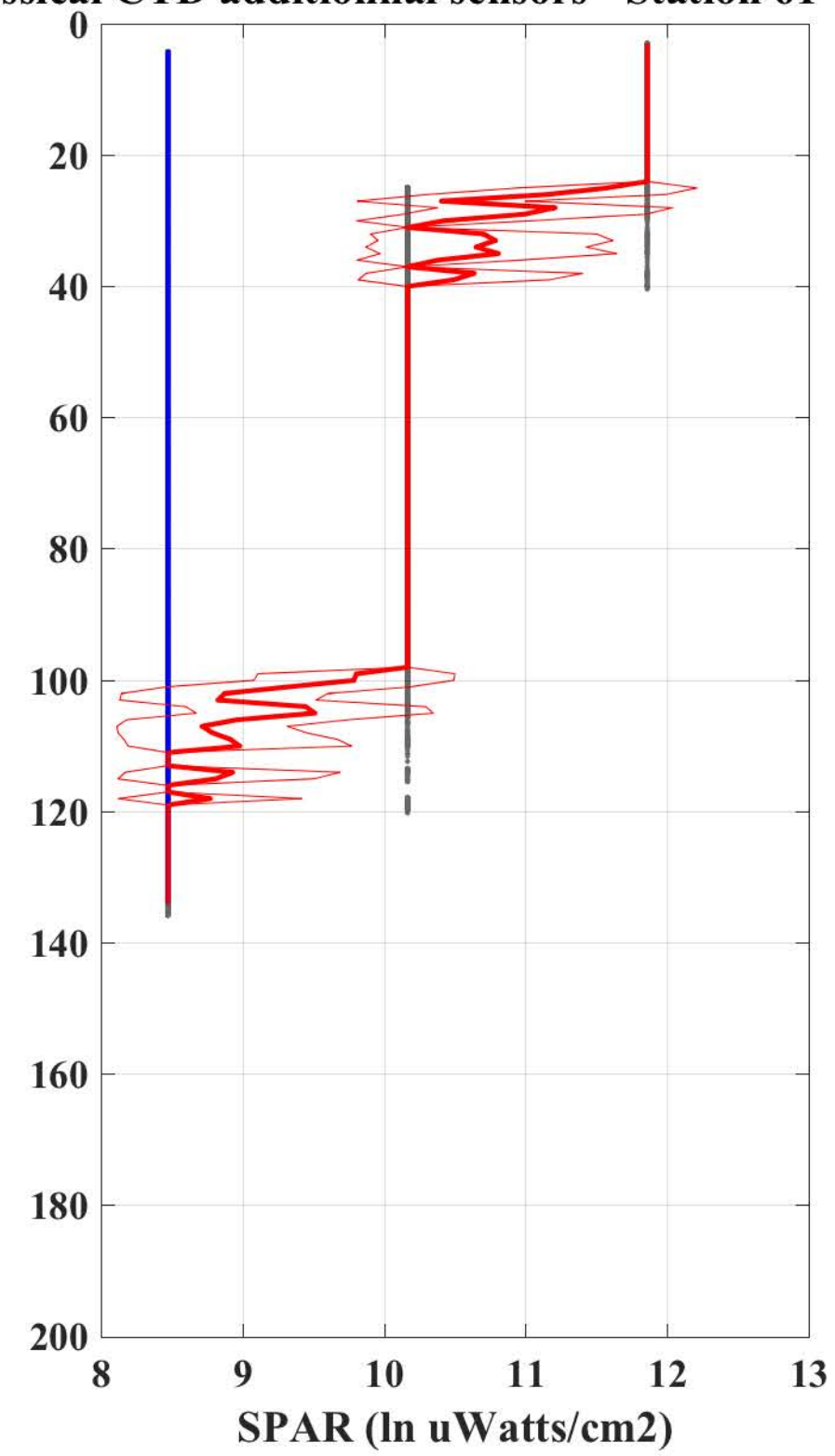
Classical CTD additional sensors - Station 61 - Cast 5
