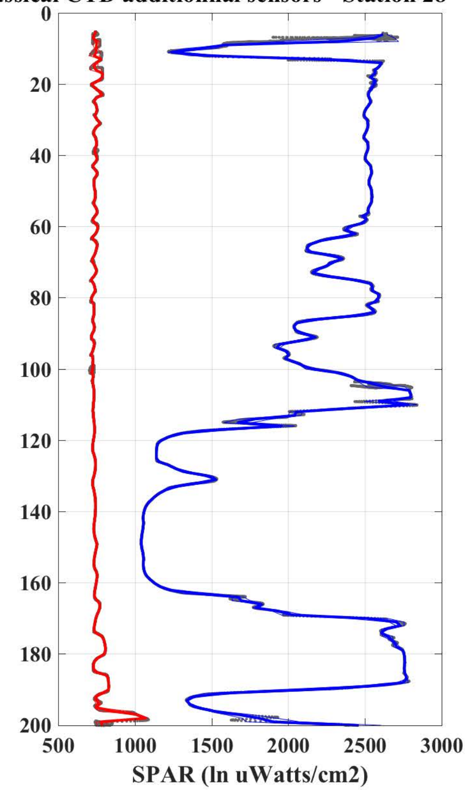
Classical CTD additionnal sensors - Station 28 - Cast 1
