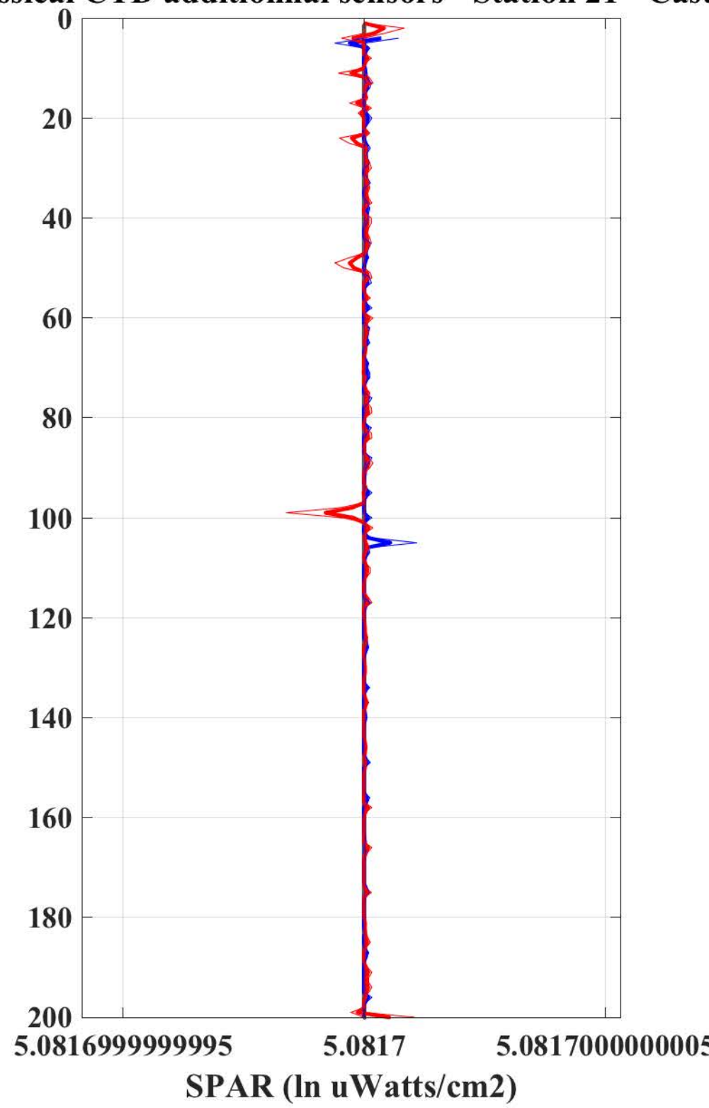
Classical CTD additional sensors - Station 21 - Cast 14
