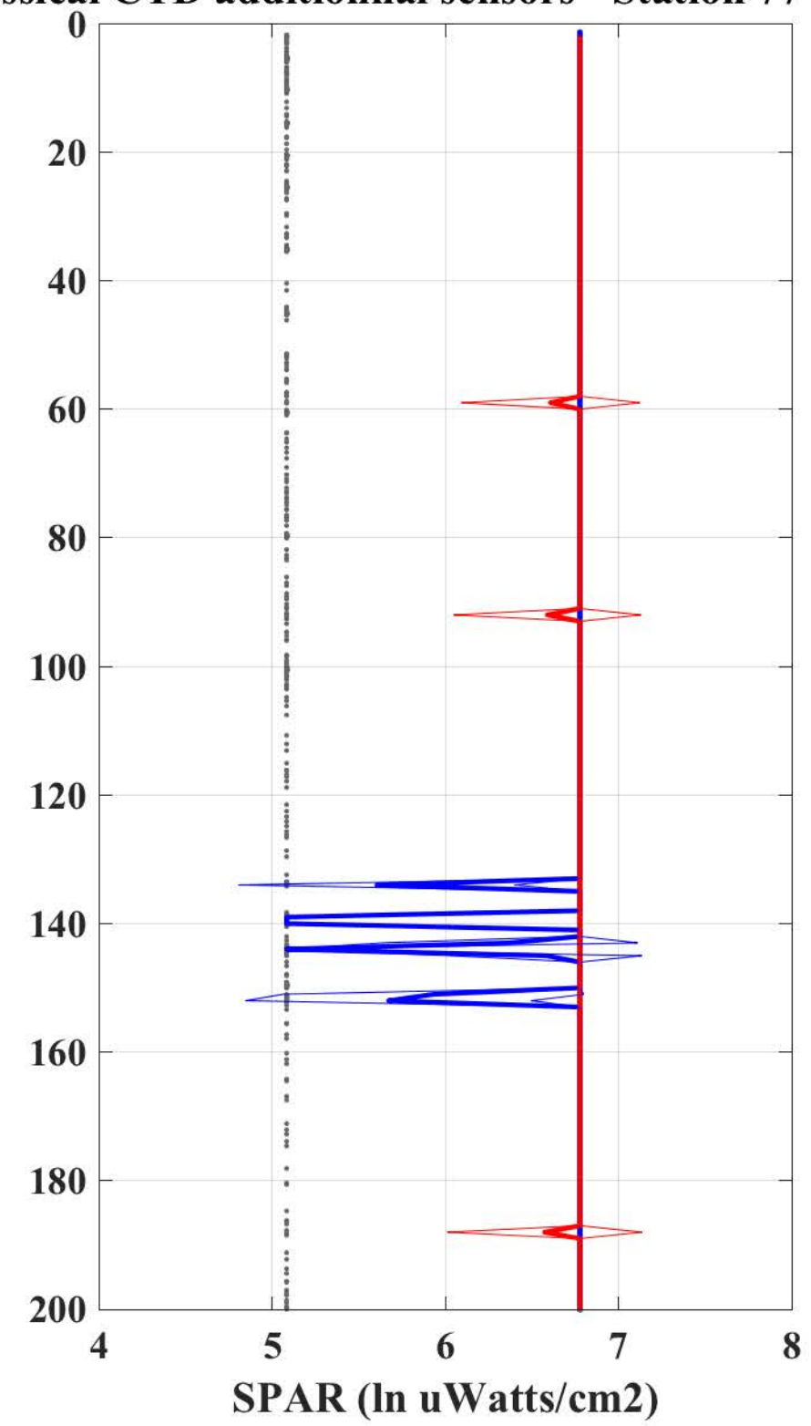
Classical CTD additional sensors - Station 77 - Cast 3
