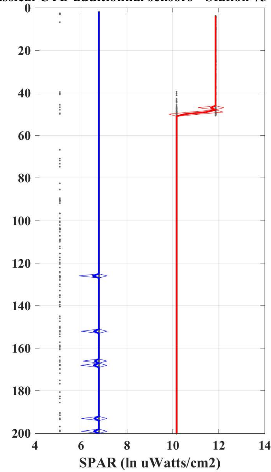
Classical CTD additional sensors - Station 73 - Cast 1
