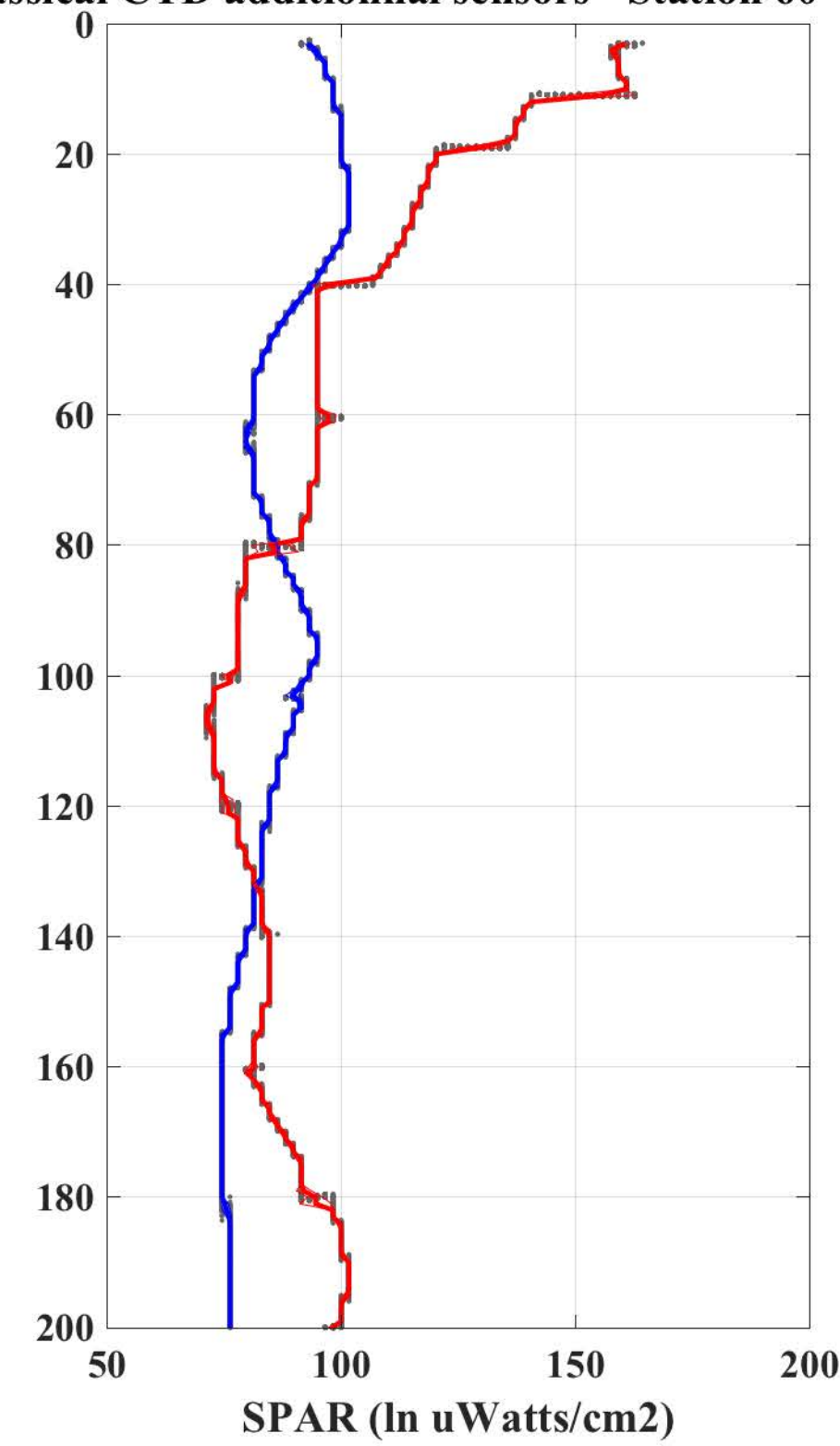
Classical CTD additional sensors - Station 60 - Cast 7
