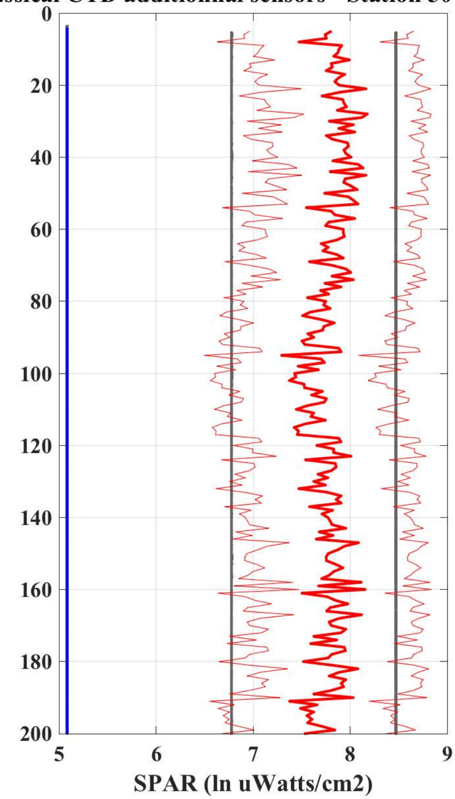
Classical CTD additional sensors - Station 50 - Cast 1
