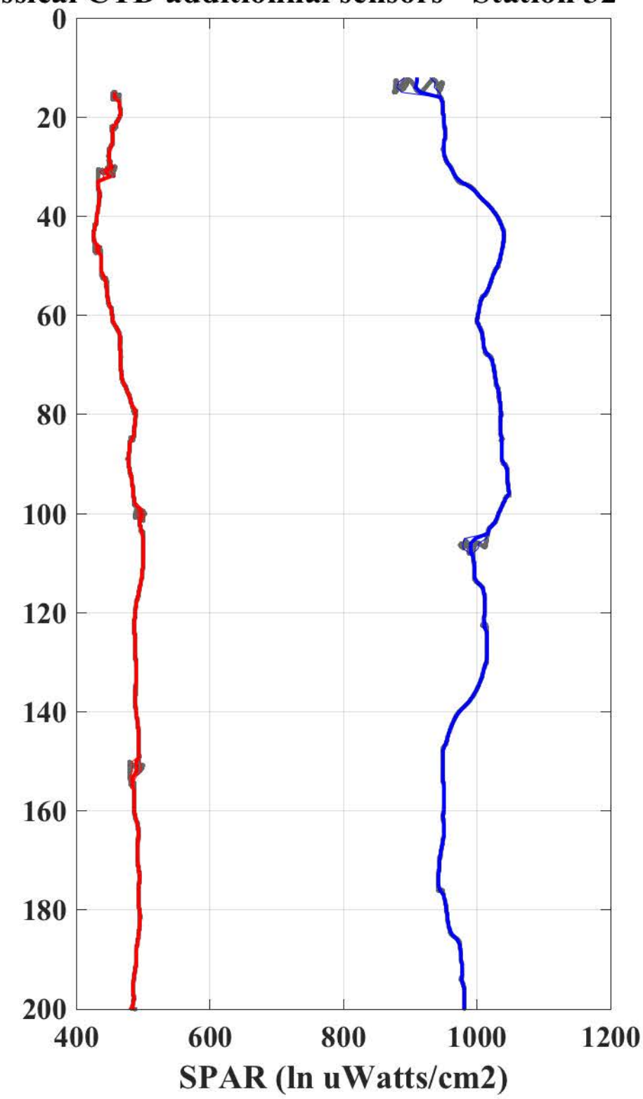
Classical CTD additional sensors - Station 32 - Cast 1
