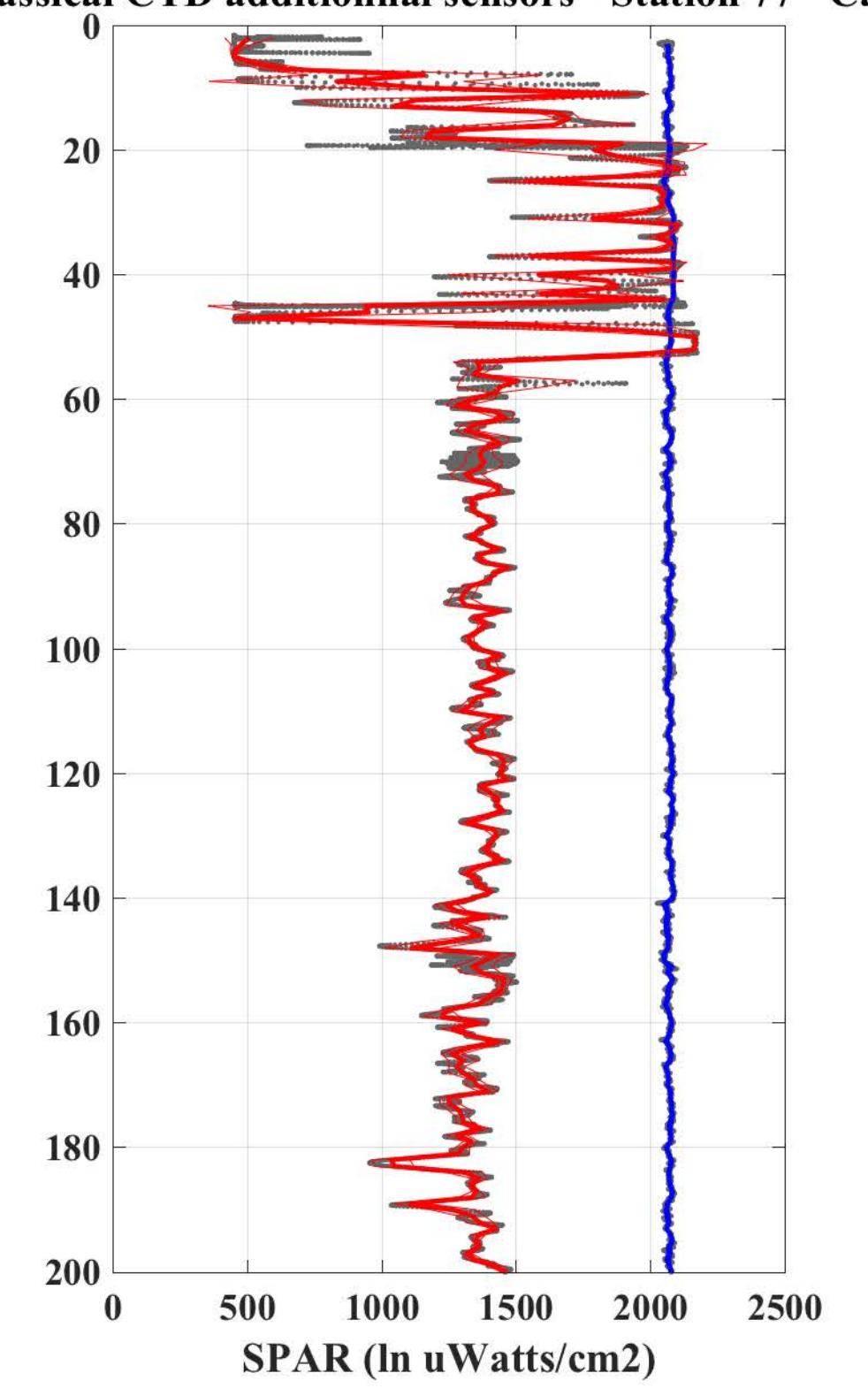
Classical CTD additional sensors - Station 77 - Cast 7
