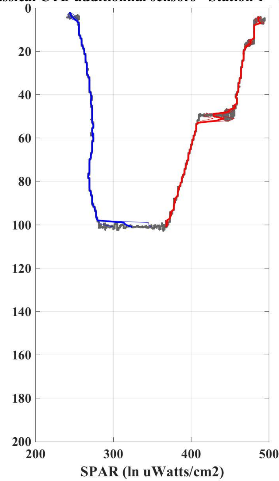
Classical CTD additional sensors - Station 1 - Cast 11
