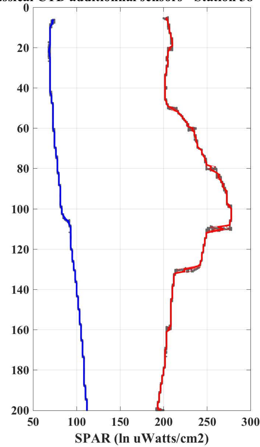
Classical CTD additionnal sensors - Station 38 - Cast 5
