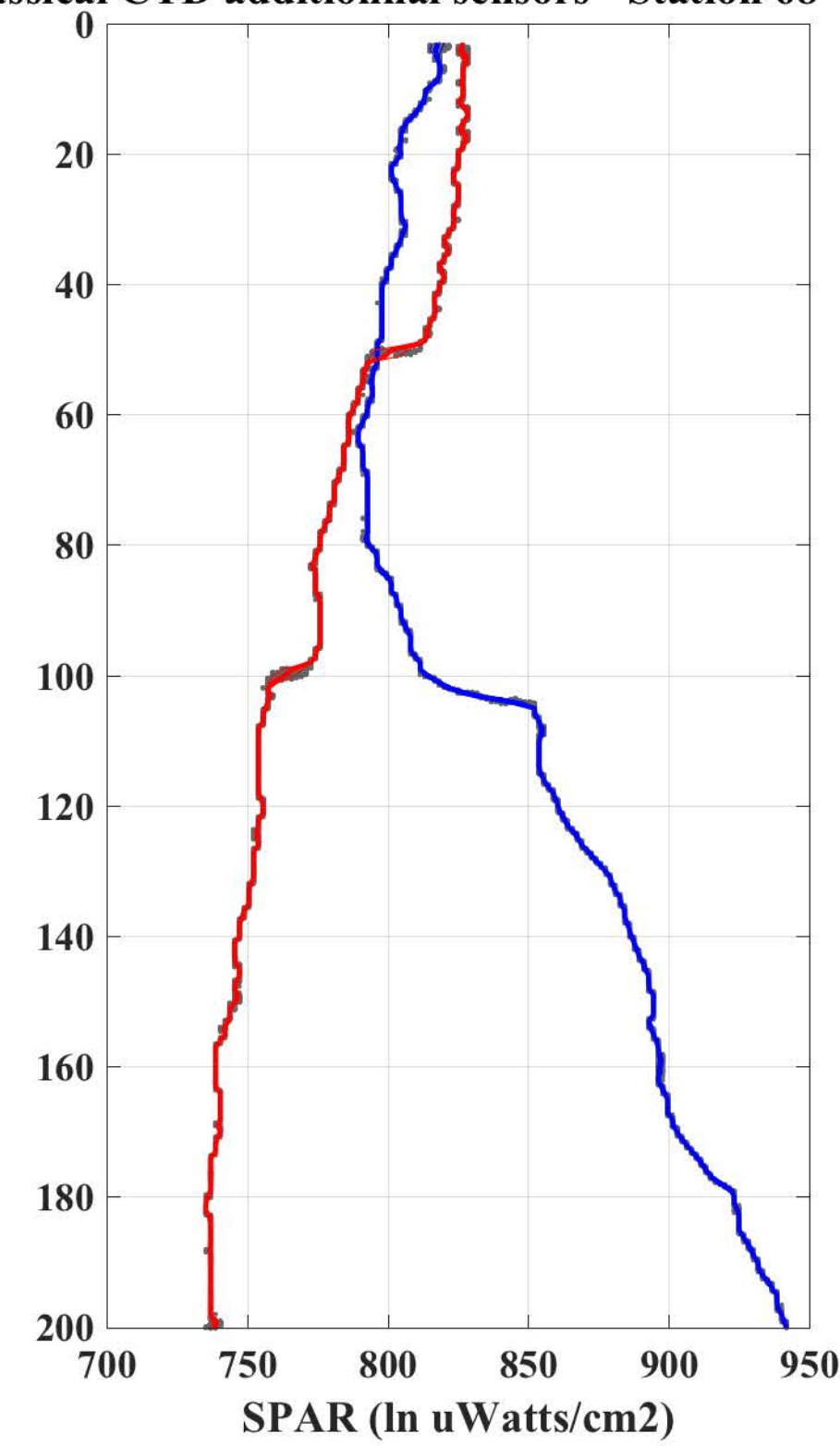
Classical CTD additional sensors - Station 68 - Cast 1
