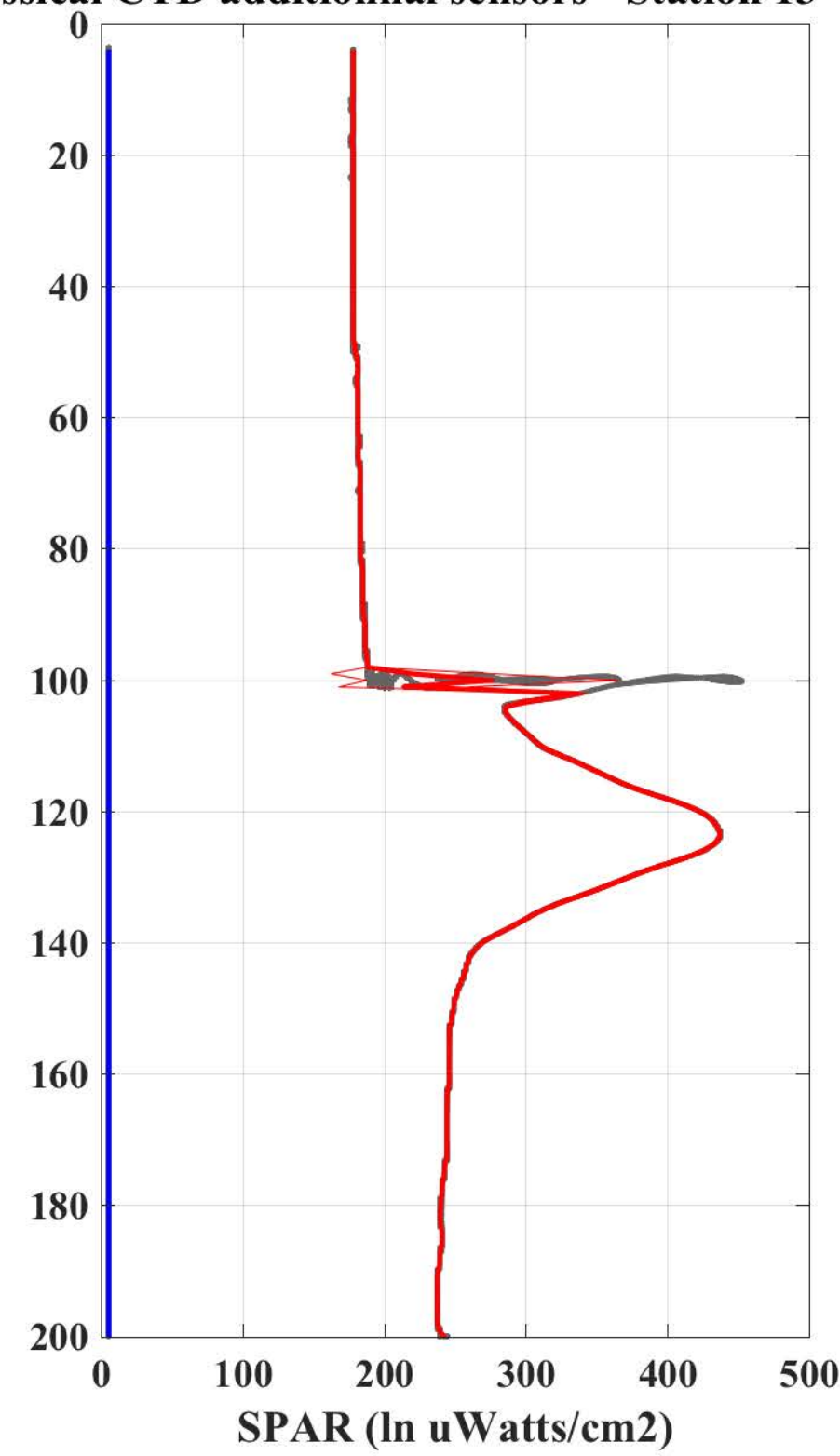
Classical CTD additional sensors - Station 13 - Cast 1
