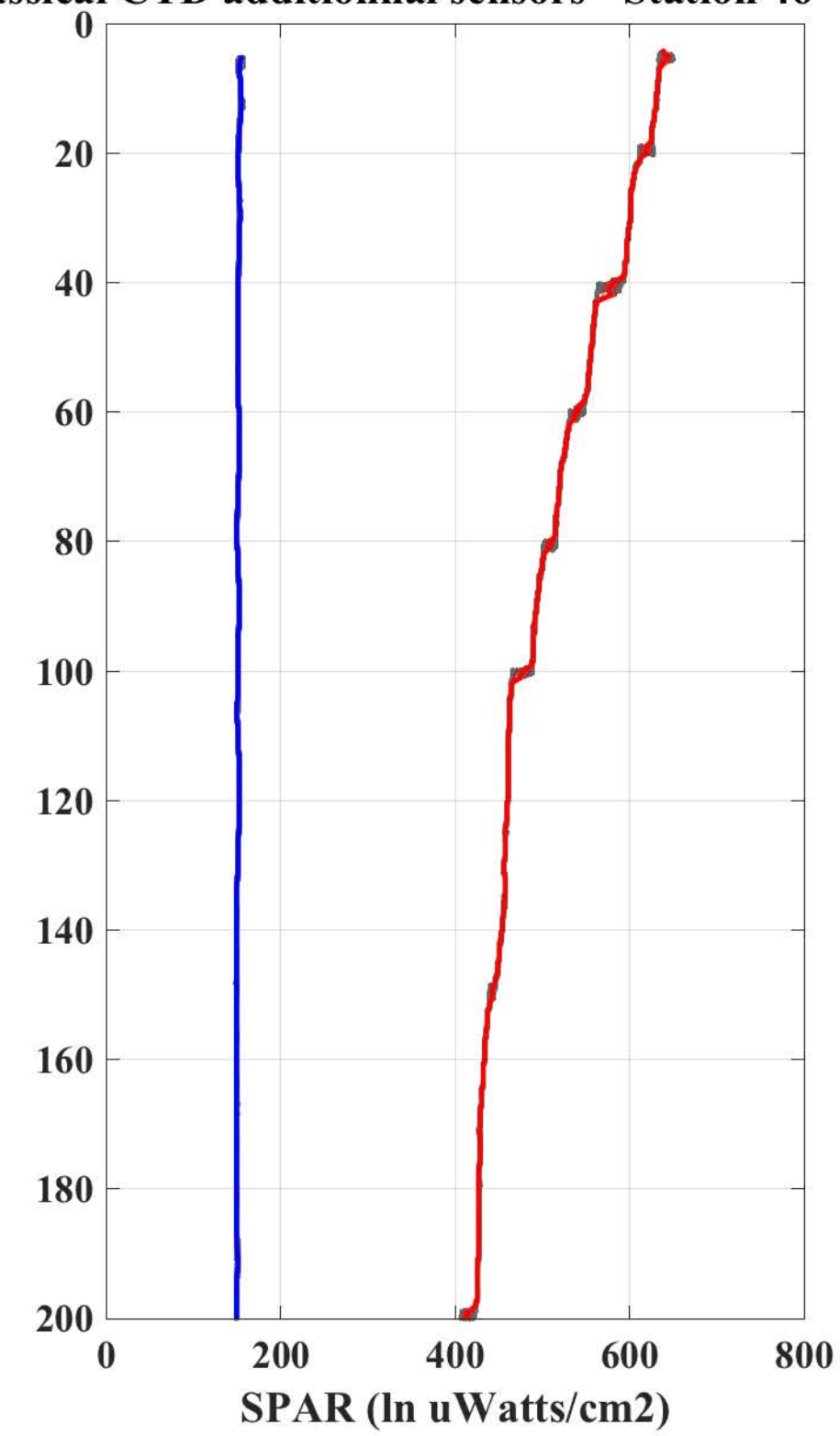
Classical CTD additional sensors - Station 46 - Cast 1
