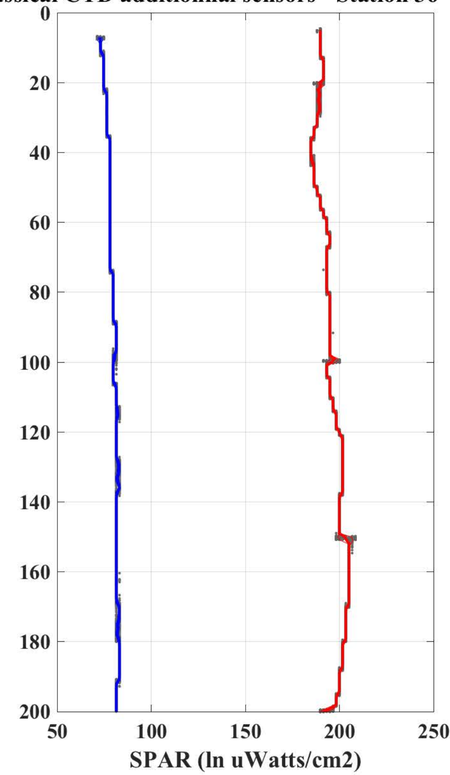
Classical CTD additional sensors - Station 36 - Cast 1
