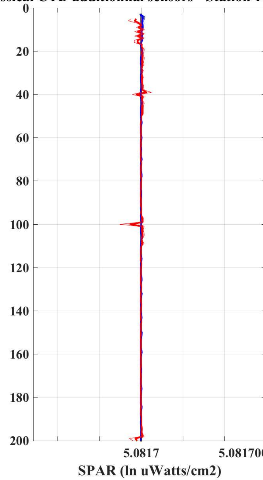
Classical CTD additional sensors - Station 14 - Cast 1
