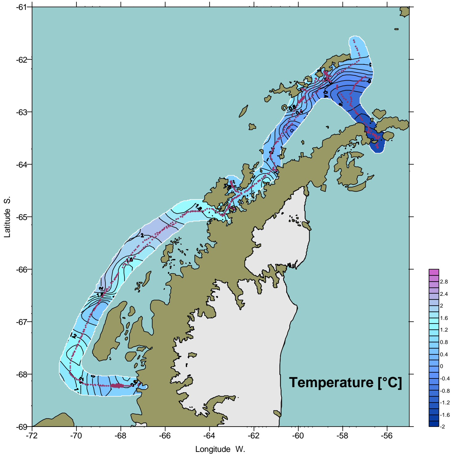
Sea-surface temperature distribution (March 2001)
