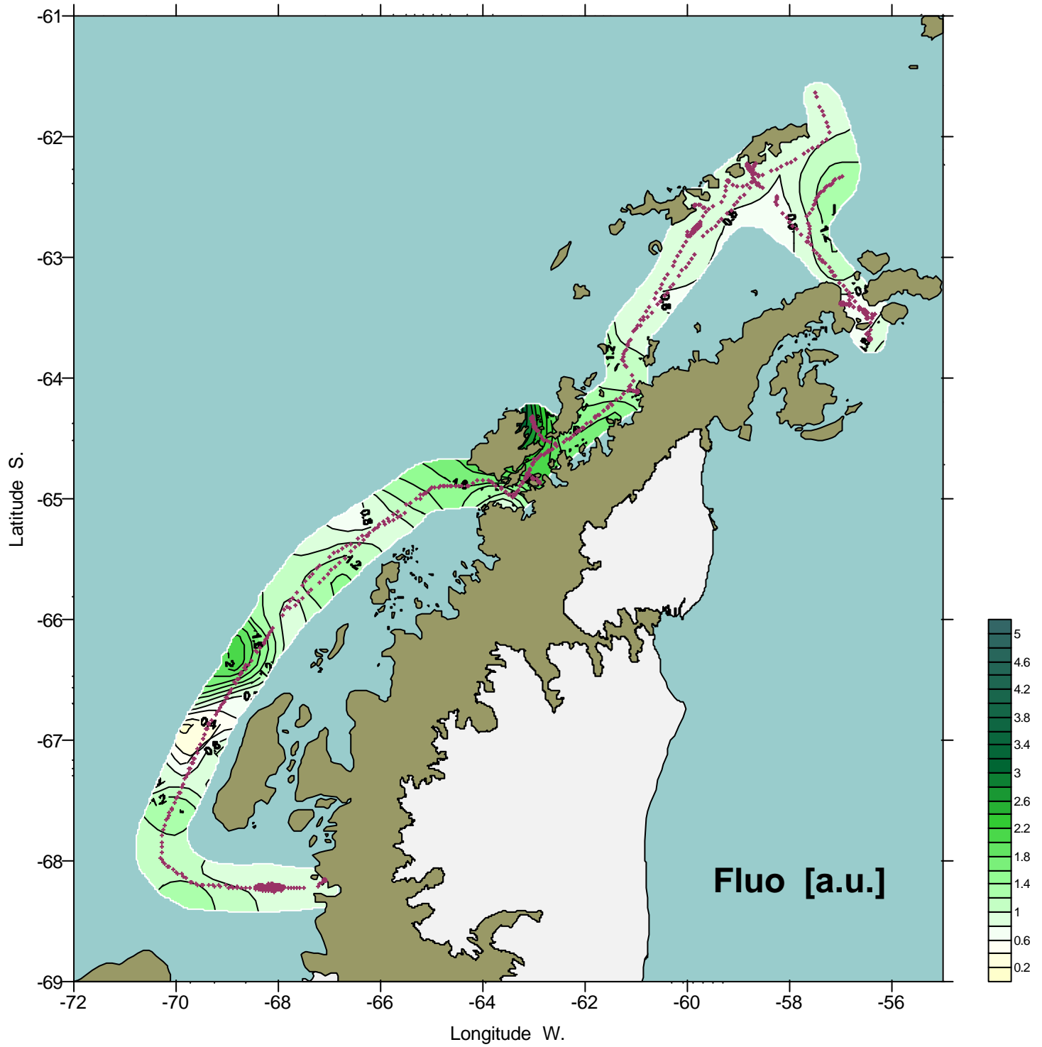
Sea-surface fluorescence distribution (March 2001)
