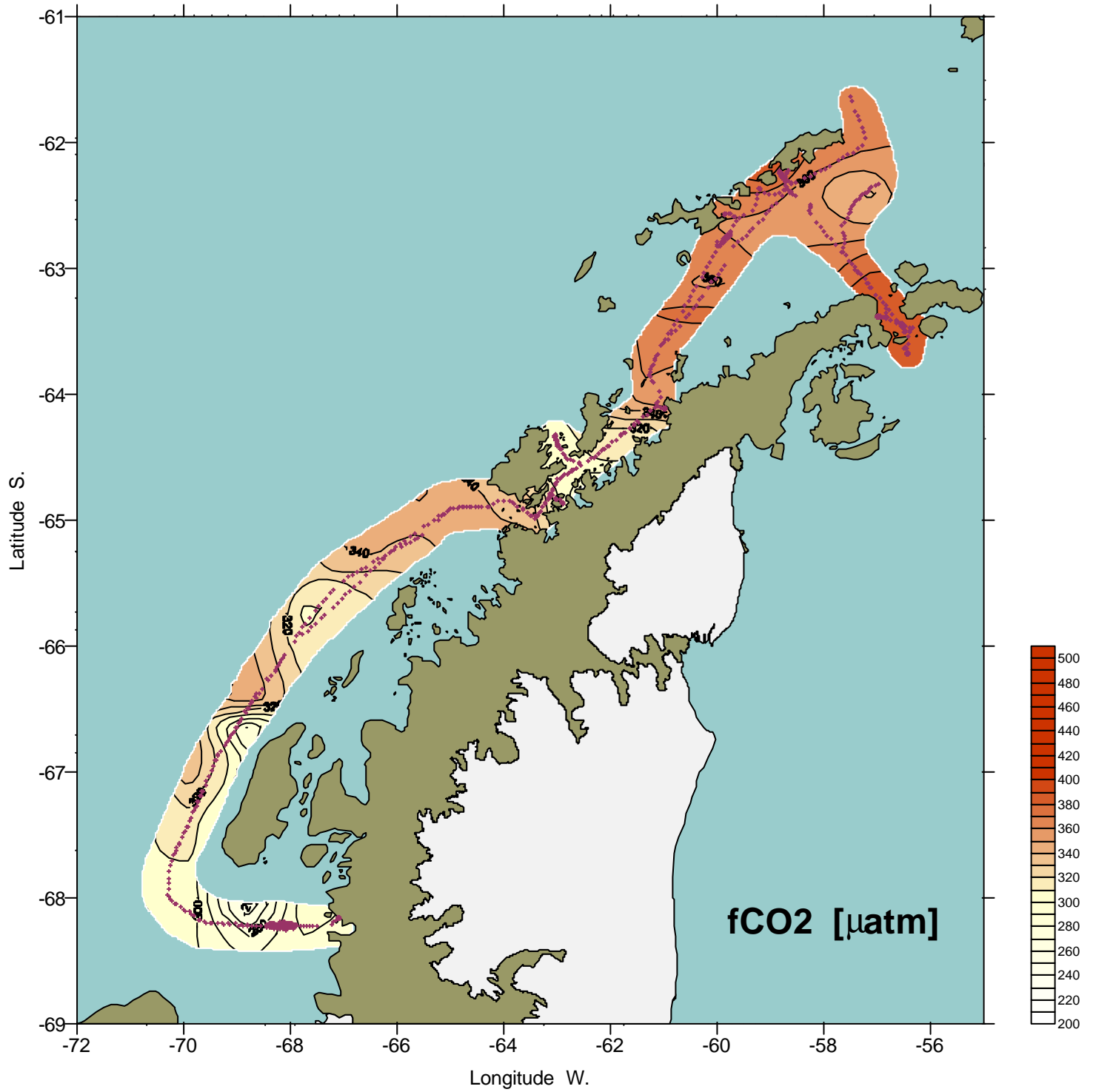
Sea-surface distribution of CO 2 in water at 1013 mb (March 2001)
