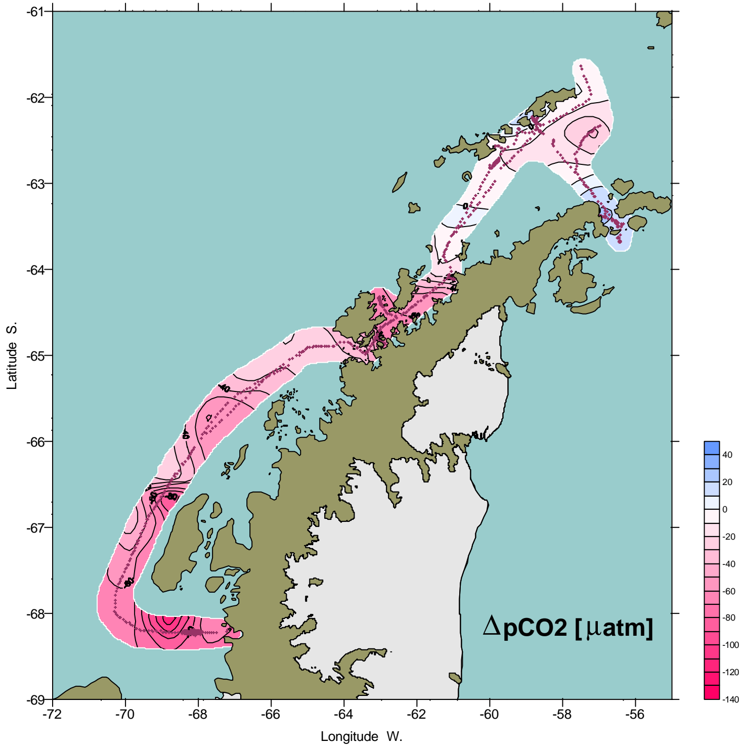
Distribution of \Delta p\text{CO}_2 between sea-surface and air (March 2001)
