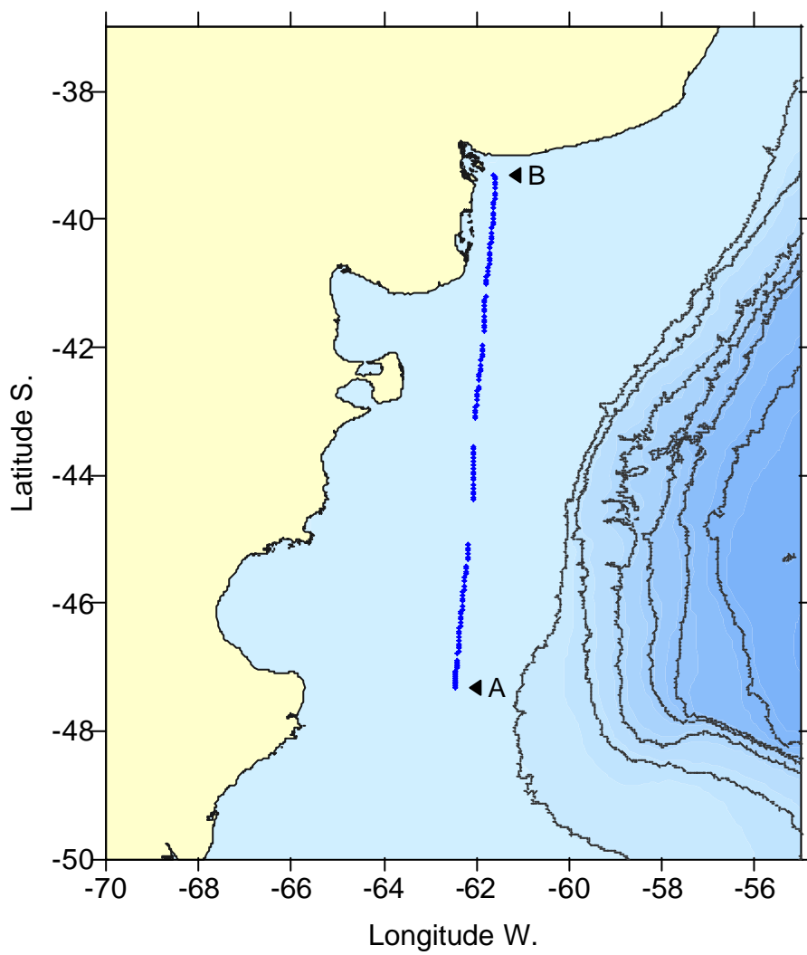
Cruise "Argau-0", Transect 0 (24 to 25 March 2000)
