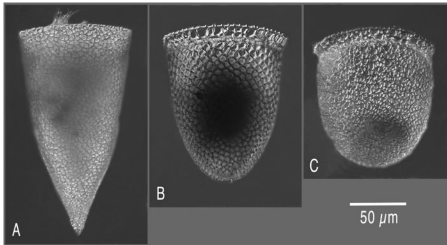
Figure 9. Cyttarocypris is both rare and variable in morphology. A sample from the west coast of Africa taken during the Tara Oceans Expedition (Station 70) contained only four specimens of Cyttarocypris : one corresponding to C. cassis (A), two corresponding to C. eucecryphalus (B) and one specimen corresponding to C. brandti (C). The four Cyttarocypris cells were among the 1070 tintinnids enumerated from a sample aliquot representing material from about 100 liters of surface layer water.
