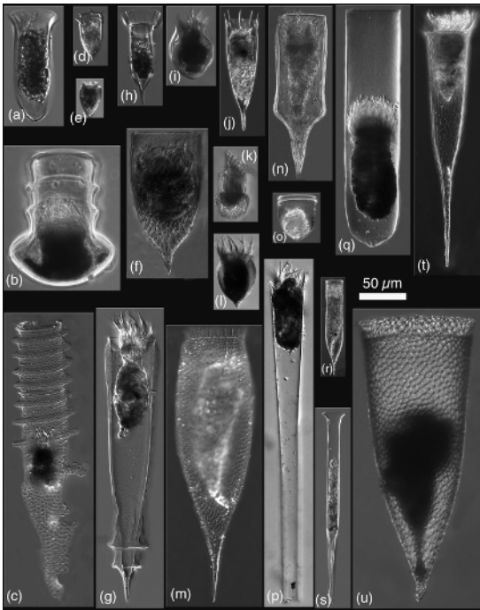
Fig. 1.5 Examples of tintinnid species with hyaline loricae: Amphorides quadrilineata (a), Amplectella collaria (b), Climacoctylis scalaria (c), Acanthostomella conicoides (d), Protorhabdonella simplex (e), Epiploctylis blanda (f), Xystonellopsis paradoxa (g), Ormosella trachelium (h), Proplectella elipisoida (i), Dadayella ganymedes (j), Dictyocysta lepida (k), Metacylis mediterranea (l), Parafavella parumdentata (m), Parundella messinensis (n), Ascampbellia tortulata (o), Eutintinnus stramentus (p), Undella hyalina (q), Helicostomella subulata (r), Salpingella acuminata (s), Rhabdonella spiralis (t), and Cyttarocylis cassis (u). All the specimens are Lugol's-fixed cells. For color version, see Plate 1.5.
