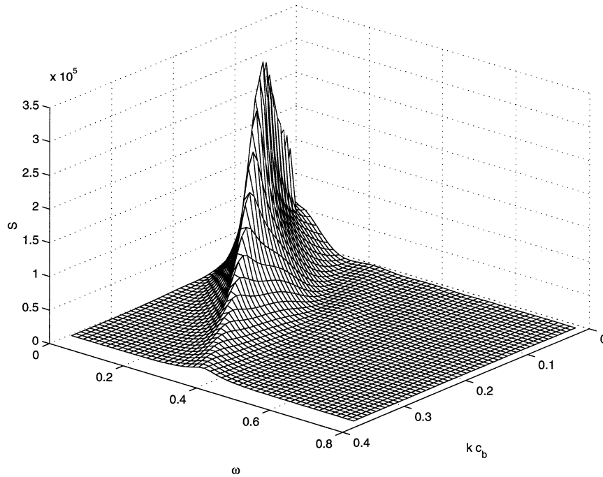
FIG. 3. Frequency–wavenumber spectrum S(k, x, \omega) for x = -3000 km and c_b = 2 cm s -1 . A peak is found for \omega_0 = c_b k_0 (and more generally along the line \omega = c_b k ).
