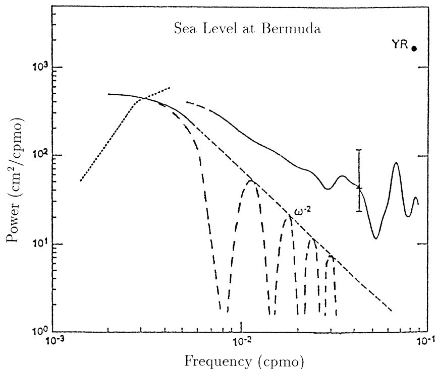
FIG. 1. Frequency spectrum of sea level at Bermuda (after Sturges and Hong 1995). Thick line: the full curve shows a calculation from the continuous portion of data beginning in 1944, smoothed by three Hanning passes (the 99% confidence interval is indicated), except for the last point (dashed); the dotted segment at low frequencies was obtained using gappy data extending back to 1932. The prediction by the linear stochastic model of FMZ for the low frequencies (continuous line) and the high frequency slope in \omega^{-2} (dashed line) are also indicated.
