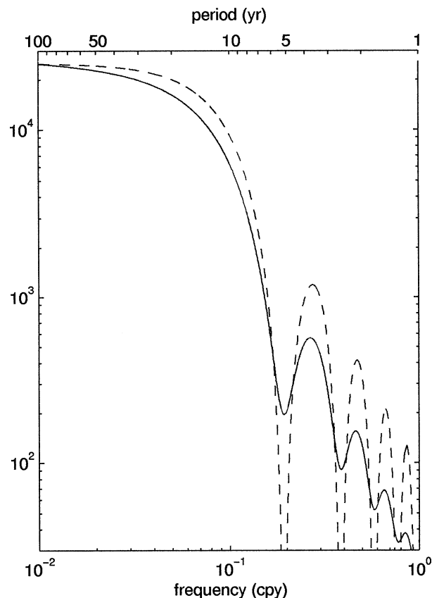
FIG. 2. Baroclinic pressure spectrum with (continuous curve) and without (dotted curve) dissipation at 3800 km from the eastern coast ( R_b = 34 km, \beta = 2 \times 10^{-11} m ^{-1} s ^{-1} , f_0 = 7 \times 10^{-5} s ^{-1} , S_0 = 4.8 \times 10^{-32} Pa ^2 m ^{-4} s ^{-2} /cpy).
