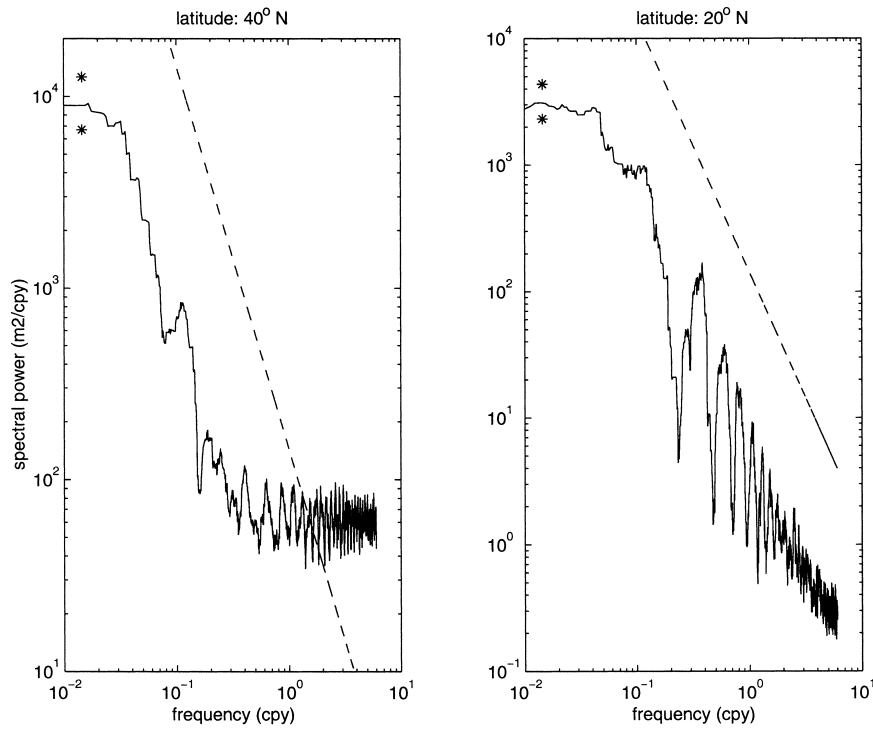
FIG. 10. Spectrum of thermocline depth fluctuations at 40°N (left) and at 20°N (right). The 99% confidence interval and the frequency slope in \omega^{-2} (dashed line) are indicated.
