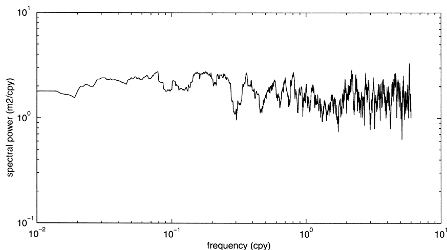
FIG. 9. Forcing spectrum used for the study of the nonlinear response of the ocean to a stochastic forcing.
