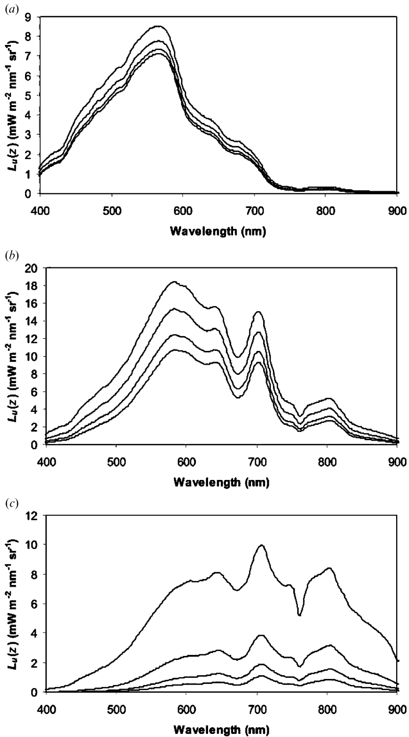
Figure 1. Examples of L_u spectra measured at different water depths (from top to bottom: 0.02, 0.10, 0.15 and 0.20 m). (a) 24 June 2003 at 10:50 U.T. ( TSMc = 7 \text{ mg l}^{-1} ). (b) 24 June 2003 at 14:25 U.T. ( TSMc = 45 \text{ mg l}^{-1} ). (c) 27 June 2003 at 14:18 U.T. ( TSMc = 303 \text{ mg l}^{-1} ).
