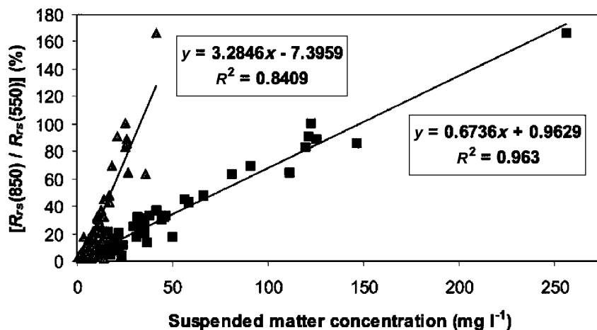
Figure 3. Ratio of reflectance, R_{rs}(850\text{ nm})/R_{rs}(550\text{ nm}) , plotted against ISM c (black squares) and OSM c (grey triangles). The corresponding equations and coefficients of determination of the linear regressions are indicated.
