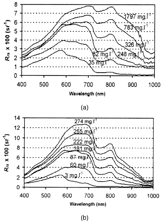
Fig. 3. Examples of typical in situ measured R_{rs} spectra carried out for different SPM concentrations in the Gironde Estuary in (a) 1996 and 1997 and then in (b) 1999.
