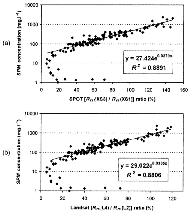
Fig. 9. Correspondence functions used to estimate SPM concentrations in the Gironde Estuary from reflectance ratios measurements in (a) SPOT bands [R_{rs}(XS3)/R_{rs}(XS1)] and (b) Landsat bands [R_{rs}(L4)/R_{rs}(L2)] . The best correlated function obtained for SPM concentration in the range (15–2500 \text{mg l}^{-1} ) is plotted on the graphs.
