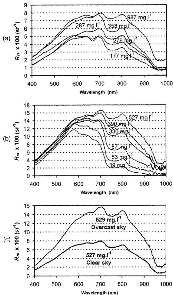
Fig. 4. Example of typical in situ measured R_{rs} spectra recorded in the Loire Estuary for different SPM concentrations: (a) on 28 February 2002 under a clear blue sky and (b) on 1 March 2002 under a thick overcast sky. (c) Comparison between R_{rs} spectra recorded at equivalent SPM concentrations under a clear sky (thick curve) and under an overcast sky (thin curve).
