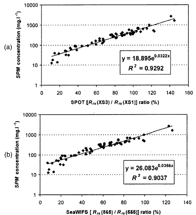
Fig. 10. Correspondence functions used to estimate SPM concentrations in the Loire Estuary from reflectance ratios measurements in (a) SPOT bands [R_{rs}(XS3)/R_{rs}(XS1)] and (b) SeaWiFS bands [R_{rs}(865)/R_{rs}(555)] . The best correlated function obtained for SPM concentration in the range [10–2600 \text{mg l}^{-1} ] is plotted on the graphs.
