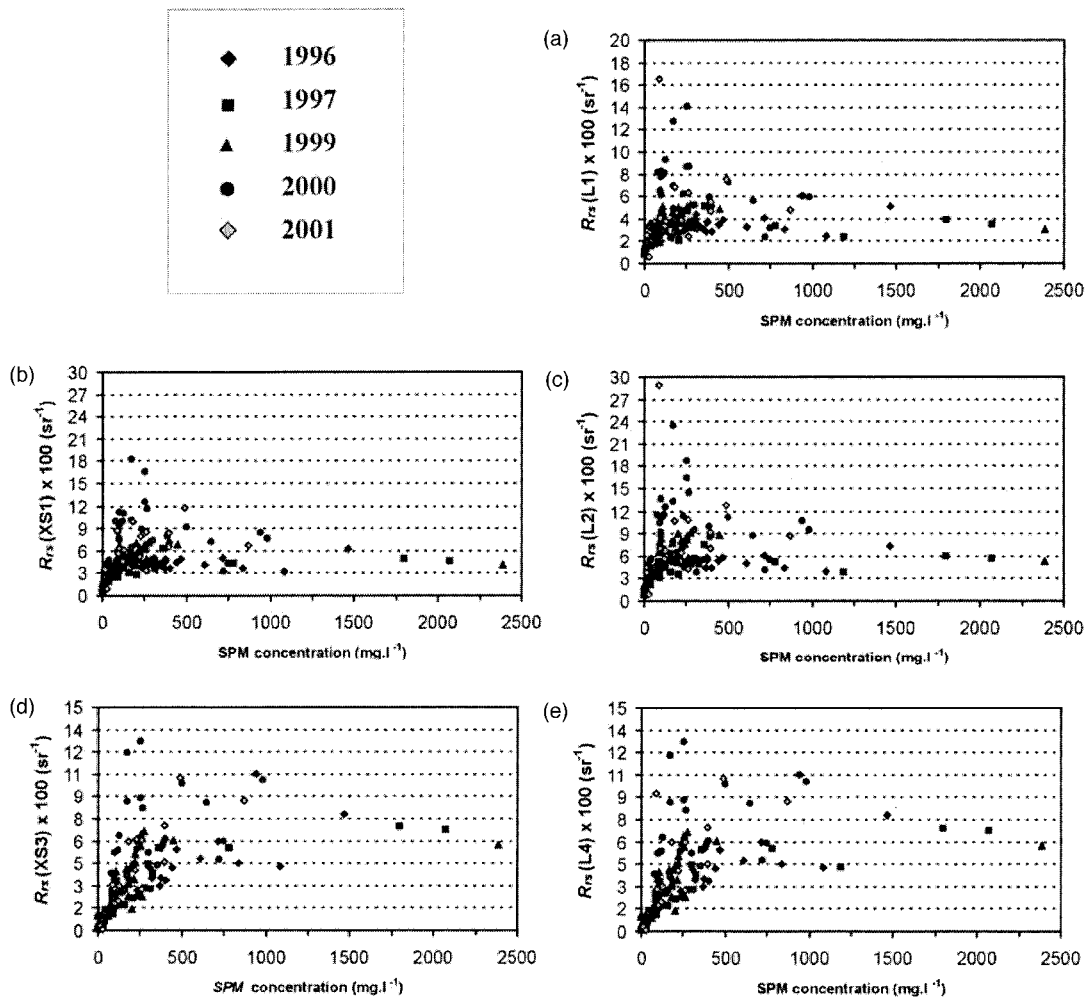
Fig. 5. Empirical relationships between R_{rsi} in (b) and (d) SPOT bands and in (a), (c), and (e) Landsat bands and SPM concentration established from all measurements carried out in the Gironde Estuary in 1996, 1997, 1999, 2000, and 2001.
