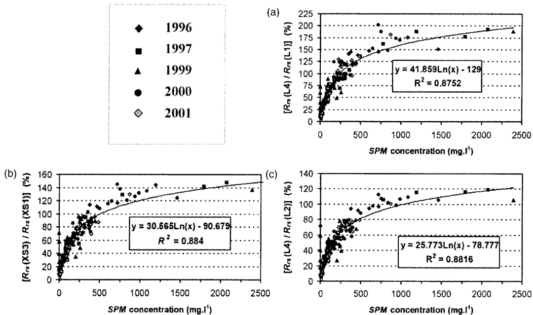
Fig. 7. Empirical relationships between reflectance ratios in (b) SPOT bands and in (a) and (c) Landsat bands and SPM, established from all field measurements carried out in the Gironde Estuary from 1996 to 2001. Plot of the logarithmic regression between 10 and 2500 \text{ mg l}^{-1} .
