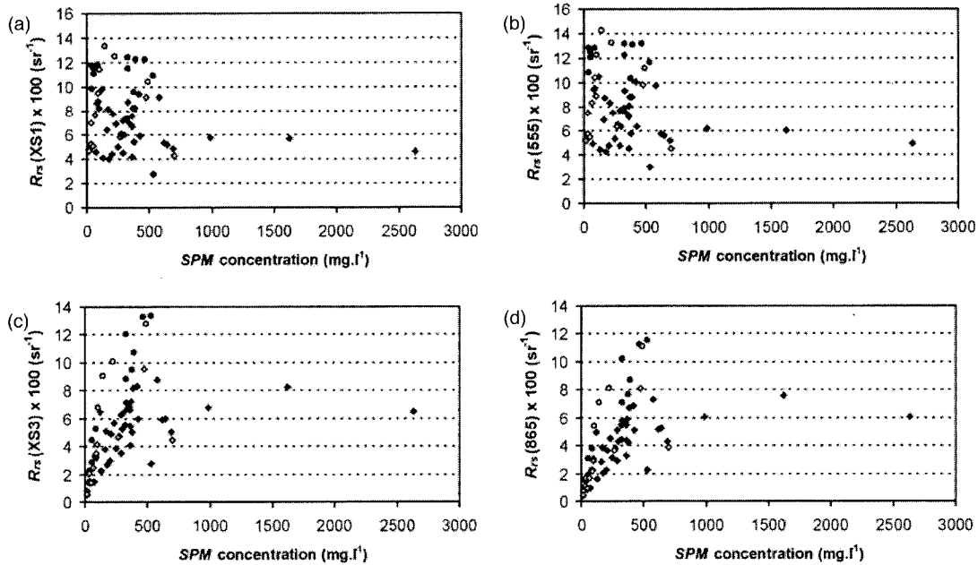
Fig. 6. Empirical relationships between R_{rsi} in (a) and (c) SPOT bands and in (b) and (d) SeaWiFS bands and SPM concentration established from measurements carried out in the Loire Estuary in February and March 2002 (black points) and in April 2002 (gray points), under a clear blue sky (diamonds) and under a thick overcast sky (circles).
