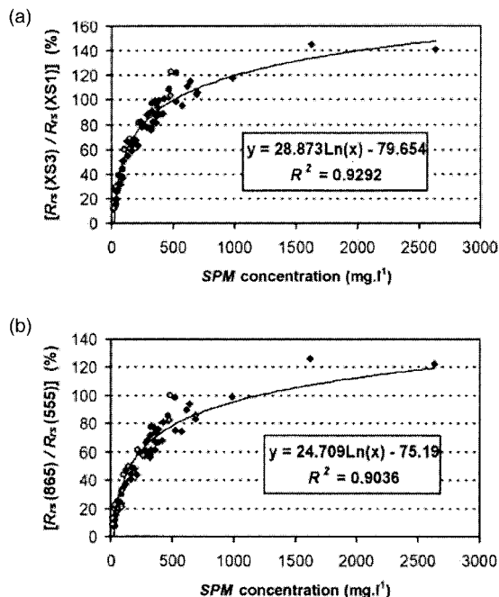
Fig. 8. Empirical relationships between reflectance ratios in (a) SPOT bands and in (b) SeaWiFS bands and SPM concentration, established from field measurements carried out in 2002 in the Loire Estuary in February and March 2002 (black points) and in April 2002 (gray points), under a clear blue sky (diamonds) and under a thick overcast sky (circles).
