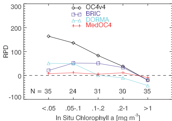
Fig. 5. Relative Percentage Difference (RPD) for all the four examined algorithms as a function of in situ chlorophyll in five different ranges. Numbers within the plot indicate the number of data points used to retrieve RPD in each range.
