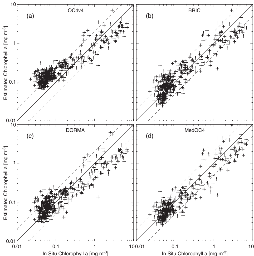
Fig. 7. Validation of SeaWiFS chlorophyll a estimates against concurrent in situ chlorophyll a data ( C_M ). (a) SeaWiFS estimates are obtained applying the OC4v4 algorithm. (b) SeaWiFS estimates are obtained applying the BRIC algorithm. (c) SeaWiFS estimates are obtained applying the DORMA algorithm. (d) SeaWiFS estimates are obtained applying the MedOC4 algorithm. The 1:1 (continuous line) 1:2 (bottom dashed line) and the 2:1 (top dashed line) lines are also plotted.
