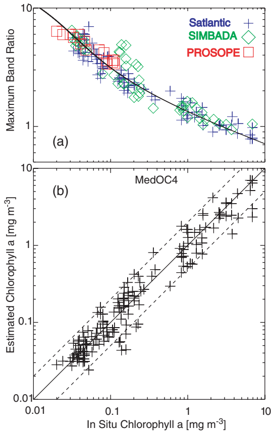
Fig. 4. (a) Relation between in situ MBR and C_M used to derive the new coefficients for the MedOC4 algorithm. Different optical data sources are highlighted with different colours and symbols. MedOC4 functional form is superimposed. (b) MedOC4-derived chlorophyll versus C_M . The 1:1 (continuous line) 1:2 (bottom dashed line) and the 2:1 (top dashed line) lines are also plotted.
