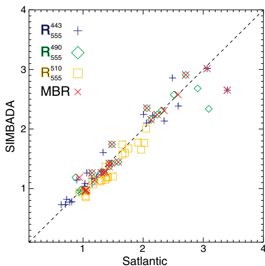
Fig. 2. Scatter plot of SIMBADA versus Satlantic Rrs ratios. R_{555}^{443} in blue, R_{555}^{490} in green, R_{555}^{510} in orange and MBR red.
