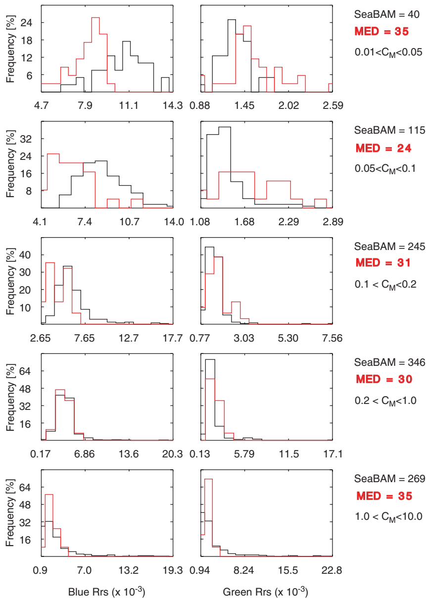
Fig. 10. Normalized frequency histograms of the Rrs for the Mediterranean (red) and SeaBAM global datasets (black) for five different chlorophyll ranges. Left panels indicate the maximum value among Rrs(443), Rrs(490) and Rrs(510) (i.e., the numerator of MBR). Right panels indicate Rrs(555) (i.e., the denominator). Chlorophyll a ranges are indicated on the right hand side of each row along with the number of points used for each of the two datasets.
