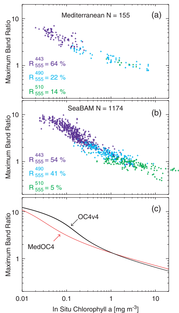
Fig. 9. Intercomparison between Mediterranean and global (SeaBAM) in situ bio-optical measurements. (a) Relationship between in situ MBR and C_M for the Mediterranean dataset (this work, Table 1) (b) Relationship between in situ MBR and C_M for the global SeaBAM dataset. Blue crosses indicate that MBR corresponds to R_{555}^{443} ; light blue crosses indicate that MBR corresponds to R_{555}^{490} ; green crosses indicate that MBR corresponds to R_{555}^{510} . The percent number of times in which the three R_{555}^2 correspond to MBR are also superimposed. (c) The two best lines fitting the Mediterranean and SeaBAM datasets are plotted: MedOC4 (red) and OC4v4 (black). SeaBAM dataset archive is available on the Internet at http://seabass.gsfc.nasa.gov/seabam/pub/maritorea_oreilly_schieber/seabam919.txt web page.
