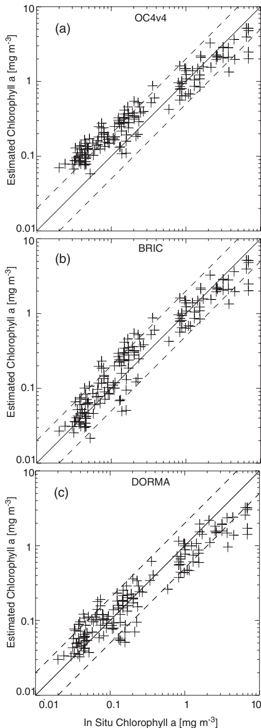
Fig. 3. Scatter plot of algorithm derived chlorophyll concentration from in situ optical data versus in situ chlorophyll ( C_M ). (a) The estimated chlorophyll is obtained using OC4v4 algorithm. (b) The estimated chlorophyll is obtained using BRIC algorithm. (c) The estimated chlorophyll is obtained using DORMA algorithm. The 1:1 (continuous line) 1:2 (bottom dashed line) and the 2:1 (top dashed line) lines are also plotted.
