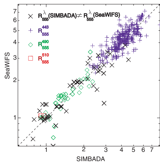
Fig. 6. Scatter plot of space-time co-located MBRs from SIMBADA and SeaWiFS. Different symbols represent different band ratio selections: blue crosses refer to R_{555}^{443} , green diamonds refer to R_{555}^{490} and red squares refer to R_{555}^{510} . Black "x"s" refer to points where MBRs selected by SIMBADA are different from those selected by SeaWiFS.
