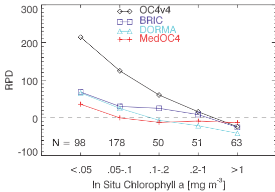
Fig. 8. Relative Percentage Difference (RPD) between SeaWiFS-derived chlorophyll and co-located in situ C_M for all the four algorithms and for five chlorophyll ranges. Numbers within the plot indicate the number of data points used to retrieve RPD in each range.
