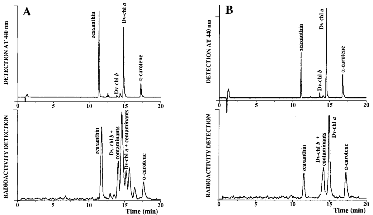
Fig. 2. Examples of HPLC chromatograms: upper panels, detection at 440 nm; lower panels, radioactivity detection. (A) Non-purified extract; (B) purified and acidified extracts; (C) purified and acidified extracts
