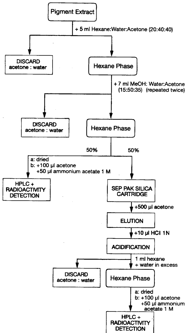
Fig. 1. Purification protocol of labelled pigments from labelled lipid contaminants
