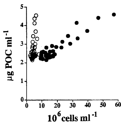
Fig. 5. Relationship between particulate organic carbon, (●) Prochlorococcus and (○) heterotrophic bacteria densities for the 4 cultures of Prochlorococcus CCMP 1378
