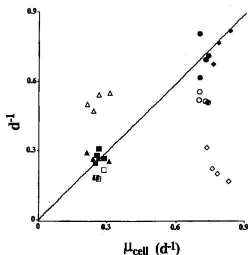
Fig. 7. Comparison of Prochlorococcus growth rate estimated after 24 h of incubation from variations in cell density ( \mu_{cell} ) with zeaxanthin and Dv-chl a synthesis rates as calculated from ^{14}C zeaxanthin and Dv-chl a labelling in LL ( 7 \mu\text{mol quanta m}^{-2} \text{s}^{-1} ), in HH ( 56 \mu\text{mol quanta m}^{-2} \text{s}^{-1} ), in LH ( 7 to 56 \mu\text{mol quanta m}^{-2} \text{s}^{-1} ) and in HL ( 56 to 7 \mu\text{mol quanta m}^{-2} \text{s}^{-1} ) light experiments. In LL: (■) \mu_{zeaP} ; (□) \mu_{dvaP} ; in HH: (●) \mu_{zeaP} ; (○) \mu_{dvaP} ; in LH: (◆) \mu_{zeaP} ; (◇) \mu_{dvaP} ; and in HL: (▲) \mu_{zeaFP} ; (△) \mu_{dvaFP}
