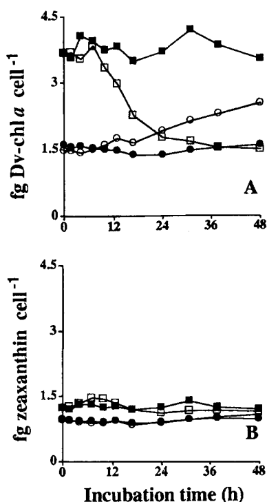
Fig. 4. (A) Dv-chl a and (B) zeaxanthin cellular content in Prochlorococcus . (●) Constant high light (HH: 56 \mu\text{mol quanta m}^{-2} \text{s}^{-1} ); (■) constant low light (LL: 7 \mu\text{mol quanta m}^{-2} \text{s}^{-1} ); (○) high to low light shift (HL: 56 to 7 \mu\text{mol quanta m}^{-2} \text{s}^{-1} ); (□) low to high light shift (LH: 7 to 56 \mu\text{mol quanta m}^{-2} \text{s}^{-1} )
