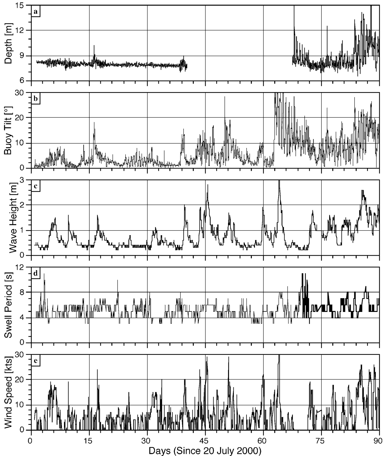
Fig. 9. The results of the qualification deployment (20 July to 20 October 2000), showing the time series of a) the depth of the buoy CTD (nominally at 8.3 m when the buoy is motionless and the sea surface perfectly flat), b) the buoy tilt, c) the swell height (the one-third most significant waves), d) the swell period, and e) the wind speed.
