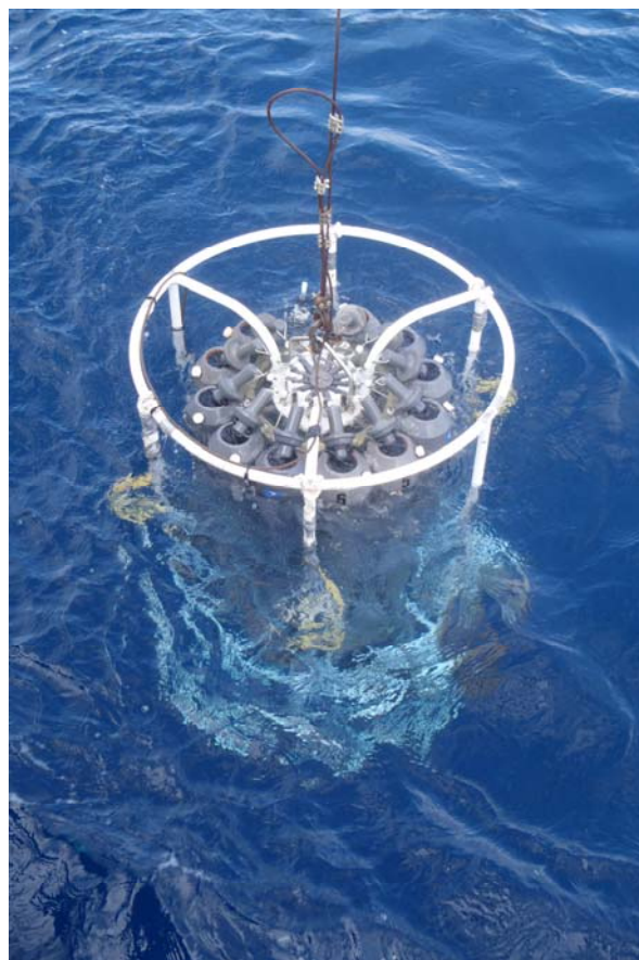
The start of a CTD cast with water sampling from the Tethys-II R/V stern
