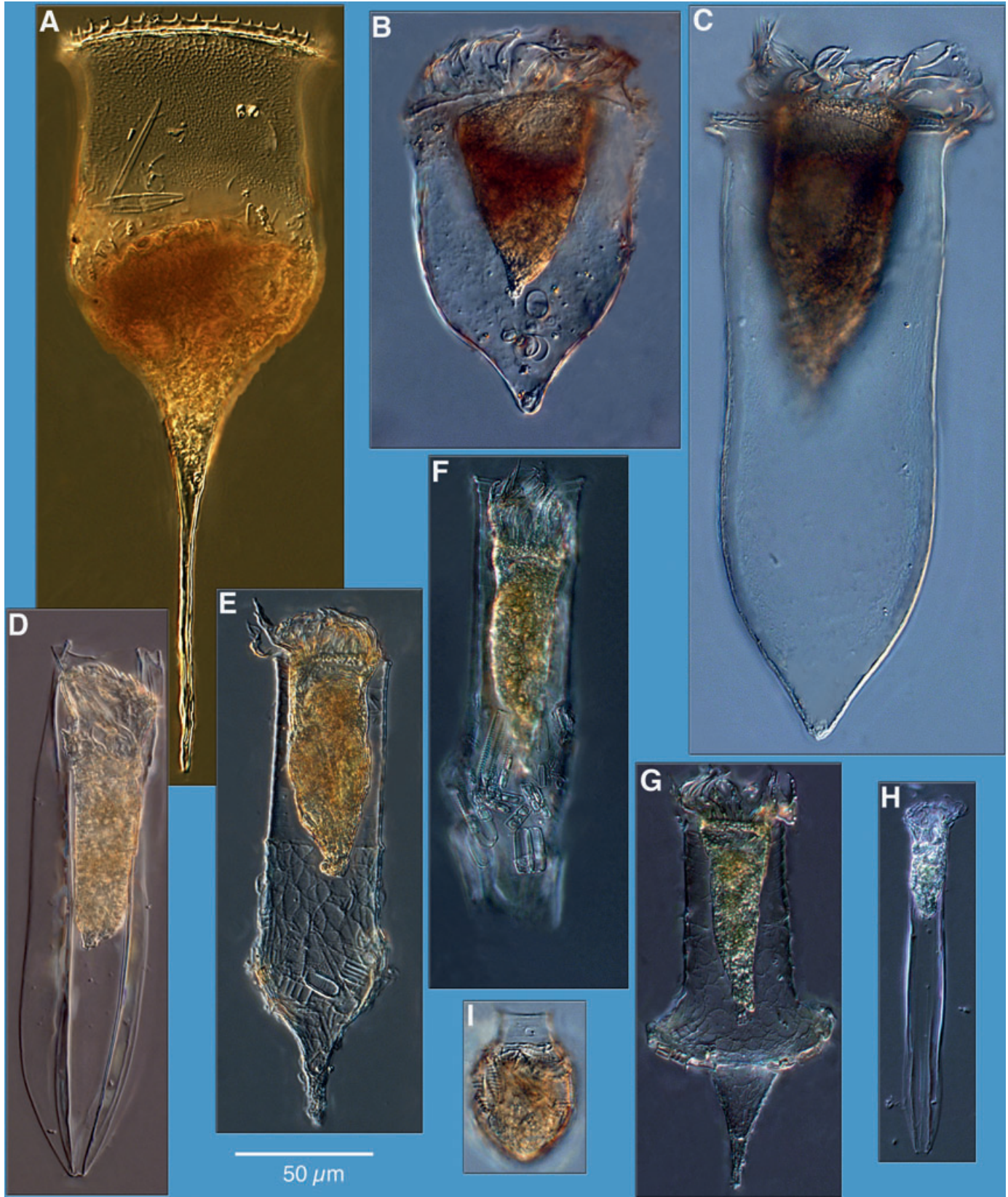
Fig. 1. Examples of tintinnid species or morphotypes commonly reported from the Southern Ocean. All are Bouin's-fixed specimens from the Amundsen Sea. (A) Cymatocyclus calcyformis , (B) Cymatocyclus convallaria-affinis , (C) Cymatocyclus drygalski , (D) Amphorellopsis quinquealata , (E) Condonellopsis gaussi f. cylindrica , (F) Laackmanniella prolongata , (G) Condonellopsis gaussi , (H) Salpingella faurei , (I) Condonellopsis pusilla . All but Salpingella faurei and Condonellopsis pusilla are forms found only in the Southern Ocean.
