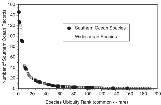
Fig. 6. Species ubiquity rank graph. The number of sites from which each species has been recorded defines its ubiquity. The species are then ordered by ubiquity, from most common to rare, and each plotted against the number of records for the species. Note that both Southern Ocean endemic species and widespread species are among the most and least common forms reported.
